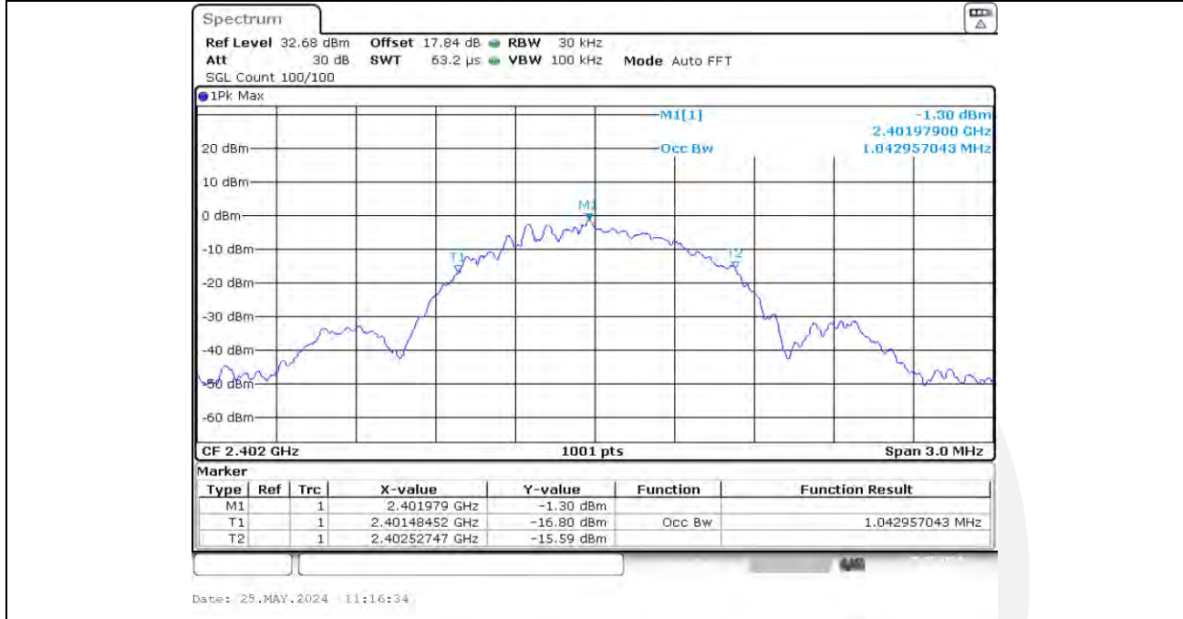
99%_Occupied_Bandwidth_NVNT_ANT1_1Mbps_2402
