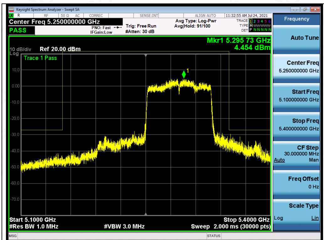
Test_Graph_802.11ac80_ANT1_5290_MCS9_Frequency Band 3
