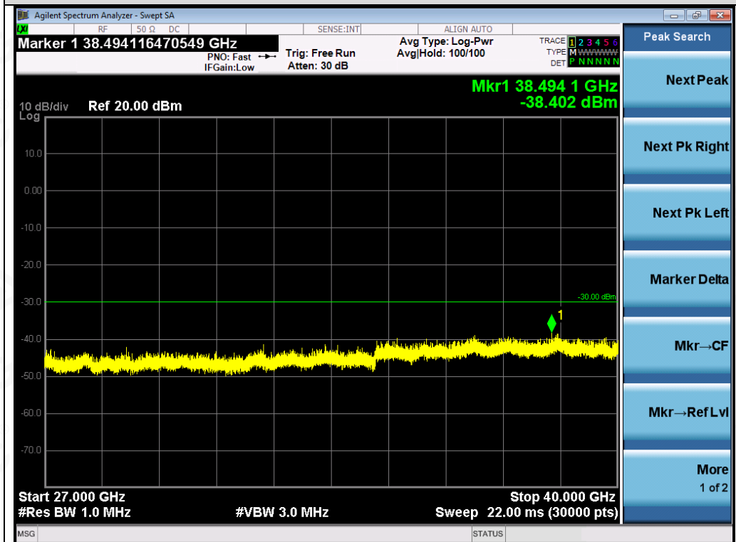
Test_Graph_802.11a_ANT1_5700_6Mbps_Frequency Band 5
