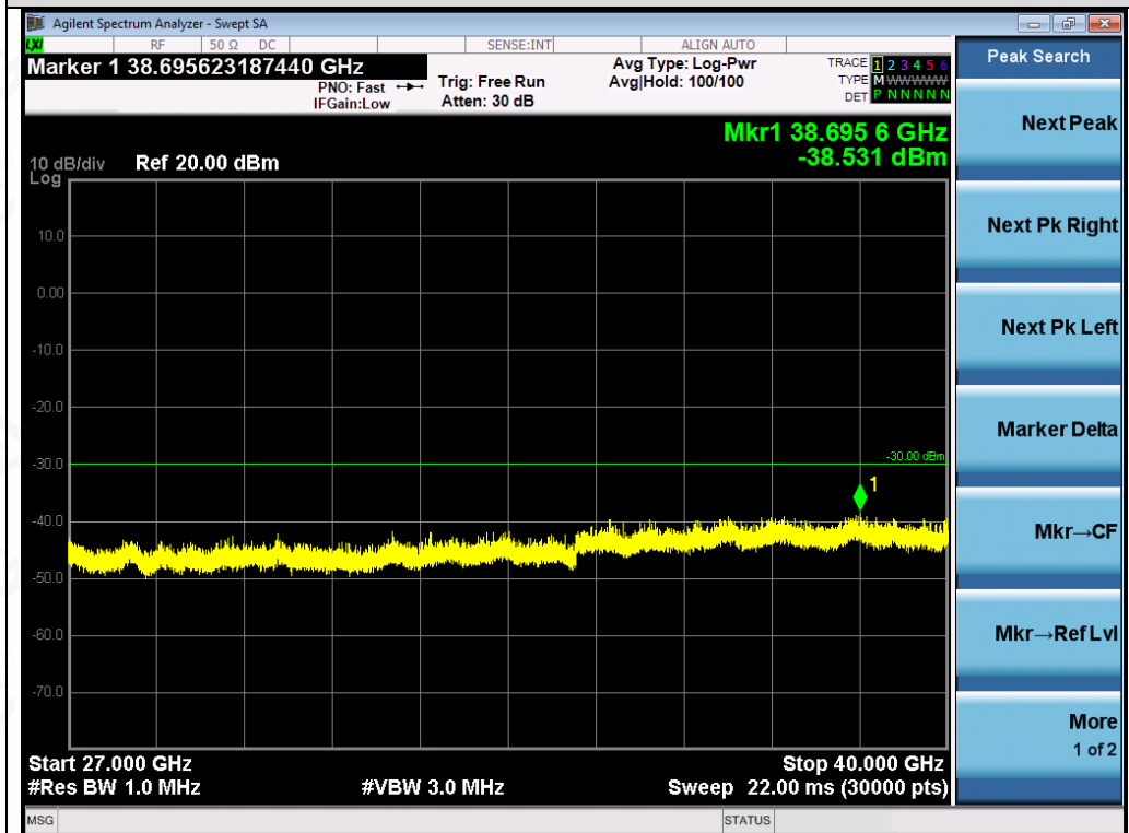
Test_Graph_802.11n40_ANT1_5590_MCS0_Frequency Band 5
