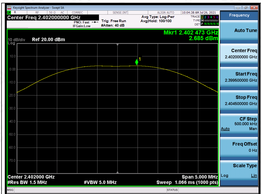
Test_Graph_LE2M_ANT1_2402_2Mbps_Peak Power
