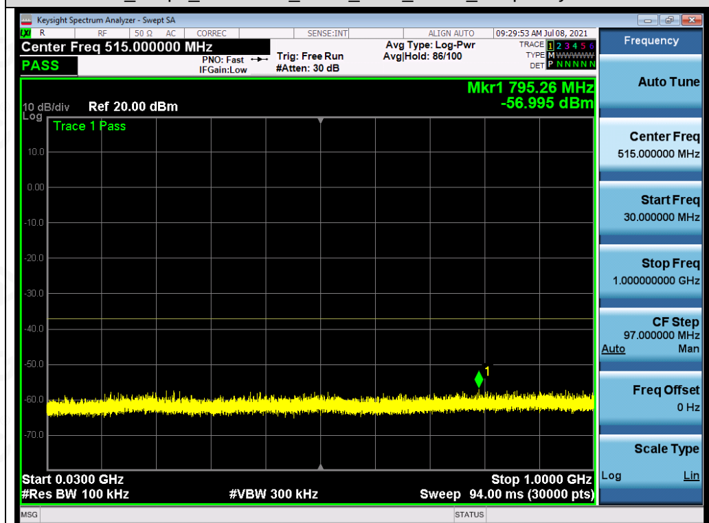
Test Graph 802.11ac80 ANT1 5530 MCS9 Frequency Band 1
