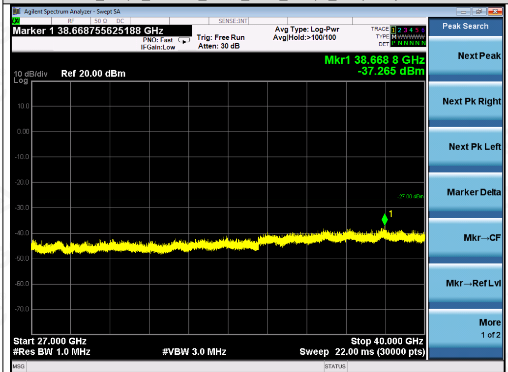
Test_Graph_802.11a_ANT1_5825_6Mbps_Frequency Band5
