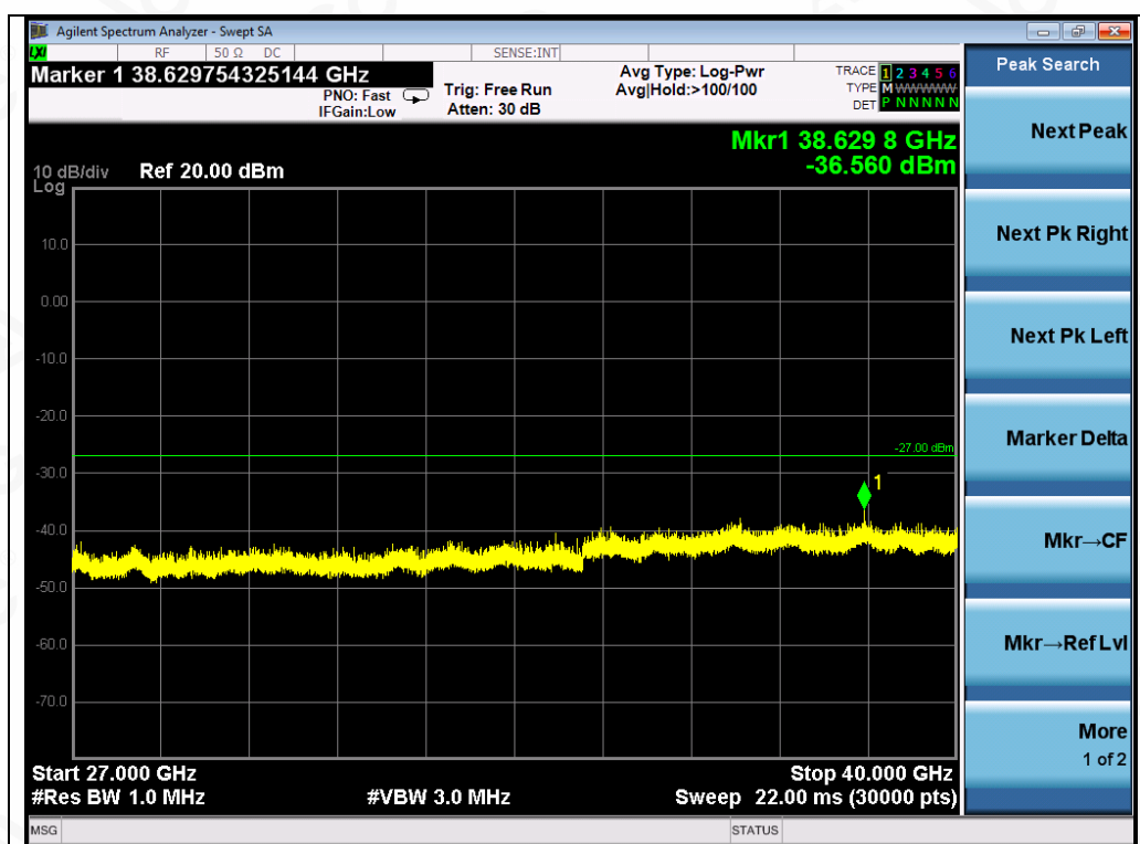
Test Graph 802.11n40 ANT1 5670 MCS0 Frequency Band 5
