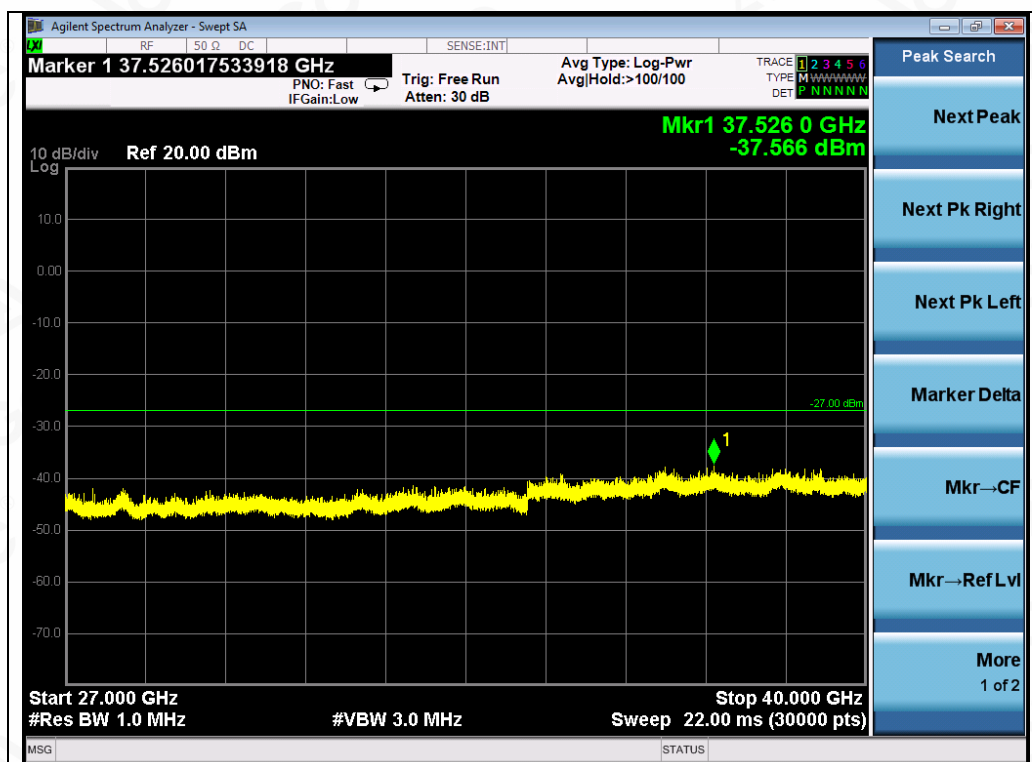
Test Graph 802.11n40 ANT1 5510 MCS0 Frequency Band 5
