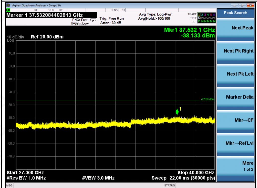
Test_Graph_802.11n40_ANT1_5590_MCS0_Frequency Band 5
