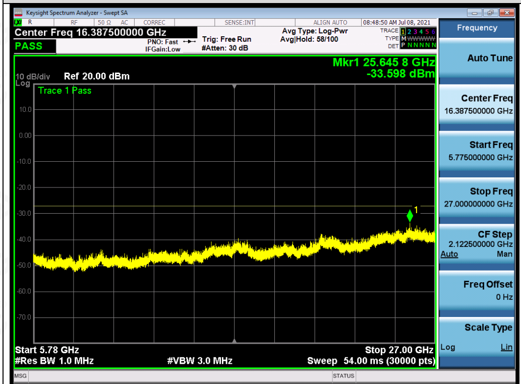
Test_Graph_802.11a_ANT1_5500_6Mbps_Frequency Band 4
