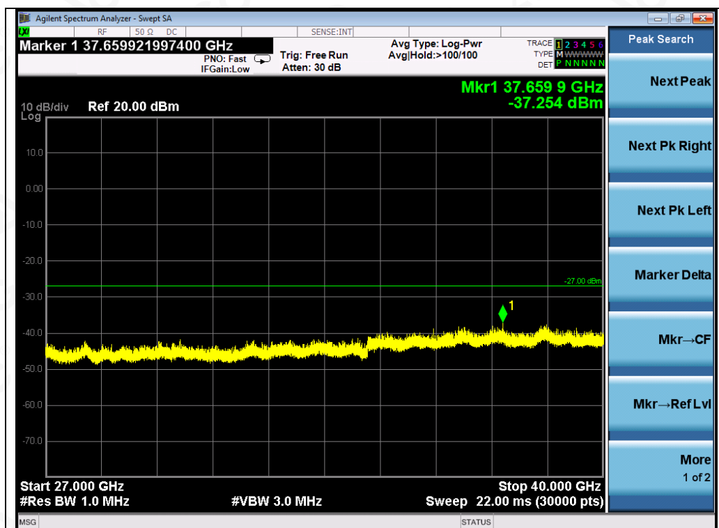
Test Graph 802.11a ANT1 5745 6Mbps Frequency Band5
