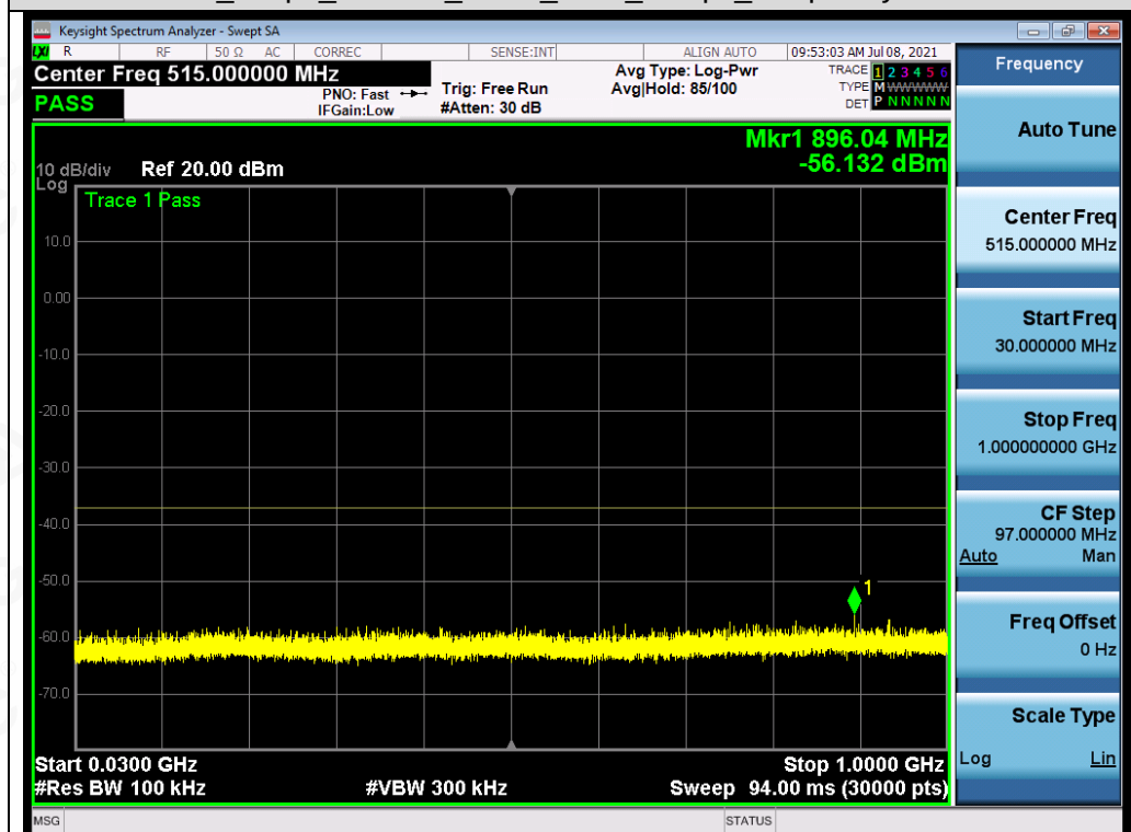
Test Graph 802.11a ANT1 5825 6Mbps Frequency Band1
