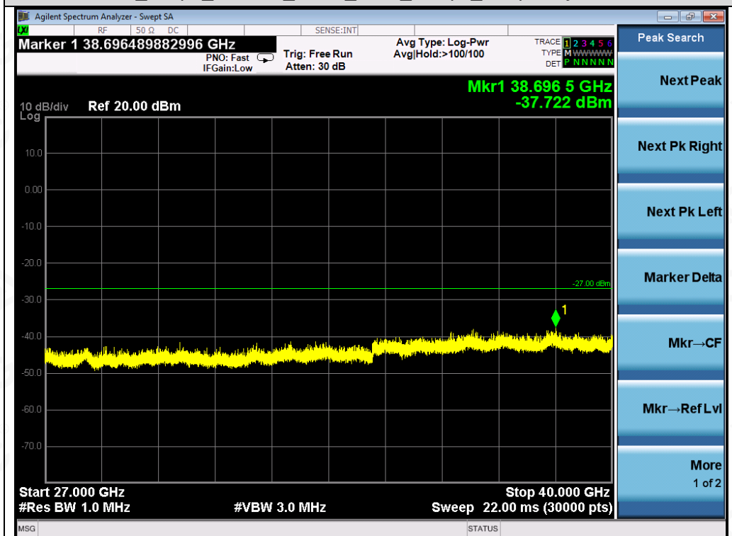
Test_Graph_802.11a_ANT1_5700_6Mbps_Frequency Band 5
