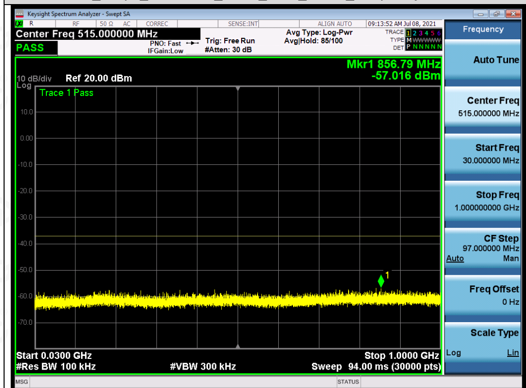
Test Graph 802.11n40 ANT1 5590 MCS0 Frequency Band 1
