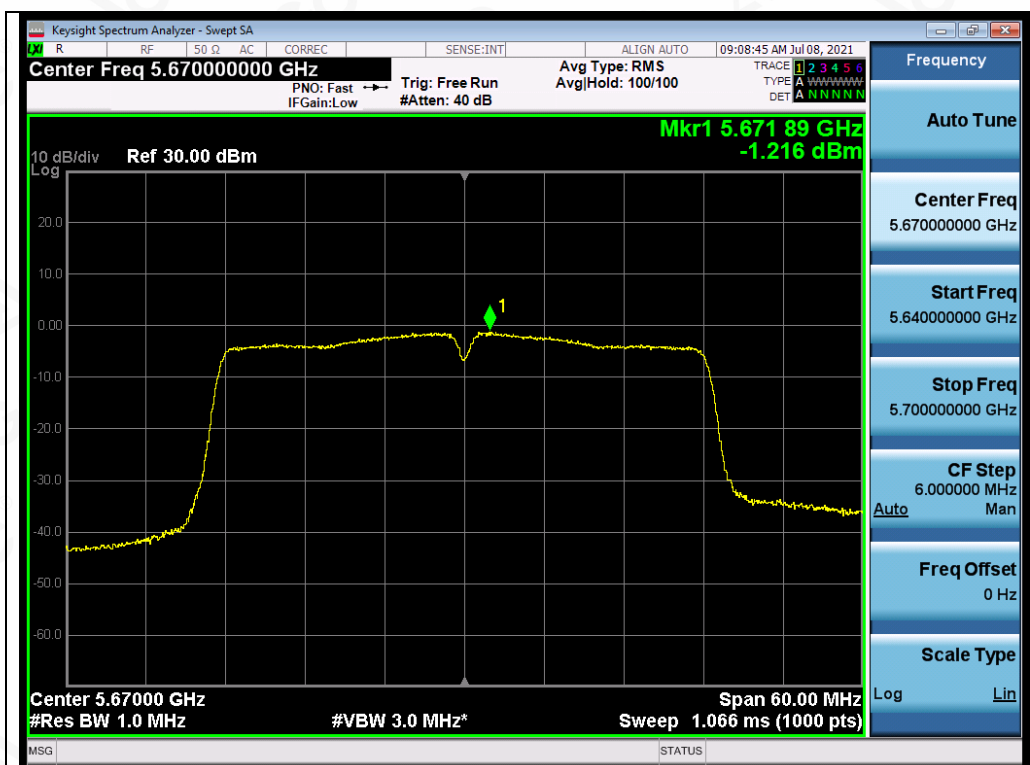
Test Graph 802.11n40 ANT1 5670 MCS0 PSD
