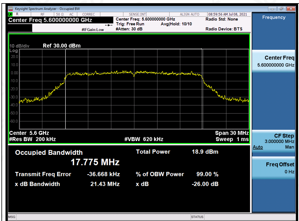
Test_Graph_802.11n20_ANT1_5600_MCS0_OBW
