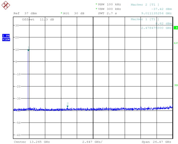
Plot 26. DH3 2480MHz, 30MHz-26.5GHz Spurious
