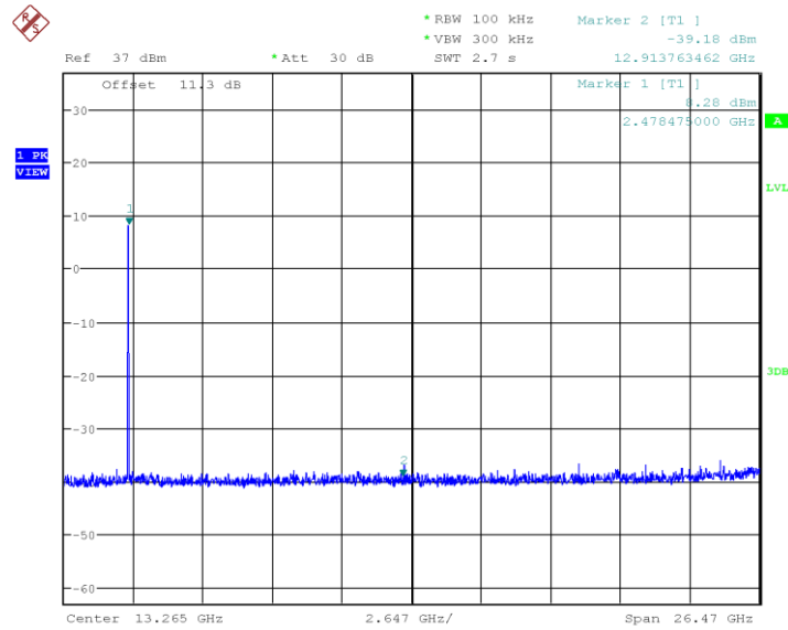
Plot 25. DH1 2480MHz, 30MHz-26.5GHz Spurious
