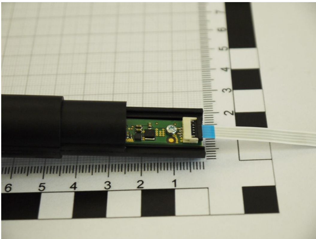
Photograph 8: Measurement Unit top side
