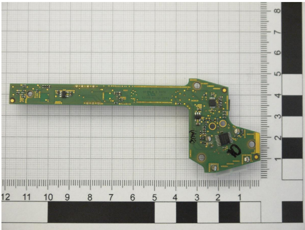
Photograph 16: PCB 3 rear side view
