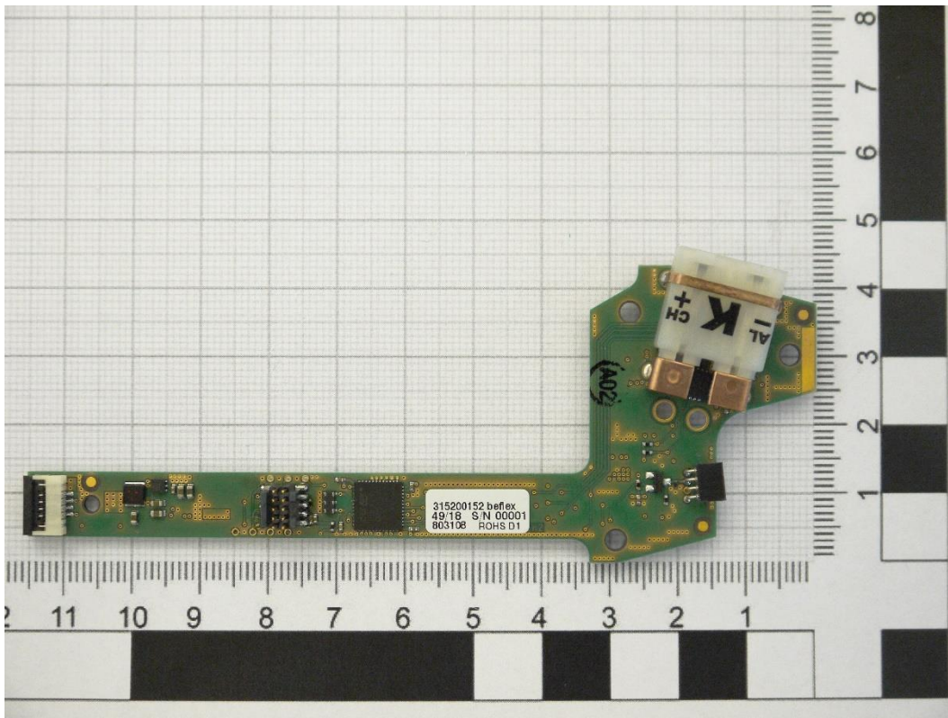
Photograph 15: PCB 3 front side view
