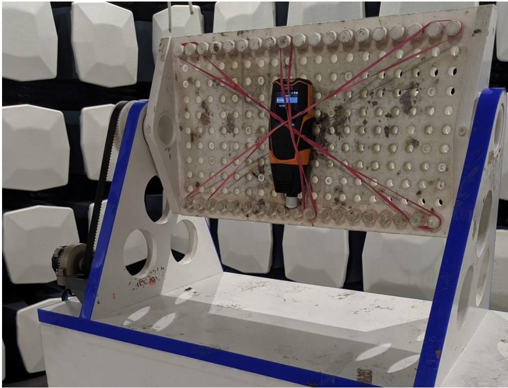
Photograph 5: Close View above 1GHz- EUT Standing
