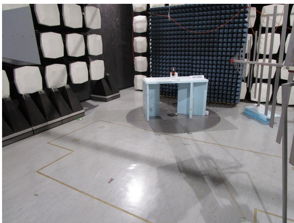
Photograph 4: Under 1GHz - Overall View EUT Standing
