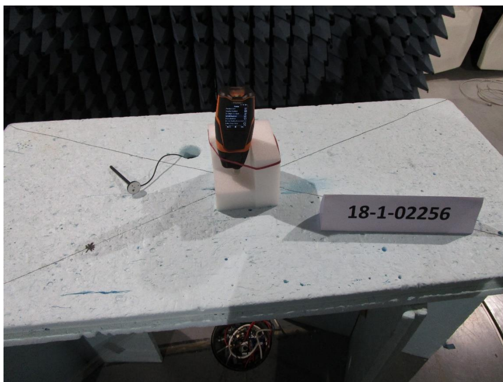
Photograph 1: H-Field - Close View EUT Standing
