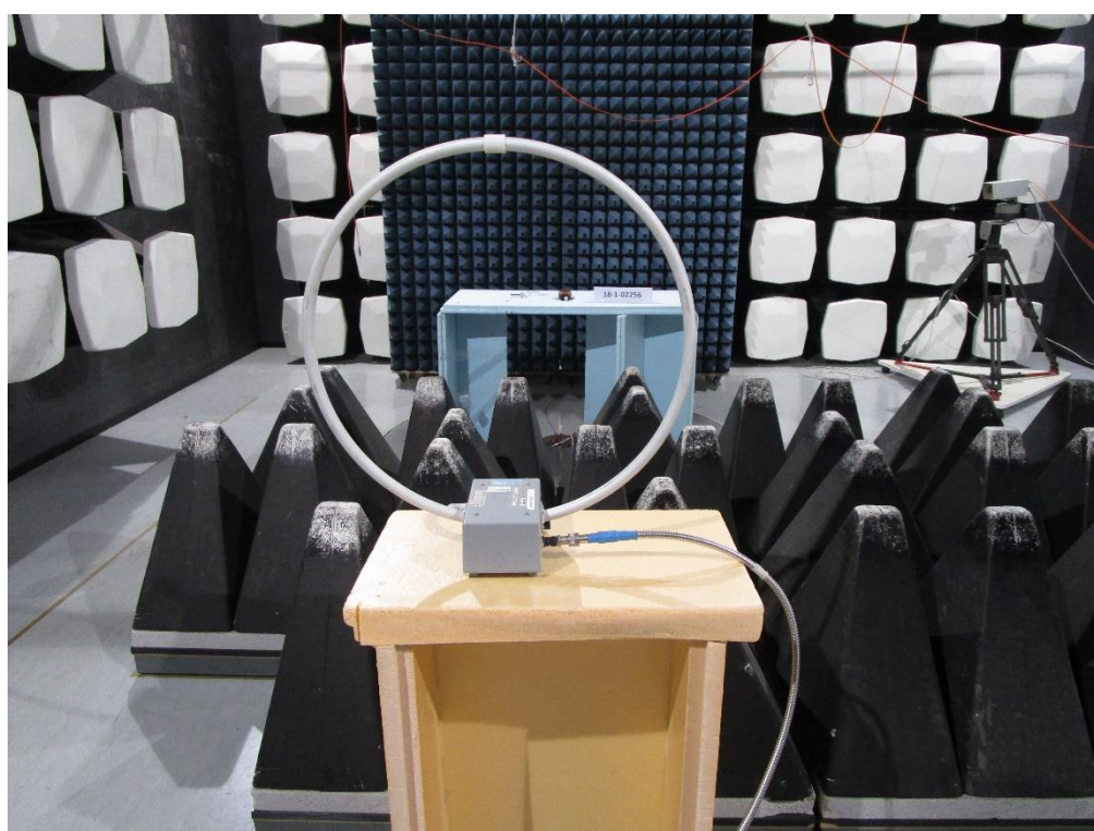
Photograph 2: H-Field - Overall View EUT Standing
