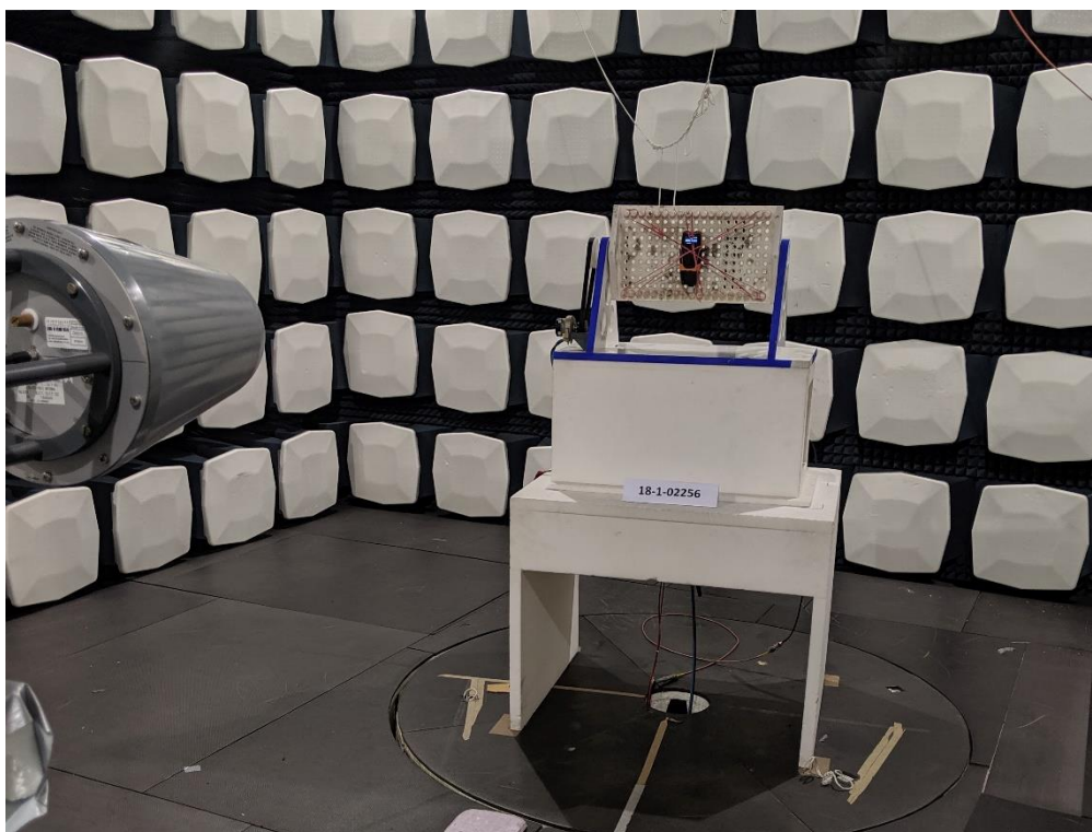
Photograph 6: Overall View above 1 GHz - EUT Standing
