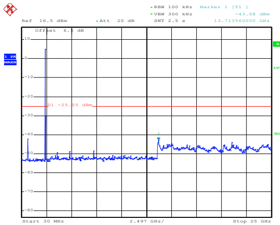
Test mode: 802.11b Lowest channel
