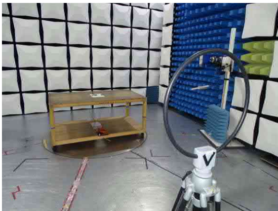
Photo 2: Test setup for radiated measurements (semi anechoic chamber, CFR 47 Part 15, Subpart C, H-Field)
