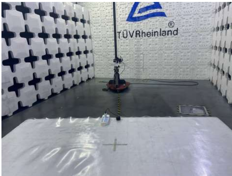
Photograph 4: Set-up photo for Radiated Emission, Below 1GHz
