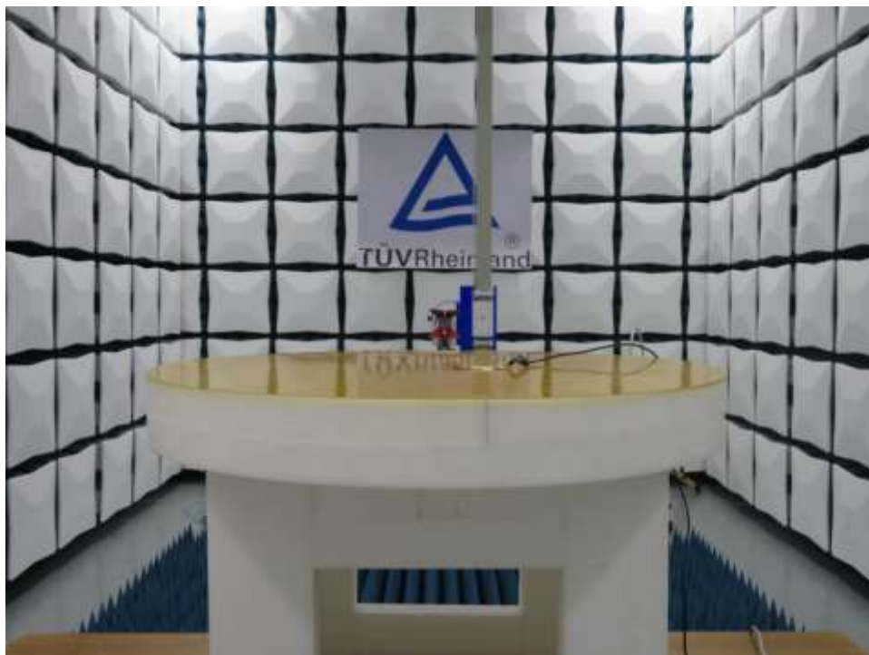
Photograph 2: Set-up photo for Radiated Emissions Above 1GHz
