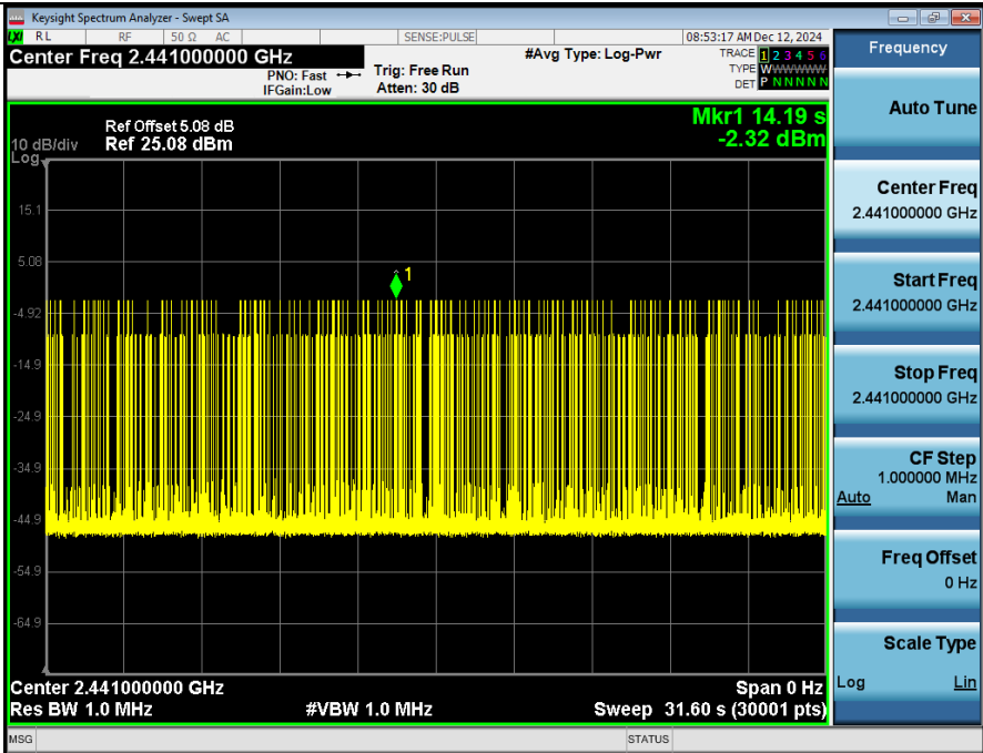
Dwell_Time_(Hopping)_NVNT_ANT1_2-DH3_2441_00_Accumulated
