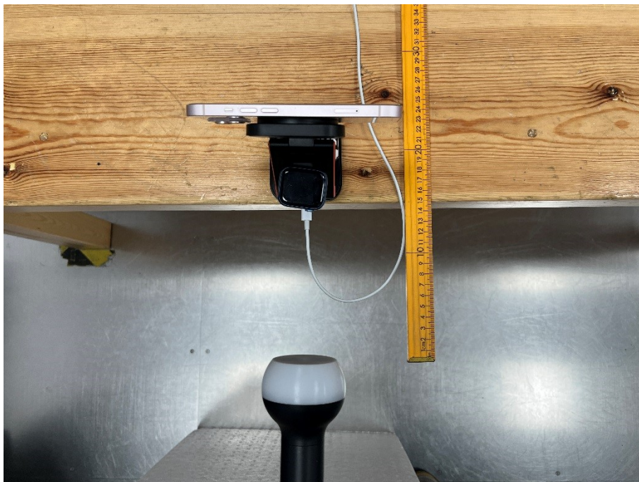
Photograph 1: Set-up photo for RF exposure
