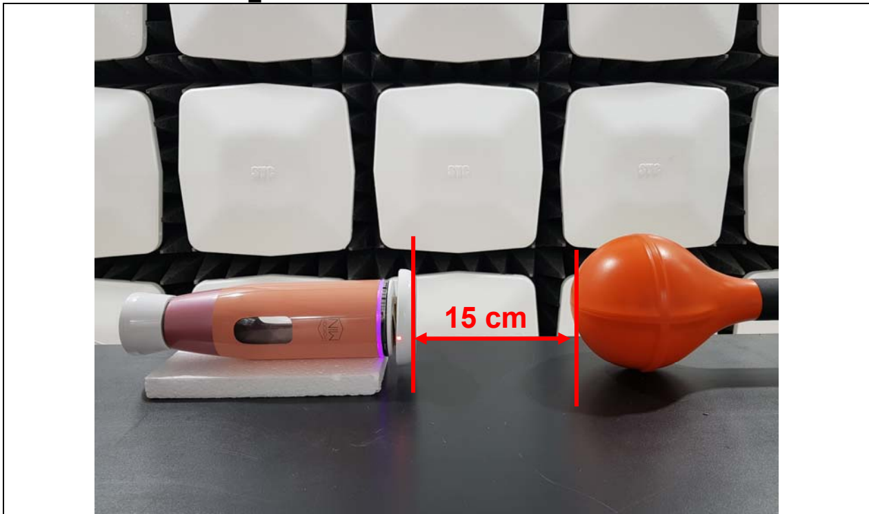
H-field Measurements _ Distance : 15 cm
