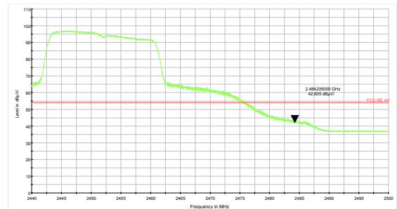
802.11n HT20 -Channel 9 Average
