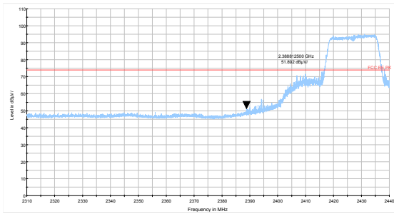
802.11n HT20 -Channel 4 Peak
