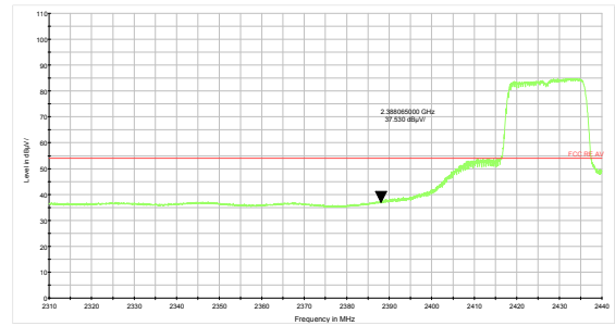
802.11n HT20 -Channel 4 Average
