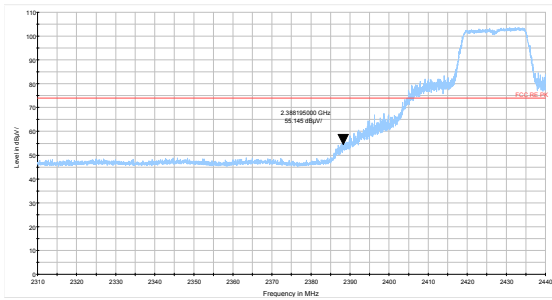
802.11g-Channel 4 Peak
