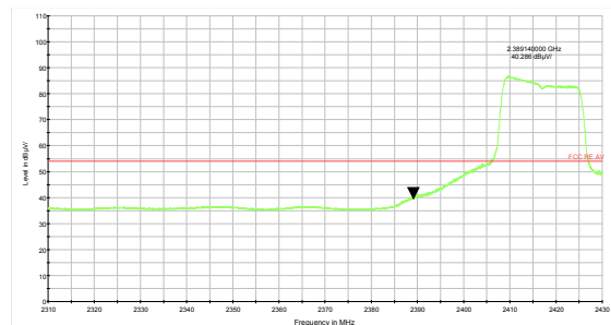
802.11g-Channel 2 Average
