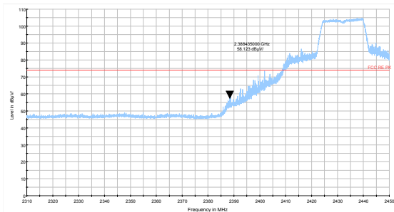
802.11g-Channel 5 Peak
