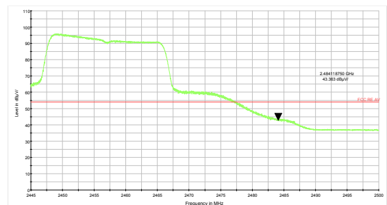
802.11n HT20 -Channel 10 Average
