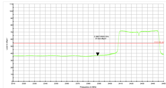
802.11n HT40 -Channel 4 Average
