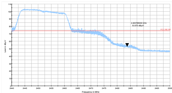
802.11n HT20 -Channel 9 Peak
