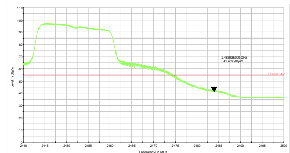
802.11g-Channel 9 Average
