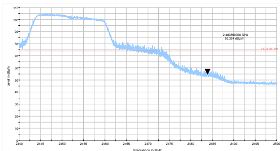
802.11g-Channel 9 Peak
