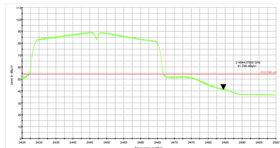
802.11n HT40 -Channel 8 Average
