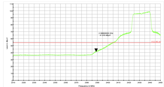
802.11g-Channel 5 Average
