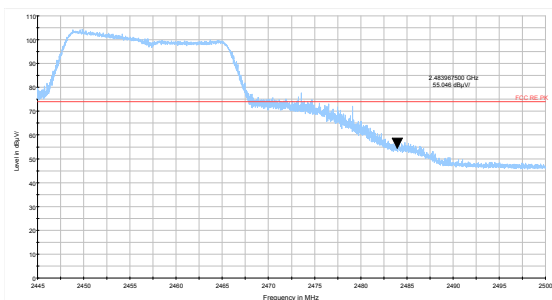
802.11n HT20 -Channel 10 Peak
