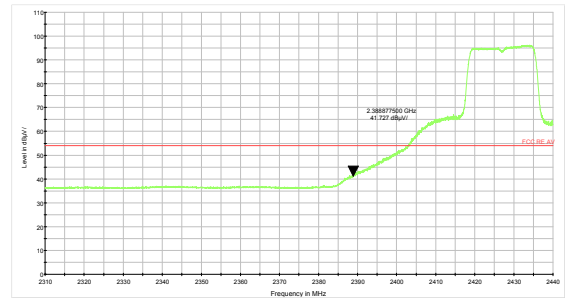
802.11g-Channel 4 Average
