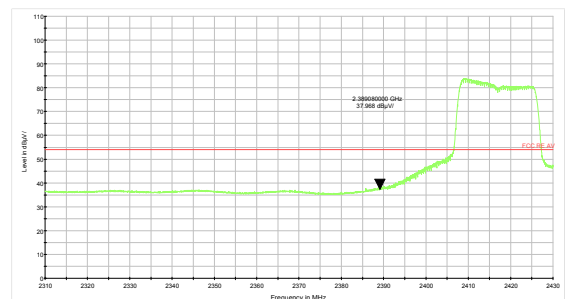
802.11n HT20 -Channel 2 Average
