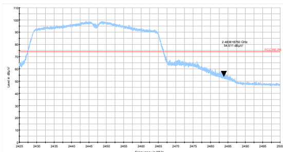
802.11n HT40 -Channel 8 Peak
