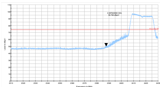
802.11n HT20 -Channel 2 Peak
