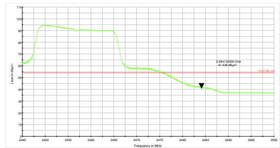
802.11g-Channel 10 Average
