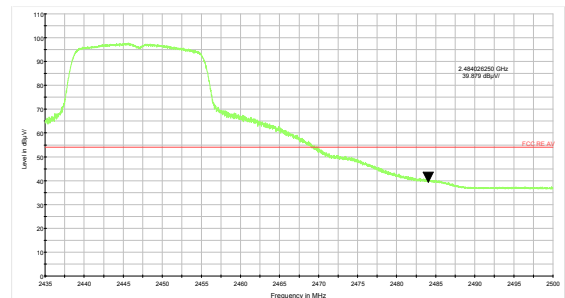
802.11g-Channel 8 Average
