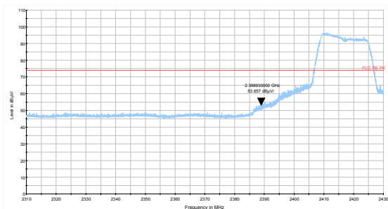
802.11g-Channel 2 Peak
