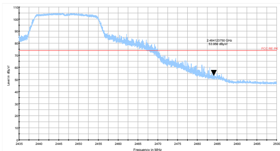
802.11g-Channel 8 Peak
