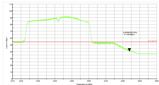
802.11n HT40 -Channel 7 Average
