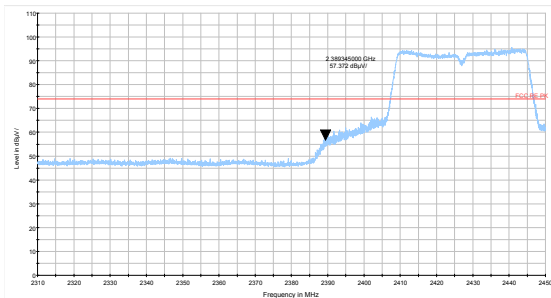
802.11n HT40 -Channel 4 Peak
