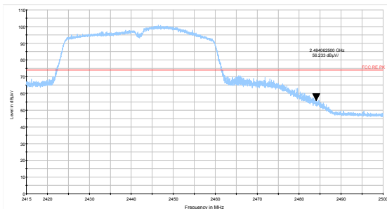
802.11n HT40 -Channel 7 Peak
