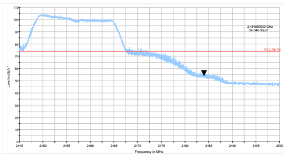
802.11g-Channel 10 Peak
