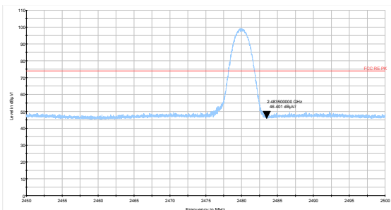
3DH5-Channel 78: Peak
