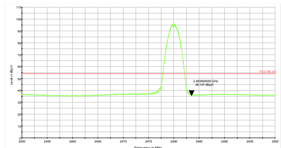
3DH5-Channel 78: Average
