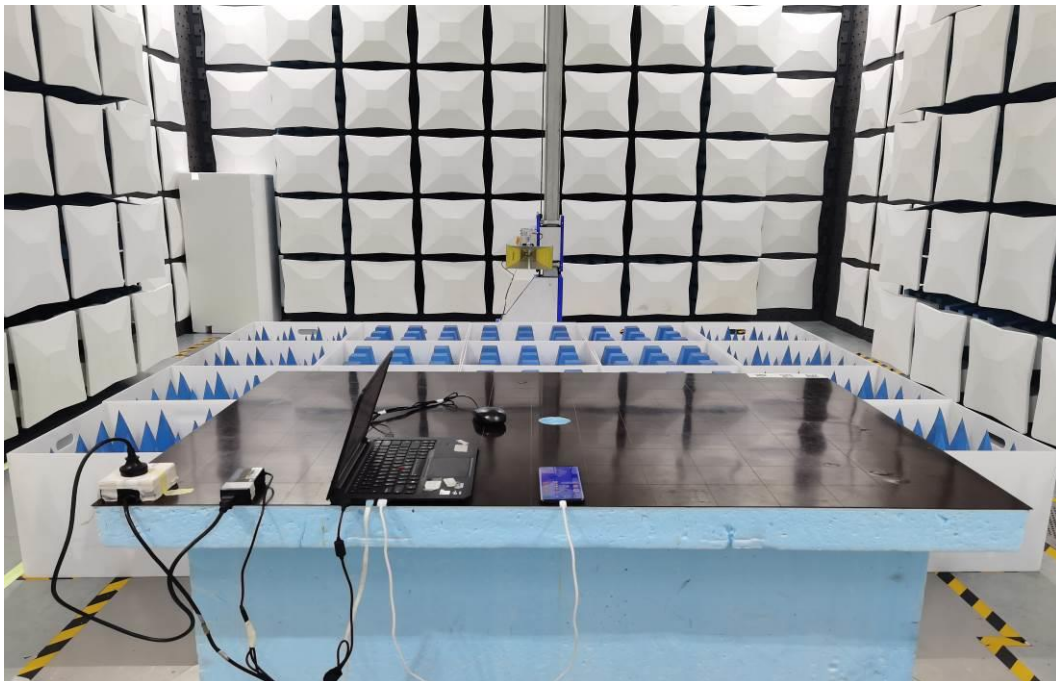
Radiated Disturbance Emissions (1GHz to 18GHz)
