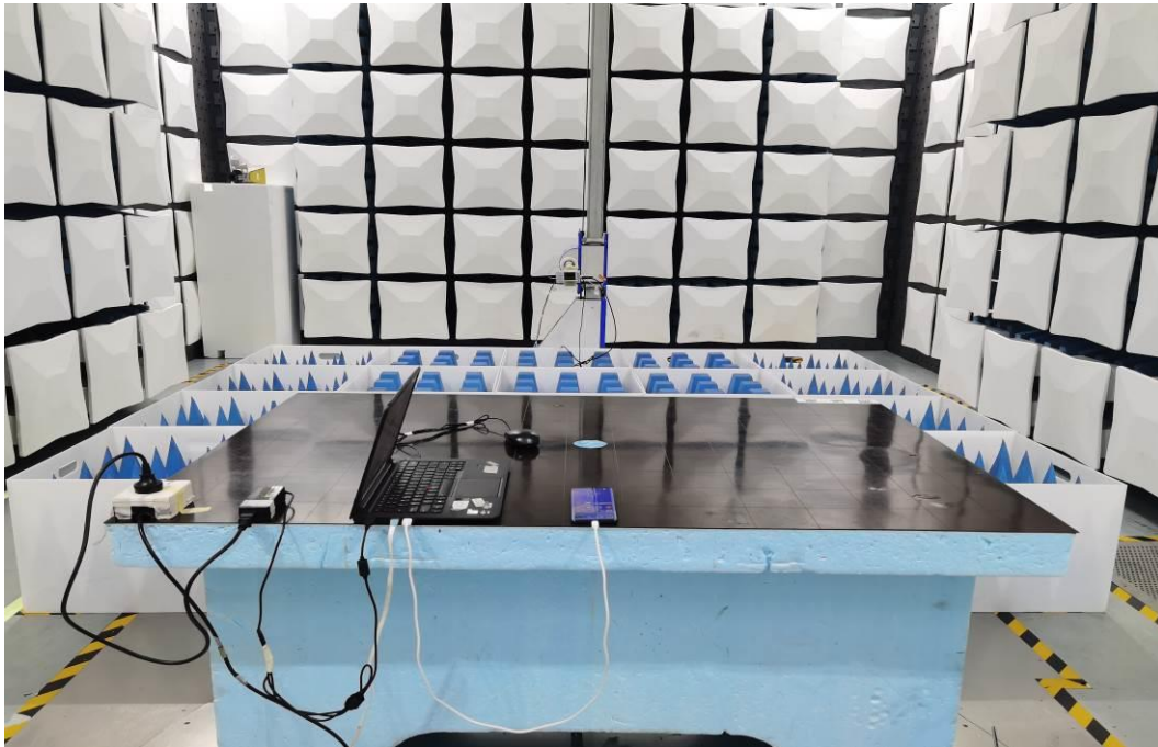
Radiated Disturbance Emissions (18GHz to 40GHz)
