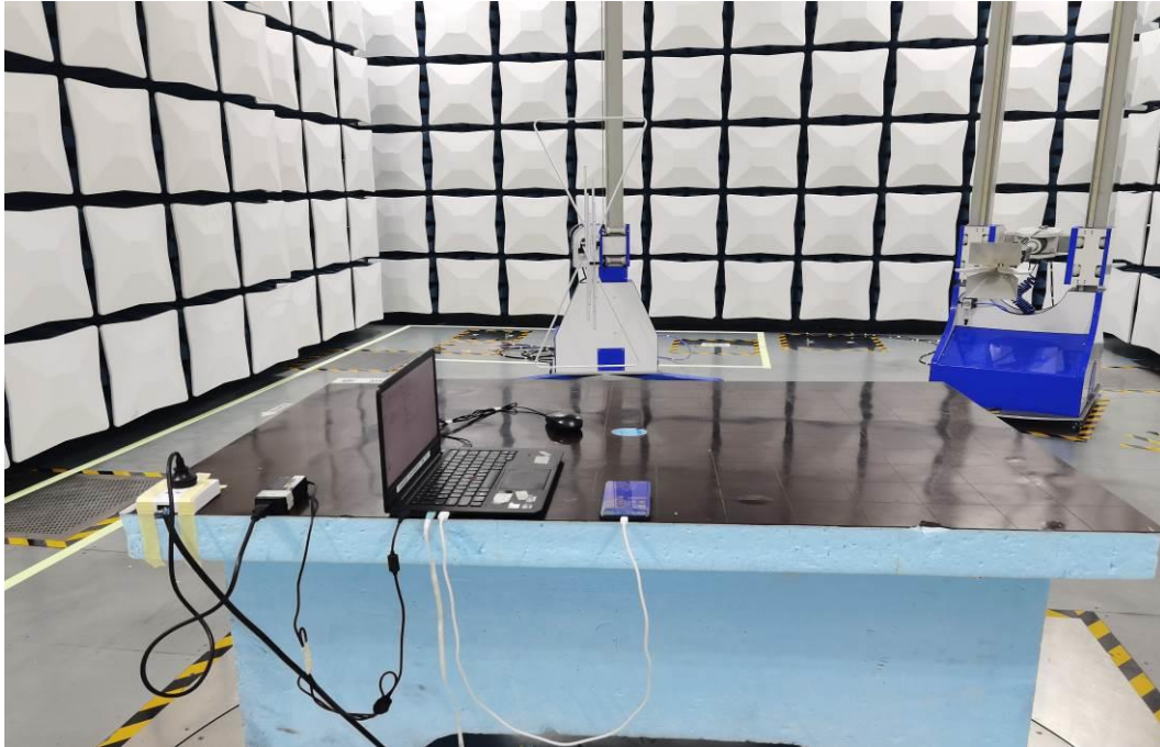
Radiated Disturbance Emissions (below 1GHz)
