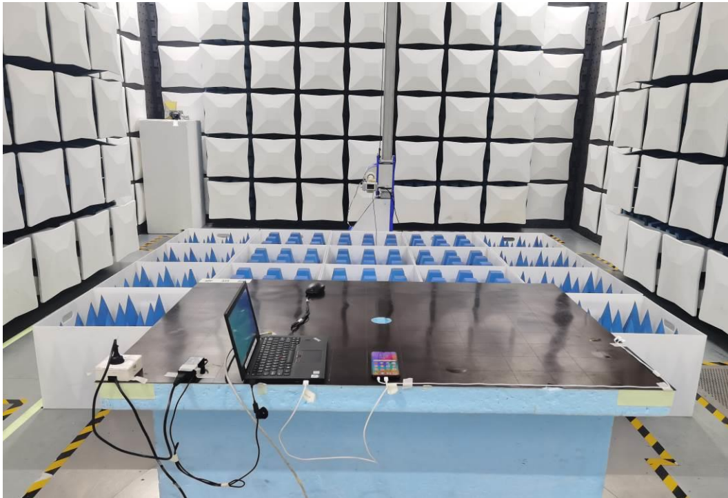
Radiated Disturbance Emissions (18GHz to 40GHz)
