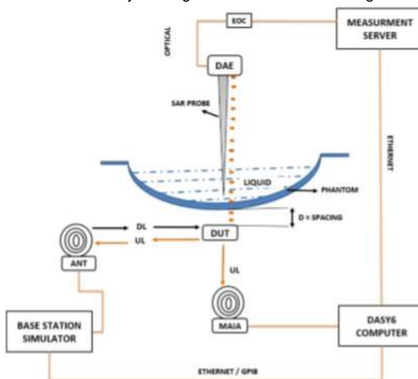
Figure: cDASY6 Dosimetric Measurement System Signal Chain
