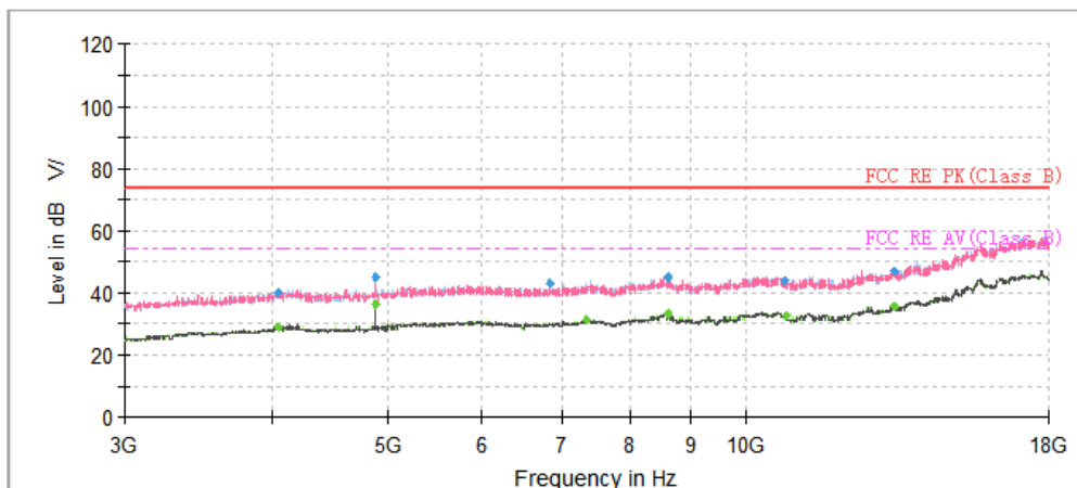
Radiates Emission from 3GHz to 18GHz
