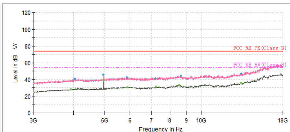
Radiates Emission from 3GHz to 18GHz
