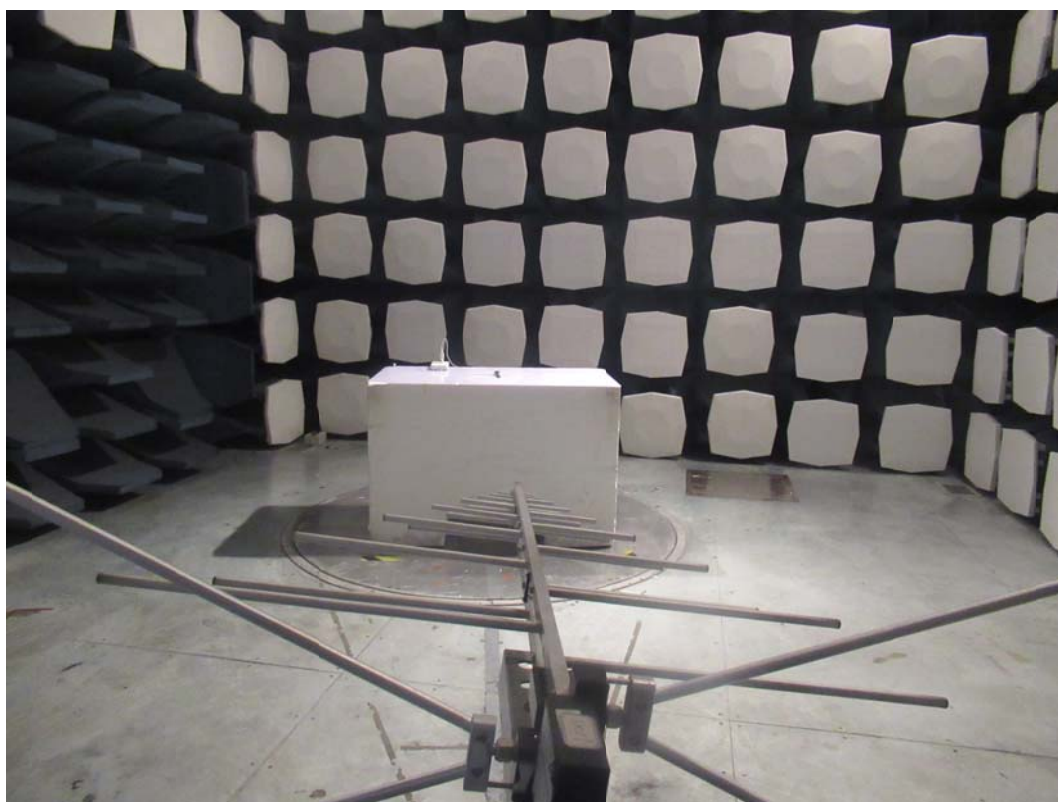
30MHz-1GHz
