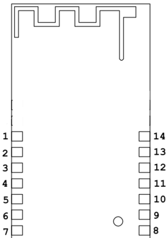
Fig 1 BL3389-P Footprint sequence
