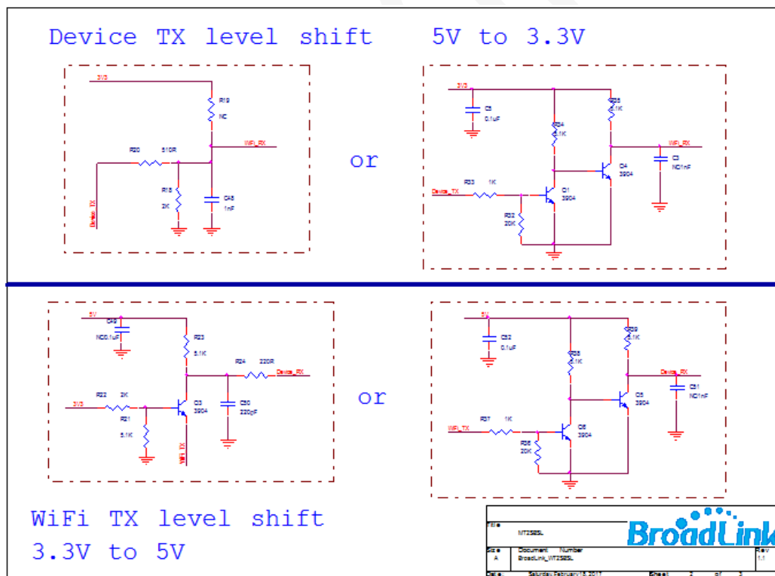
Fig 4 Circuit diagram (5V)
