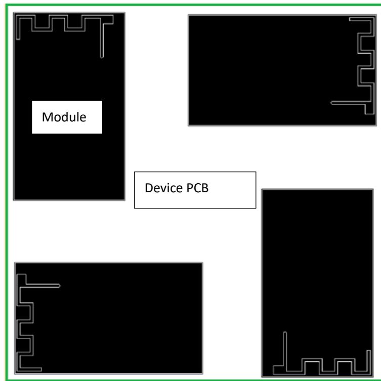
Fig 2 BL3389-P Recommended PCB layout
