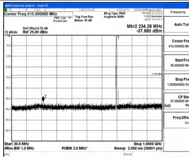
Band85-10MHz-16QAM-134092-1-0-Low-30-1000--37.88-PASS
