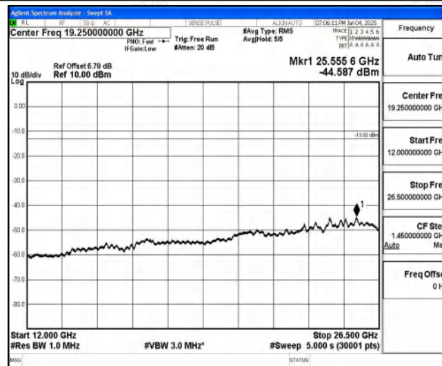
Band85-10MHz-QPSK-134092-1-0-Low-12000-26500--44.59-PASS
