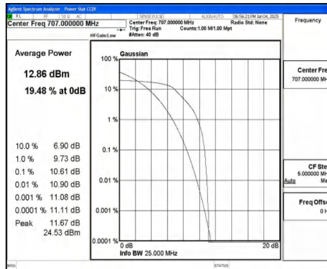
Band85-10MHz-QPSK-134092-6-0-Low-10.61-&lt;=13-PASS
