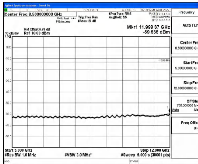
Band85-10MHz-16QAM-134052-1-0-Low-5000-12000--59.54-PASS
