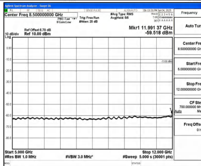
Band85-5MHz-16QAM-134157-1-0-High-5000-12000--59.52-PASS
