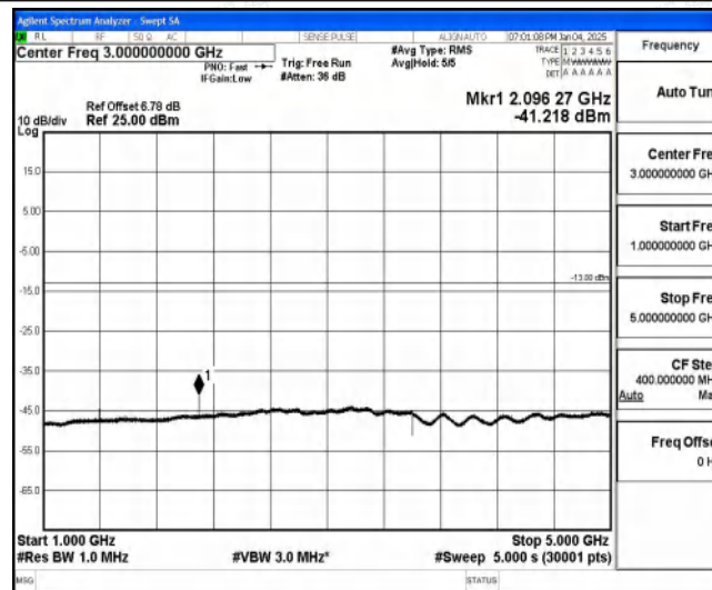
Band85-10MHz-QPSK-134052-1-0-Low-1000-5000--41.22-PASS
