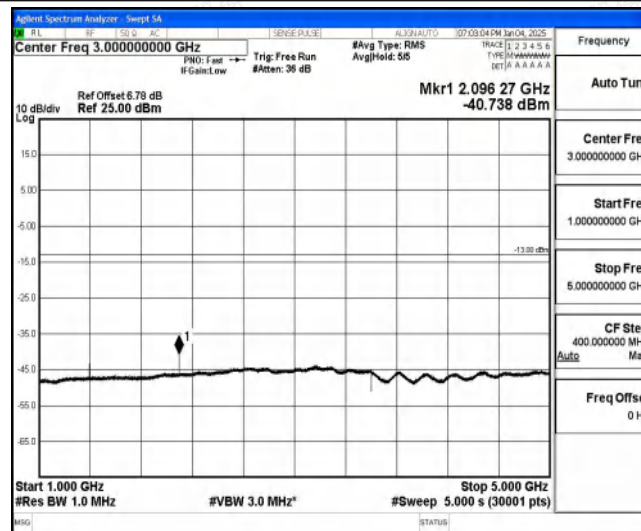
Band85-10MHz-16QAM-134052-1-0-Low-1000-5000--40.74-PASS
