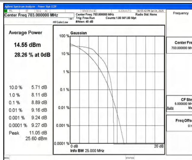
Band85-10MHz-QPSK-134052-6-0-Low-8.89-&lt;=13-PASS
