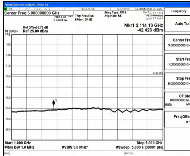
Band85-5MHz-16QAM-134092-1-0-Low-1000-5000--42.42-PASS
