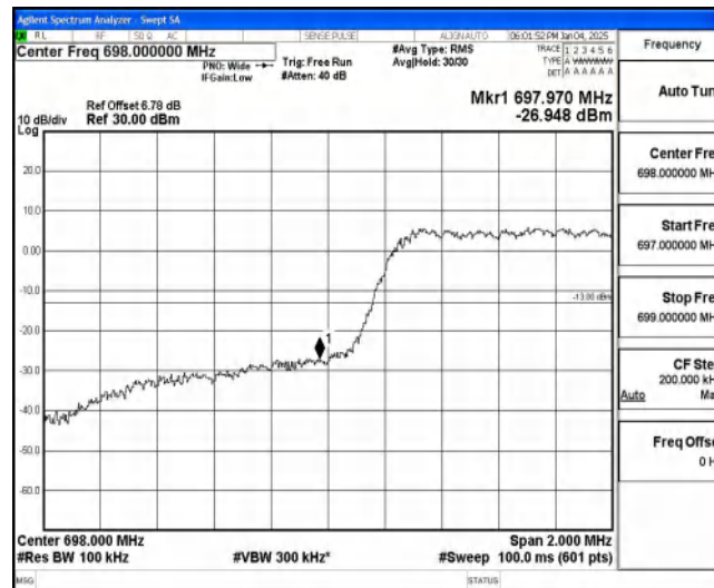
Band85-5MHz-16QAM-134027-6-0-Low--26.95-PASS
