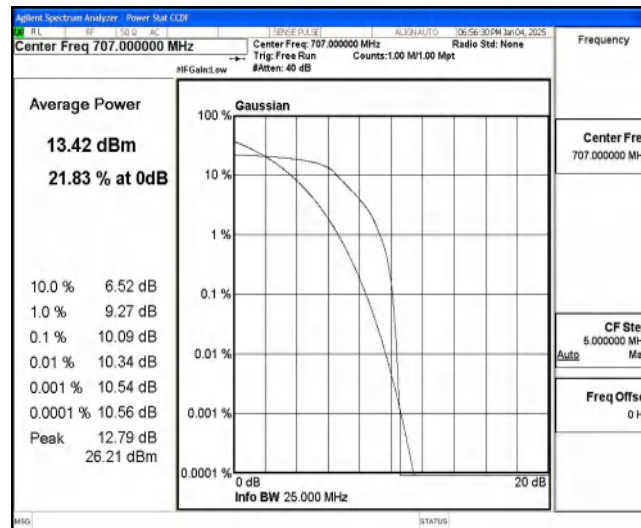
Band85-10MHz-16QAM-134092-6-0-Low-10.09-&lt;=13-PASS
