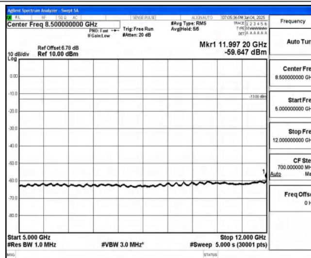
Band85-10MHz-QPSK-134092-1-0-Low-5000-12000--59.65-PASS
