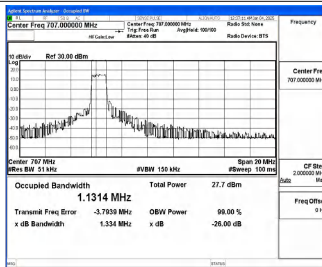
Band85-10MHz-16QAM-134092-6-0-Low-1.1314-1.334-PASS
