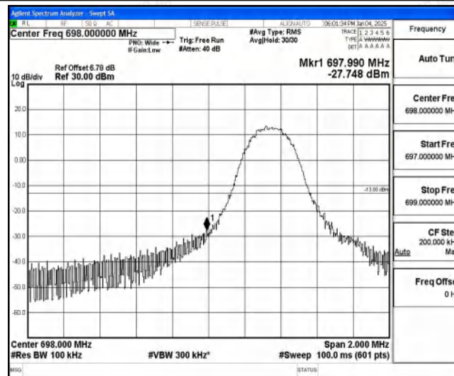
Band85-5MHz-16QAM-134027-1-0-Low--27.75-PASS
