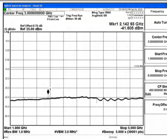
Band85-10MHz-QPSK-134132-1-0-High-1000-5000--41.61-PASS
