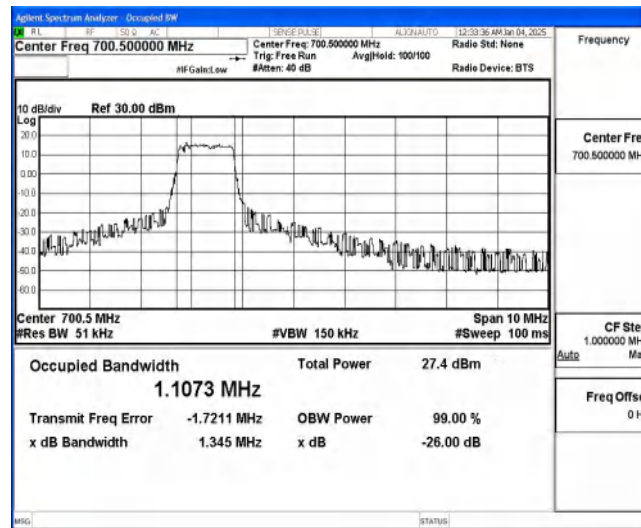
Band85-5MHz-16QAM-134027-6-0-Low-1.1073-1.345-PASS
