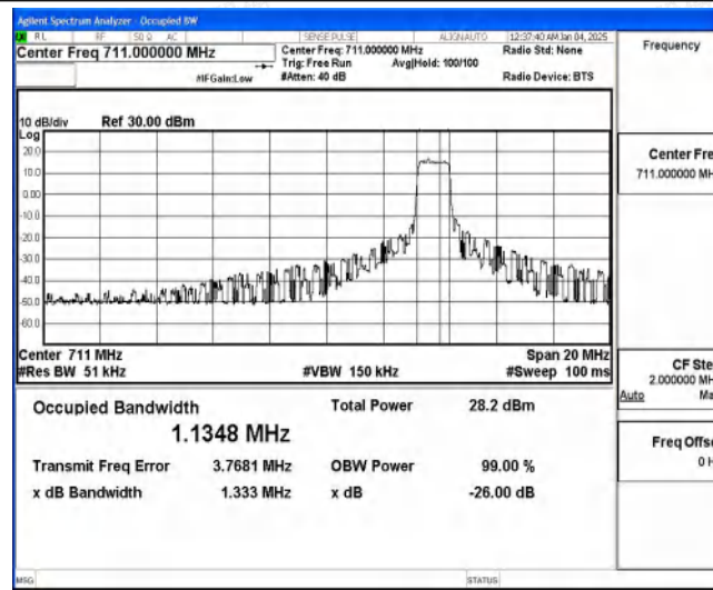
Band85-10MHz-QPSK-134132-6-0-High-1.1348-1.333-PASS
