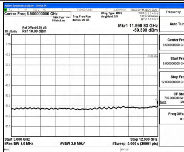
Band85-5MHz-16QAM-134092-1-0-Low-5000-12000--59.39-PASS
