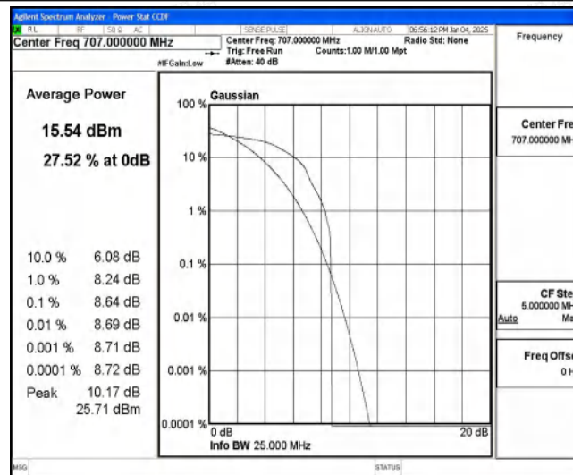
Band85-10MHz-16QAM-134092-1-0-Low-8.64-&lt;=13-PASS
