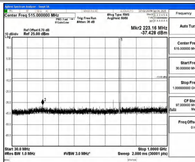
Band85-10MHz-16QAM-134052-1-0-Low-30-1000--37.43-PASS
