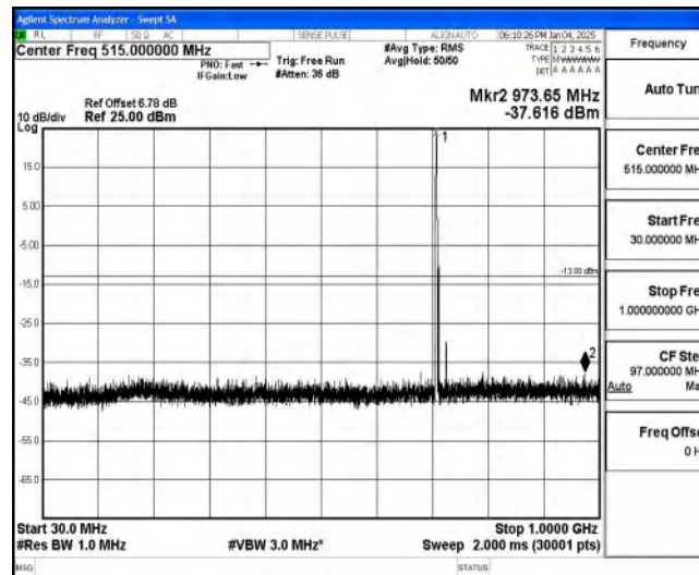
Band85-5MHz-QPSK-134157-1-0-High-30-1000--37.62-PASS
