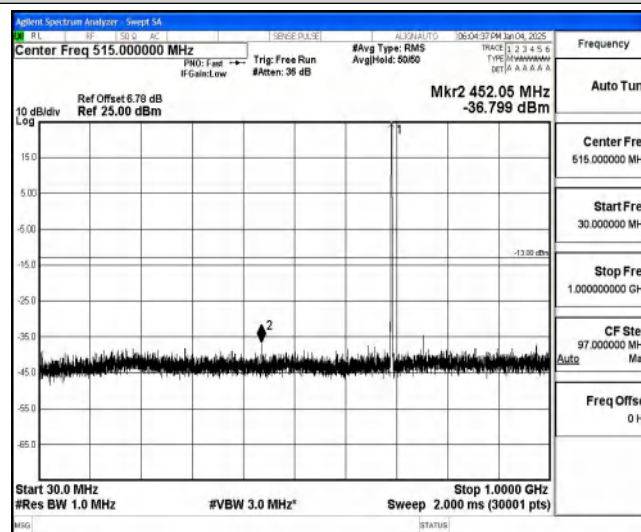
Band85-5MHz-16QAM-134027-1-0-Low-30-1000--36.8-PASS
