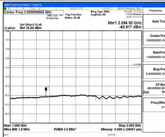
Band85-5MHz-16QAM-134027-1-0-Low-1000-5000--40.92-PASS
