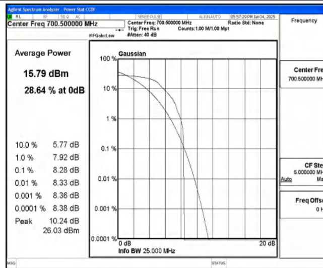
Band85-5MHz-QPSK-134027-1-0-Low-8.28-&lt;=13-PASS
