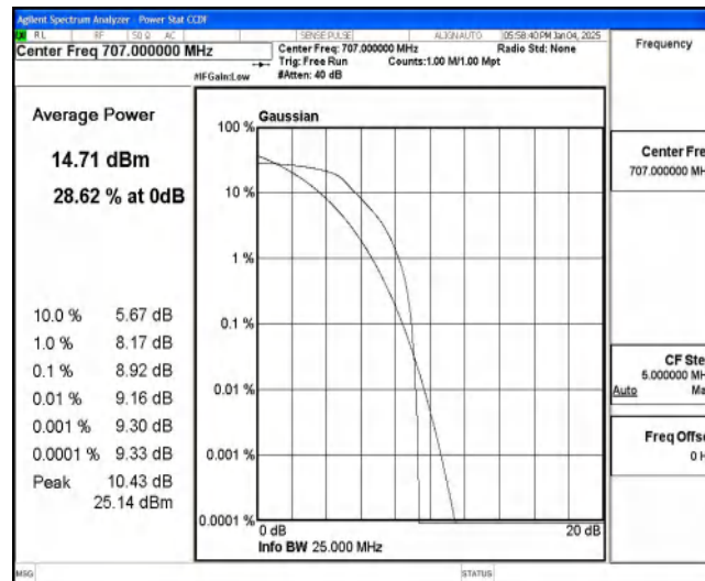
Band85-5MHz-16QAM-134092-6-0-Low-8.92-&lt;=13-PASS
