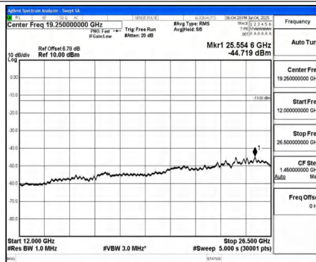
Band85-5MHz-QPSK-134027-1-0-Low-12000-26500--44.72-PASS
