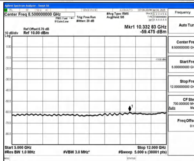
Band85-10MHz-QPSK-134132-1-0-High-5000-12000--59.48-PASS
