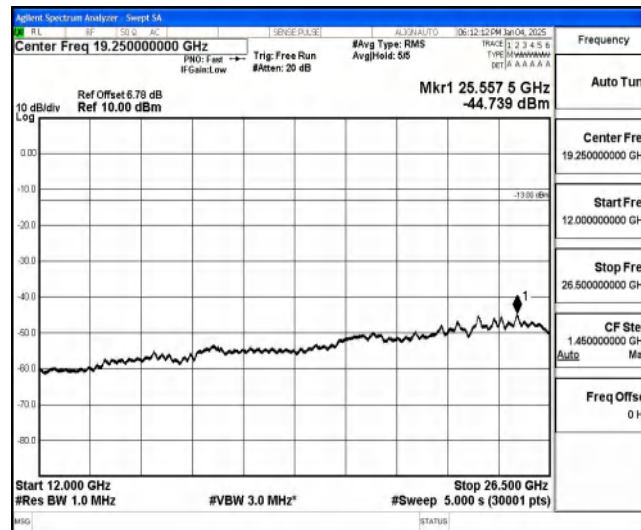
Band85-5MHz-QPSK-134157-1-0-High-12000-26500--44.74-PASS
