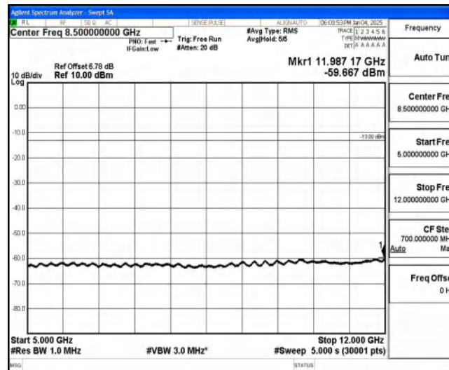
Band85-5MHz-QPSK-134027-1-0-Low-5000-12000--59.67-PASS
