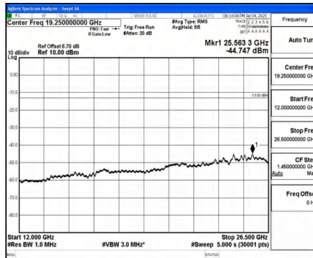
Band85-5MHz-16QAM-134157-1-0-High-12000-26500--44.75-PASS
