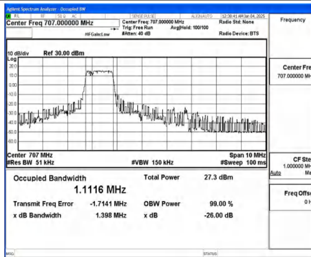
Band85-5MHz-QPSK-134092-6-0-Low-1.1116-1.398-PASS
