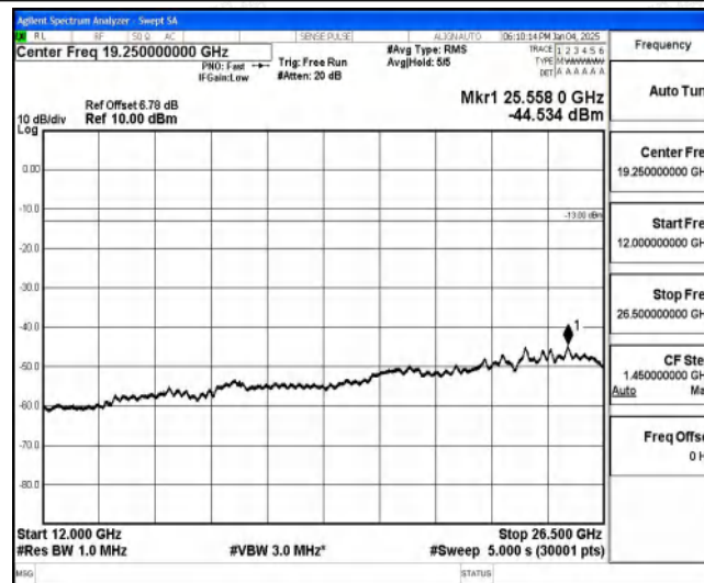
Band85-5MHz-16QAM-134092-1-0-Low-12000-26500--44.53-PASS
