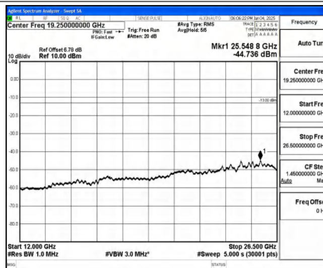
Band85-5MHz-16QAM-134027-1-0-Low-12000-26500--44.74-PASS
