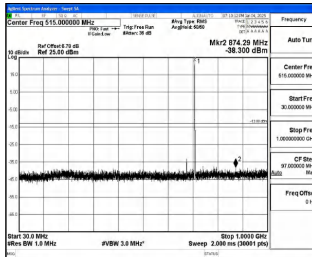
Band85-10MHz-16QAM-134132-1-0-High-30-1000--38.3-PASS
