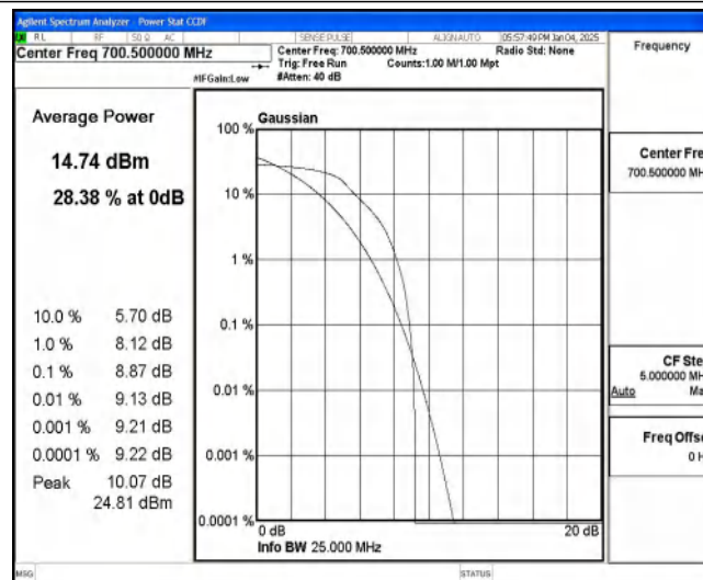
Band85-5MHz-QPSK-134027-6-0-Low-8.87-&lt;=13-PASS
