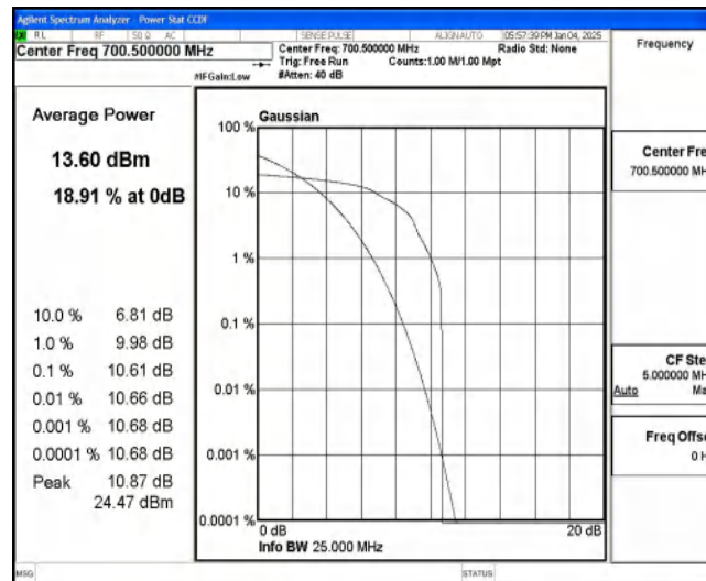
Band85-5MHz-16QAM-134027-1-0-Low-10.61-&lt;=13-PASS
