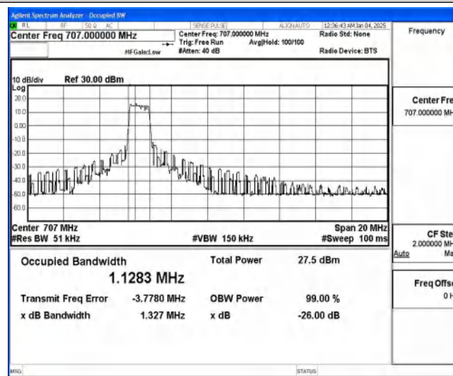
Band85-10MHz-QPSK-134092-6-0-Low-1.1283-1.327-PASS
