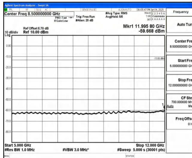
Band85-5MHz-16QAM-134027-1-0-Low-5000-12000--59.67-PASS
