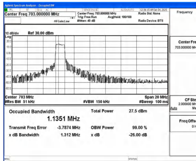
Band85-10MHz-16QAM-134052-6-0-Low-1.1351-1.312-PASS
