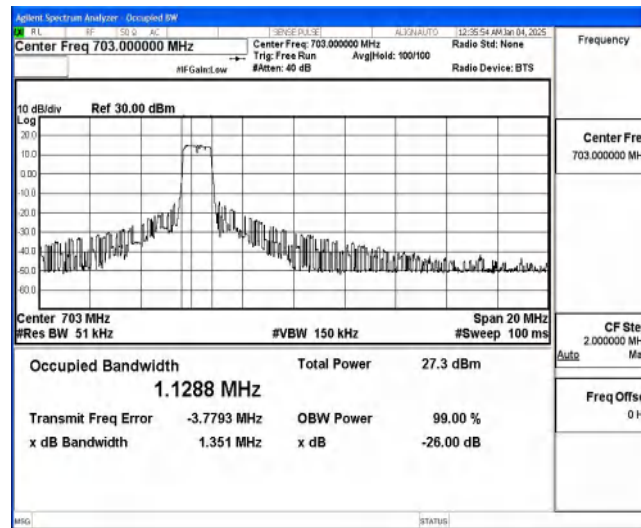
Band85-10MHz-QPSK-134052-6-0-Low-1.1288-1.351-PASS
