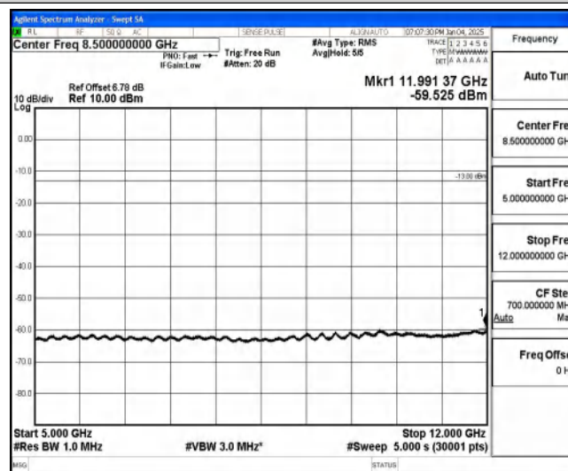
Band85-10MHz-16QAM-134092-1-0-Low-5000-12000--59.53-PASS
