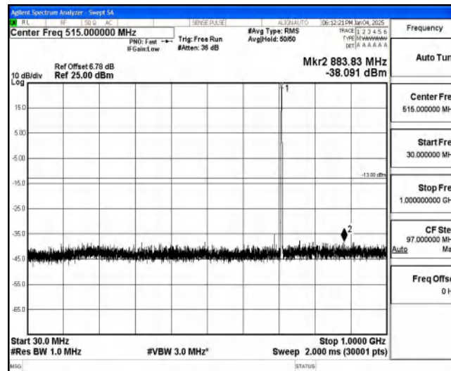
Band85-5MHz-16QAM-134157-1-0-High-30-1000--38.09-PASS
