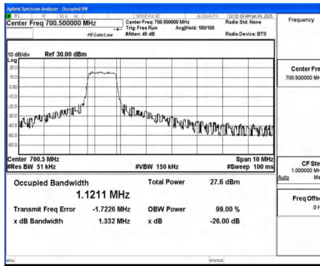
Band85-5MHz-QPSK-134027-6-0-Low-1.1211-1.332-PASS
