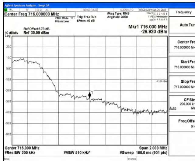
Band85-10MHz-QPSK-134132-6-0-High--26.92-PASS
