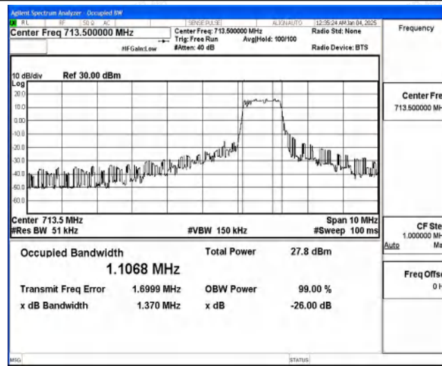
Band85-5MHz-16QAM-134157-6-0-High-1.1068-1.370-PASS
