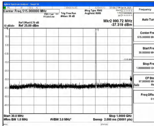
Band85-10MHz-QPSK-134132-1-0-High-30-1000--37.32-PASS
