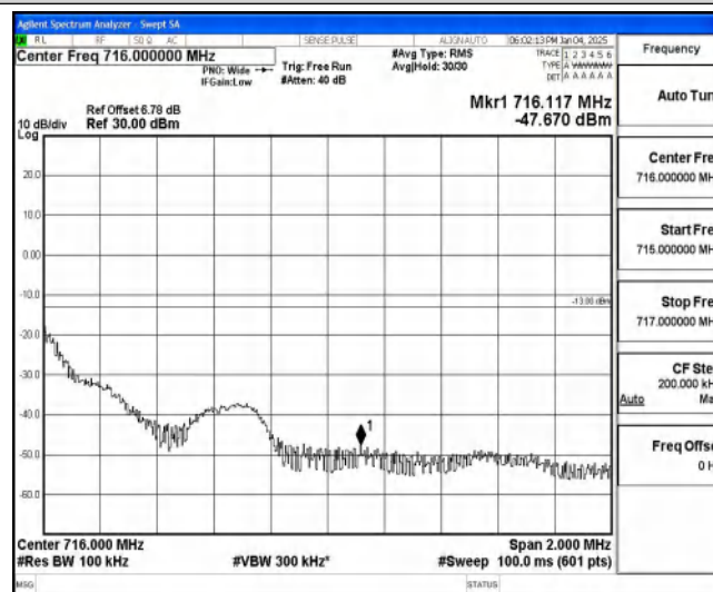
Band85-5MHz-16QAM-134157-1-0-High--47.67-PASS
