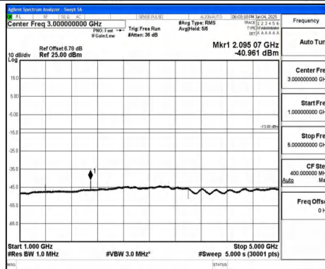
Band85-5MHz-QPSK-134027-1-0-Low-1000-5000--40.96-PASS
