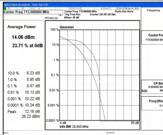
Band85-5MHz-16QAM-134157-6-0-High-9.87-&lt;=13-PASS
