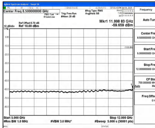
Band85-10MHz-QPSK-134052-1-0-Low-5000-12000--59.66-PASS
