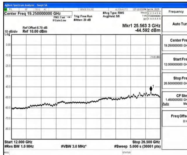
Band85-10MHz-QPSK-134132-1-0-High-12000-26500--44.59-PASS
