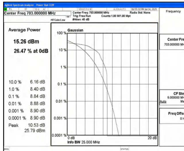
Band85-10MHz-16QAM-134052-1-0-Low-8.84-&lt;=13-PASS
