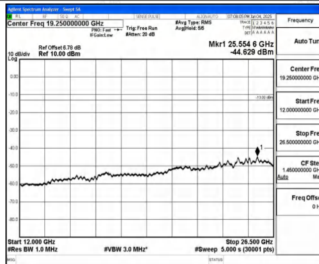
Band85-10MHz-16QAM-134092-1-0-Low-12000-26500--44.63-PASS
