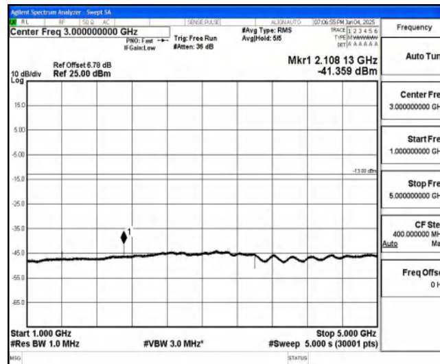
Band85-10MHz-16QAM-134092-1-0-Low-1000-5000--41.36-PASS
