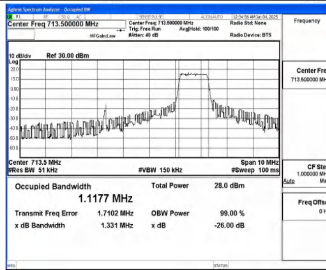
Band85-5MHz-QPSK-134157-6-0-High-1.1177-1.331-PASS
