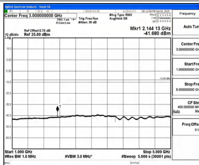
Band85-5MHz-16QAM-134157-1-0-High-1000-5000--41.68-PASS
