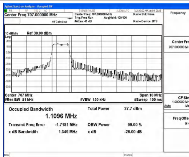
Band85-5MHz-16QAM-134092-6-0-Low-1.1096-1.349-PASS
