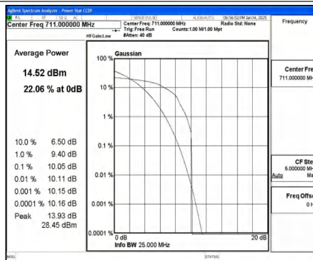
Band85-10MHz-16QAM-134132-1-0-High-10.05-&lt;=13-PASS
