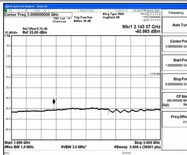
Band85-10MHz-16QAM-134132-1-0-High-1000-5000--40.98-PASS
