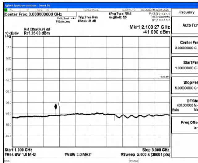
Band85-10MHz-QPSK-134092-1-0-Low-1000-5000--41.09-PASS
