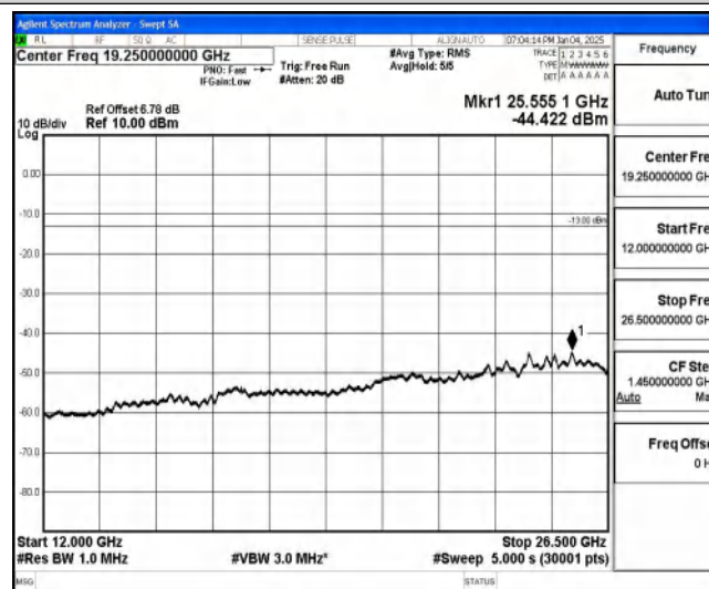
Band85-10MHz-16QAM-134052-1-0-Low-12000-26500--44.42-PASS
