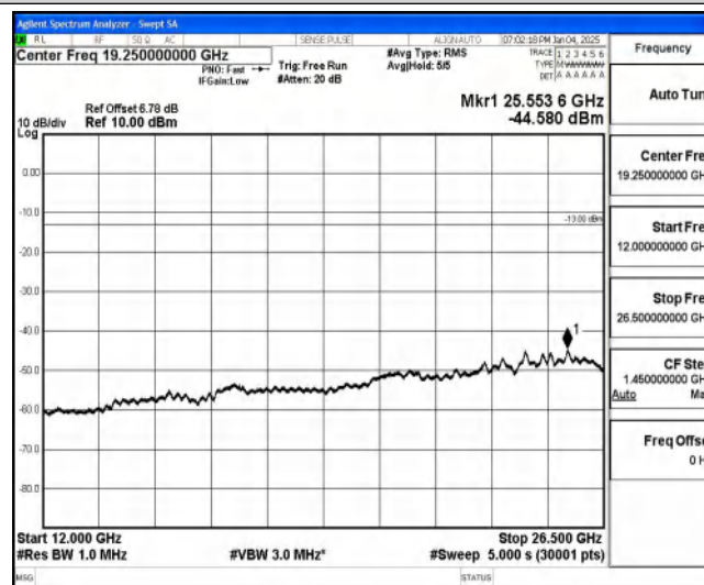
Band85-10MHz-QPSK-134052-1-0-Low-12000-26500--44.58-PASS
