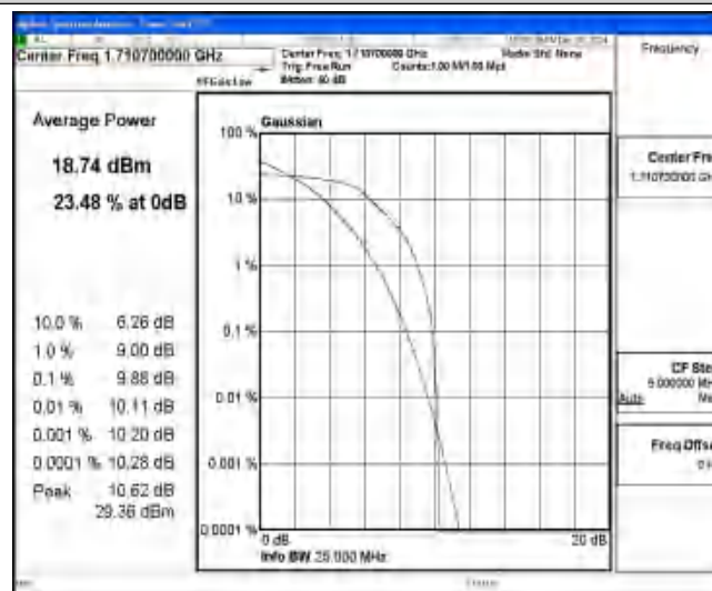
Band4-1.4MHz-16QAM-19957-6-0-Low-9.88-≤13-PASS
