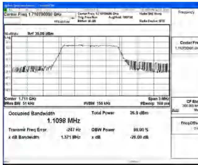
Band4-1.4MHz-QPSK-19957-6-0-Low-1.1098-1.371-PASS
