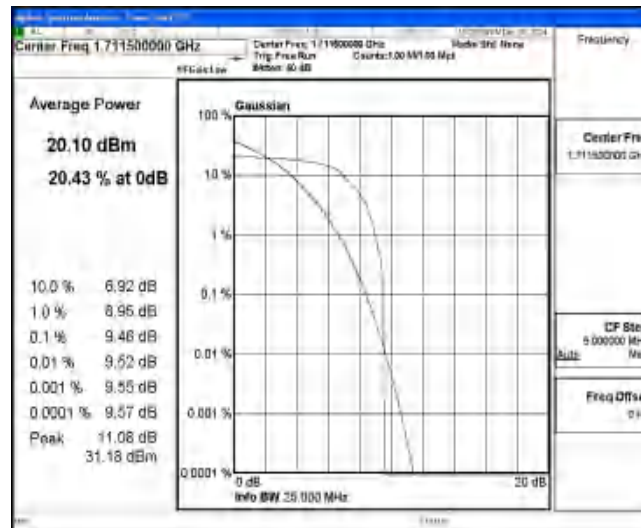
Band4-3MHz-QPSK-19965-1-0-Low-9.46-&lt;=13-PASS
