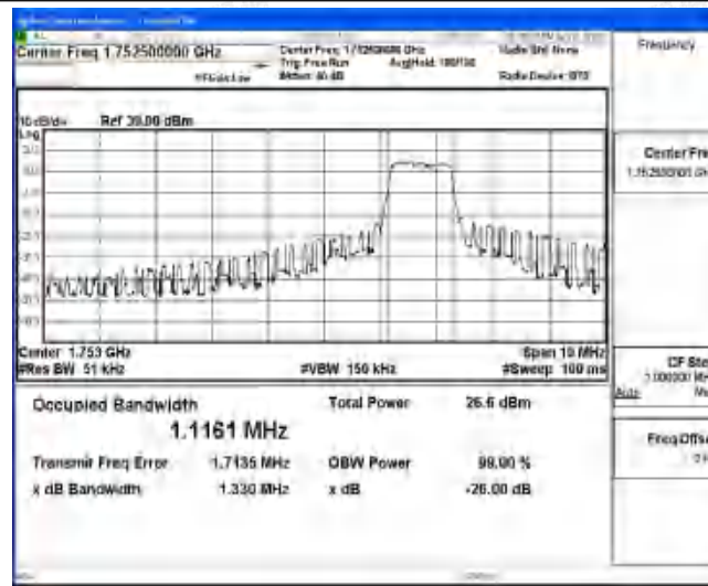
Band4-5MHz-QPSK-20375-6-0-High-1.1161-1.330-PASS
