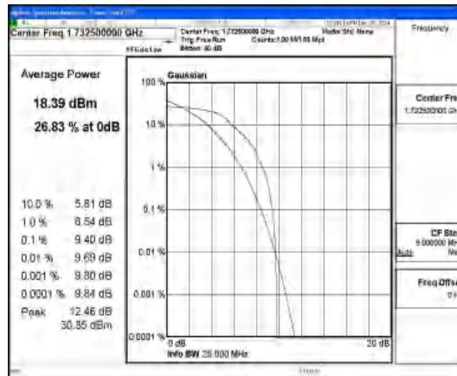
Band4-1.4MHz-16QAM-20175-6-0-Low-9.40-&lt;=13-PASS
