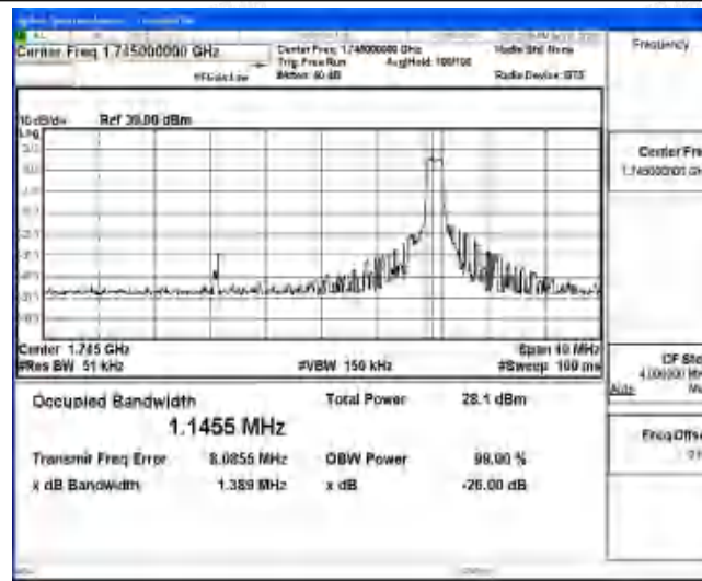
Band4-20MHz-QPSK-20300-6-0-High-1.1455-1.389-PASS
