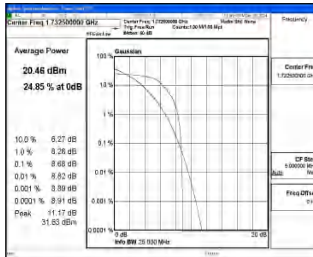
Band4-15MHz-QPSK-20175-6-0-Low-8.68-13-PASS
