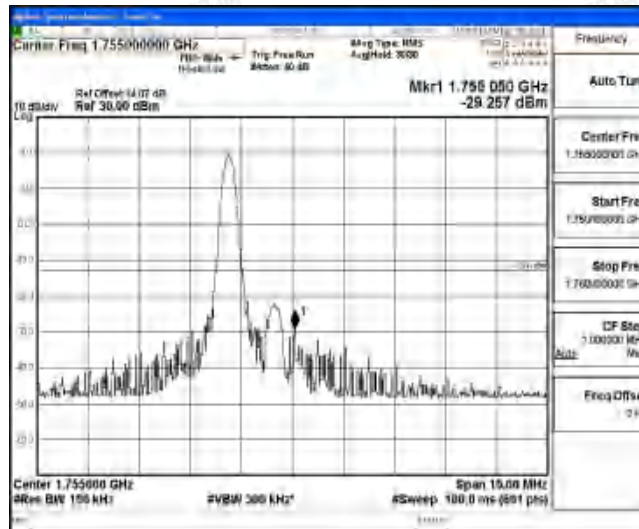
Band4-5MHz-16QAM-20375-1-0-High--29.26-PASS
