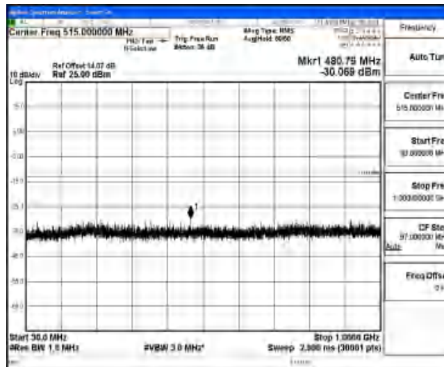
Band4-15MHz-QPSK-20025-1-0-Low-30-1000--30.07-PASS
