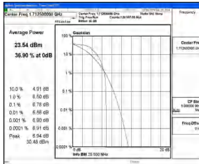
Band4-5MHz-QPSK-19975-1-0-Low-6.78-&lt;=13-PASS
