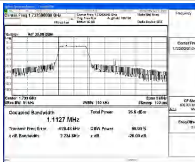
Band4-3MHz-16QAM-20175-6-0-Low-1.1127-2.234-PASS
