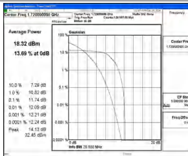
Band4-20MHz-16QAM-20050-6-0-Low-11.74-≤13-PASS
