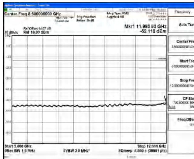
Band4-5MHz-16QAM-20175-1-0-Low-5000-12000--52.12-PASS
