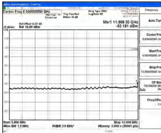
Band4-15MHz-16QAM-20175-1-0-Low-5000-12000--52.19-PASS
