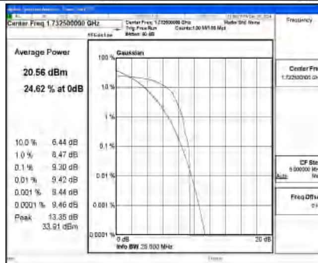
Band4-20MHz-16QAM-20175-1-0-Low-9.30-≤13-PASS
