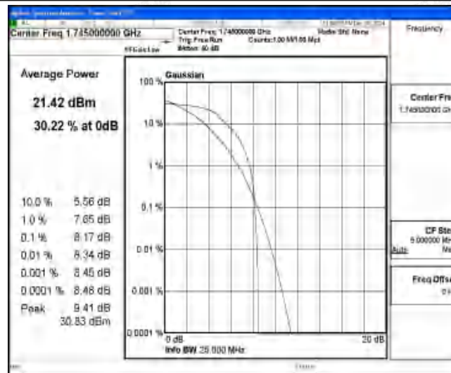
Band4-20MHz-QPSK-20300-6-0-High-8.17-≤13-PASS
