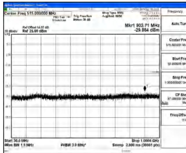
Band4-5MHz-16QAM-19975-1-0-Low-30-1000--29.88-PASS
