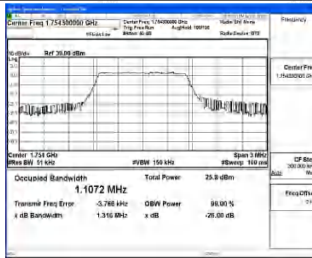
Band4-1.4MHz-16QAM-20393-6-0-High-1.1072-1.316-PASS
