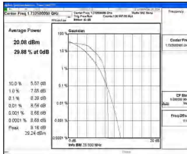
Band4-10MHz-QPSK-20175-6-0-Low-8.39-&lt;=13-PASS
