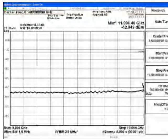
Band4-15MHz-QPSK-20175-1-0-Low-5000-12000--52.05-PASS
