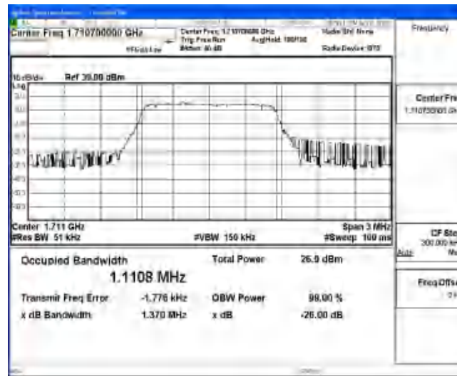
Band4-1.4MHz-16QAM-19957-6-0-Low-1.1108-1.370-PASS
