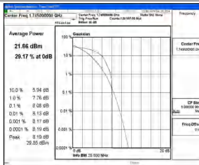
Band4-20MHz-16QAM-20300-1-0-High-8.08-≤13-PASS
