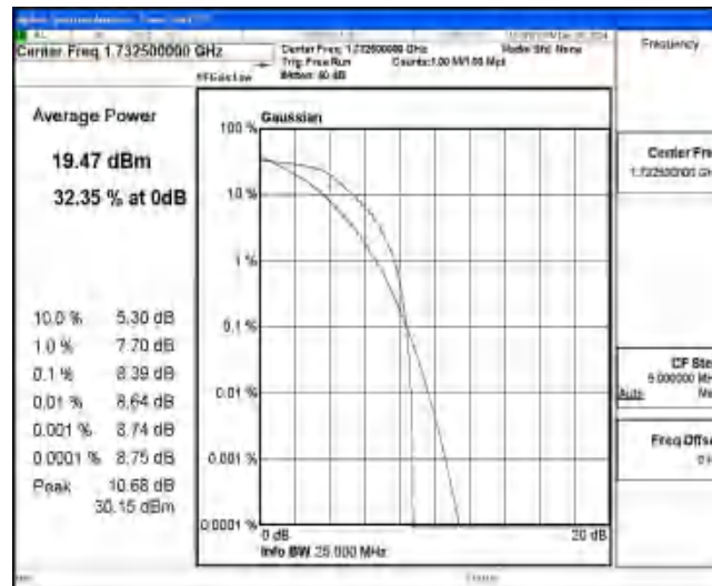
Band4-3MHz-16QAM-20175-6-0-Low-8.39-&lt;=13-PASS
