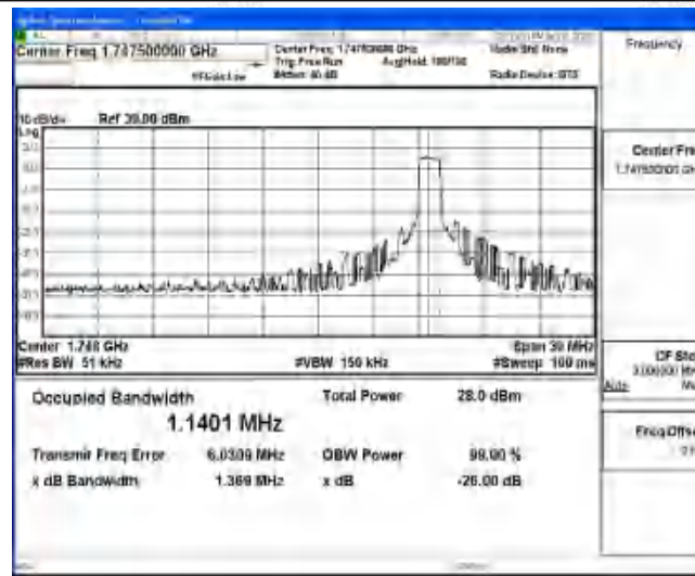
Band4-15MHz-QPSK-20325-6-0-High-1.1401-1.369-PASS
