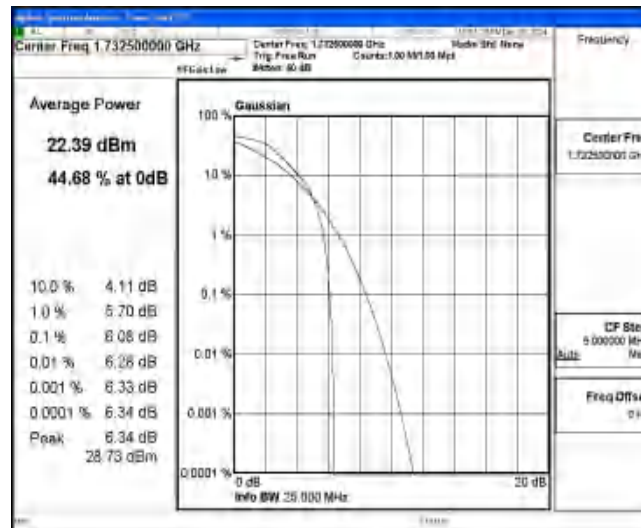
Band4-5MHz-QPSK-20175-6-0-Low-6.08-&lt;=13-PASS
