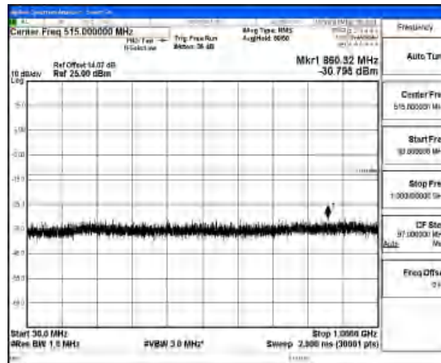
Band4-3MHz-16QAM-19965-1-0-Low-30-1000--30.8-PASS
