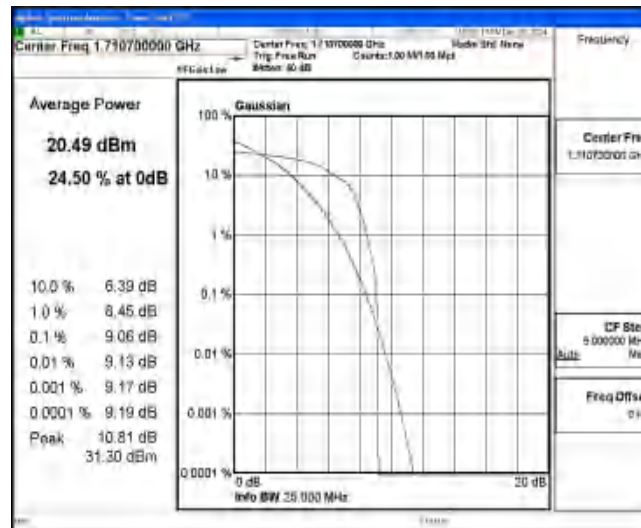
Band4-1.4MHz-16QAM-19957-1-0-Low-9.06-≤13-PASS
