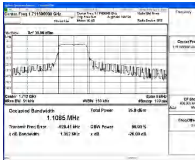
Band4-3MHz-QPSK-19965-6-0-Low-1.1065-1.352-PASS
