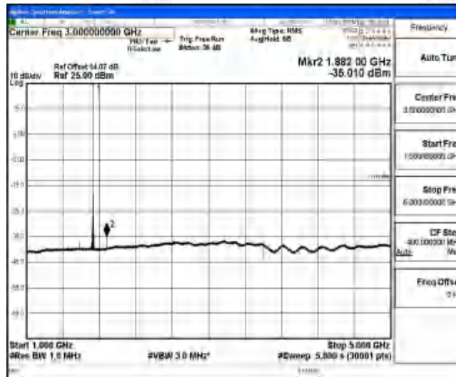
Band4-3MHz-16QAM-20175-1-0-Low-1000-5000--35.01-PASS
