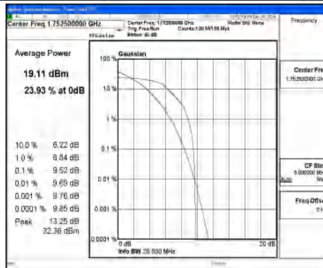
Band4-5MHz-QPSK-20375-6-0-High-9.52-≤13-PASS
