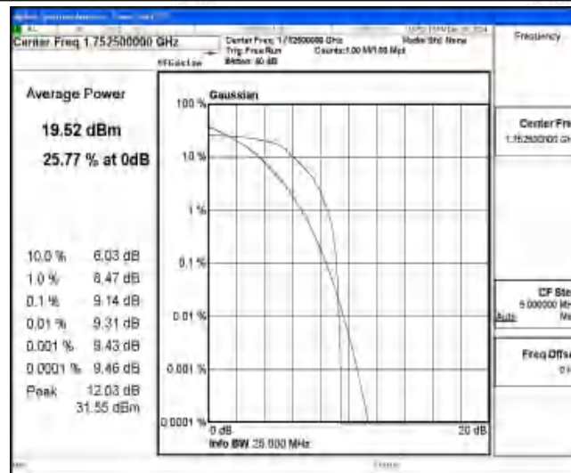
Band4-5MHz-16QAM-20375-6-0-High-9.14-13-PASS
