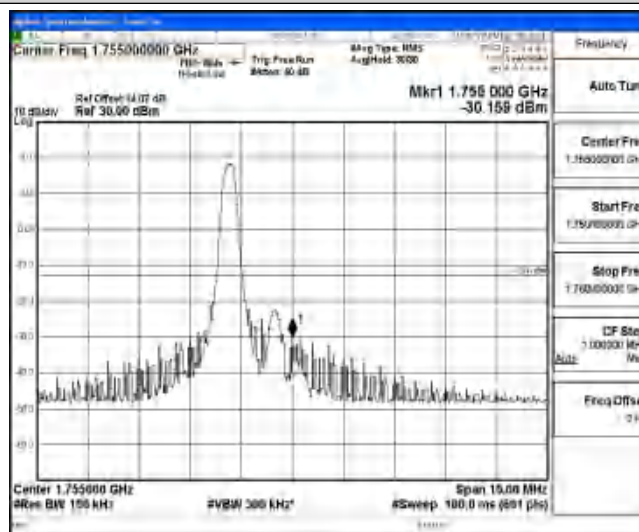
Band4-5MHz-QPSK-20375-1-0-High--30.16-PASS
