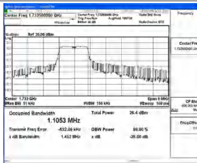
Band4-3MHz-QPSK-20175-6-0-Low-1.1053-1.452-PASS
