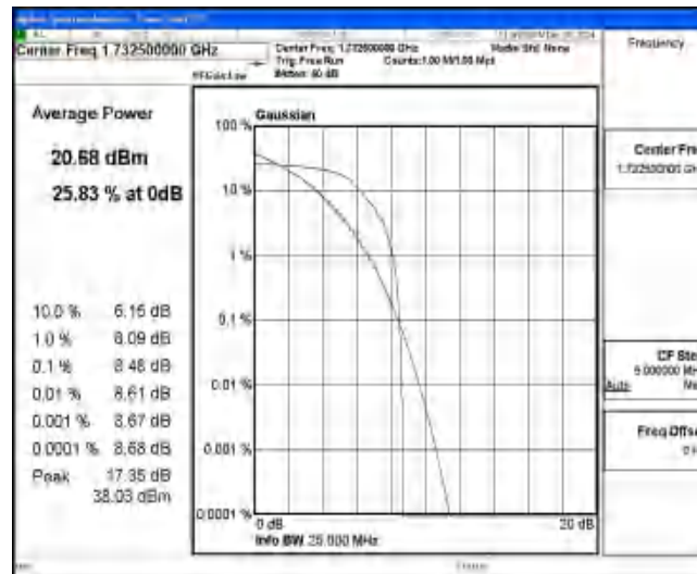
Band4-15MHz-16QAM-20175-6-0-Low-8.48-&lt;=13-PASS
