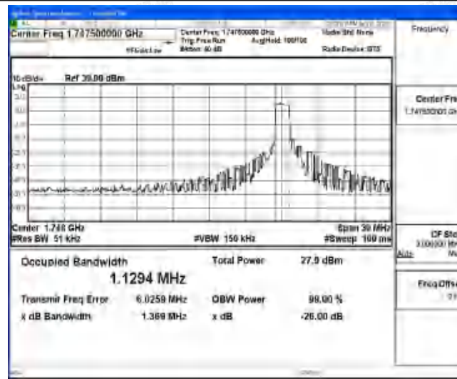
Band4-15MHz-16QAM-20325-6-0-High-1.1294-1.369-PASS
