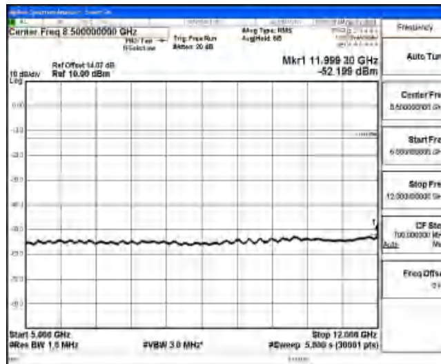
Band4-20MHz-QPSK-20175-1-0-Low-5000-12000--52.2-PASS
