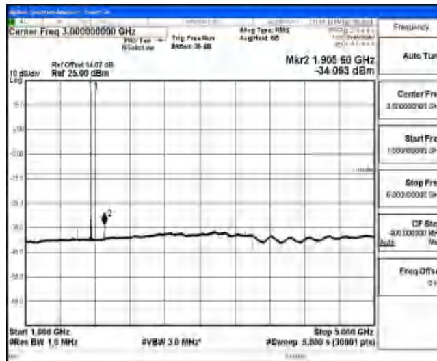
Band4-15MHz-16QAM-20325-1-0-High-1000-5000--34.09-PASS
