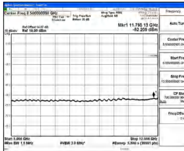
Band4-10MHz-QPSK-20175-1-0-Low-5000-12000--52.21-PASS
