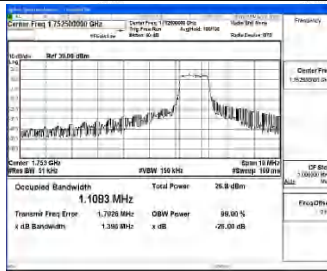
Band4-5MHz-16QAM-20375-6-0-High-1.1083-1.396-PASS
