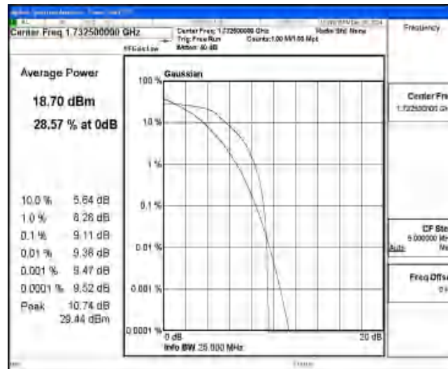
Band4-1.4MHz-QPSK-20175-6-0-Low-9.11-&lt;=13-PASS
