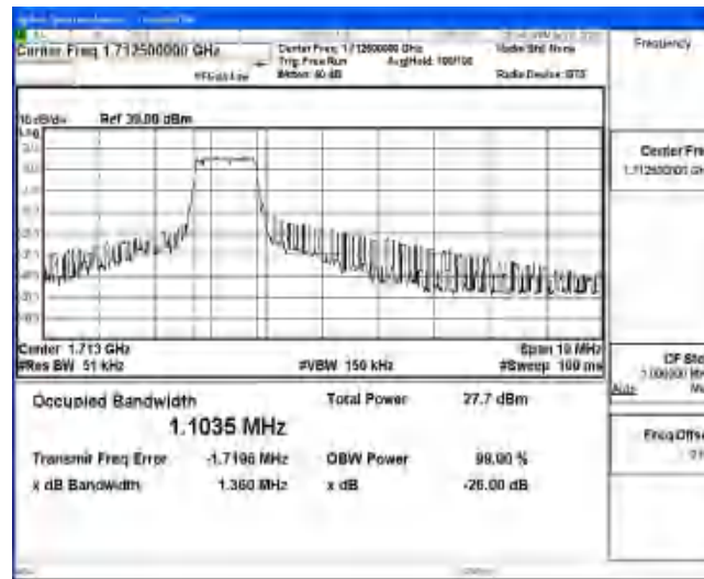
Band4-5MHz-16QAM-19975-6-0-Low-1.1035-1.360-PASS
