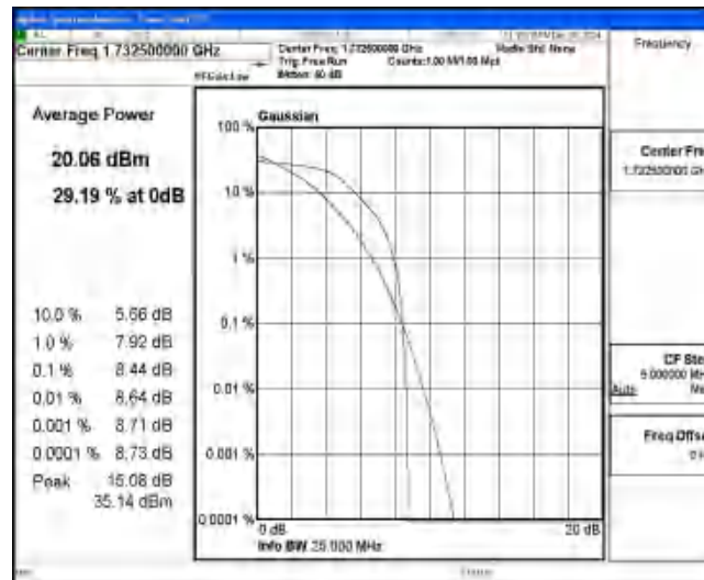
Band4-10MHz-16QAM-20175-6-0-Low-8.44-&lt;=13-PASS
