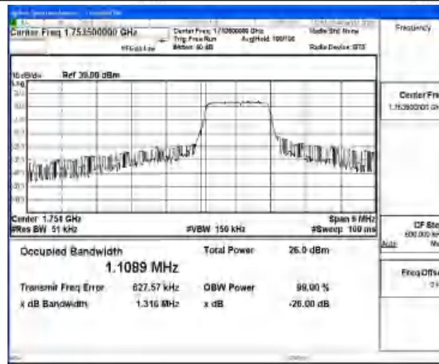
Band4-3MHz-16QAM-20385-6-0-High-1.1089-1.316-PASS
