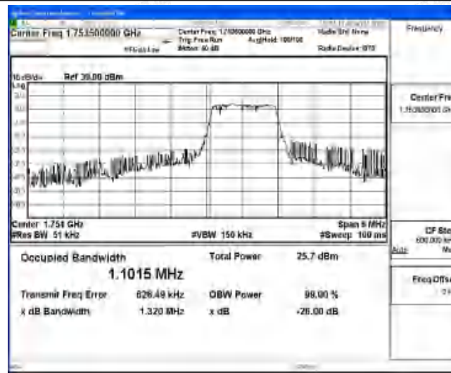
Band4-3MHz-QPSK-20385-6-0-High-1.1015-1.320-PASS
