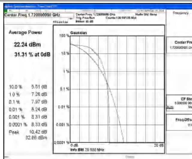
Band4-20MHz-QPSK-20050-6-0-Low-7.97-&lt;=13-PASS
