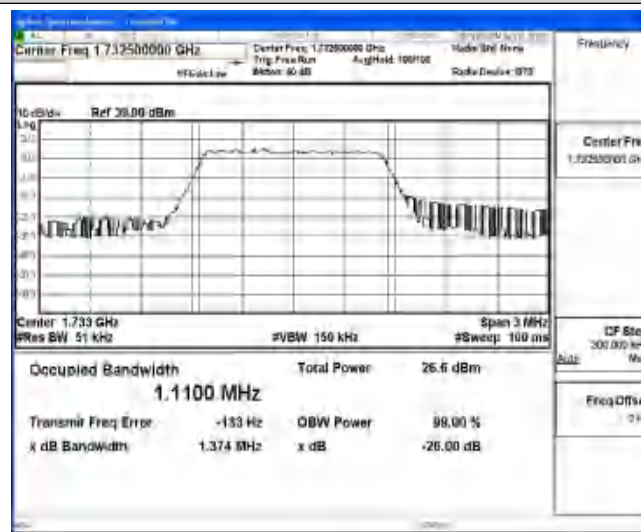
Band4-1.4MHz-16QAM-20175-6-0-Low-1.1100-1.374-PASS
