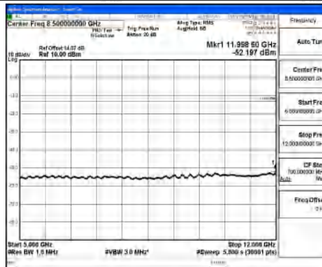
Band4-1.4MHz-QPSK-19957-1-0-Low-5000-12000--52.2-PASS
