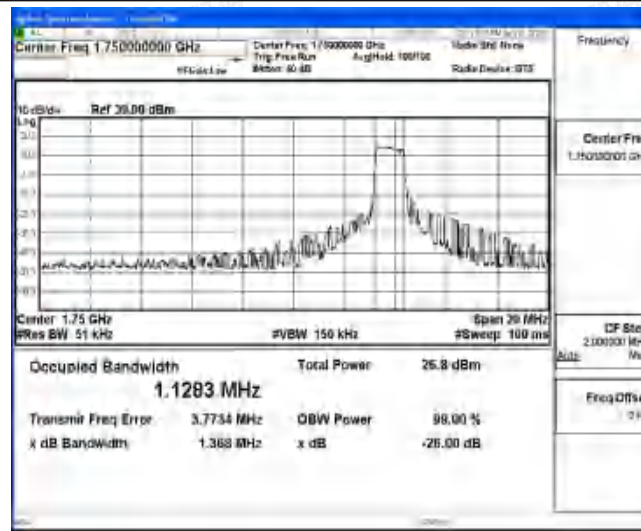
Band4-10MHz-16QAM-20350-6-0-High-1.1283-1.368-PASS
