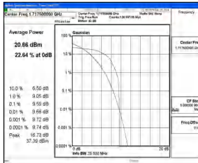
Band4-15MHz-16QAM-20025-1-0-Low-9.59-&lt;=13-PASS
