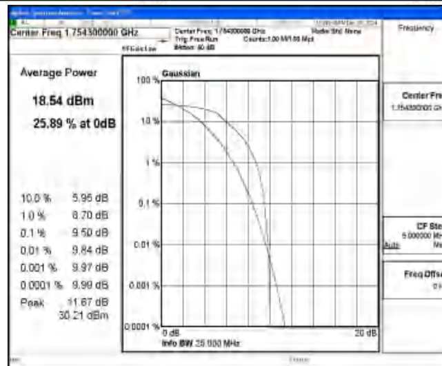
Band4-1.4MHz-QPSK-20393-6-0-High-9.50-≤13-PASS
