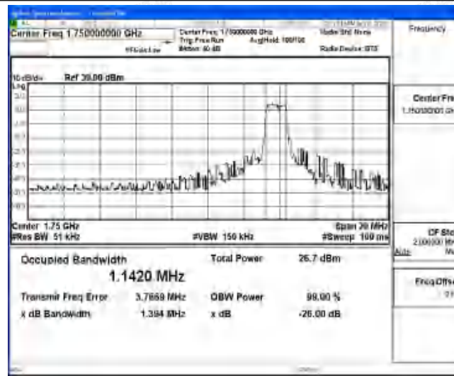
Band4-10MHz-QPSK-20350-6-0-High-1.1420-1.394-PASS
