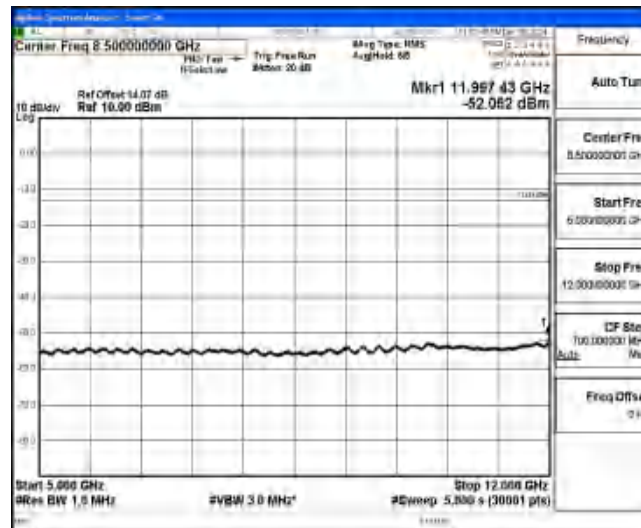
Band4-5MHz-QPSK-20175-1-0-Low-5000-12000--52.05-PASS
