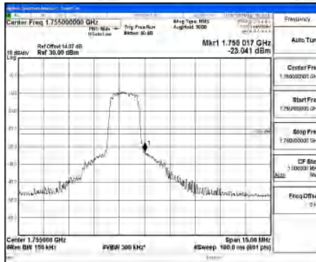
Band4-5MHz-QPSK-20375-6-0-High--23.04-PASS
