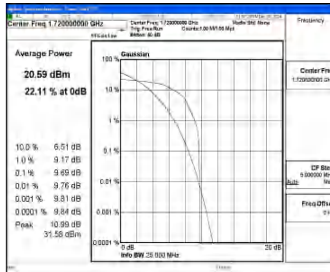
Band4-20MHz-16QAM-20050-1-0-Low-9.69-≤13-PASS
