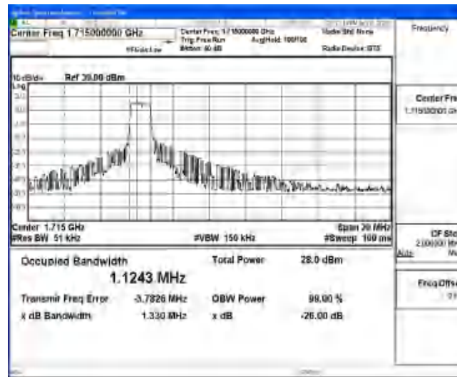
Band4-10MHz-16QAM-20000-6-0-Low-1.1243-1.330-PASS
