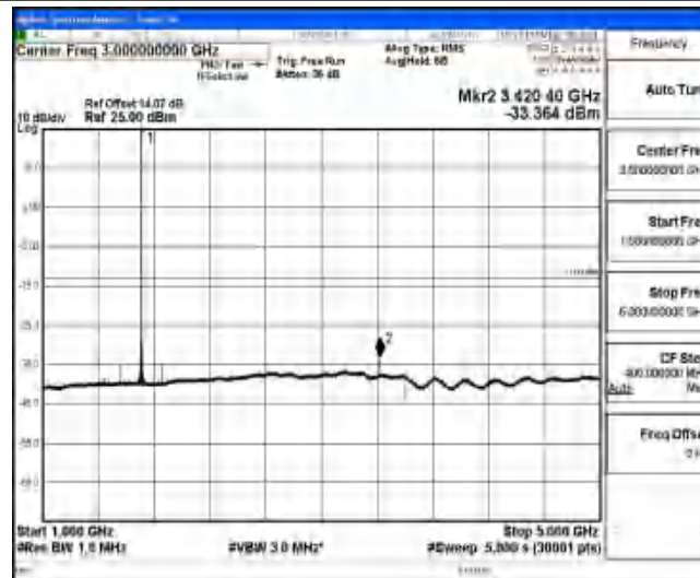
Band4-1.4MHz-QPSK-19957-1-0-Low-1000-5000--33.36-PASS
