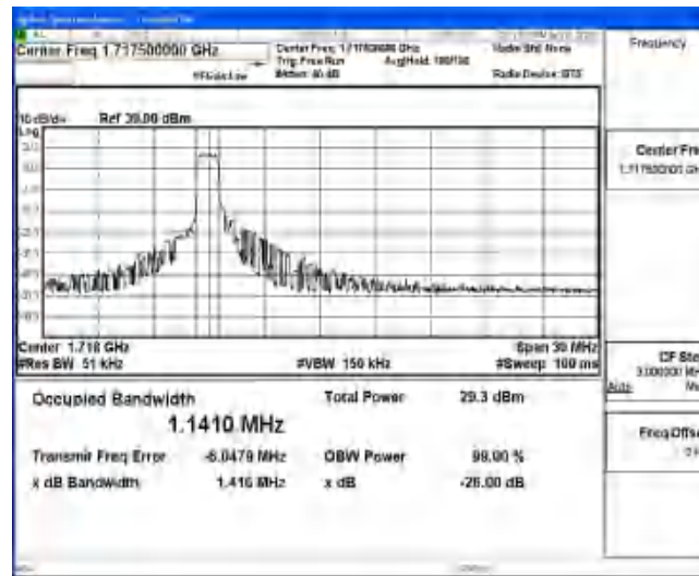
Band4-15MHz-QPSK-20025-6-0-Low-1.1410-1.416-PASS
