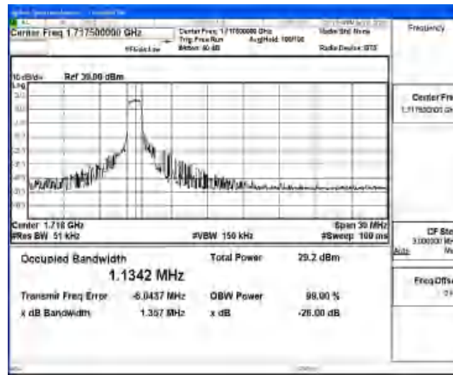
Band4-15MHz-16QAM-20025-6-0-Low-1.1342-1.357-PASS
