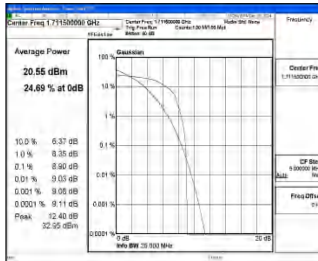
Band4-3MHz-16QAM-19965-1-0-Low-8.90-13-PASS
