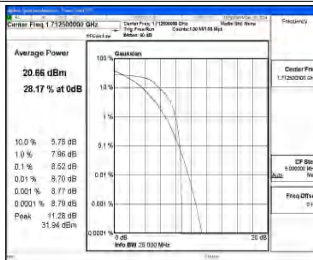
Band4-5MHz-16QAM-19975-6-0-Low-8.52-≤13-PASS
