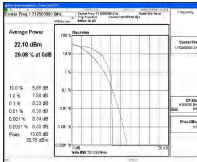
Band4-5MHz-16QAM-19975-1-0-Low-8.23-≤13-PASS
