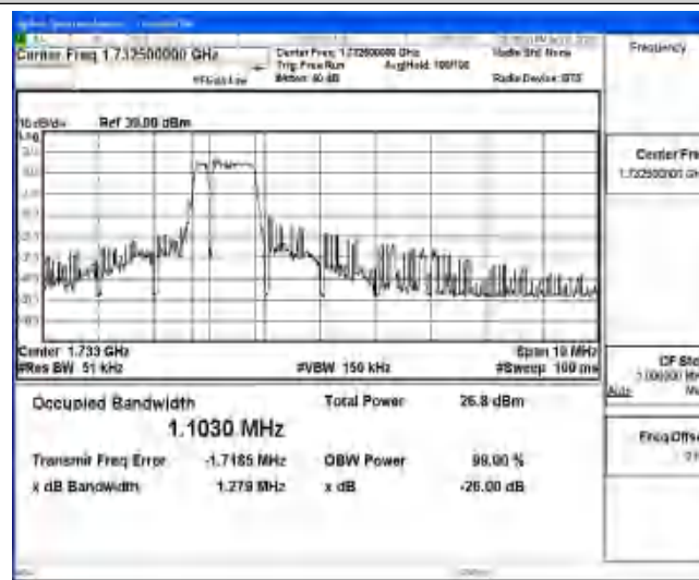
Band4-5MHz-16QAM-20175-6-0-Low-1.1030-1.279-PASS
