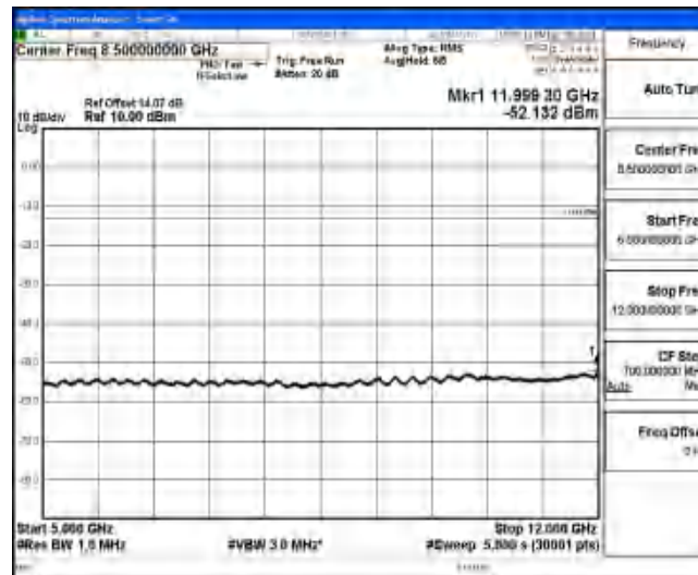
Band4-3MHz-QPSK-20175-1-0-Low-5000-12000--52.13-PASS
