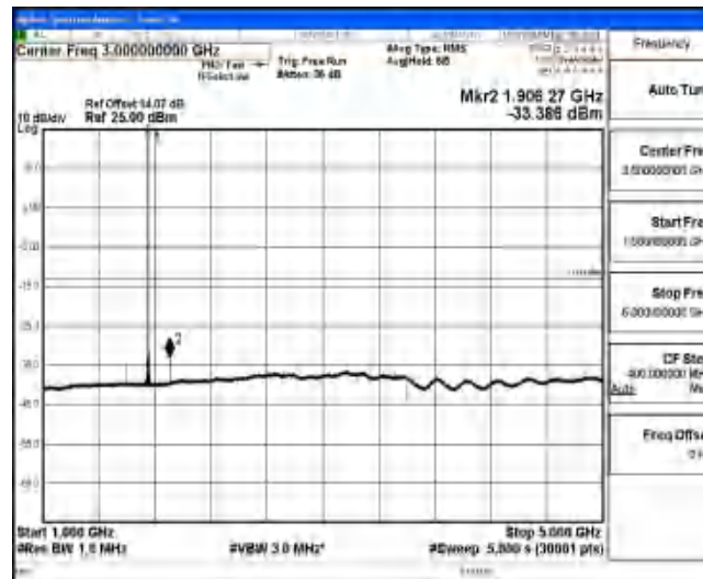
Band4-1.4MHz-QPSK-20393-1-0-High-1000-5000--33.39-PASS
