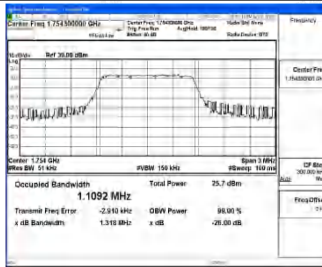
Band4-1.4MHz-QPSK-20393-6-0-High-1.1092-1.318-PASS
