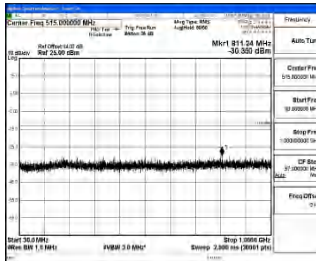
Band4-5MHz-QPSK-19975-1-0-Low-30-1000--30.35-PASS
