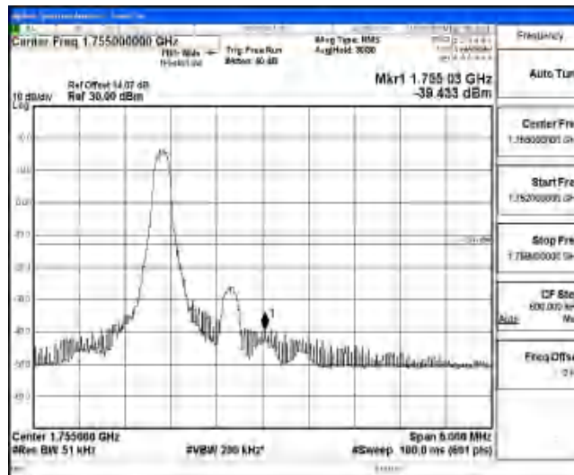
Band4-3MHz-16QAM-20385-1-0-High--39.43-PASS
