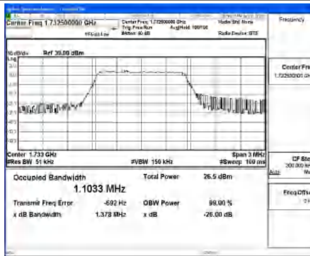
Band4-1.4MHz-QPSK-20175-6-0-Low-1.1033-1.378-PASS
