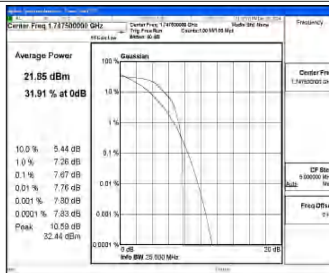
Band4-15MHz-QPSK-20325-1-0-High-7.67-13-PASS
