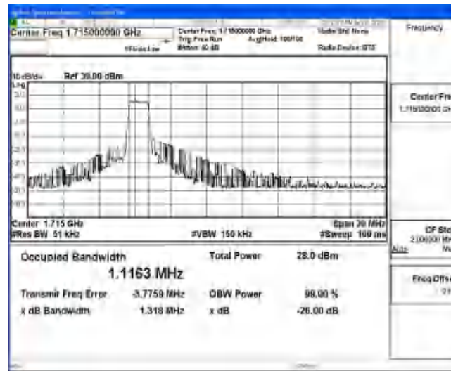
Band4-10MHz-QPSK-20000-6-0-Low-1.1163-1.318-PASS
