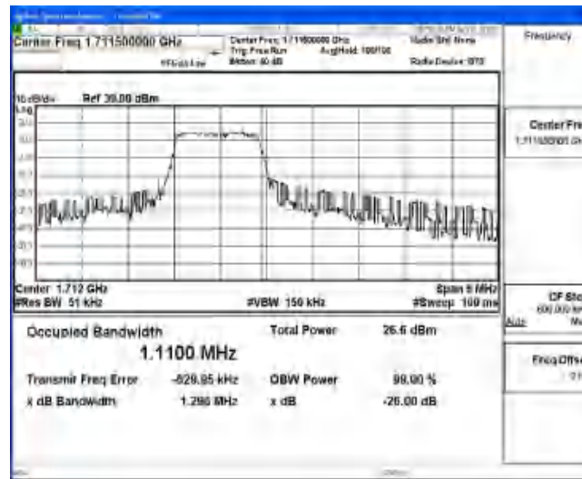
Band4-3MHz-16QAM-19965-6-0-Low-1.1100-1.296-PASS
