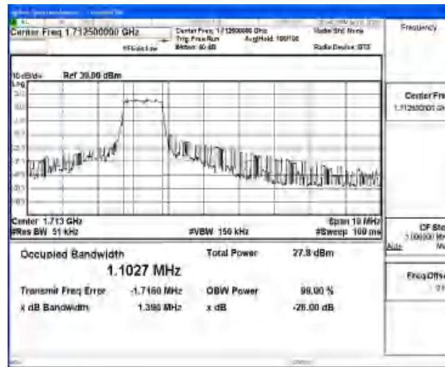
Band4-5MHz-QPSK-19975-6-0-Low-1.1027-1.396-PASS
