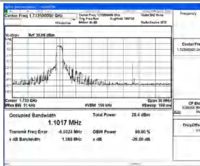
Band4-15MHz-QPSK-20175-6-0-Low-1.1017-1.388-PASS
