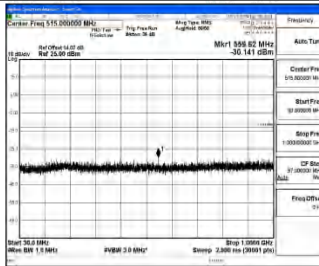
Band4-1.4MHz-QPSK-19957-1-0-Low-30-1000--30.14-PASS
