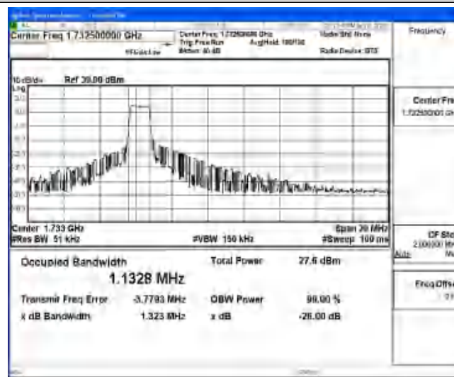
Band4-10MHz-QPSK-20175-6-0-Low-1.1328-1.323-PASS
