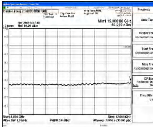
Band4-3MHz-16QAM-20175-1-0-Low-5000-12000--52.22-PASS
