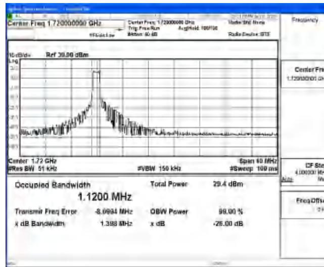
Band4-20MHz-QPSK-20050-6-0-Low-1.1200-1.398-PASS
