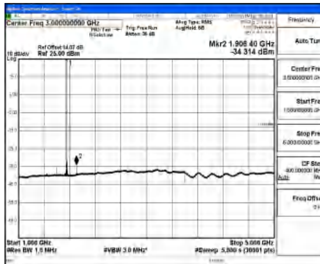
Band4-1.4MHz-16QAM-20393-1-0-High-1000-5000--34.31-PASS
