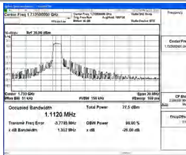
Band4-10MHz-16QAM-20175-6-0-Low-1.1120-1.352-PASS
