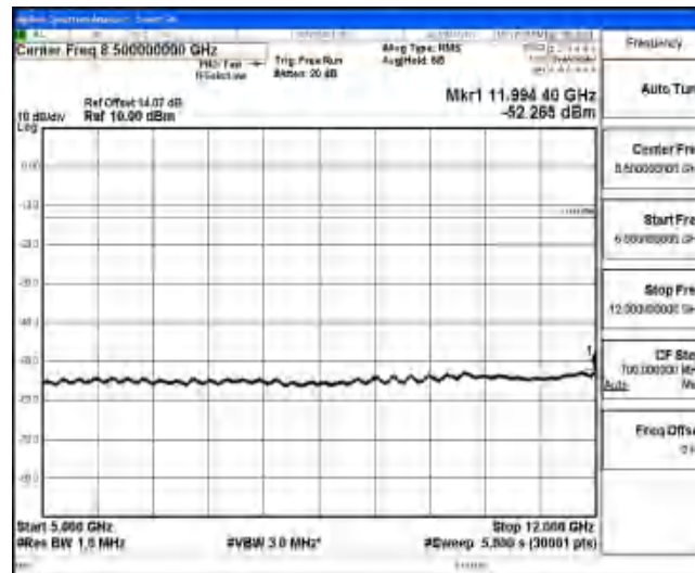
Band4-1.4MHz-QPSK-20175-1-0-Low-5000-12000--52.27-PASS
