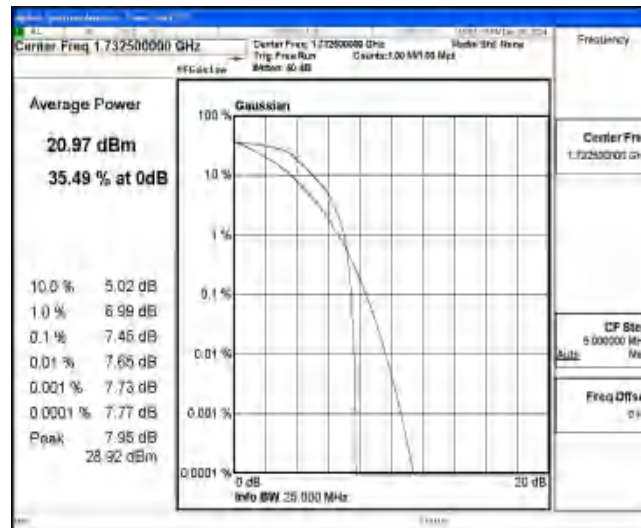
Band4-5MHz-16QAM-20175-6-0-Low-7.45-&lt;=13-PASS
