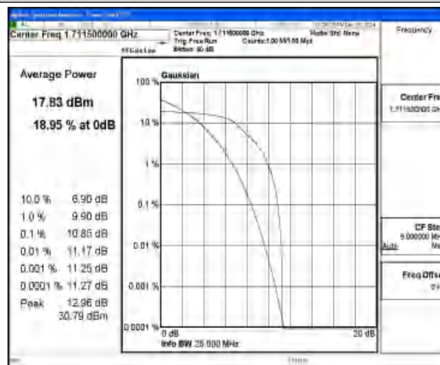
Band4-3MHz-16QAM-19965-6-0-Low-10.85-13-PASS
