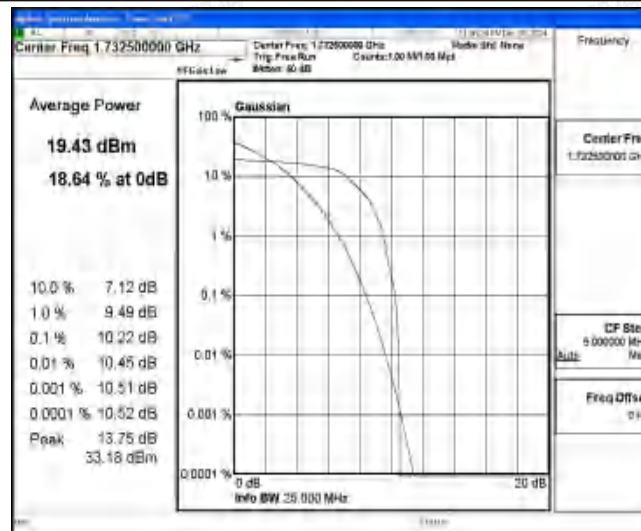
Band4-15MHz-QPSK-20175-1-0-Low-10.22-13-PASS
