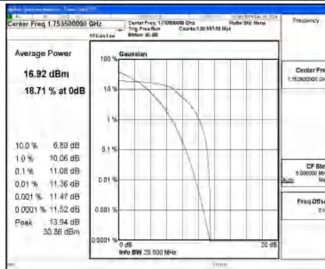
Band4-3MHz-QPSK-20385-6-0-High-11.08-13-PASS
