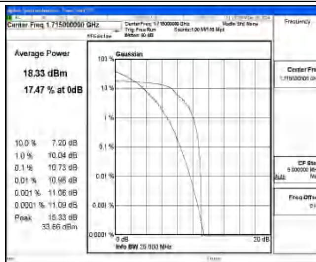
Band4-10MHz-QPSK-20000-6-0-Low-10.73-13-PASS
