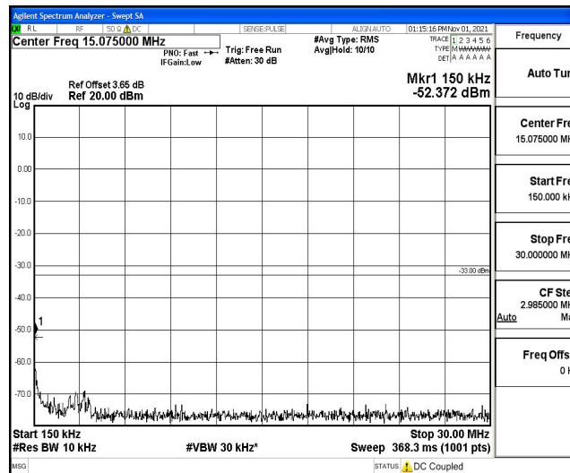
Band26-5MHz-16QAM-26815-1RB#0-Range3:30~1000MHz
