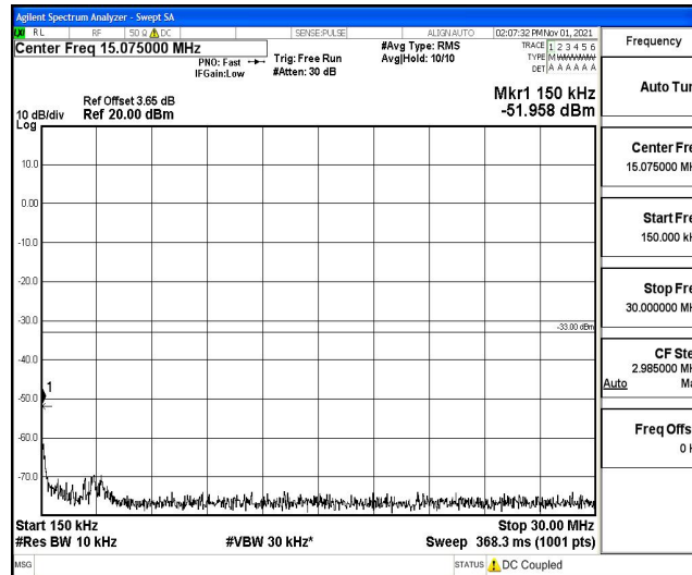
Band26-15MHz-QPSK-26865-1RB#0-Range3:30~1000MHz
