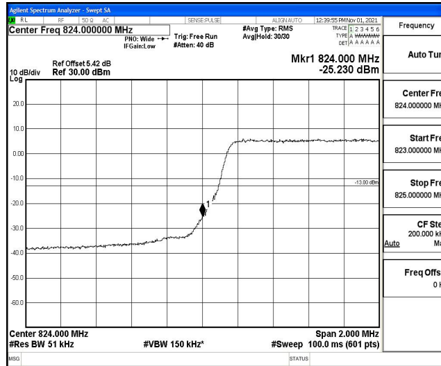
Band26-3MHz-QPSK-27025-15RB#0
