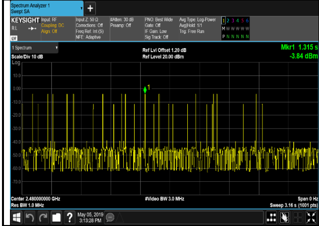
GFSK,2480,DH5,Transmission Number
