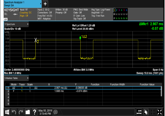
GFSK,2480,DH5,Transmission Time
