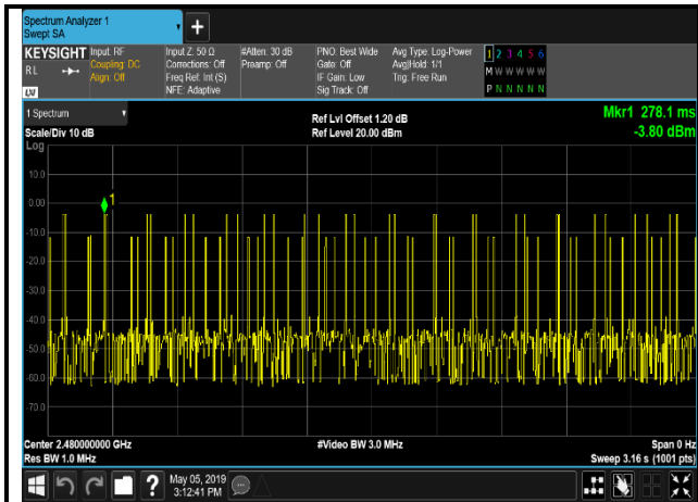
GFSK,2480,DH3,Transmission Number
