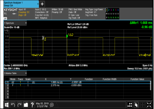
GFSK,2480,DH5,Transmission Time
