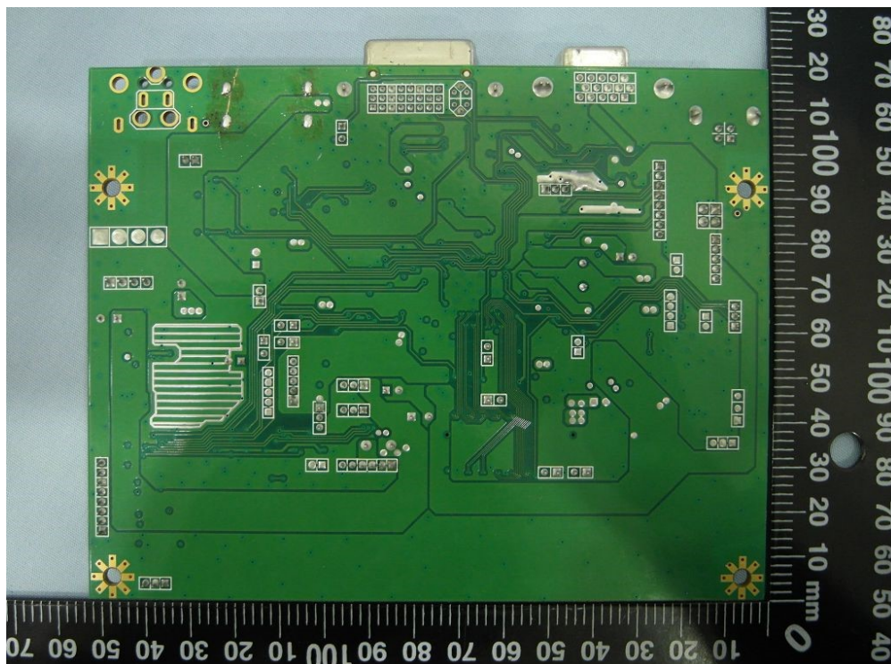
(29) EUT Photo
