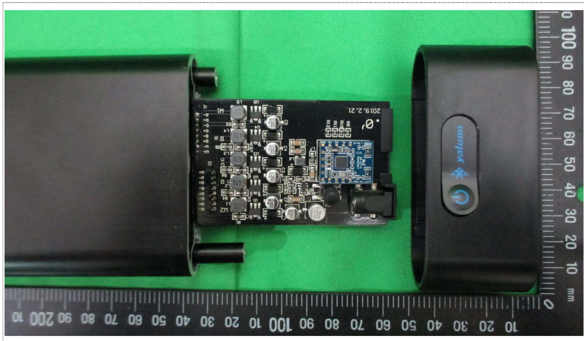
Inner View of EUT-3
