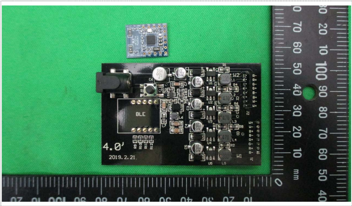
Inner View of EUT-5
