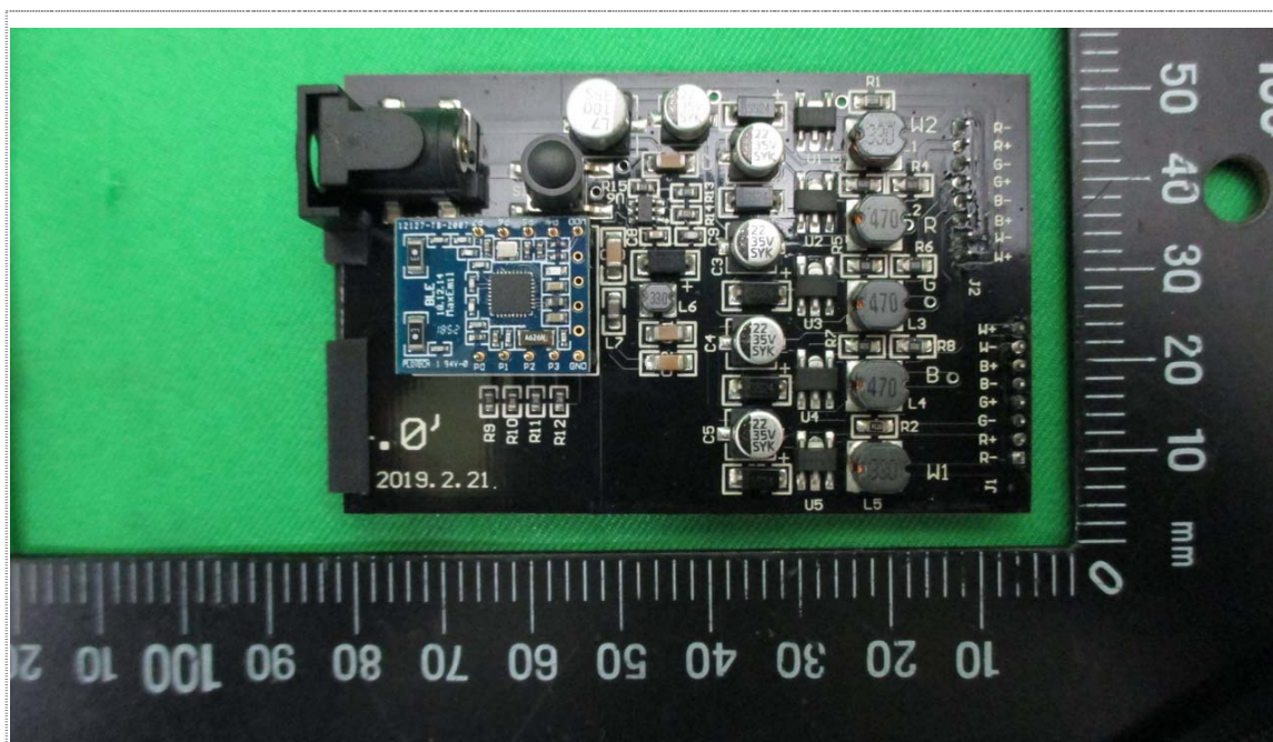
Front View of Main Board
