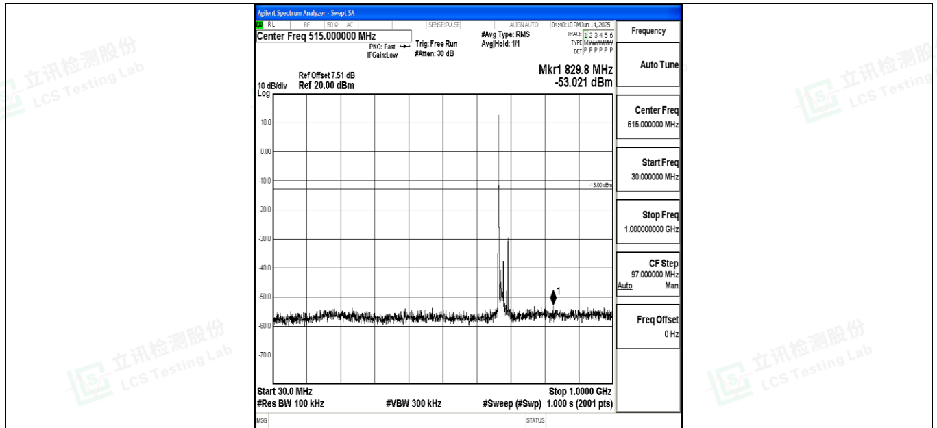
Band71_15MHz_QPSK_133297_1RB#0_30~1000_30~1000
