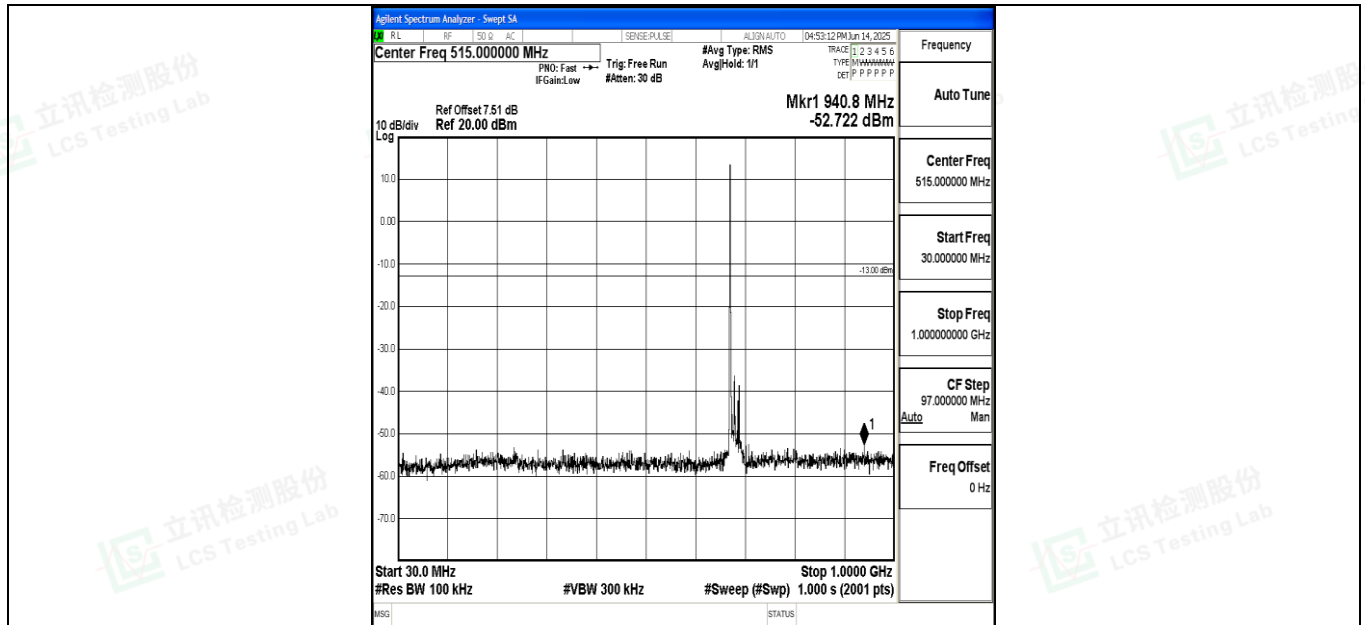
Band71_20MHz_QPSK_133372_1RB#0_30~1000_30~1000
