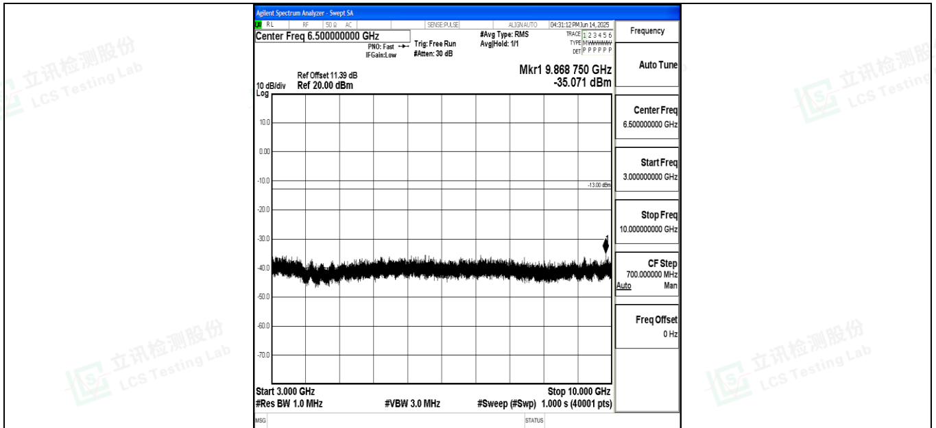
Band71_10MHz_QPSK_133297_1RB#0_3000~10000_3000~10000
