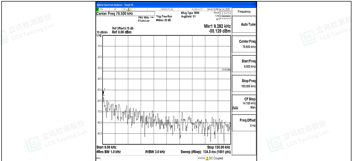
Band71_15MHz_QPSK_133397_1RB#0_0.009~0.15_0.009~0.15
