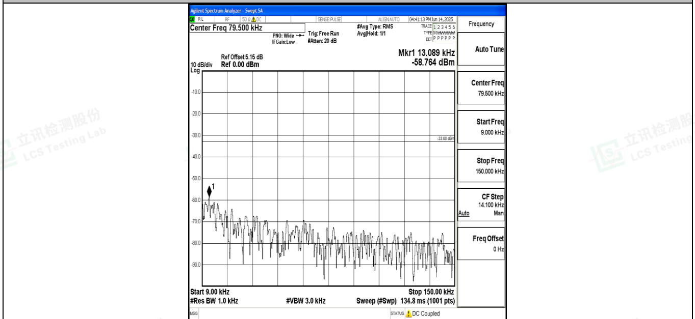
Band71_15MHz_16QAM_133297_1RB#0_0.009~0.15_0.009~0.15
