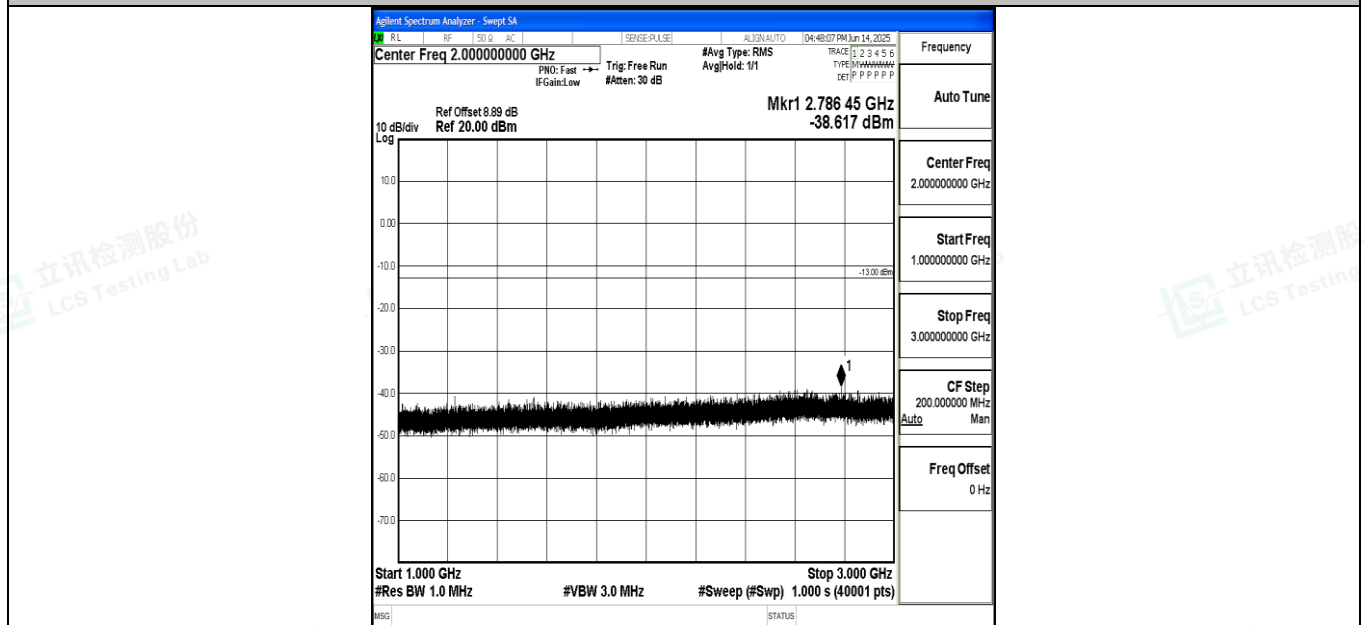
Band71_20MHz_QPSK_133222_1RB#0_1000~3000_1000~3000
