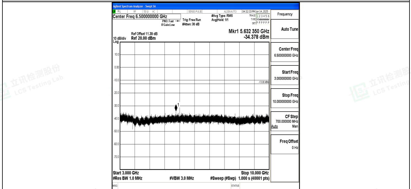
Band71_10MHz_16QAM_133297_1RB#0_3000~10000_3000~10000
