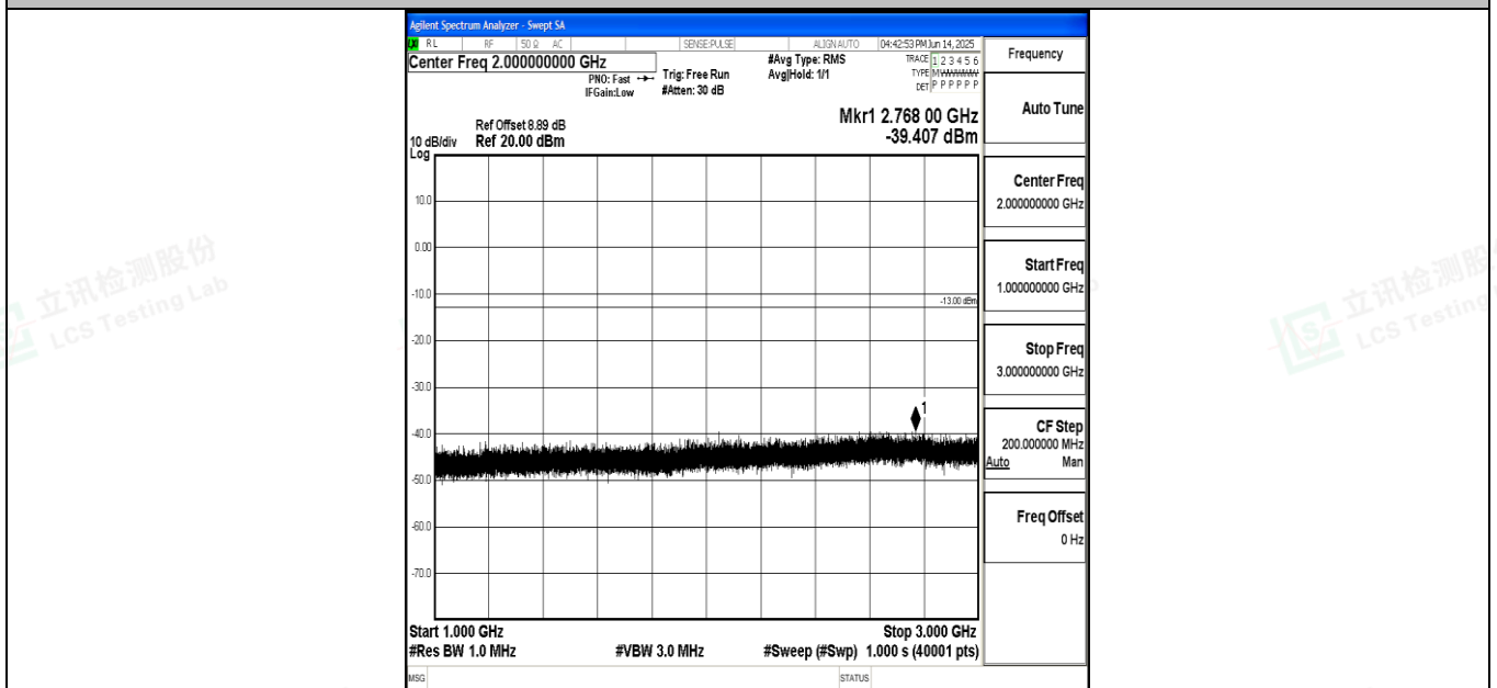
Band71_15MHz_QPSK_133397_1RB#0_1000~3000_1000~3000
