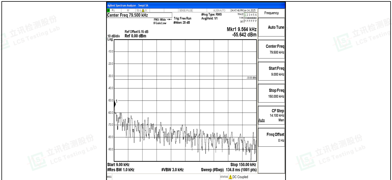
Band71_20MHz_QPSK_133222_1RB#0_0.009~0.15_0.009~0.15
