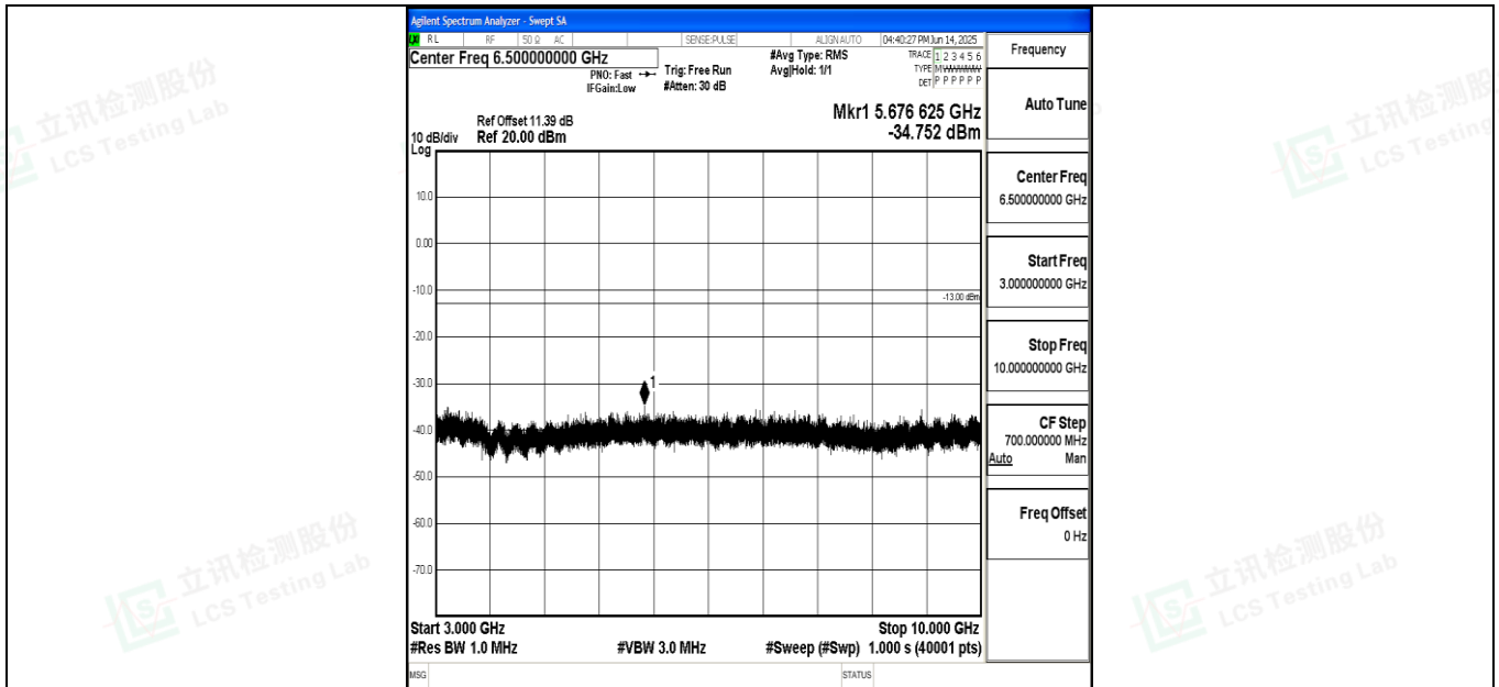
Band71_15MHz_QPSK_133297_1RB#0_3000~10000_3000~10000
