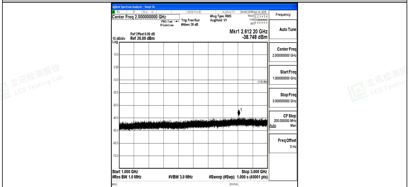
Band71_15MHz_QPSK_133297_1RB#0_1000~3000_1000~3000
