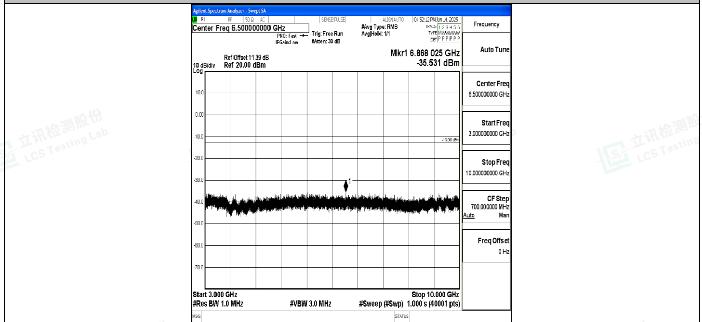
Band71_20MHz_16QAM_133322_1RB#0_3000~10000_3000~10000
