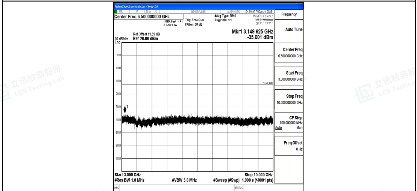
Band71_20MHz_16QAM_133372_1RB#0_3000~10000_3000~10000
