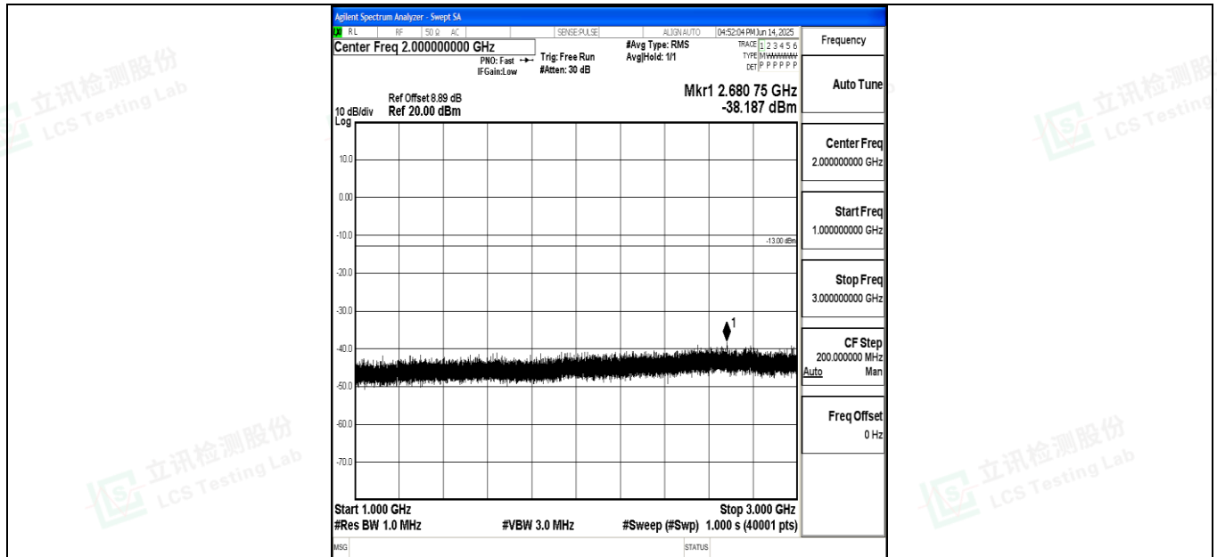
Band71_20MHz_16QAM_133322_1RB#0_1000~3000_1000~3000
