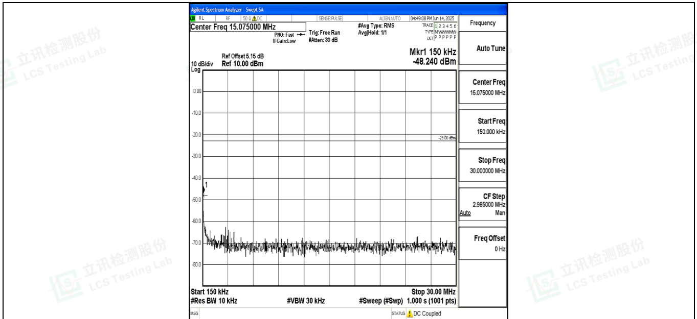
Band71_20MHz_16QAM_133222_1RB#0_0.15~30_0.15~30
