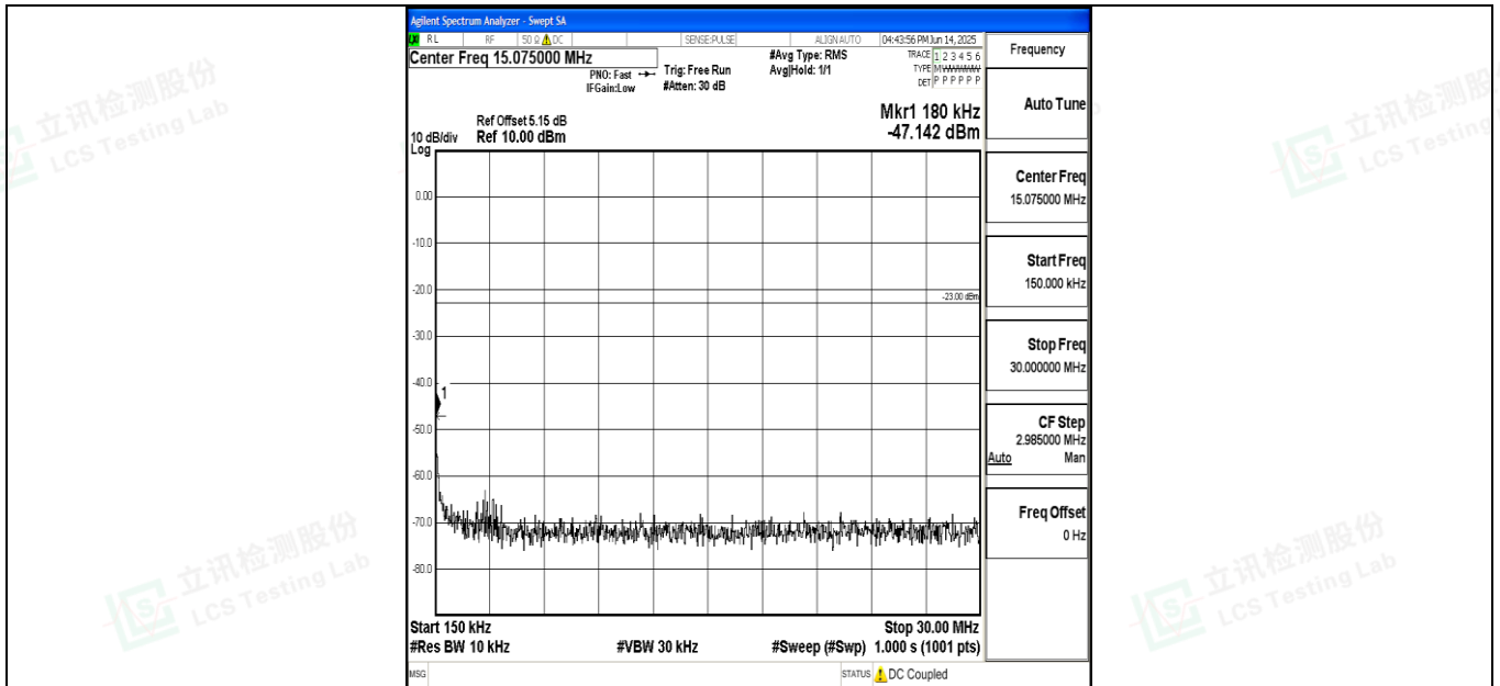
Band71_15MHz_16QAM_133397_1RB#0_0.15~30_0.15~30
