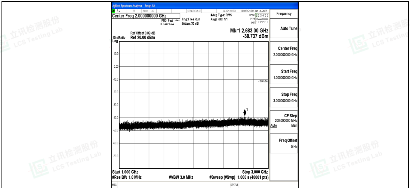
Band71_20MHz_16QAM_133222_1RB#0_1000~3000_1000~3000
