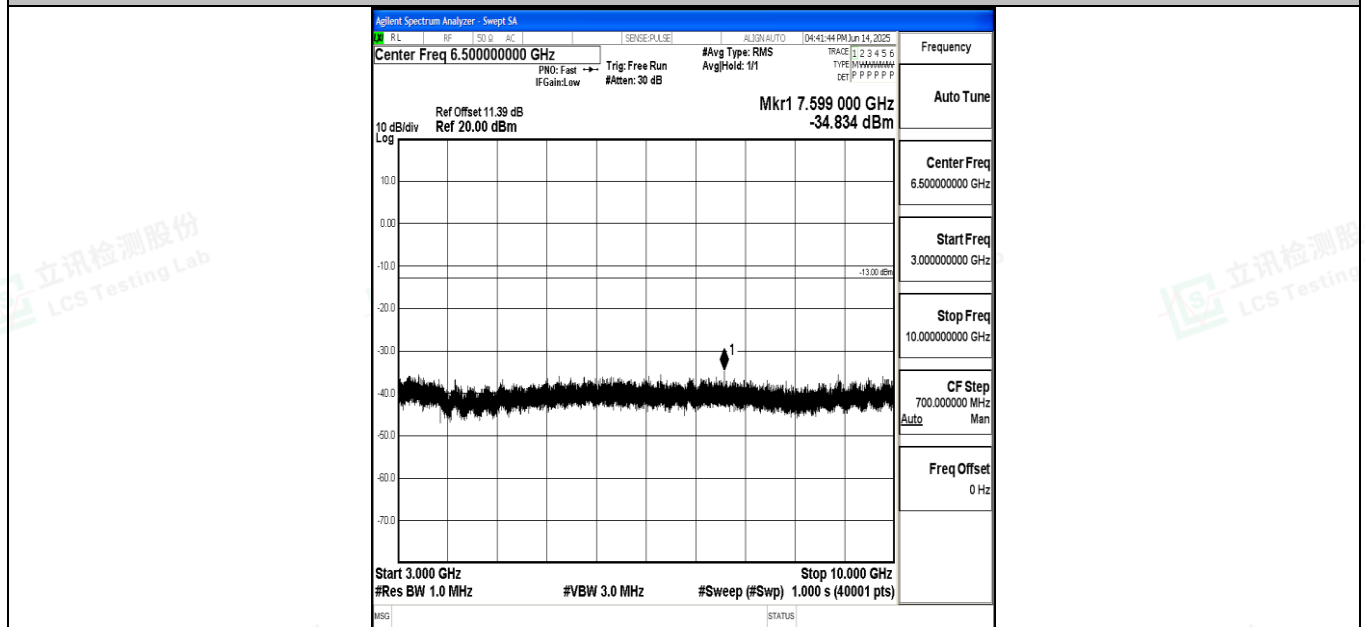
Band71_15MHz_16QAM_133297_1RB#0_3000~10000_3000~10000
