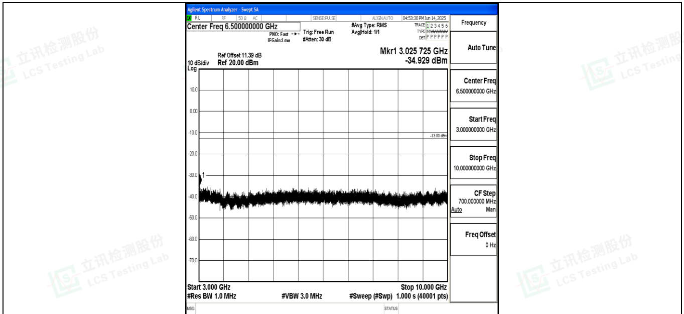
Band71_20MHz_QPSK_133372_1RB#0_3000~10000_3000~10000
