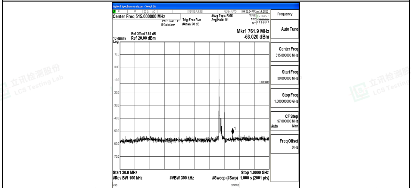
Band71_20MHz_16QAM_133322_1RB#0_30~1000_30~1000
