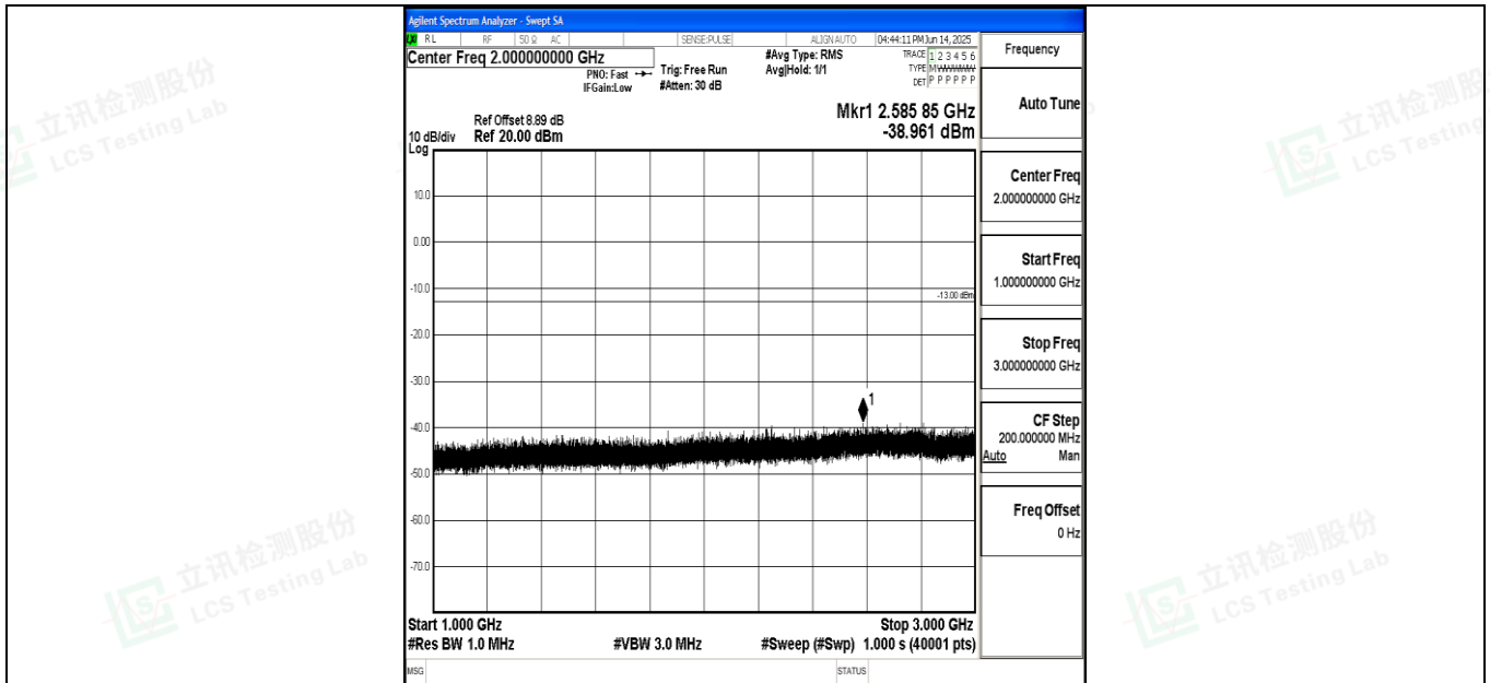
Band71_15MHz_16QAM_133397_1RB#0_1000~3000_1000~3000
