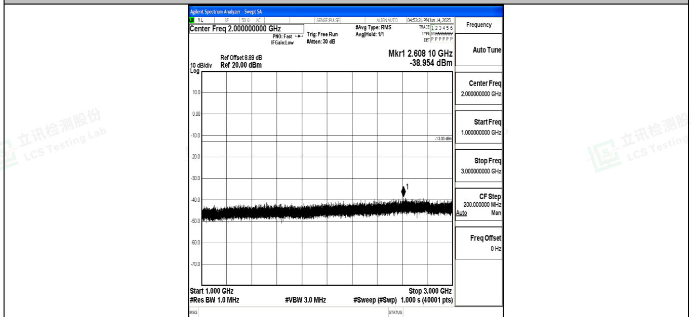
Band71_20MHz_QPSK_133372_1RB#0_1000~3000_1000~3000
