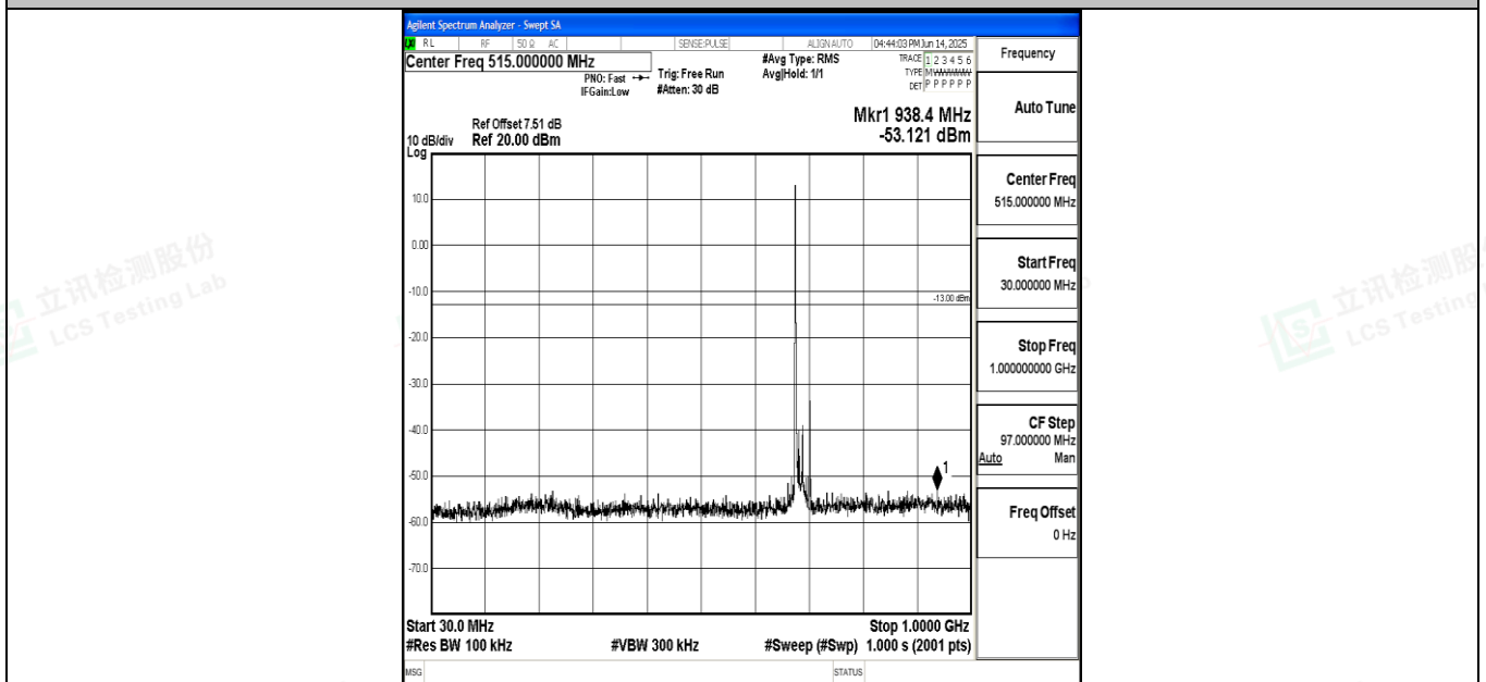
Band71_15MHz_16QAM_133397_1RB#0_30~1000_30~1000
