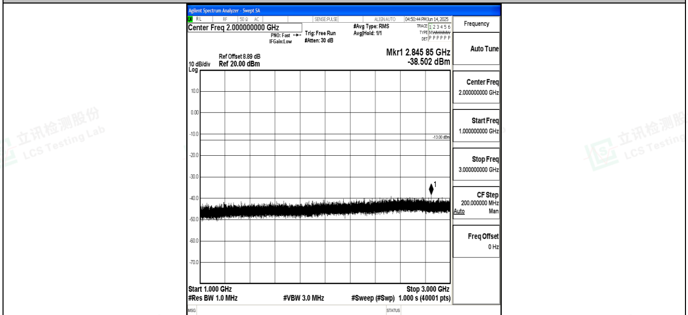
Band71_20MHz_QPSK_133322_1RB#0_1000~3000_1000~3000
