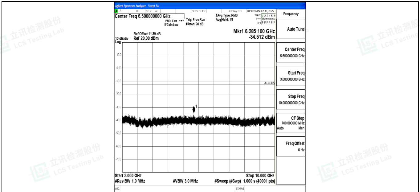
Band71_20MHz_QPSK_133222_1RB#0_3000~10000_3000~10000
