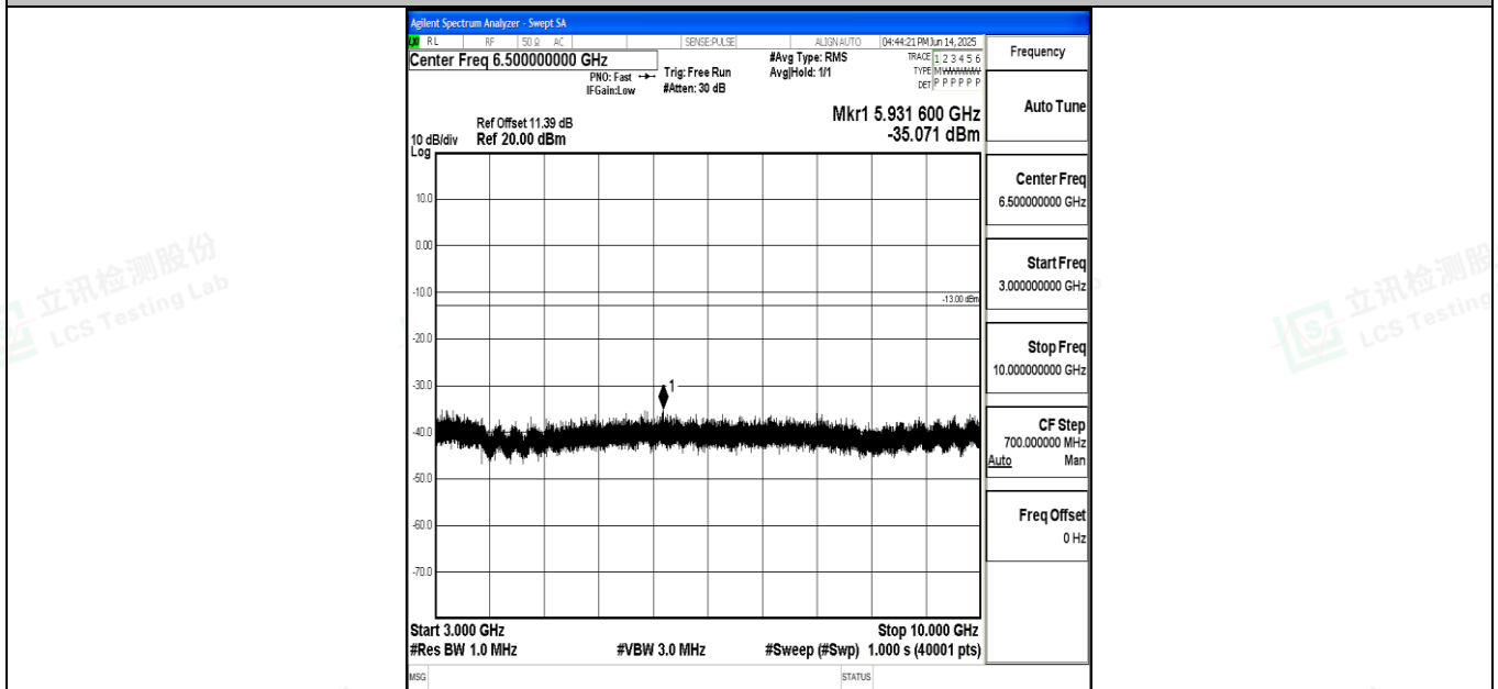
Band71_15MHz_16QAM_133397_1RB#0_3000~10000_3000~10000
