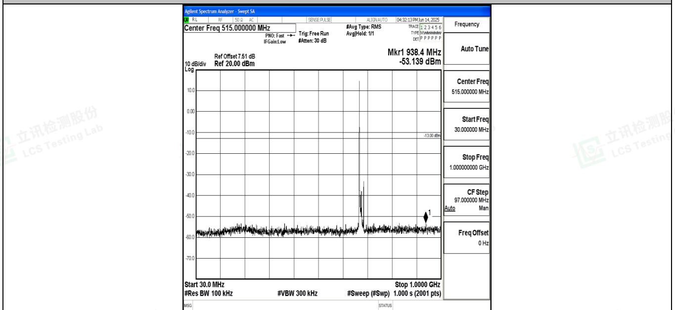
Band71_10MHz_16QAM_133297_1RB#0_30~1000_30~1000
