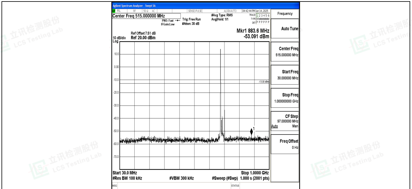
Band71_15MHz_QPSK_133397_1RB#0_30~1000_30~1000
