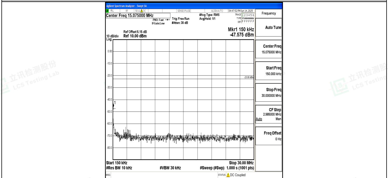
Band71_20MHz_QPSK_133222_1RB#0_0.15~30_0.15~30
