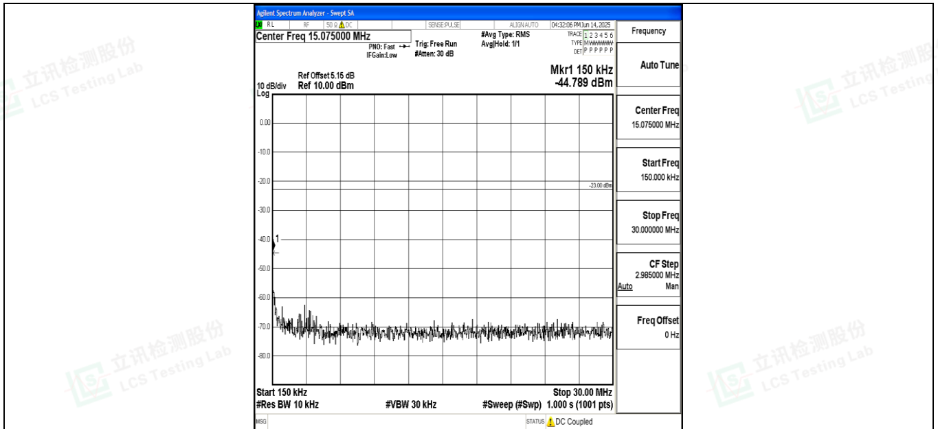
Band71_10MHz_16QAM_133297_1RB#0_0.15~30_0.15~30
