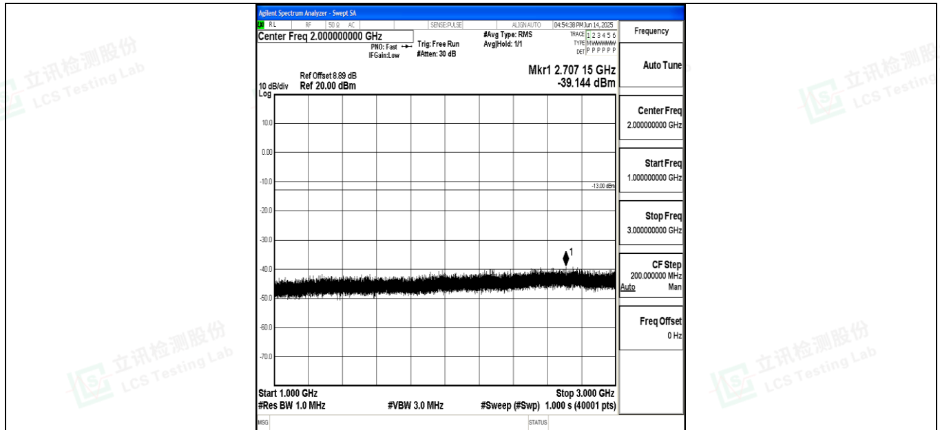
Band71_20MHz_16QAM_133372_1RB#0_1000~3000_1000~3000
