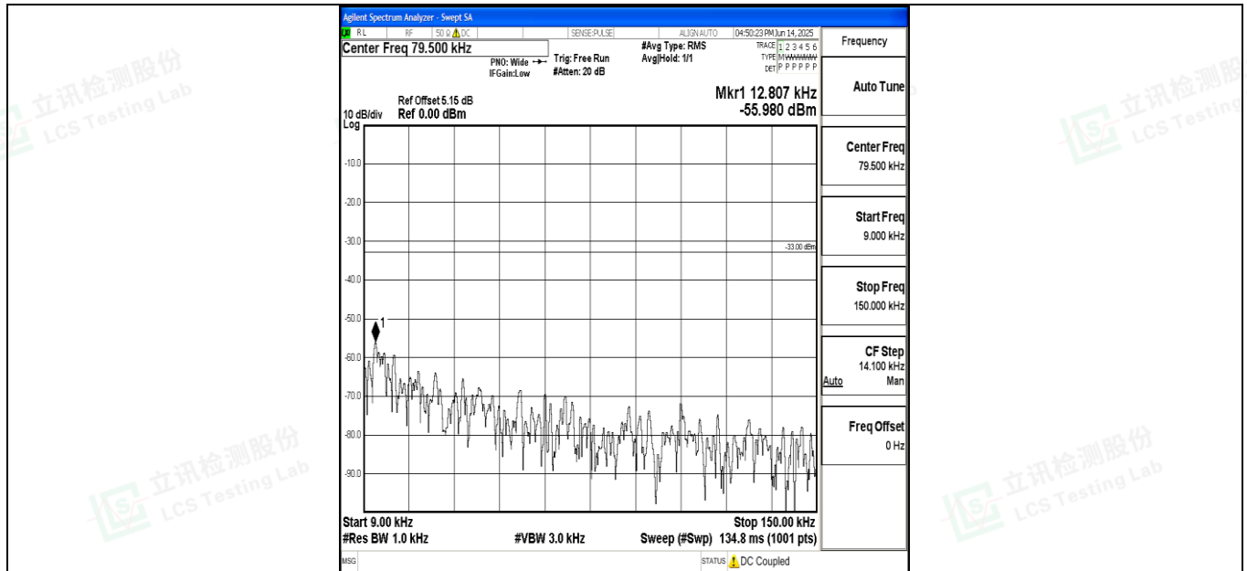
Band71_20MHz_QPSK_133322_1RB#0_0.009~0.15_0.009~0.15
