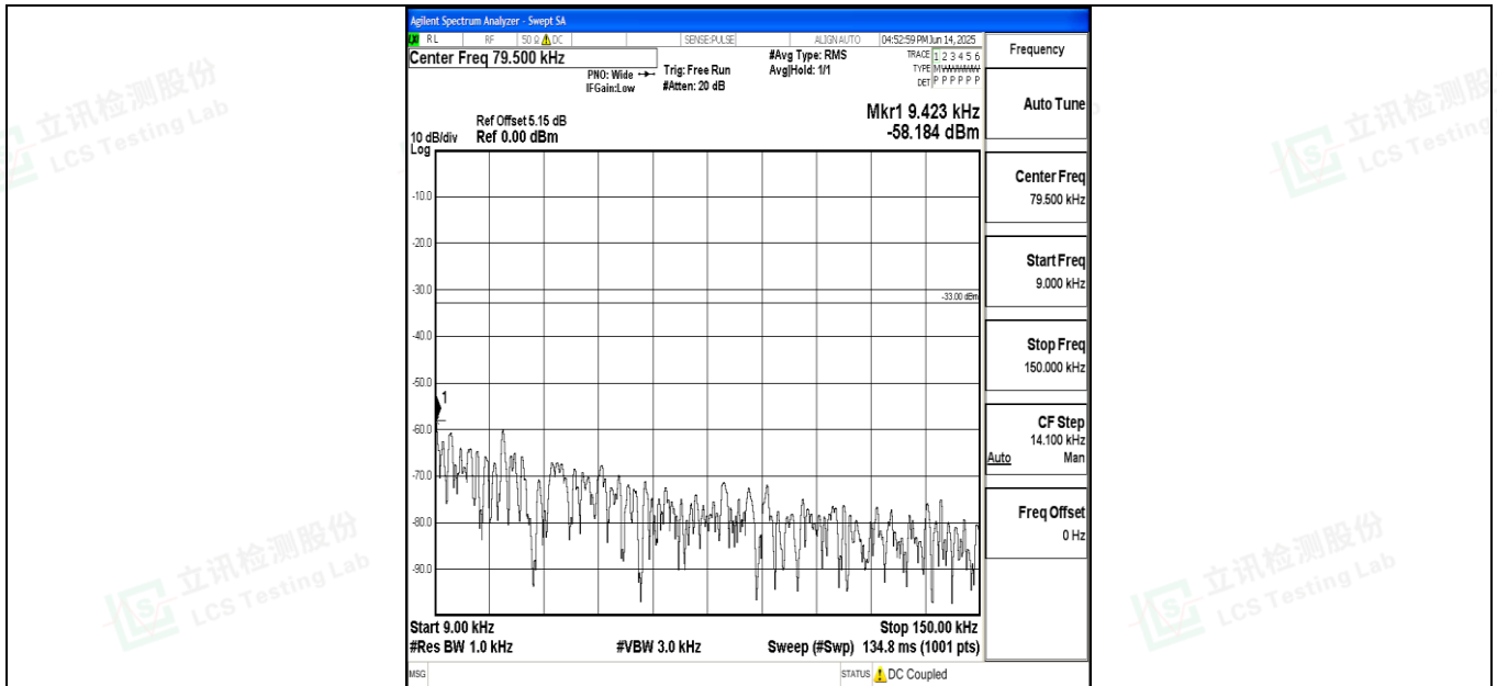
Band71_20MHz_QPSK_133372_1RB#0_0.009~0.15_0.009~0.15
