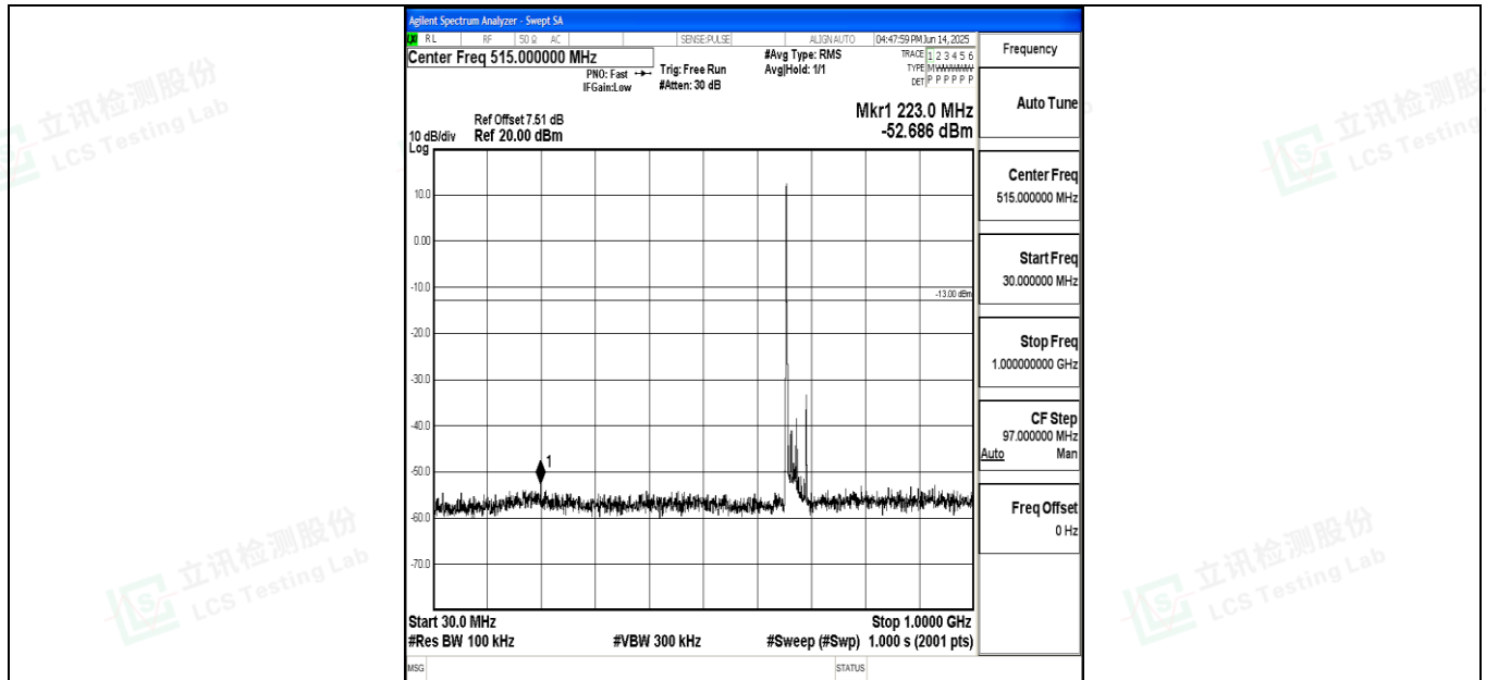
Band71_20MHz_QPSK_133222_1RB#0_30~1000_30~1000
