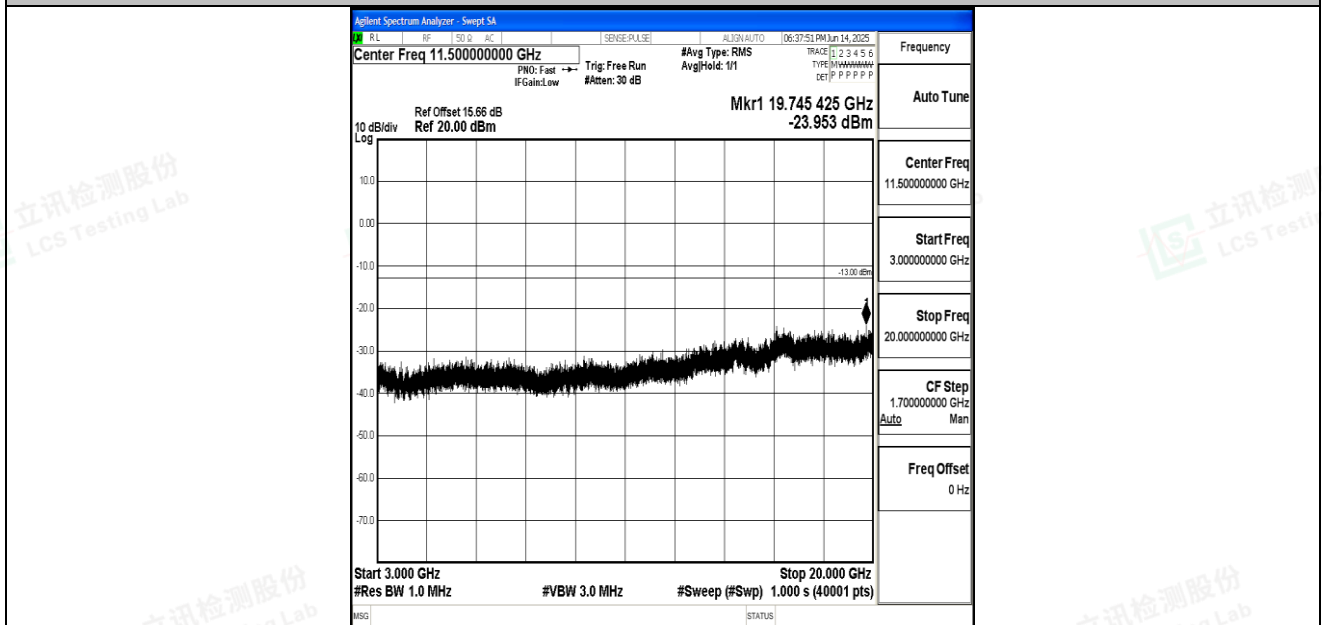
Band66_15MHz_16QAM_132597_1RB#0_3000~20000_3000~20000
