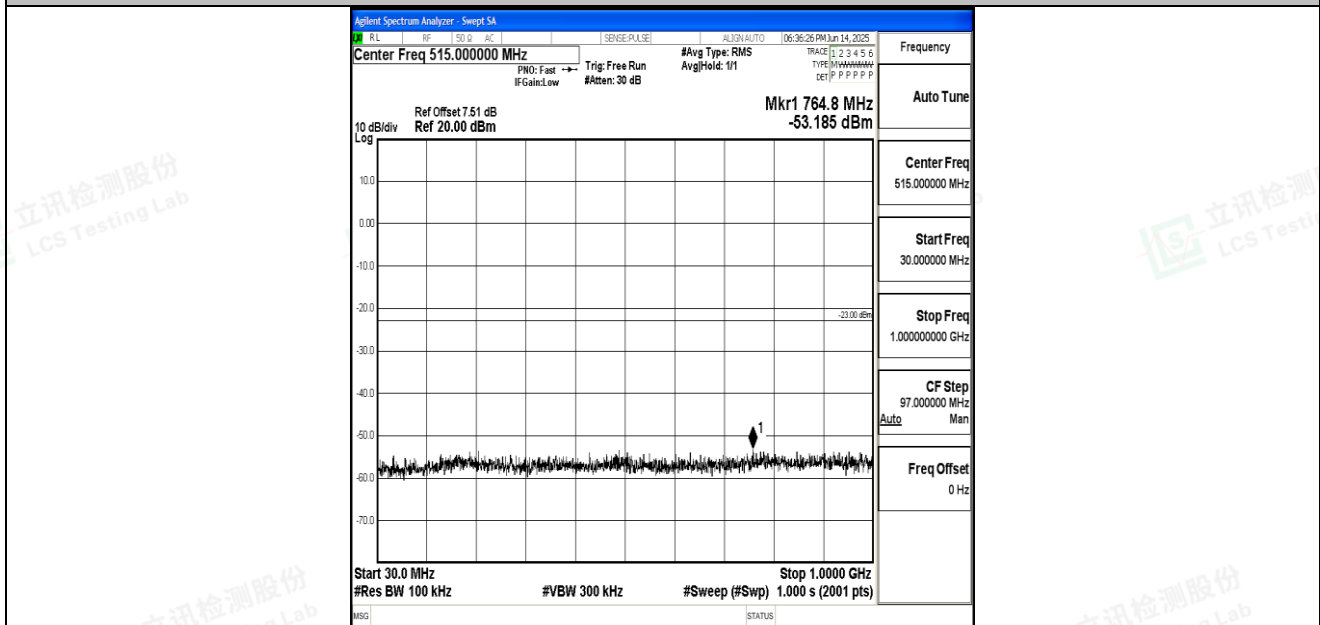
Band66_15MHz_16QAM_132322_1RB#0_30~1000_30~1000
