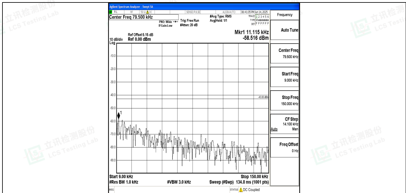
Band66_20MHz_QPSK_132572_1RB#0_0.009~0.15_0.009~0.15
