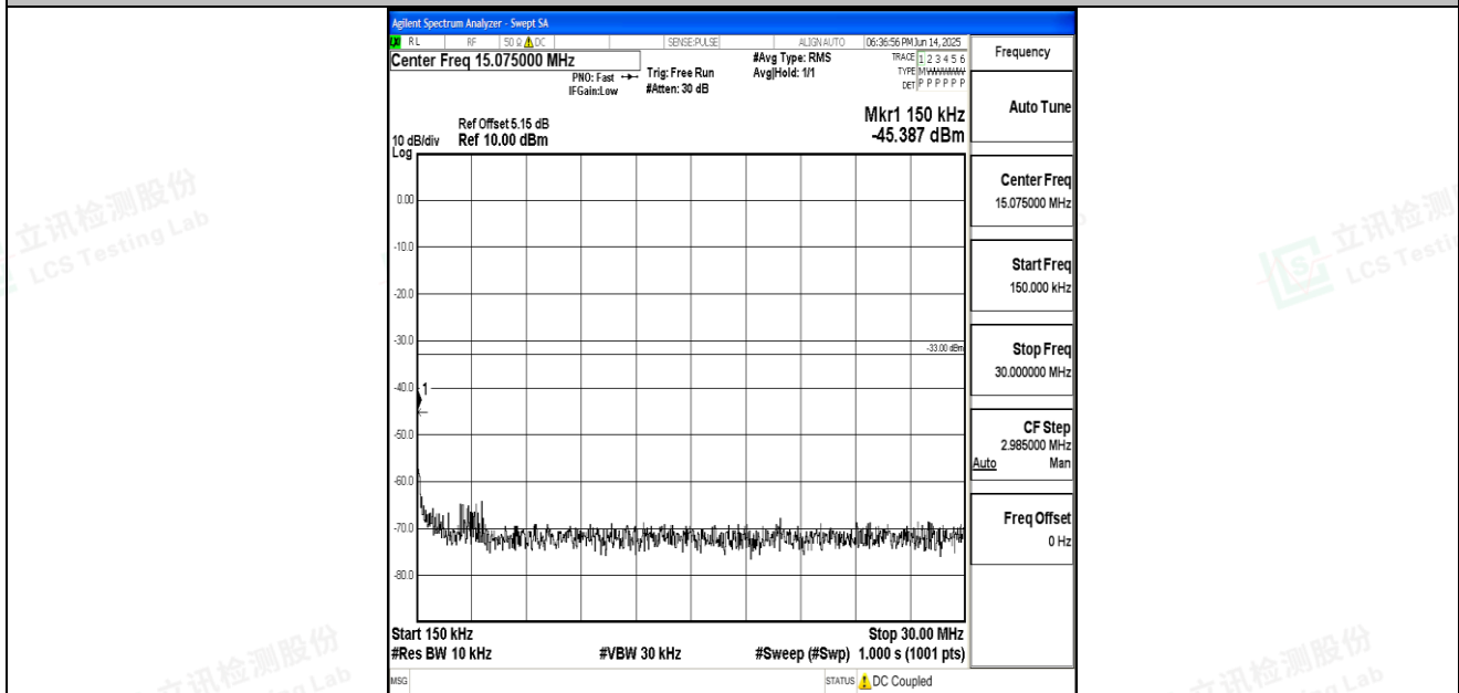
Band66_15MHz_QPSK_132597_1RB#0_0.15~30_0.15~30
