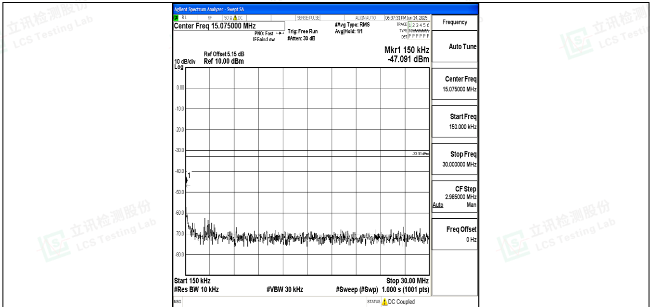
Band66_15MHz_16QAM_132597_1RB#0_0.15~30_0.15~30
