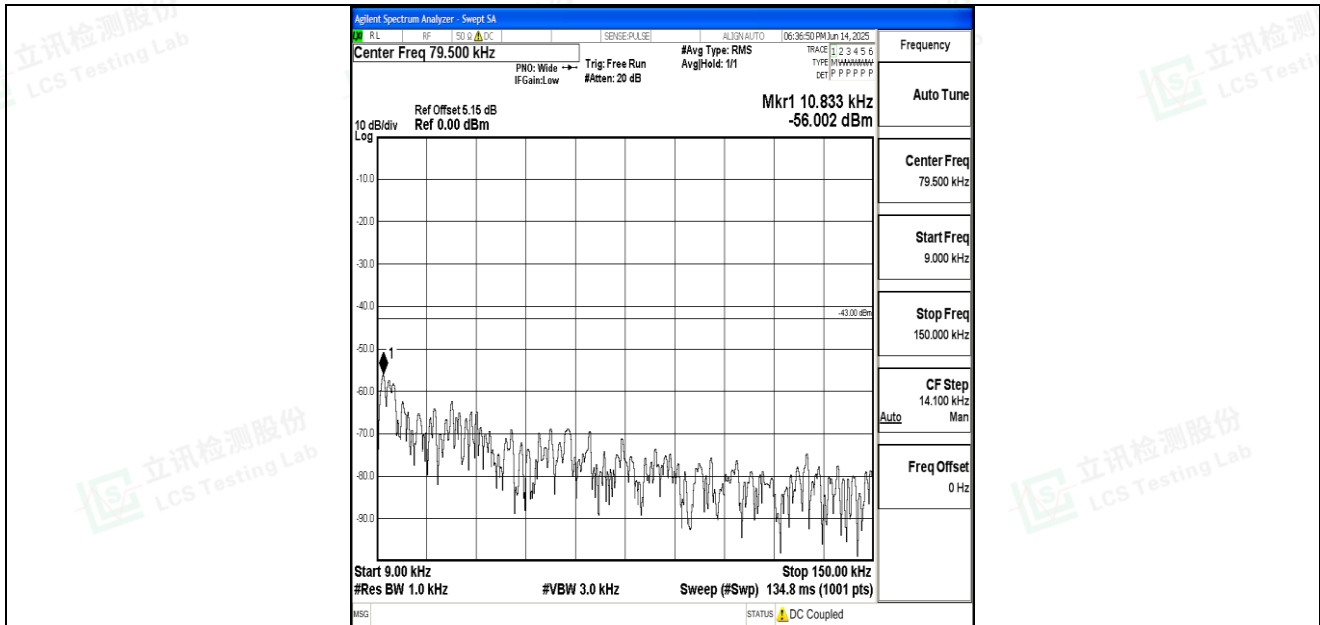
Band66_15MHz_QPSK_132597_1RB#0_0.009~0.15_0.009~0.15
