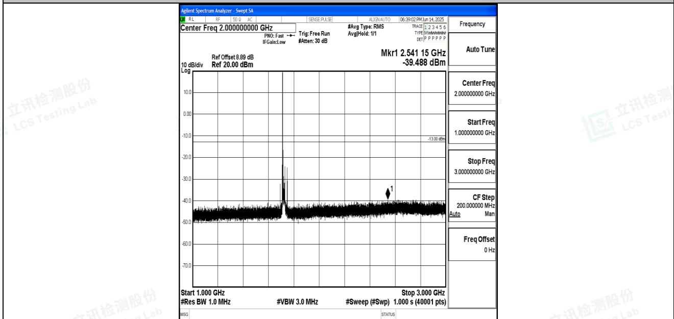
Band66_20MHz_QPSK_132072_1RB#0_1000~3000_1000~3000
