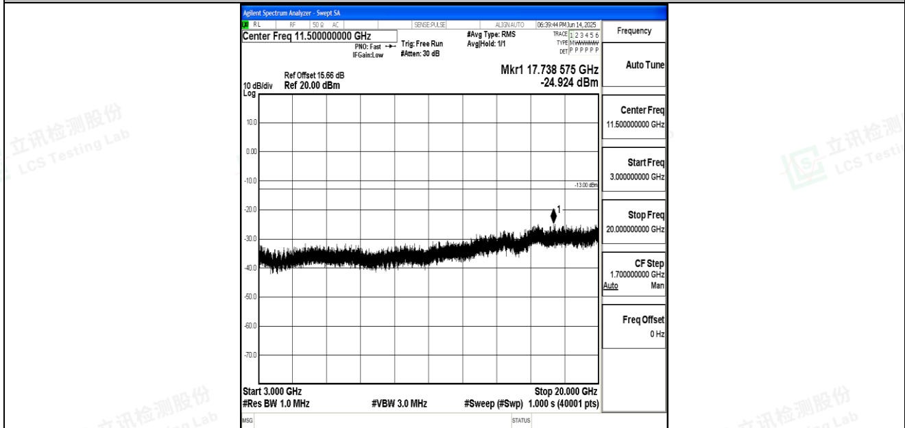
Band66_20MHz_16QAM_132072_1RB#0_3000~20000_3000~20000
