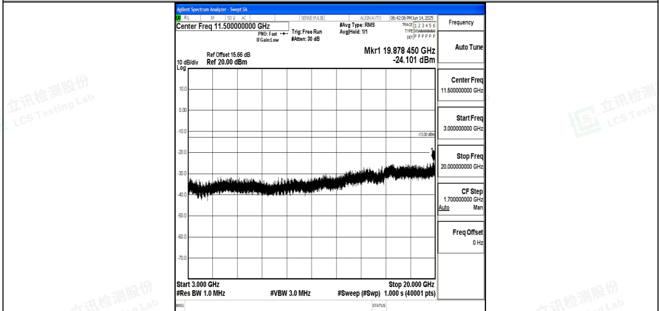
Band66_20MHz_16QAM_132572_1RB#0_3000~20000_3000~20000
