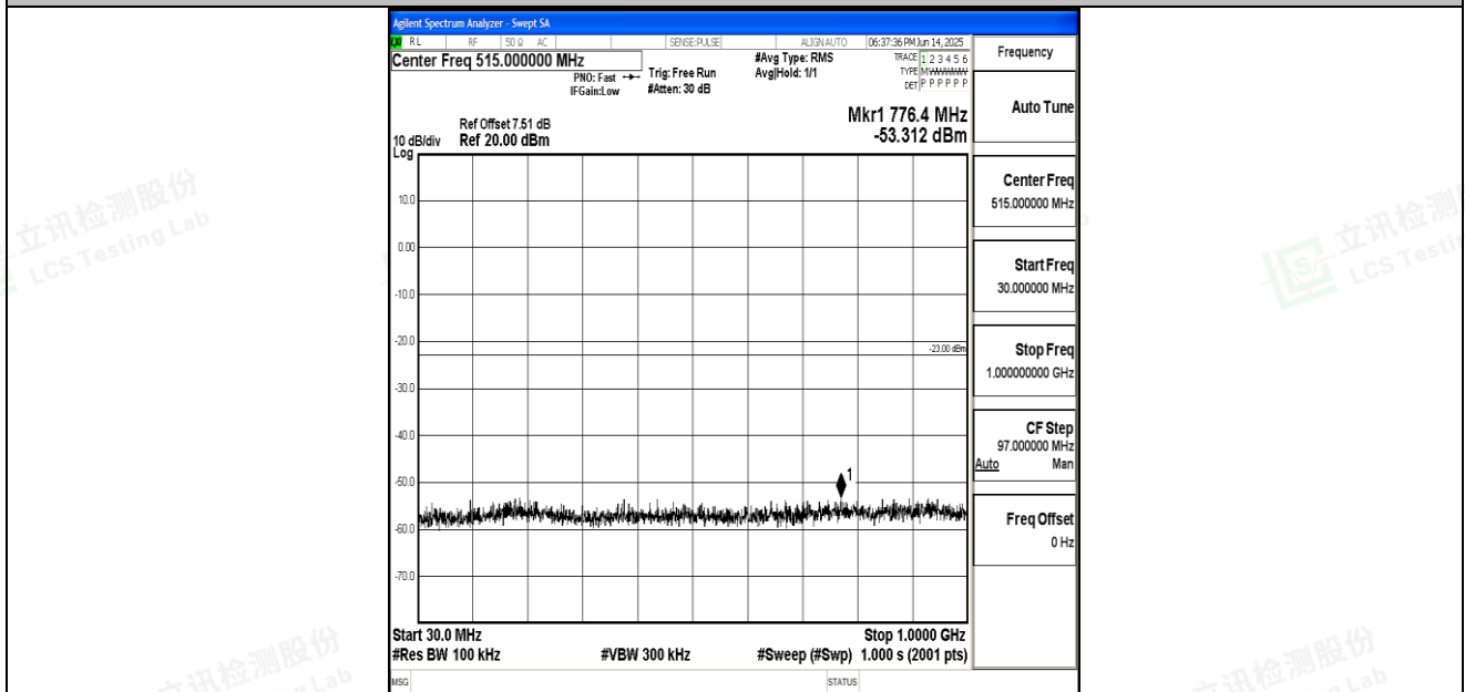
Band66_15MHz_16QAM_132597_1RB#0_30~1000_30~1000
