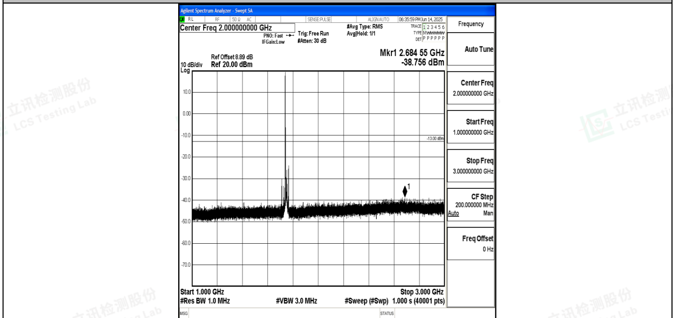
Band66_15MHz_QPSK_132322_1RB#0_1000~3000_1000~3000
