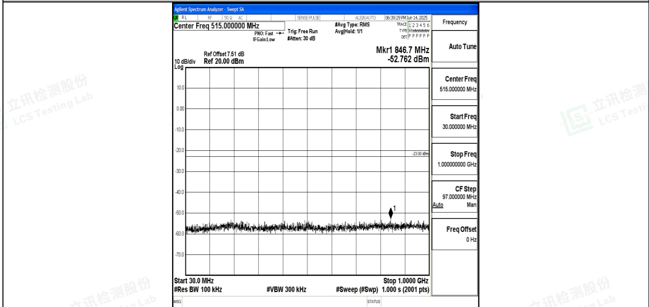
Band66_20MHz_16QAM_132072_1RB#0_30~1000_30~1000
