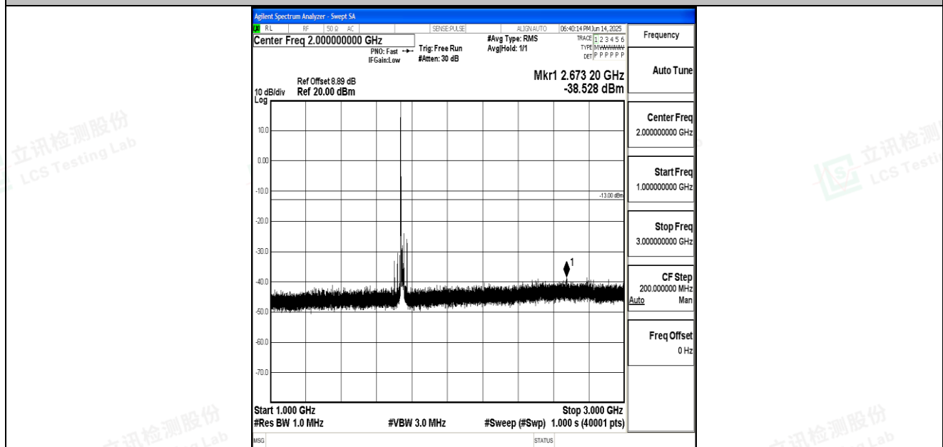
Band66_20MHz_QPSK_132322_1RB#0_1000~3000_1000~3000
