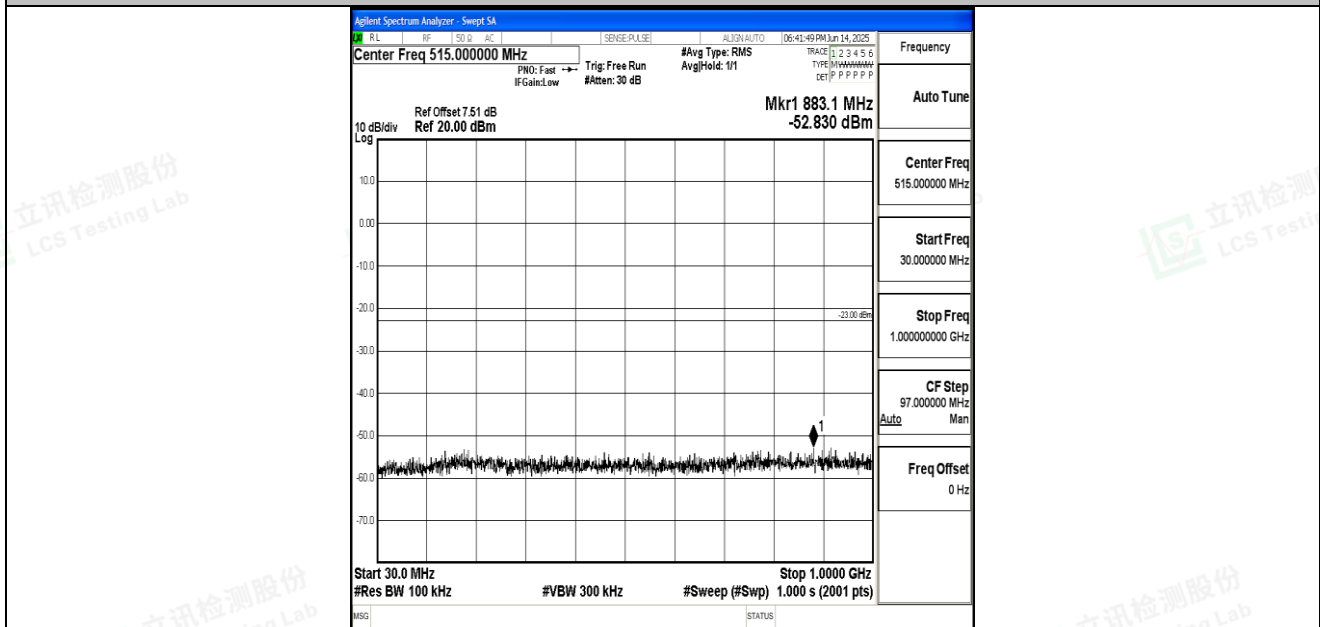
Band66_20MHz_16QAM_132572_1RB#0_30~1000_30~1000
