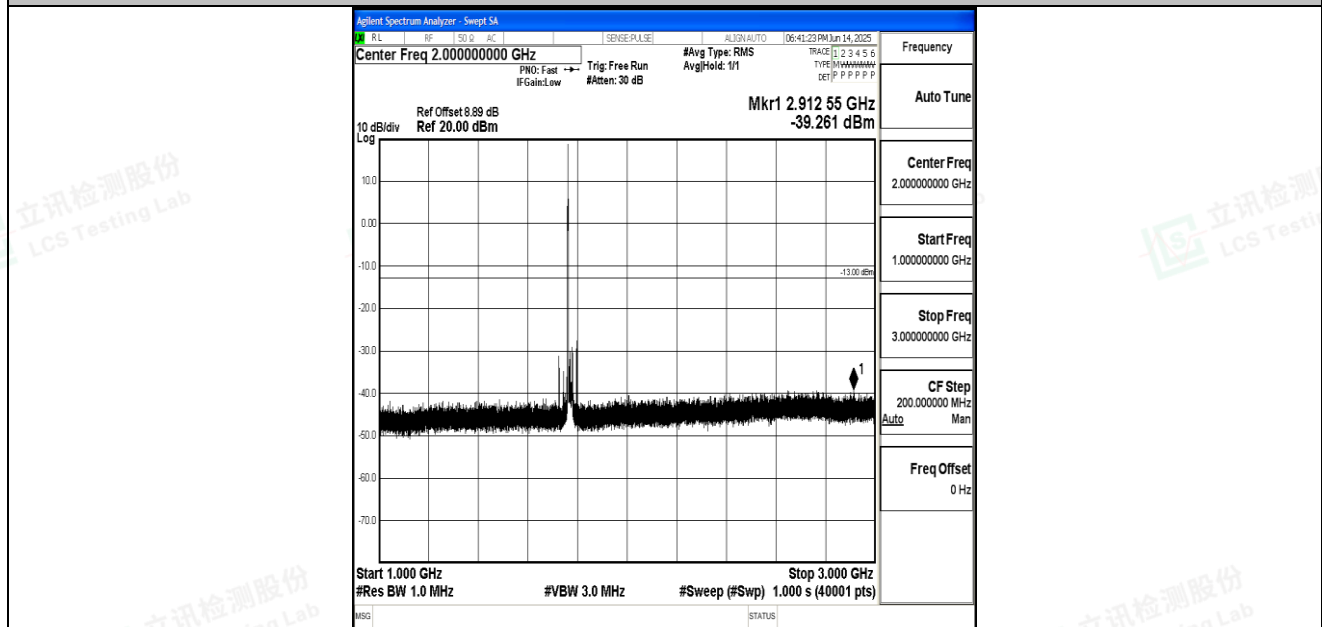
Band66_20MHz_QPSK_132572_1RB#0_1000~3000_1000~3000
