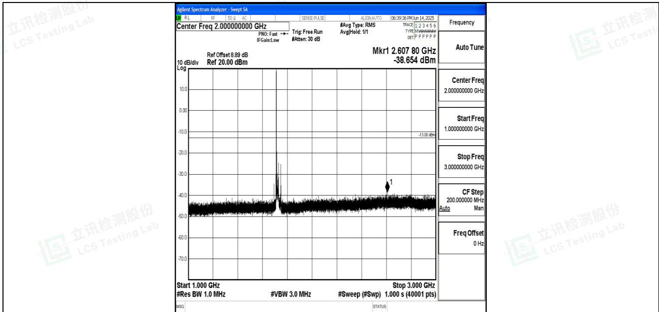
Band66_20MHz_16QAM_132072_1RB#0_1000~3000_1000~3000
