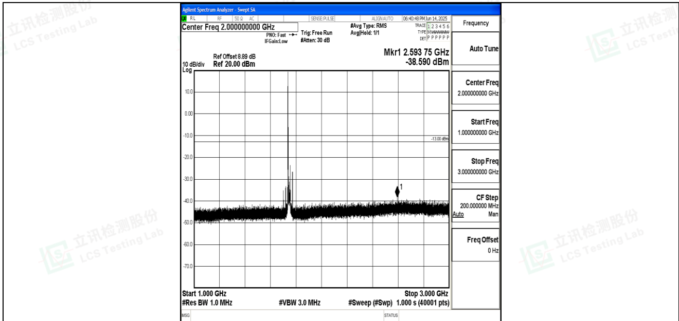
Band66_20MHz_16QAM_132322_1RB#0_1000~3000_1000~3000
