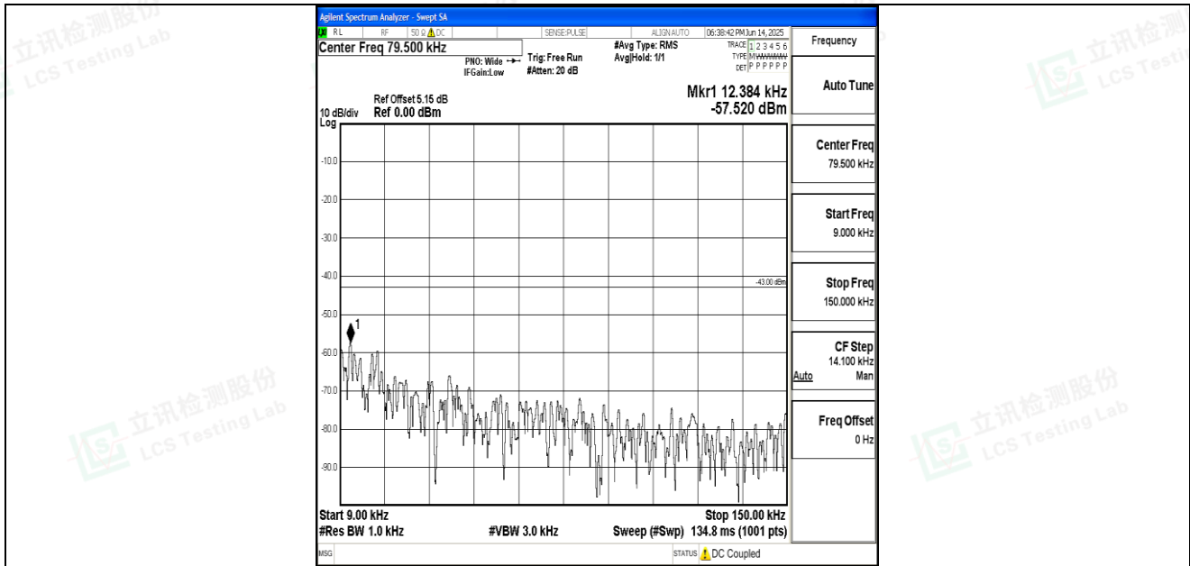
Band66_20MHz_QPSK_132072_1RB#0_0.009~0.15_0.009~0.15
