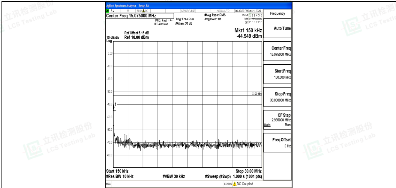
Band66_20MHz_16QAM_132072_1RB#0_0.15~30_0.15~30
