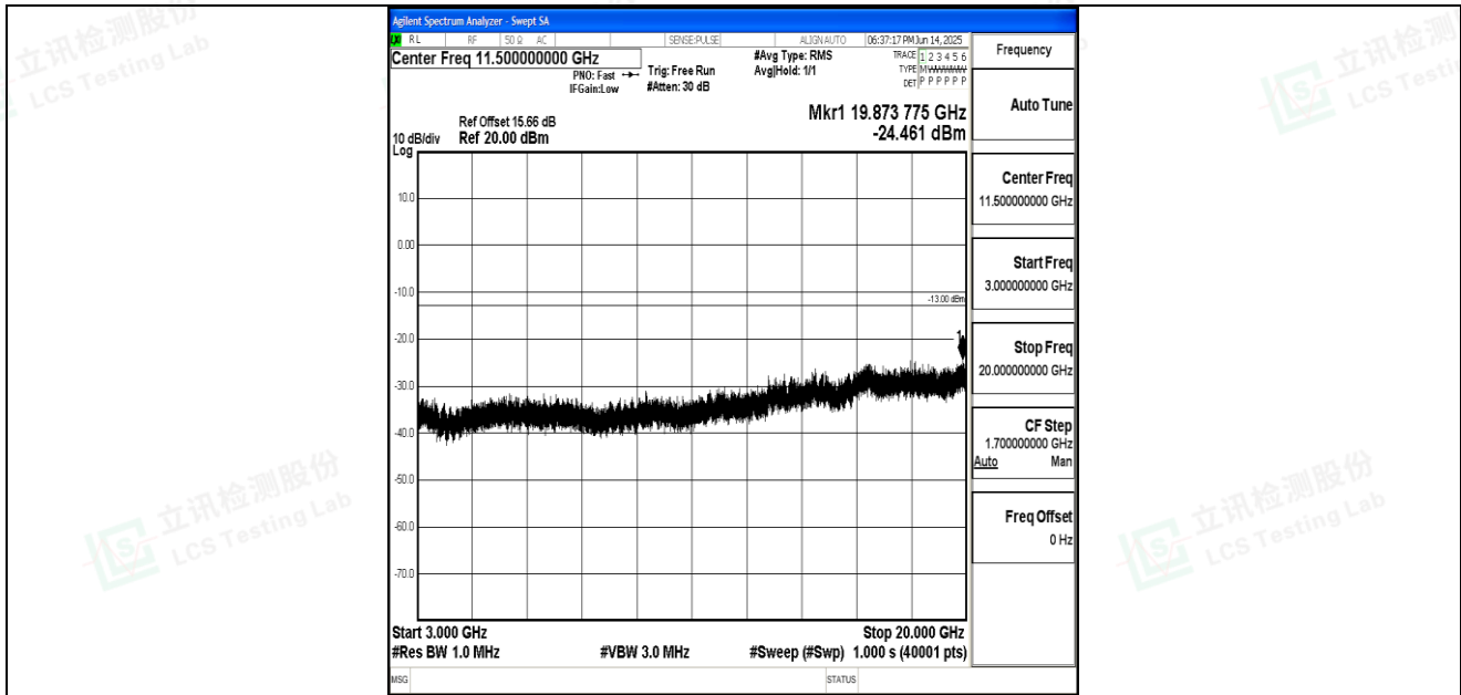
Band66_15MHz_QPSK_132597_1RB#0_3000~20000_3000~20000
