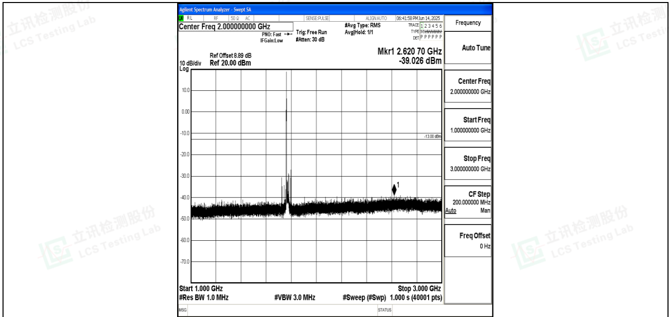
Band66_20MHz_16QAM_132572_1RB#0_1000~3000_1000~3000
