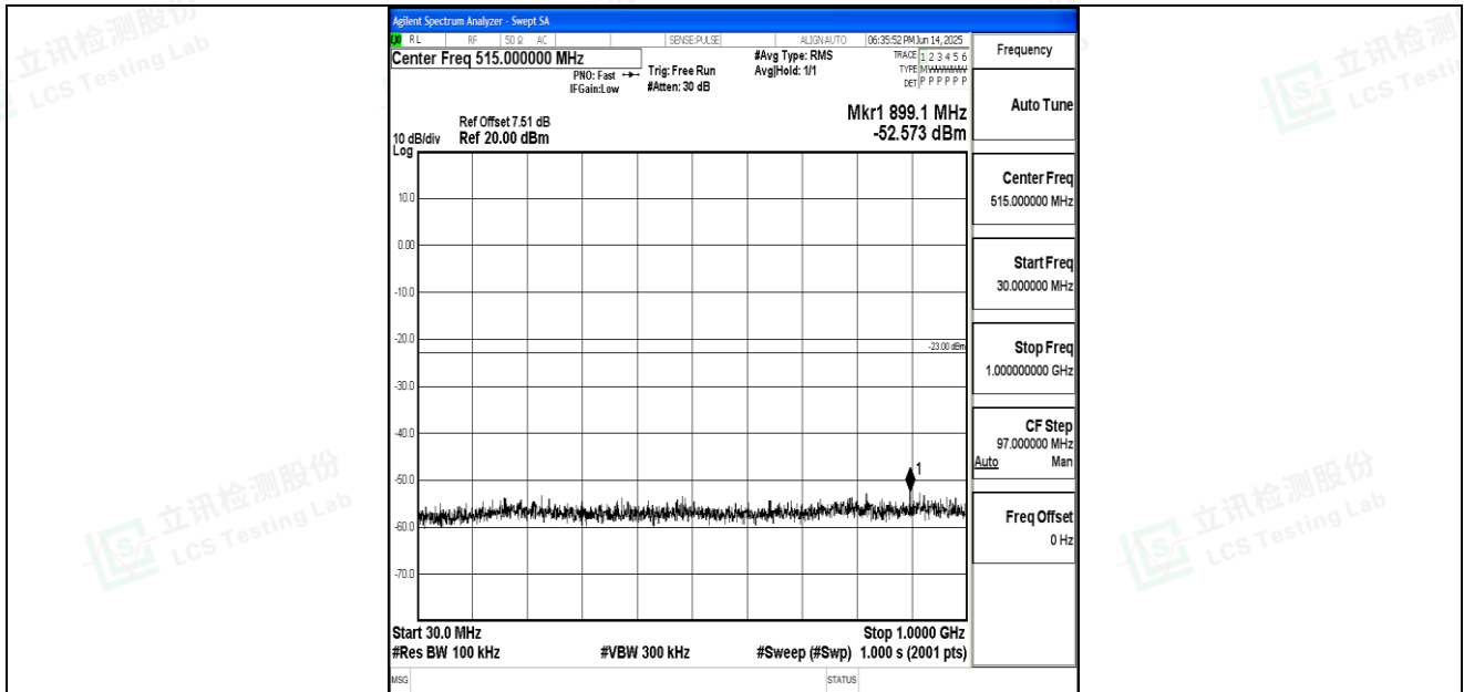
Band66_15MHz_QPSK_132322_1RB#0_30~1000_30~1000
