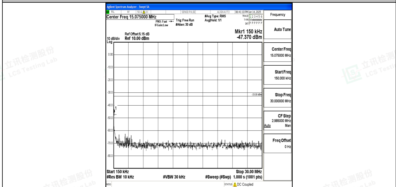
Band66_20MHz_QPSK_132572_1RB#0_0.15~30_0.15~30
