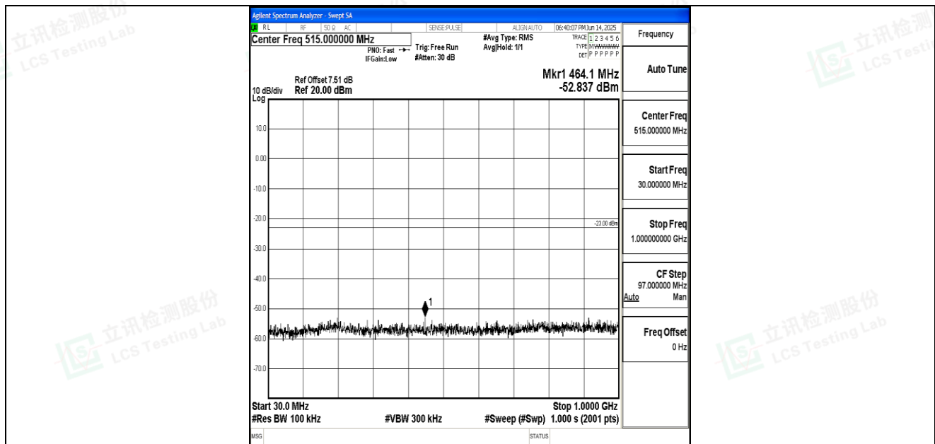
Band66_20MHz_QPSK_132322_1RB#0_30~1000_30~1000
