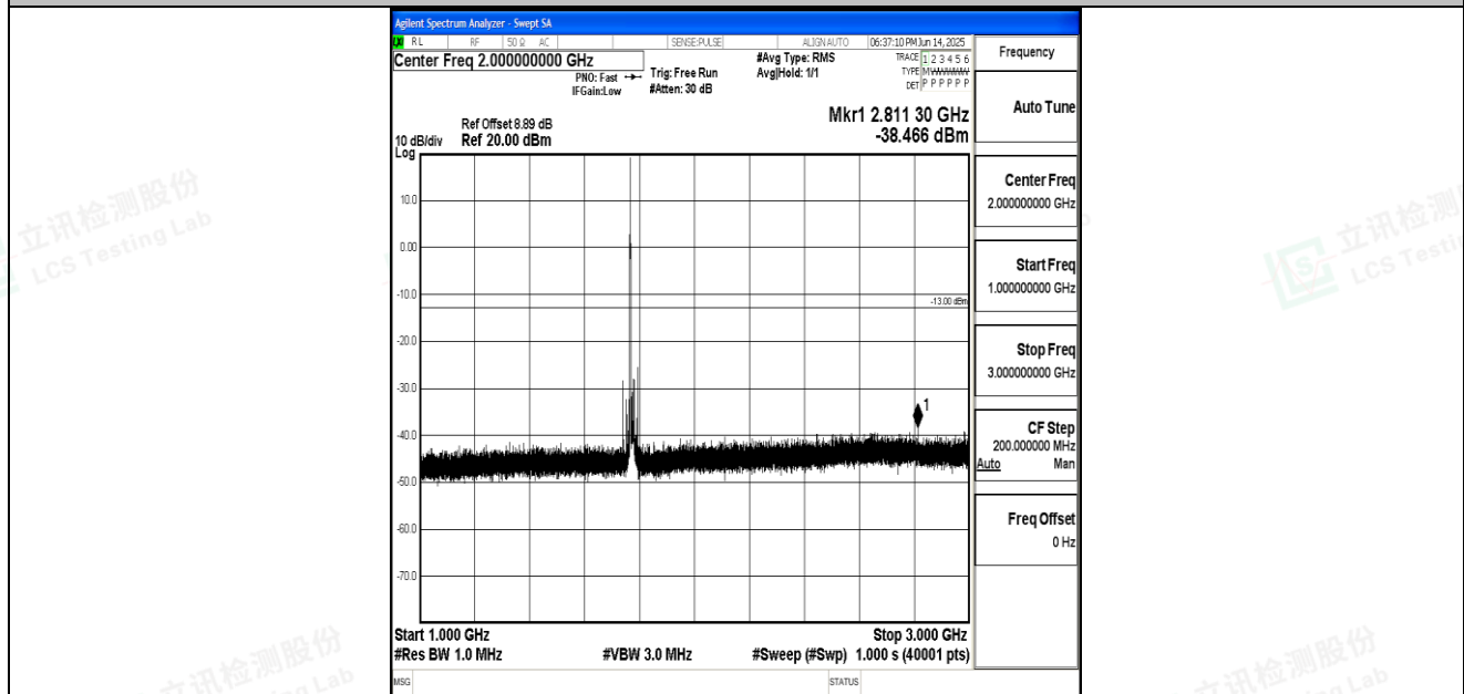
Band66_15MHz_QPSK_132597_1RB#0_1000~3000_1000~3000
