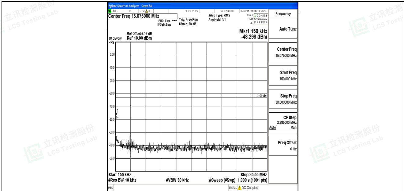
Band66_20MHz_16QAM_132572_1RB#0_0.15~30_0.15~30
