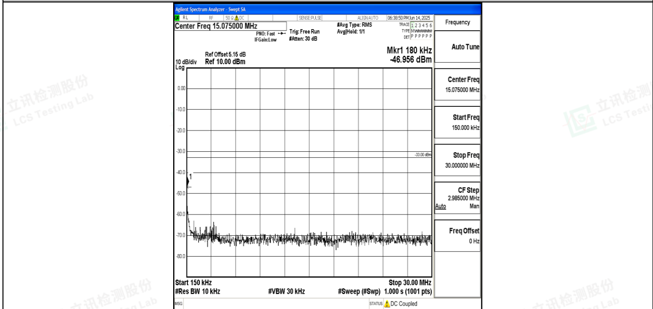
Band66_20MHz_QPSK_132072_1RB#0_0.15~30_0.15~30
