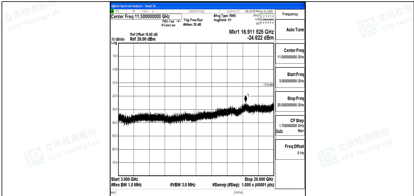
Band66_15MHz_QPSK_132047_1RB#0_3000~20000_3000~20000
