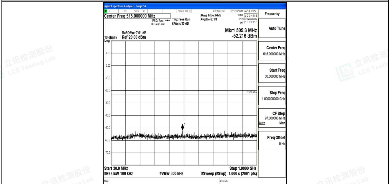
Band66_10MHz_16QAM_132622_1RB#0_30~1000_30~1000
