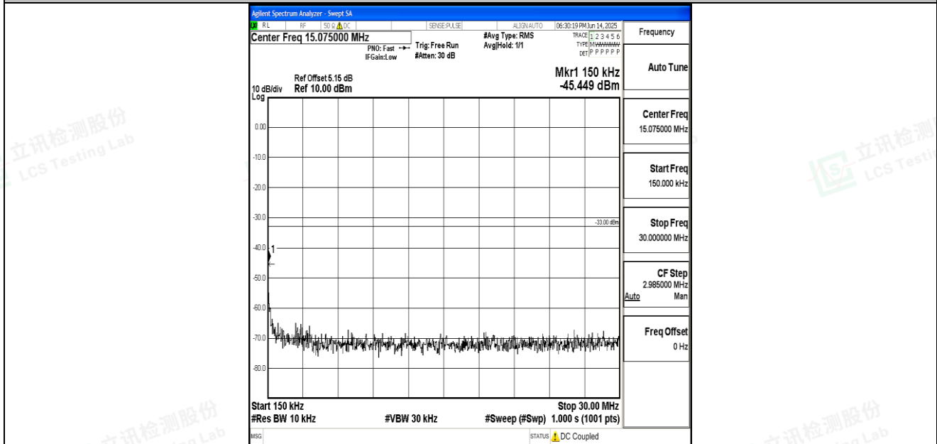
Band66_10MHz_QPSK_132022_1RB#0_0.15~30_0.15~30
