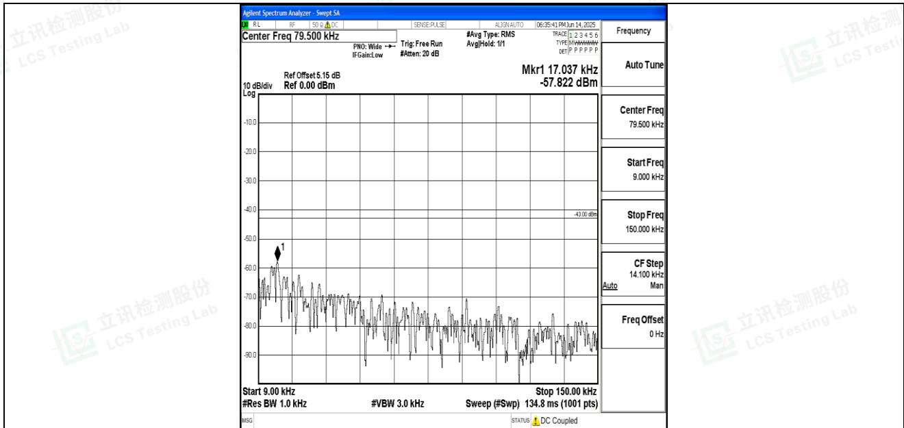
Band66_15MHz_QPSK_132322_1RB#0_0.009~0.15_0.009~0.15
