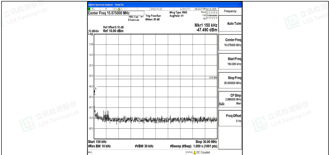
Band66_3MHz_16QAM_131987_1RB#0_0.15~30_0.15~30
