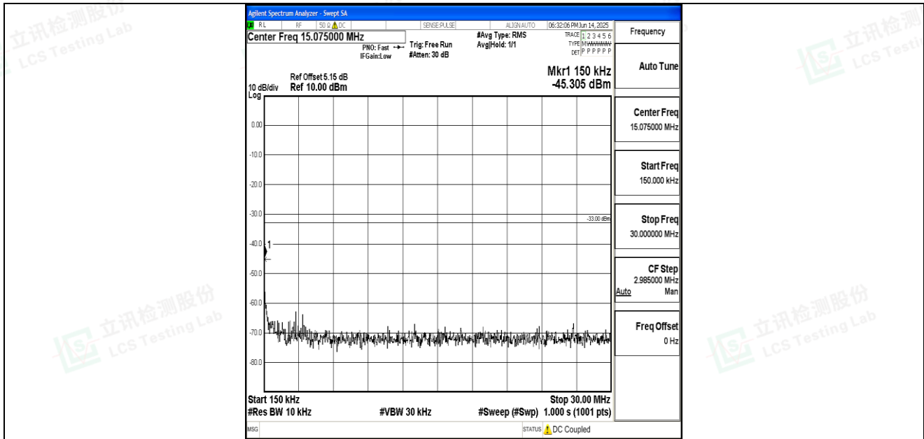
Band66_10MHz_16QAM_132322_1RB#0_0.15~30_0.15~30
