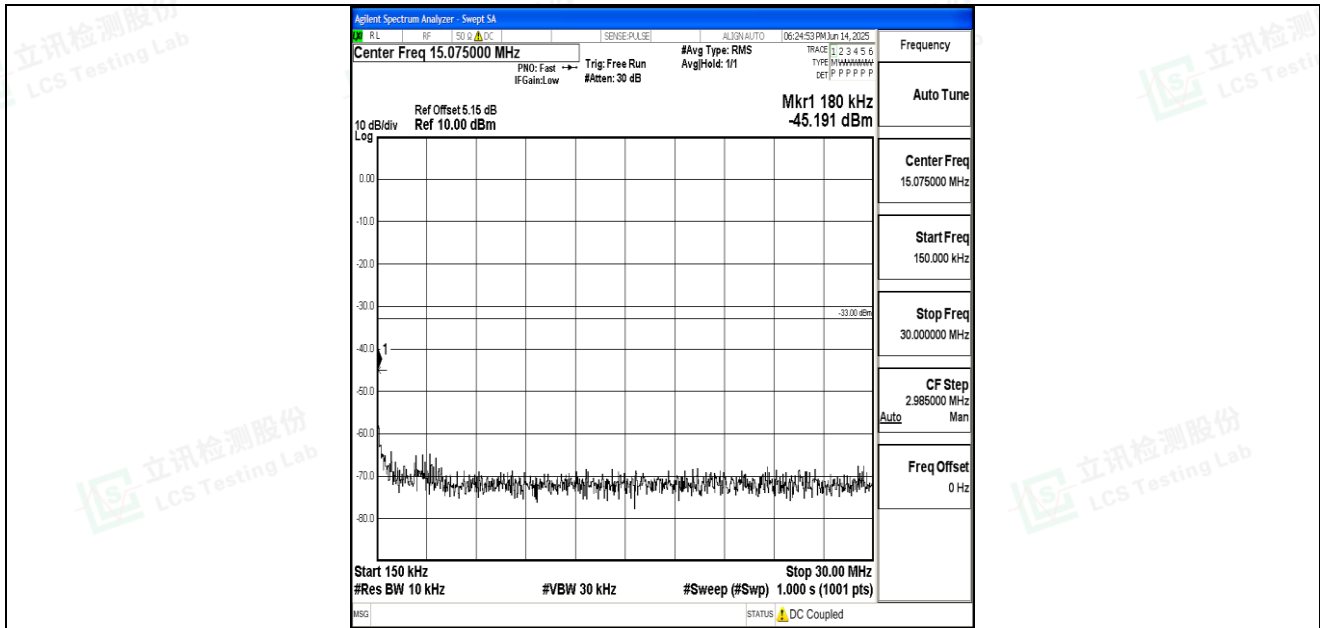
Band66_3MHz_16QAM_132657_1RB#0_0.15~30_0.15~30
