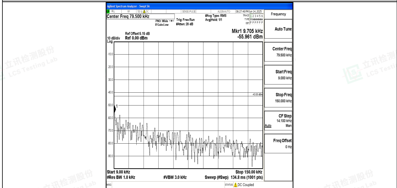
Band66_5MHz_16QAM_132322_1RB#0_0.009~0.15_0.009~0.15
