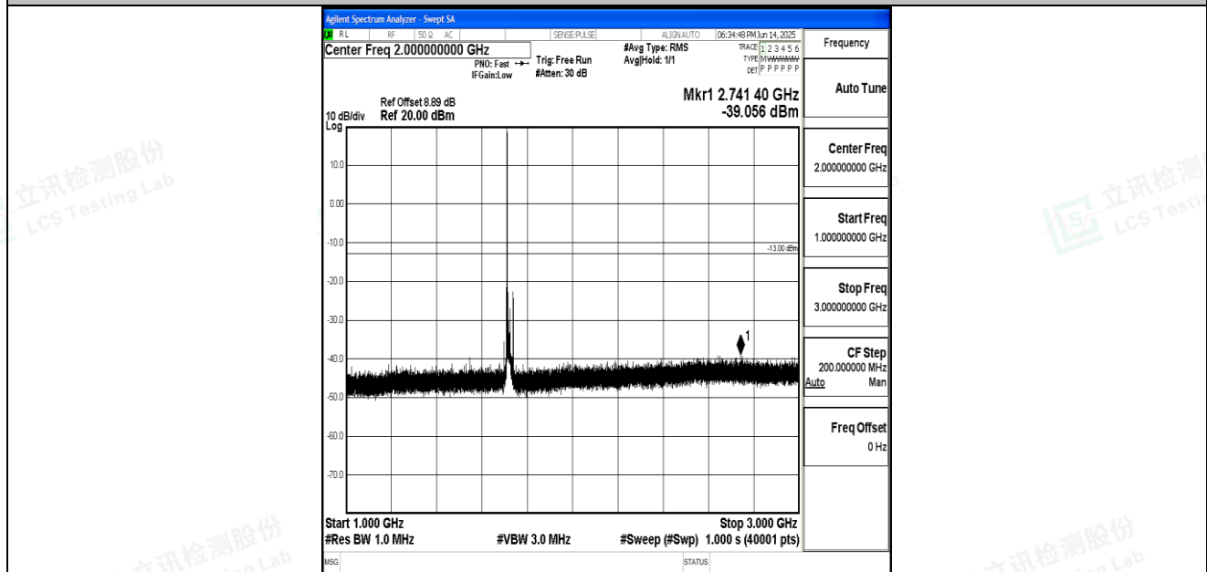
Band66_15MHz_QPSK_132047_1RB#0_1000~3000_1000~3000
