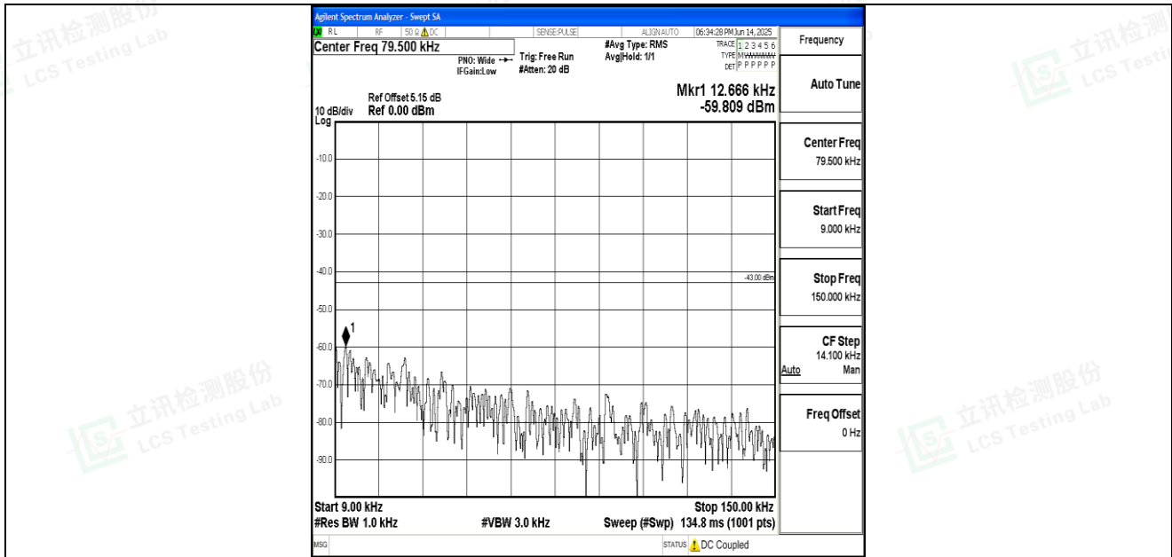
Band66_15MHz_QPSK_132047_1RB#0_0.009~0.15_0.009~0.15
