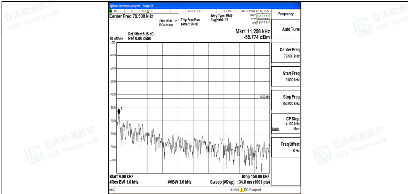
Band66_5MHz_QPSK_132322_1RB#0_0.009~0.15_0.009~0.15
