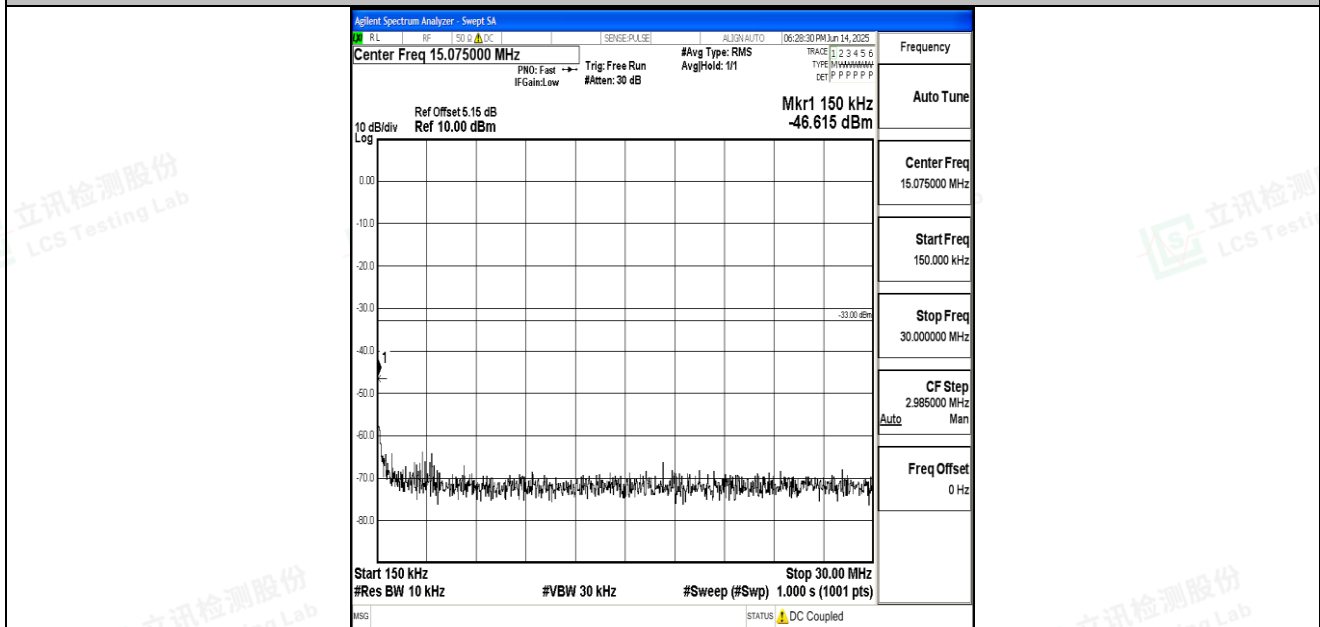
Band66_5MHz_QPSK_132647_1RB#0_0.15~30_0.15~30
