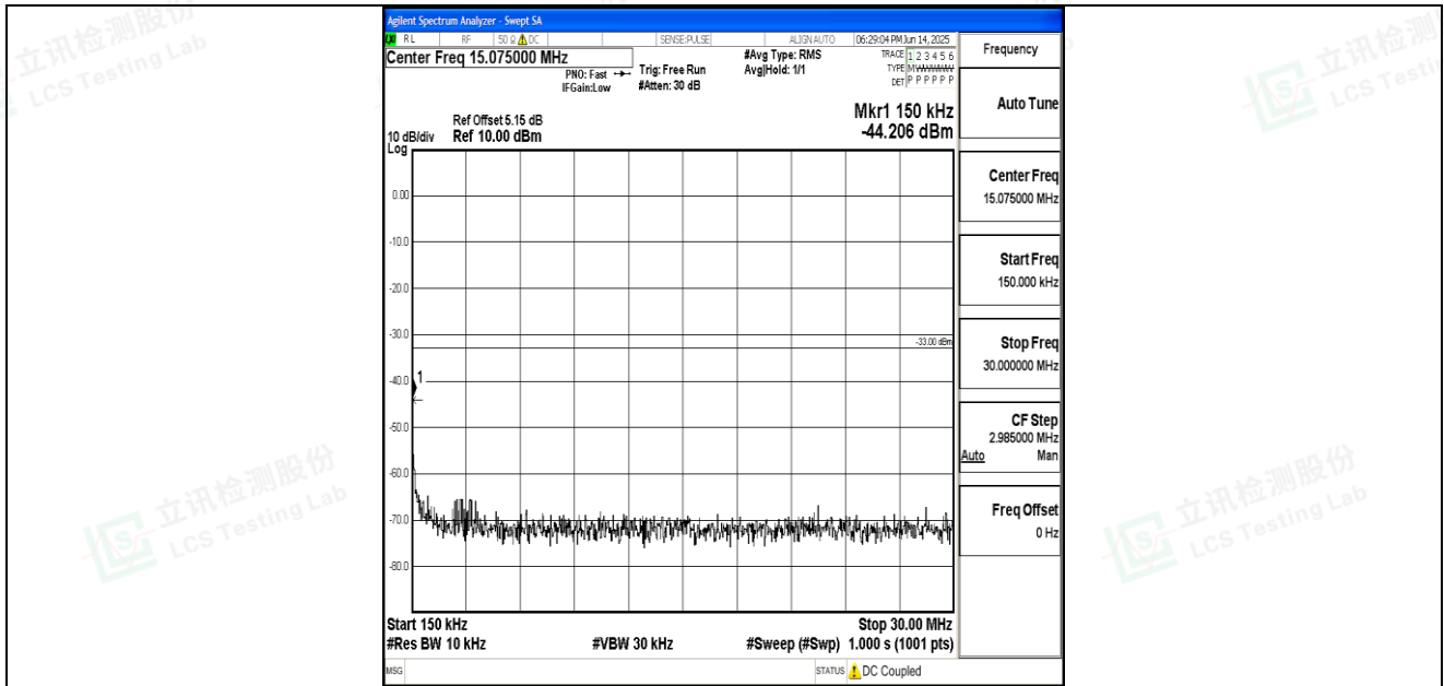
Band66_5MHz_16QAM_132647_1RB#0_0.15~30_0.15~30
