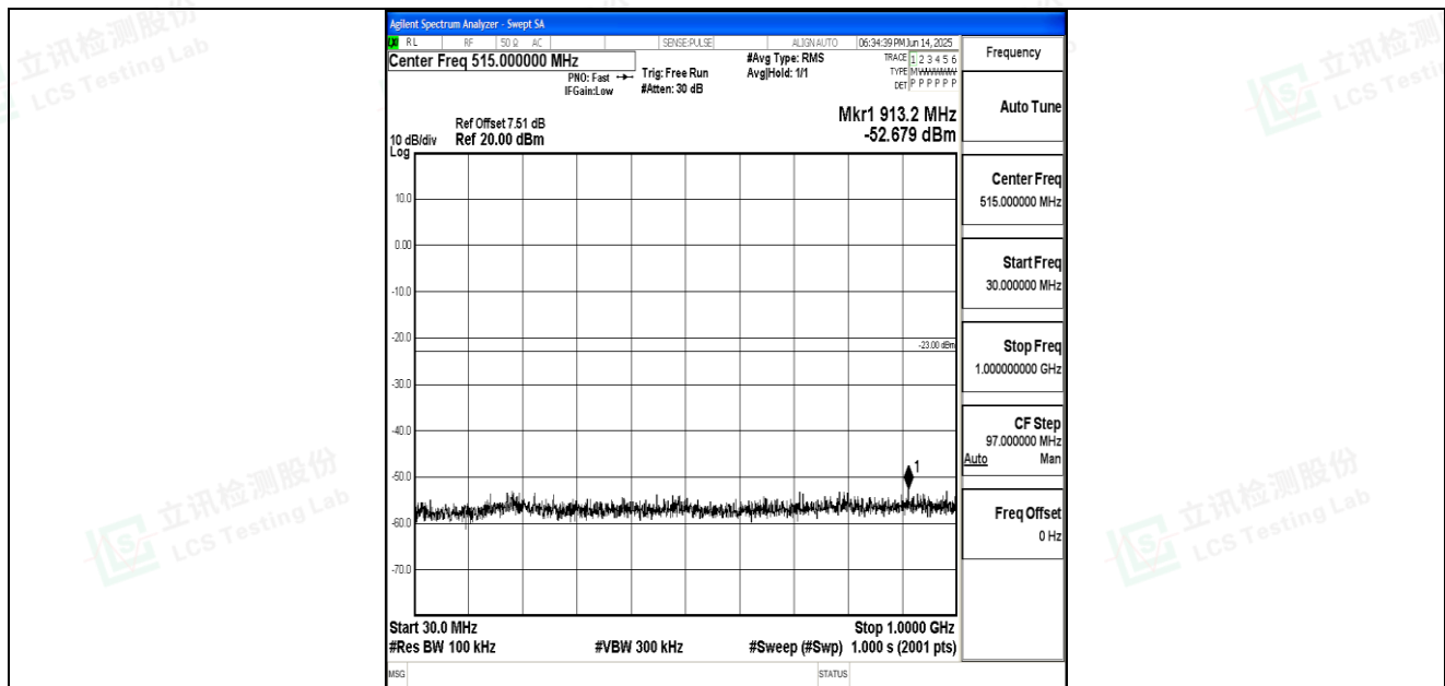
Band66_15MHz_QPSK_132047_1RB#0_30~1000_30~1000
