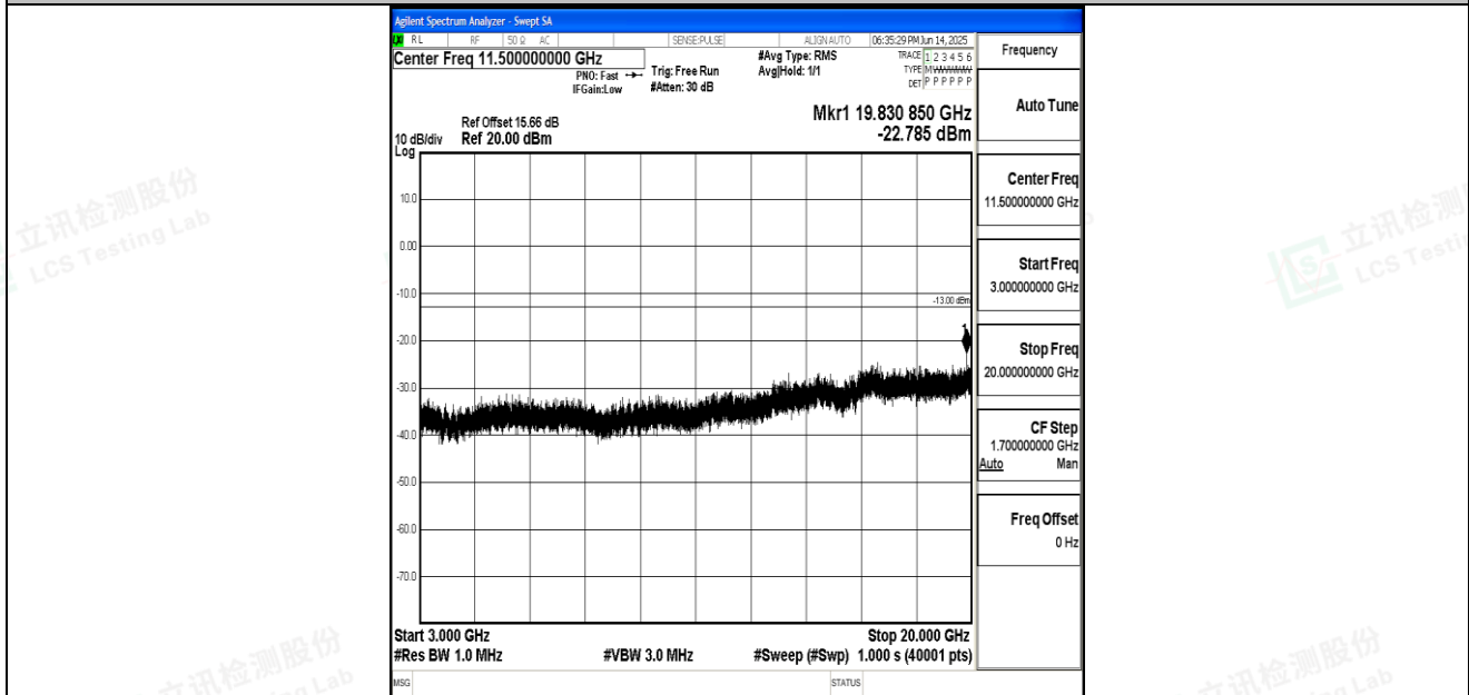
Band66_15MHz_16QAM_132047_1RB#0_3000~20000_3000~20000
