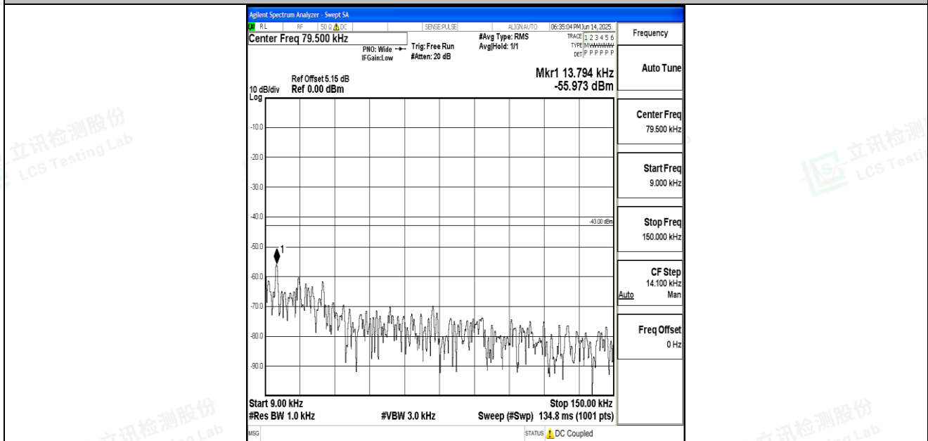
Band66_15MHz_16QAM_132047_1RB#0_0.009~0.15_0.009~0.15
