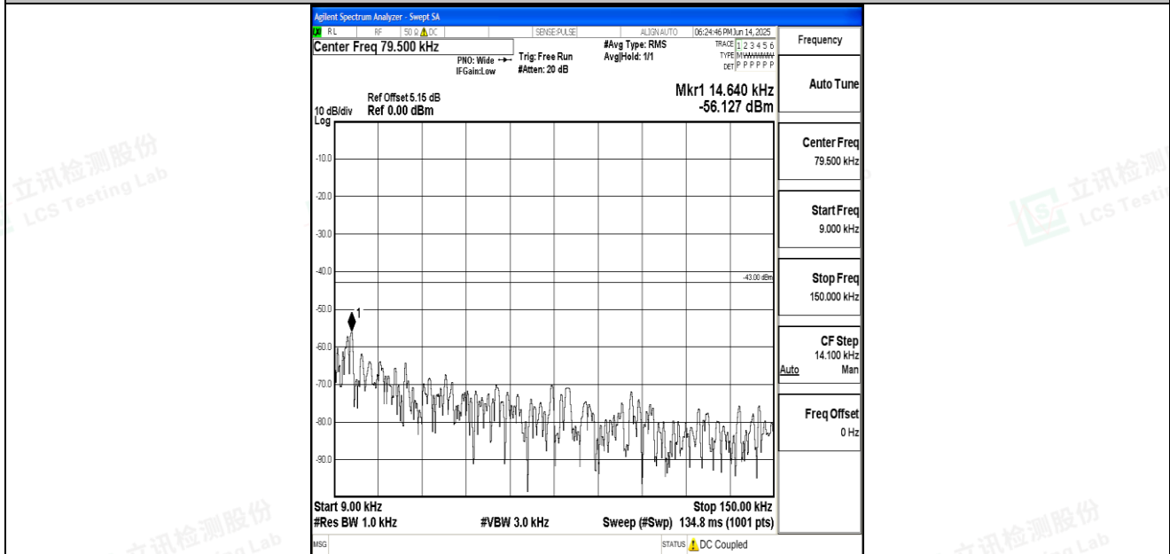
Band66_3MHz_16QAM_132657_1RB#0_0.009~0.15_0.009~0.15
