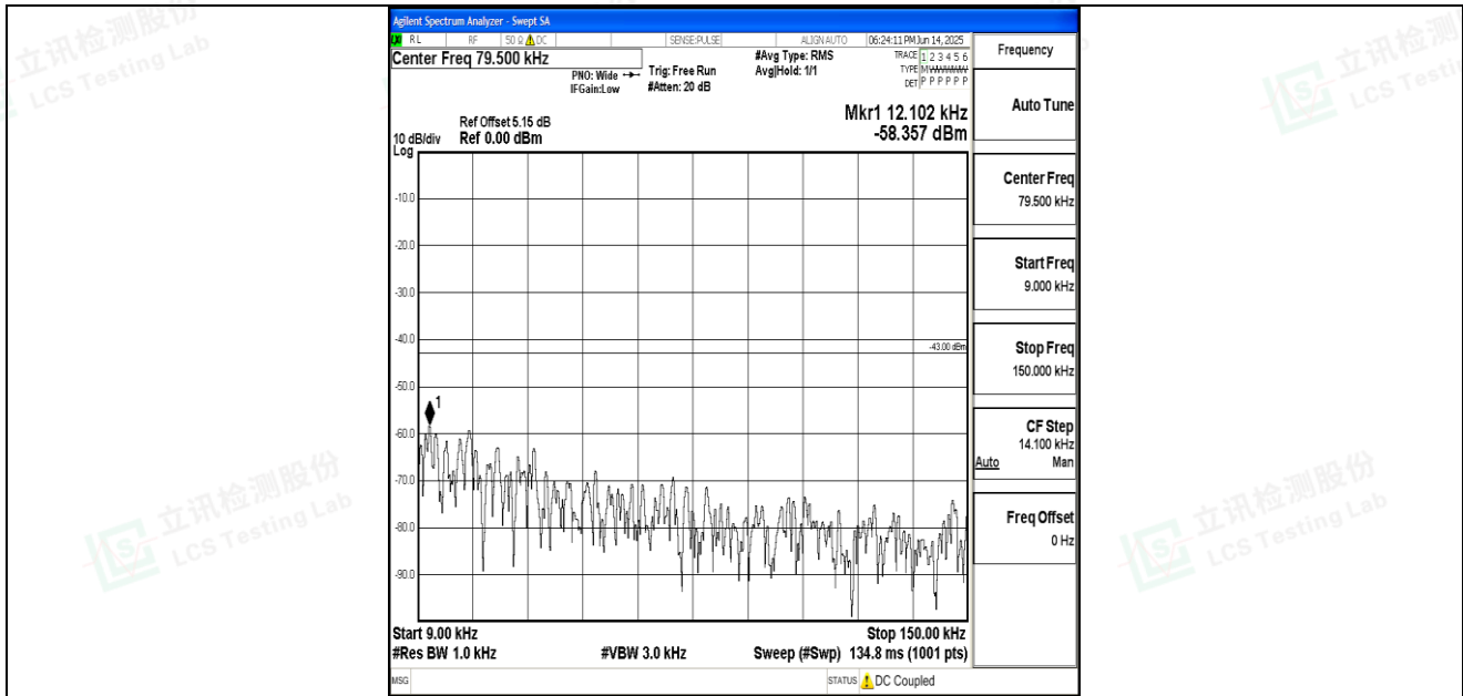
Band66_3MHz_QPSK_132657_1RB#0_0.009~0.15_0.009~0.15
