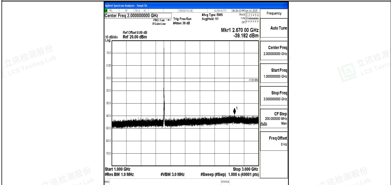
Band66_5MHz_QPSK_131997_1RB#0_1000~3000_1000~3000
