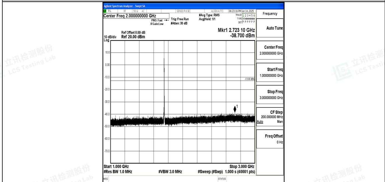
Band66_3MHz_QPSK_132322_1RB#0_1000~3000_1000~3000
