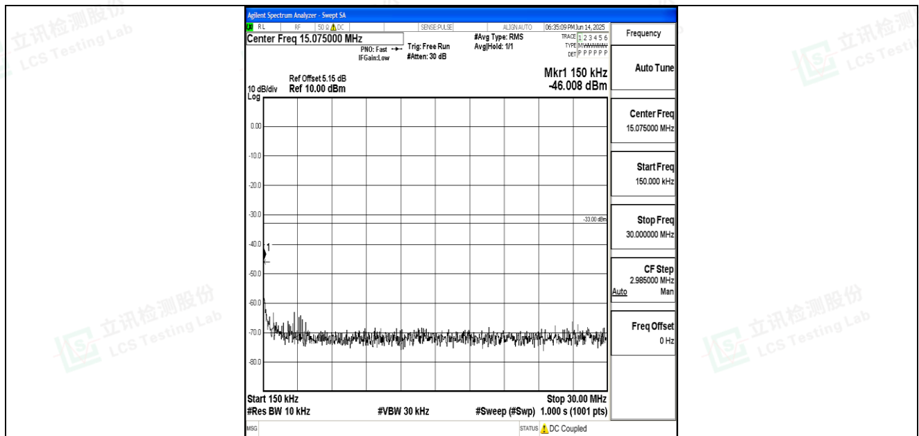
Band66_15MHz_16QAM_132047_1RB#0_0.15~30_0.15~30
