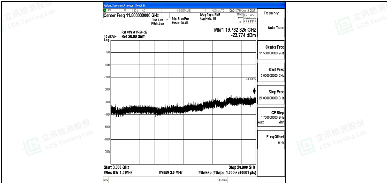
Band66_3MHz_QPSK_132657_1RB#0_3000~20000_3000~20000
