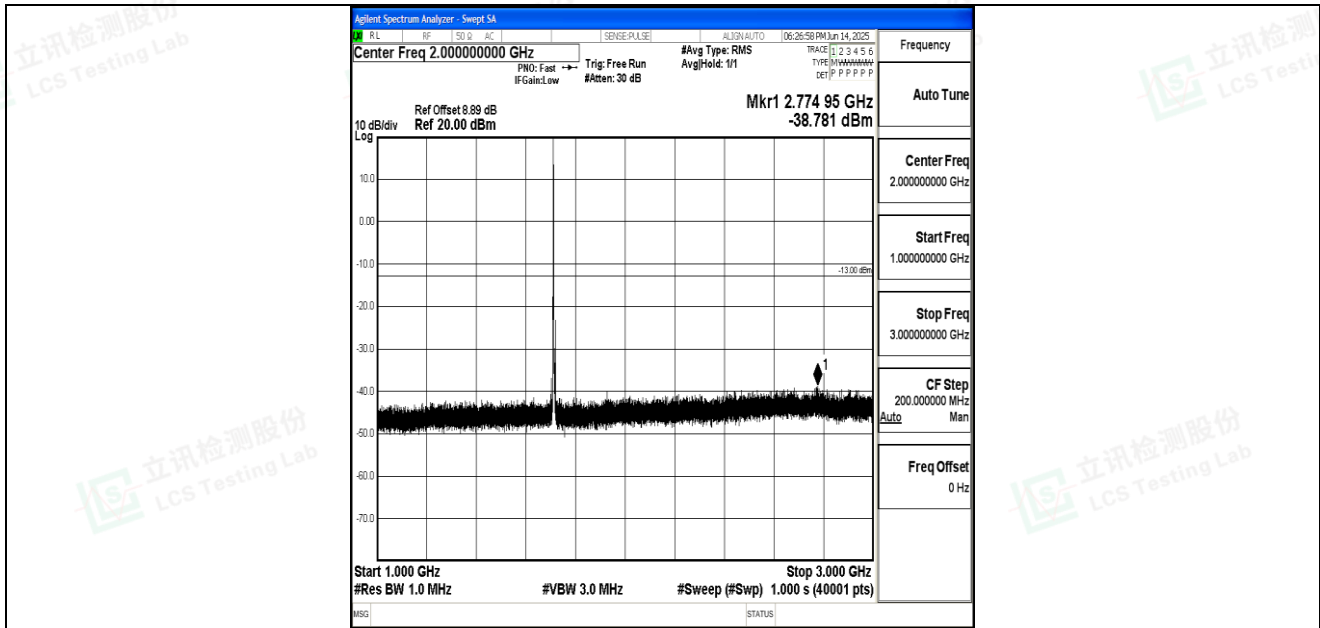
Band66_5MHz_16QAM_131997_1RB#0_1000~3000_1000~3000
