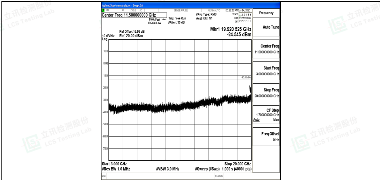
Band66_3MHz_QPSK_131987_1RB#0_3000~20000_3000~20000
