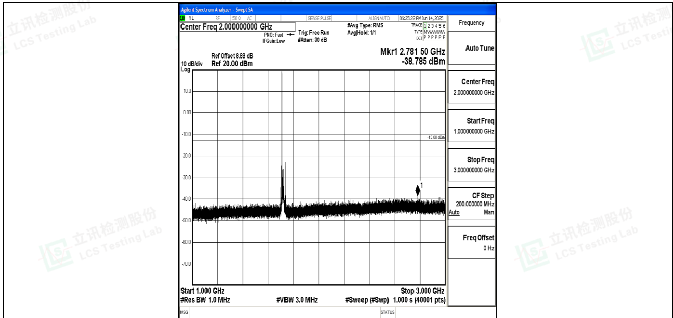
Band66_15MHz_16QAM_132047_1RB#0_1000~3000_1000~3000
