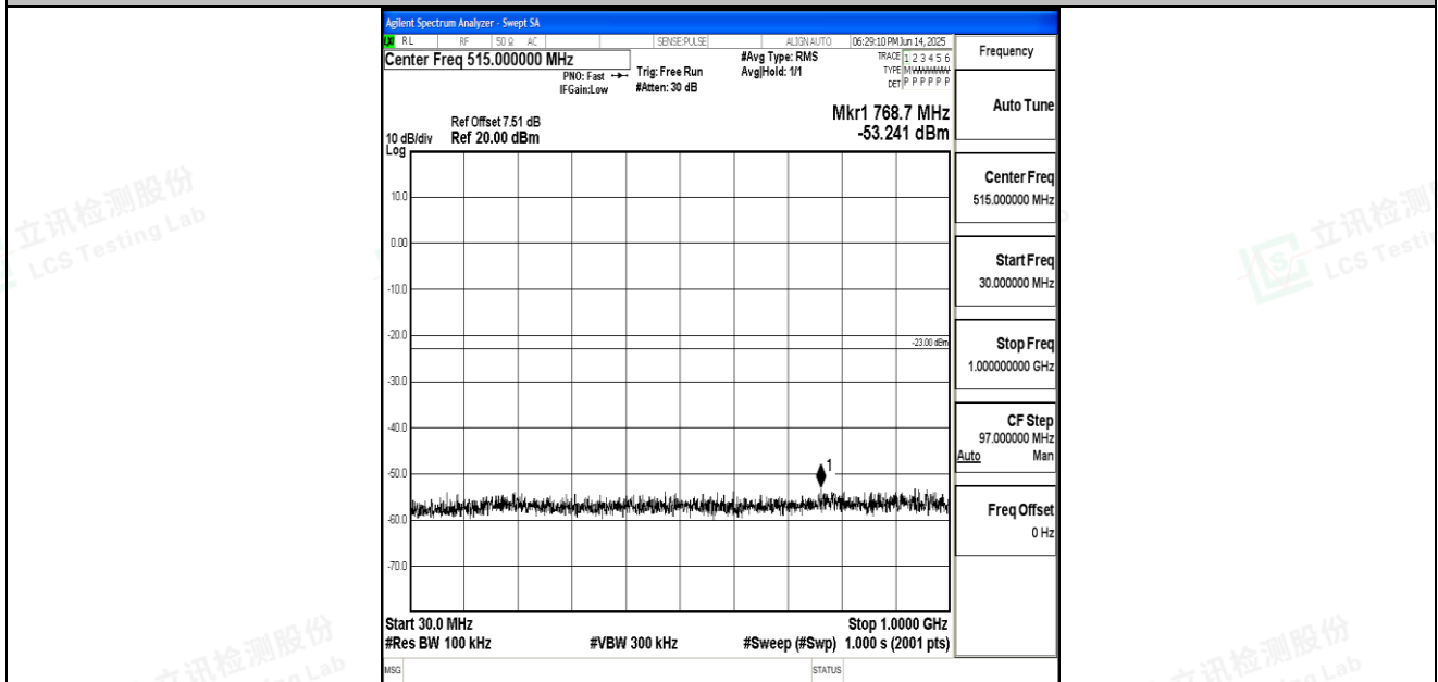
Band66_5MHz_16QAM_132647_1RB#0_30~1000_30~1000
