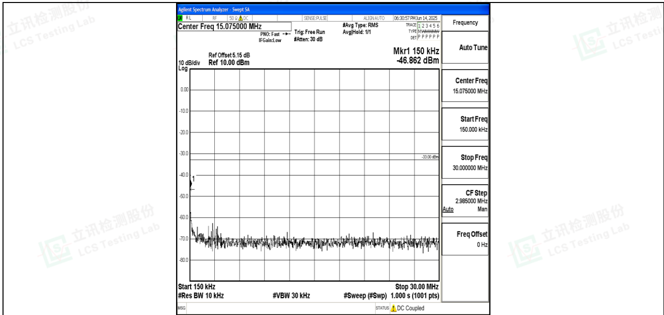
Band66_10MHz_16QAM_132022_1RB#0_0.15~30_0.15~30
