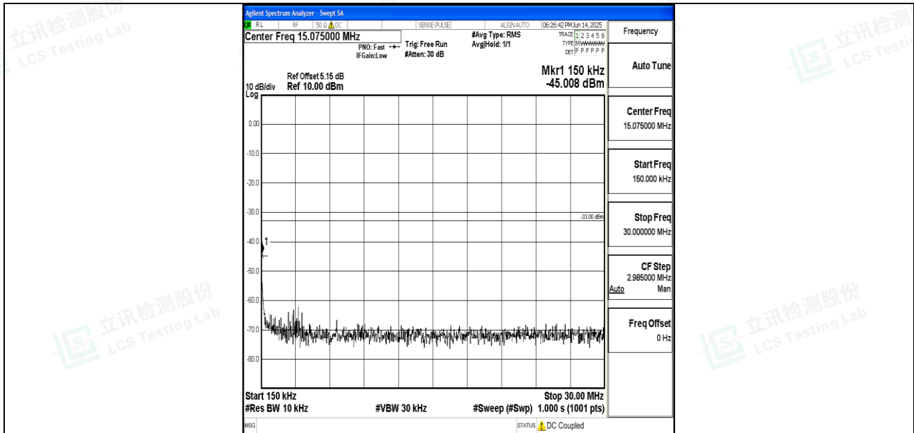
Band66_5MHz_16QAM_131997_1RB#0_0.15~30_0.15~30
