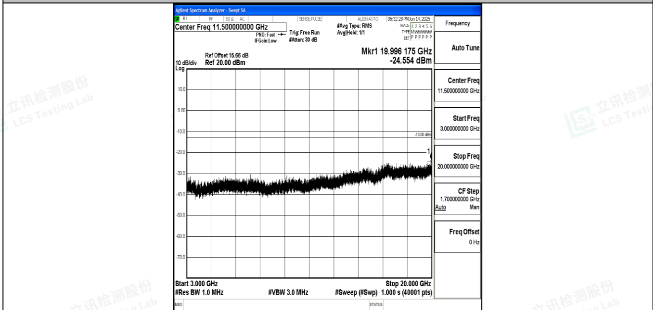
Band66_10MHz_16QAM_132322_1RB#0_3000~20000_3000~20000
