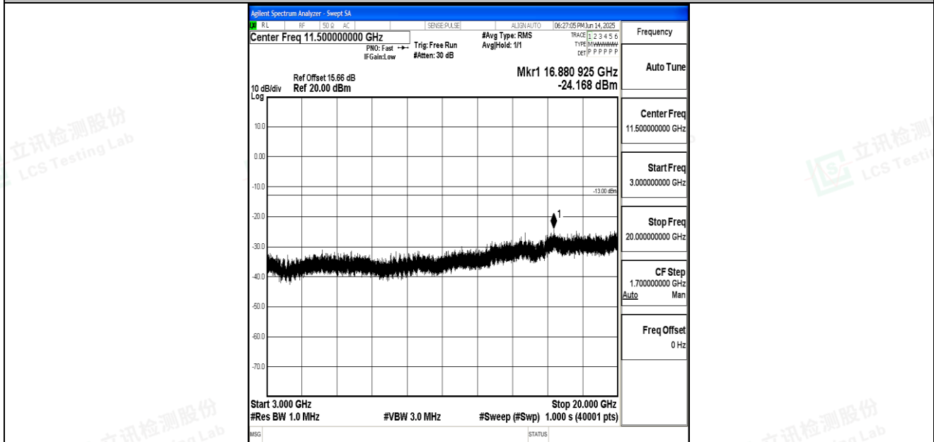
Band66_5MHz_16QAM_131997_1RB#0_3000~20000_3000~20000
