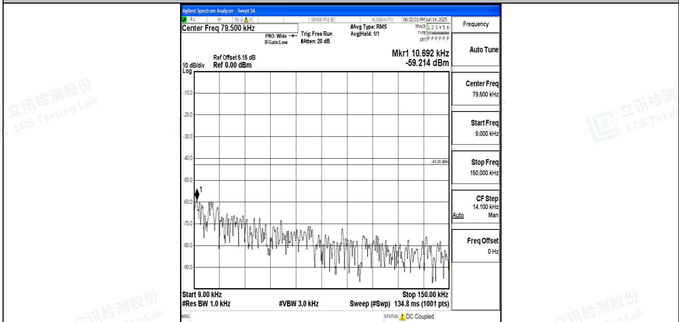
Band66_10MHz_16QAM_132322_1RB#0_0.009~0.15_0.009~0.15
