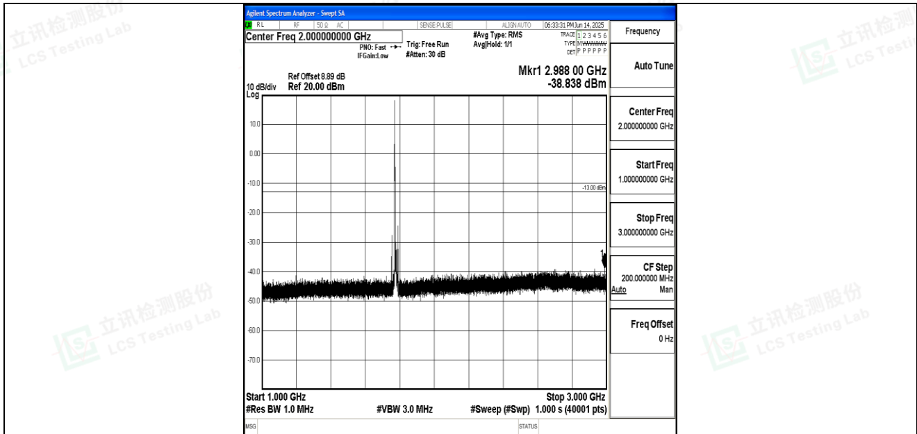
Band66_10MHz_16QAM_132622_1RB#0_1000~3000_1000~3000
