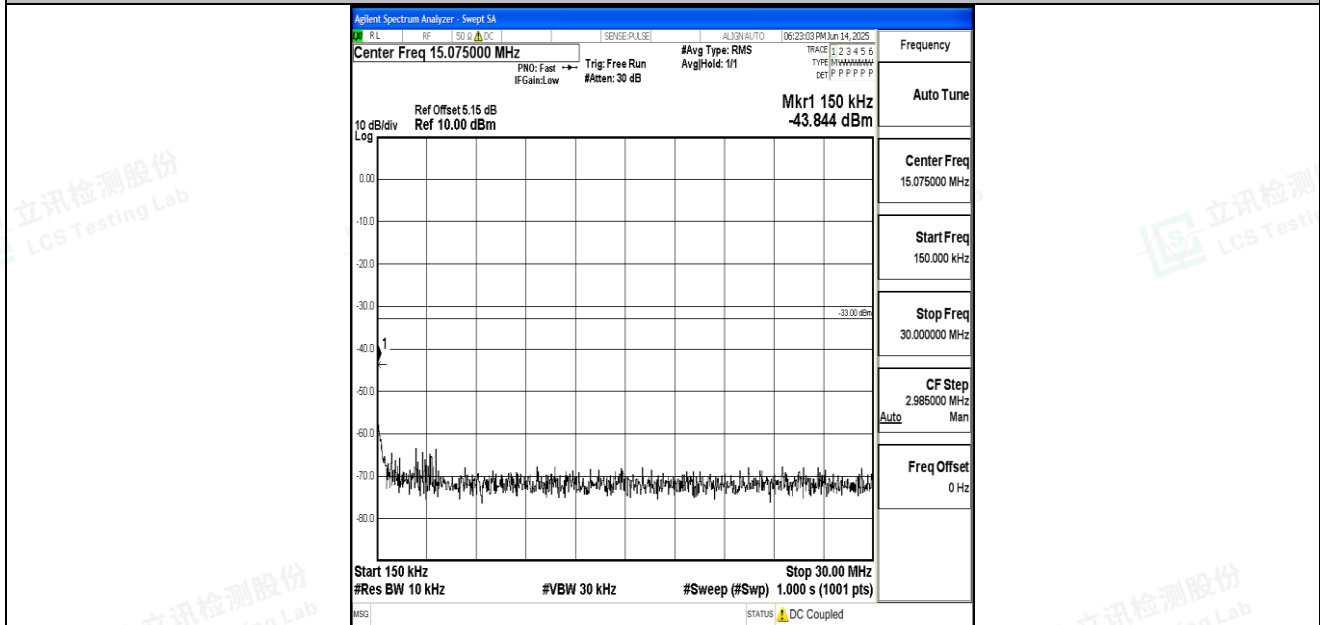
Band66_3MHz_QPSK_132322_1RB#0_0.15~30_0.15~30
