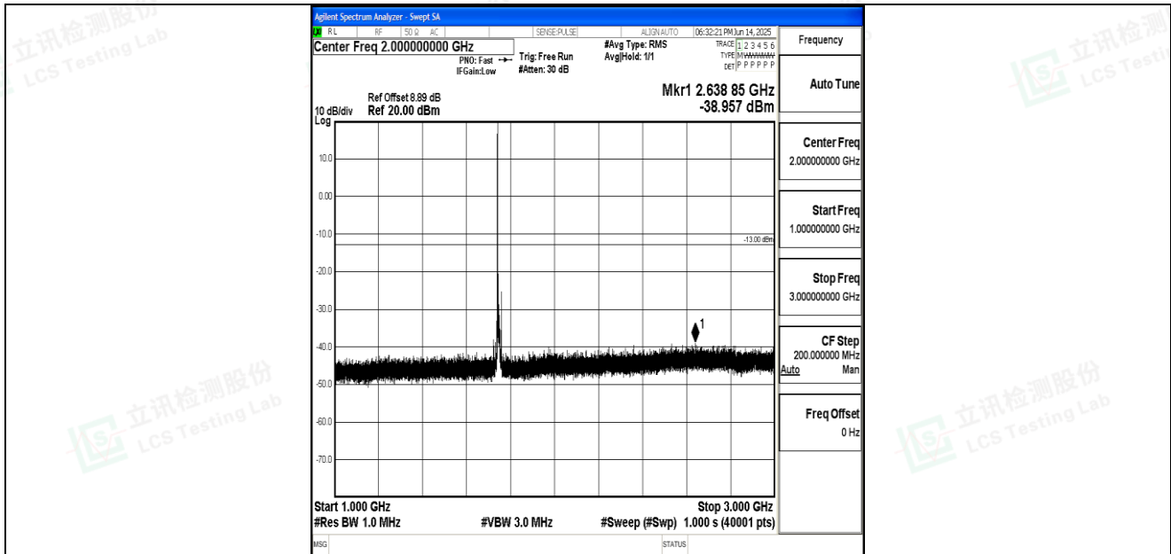
Band66_10MHz_16QAM_132322_1RB#0_1000~3000_1000~3000
