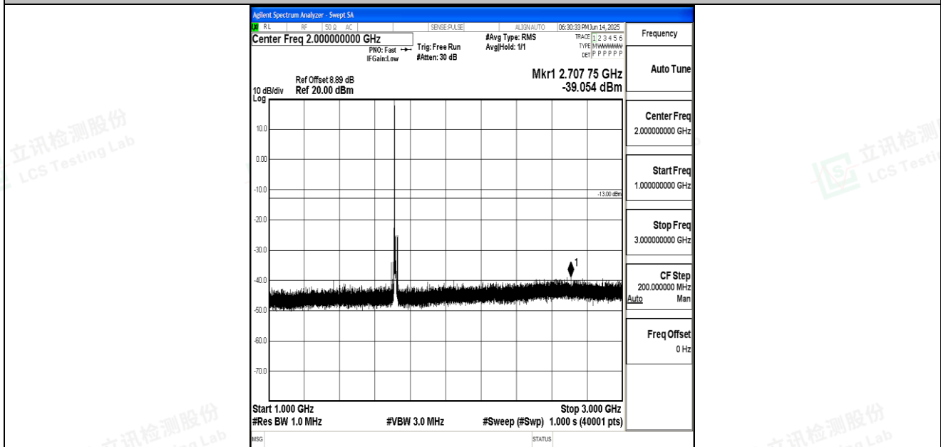
Band66_10MHz_QPSK_132022_1RB#0_1000~3000_1000~3000
