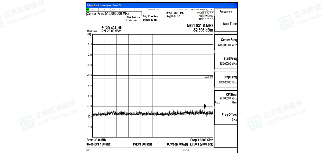
Band66_10MHz_QPSK_132322_1RB#0_30~1000_30~1000
