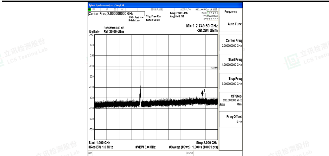
Band66_10MHz_QPSK_132322_1RB#0_1000~3000_1000~3000
