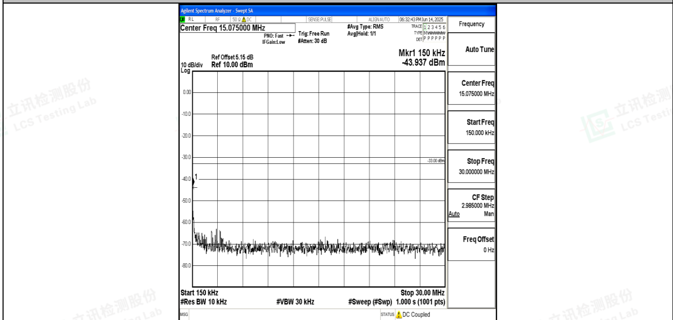
Band66_10MHz_QPSK_132622_1RB#0_0.15~30_0.15~30
