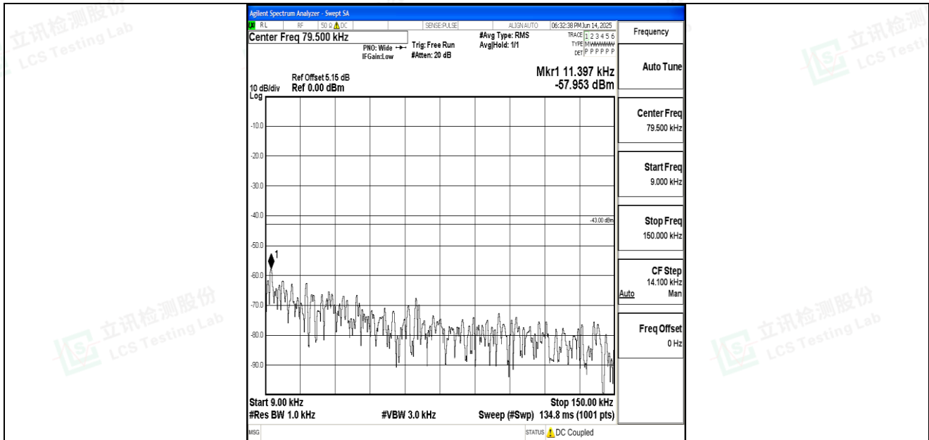
Band66_10MHz_QPSK_132622_1RB#0_0.009~0.15_0.009~0.15
