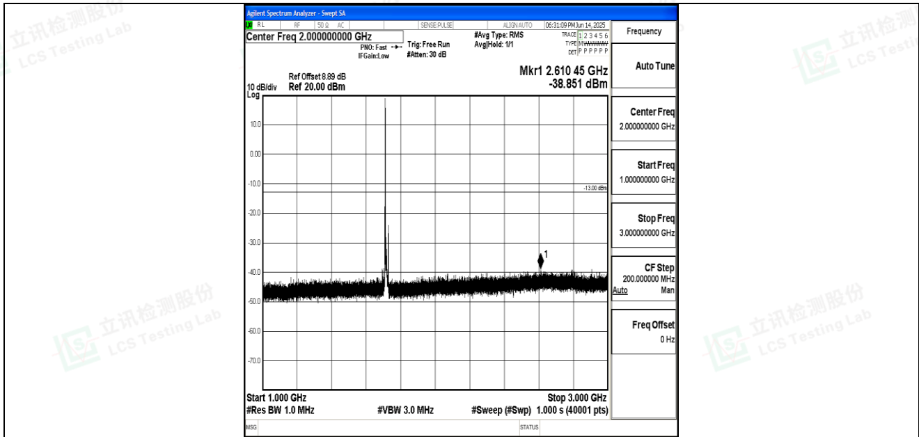
Band66_10MHz_16QAM_132022_1RB#0_1000~3000_1000~3000
