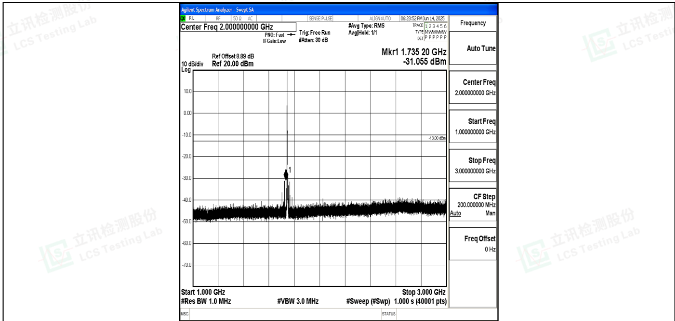
Band66_3MHz_16QAM_132322_1RB#0_1000~3000_1000~3000
