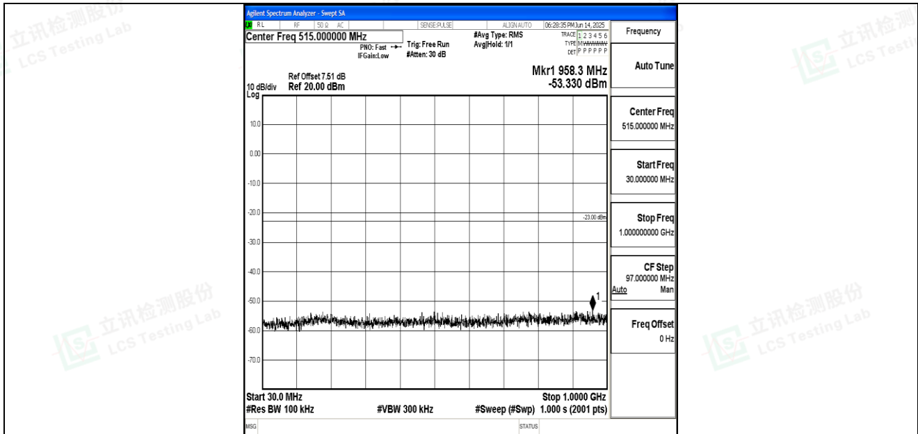
Band66_5MHz_QPSK_132647_1RB#0_30~1000_30~1000
