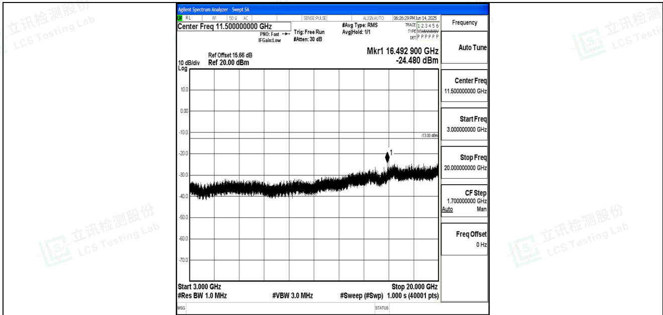
Band66_5MHz_QPSK_131997_1RB#0_3000~20000_3000~20000
