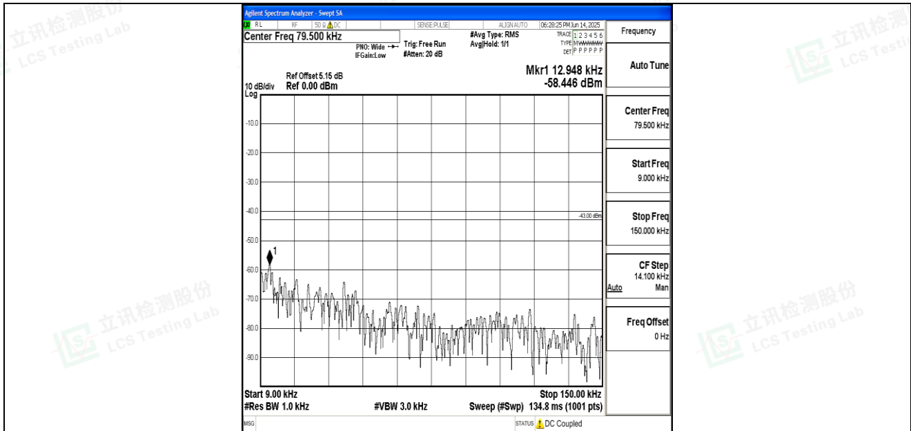
Band66_5MHz_QPSK_132647_1RB#0_0.009~0.15_0.009~0.15
