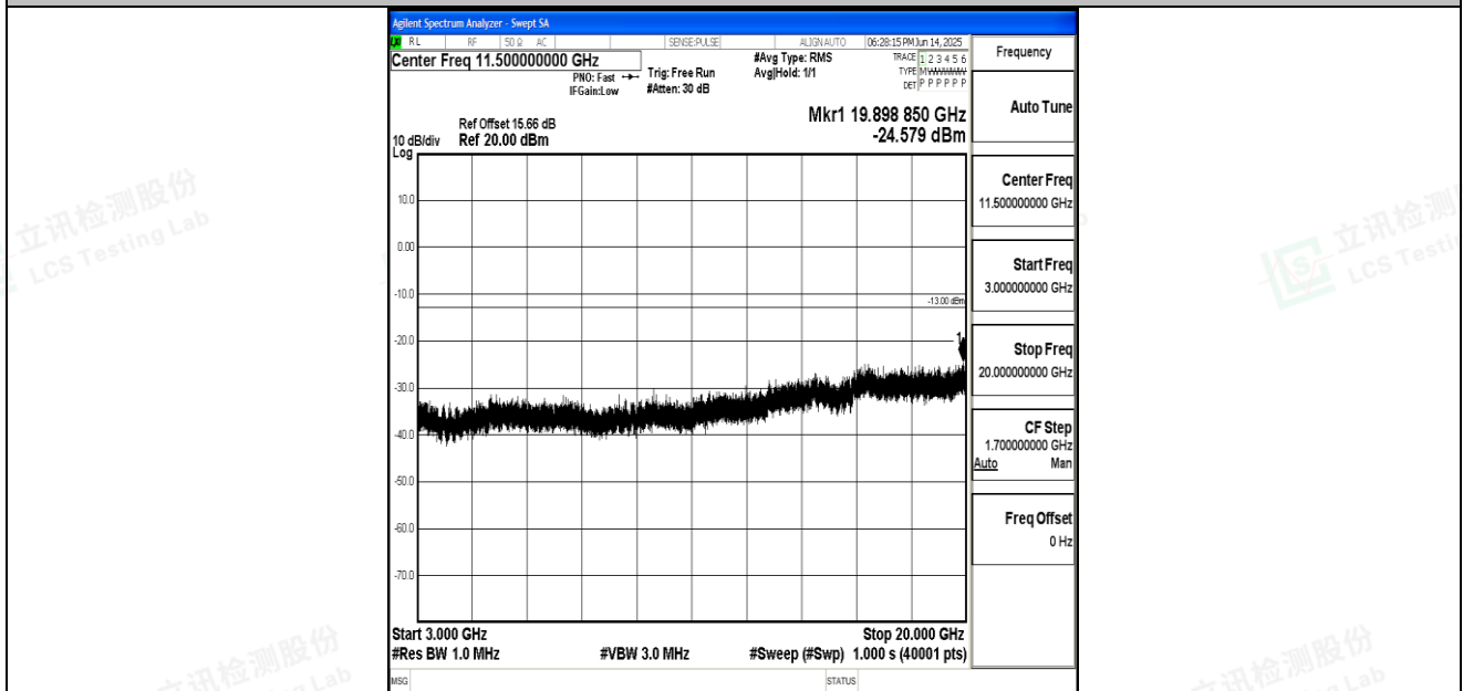
Band66_5MHz_16QAM_132322_1RB#0_3000~20000_3000~20000
