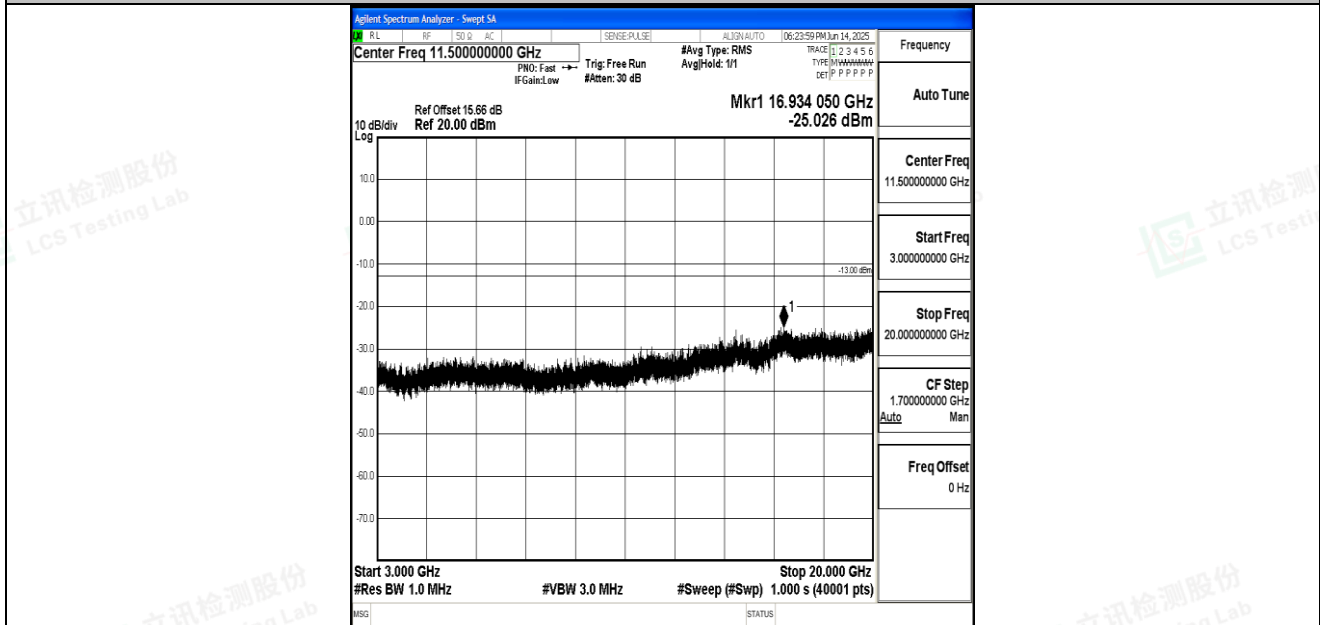
Band66_3MHz_16QAM_132322_1RB#0_3000~20000_3000~20000
