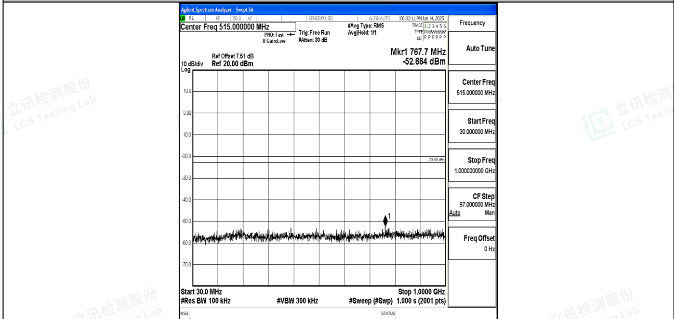
Band66_10MHz_16QAM_132322_1RB#0_30~1000_30~1000
