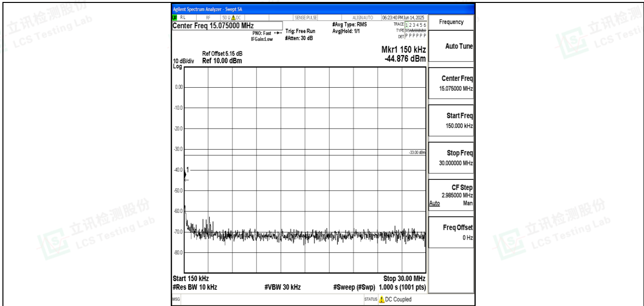
Band66_3MHz_16QAM_132322_1RB#0_0.15~30_0.15~30
