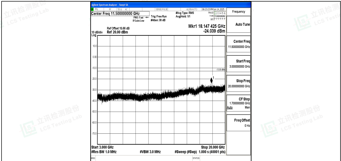
Band66_3MHz_QPSK_132322_1RB#0_3000~20000_3000~20000
