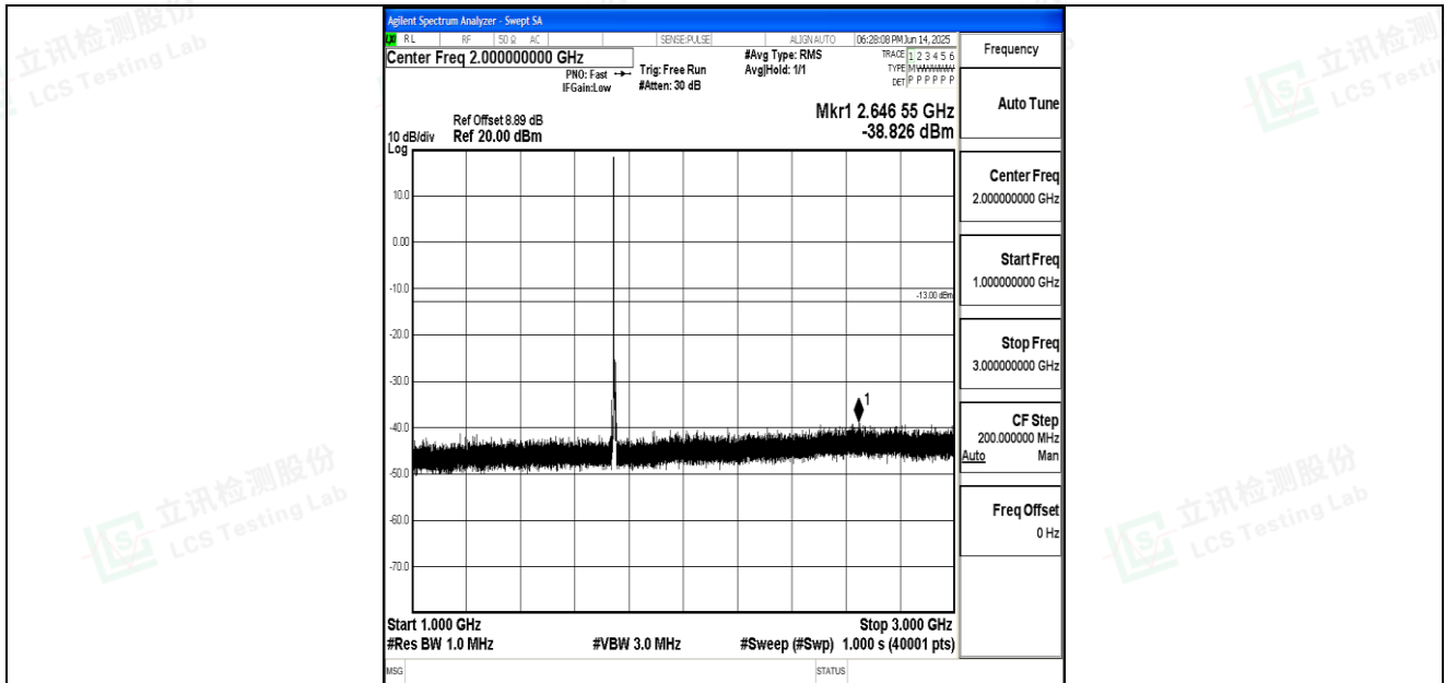
Band66_5MHz_16QAM_132322_1RB#0_1000~3000_1000~3000
