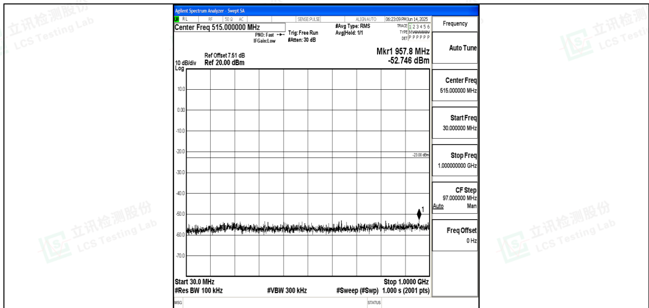
Band66_3MHz_QPSK_132322_1RB#0_30~1000_30~1000
