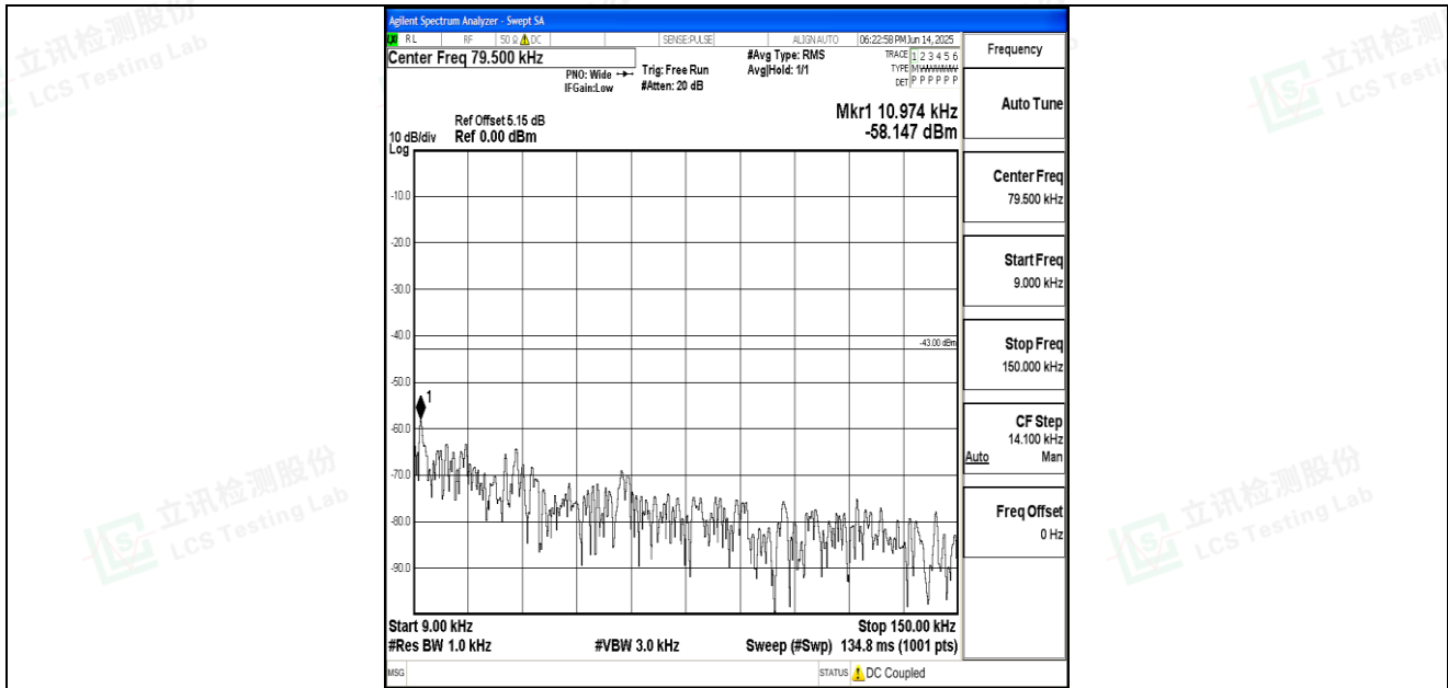
Band66_3MHz_QPSK_132322_1RB#0_0.009~0.15_0.009~0.15
