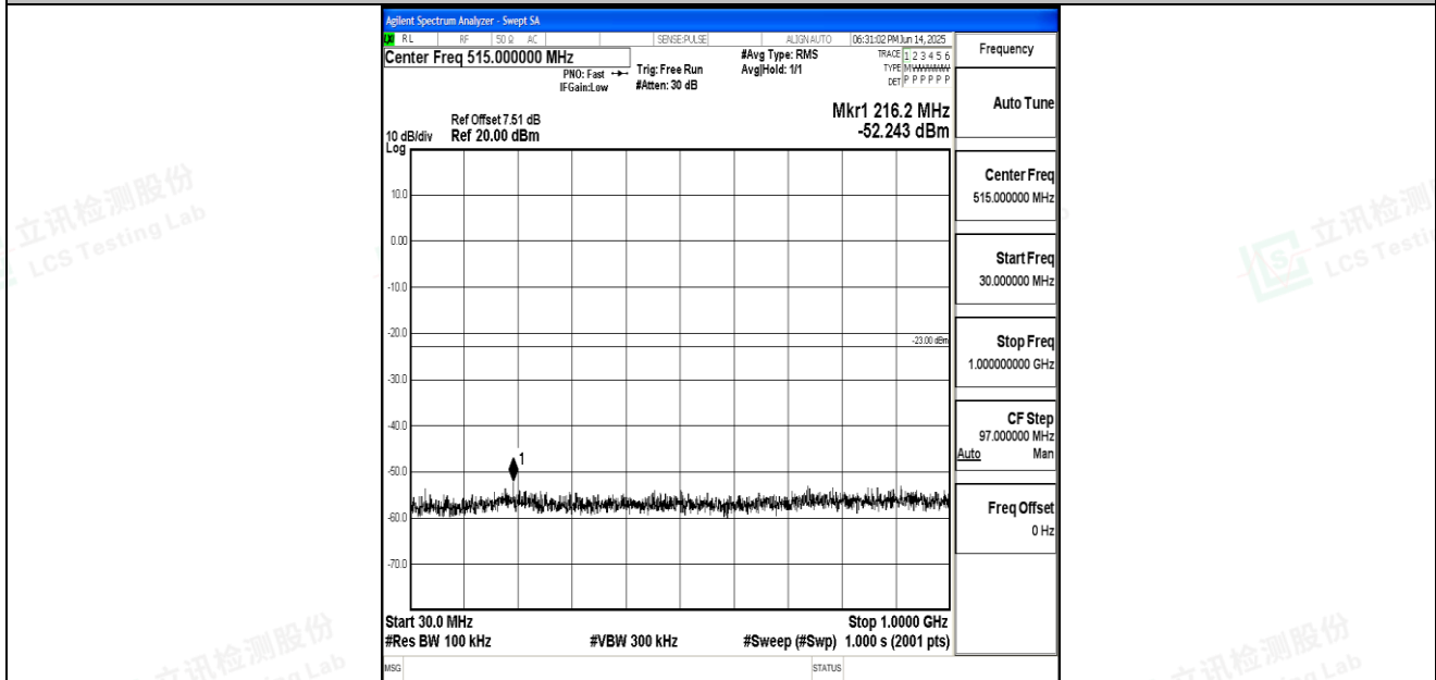
Band66_10MHz_16QAM_132022_1RB#0_30~1000_30~1000
