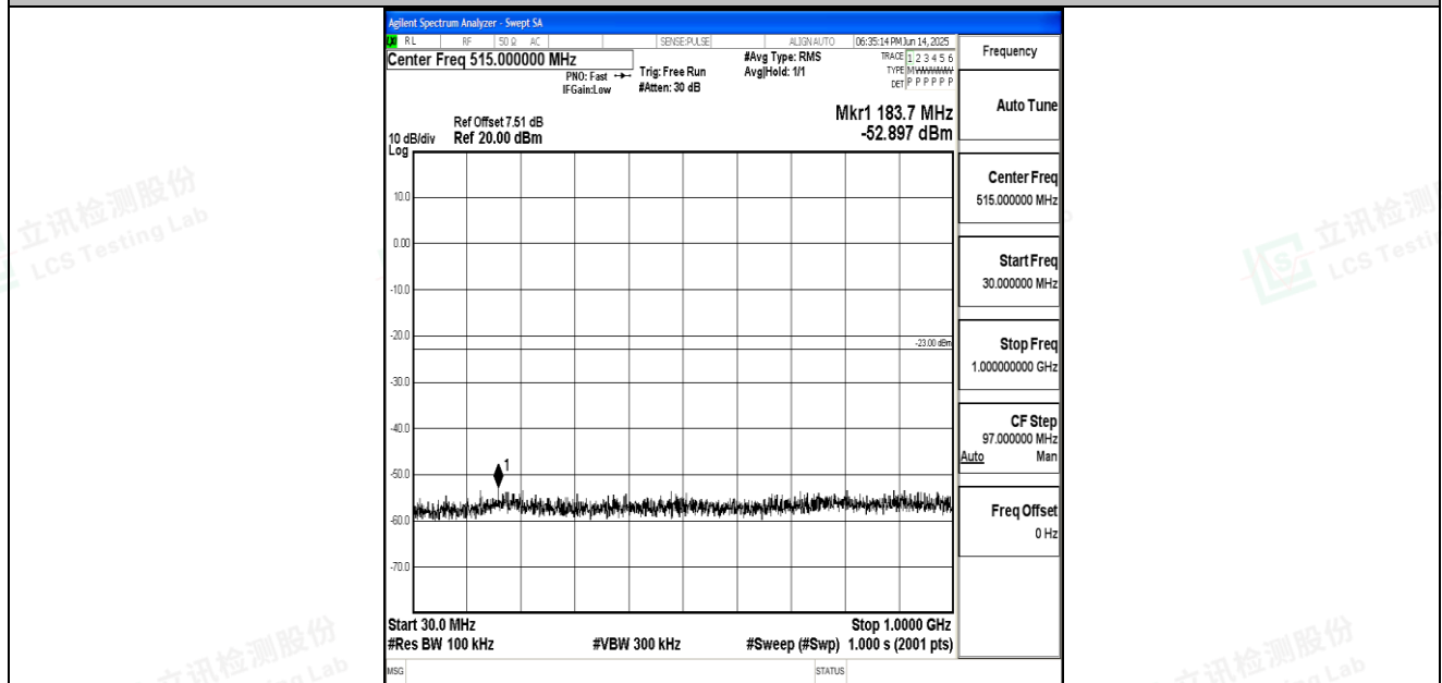
Band66_15MHz_16QAM_132047_1RB#0_30~1000_30~1000
