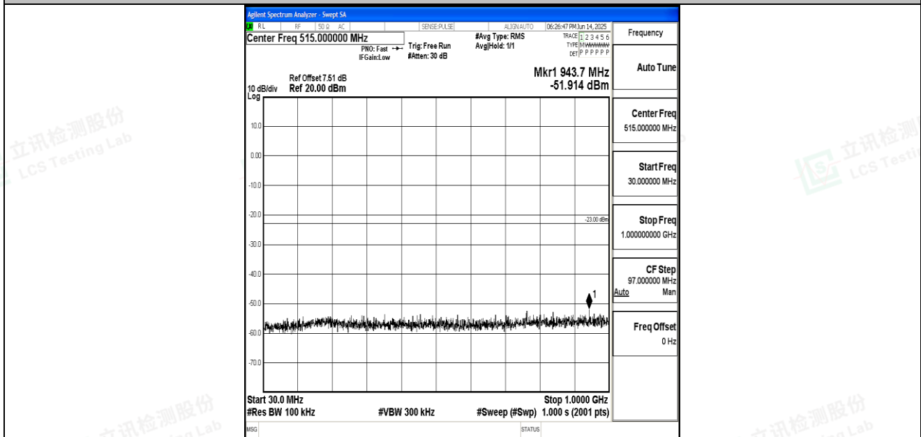
Band66_5MHz_16QAM_131997_1RB#0_30~1000_30~1000
