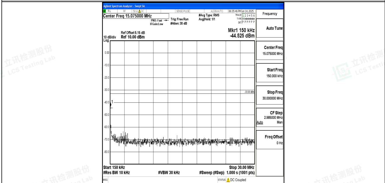
Band66_15MHz_QPSK_132322_1RB#0_0.15~30_0.15~30
