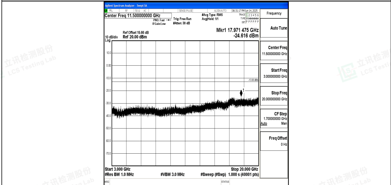
Band66_10MHz_16QAM_132022_1RB#0_3000~20000_3000~20000
