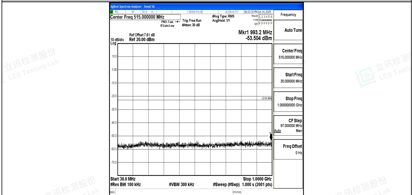
Band66_3MHz_16QAM_131987_1RB#0_30~1000_30~1000
