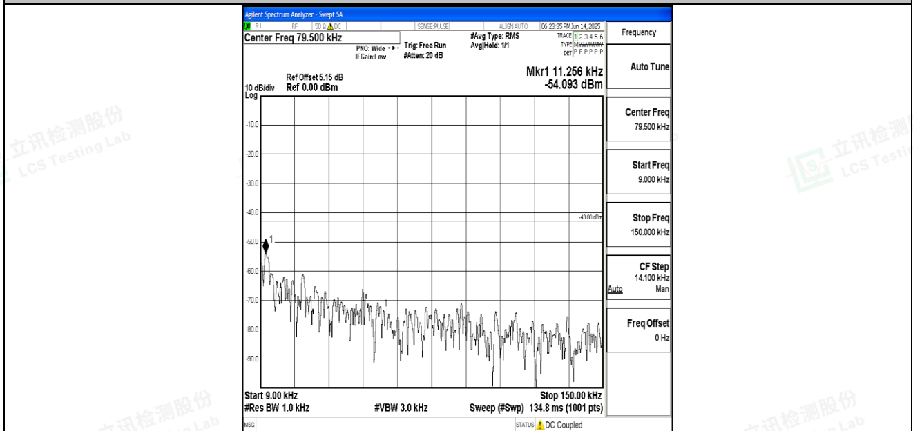
Band66_3MHz_16QAM_132322_1RB#0_0.009~0.15_0.009~0.15
