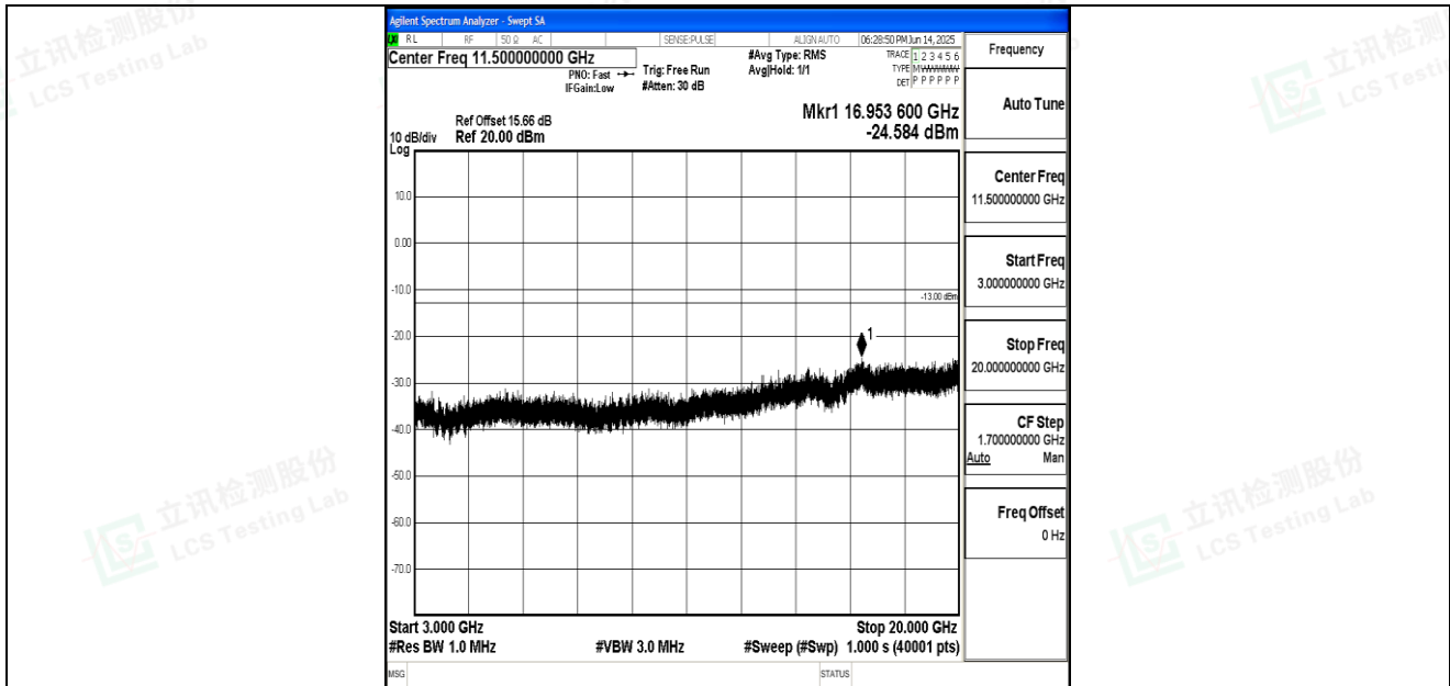
Band66_5MHz_QPSK_132647_1RB#0_3000~20000_3000~20000
