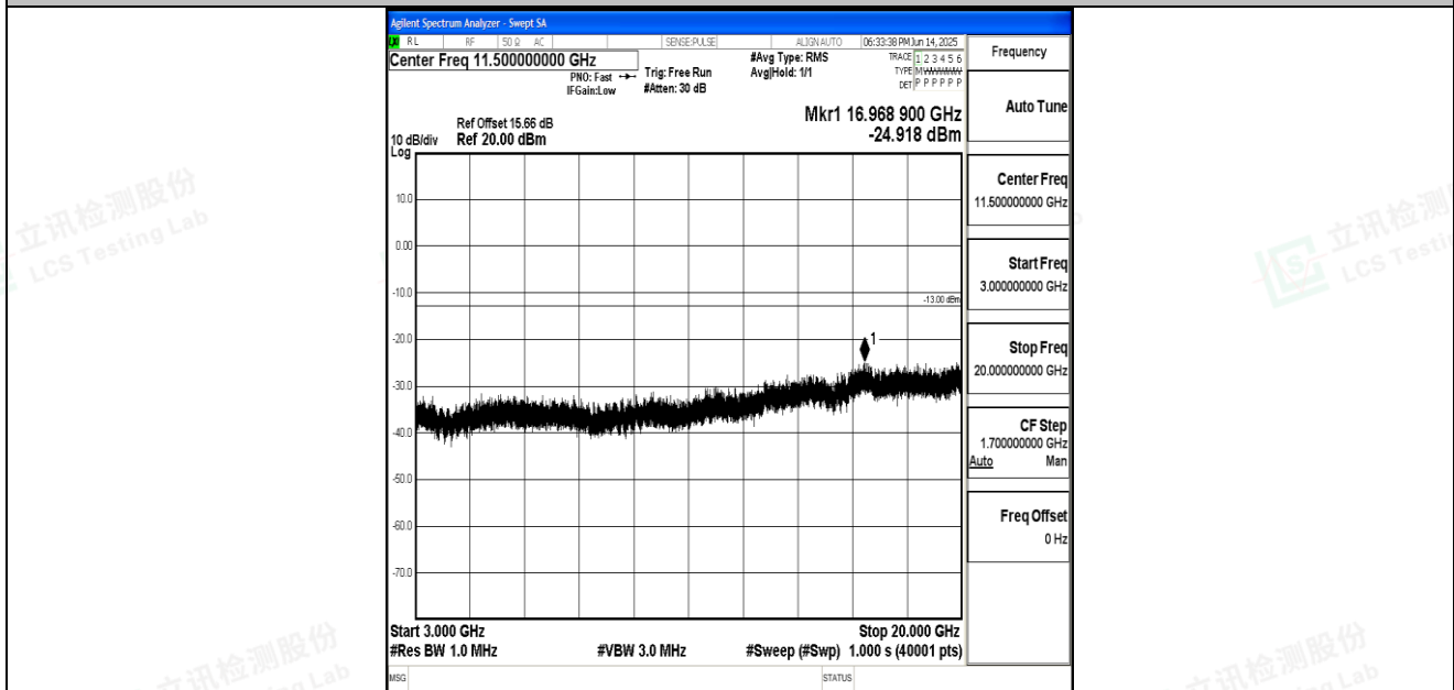
Band66_10MHz_16QAM_132622_1RB#0_3000~20000_3000~20000
