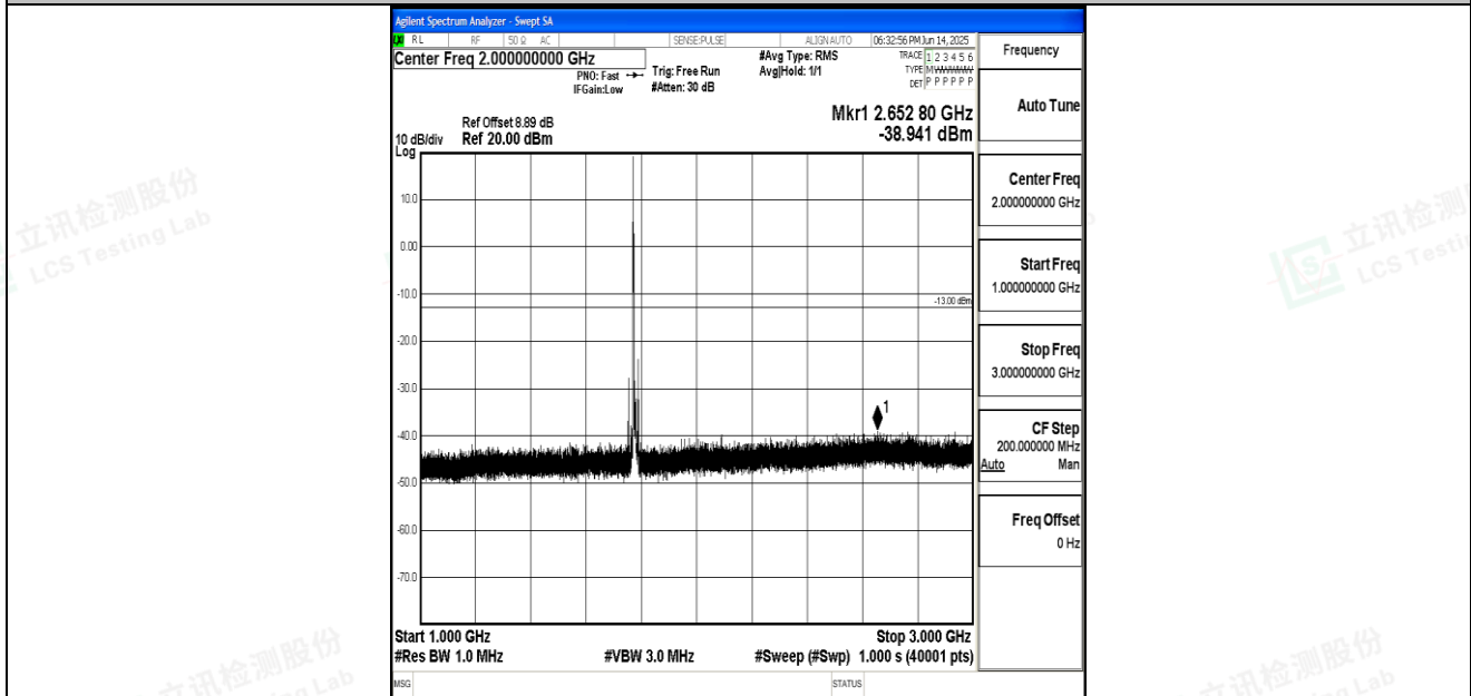
Band66_10MHz_QPSK_132622_1RB#0_1000~3000_1000~3000
