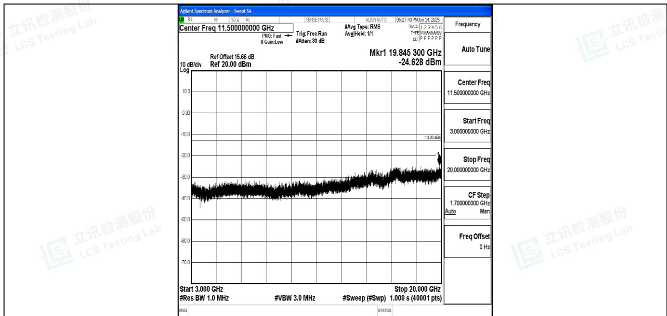
Band66_5MHz_QPSK_132322_1RB#0_3000~20000_3000~20000
