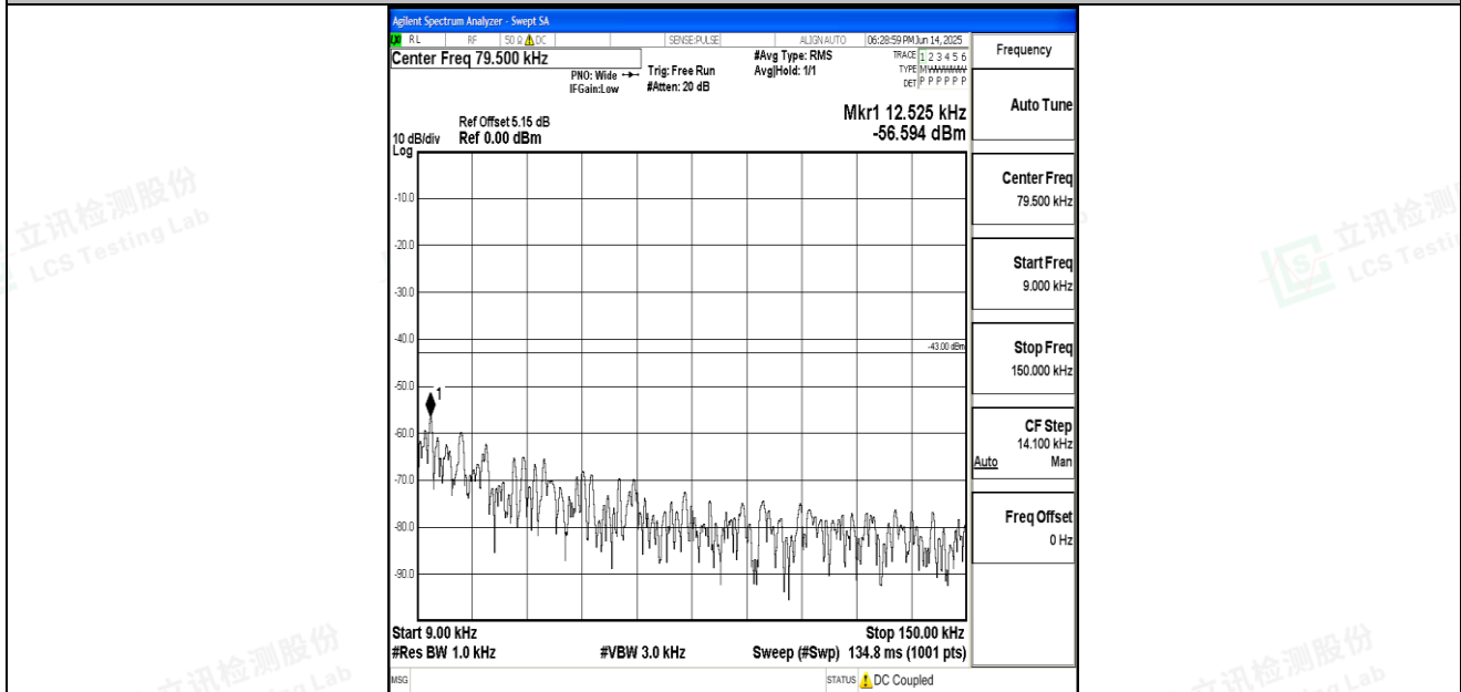
Band66_5MHz_16QAM_132647_1RB#0_0.009~0.15_0.009~0.15
