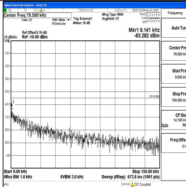
Band41_15MHz_16QAM_40620_1RB#0_0.009~0.15_0.009~0.15
