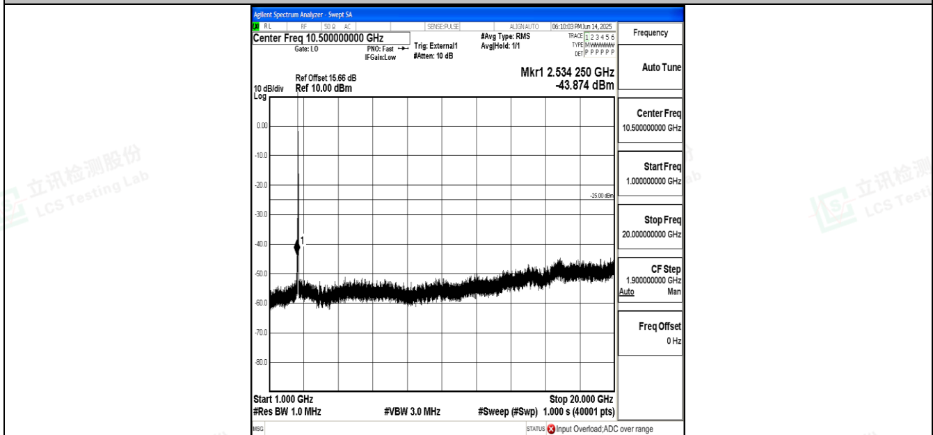
Band41_20MHz_QPSK_40620_1RB#0_1000~20000_1000~20000
