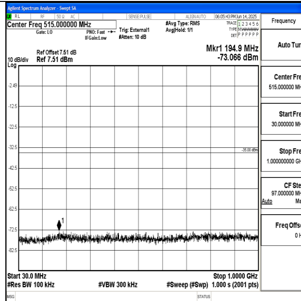
Band41_20MHz_QPSK_39750_1RB#0_30~1000_30~1000
