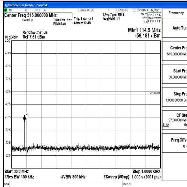
Band41_15MHz_QPSK_41515_1RB#0_30~1000_30~1000
