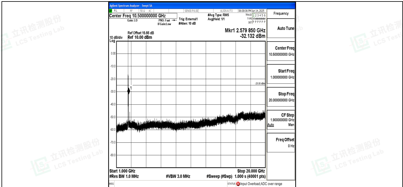
Band41_20MHz_16QAM_39750_1RB#0_1000~20000_1000~20000
