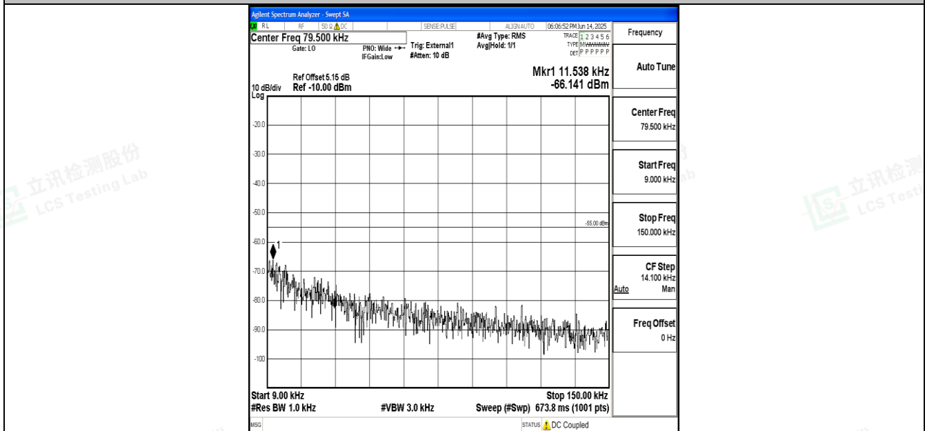
Band41_20MHz_16QAM_39750_1RB#0_0.009~0.15_0.009~0.15
