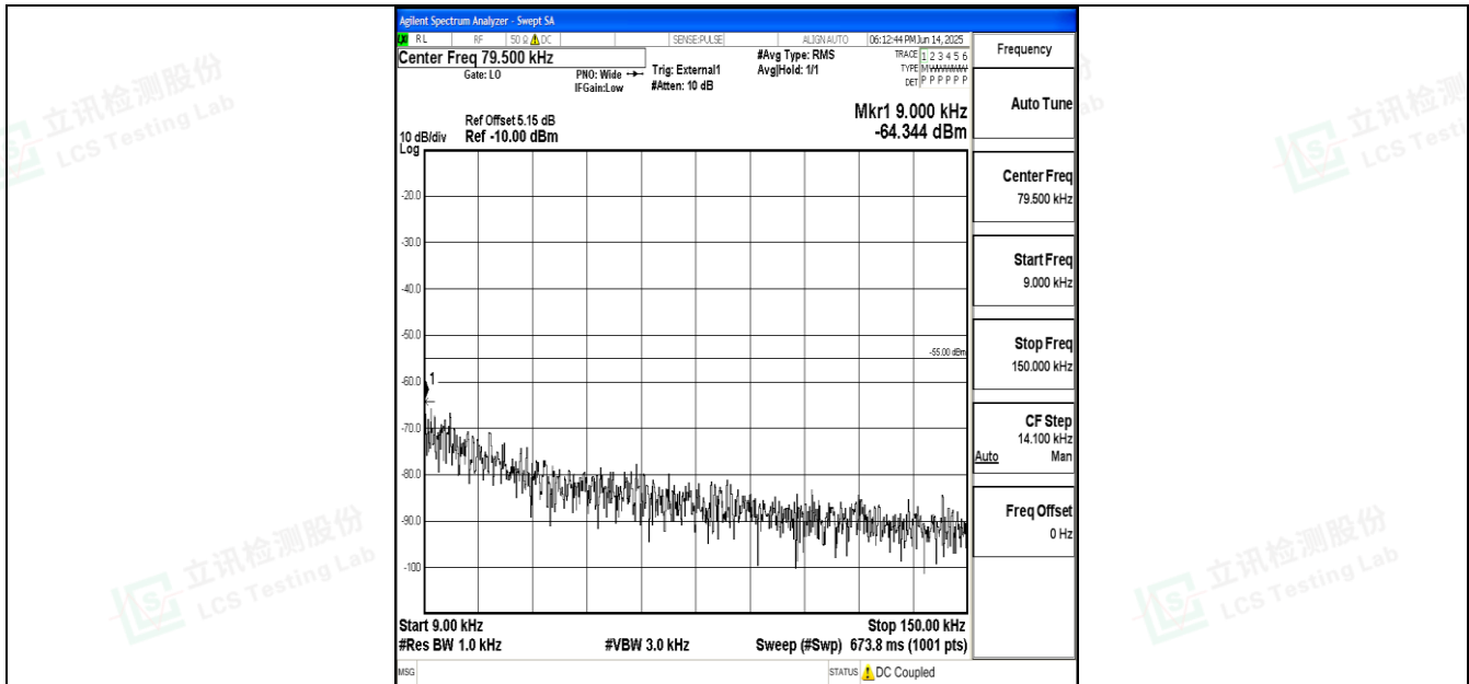
Band41_20MHz_QPSK_41490_1RB#0_0.009~0.15_0.009~0.15
