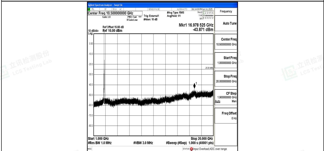
Band41_20MHz_QPSK_41490_1RB#0_1000~20000_1000~20000
