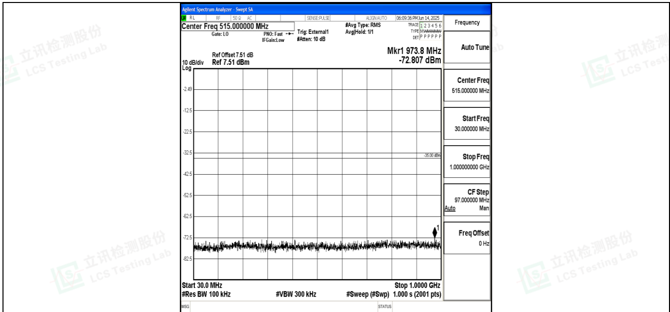
Band41_20MHz_QPSK_40620_1RB#0_30~1000_30~1000
