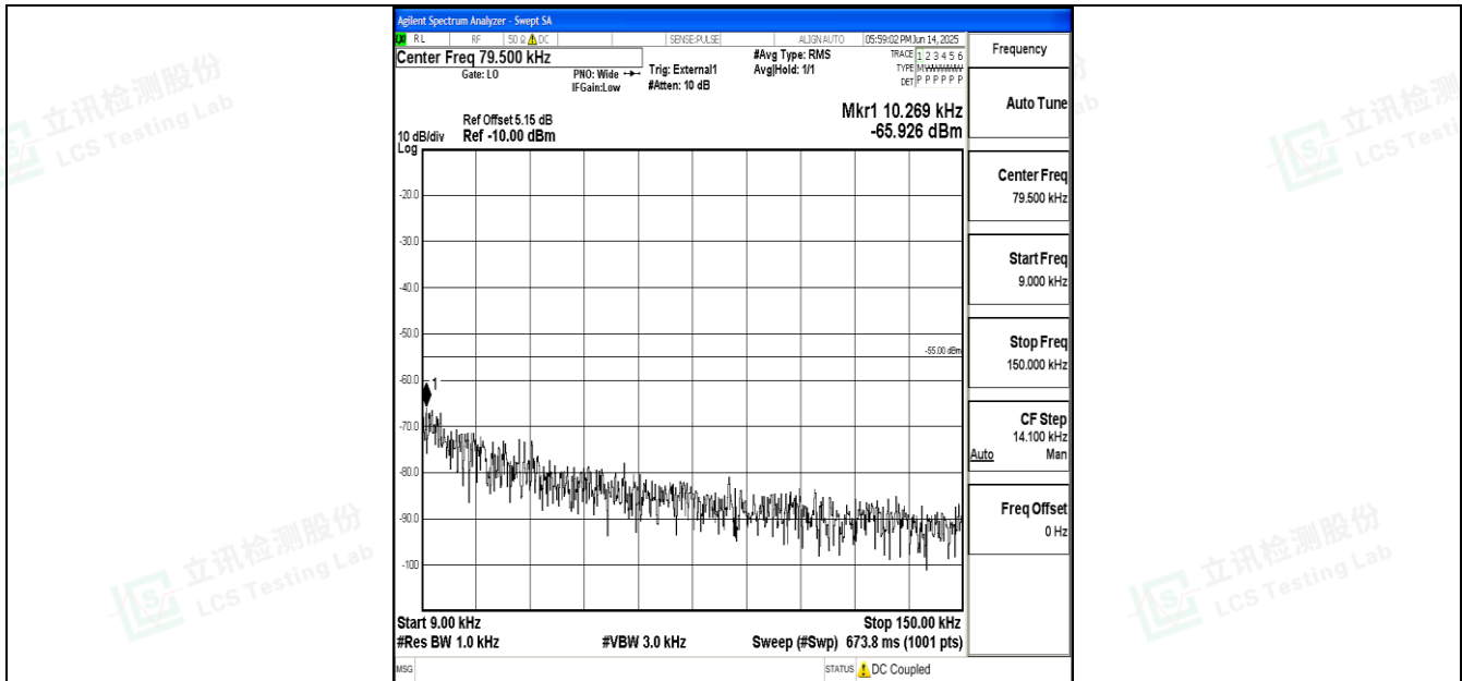
Band41_15MHz_QPSK_41515_1RB#0_0.009~0.15_0.009~0.15
