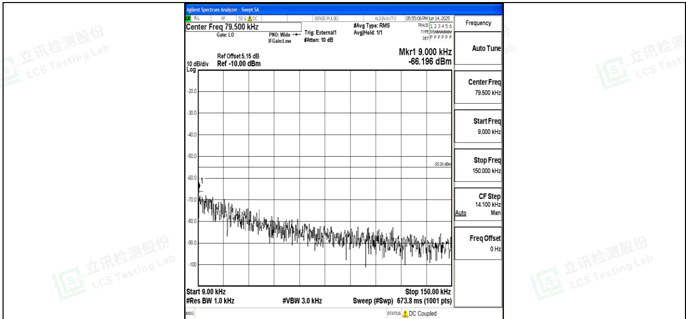
Band41_15MHz_QPSK_40620_1RB#0_0.009~0.15_0.009~0.15
