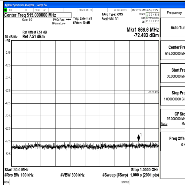
Band41_15MHz_QPSK_40620_1RB#0_30~1000_30~1000
