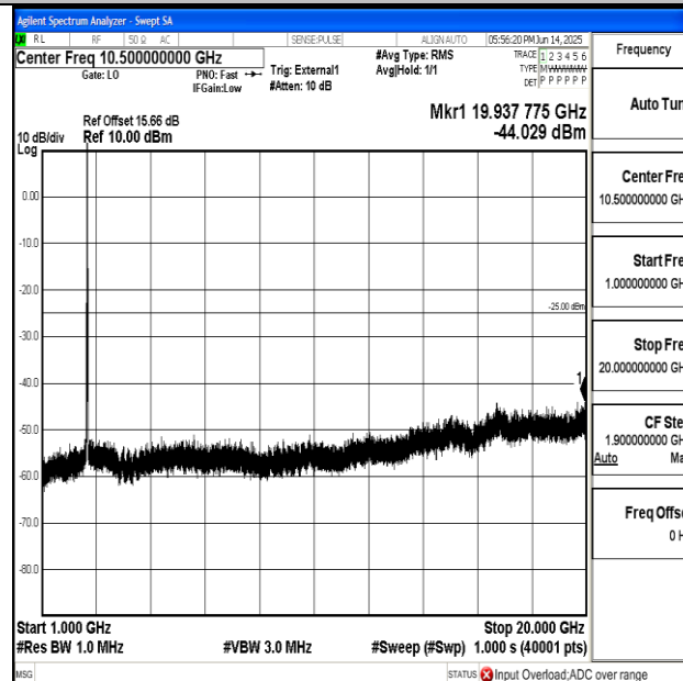
Band41 15MHz QPSK 40620 1RB#0 1000~20000 1000~20000
