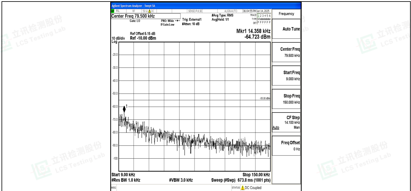
Band41_20MHz_QPSK_39750_1RB#0_0.009~0.15_0.009~0.15
