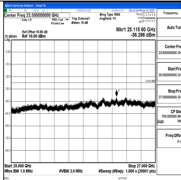
Band41_20MHz_16QAM_40620_1RB#0_20000~27000_20000~27000
