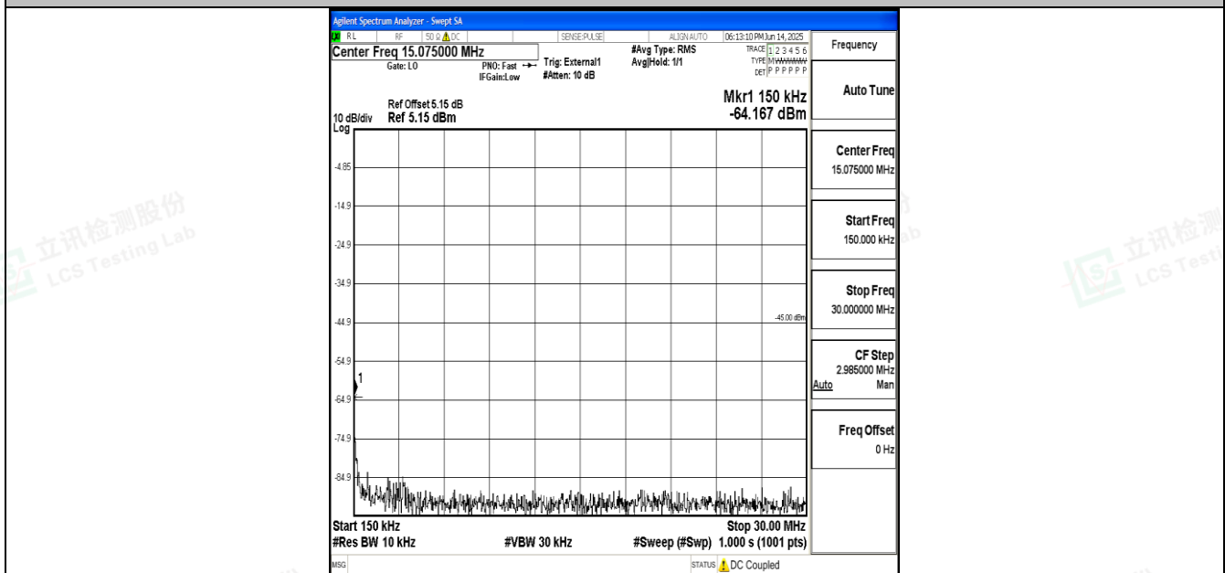
Band41_20MHz_QPSK_41490_1RB#0_0.15~30_0.15~30
