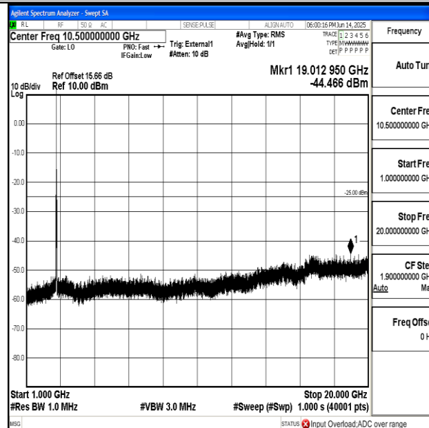
Band41_15MHz_QPSK_41515_1RB#0_1000~20000_1000~20000
