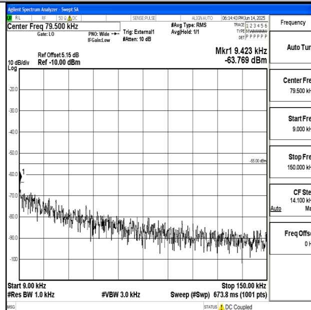
Band41_20MHz_16QAM_41490_1RB#0_0.009~0.15_0.009~0.15
