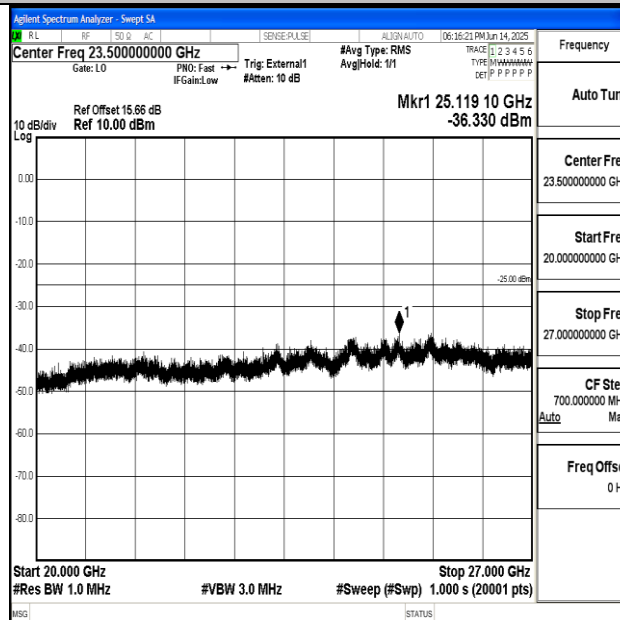
Band41_20MHz_16QAM_41490_1RB#0_20000~27000_20000~27000
