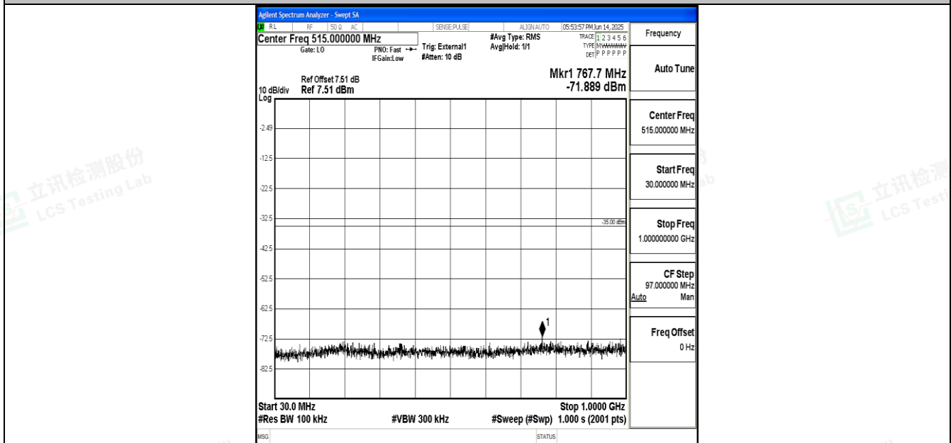
Band41_15MHz_16QAM_39725_1RB#0_30~1000_30~1000
