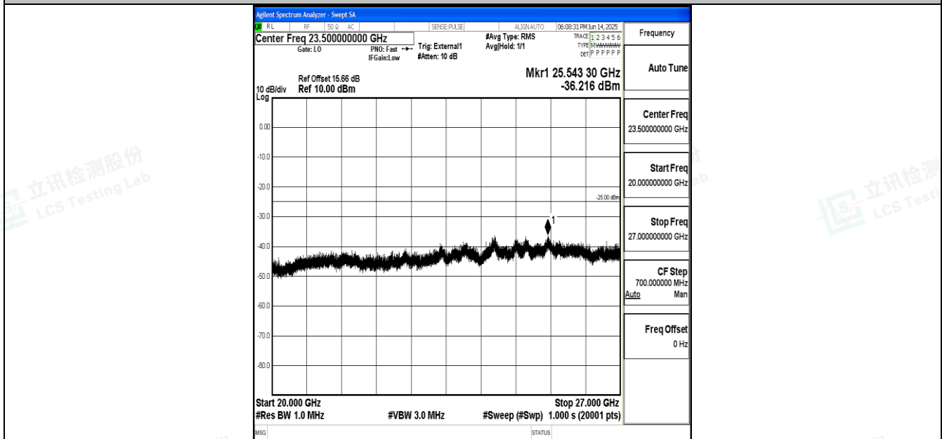
Band41_20MHz_16QAM_39750_1RB#0_20000~27000_20000~27000
