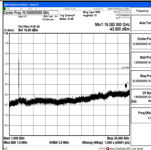
Band41_20MHz_QPSK_39750_1RB#0_1000~20000_1000~20000
