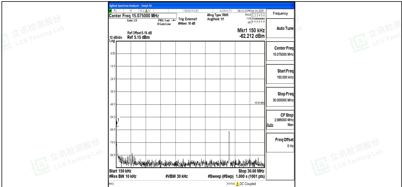
Band41_20MHz_16QAM_40620_1RB#0_0.15~30_0.15~30
