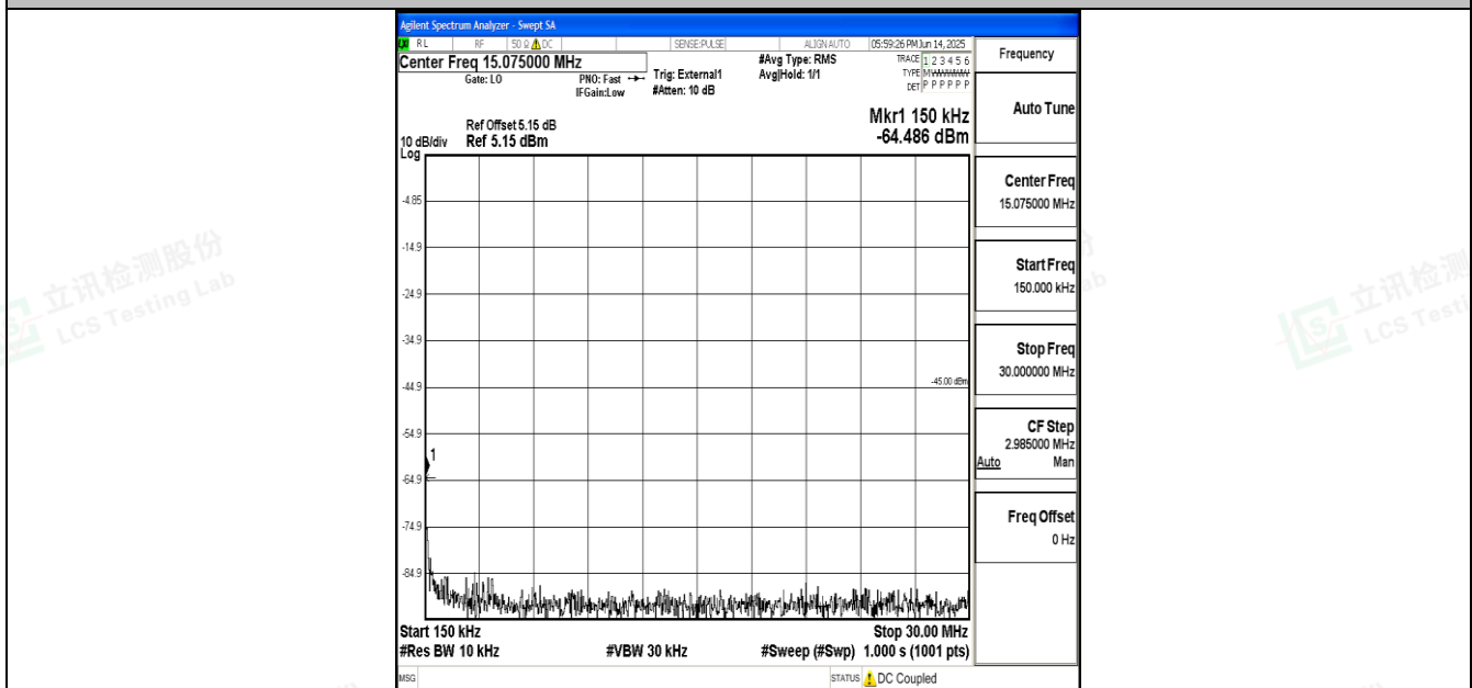
Band41_15MHz_QPSK_41515_1RB#0_0.15~30_0.15~30
