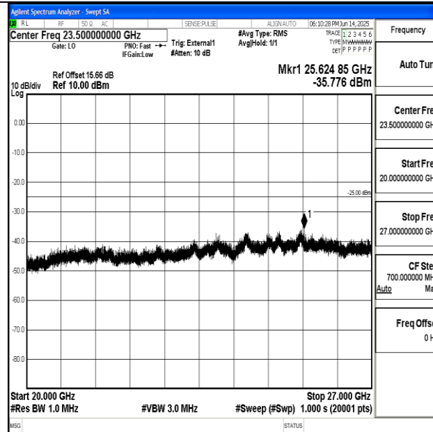
Band41_20MHz_QPSK_40620_1RB#0_20000~27000_20000~27000
