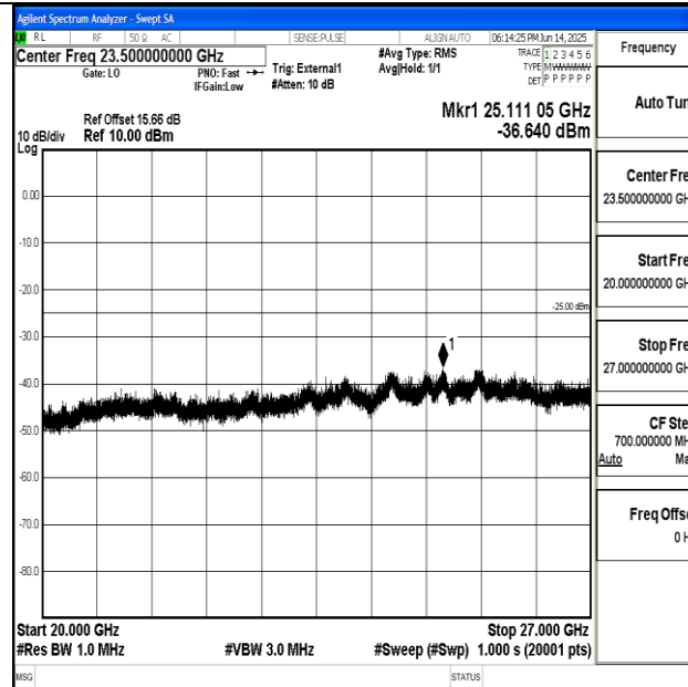
Band41_20MHz_QPSK_41490_1RB#0_20000~27000_20000~27000
