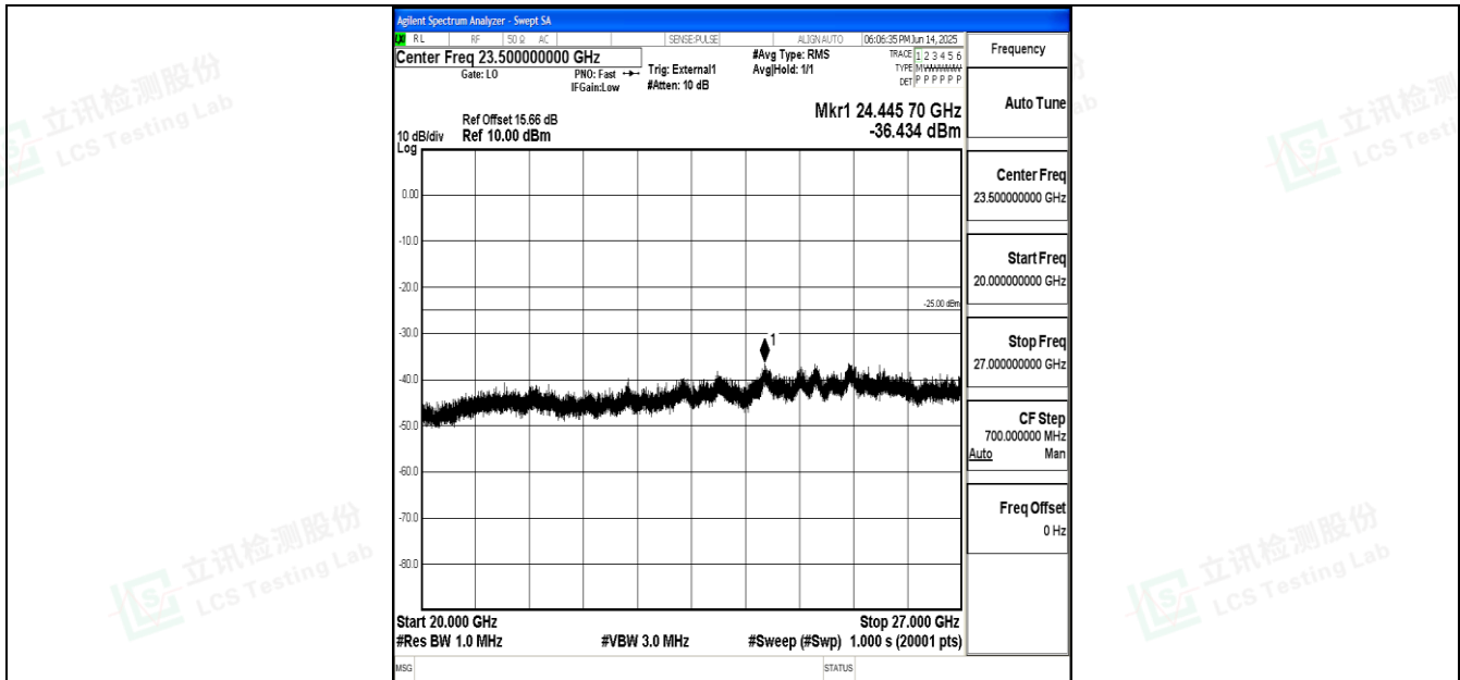
Band41_20MHz_QPSK_39750_1RB#0_20000~27000_20000~27000
