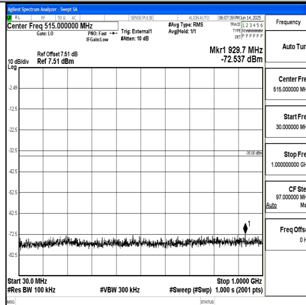
Band41 20MHz 16QAM 39750 1RB#0 30~1000 30~1000
