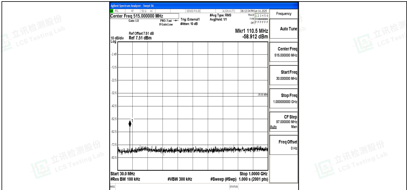
Band41_20MHz_QPSK_41490_1RB#0_30~1000_30~1000
