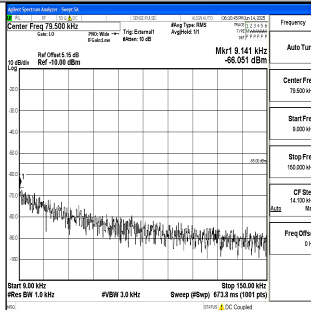
Band41_20MHz_16QAM_40620_1RB#0_0.009~0.15_0.009~0.15
