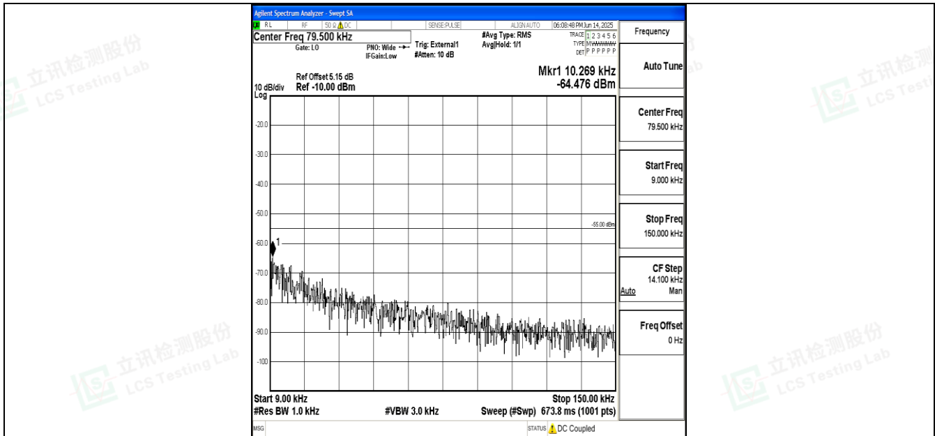
Band41_20MHz_QPSK_40620_1RB#0_0.009~0.15_0.009~0.15
