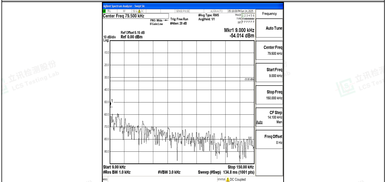
Band26_15MHz_16QAM_26865_1RB#0_0.009~0.15_0.009~0.15
