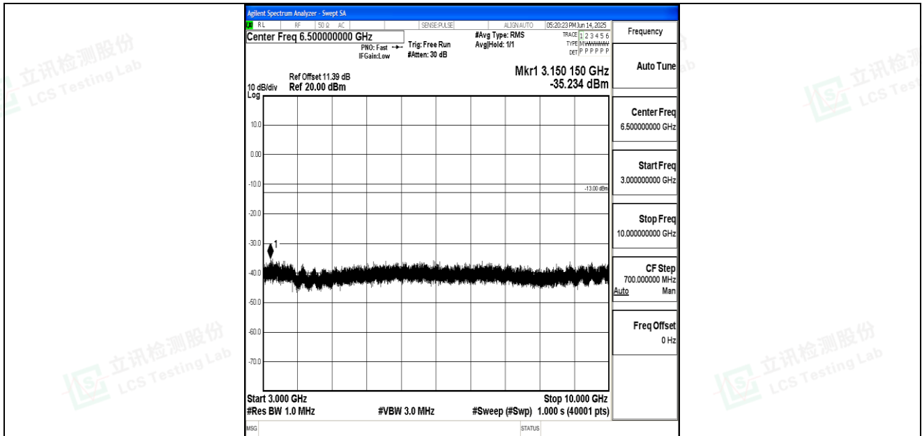
Band26_15MHz_QPSK_26965_1RB#0_3000~10000_3000~10000
