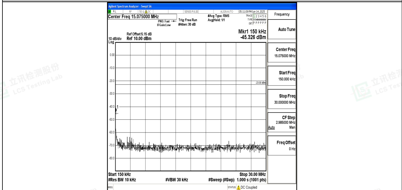
Band26_5MHz_QPSK_27015_1RB#0_0.15~30_0.15~30
