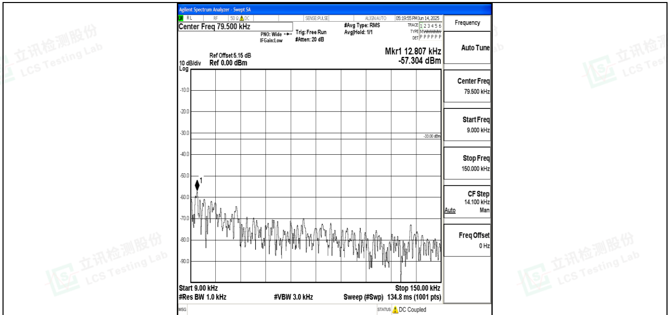
Band26_15MHz_QPSK_26965_1RB#0_0.009~0.15_0.009~0.15
