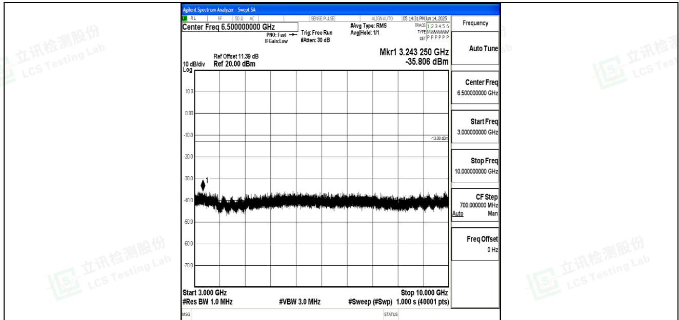
Band26_10MHz_QPSK_26915_1RB#0_3000~10000_3000~10000
