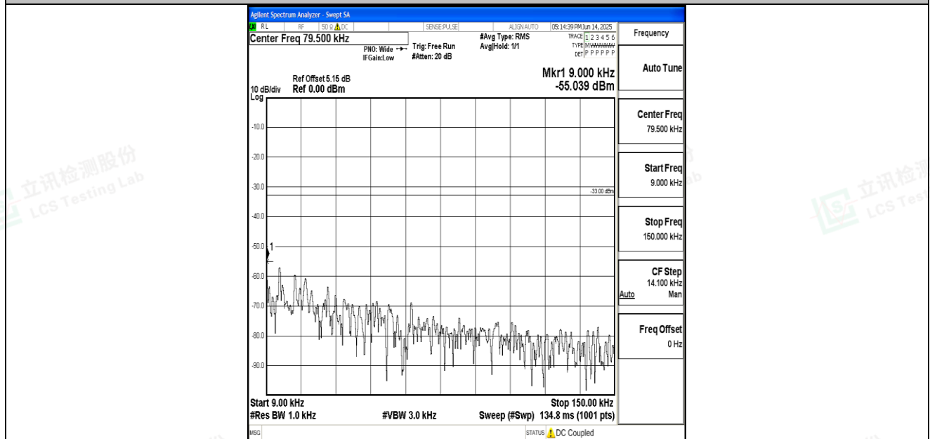
Band26_10MHz_16QAM_26915_1RB#0_0.009~0.15_0.009~0.15
