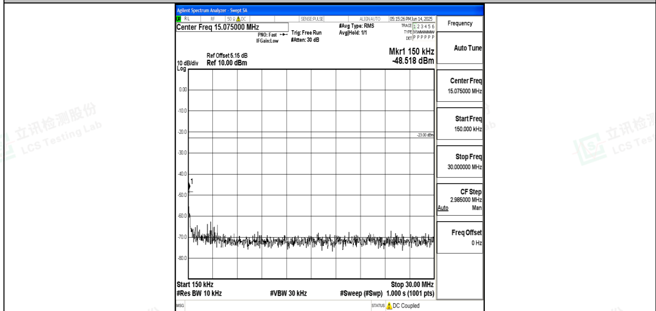
Band26_10MHz_QPSK_26990_1RB#0_0.15~30_0.15~30
