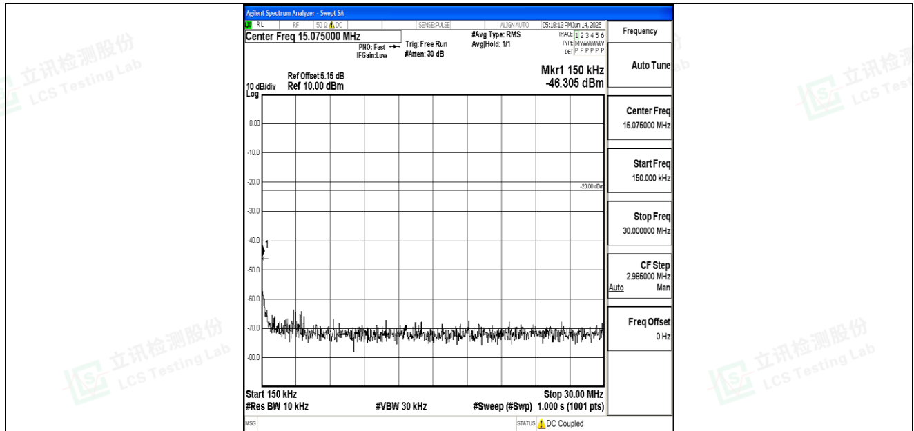
Band26_15MHz_16QAM_26865_1RB#0_0.15~30_0.15~30
