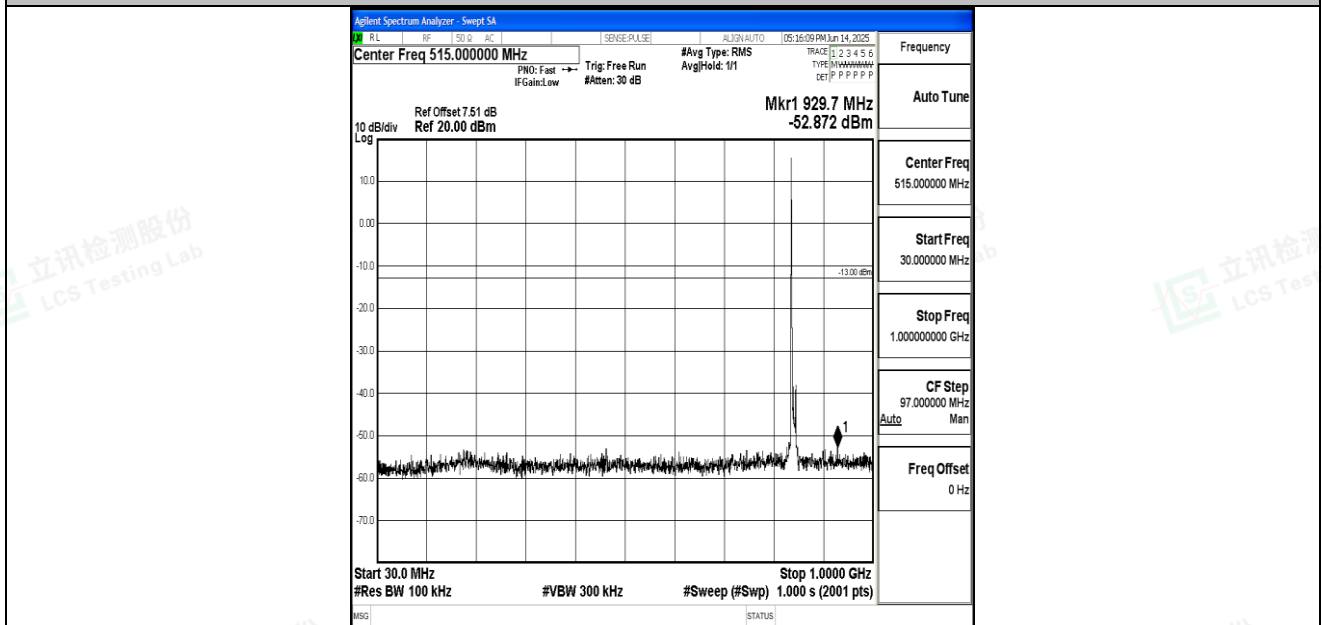
Band26_10MHz_16QAM_26990_1RB#0_30~1000_30~1000
