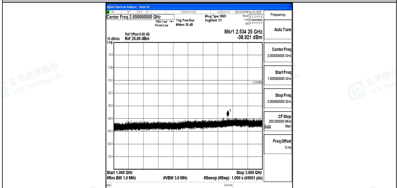
Band26_10MHz_QPSK_26915_1RB#0_1000~3000_1000~3000
