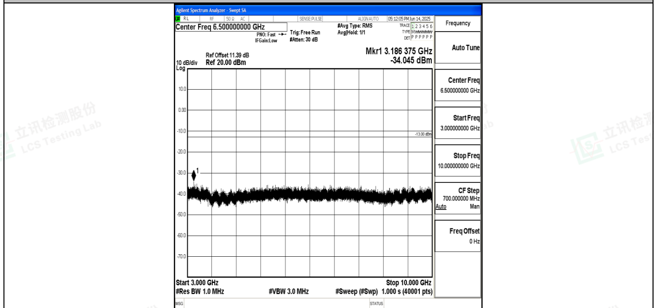
Band26_5MHz_16QAM_27015_1RB#0_3000~10000_3000~10000
