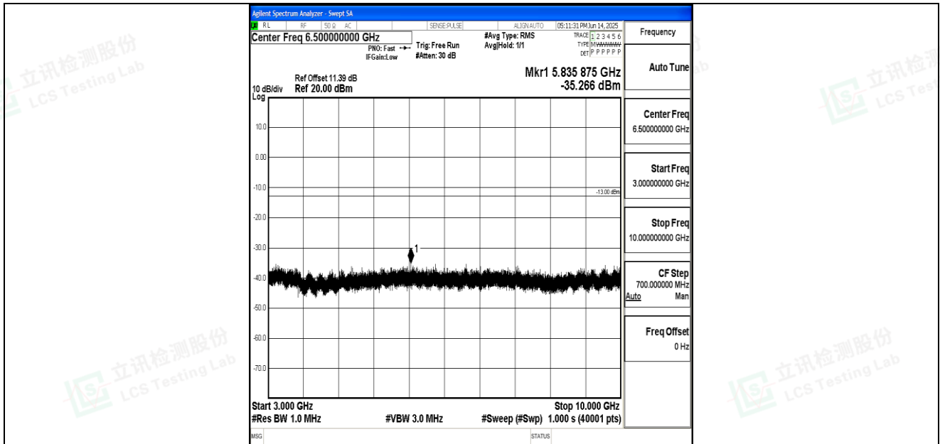
Band26_5MHz_QPSK_27015_1RB#0_3000~10000_3000~10000
