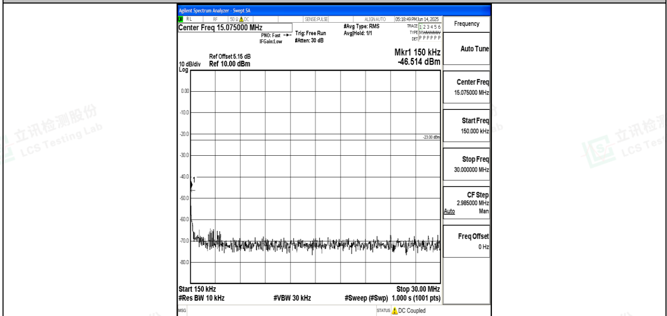
Band26_15MHz_QPSK_26915_1RB#0_0.15~30_0.15~30
