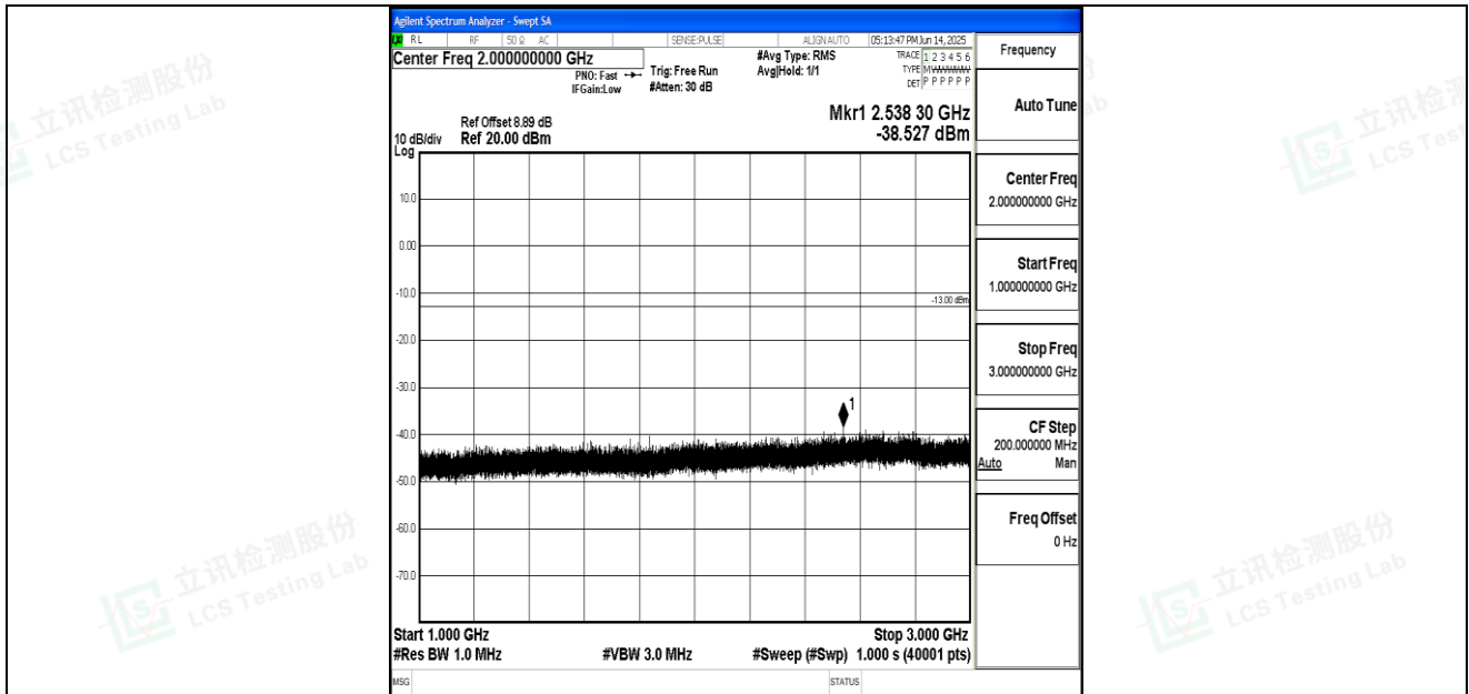
Band26_10MHz_16QAM_26840_1RB#0_1000~3000_1000~3000
