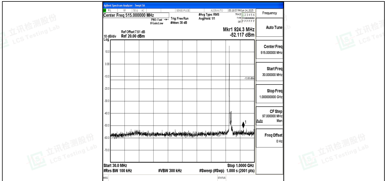
Band26_15MHz_QPSK_26915_1RB#0_30~1000_30~1000
