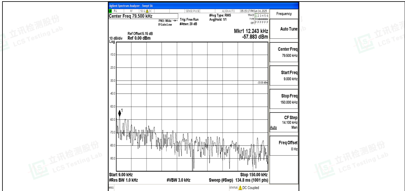
Band26_10MHz_QPSK_26990_1RB#0_0.009~0.15_0.009~0.15
