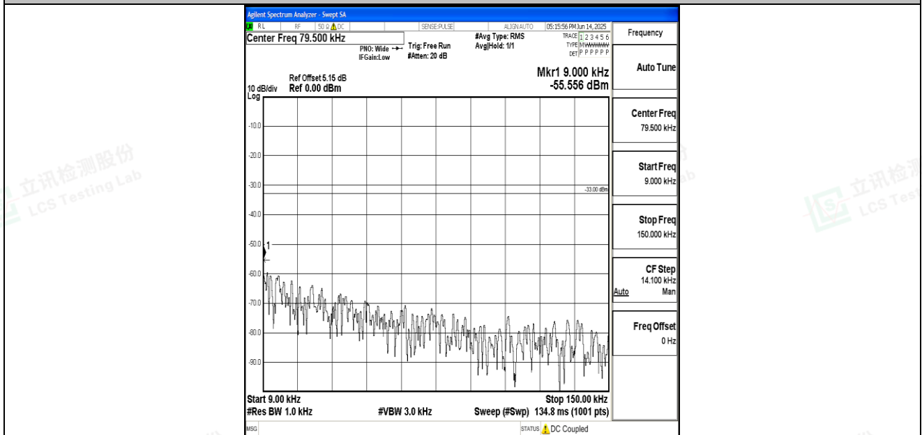
Band26_10MHz_16QAM_26990_1RB#0_0.009~0.15_0.009~0.15
