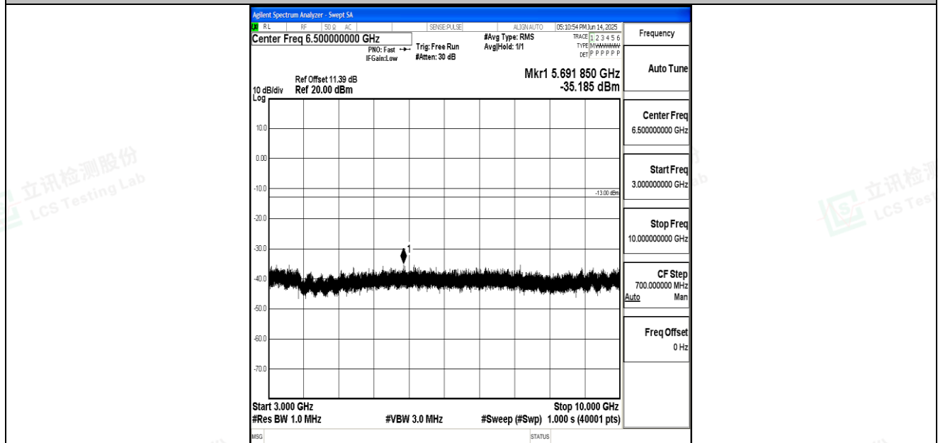
Band26_5MHz_16QAM_26915_1RB#0_3000~10000_3000~10000
