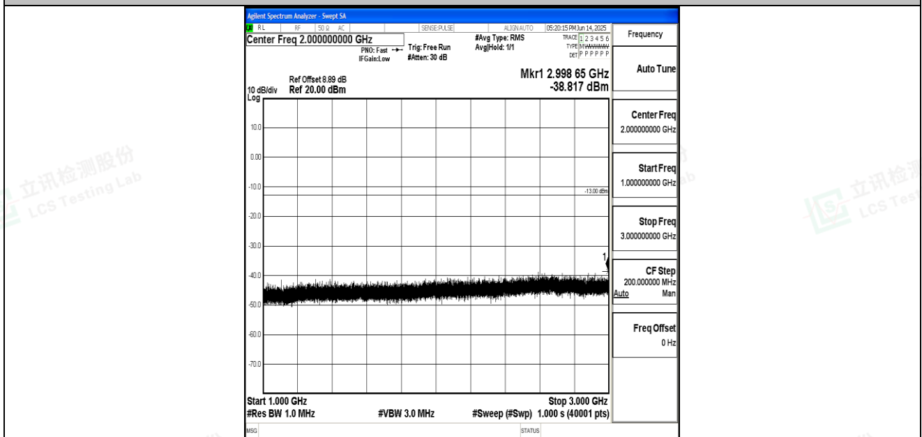
Band26_15MHz_QPSK_26965_1RB#0_1000~3000_1000~3000
