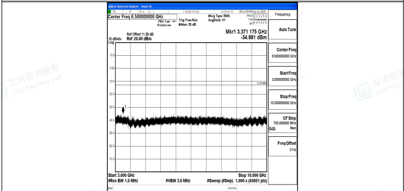
Band26_10MHz_16QAM_26840_1RB#0_3000~10000_3000~10000
