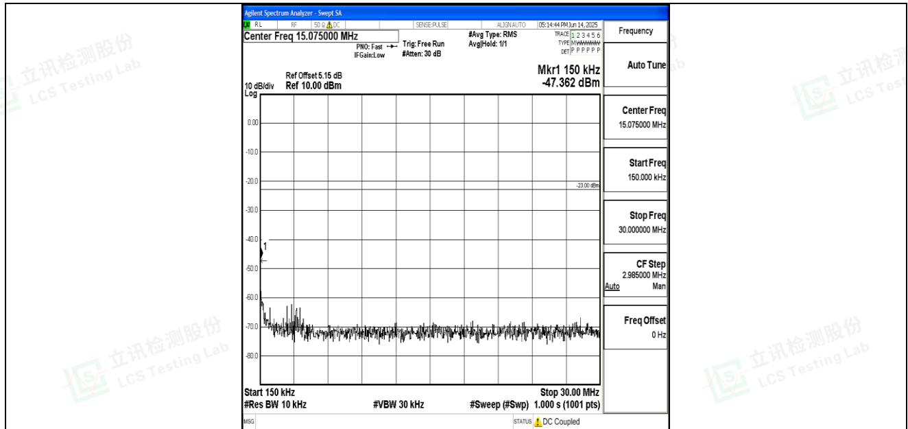
Band26_10MHz_16QAM_26915_1RB#0_0.15~30_0.15~30
