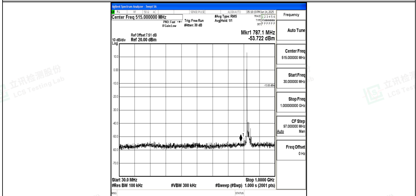
Band26_15MHz_16QAM_26865_1RB#0_30~1000_30~1000
