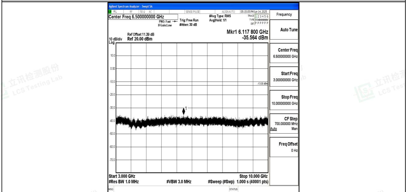
Band26_10MHz_16QAM_26915_1RB#0_3000~10000_3000~10000
