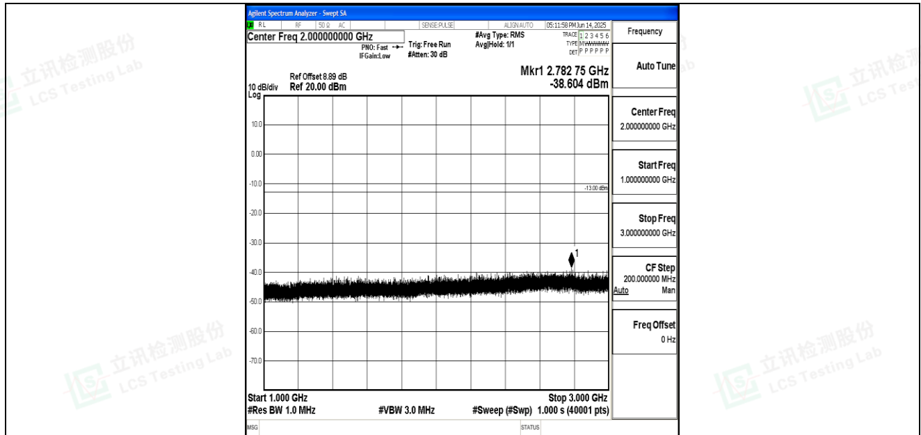
Band26_5MHz_16QAM_27015_1RB#0_1000~3000_1000~3000
