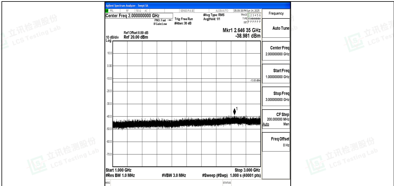
Band26_5MHz_16QAM_26815_1RB#0_1000~3000_1000~3000
