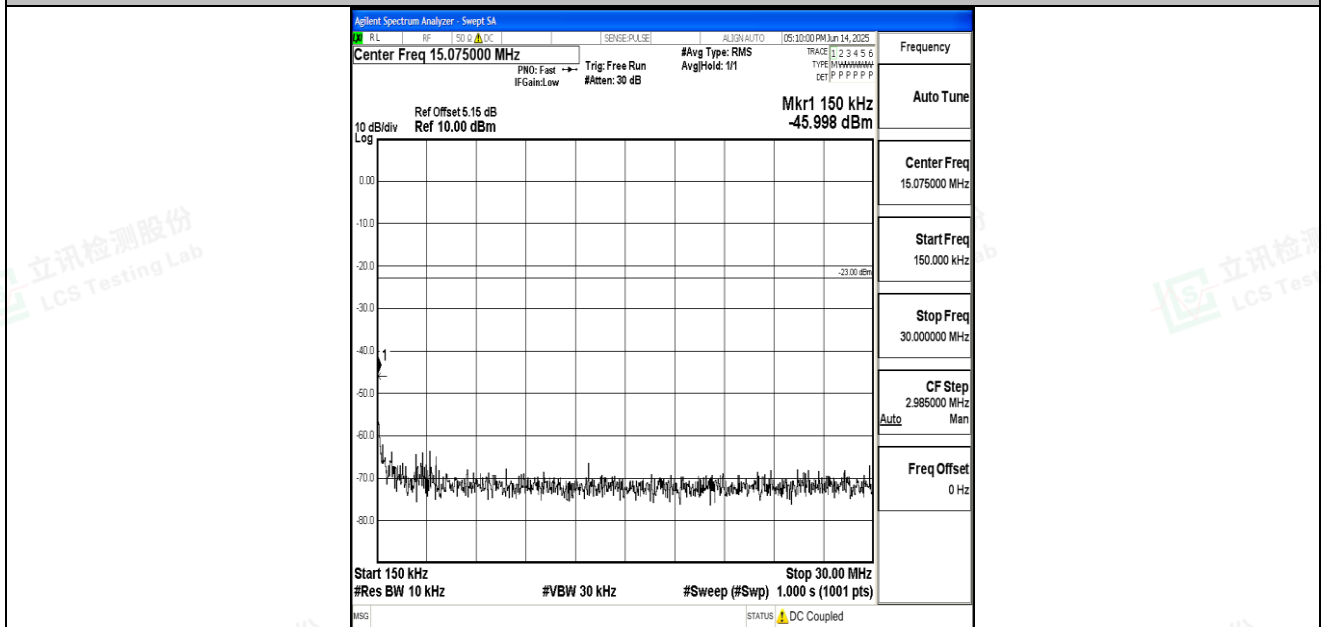
Band26_5MHz_QPSK_26915_1RB#0_0.15~30_0.15~30
