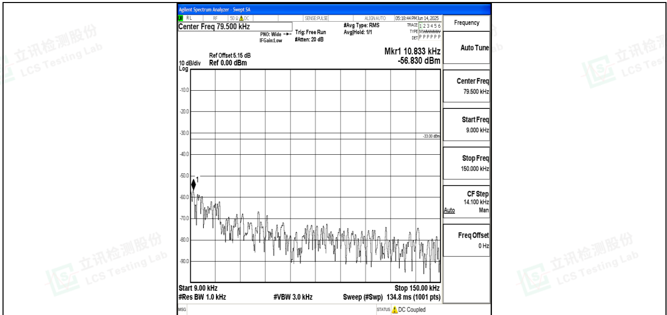
Band26_15MHz_QPSK_26915_1RB#0_0.009~0.15_0.009~0.15
