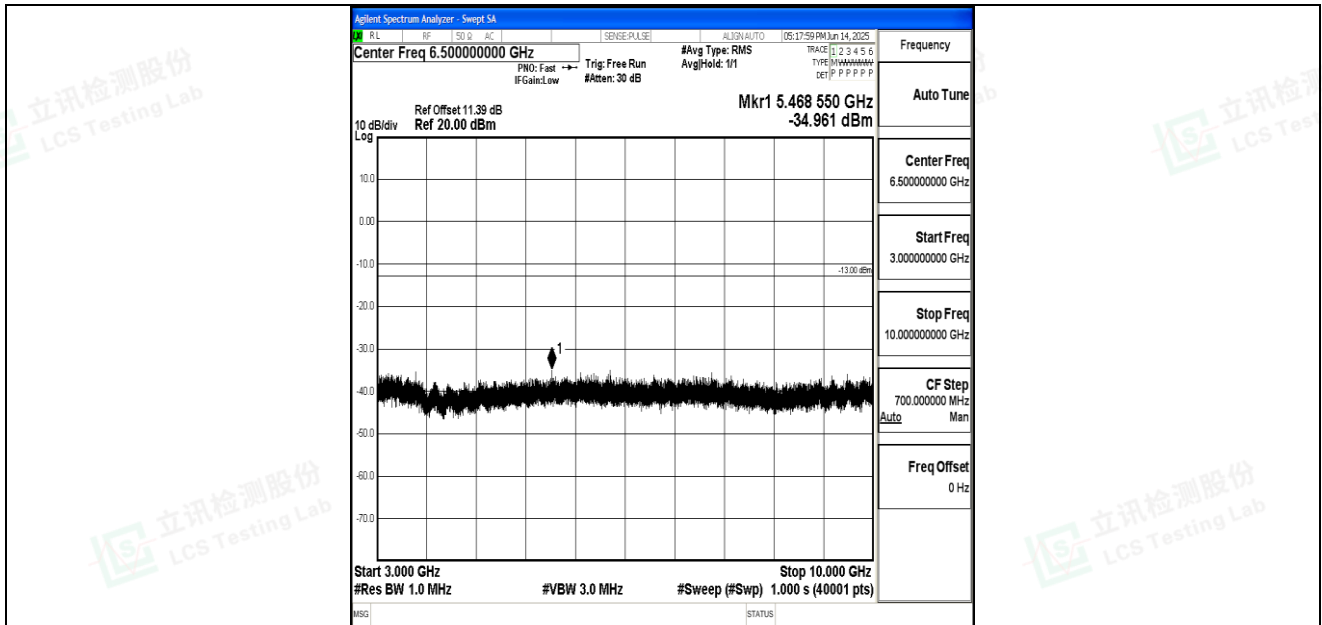
Band26_15MHz_QPSK_26865_1RB#0_3000~10000_3000~10000
