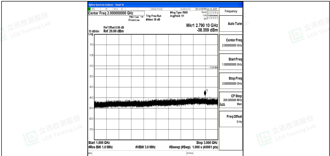
Band26_10MHz_16QAM_26915_1RB#0_1000~3000_1000~3000
