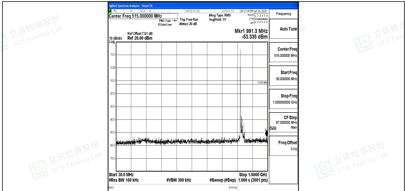
Band26_15MHz_QPSK_26865_1RB#0_30~1000_30~1000
