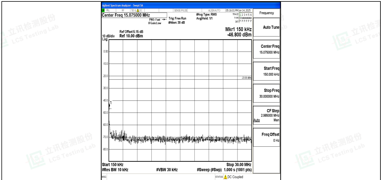
Band26_10MHz_16QAM_26990_1RB#0_0.15~30_0.15~30
