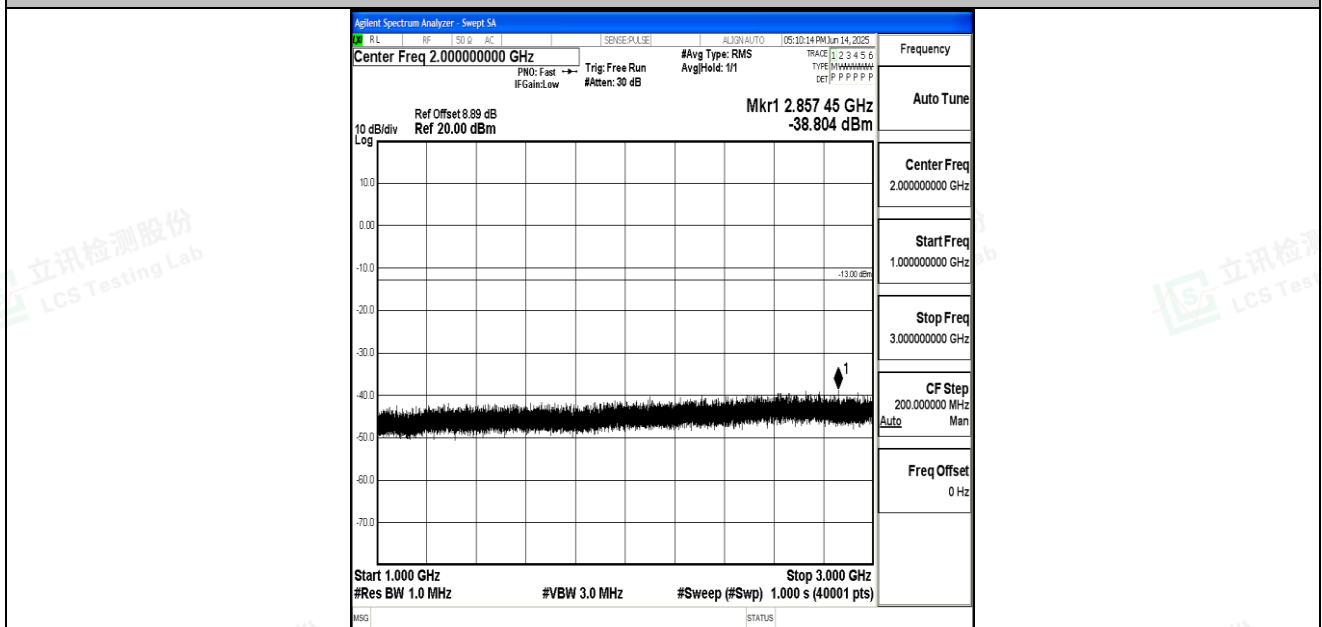
Band26_5MHz_QPSK_26915_1RB#0_1000~3000_1000~3000
