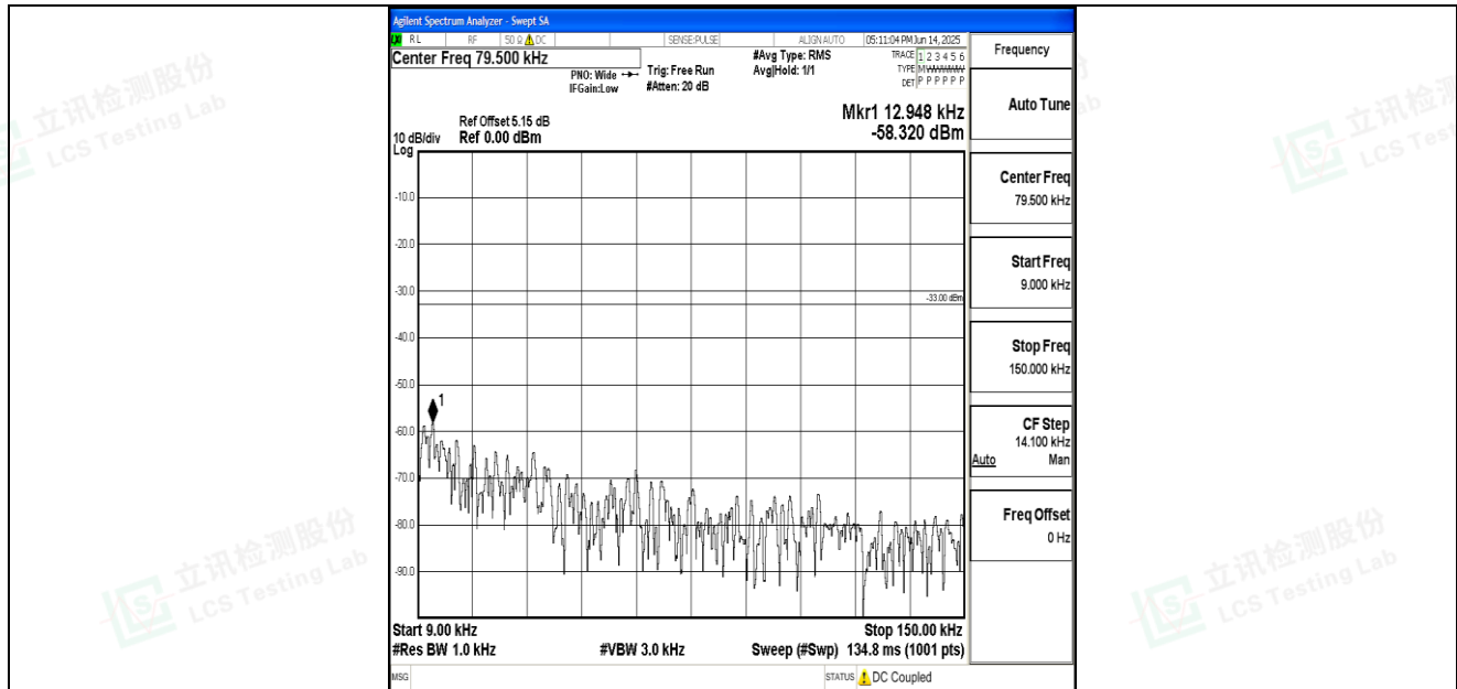
Band26_5MHz_QPSK_27015_1RB#0_0.009~0.15_0.009~0.15
