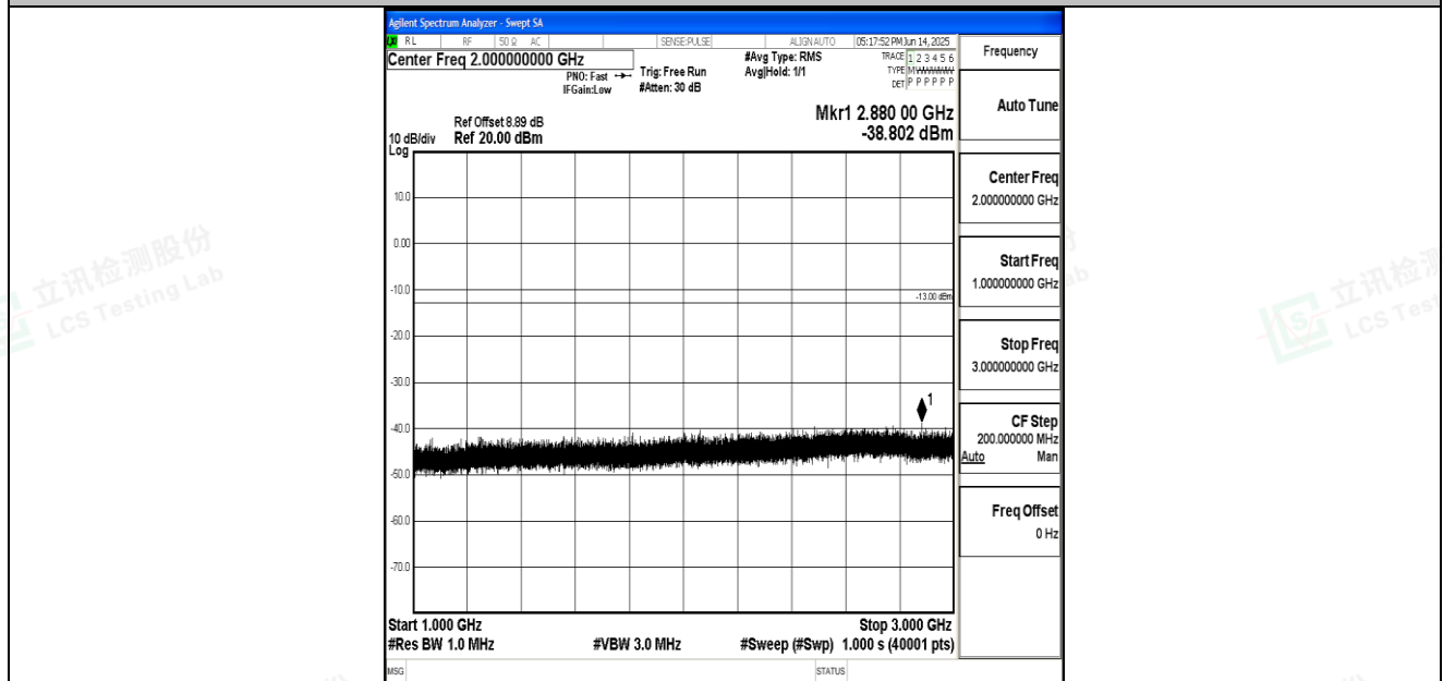
Band26_15MHz_QPSK_26865_1RB#0_1000~3000_1000~3000
