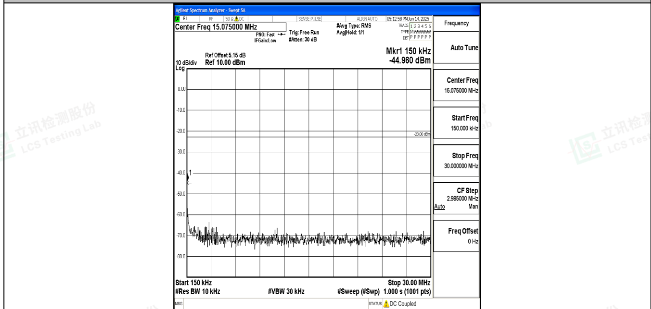
Band26_10MHz_QPSK_26840_1RB#0_0.15~30_0.15~30
