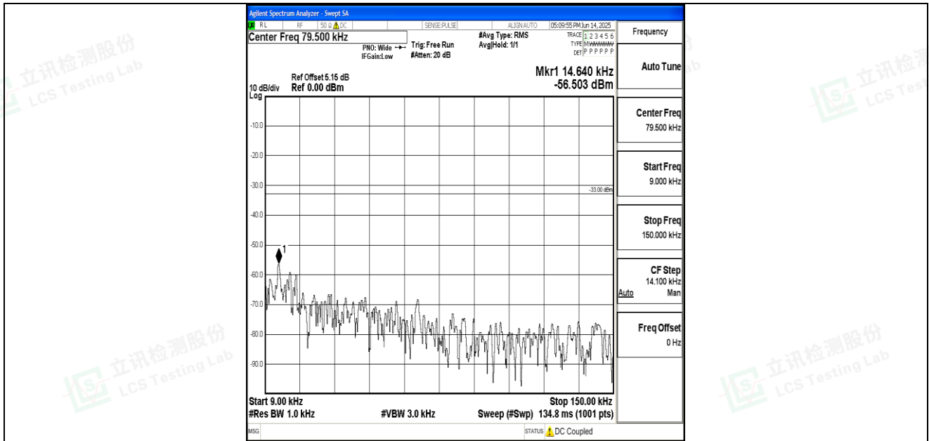
Band26_5MHz_QPSK_26915_1RB#0_0.009~0.15_0.009~0.15
