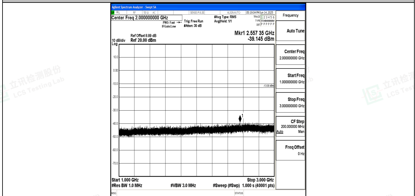
Band26_15MHz_QPSK_26915_1RB#0_1000~3000_1000~3000
