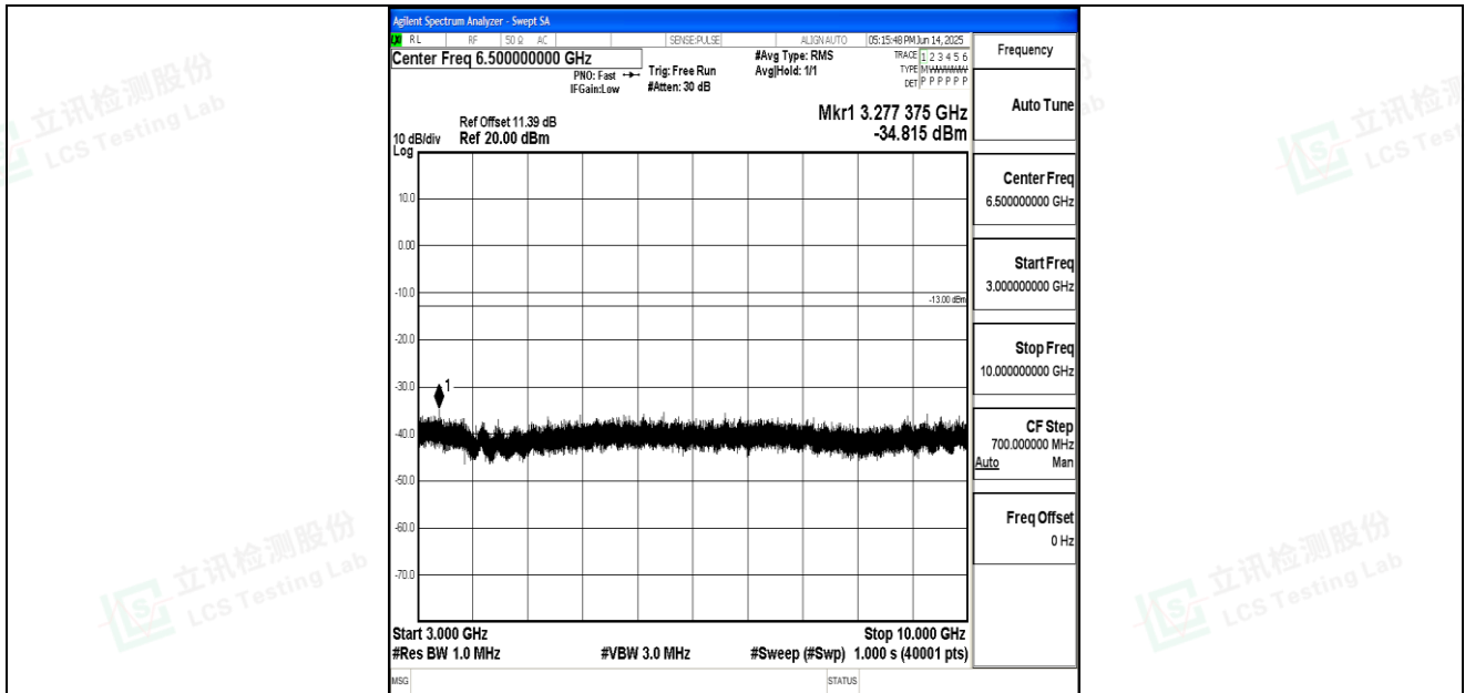
Band26_10MHz_QPSK_26990_1RB#0_3000~10000_3000~10000
