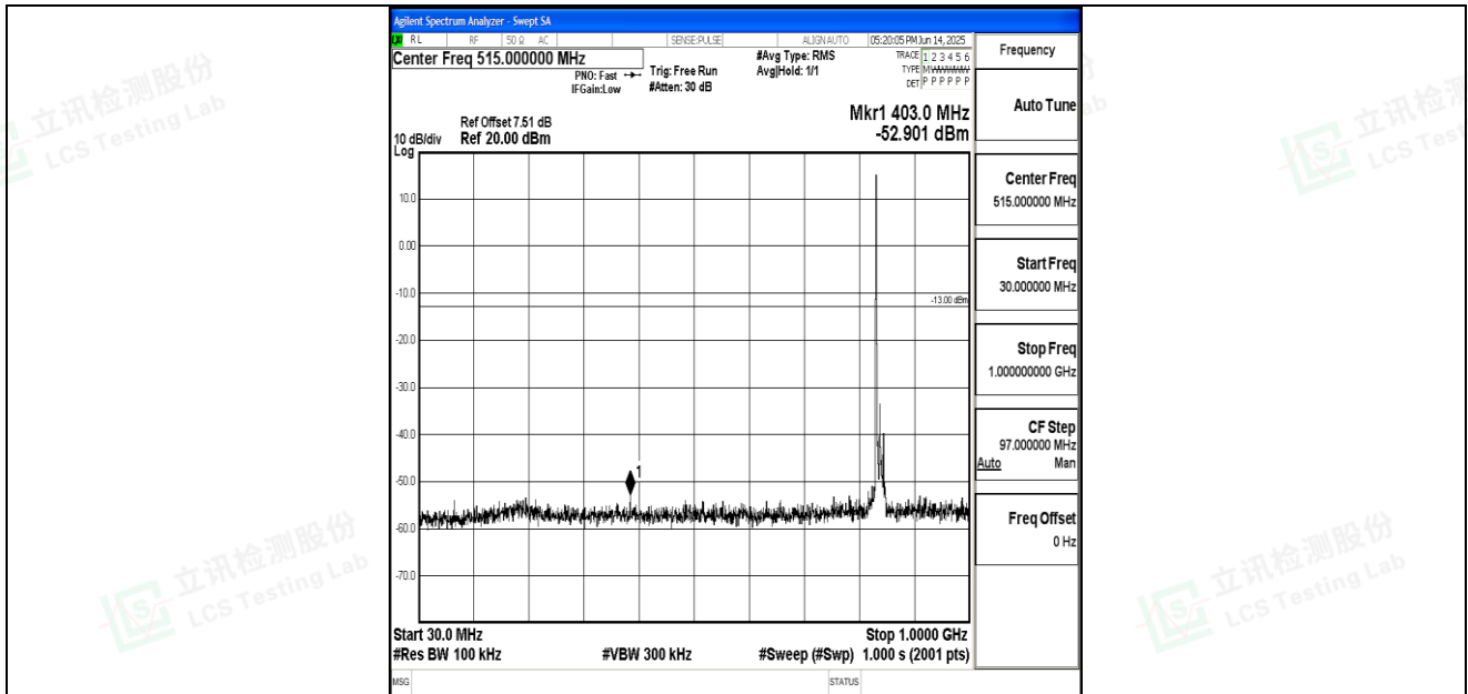
Band26_15MHz_QPSK_26965_1RB#0_30~1000_30~1000
