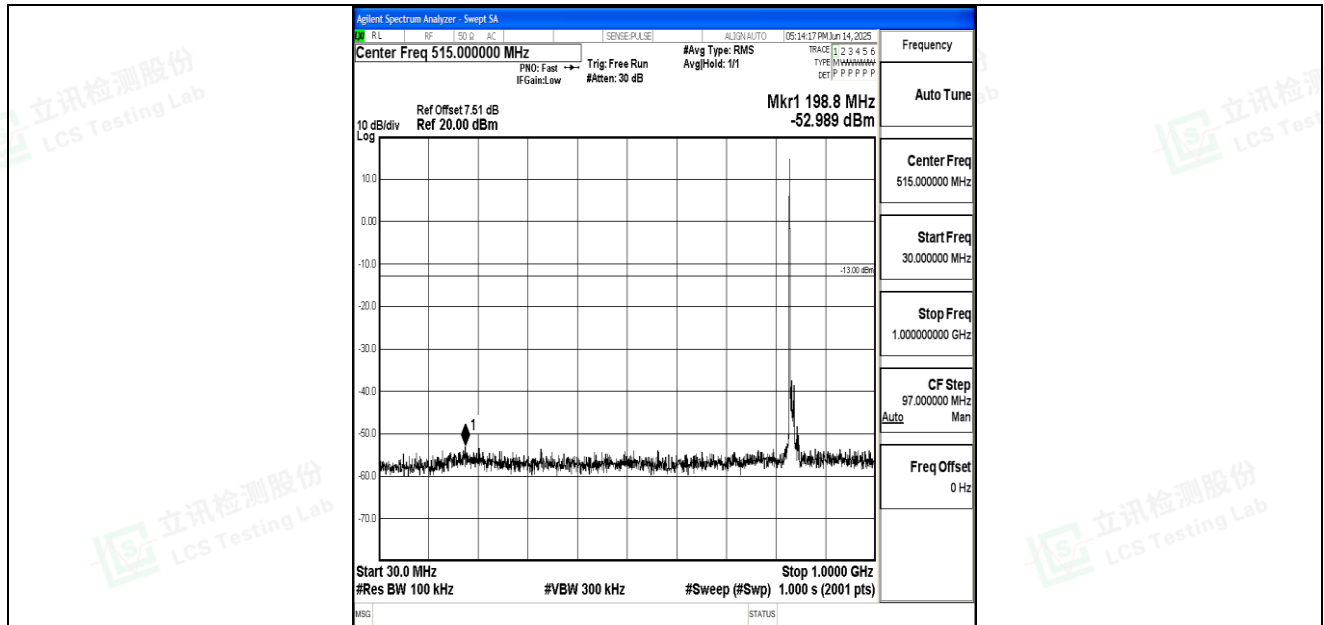
Band26_10MHz_QPSK_26915_1RB#0_30~1000_30~1000
