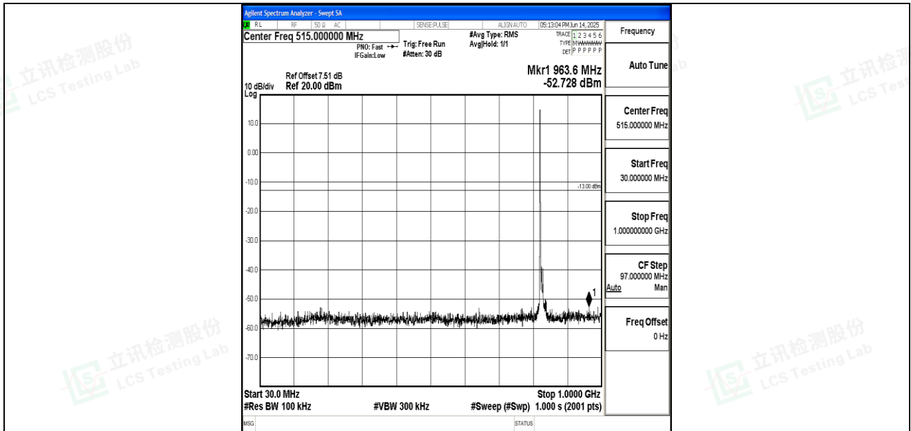
Band26_10MHz_QPSK_26840_1RB#0_30~1000_30~1000
