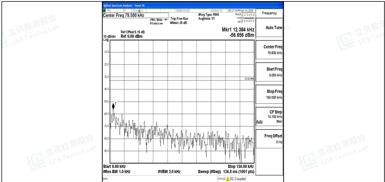
Band26_15MHz_QPSK_26865_1RB#0_0.009~0.15_0.009~0.15
