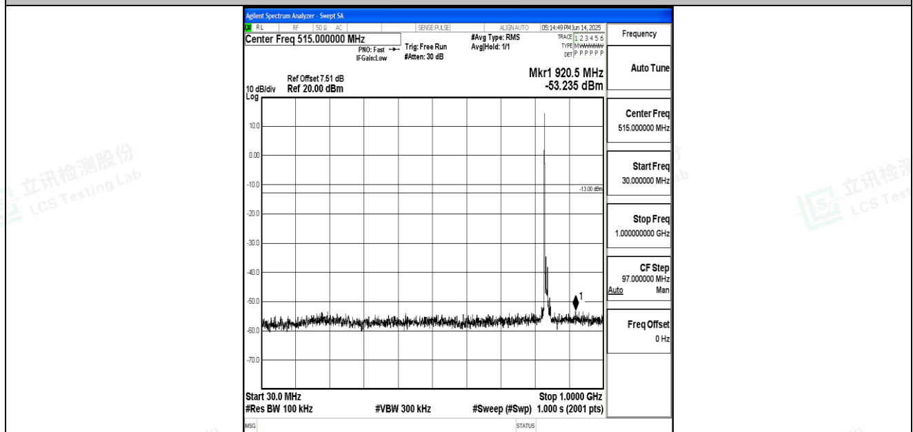
Band26_10MHz_16QAM_26915_1RB#0_30~1000_30~1000
