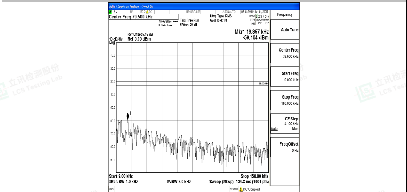
Band26_5MHz_16QAM_27015_1RB#0_0.009~0.15_0.009~0.15
