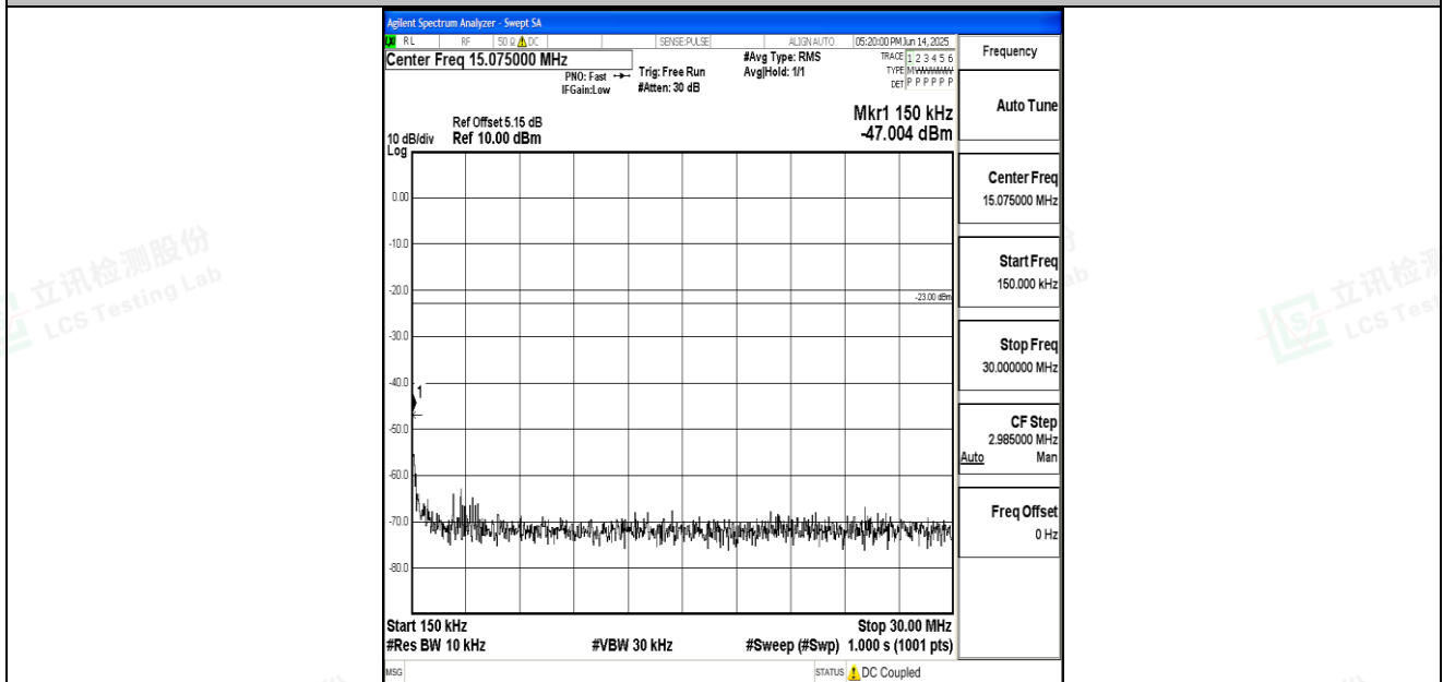
Band26_15MHz_QPSK_26965_1RB#0_0.15~30_0.15~30
