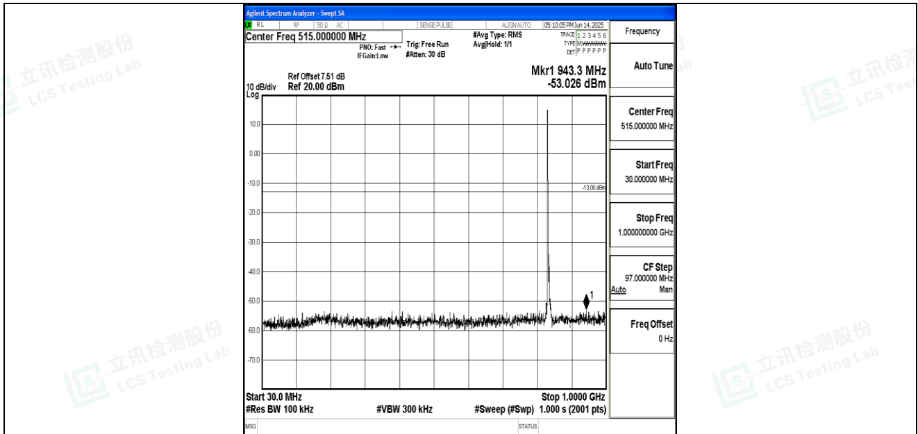
Band26_5MHz_QPSK_26915_1RB#0_30~1000_30~1000
