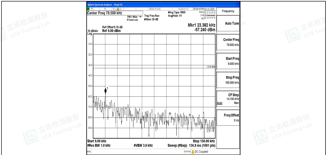
Band26_5MHz_QPSK_26815_1RB#0_0.009~0.15_0.009~0.15
