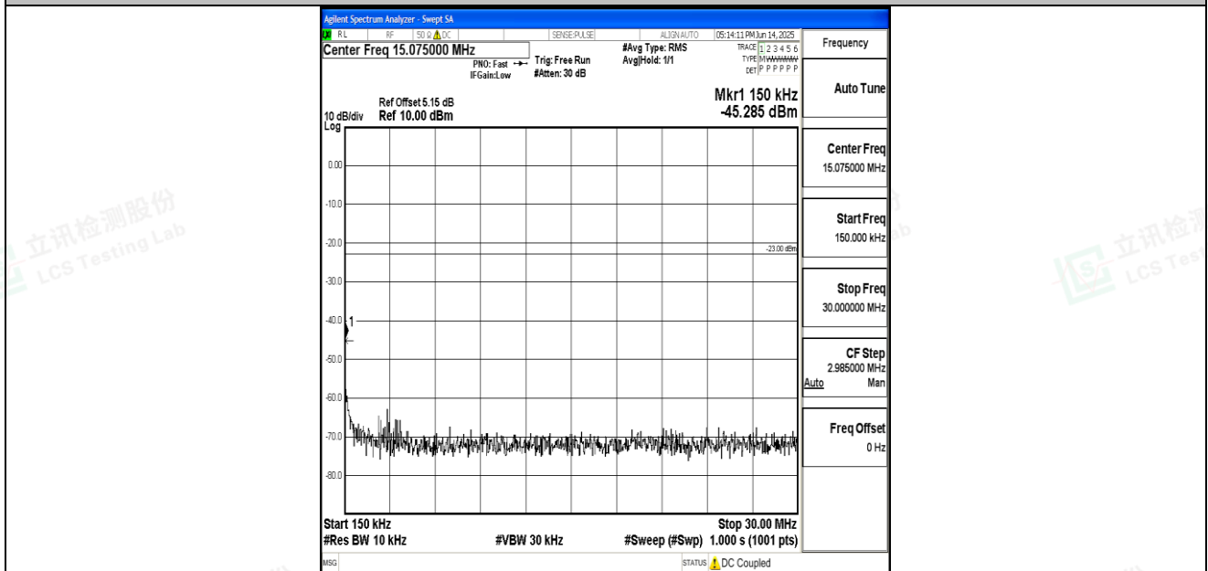
Band26_10MHz_QPSK_26915_1RB#0_0.15~30_0.15~30
