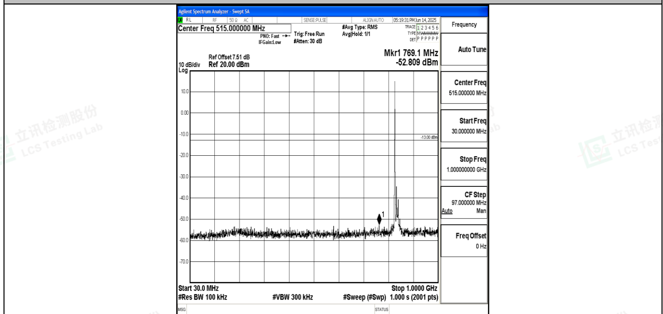
Band26_15MHz_16QAM_26915_1RB#0_30~1000_30~1000
