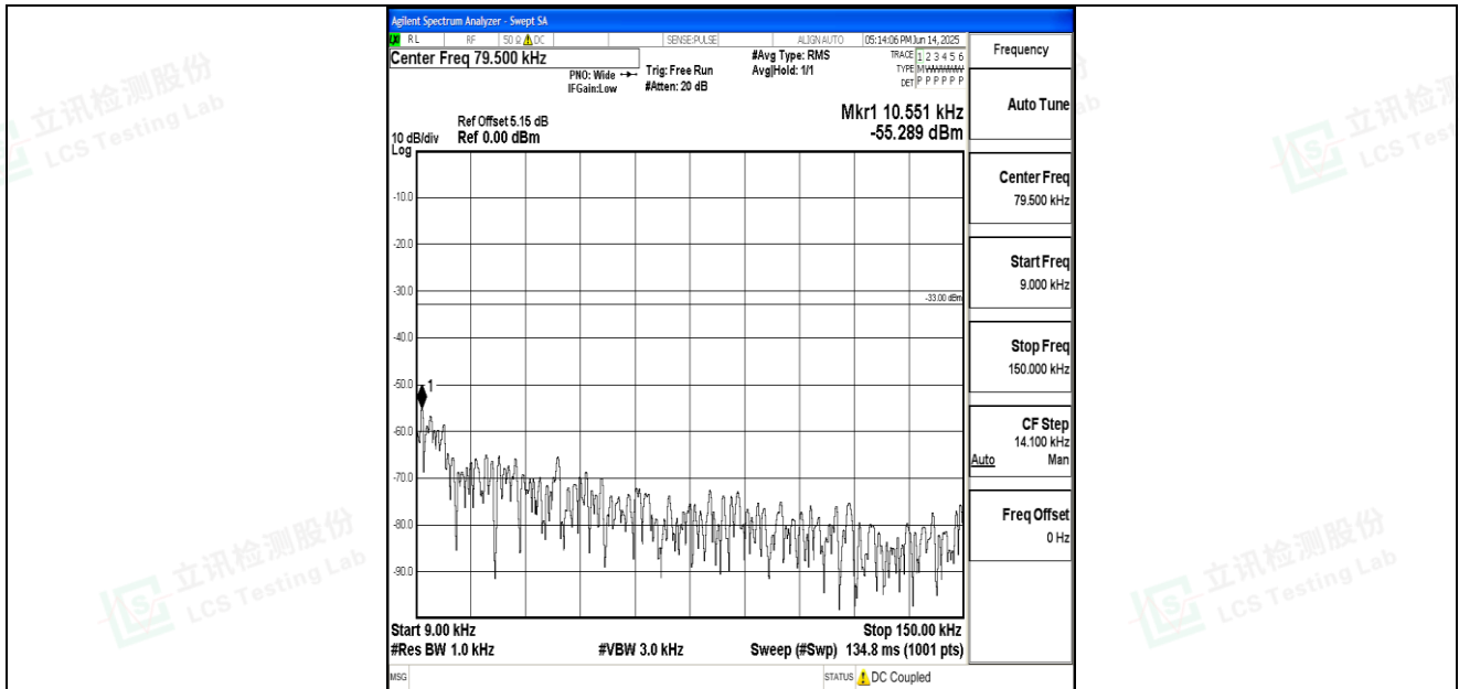
Band26_10MHz_QPSK_26915_1RB#0_0.009~0.15_0.009~0.15
