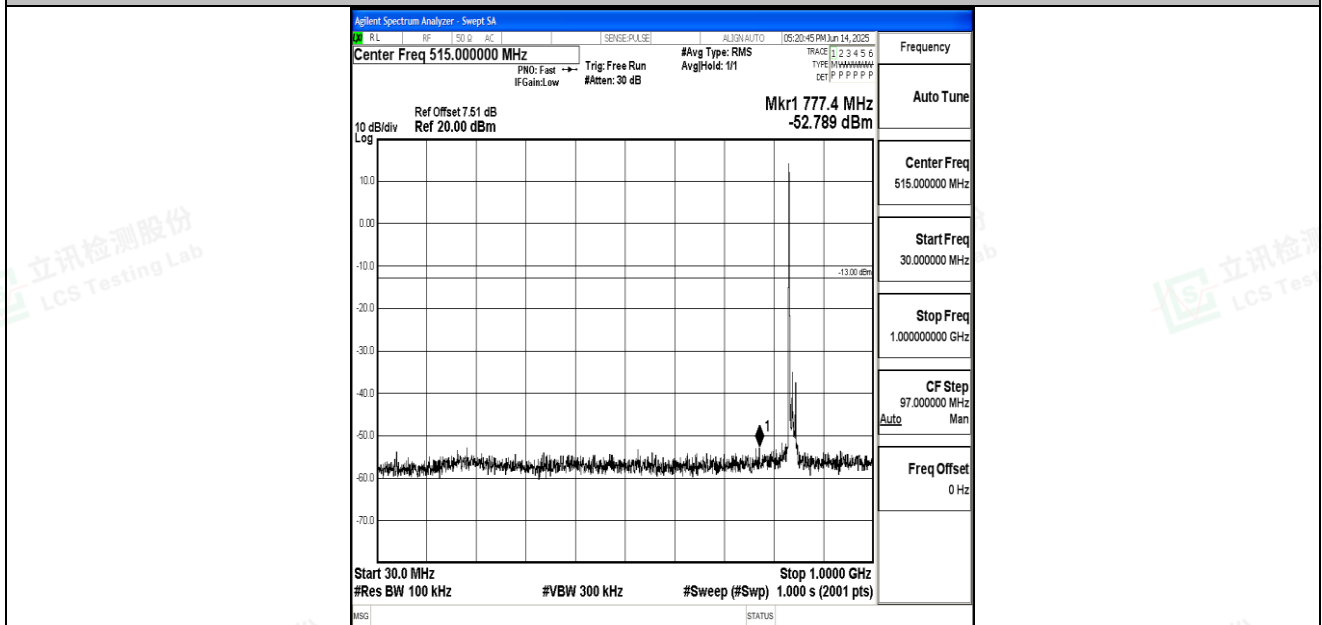
Band26_15MHz_16QAM_26965_1RB#0_30~1000_30~1000
