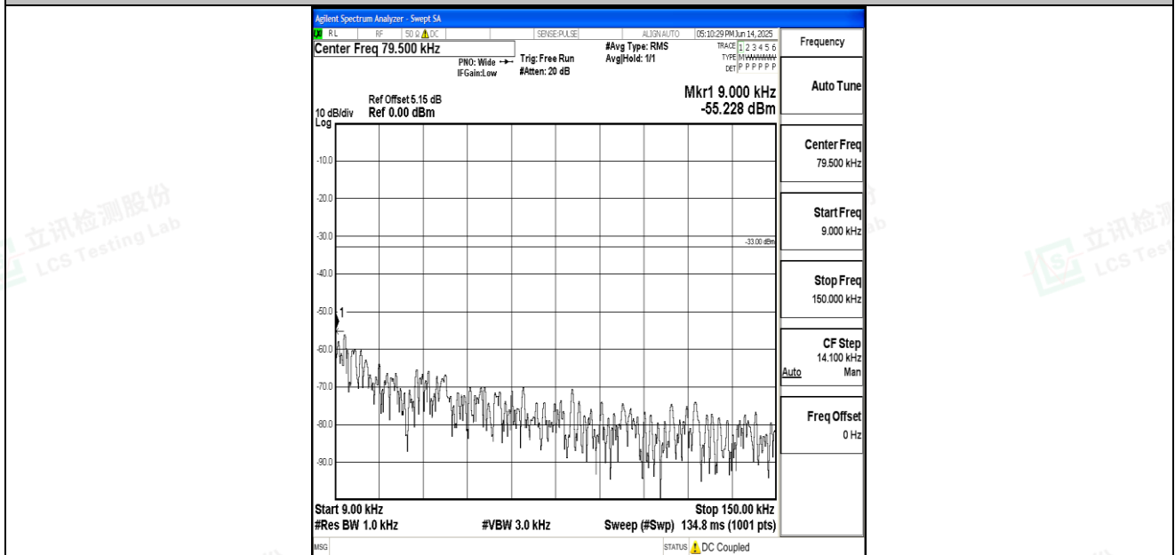
Band26_5MHz_16QAM_26915_1RB#0_0.009~0.15_0.009~0.15
