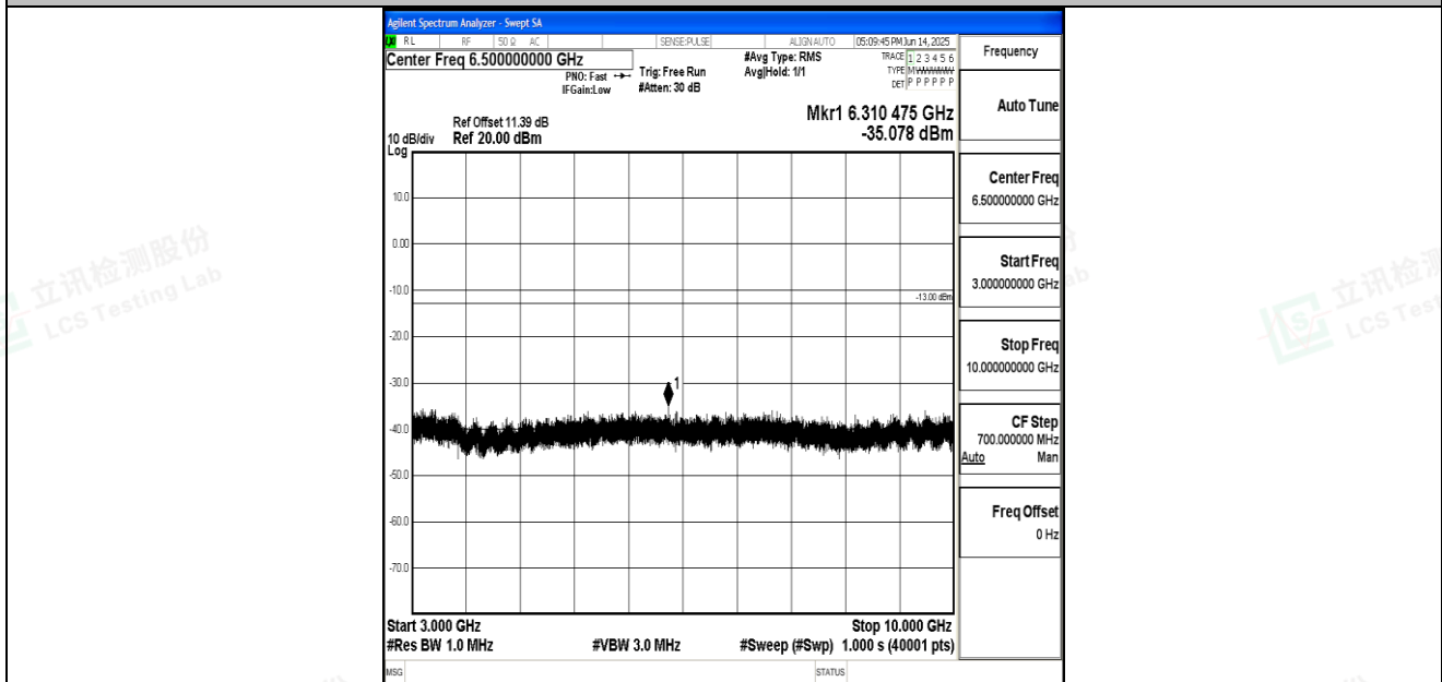
Band26_5MHz_16QAM_26815_1RB#0_3000~10000_3000~10000
