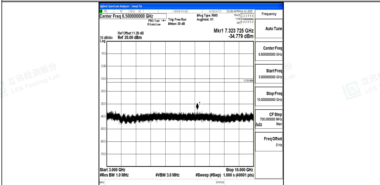
Band26_3MHz_16QAM_26740_1RB#0_3000~10000_3000~10000
