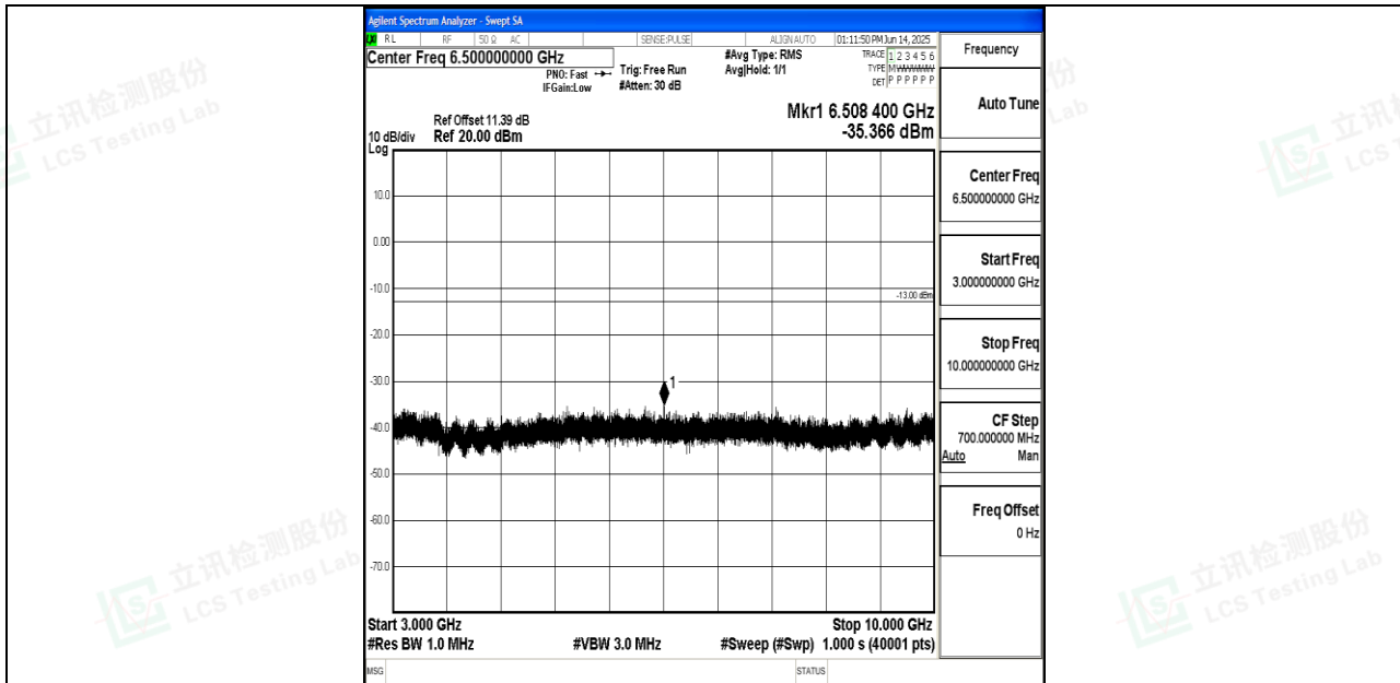
Band26_5MHz_QPSK_26765_1RB#0_3000~10000_3000~10000
