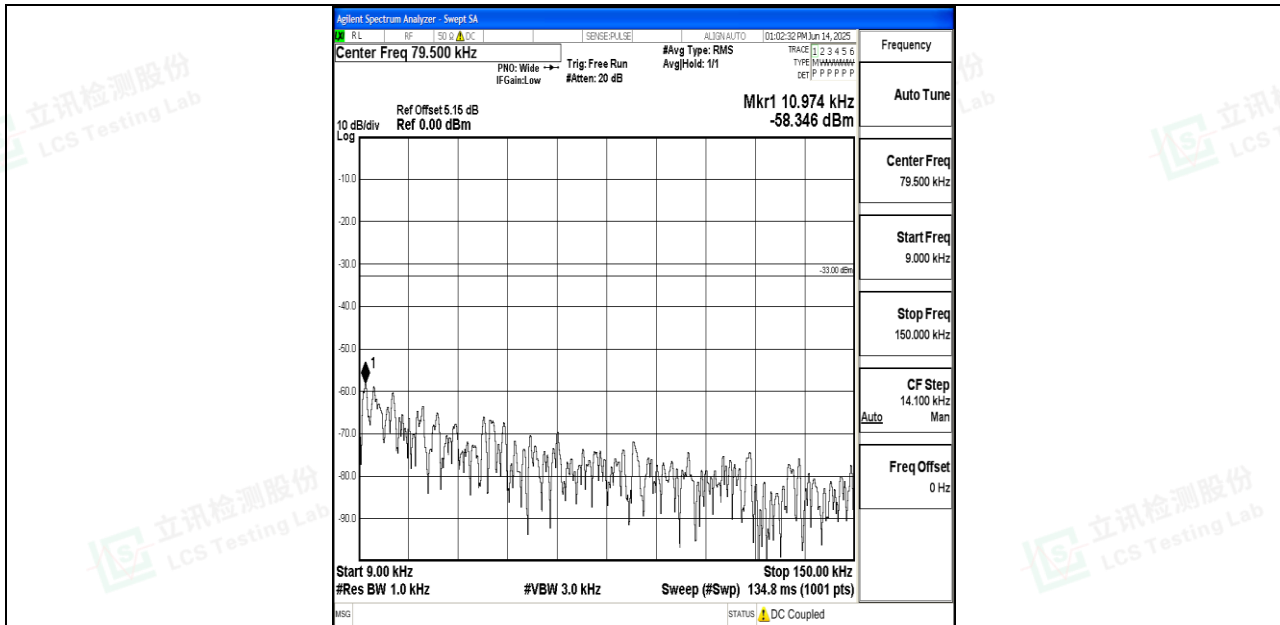
Band26_1.4MHz_QPSK_26783_1RB#0_0.009~0.15_0.009~0.15
