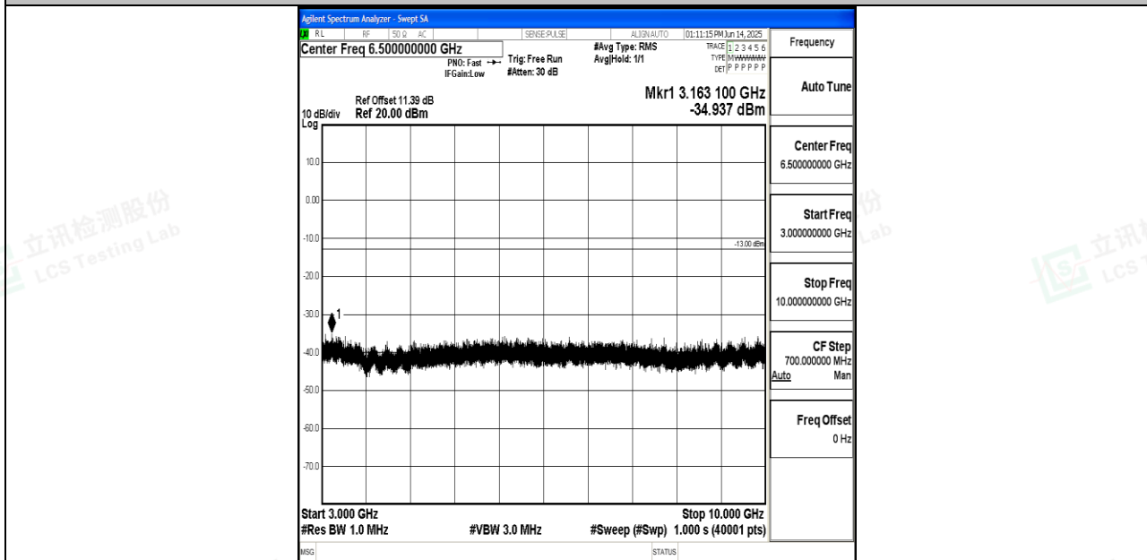
Band26_5MHz_16QAM_26740_1RB#0_3000~10000_3000~10000
