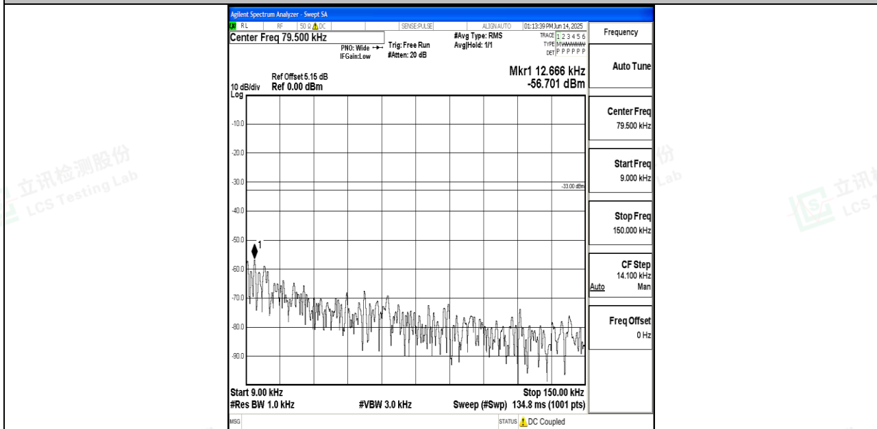
Band26_10MHz_16QAM_26740_1RB#0_0.009~0.15_0.009~0.15
