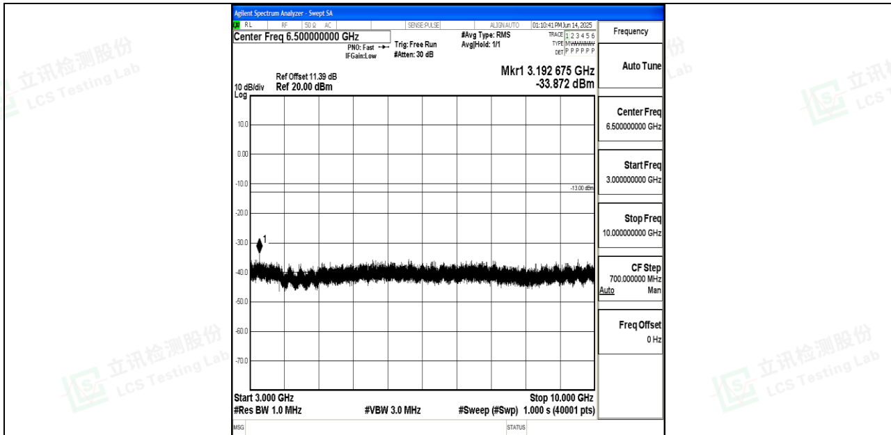
Band26_5MHz_QPSK_26740_1RB#0_3000~10000_3000~10000
