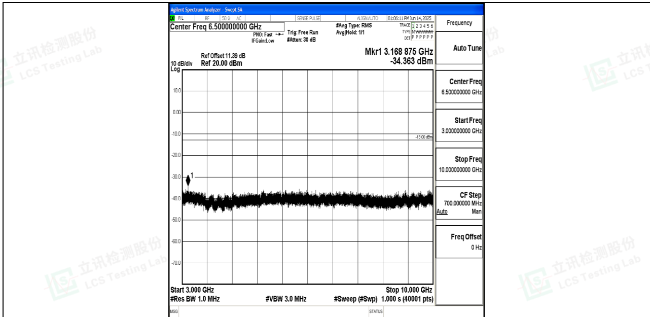
Band26_3MHz_QPSK_26740_1RB#0_3000~10000_3000~10000
