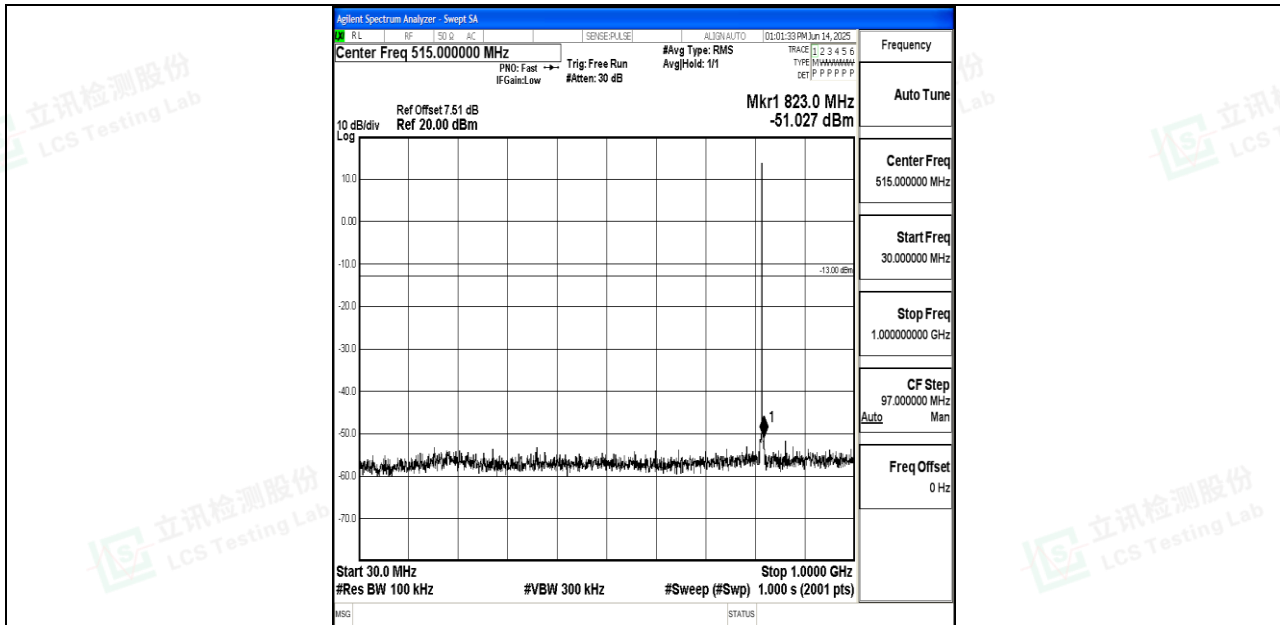
Band26_1.4MHz_QPSK_26740_1RB#0_30~1000_30~1000
