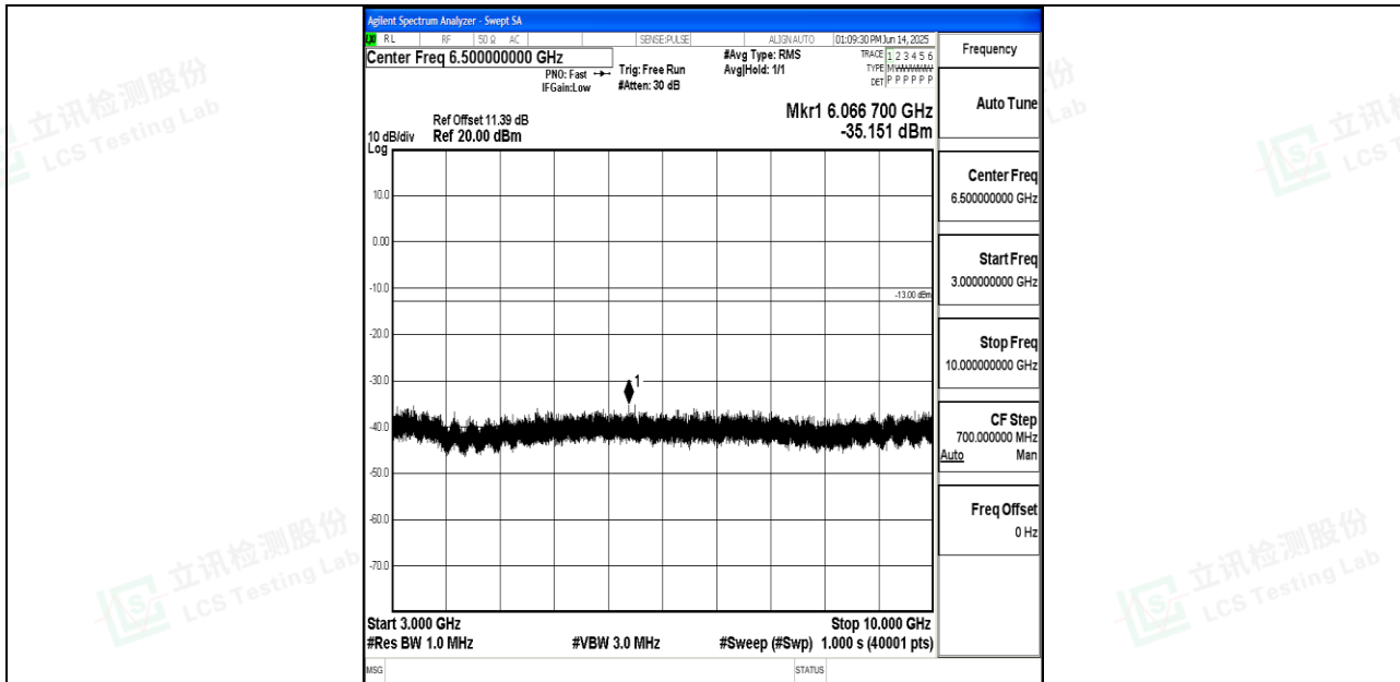
Band26_5MHz_QPSK_26715_1RB#0_3000~10000_3000~10000
