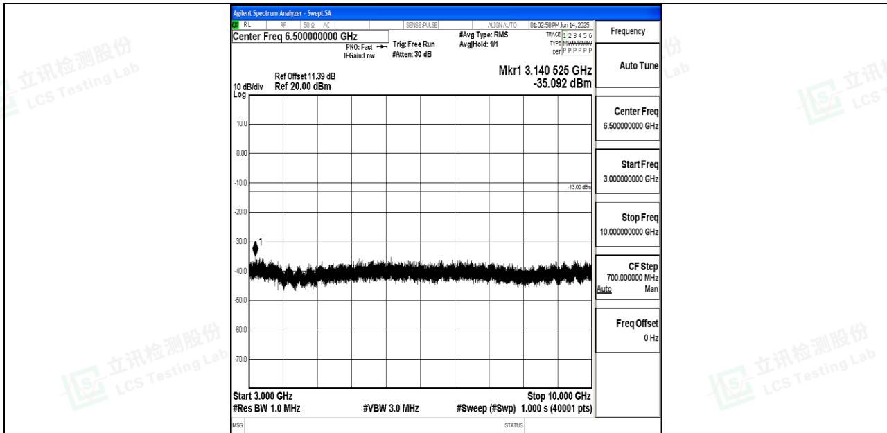
Band26_1.4MHz_QPSK_26783_1RB#0_3000~10000_3000~10000
