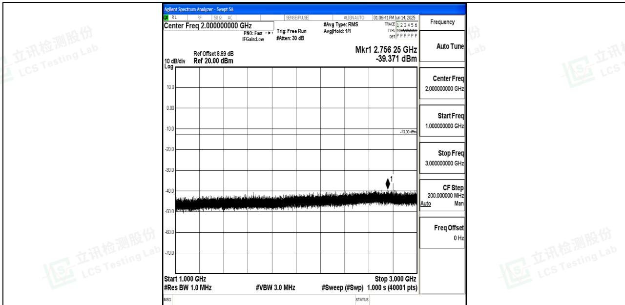
Band26_3MHz_16QAM_26740_1RB#0_1000~3000_1000~3000
