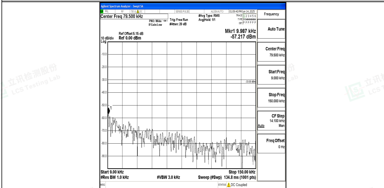
Band26_5MHz_16QAM_26715_1RB#0_0.009~0.15_0.009~0.15
