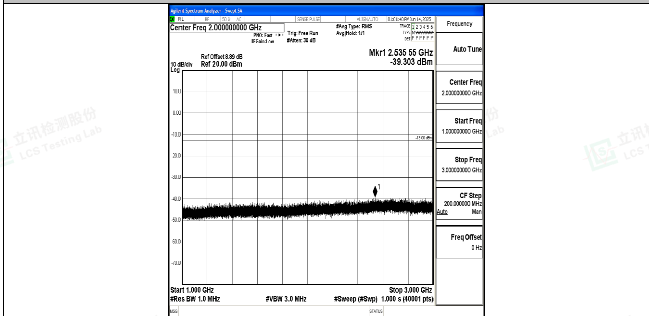
Band26_1.4MHz_QPSK_26740_1RB#0_1000~3000_1000~3000
