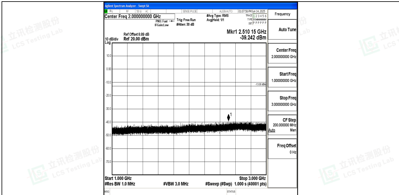
Band26_3MHz_16QAM_26775_1RB#0_1000~3000_1000~3000
