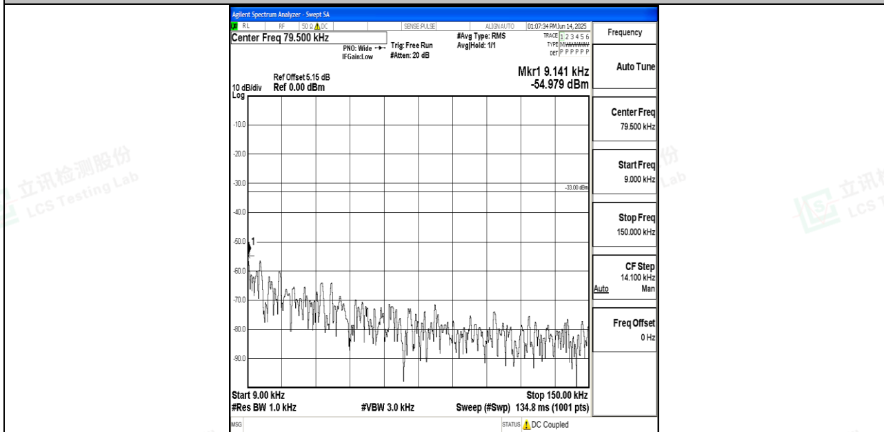
Band26_3MHz_16QAM_26775_1RB#0_0.009~0.15_0.009~0.15
