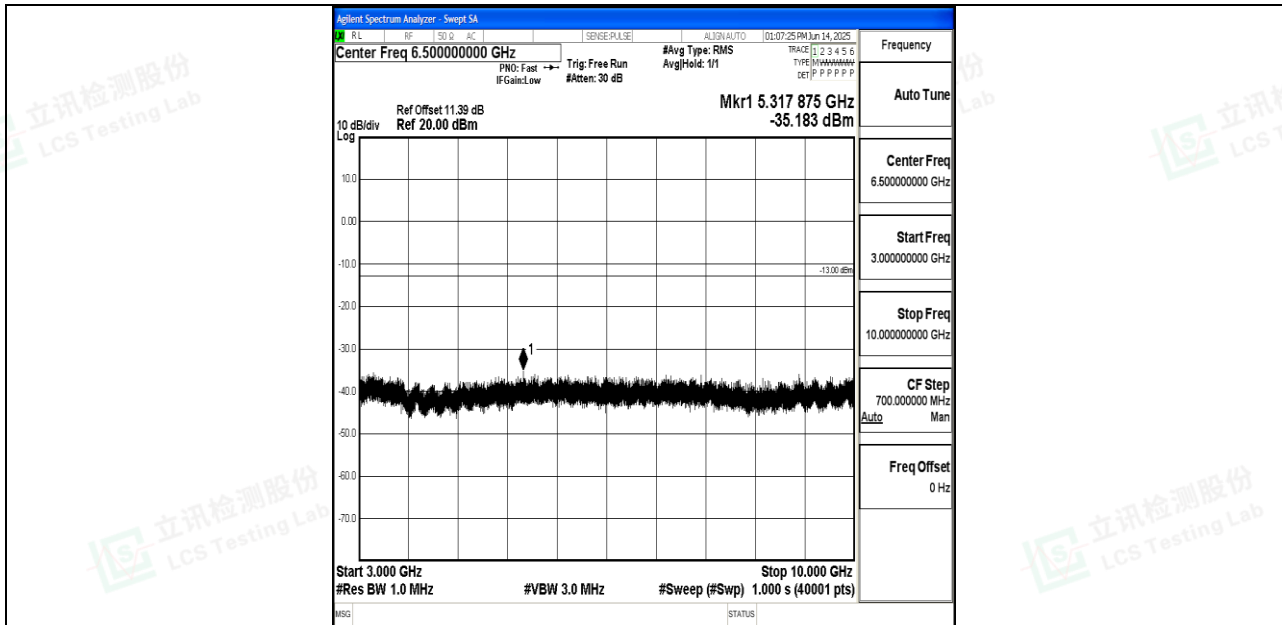
Band26_3MHz_QPSK_26775_1RB#0_3000~10000_3000~10000
