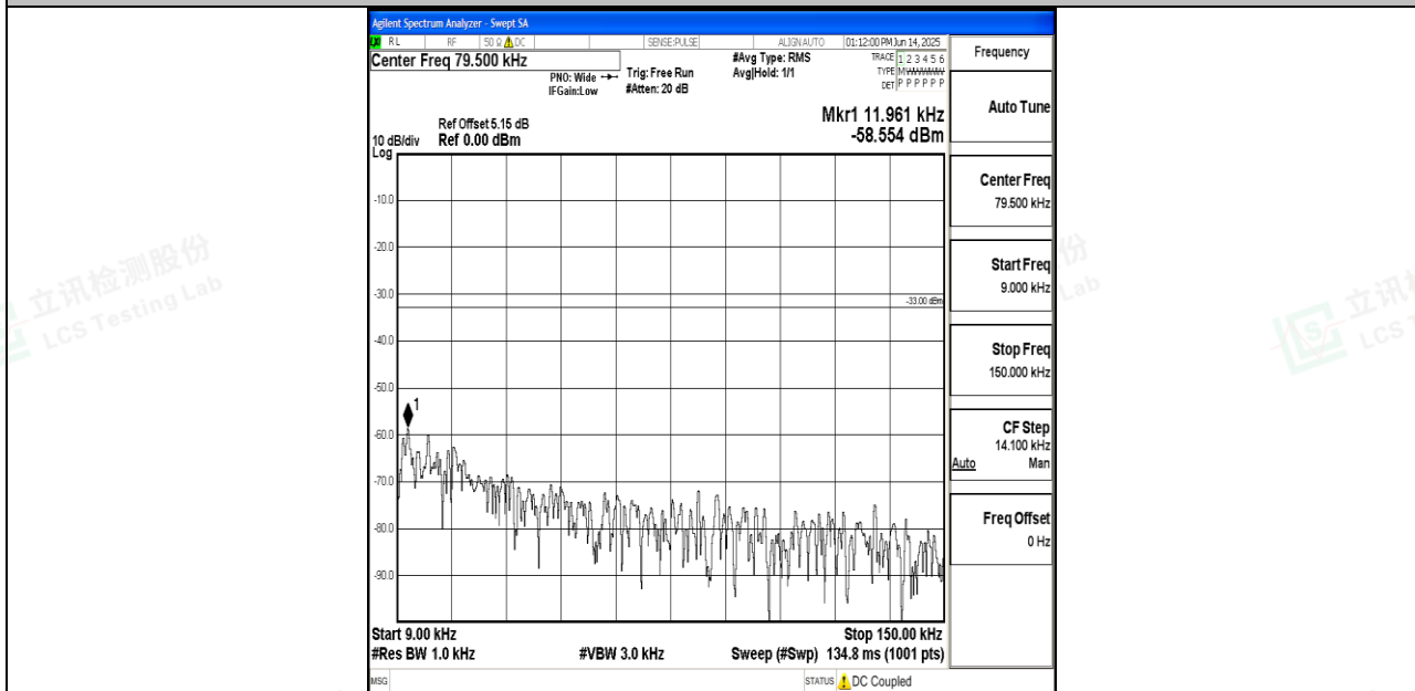
Band26_5MHz_16QAM_26765_1RB#0_0.009~0.15_0.009~0.15
