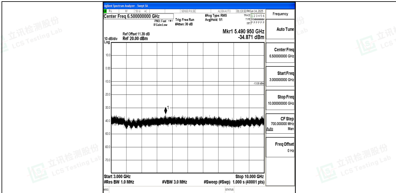
Band26_10MHz_QPSK_26740_1RB#0_3000~10000_3000~10000
