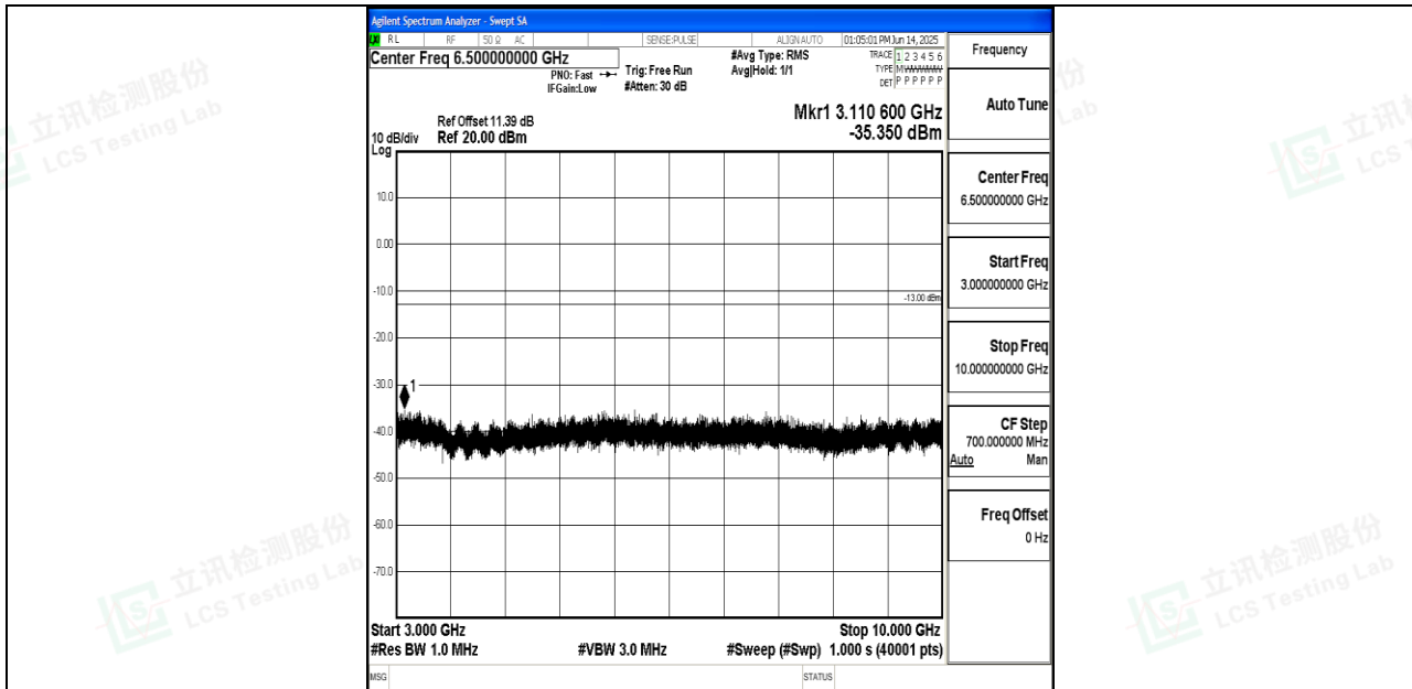
Band26_3MHz_QPSK_26705_1RB#0_3000~10000_3000~10000
