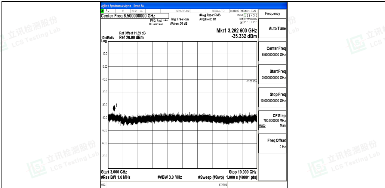
Band26_1.4MHz_QPSK_26740_1RB#0_3000~10000_3000~10000
