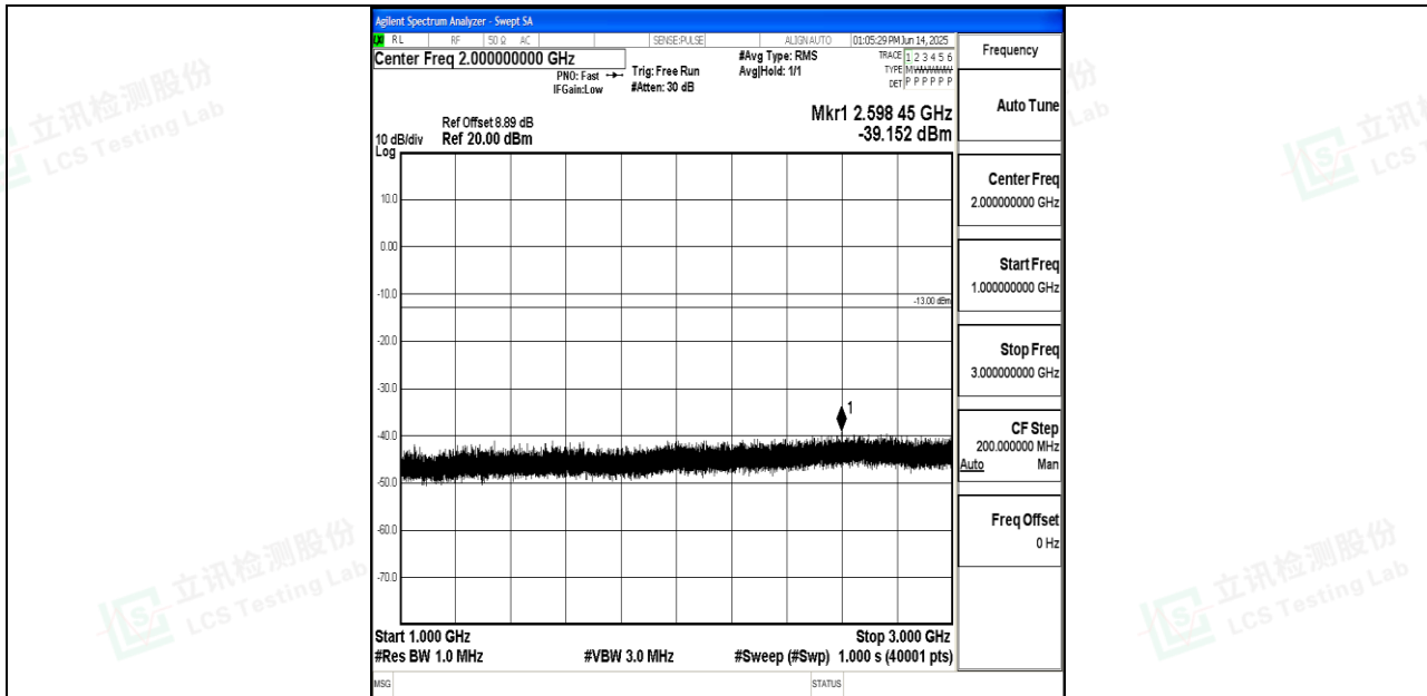
Band26_3MHz_16QAM_26705_1RB#0_1000~3000_1000~3000
