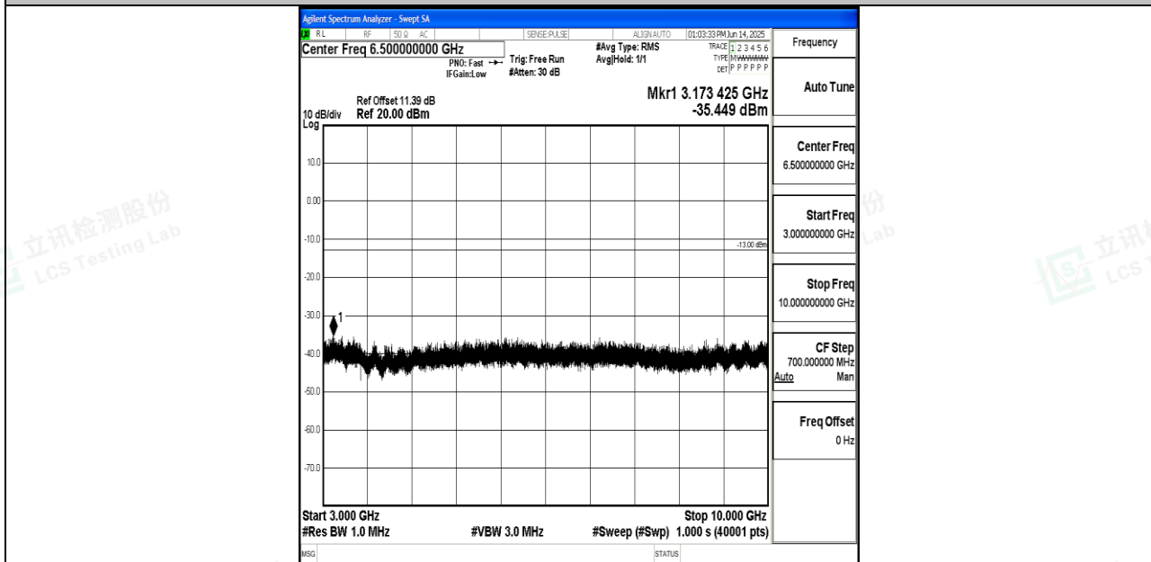
Band26_1.4MHz_16QAM_26783_1RB#0_3000~10000_3000~10000
