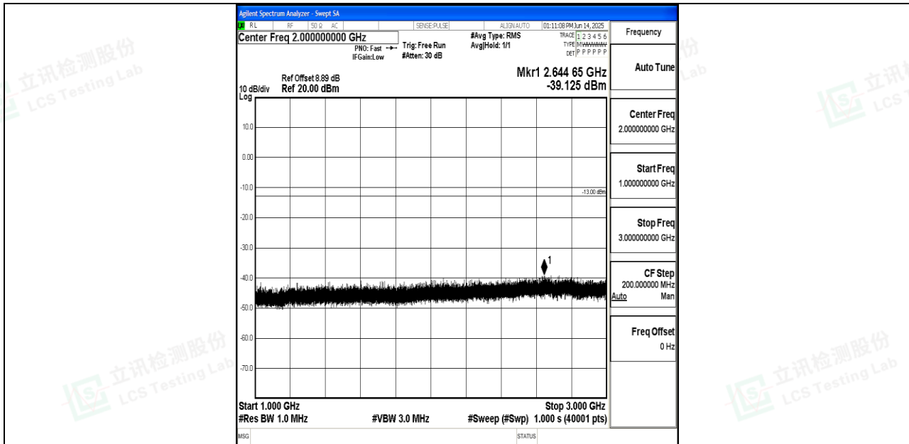
Band26_5MHz_16QAM_26740_1RB#0_1000~3000_1000~3000
