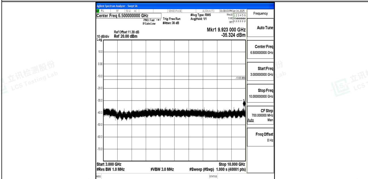
Band26_3MHz_16QAM_26775_1RB#0_3000~10000_3000~10000
