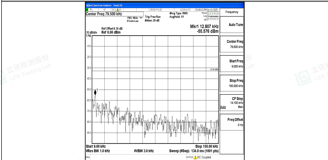
Band26_3MHz_16QAM_26740_1RB#0_0.009~0.15_0.009~0.15
