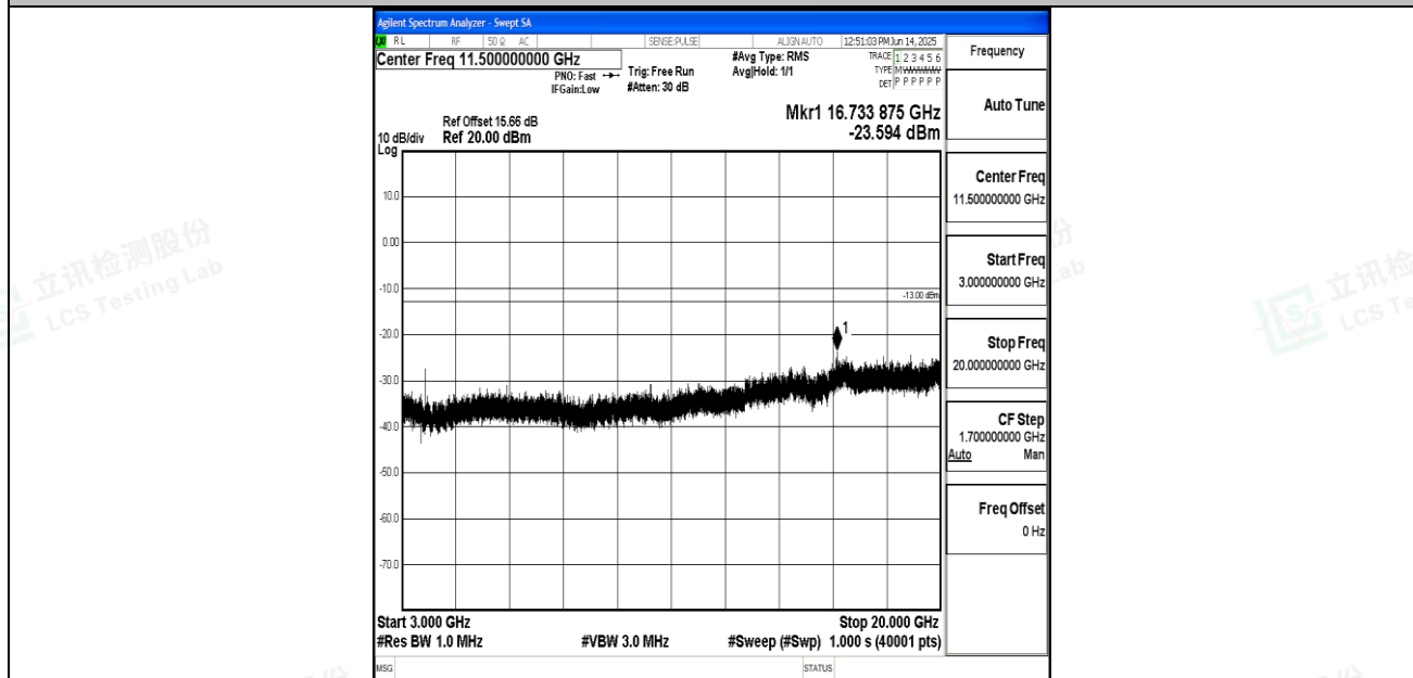
Band25_15MHz_QPSK_26365_1RB#0_3000~20000_3000~20000
