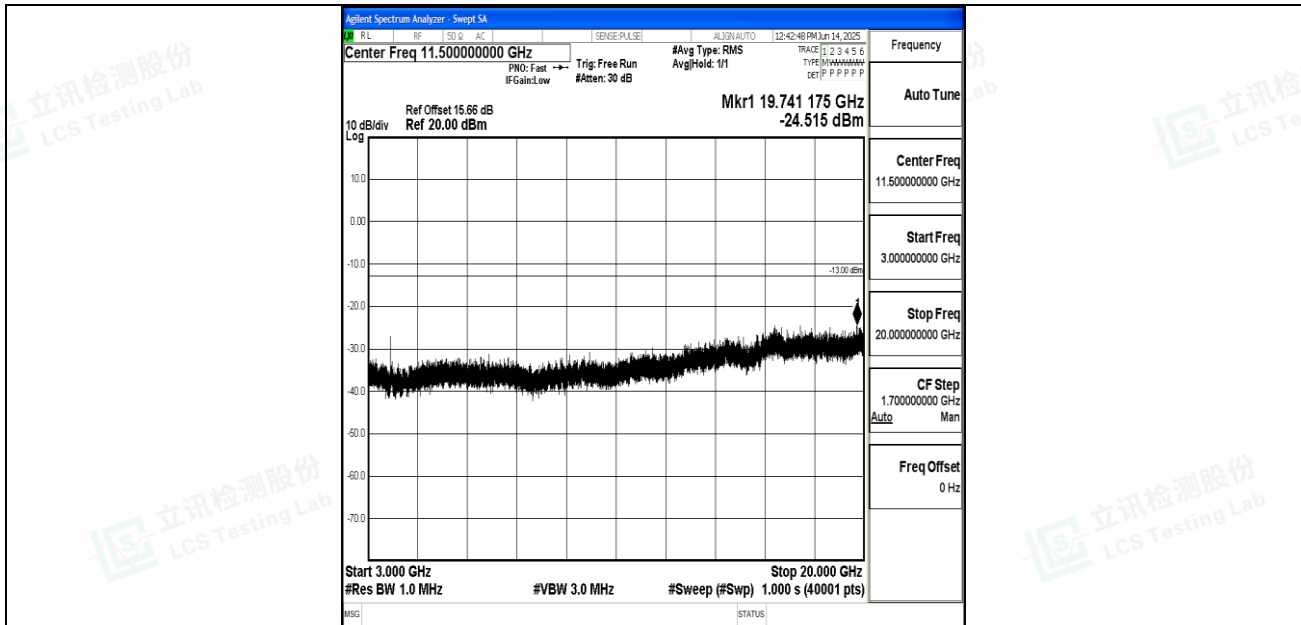
Band25_5MHz_16QAM_26365_1RB#0_3000~20000_3000~20000
