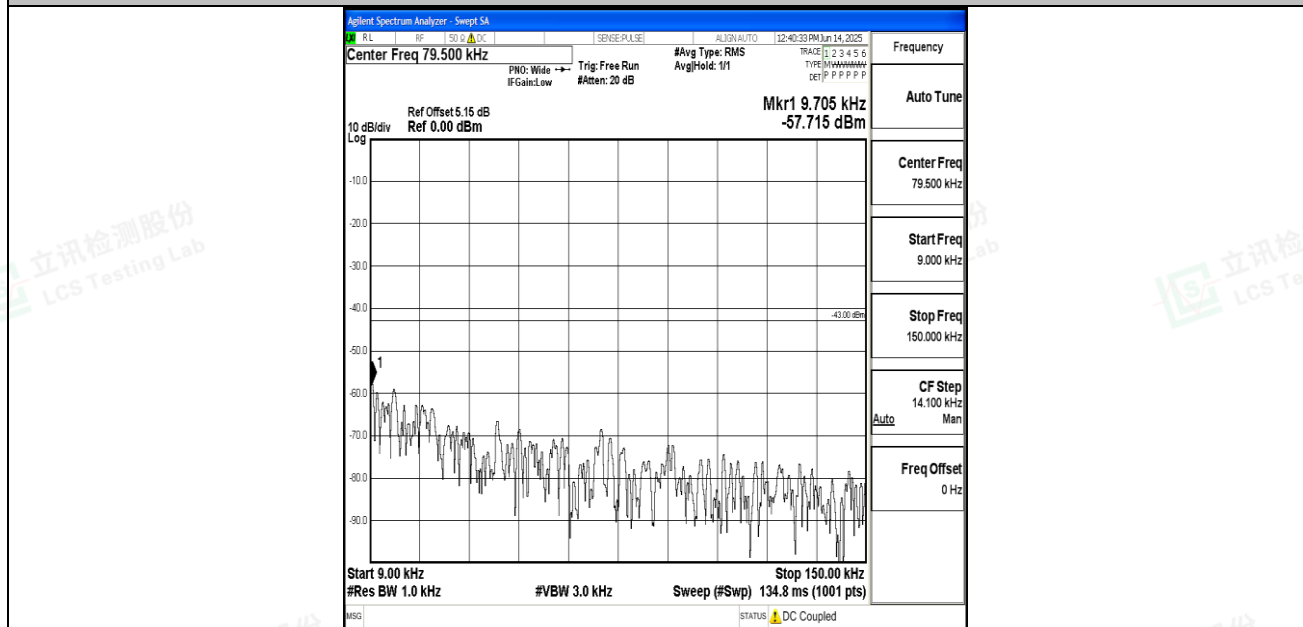
Band25_5MHz_QPSK_26065_1RB#0_0.009~0.15_0.009~0.15
