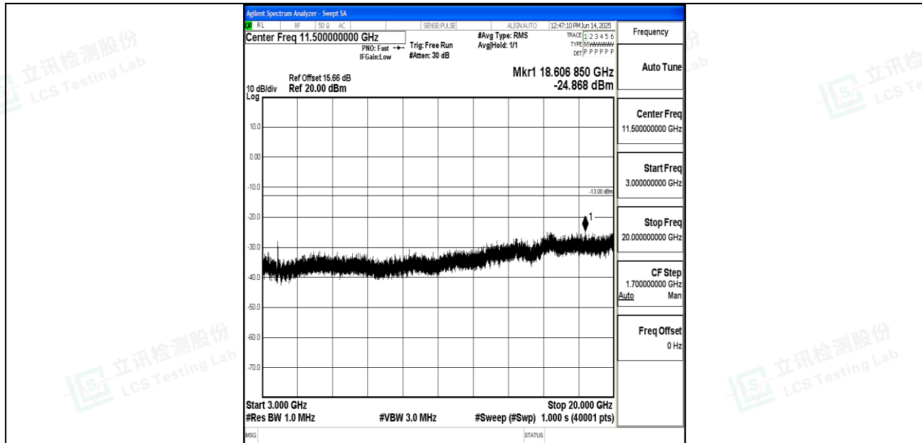
Band25_10MHz_16QAM_26365_1RB#0_3000~20000_3000~20000
