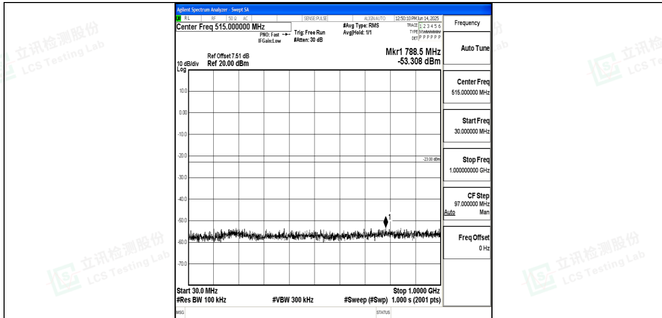
Band25_15MHz_16QAM_26115_1RB#0_30~1000_30~1000
