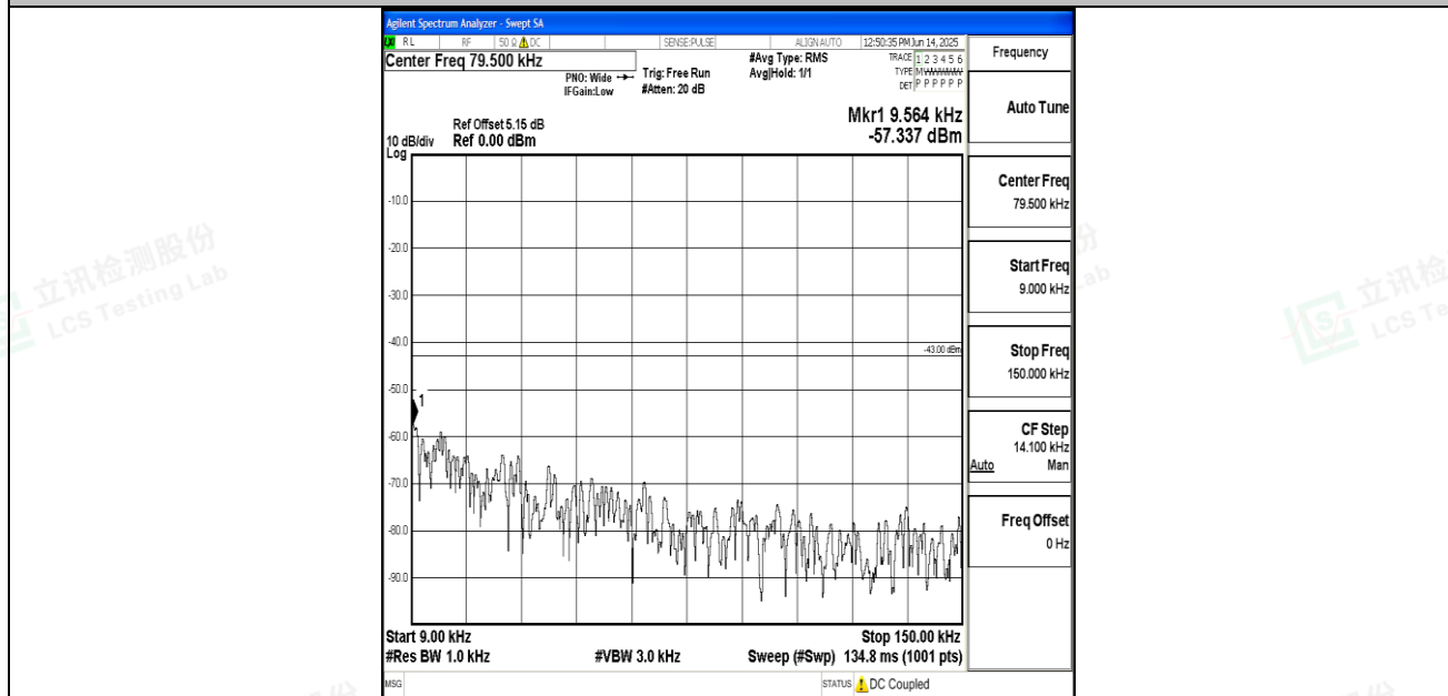
Band25_15MHz_QPSK_26365_1RB#0_0.009~0.15_0.009~0.15
