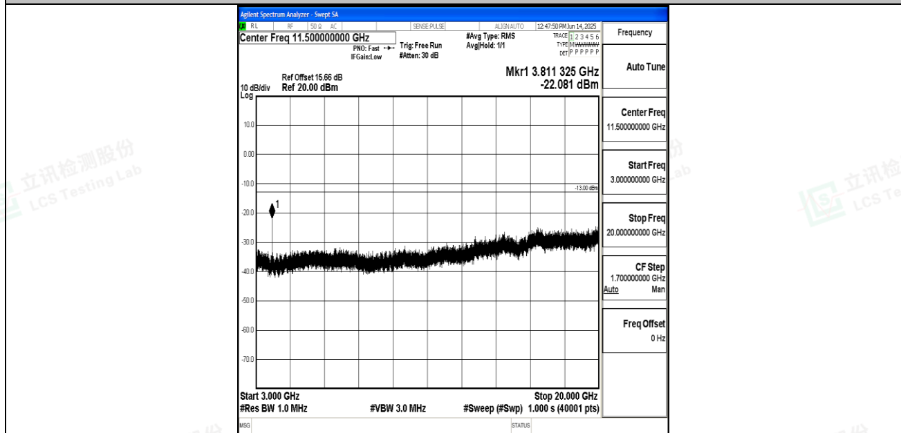
Band25_10MHz_QPSK_26640_1RB#0_3000~20000_3000~20000
