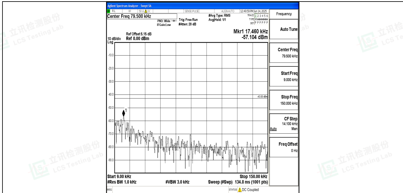
Band25_15MHz_16QAM_26115_1RB#0_0.009~0.15_0.009~0.15
