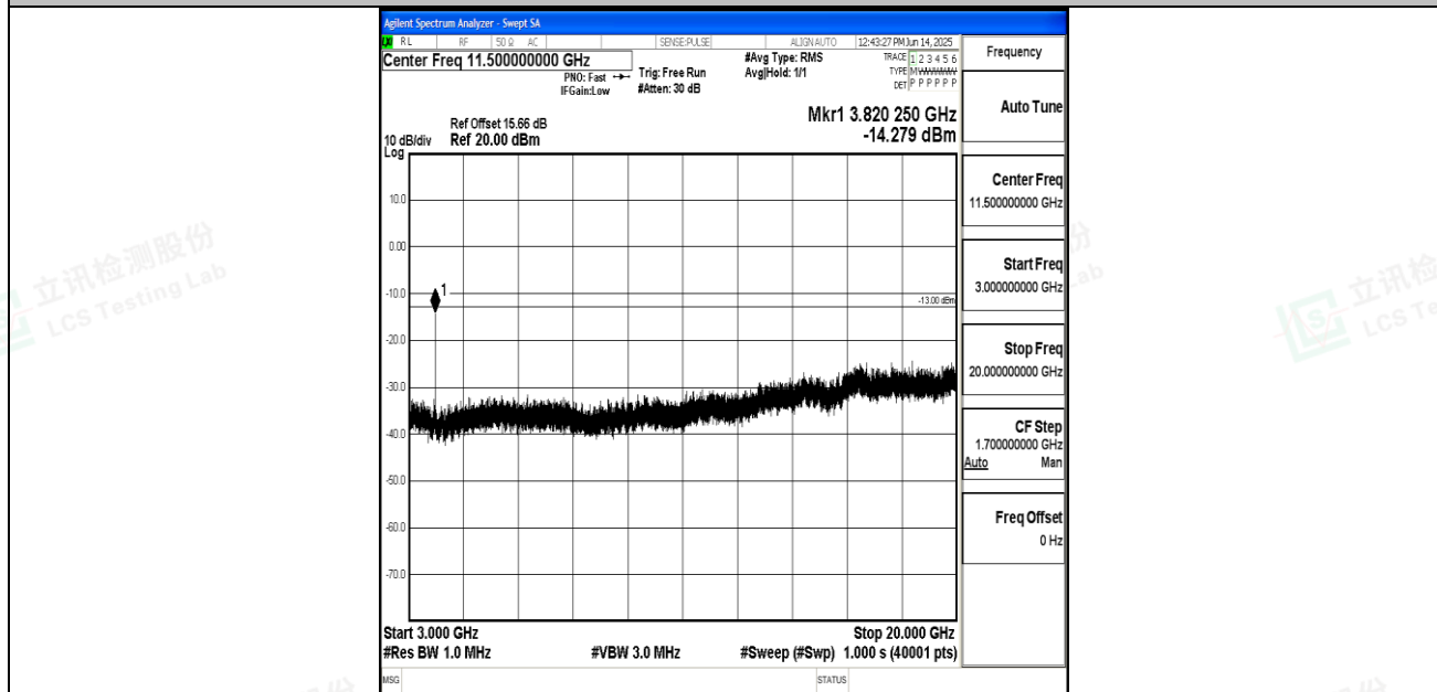
Band25_5MHz_QPSK_26665_1RB#0_3000~20000_3000~20000
