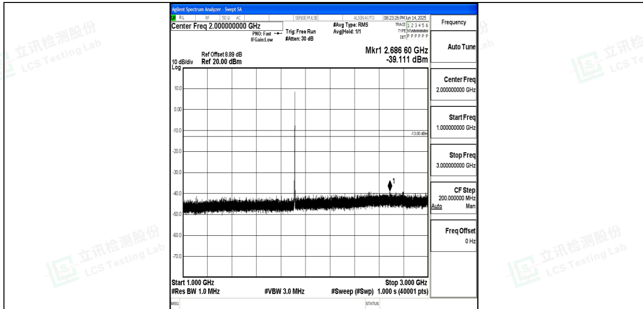
Band25_3MHz_QPSK_26675_1RB#0_1000~3000_1000~3000
