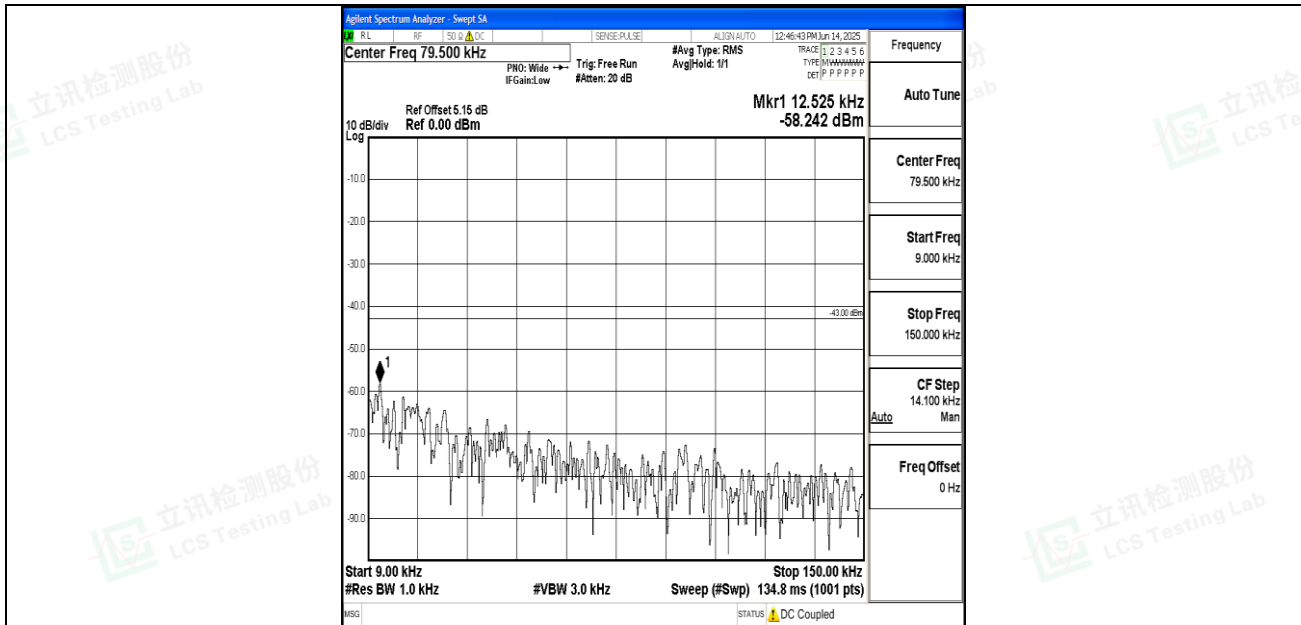
Band25_10MHz_16QAM_26365_1RB#0_0.009~0.15_0.009~0.15
