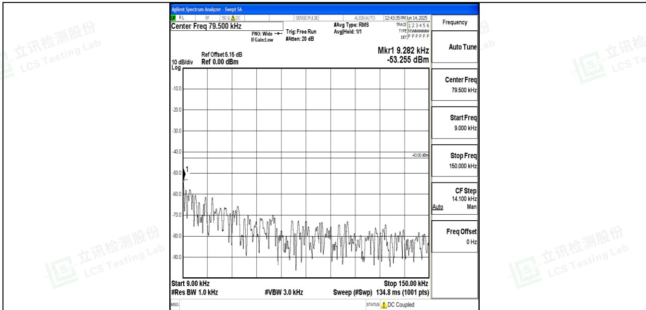
Band25_5MHz_16QAM_26665_1RB#0_0.009~0.15_0.009~0.15
