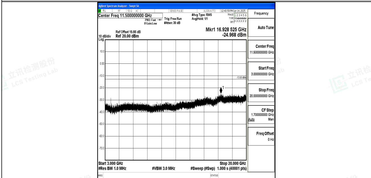
Band25_5MHz_QPSK_26065_1RB#0_3000~20000_3000~20000
