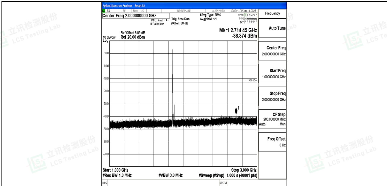
Band25_15MHz_QPSK_26115_1RB#0_1000~3000_1000~3000
