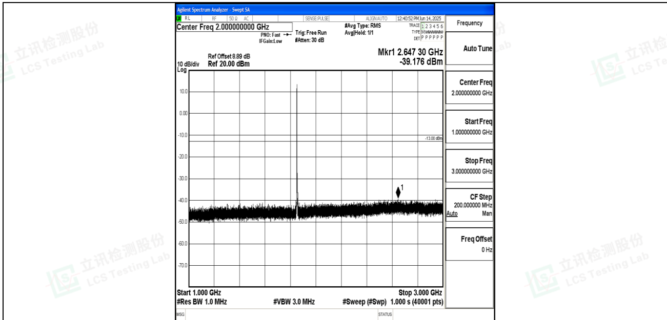
Band25_5MHz_QPSK_26065_1RB#0_1000~3000_1000~3000
