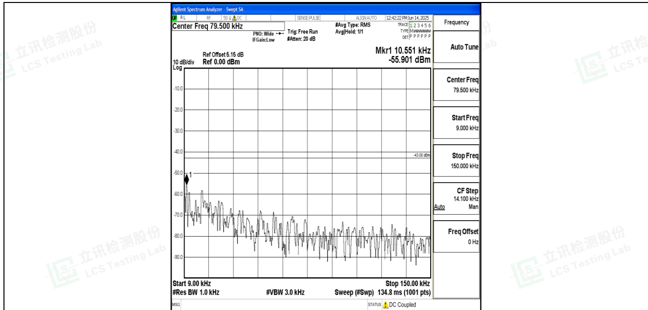
Band25_5MHz_16QAM_26365_1RB#0_0.009~0.15_0.009~0.15
