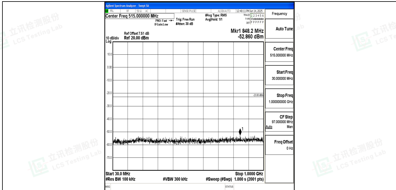
Band25_10MHz_16QAM_26640_1RB#0_30~1000_30~1000
