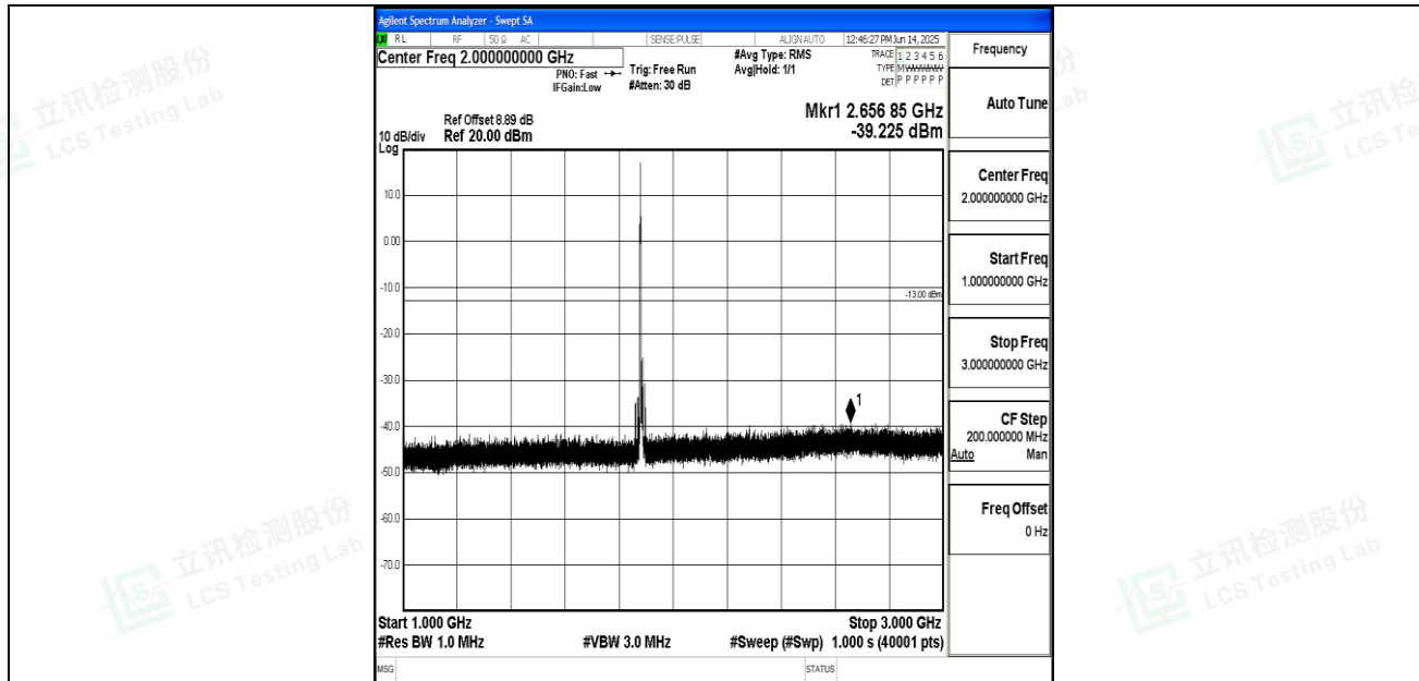
Band25_10MHz_QPSK_26365_1RB#0_1000~3000_1000~3000
