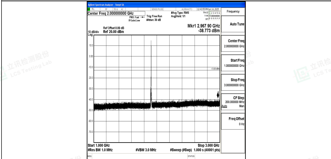
Band25_5MHz_16QAM_26665_1RB#0_1000~3000_1000~3000
