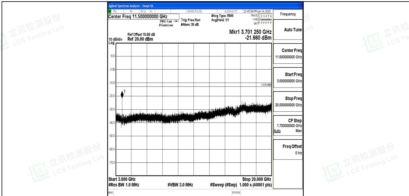
Band25_10MHz_16QAM_26090_1RB#0_3000~20000_3000~20000
