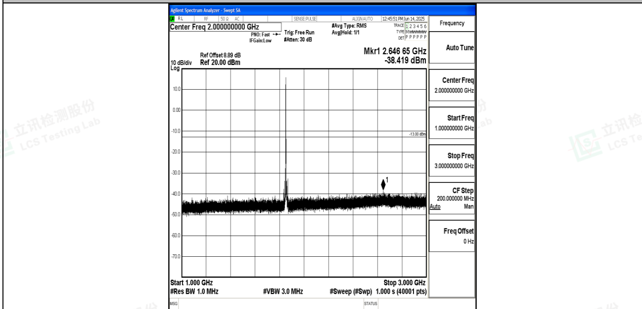
Band25_10MHz_16QAM_26090_1RB#0_1000~3000_1000~3000
