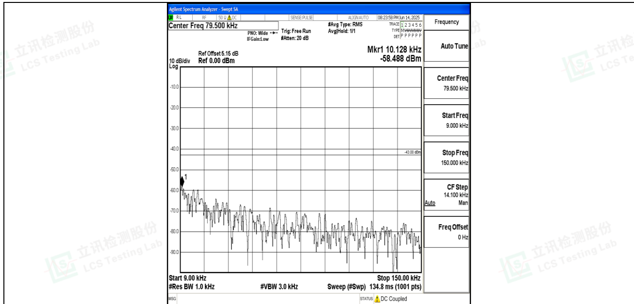
Band25_3MHz_16QAM_26675_1RB#0_0.009~0.15_0.009~0.15
