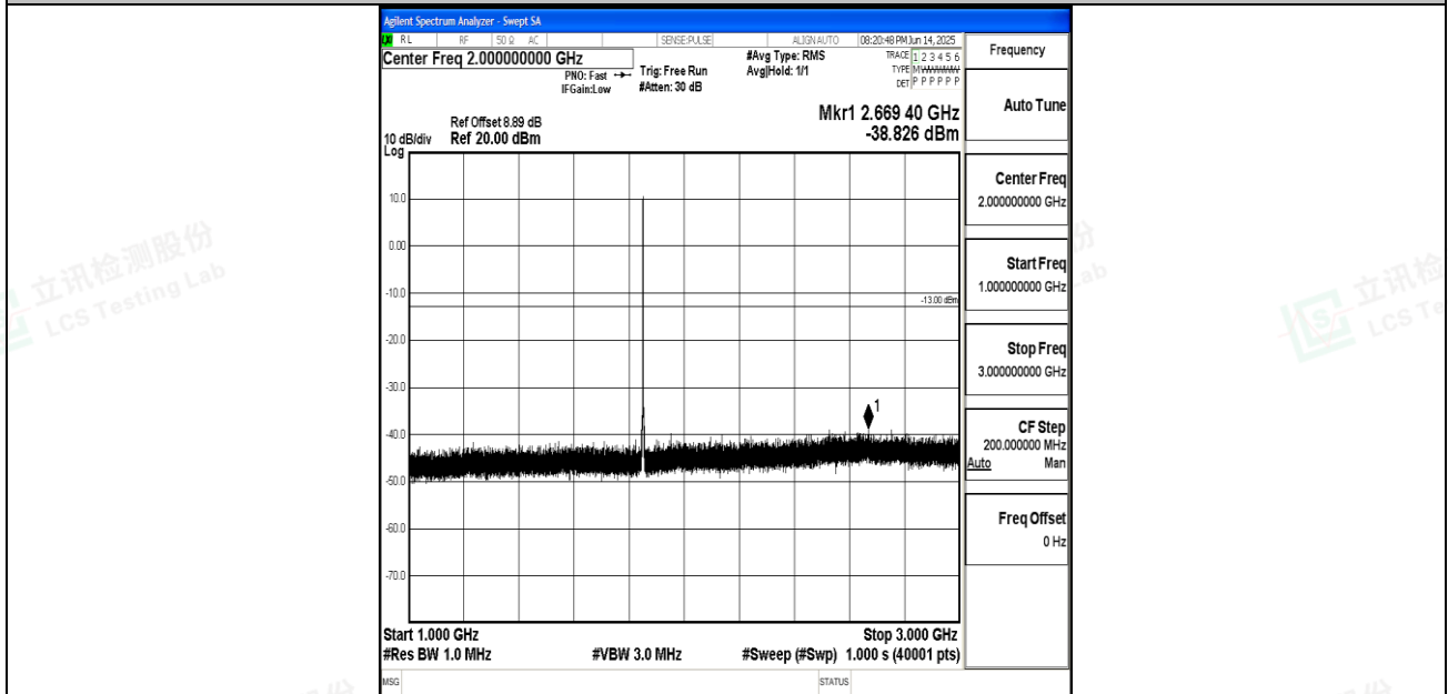
Band25_3MHz_QPSK_26055_1RB#0_1000~3000_1000~3000
