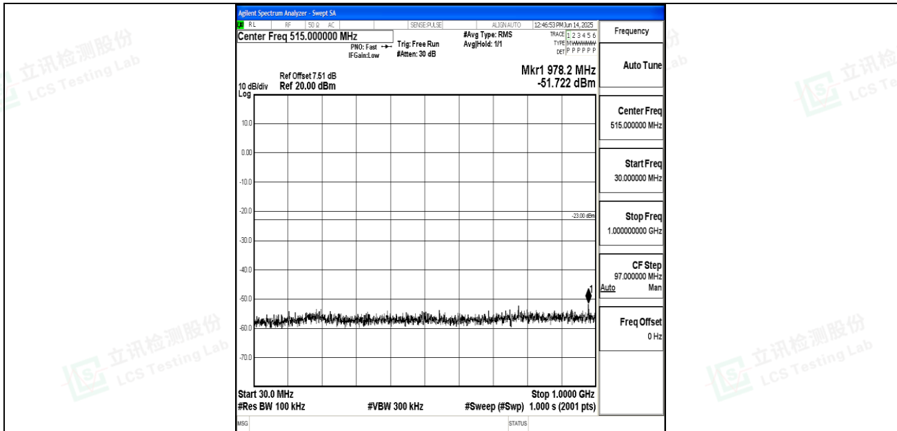
Band25_10MHz_16QAM_26365_1RB#0_30~1000_30~1000
