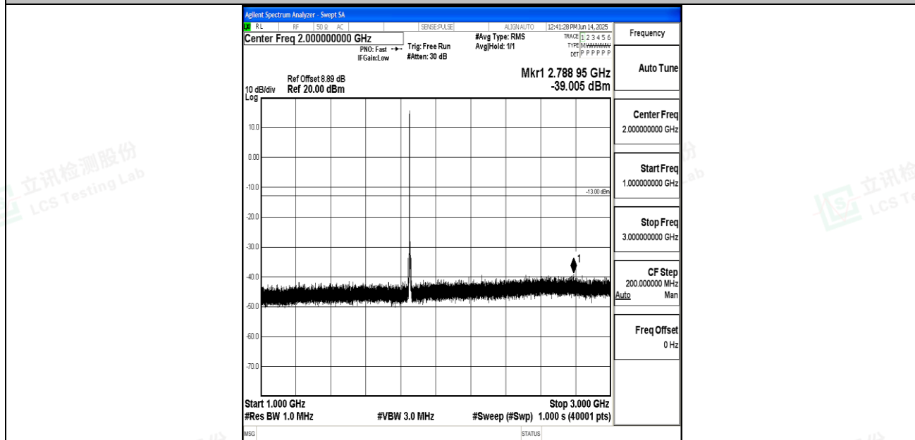
Band25_5MHz_16QAM_26065_1RB#0_1000~3000_1000~3000
