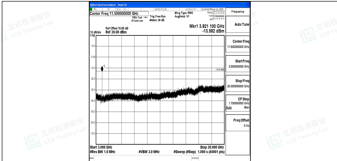
Band25_5MHz_16QAM_26665_1RB#0_3000~20000_3000~20000
