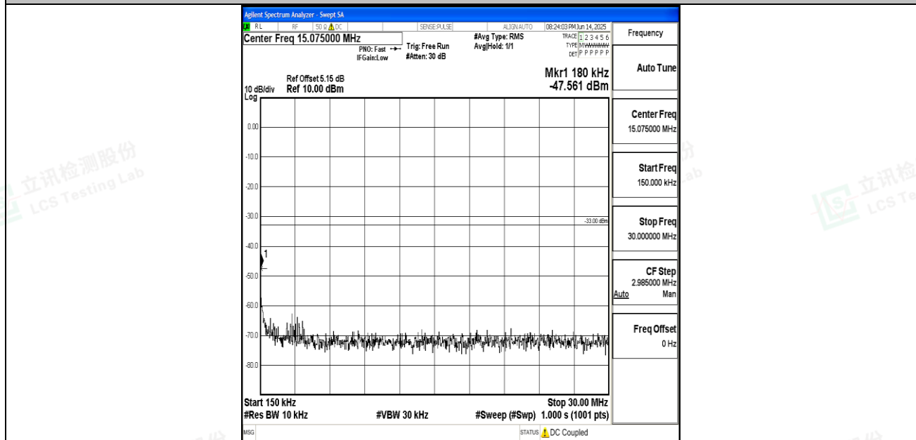
Band25_3MHz_16QAM_26675_1RB#0_0.15~30_0.15~30
