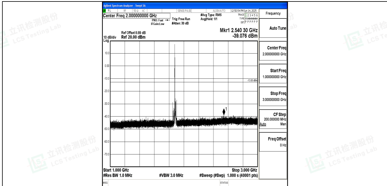
Band25_15MHz_QPSK_26365_1RB#0_1000~3000_1000~3000
