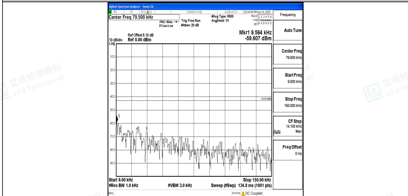
Band25_10MHz_QPSK_26090_1RB#0_0.009~0.15_0.009~0.15
