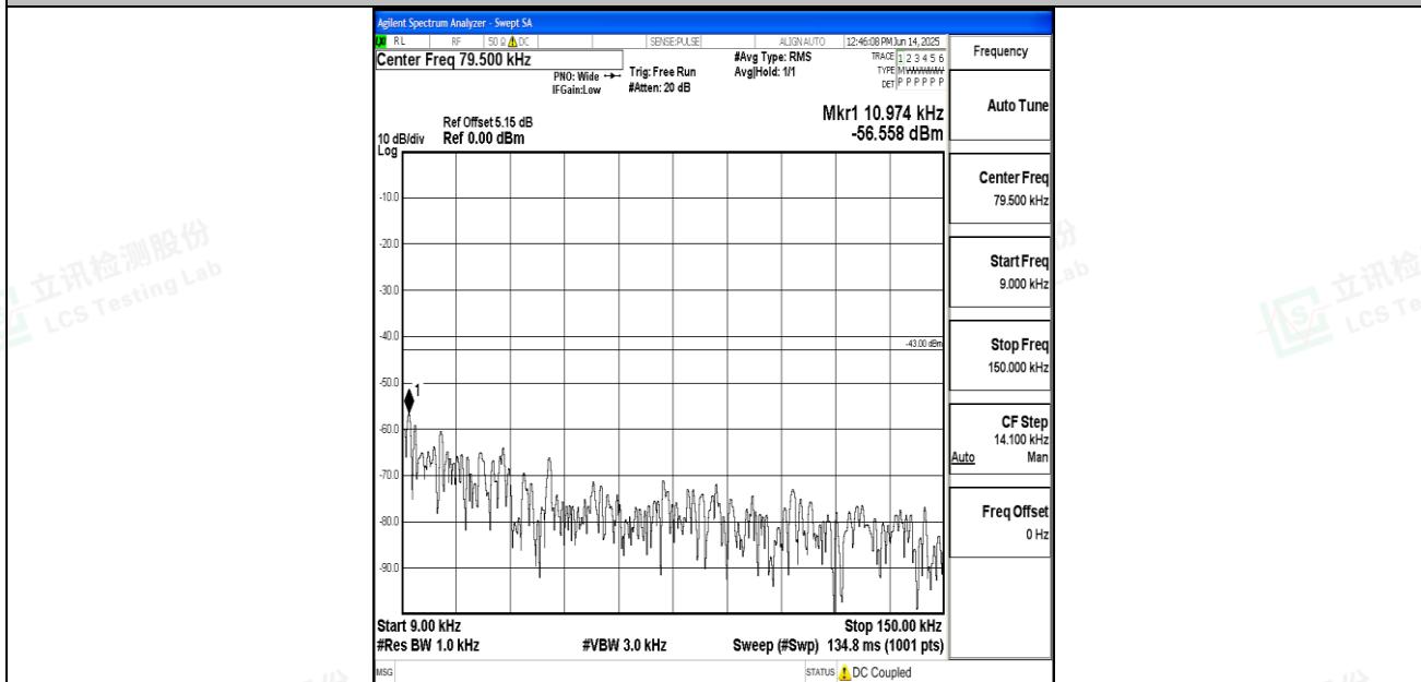
Band25_10MHz_QPSK_26365_1RB#0_0.009~0.15_0.009~0.15
