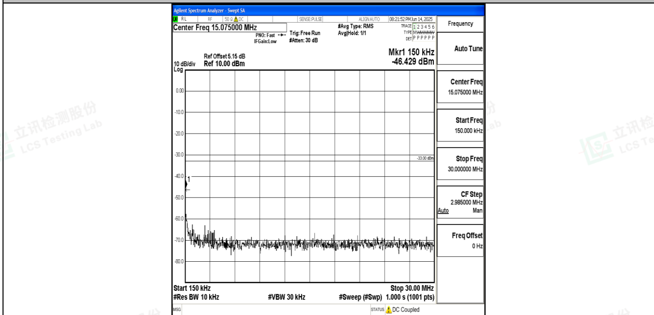
Band25_3MHz_QPSK_26365_1RB#0_0.15~30_0.15~30
