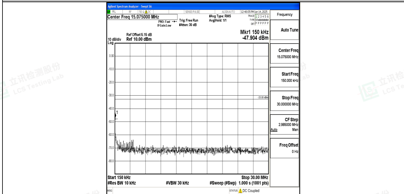
Band25_10MHz_16QAM_26640_1RB#0_0.15~30_0.15~30
