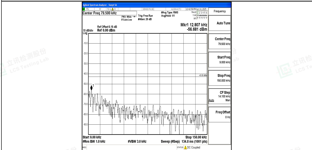
Band25_5MHz_QPSK_26665_1RB#0_0.009~0.15_0.009~0.15
