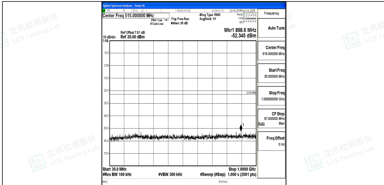
Band25_5MHz_16QAM_26065_1RB#0_30~1000_30~1000
