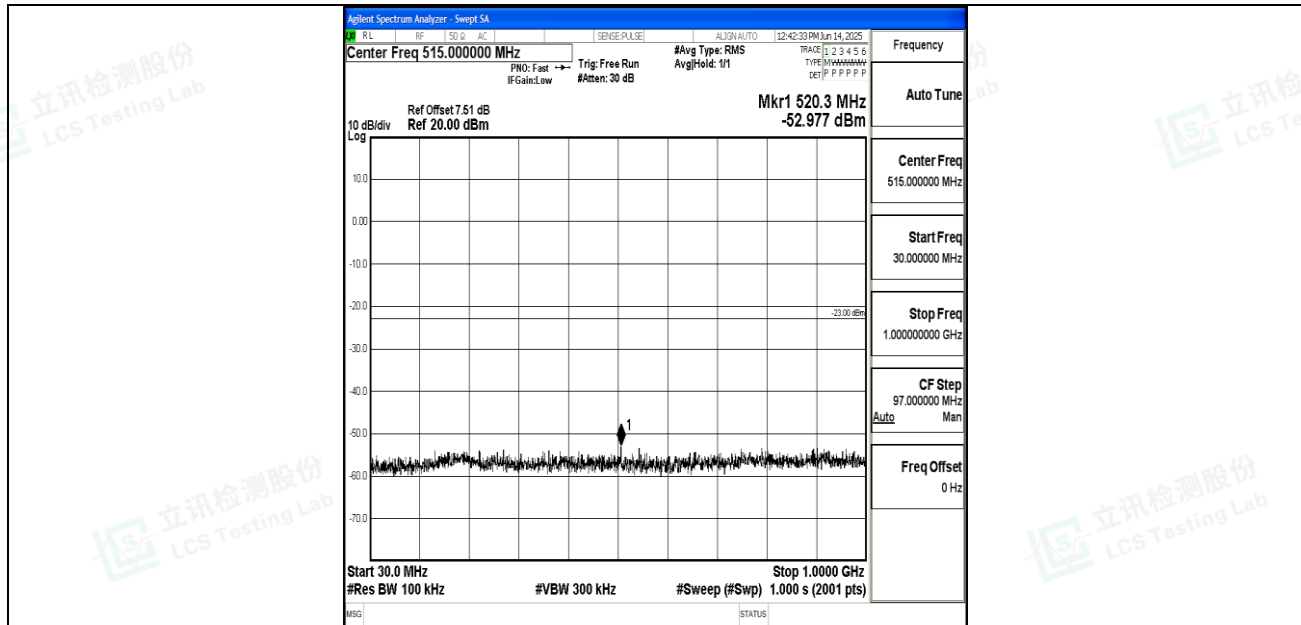
Band25_5MHz_16QAM_26365_1RB#0_30~1000_30~1000
