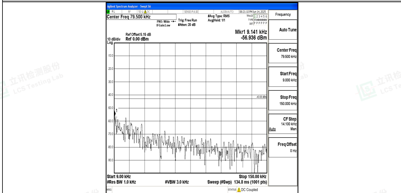
Band25_3MHz_16QAM_26055_1RB#0_0.009~0.15_0.009~0.15
