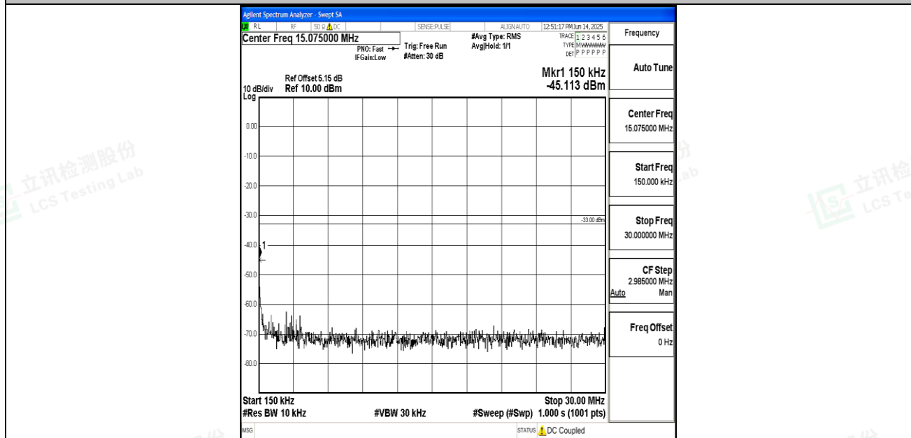
Band25_15MHz_16QAM_26365_1RB#0_0.15~30_0.15~30
