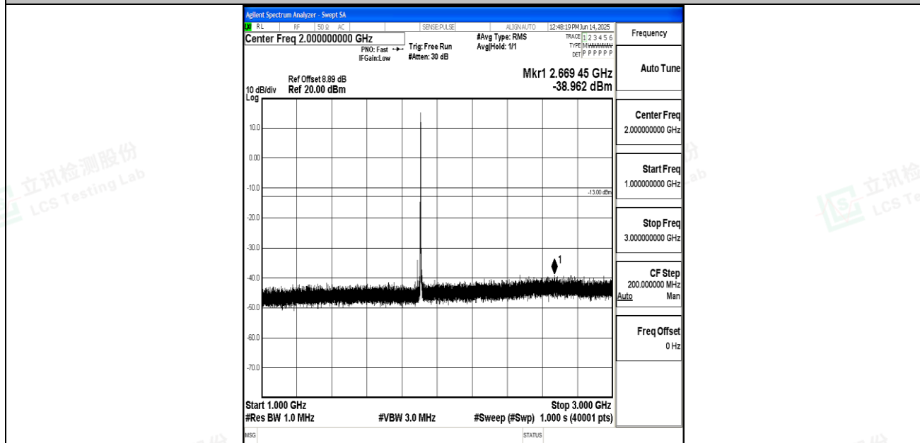
Band25_10MHz_16QAM_26640_1RB#0_1000~3000_1000~3000
