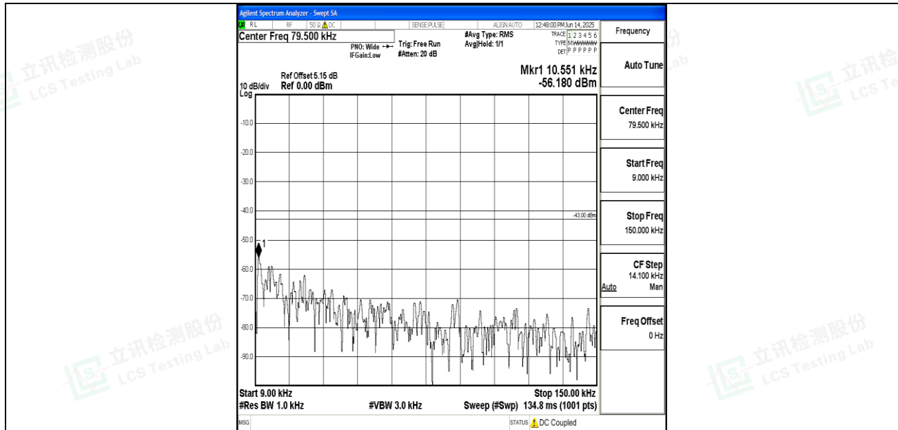
Band25_10MHz_16QAM_26640_1RB#0_0.009~0.15_0.009~0.15
