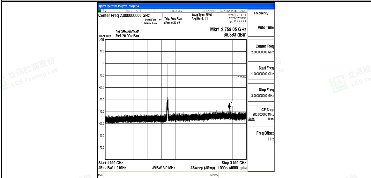
Band25_10MHz_16QAM_26365_1RB#0_1000~3000_1000~3000
