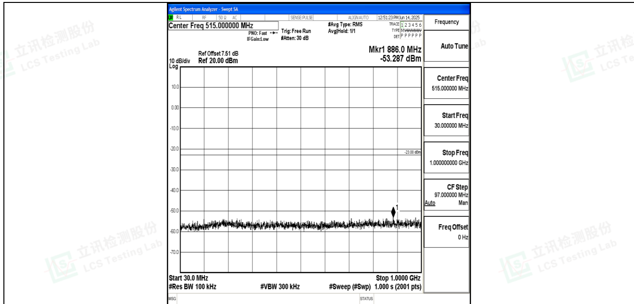
Band25_15MHz_16QAM_26365_1RB#0_30~1000_30~1000
