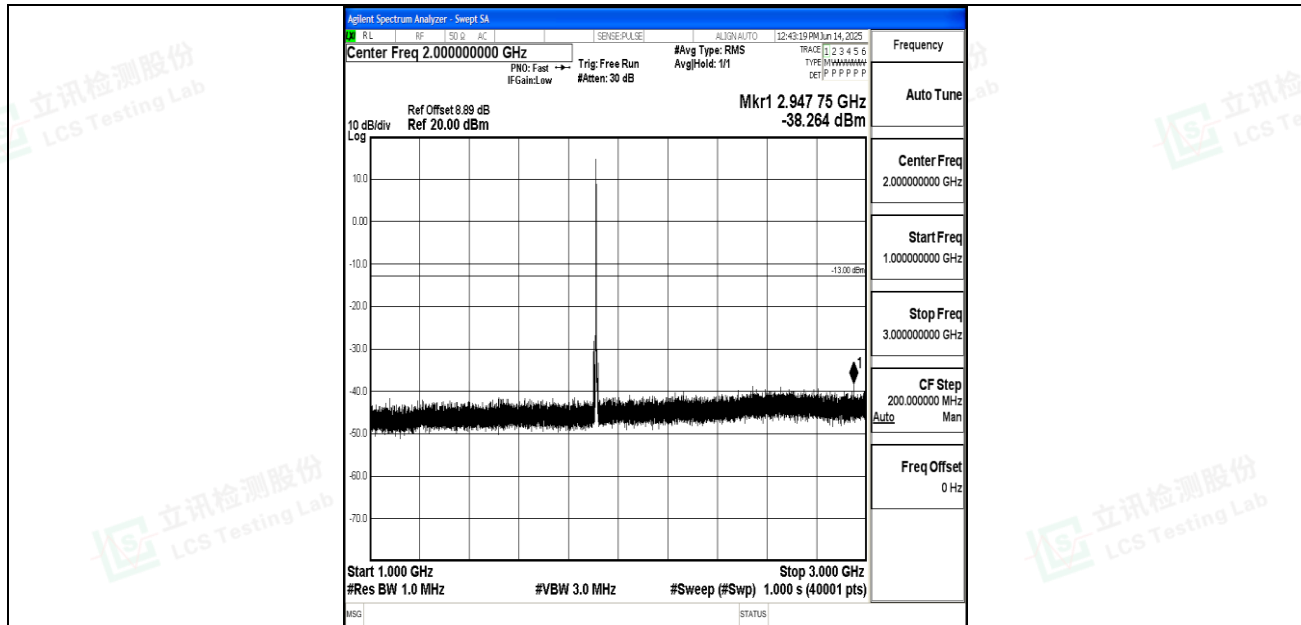
Band25_5MHz_QPSK_26665_1RB#0_1000~3000_1000~3000
