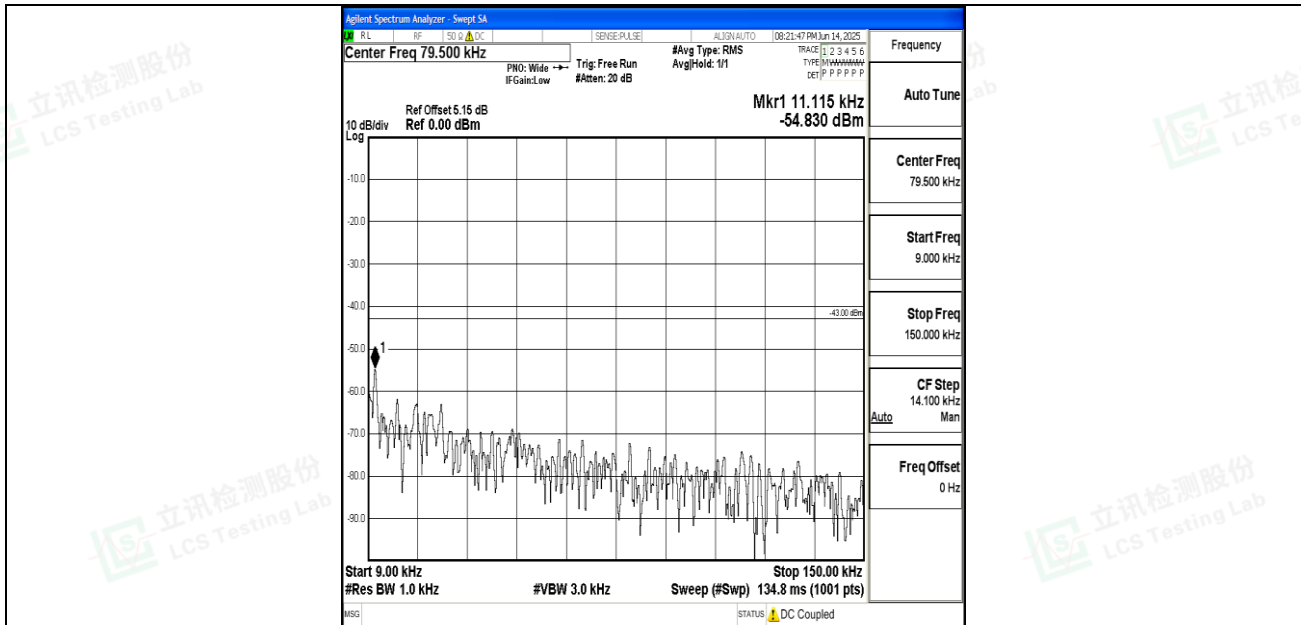
Band25_3MHz_QPSK_26365_1RB#0_0.009~0.15_0.009~0.15
