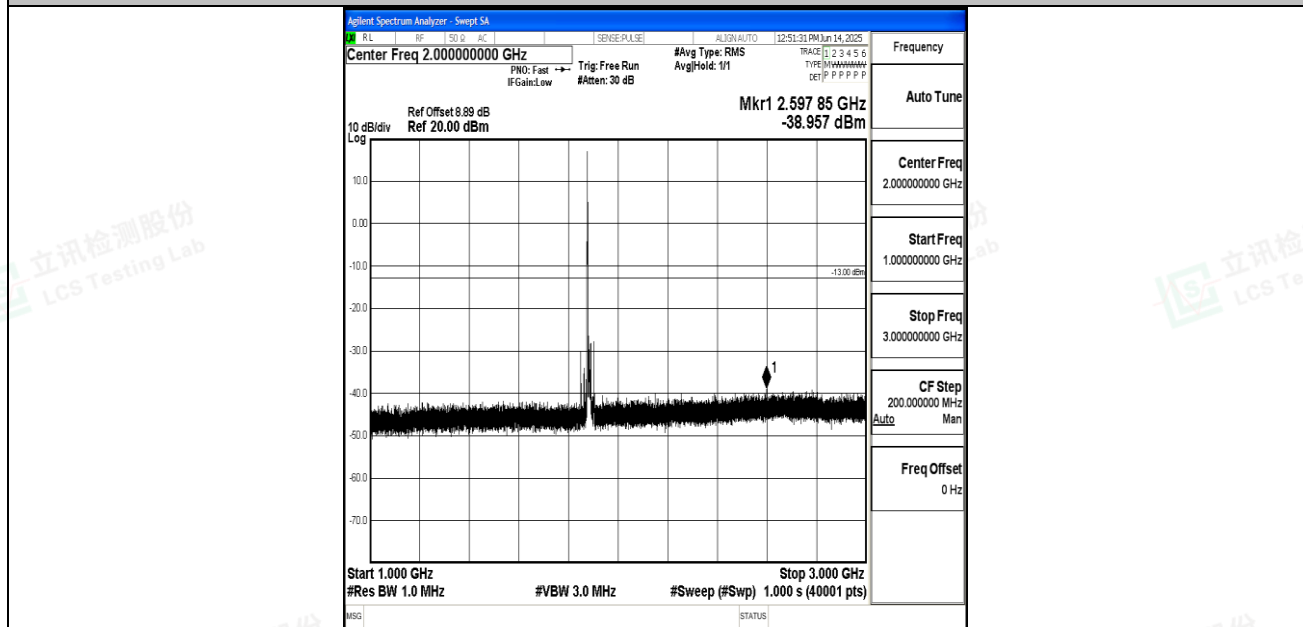
Band25_15MHz_16QAM_26365_1RB#0_1000~3000_1000~3000
