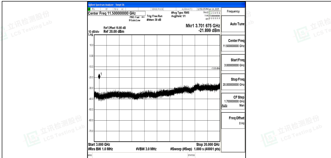
Band25_15MHz_16QAM_26115_1RB#0_3000~20000_3000~20000
