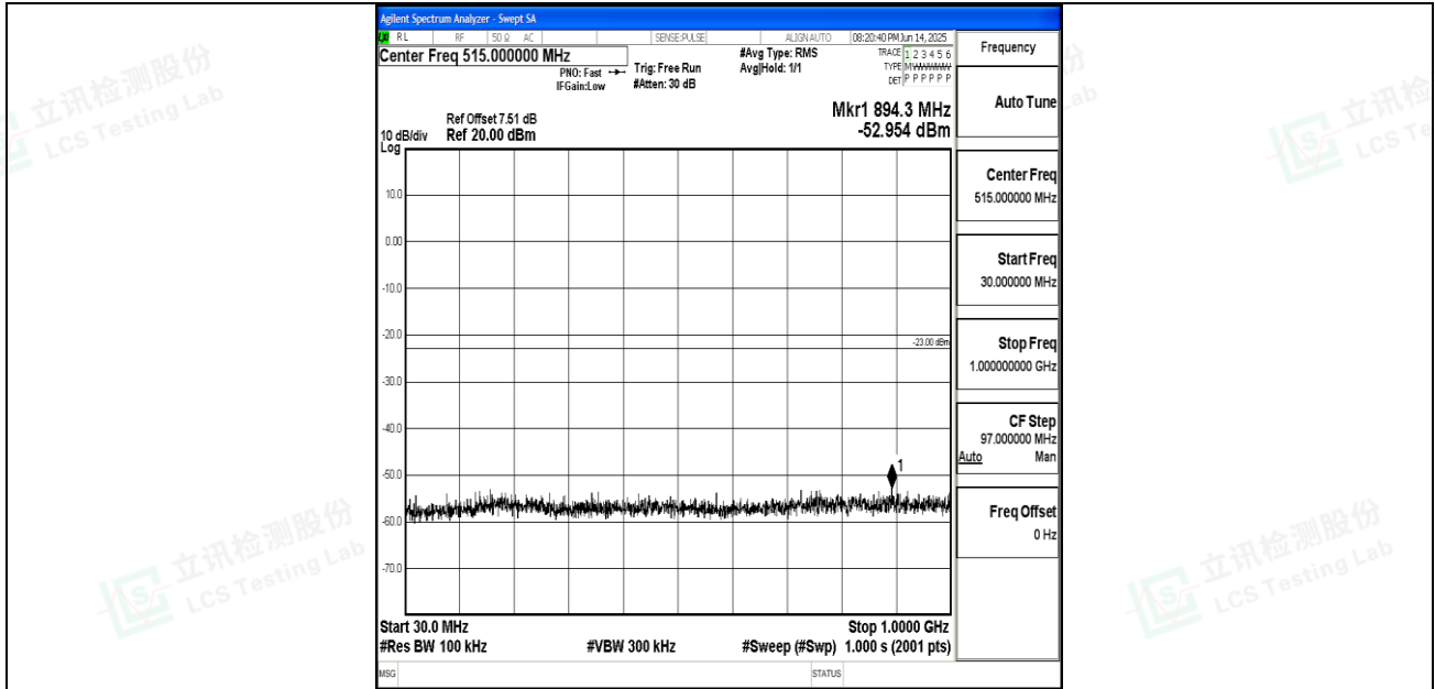
Band25_3MHz_QPSK_26055_1RB#0_30~1000_30~1000
