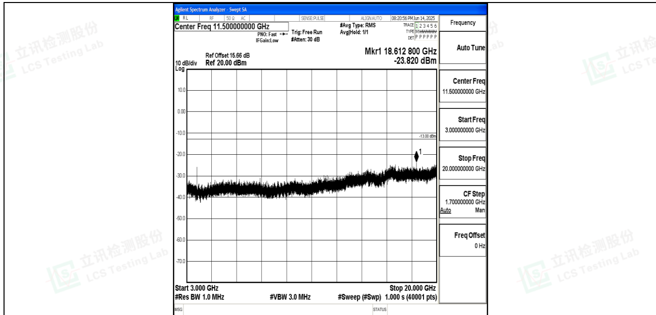
Band25_3MHz_QPSK_26055_1RB#0_3000~20000_3000~20000
