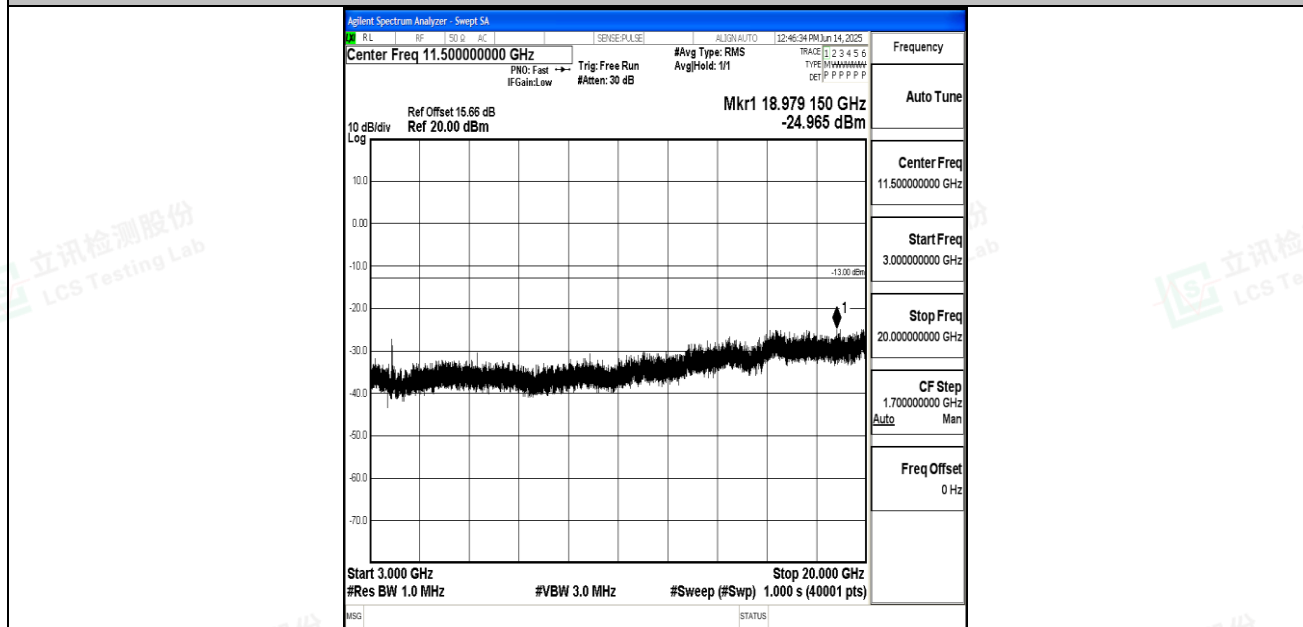
Band25_10MHz_QPSK_26365_1RB#0_3000~20000_3000~20000
