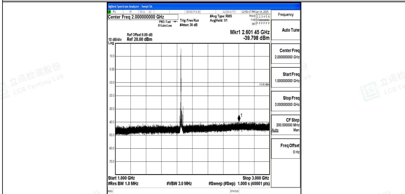
Band25_15MHz_16QAM_26115_1RB#0_1000~3000_1000~3000
