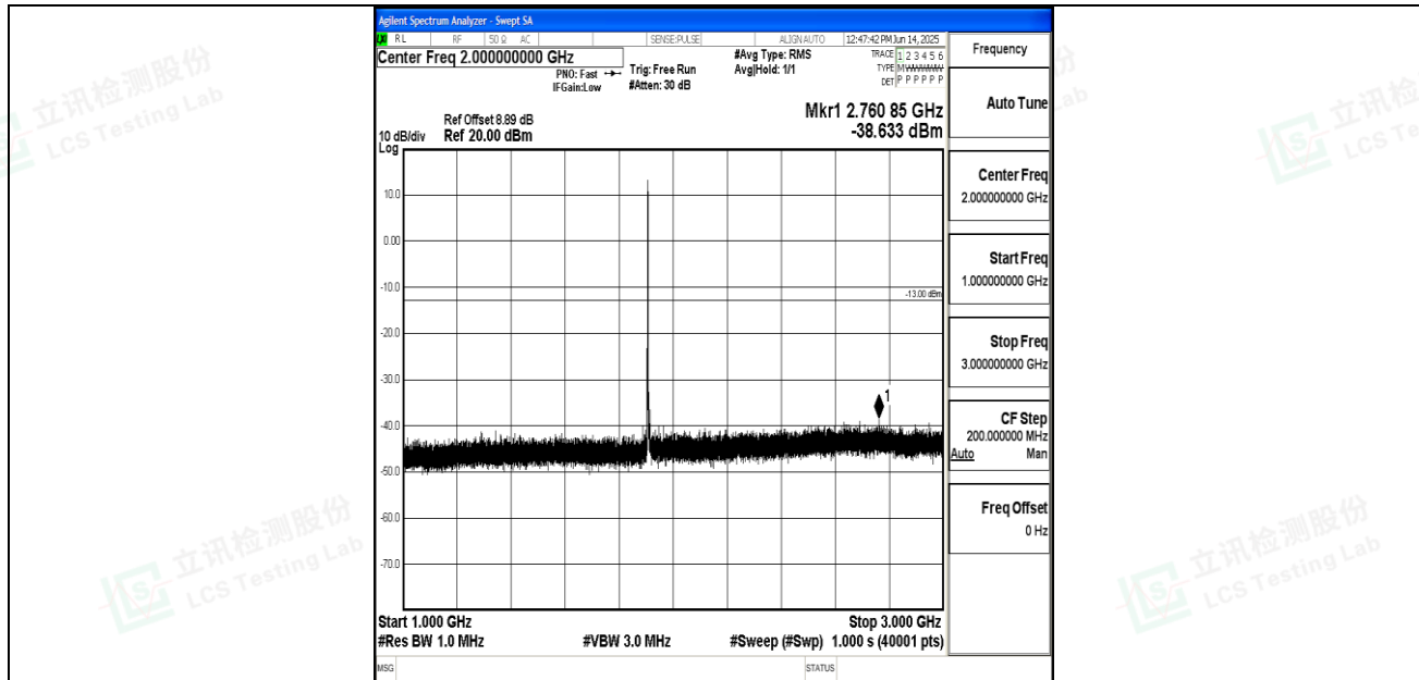
Band25_10MHz_QPSK_26640_1RB#0_1000~3000_1000~3000
