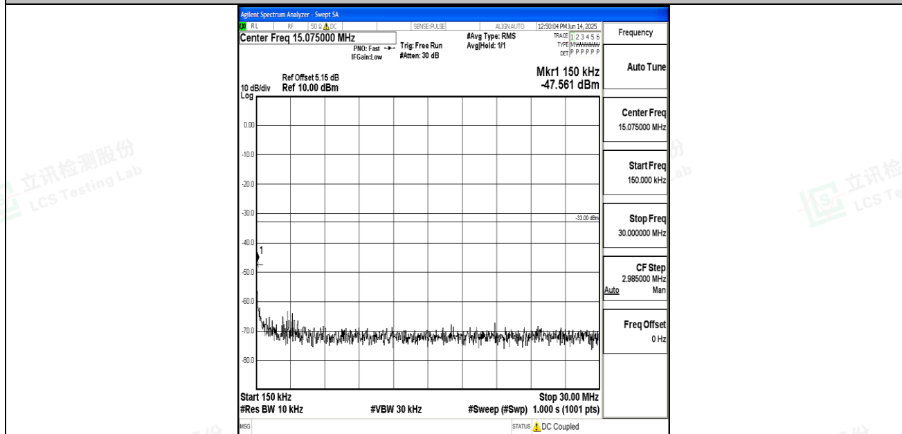
Band25_15MHz_16QAM_26115_1RB#0_0.15~30_0.15~30
