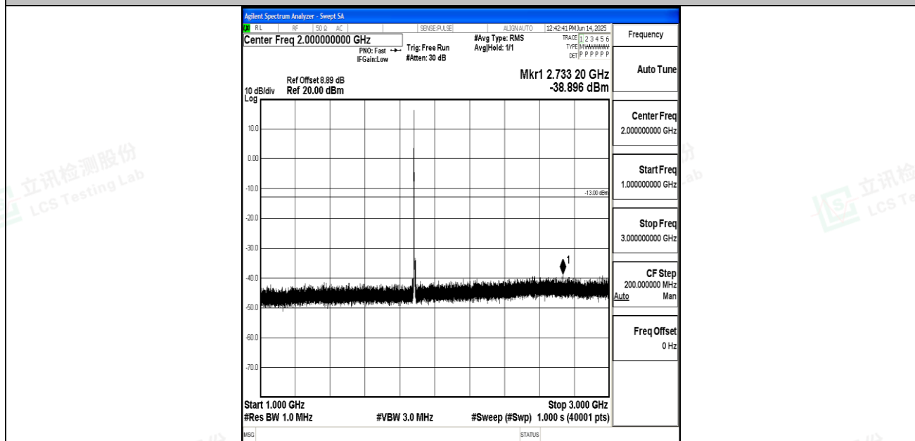
Band25_5MHz_16QAM_26365_1RB#0_1000~3000_1000~3000
