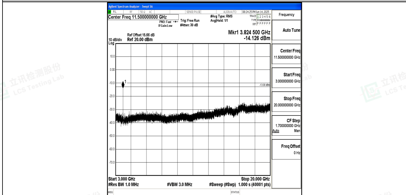
Band25_3MHz_16QAM_26675_1RB#0_3000~20000_3000~20000
