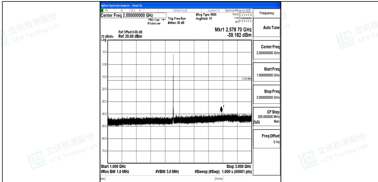
Band25_3MHz_16QAM_26675_1RB#0_1000~3000_1000~3000
