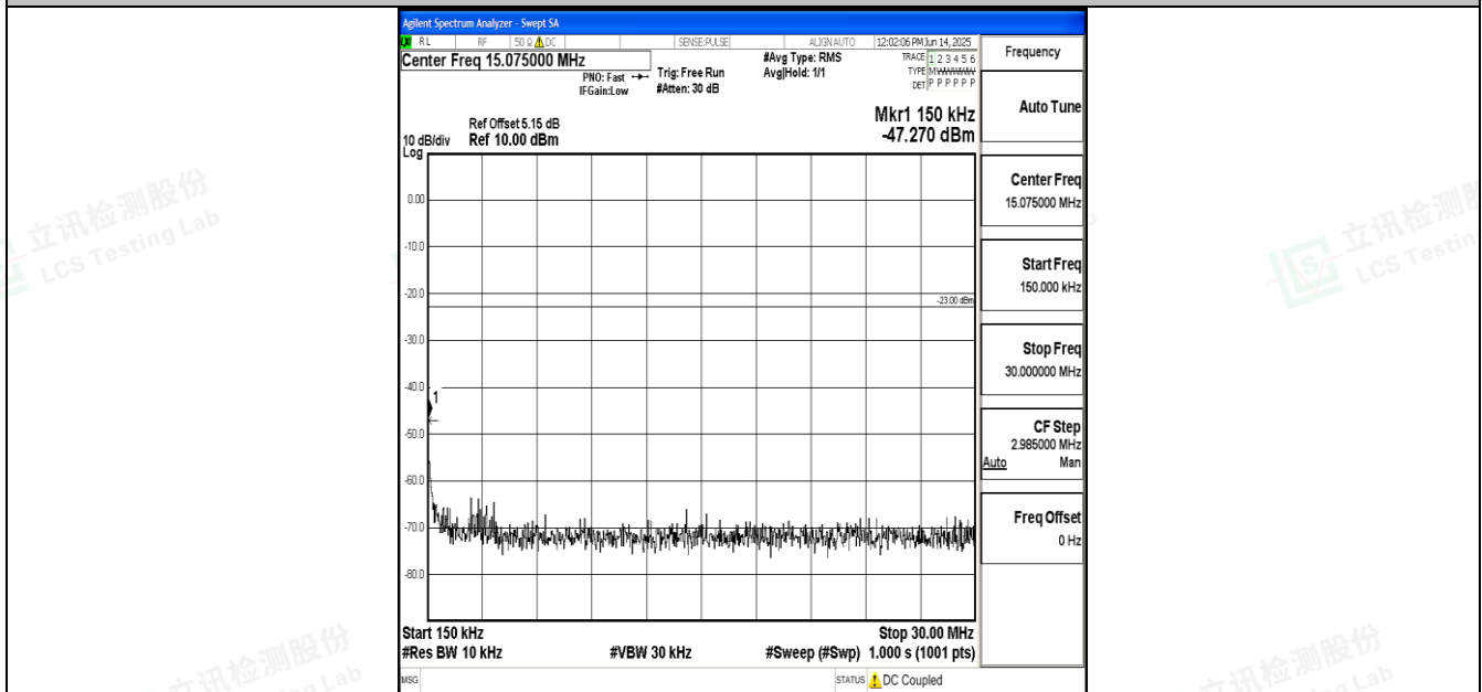
Band12_10MHz_QPSK_23095_1RB#0_0.15~30_0.15~30
