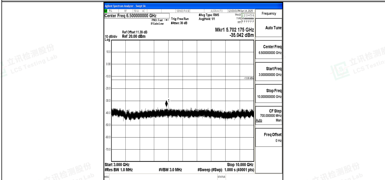
Band12_10MHz_16QAM_23095_1RB#0_3000~10000_3000~10000
