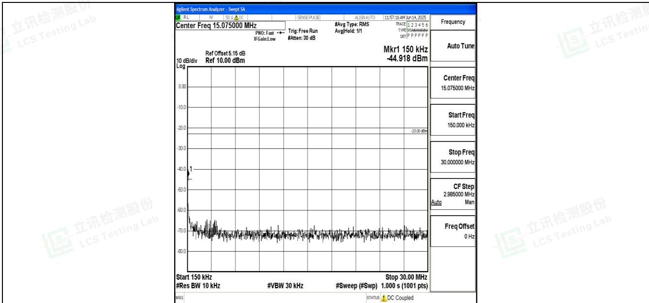
Band12_5MHz_16QAM_23035_1RB#0_0.15~30_0.15~30
