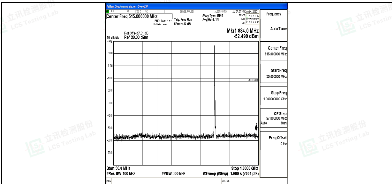
Band12_5MHz_QPSK_23095_1RB#0_30~1000_30~1000
