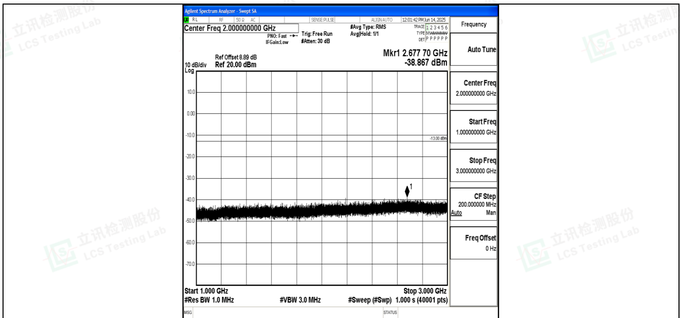
Band12_10MHz_16QAM_23060_1RB#0_1000~3000_1000~3000
