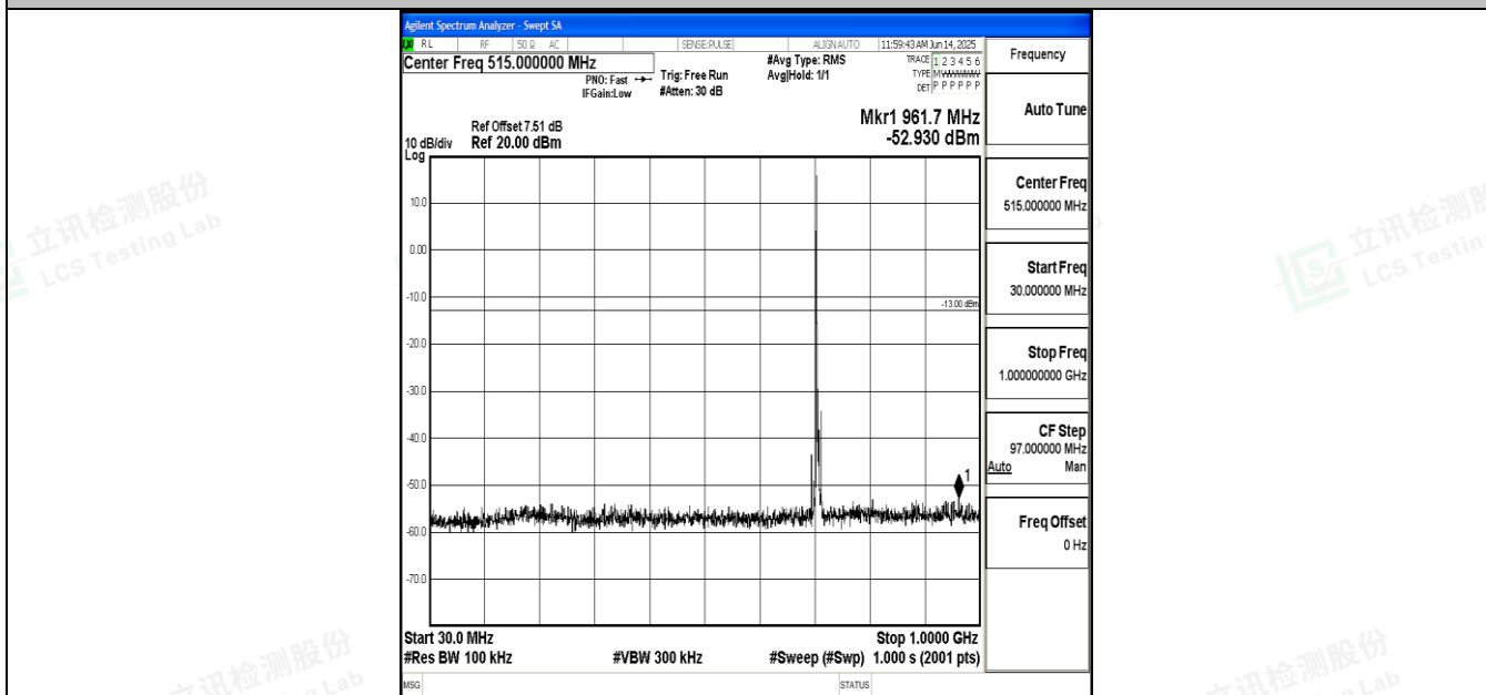
Band12_5MHz_16QAM_23155_1RB#0_30~1000_30~1000
