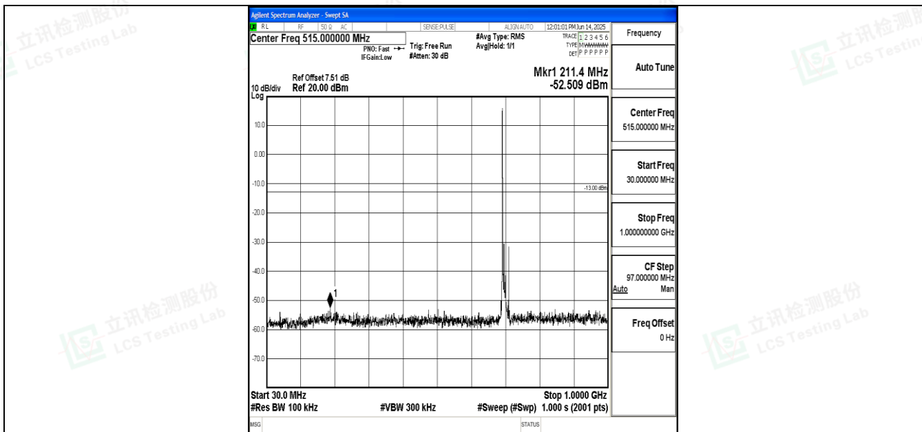
Band12_10MHz_QPSK_23060_1RB#0_30~1000_30~1000
