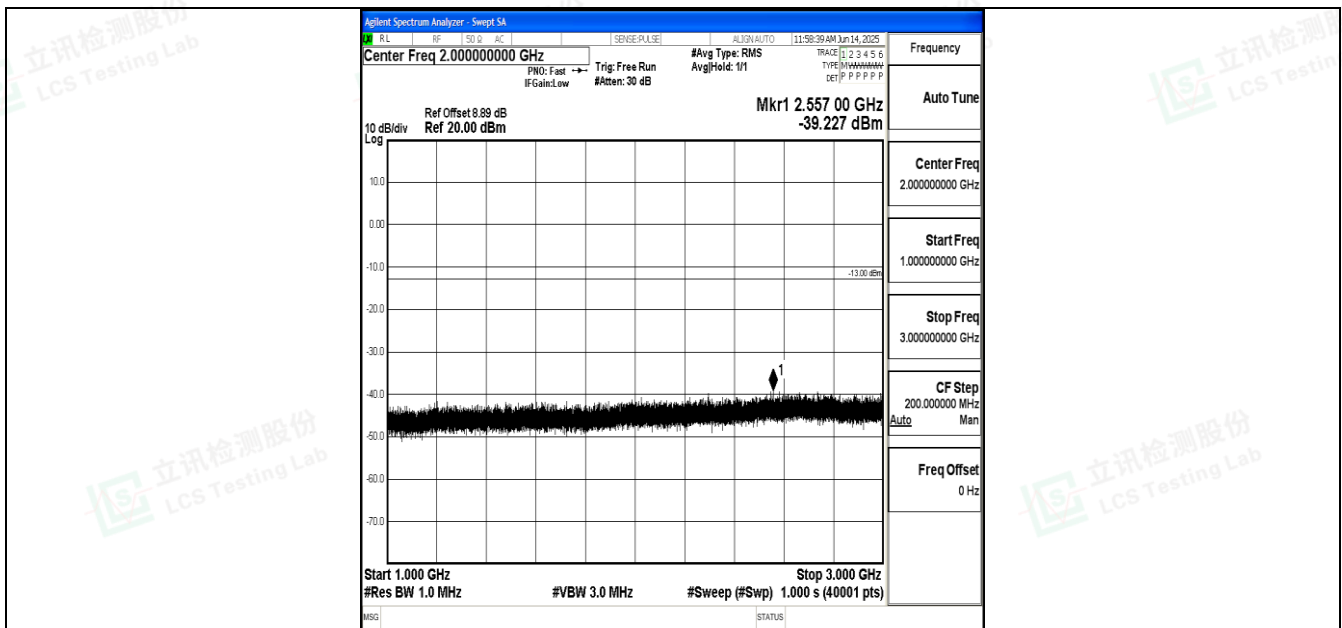
Band12_5MHz_16QAM_23095_1RB#0_1000~3000_1000~3000
