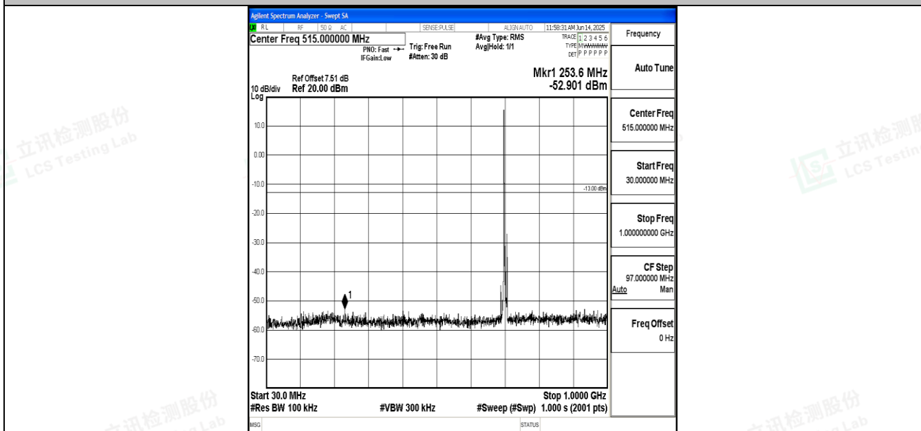
Band12_5MHz_16QAM_23095_1RB#0_30~1000_30~1000
