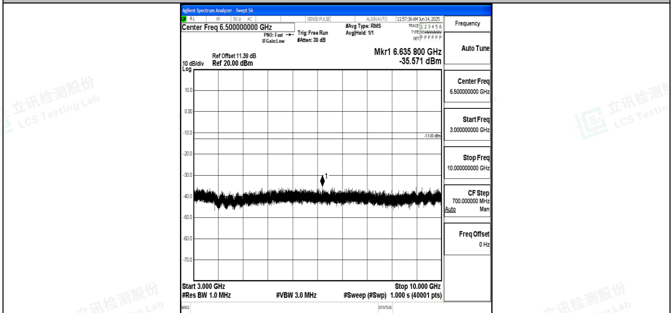
Band12_5MHz_16QAM_23035_1RB#0_3000~10000_3000~10000
