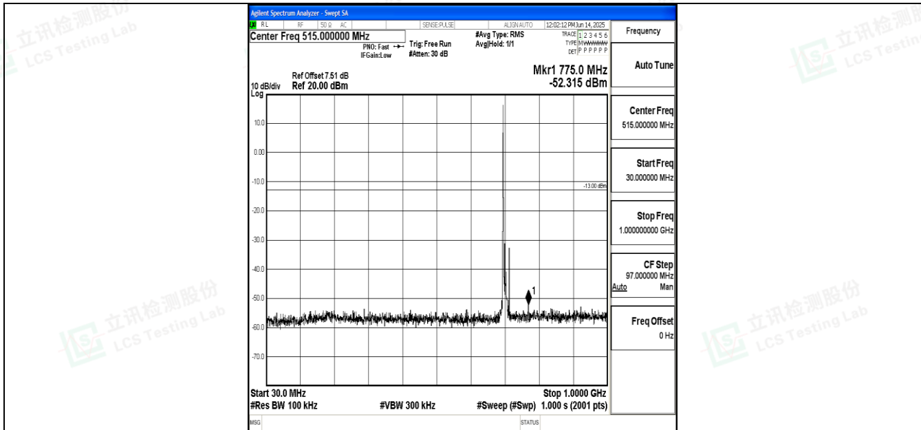
Band12_10MHz_QPSK_23095_1RB#0_30~1000_30~1000
