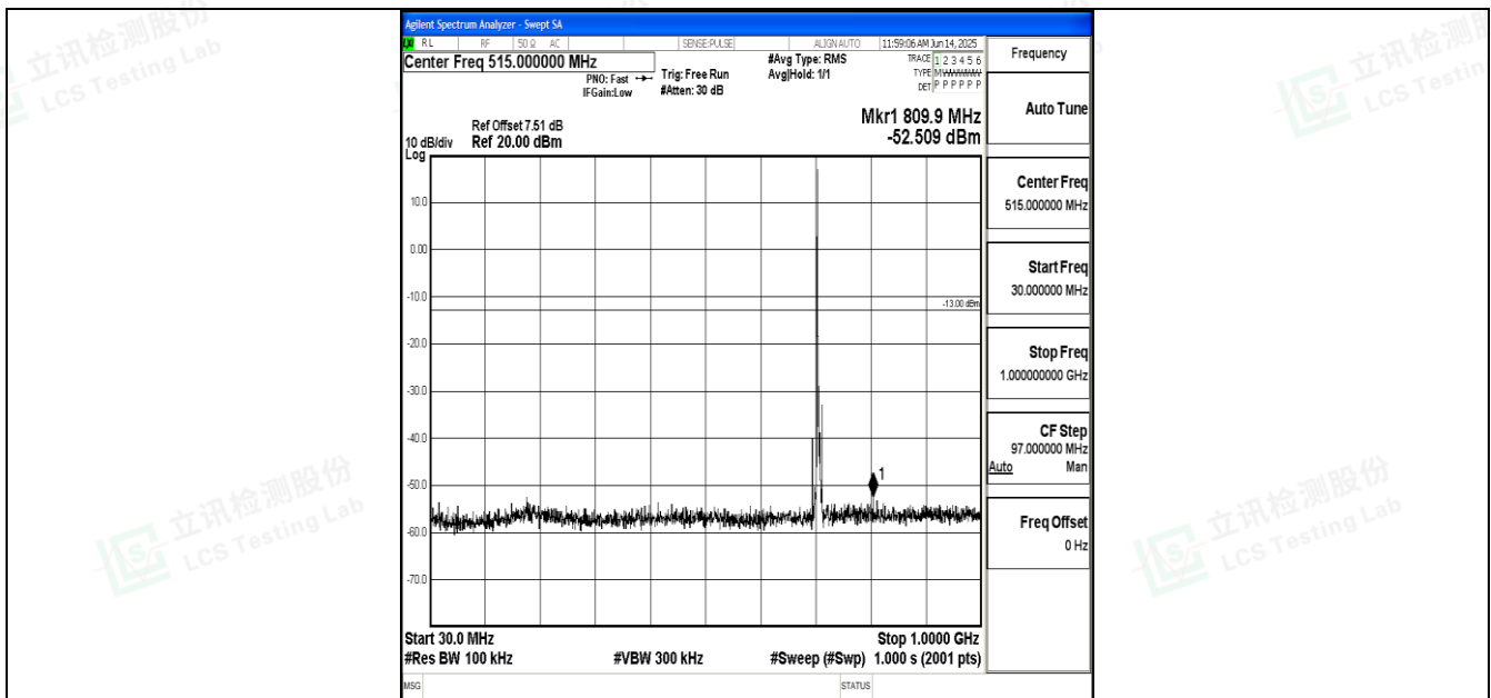
Band12_5MHz_QPSK_23155_1RB#0_30~1000_30~1000
