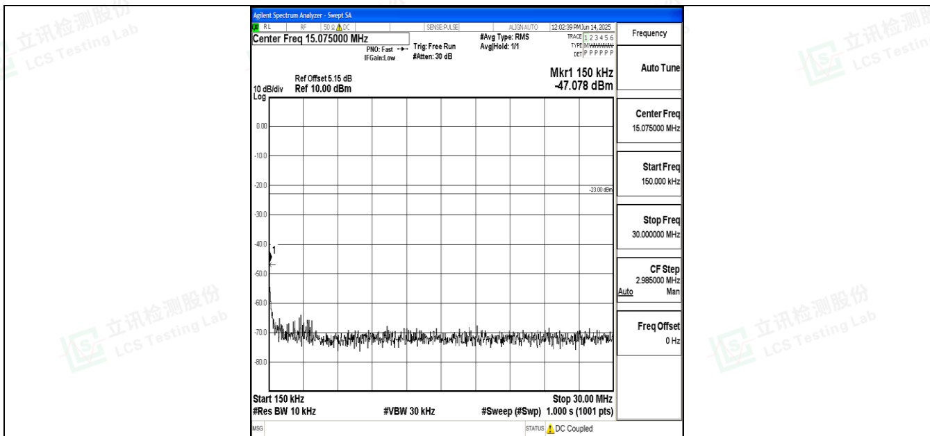
Band12_10MHz_16QAM_23095_1RB#0_0.15~30_0.15~30
