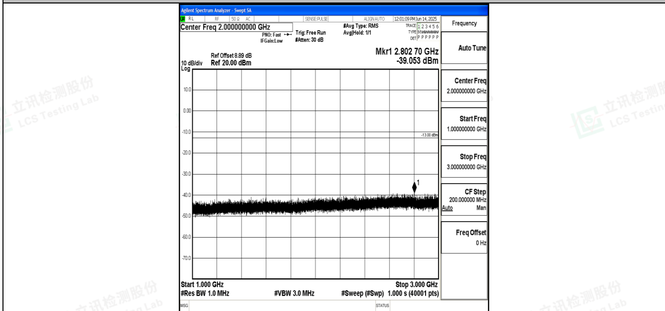
Band12_10MHz_QPSK_23060_1RB#0_1000~3000_1000~3000
