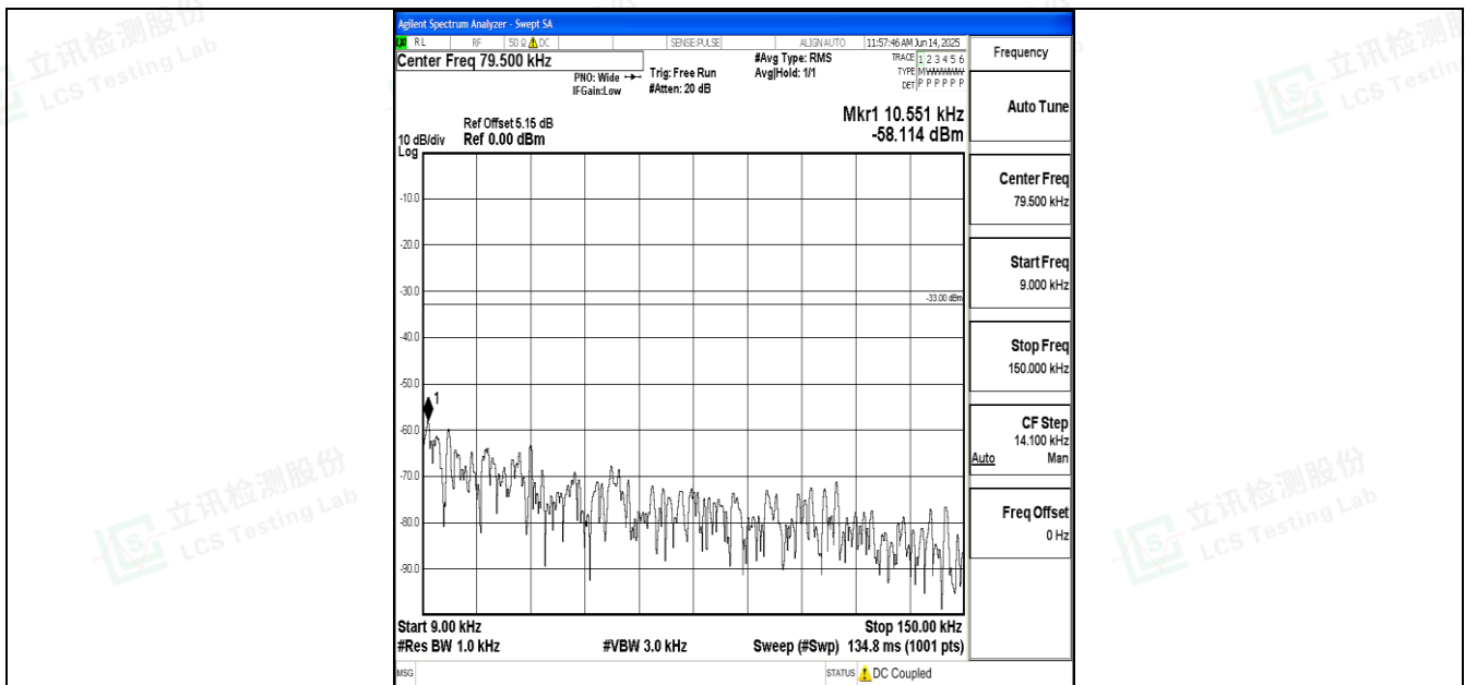
Band12_5MHz_QPSK_23095_1RB#0_0.009~0.15_0.009~0.15
