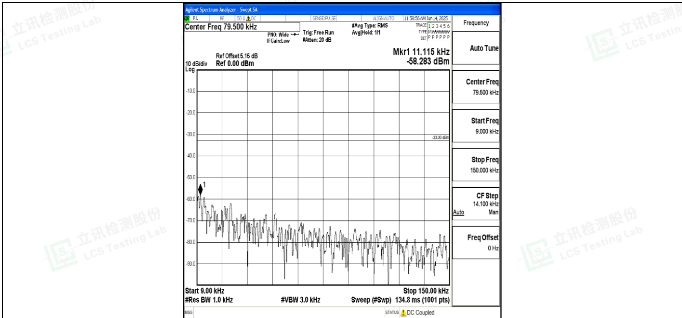
Band12_5MHz_QPSK_23155_1RB#0_0.009~0.15_0.009~0.15
