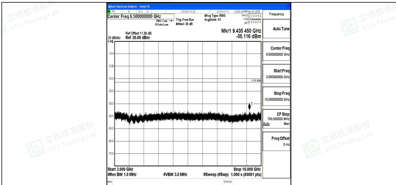
Band12_10MHz_QPSK_23060_1RB#0_3000~10000_3000~10000
