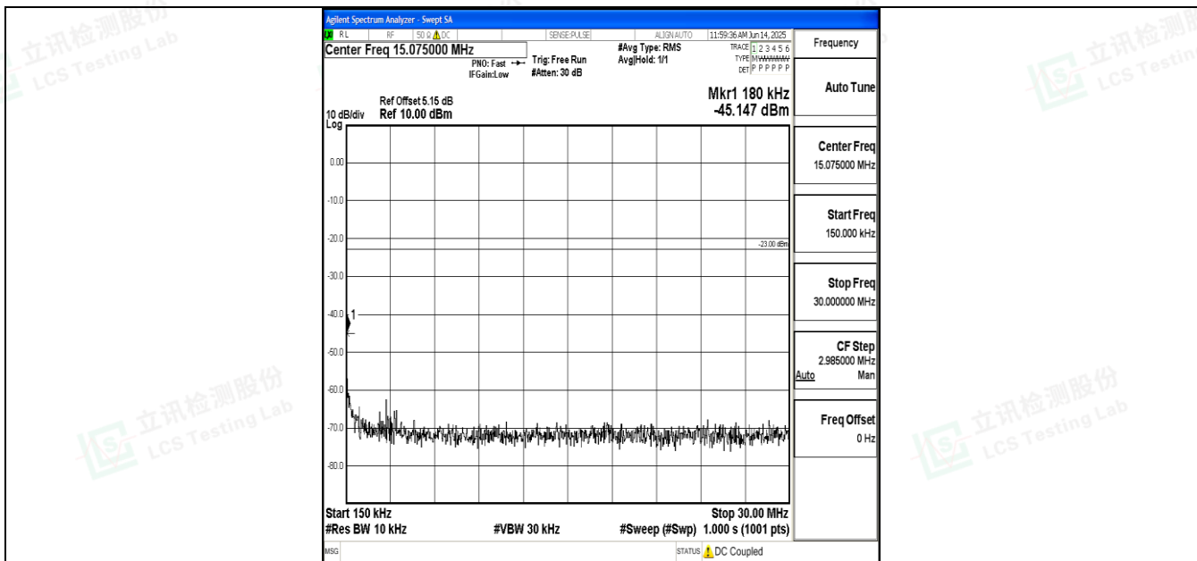
Band12_5MHz_16QAM_23155_1RB#0_0.15~30_0.15~30
