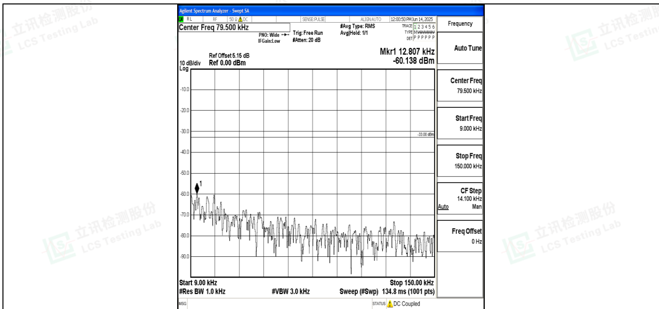
Band12_10MHz_QPSK_23060_1RB#0_0.009~0.15_0.009~0.15
