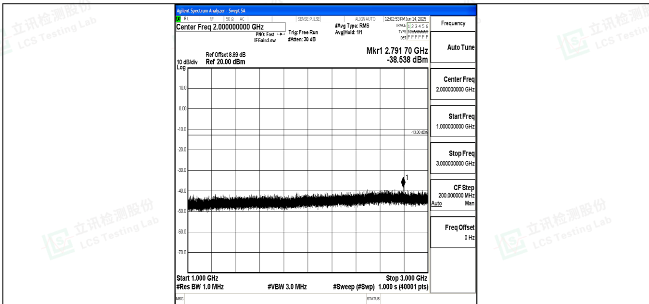
Band12_10MHz_16QAM_23095_1RB#0_1000~3000_1000~3000
