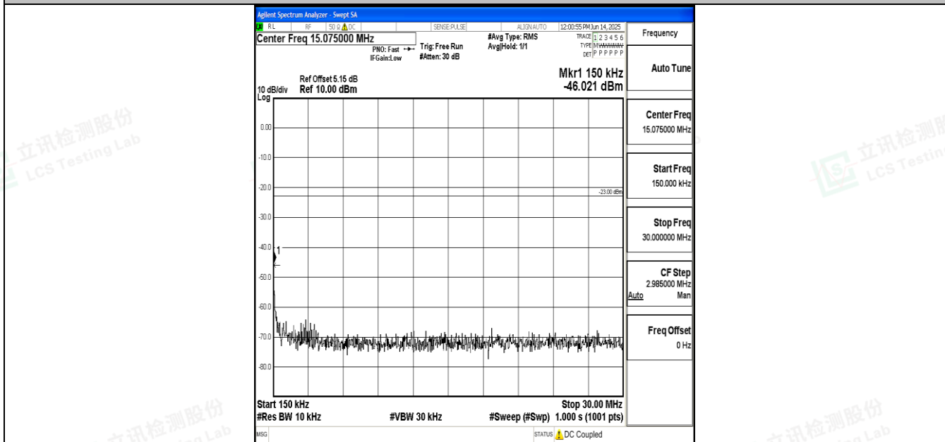
Band12_10MHz_QPSK_23060_1RB#0_0.15~30_0.15~30
