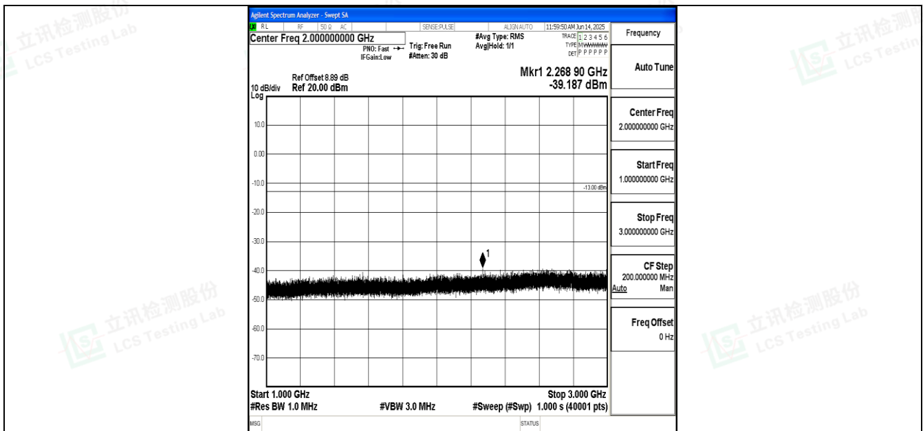
Band12_5MHz_16QAM_23155_1RB#0_1000~3000_1000~3000
