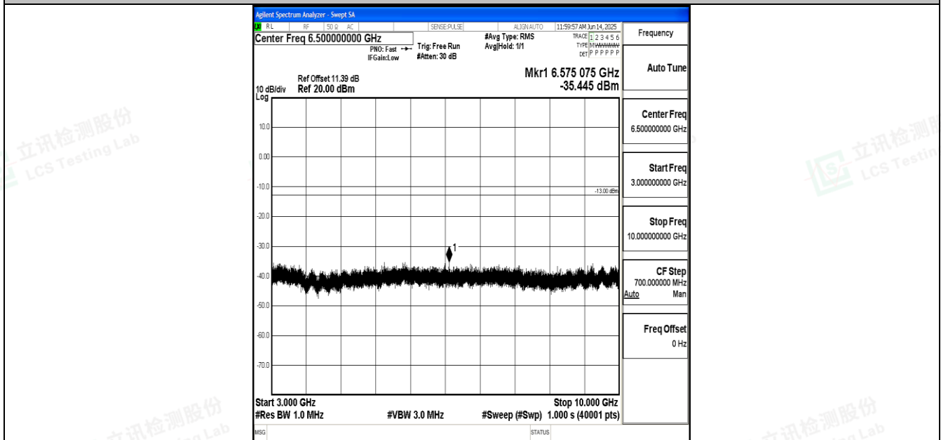
Band12_5MHz_16QAM_23155_1RB#0_3000~10000_3000~10000
