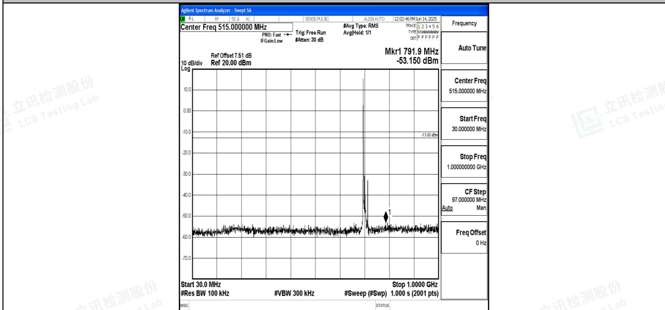
Band12_10MHz_16QAM_23095_1RB#0_30~1000_30~1000
