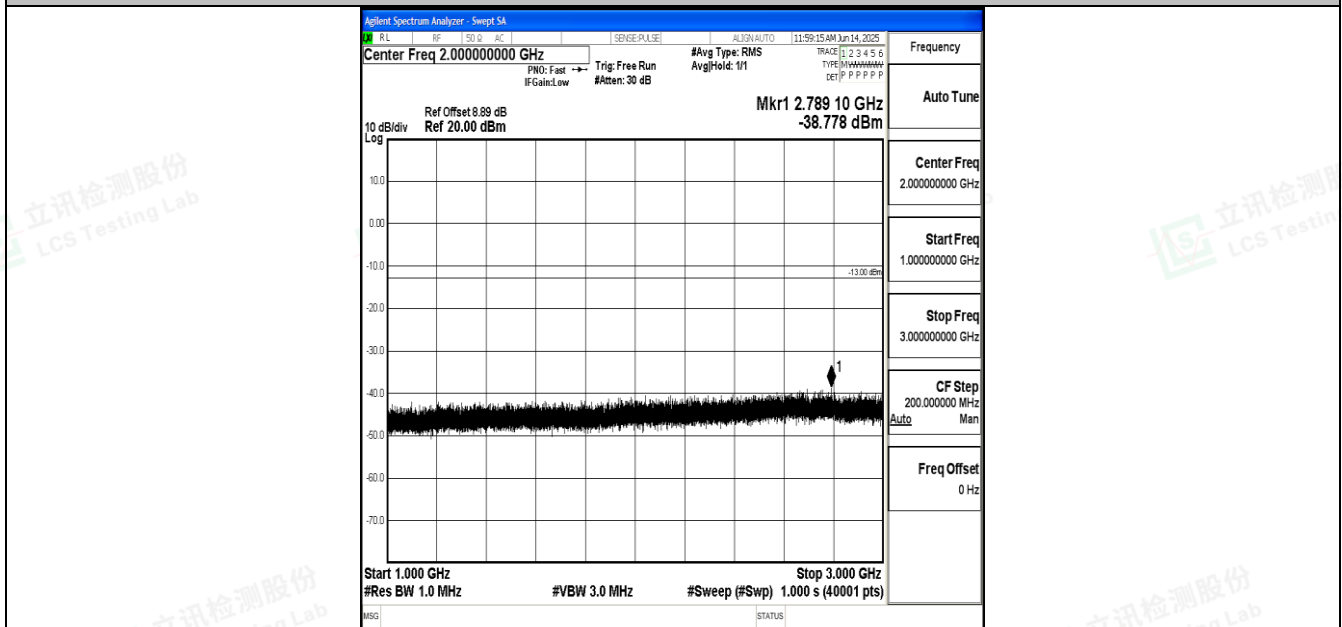
Band12_5MHz_QPSK_23155_1RB#0_1000~3000_1000~3000
