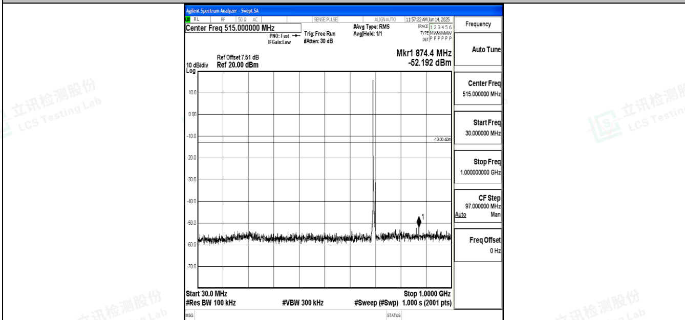
Band12_5MHz_16QAM_23035_1RB#0_30~1000_30~1000
