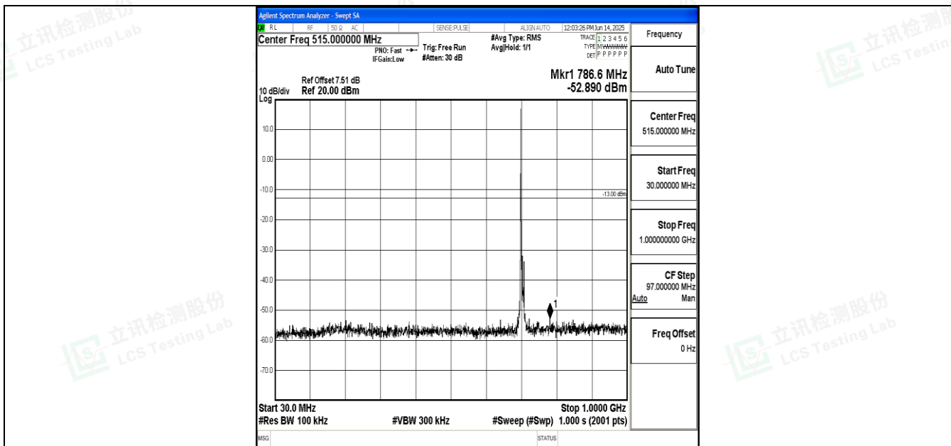
Band12_10MHz_QPSK_23130_1RB#0_30~1000_30~1000
