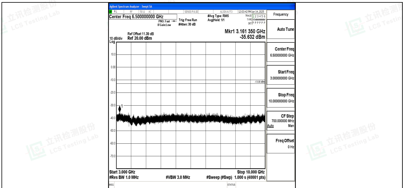
Band12_10MHz_QPSK_23130_1RB#0_3000~10000_3000~10000
