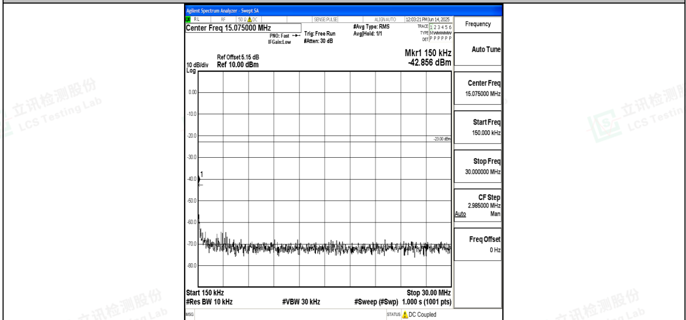
Band12_10MHz_QPSK_23130_1RB#0_0.15~30_0.15~30
