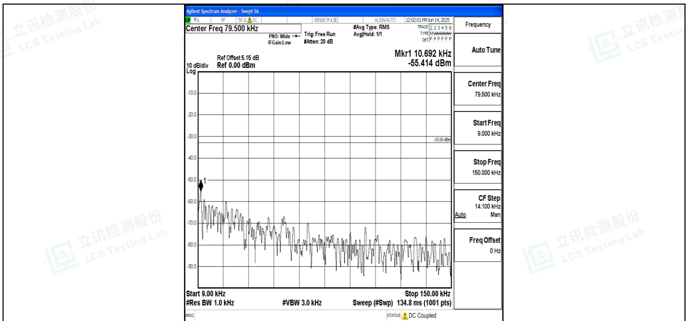
Band12_10MHz_QPSK_23095_1RB#0_0.009~0.15_0.009~0.15
