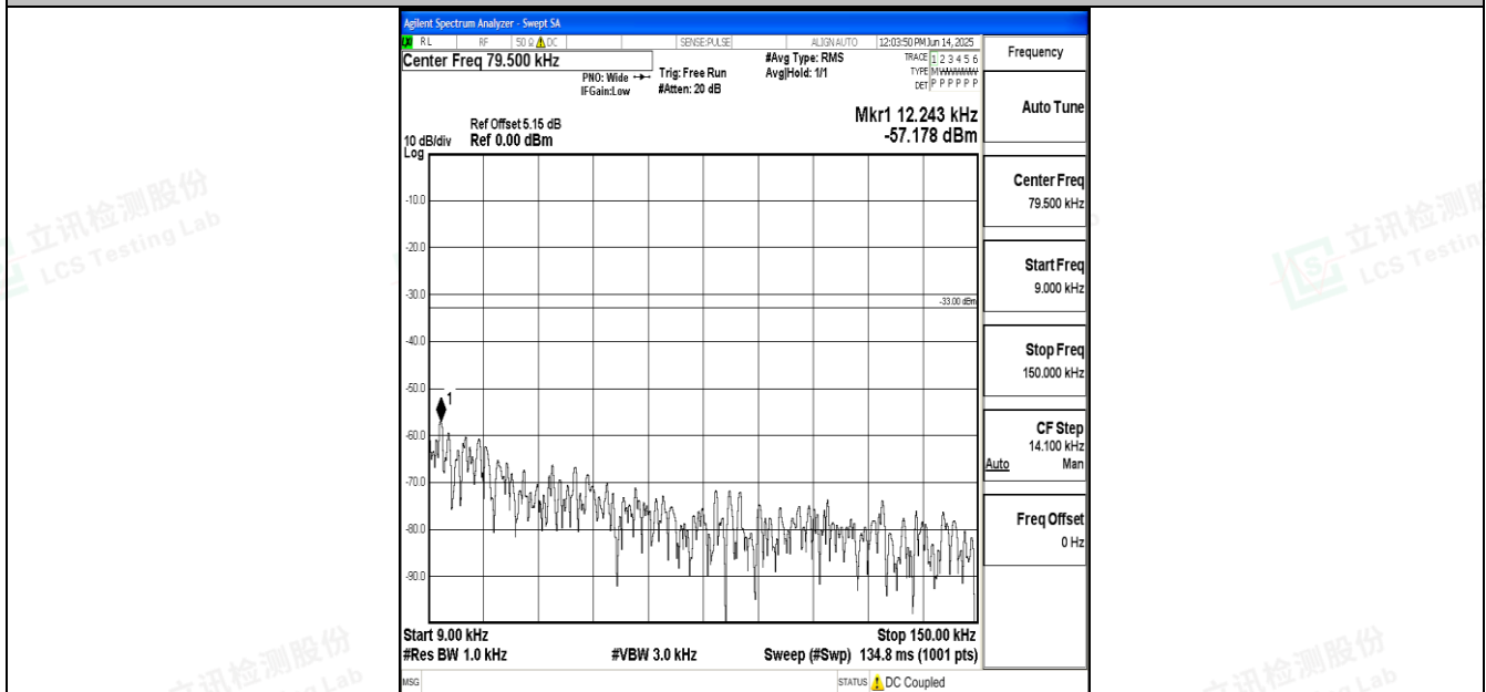
Band12_10MHz_16QAM_23130_1RB#0_0.009~0.15_0.009~0.15
