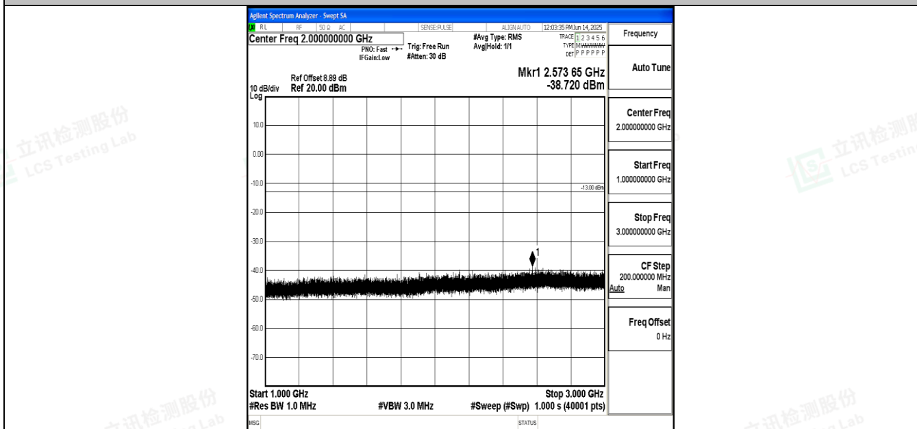
Band12_10MHz_QPSK_23130_1RB#0_1000~3000_1000~3000
