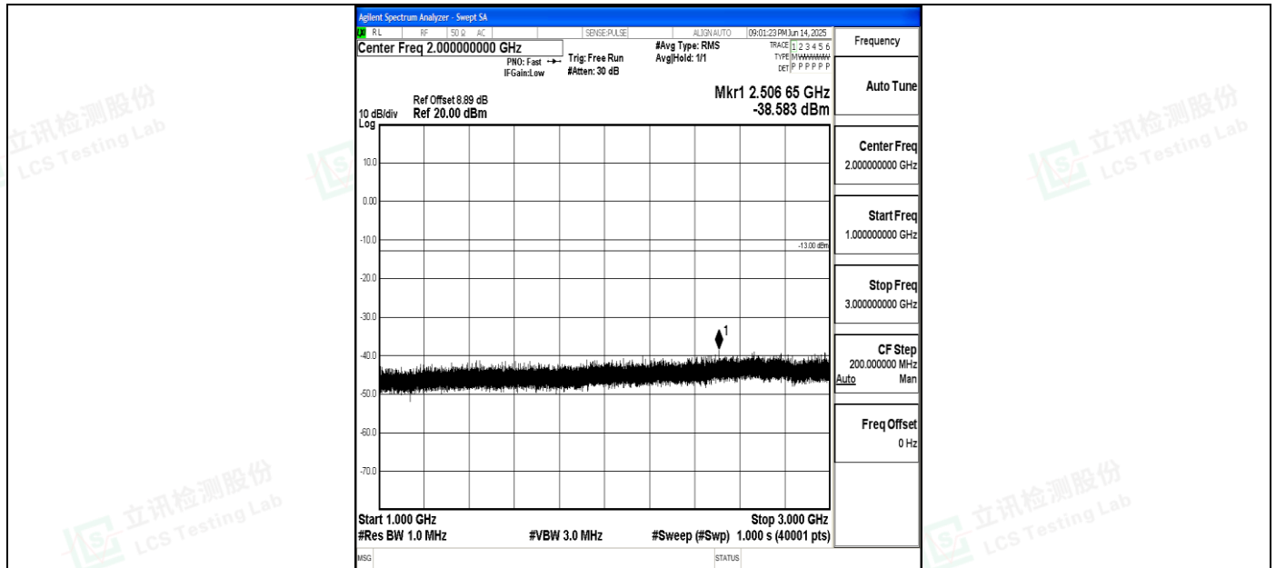
Band5_5MHz_QPSK_20525_1RB#0_1000~3000_1000~3000
