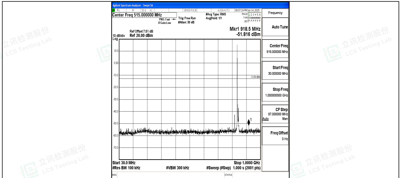
Band5_10MHz_16QAM_20600_1RB#0_30~1000_30~1000
