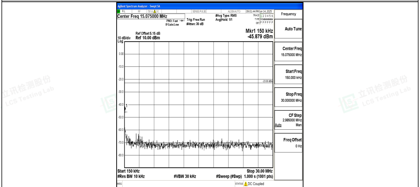
Band5_5MHz_16QAM_20525_1RB#0_0.15~30_0.15~30
