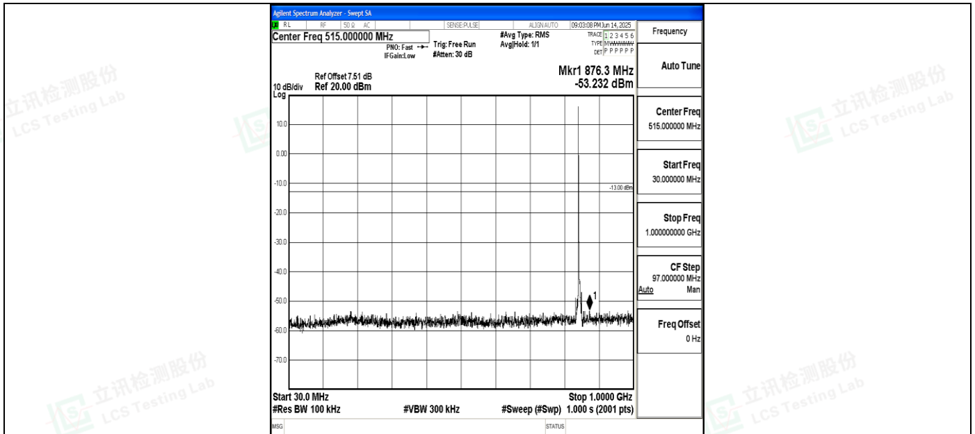
Band5_5MHz_16QAM_20625_1RB#0_30~1000_30~1000
