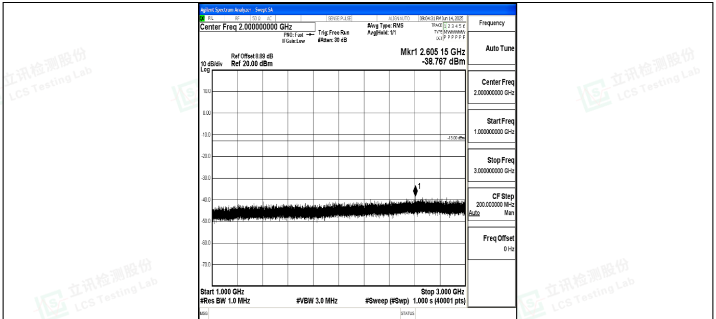
Band5_10MHz_QPSK_20450_1RB#0_1000~3000_1000~3000
