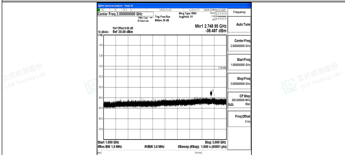
Band5_10MHz_16QAM_20450_1RB#0_1000~3000_1000~3000
