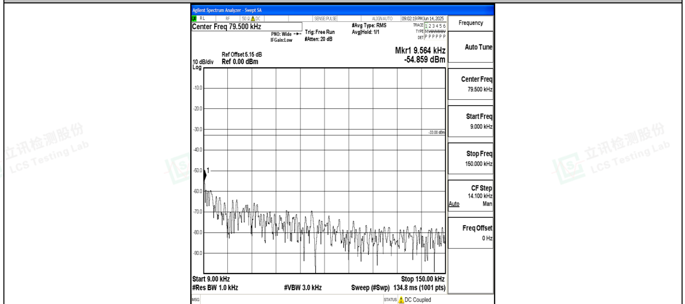
Band5_5MHz_QPSK_20625_1RB#0_0.009~0.15_0.009~0.15
