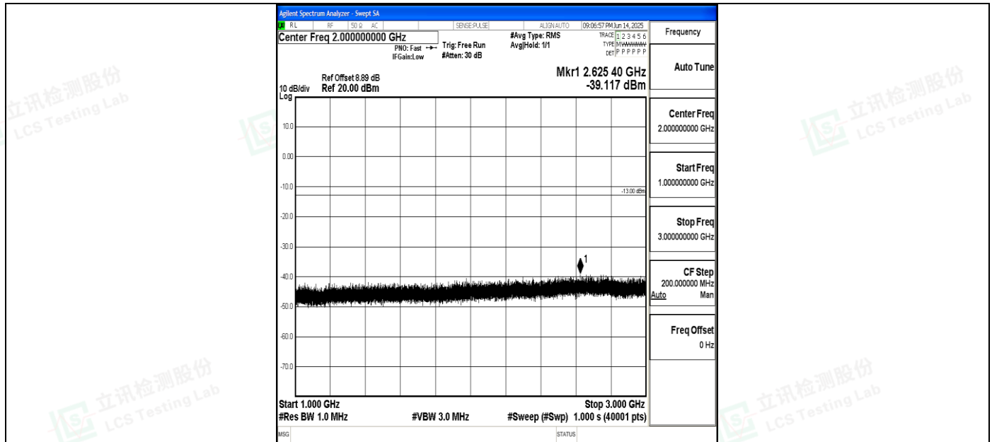
Band5_10MHz_QPSK_20600_1RB#0_1000~3000_1000~3000
