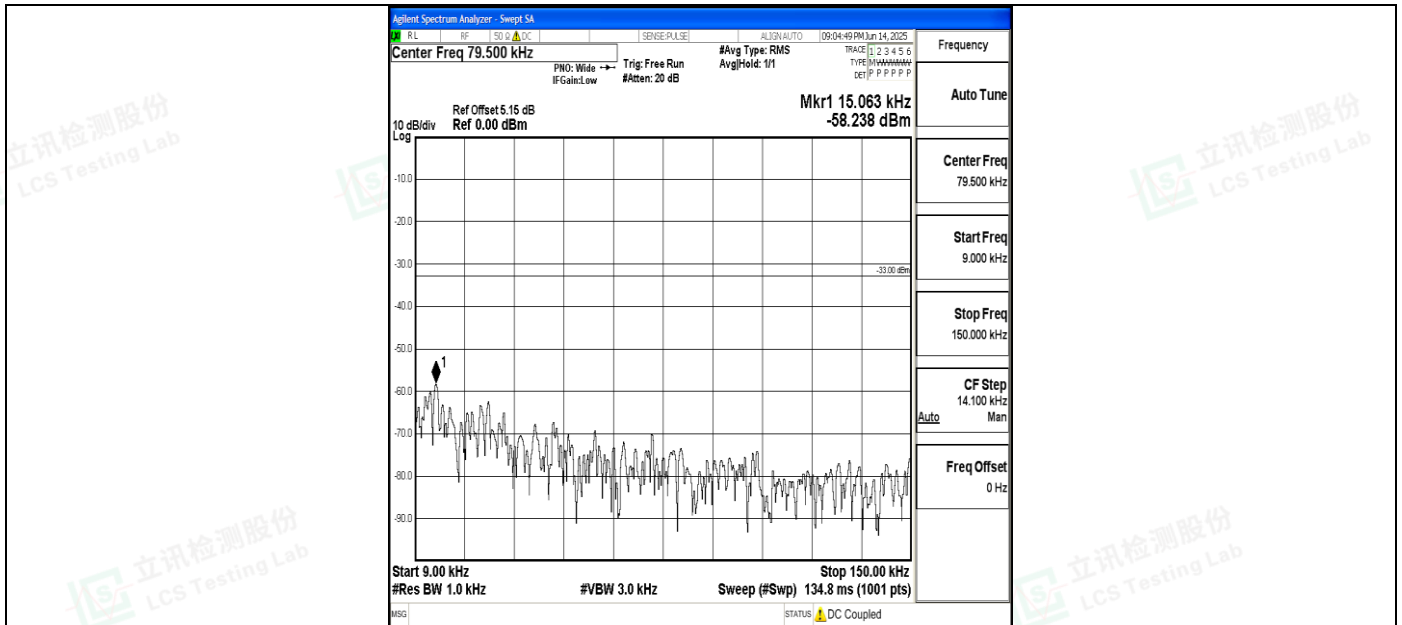
Band5_10MHz_16QAM_20450_1RB#0_0.009~0.15_0.009~0.15
