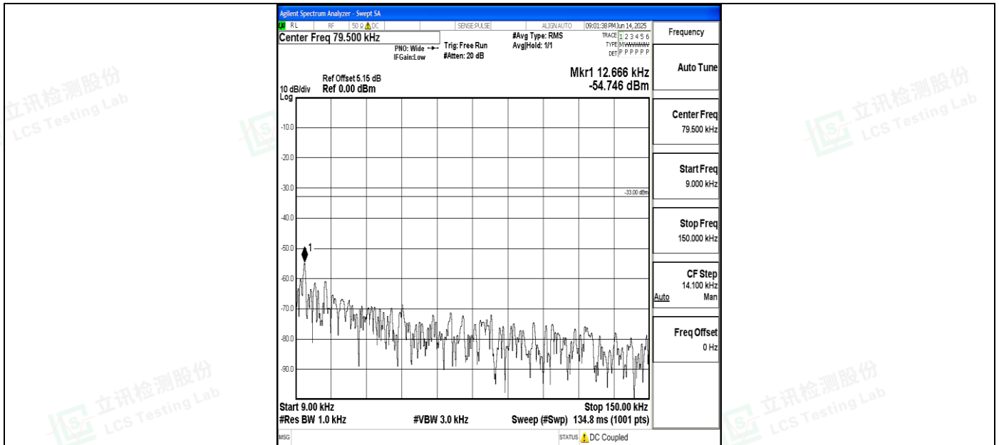
Band5_5MHz_16QAM_20525_1RB#0_0.009~0.15_0.009~0.15
