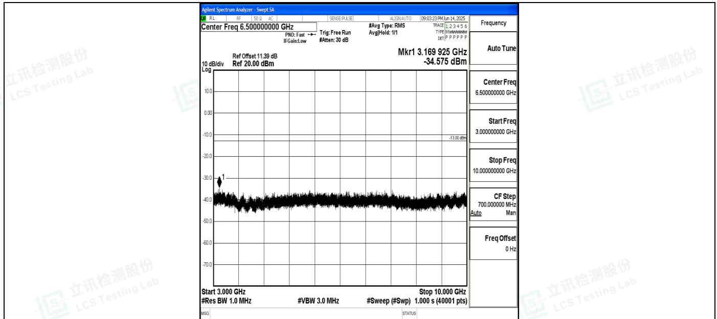
Band5_5MHz_16QAM_20625_1RB#0_3000~10000_3000~10000
