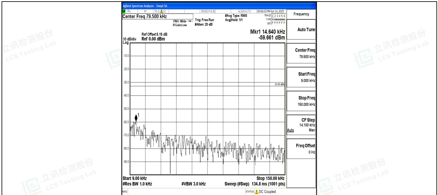
Band5_10MHz_16QAM_20525_1RB#0_0.009~0.15_0.009~0.15
