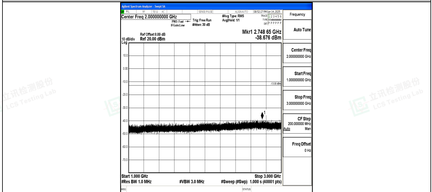
Band5_1.4MHz_QPSK_20525_1RB#0_1000~3000_1000~3000
