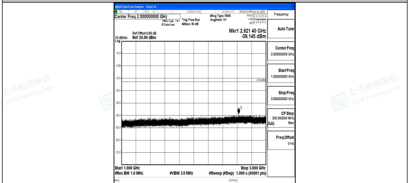
Band5_5MHz_16QAM_20525_1RB#0_1000~3000_1000~3000
