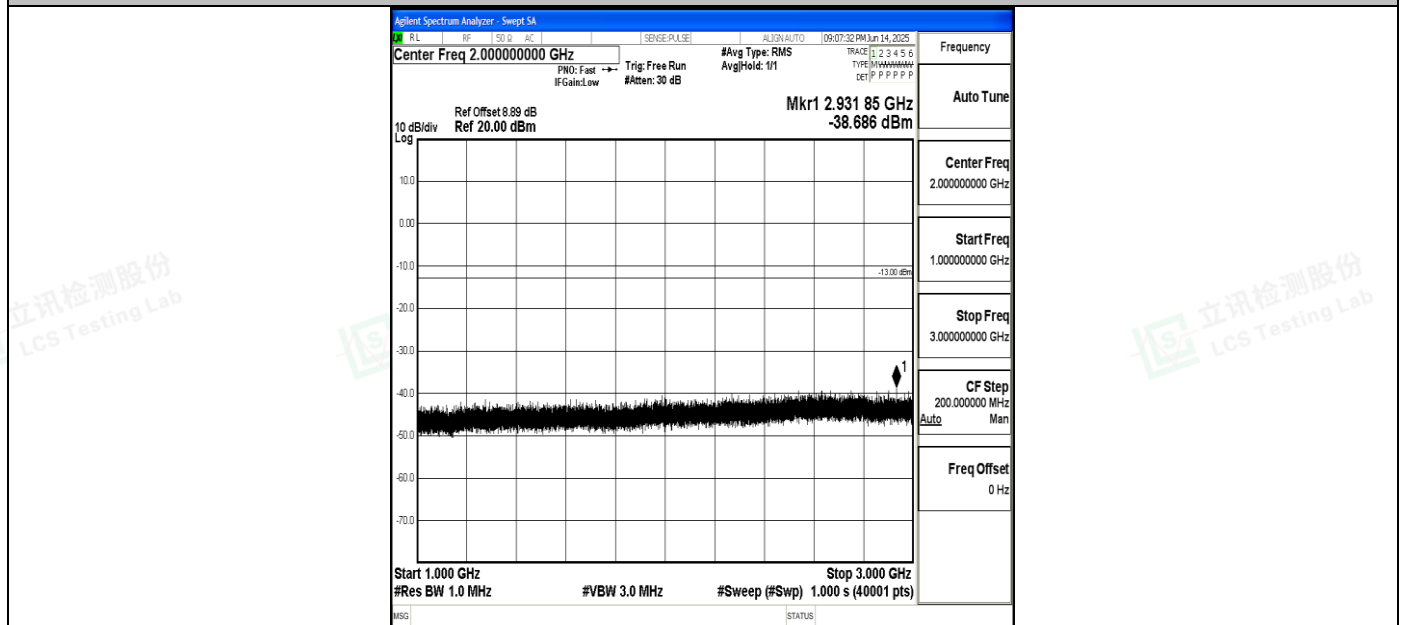
Band5_10MHz_16QAM_20600_1RB#0_1000~3000_1000~3000
