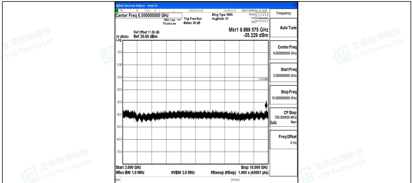
Band5_10MHz_16QAM_20600_1RB#0_3000~10000_3000~10000
