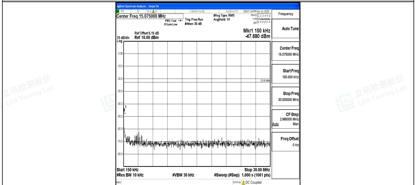
Band5_10MHz_16QAM_20600_1RB#0_0.15~30_0.15~30
