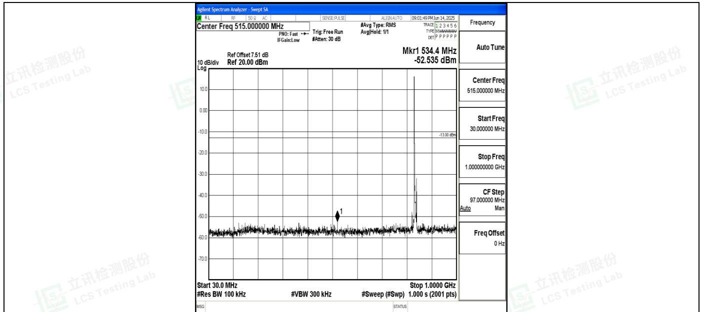
Band5_5MHz_16QAM_20525_1RB#0_30~1000_30~1000
