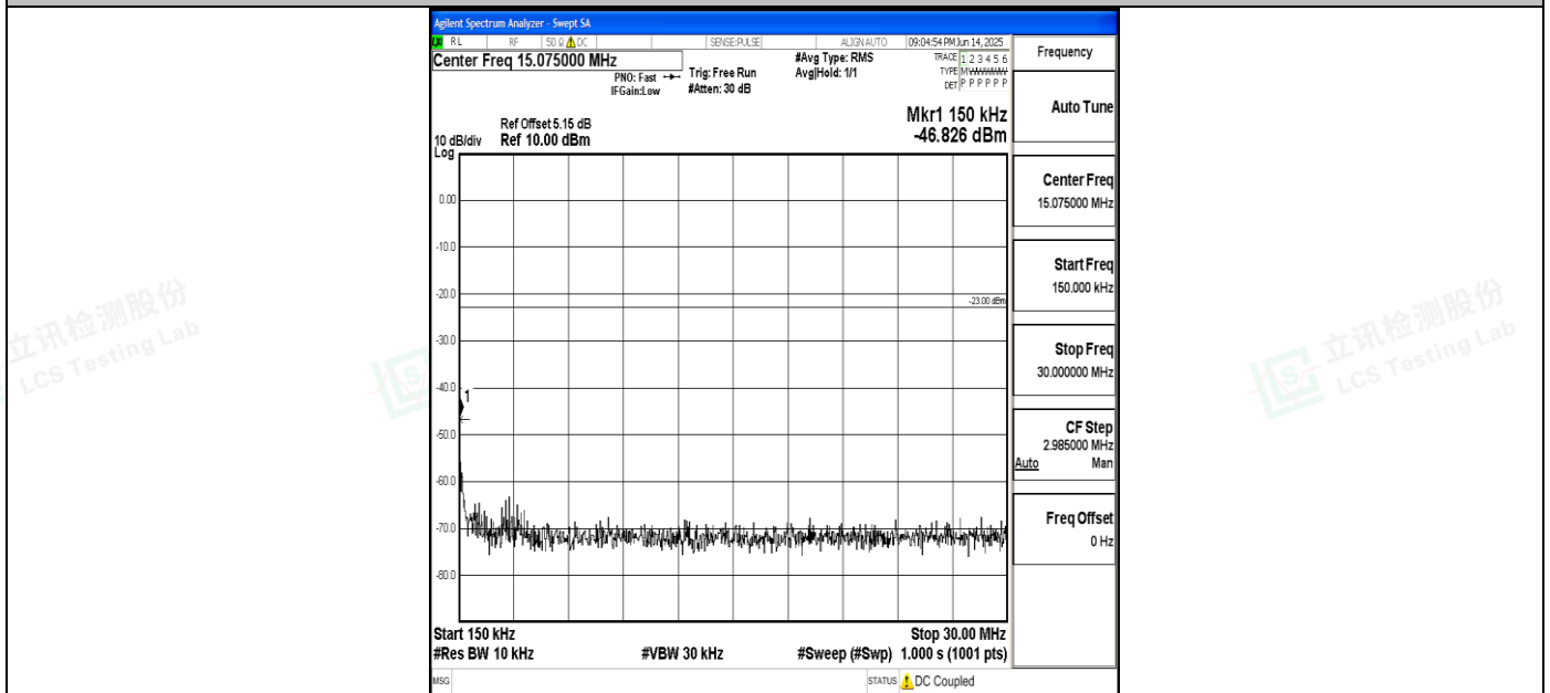
Band5_10MHz_16QAM_20450_1RB#0_0.15~30_0.15~30
