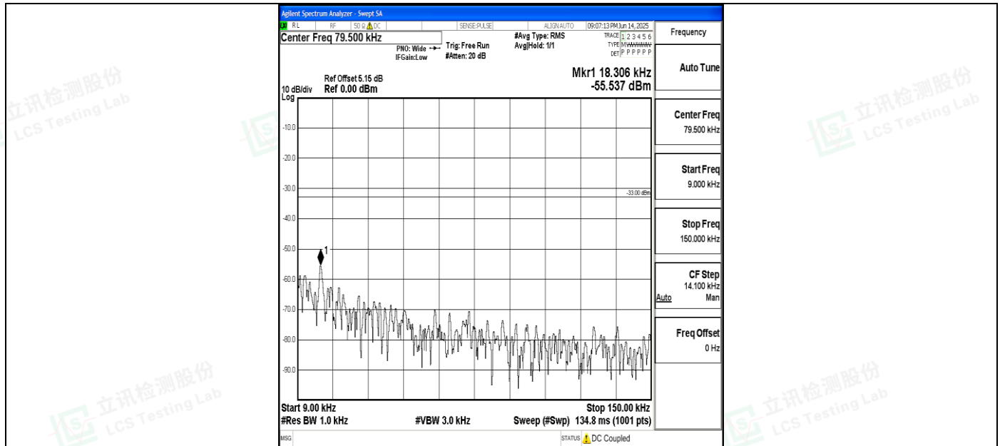
Band5_10MHz_16QAM_20600_1RB#0_0.009~0.15_0.009~0.15
