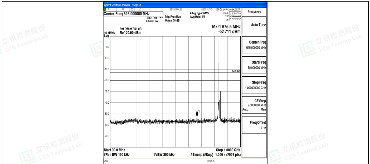
Band5_10MHz_16QAM_20525_1RB#0_30~1000_30~1000
