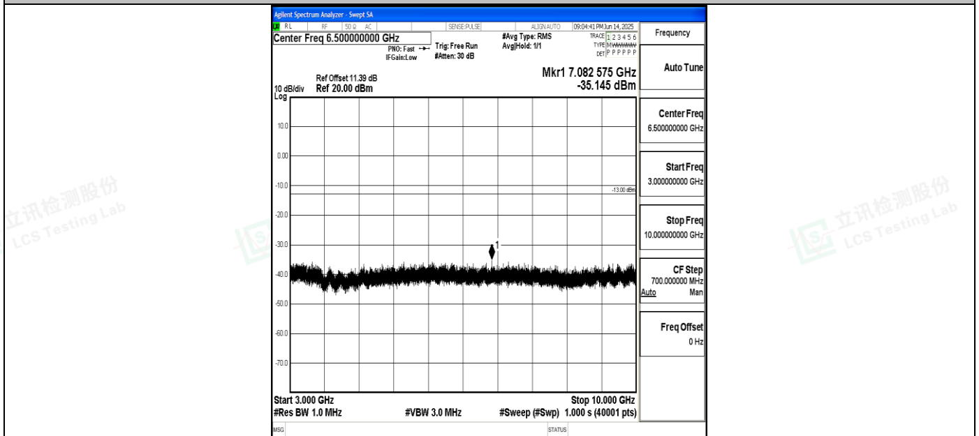
Band5_10MHz_QPSK_20450_1RB#0_3000~10000_3000~10000
