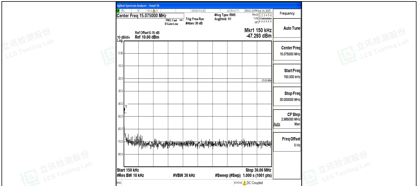
Band5_5MHz_QPSK_20525_1RB#0_0.15~30_0.15~30
