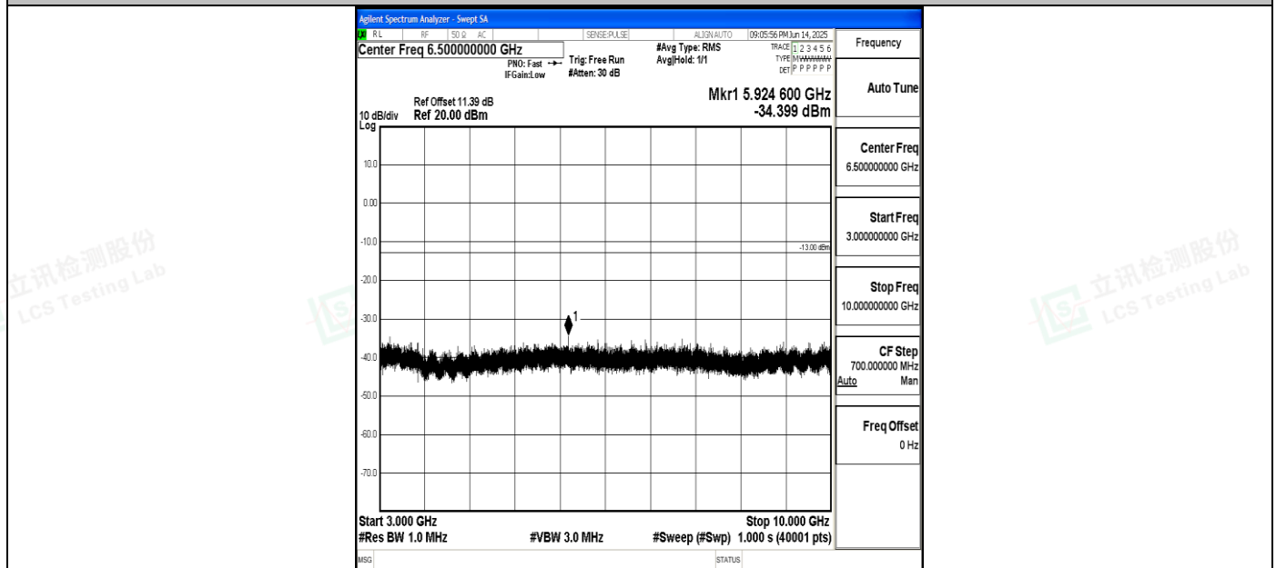
Band5_10MHz_QPSK_20525_1RB#0_3000~10000_3000~10000
