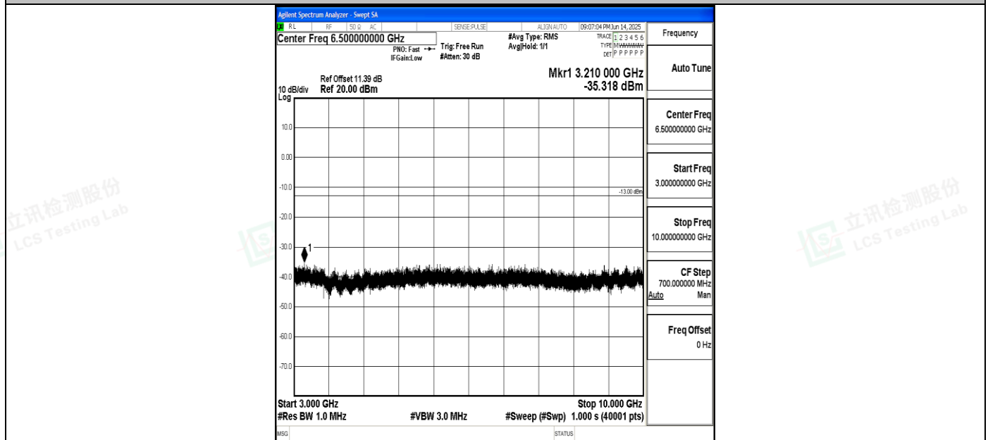
Band5_10MHz_QPSK_20600_1RB#0_3000~10000_3000~10000
