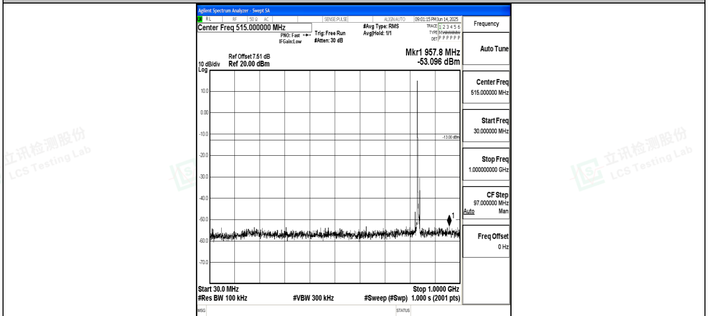
Band5_5MHz_QPSK_20525_1RB#0_30~1000_30~1000
