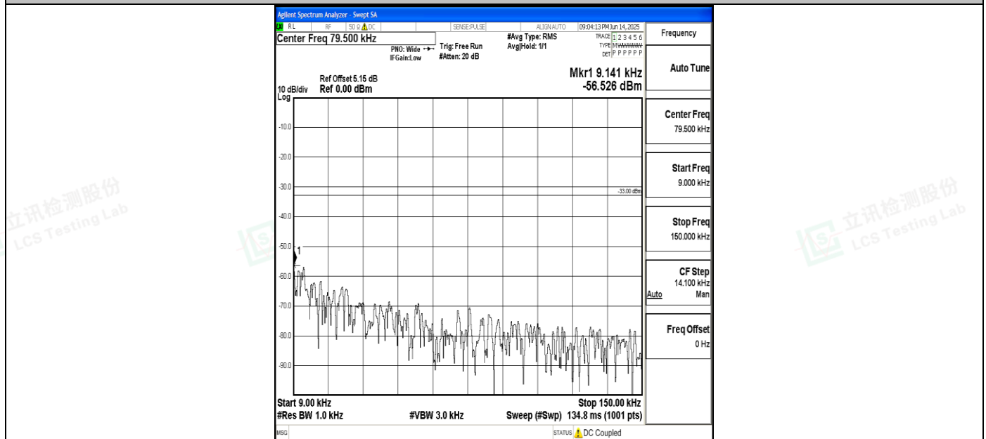
Band5_10MHz_QPSK_20450_1RB#0_0.009~0.15_0.009~0.15
