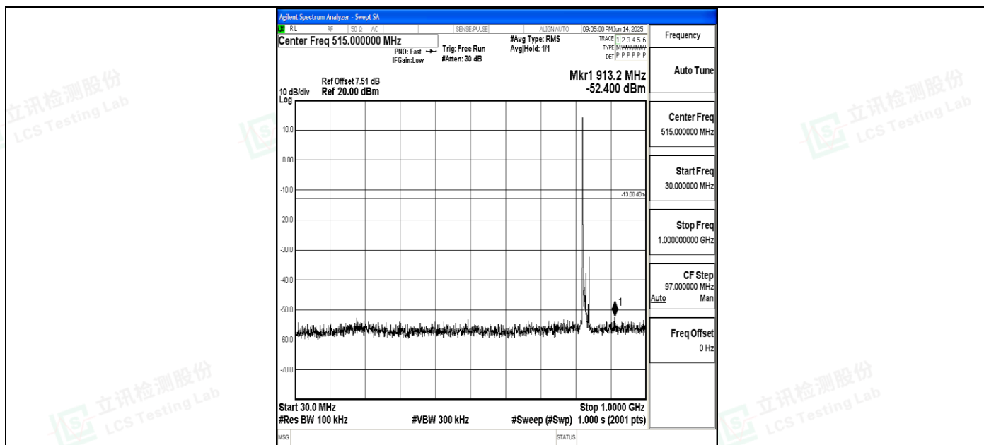
Band5_10MHz_16QAM_20450_1RB#0_30~1000_30~1000
