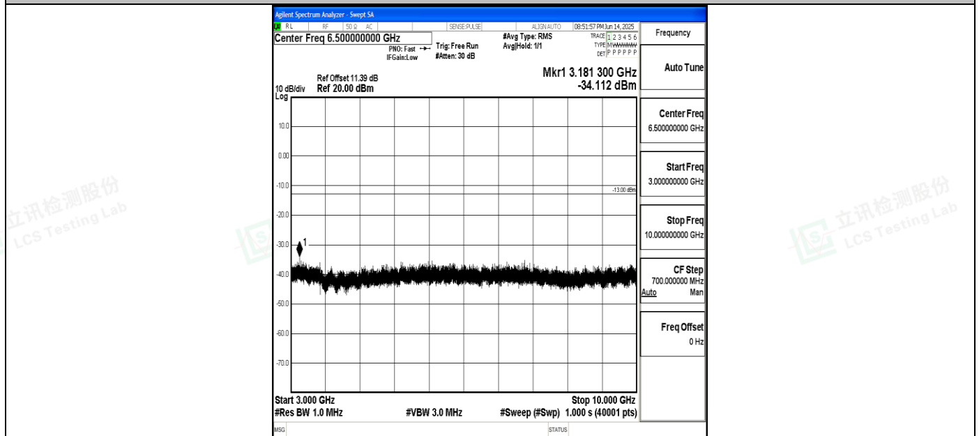
Band5_1.4MHz_16QAM_20407_1RB#0_3000~10000_3000~10000
