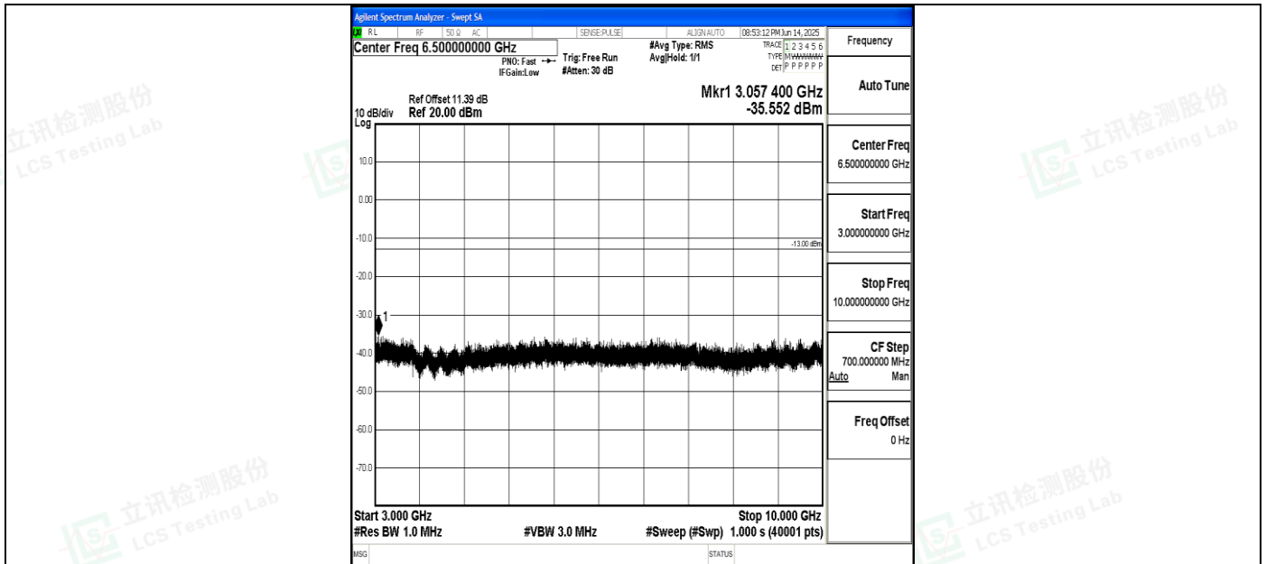
Band5_1.4MHz_16QAM_20525_1RB#0_3000~10000_3000~10000
