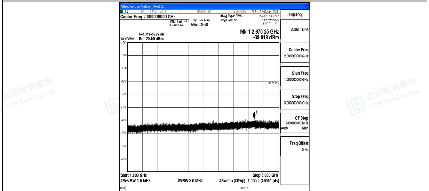
Band5_1.4MHz_QPSK_20407_1RB#0_1000~3000_1000~3000
