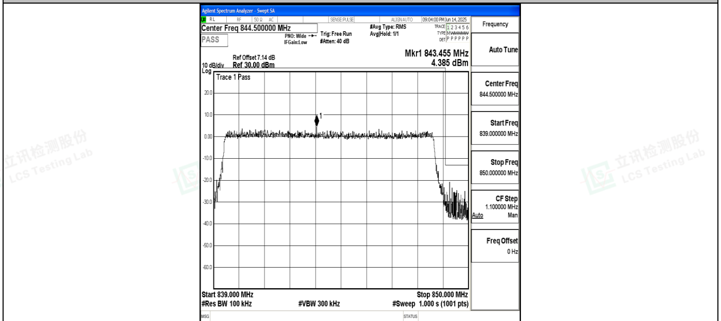
Band5_10MHz_16QAM_20600_50RB#0
