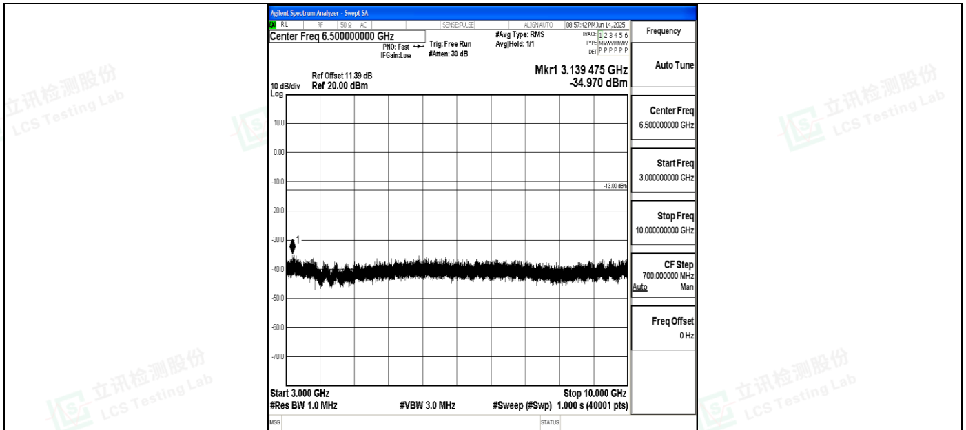
Band5_3MHz_16QAM_20525_1RB#0_3000~10000_3000~10000
