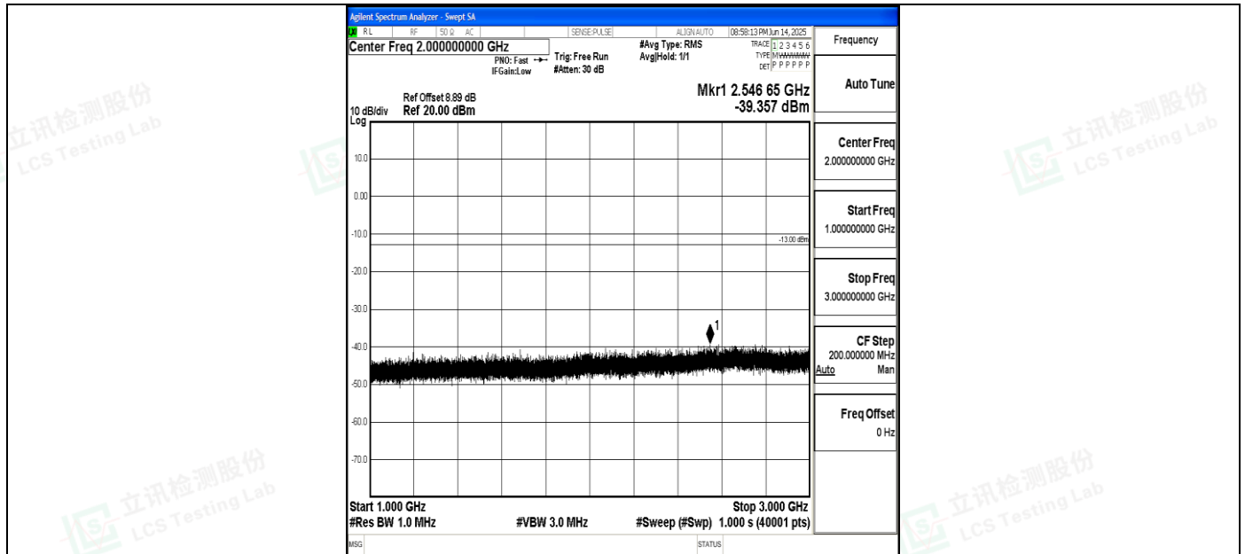
Band5_3MHz_QPSK_20635_1RB#0_1000~3000_1000~3000
