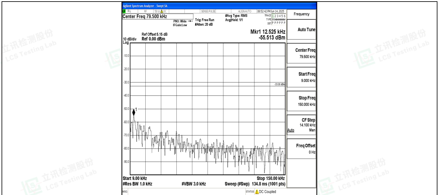
Band5_1.4MHz_16QAM_20525_1RB#0_0.009~0.15_0.009~0.15
