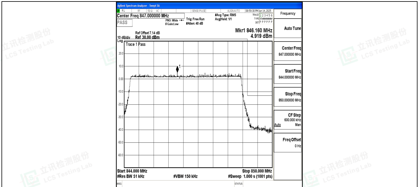
Band5_5MHz_QPSK_20625_25RB#0
