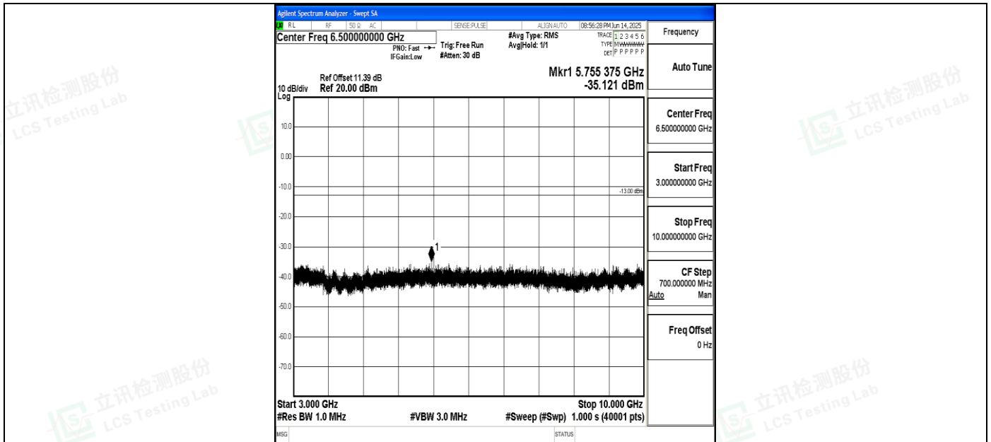
Band5_3MHz_16QAM_20415_1RB#0_3000~10000_3000~10000
