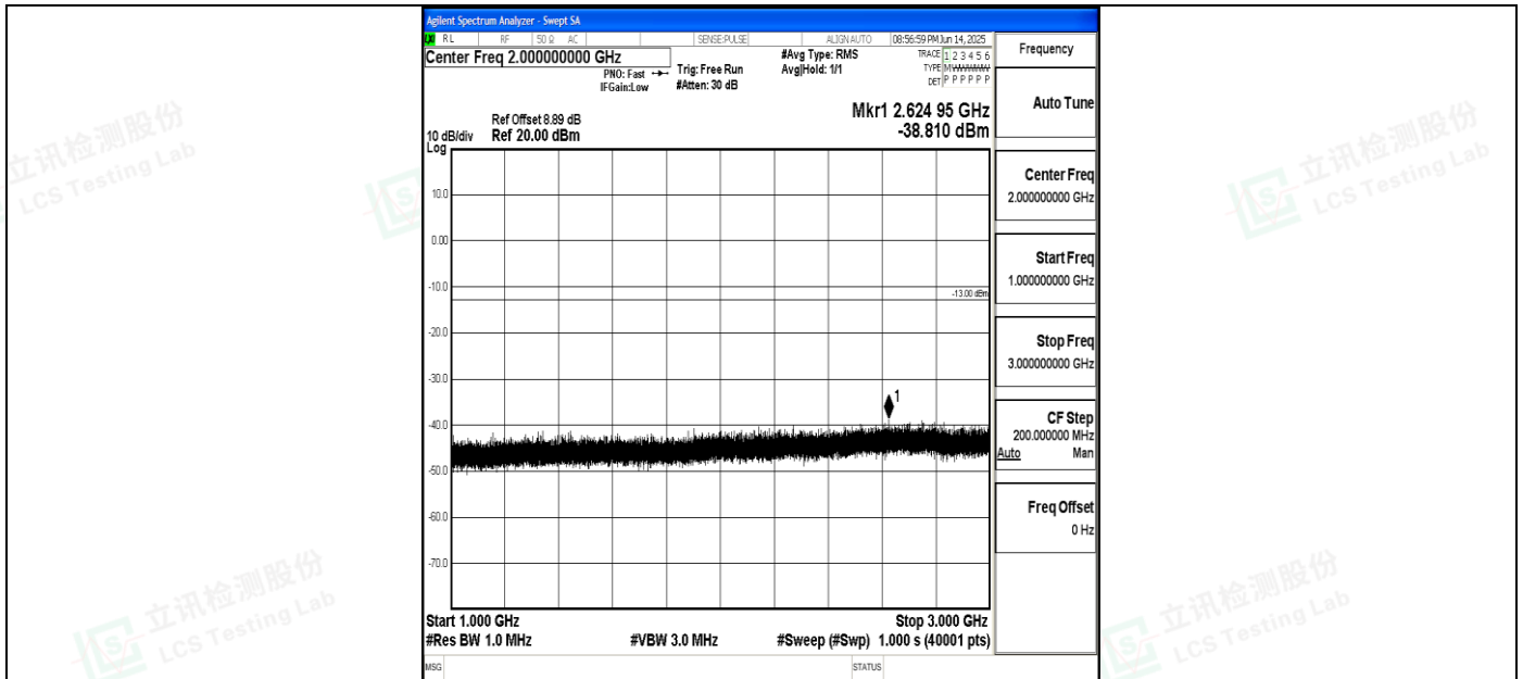
Band5_3MHz_QPSK_20525_1RB#0_1000~3000_1000~3000
