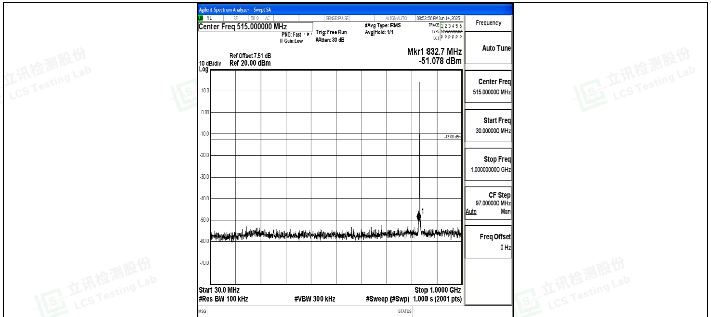
Band5_1.4MHz_16QAM_20525_1RB#0_30~1000_30~1000
