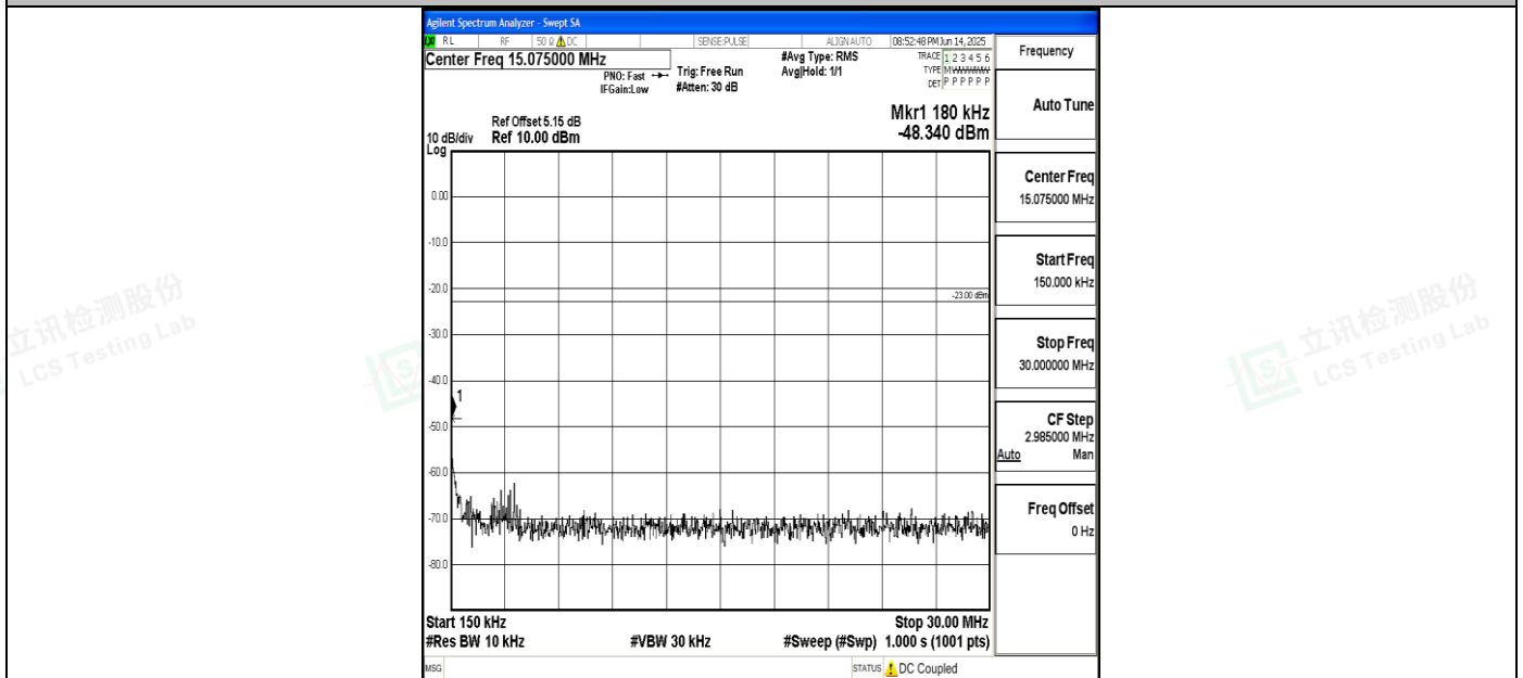
Band5_1.4MHz_16QAM_20525_1RB#0_0.15~30_0.15~30
