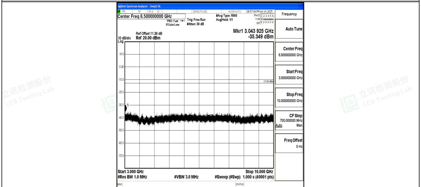
Band5_3MHz_QPSK_20525_1RB#0_3000~10000_3000~10000
