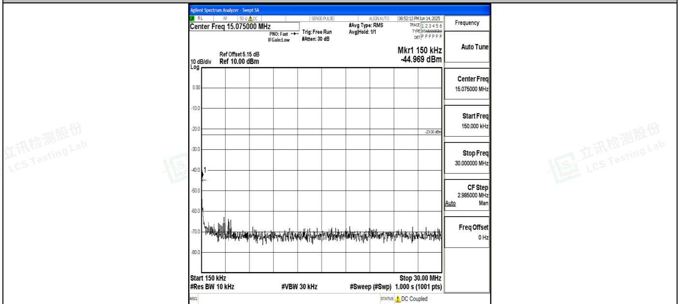
Band5_1.4MHz_QPSK_20525_1RB#0_0.15~30_0.15~30
