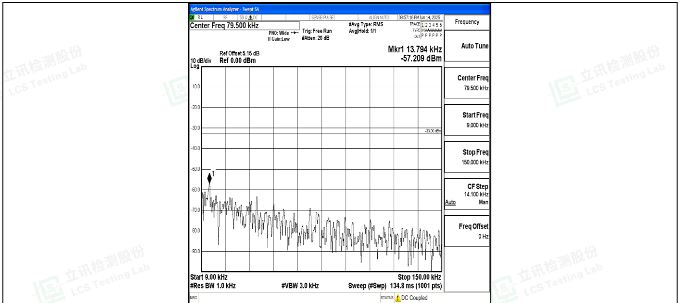
Band5_3MHz_16QAM_20525_1RB#0_0.009~0.15_0.009~0.15
