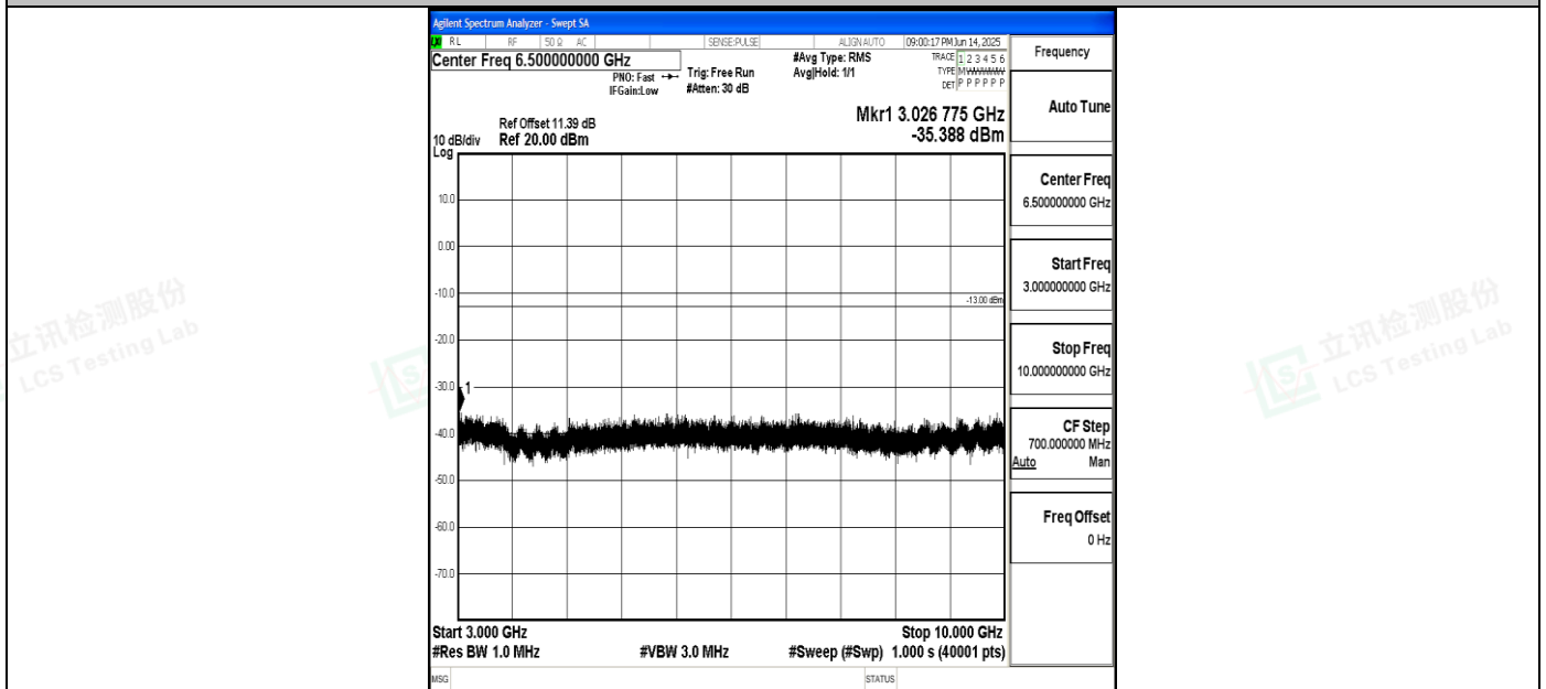
Band5_5MHz_QPSK_20425_1RB#0_3000~10000_3000~10000
