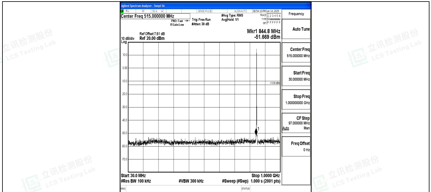
Band5_1.4MHz_16QAM_20643_1RB#0_30~1000_30~1000
