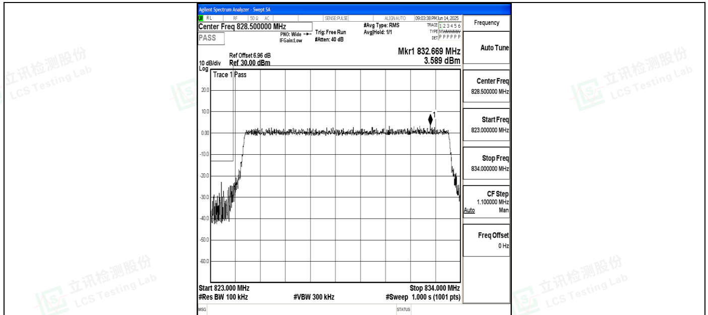
Band5_10MHz_QPSK_20450_50RB#0
