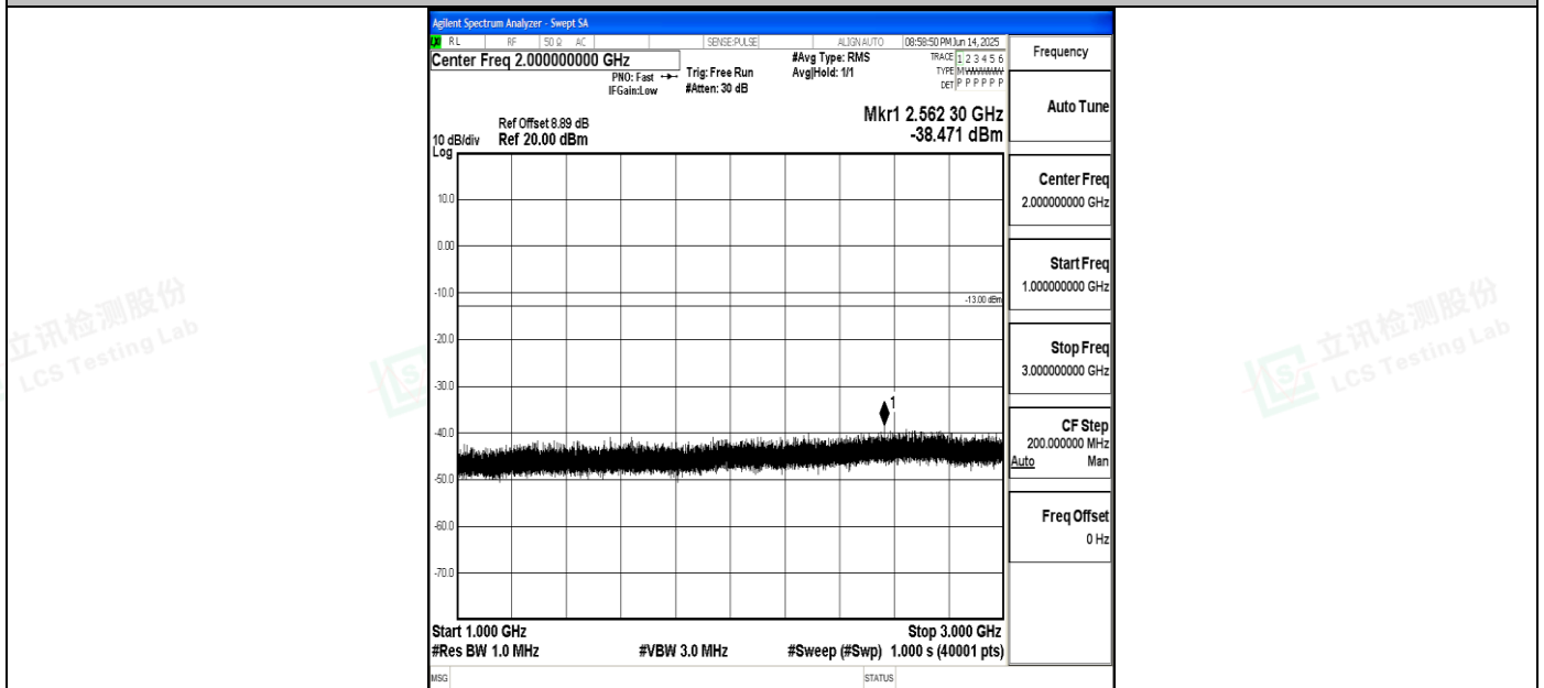
Band5_3MHz_16QAM_20635_1RB#0_1000~3000_1000~3000
