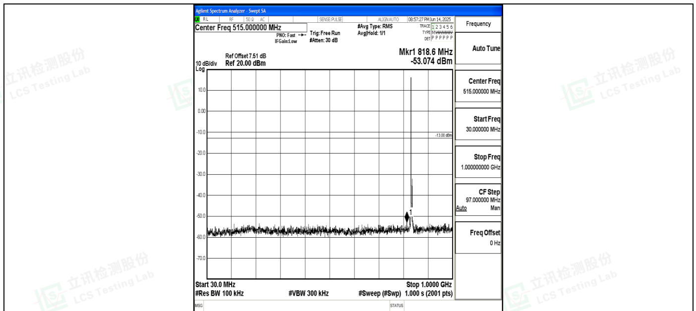
Band5_3MHz_16QAM_20525_1RB#0_30~1000_30~1000
