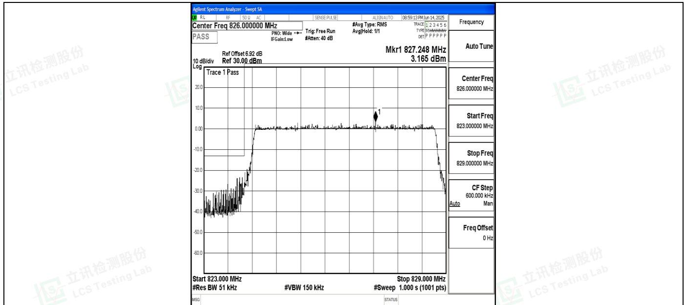
Band5_5MHz_QPSK_20425_25RB#0
