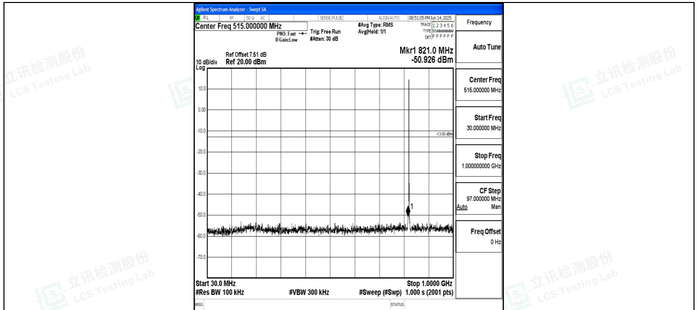
Band5_1.4MHz_QPSK_20407_1RB#0_30~1000_30~1000
