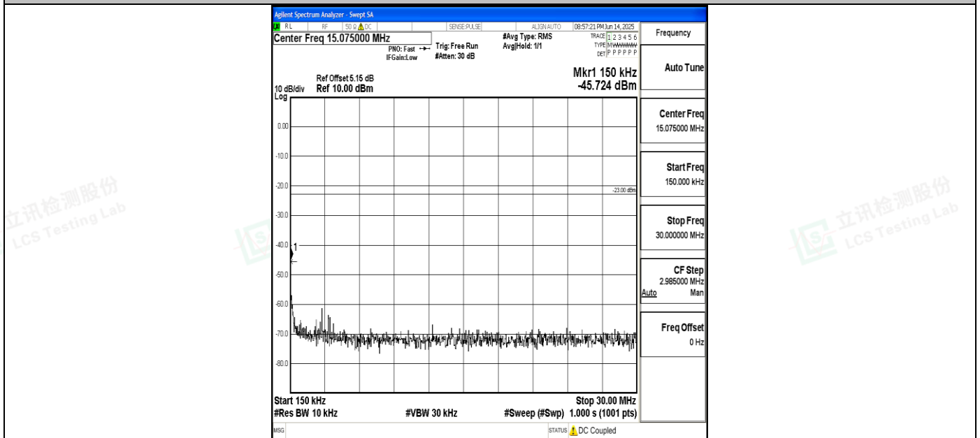
Band5_3MHz_16QAM_20525_1RB#0_0.15~30_0.15~30
