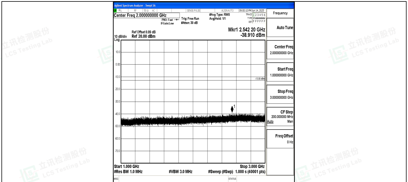
Band5_5MHz_QPSK_20425_1RB#0_1000~3000_1000~3000
