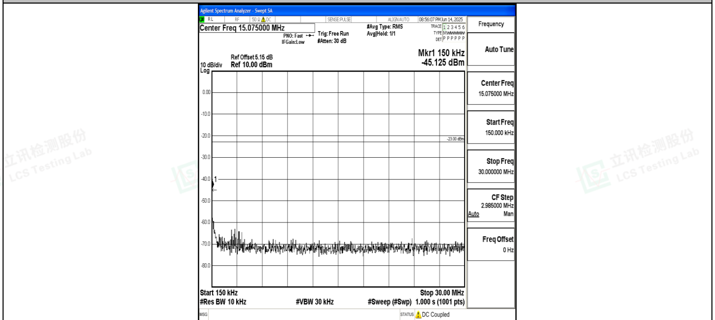
Band5_3MHz_16QAM_20415_1RB#0_0.15~30_0.15~30
