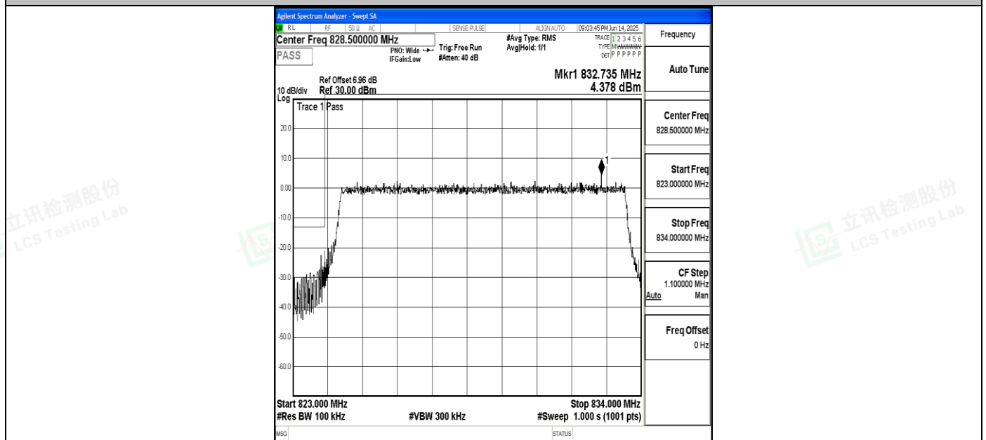
Band5_10MHz_16QAM_20450_50RB#0
