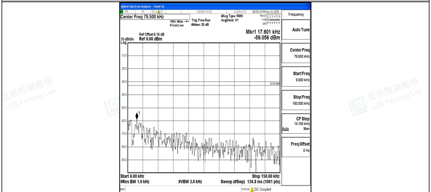
Band5_1.4MHz_QPSK_20643_1RB#0_0.009~0.15_0.009~0.15
