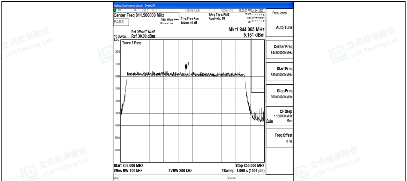
Band5_10MHz_QPSK_20600_50RB#0
