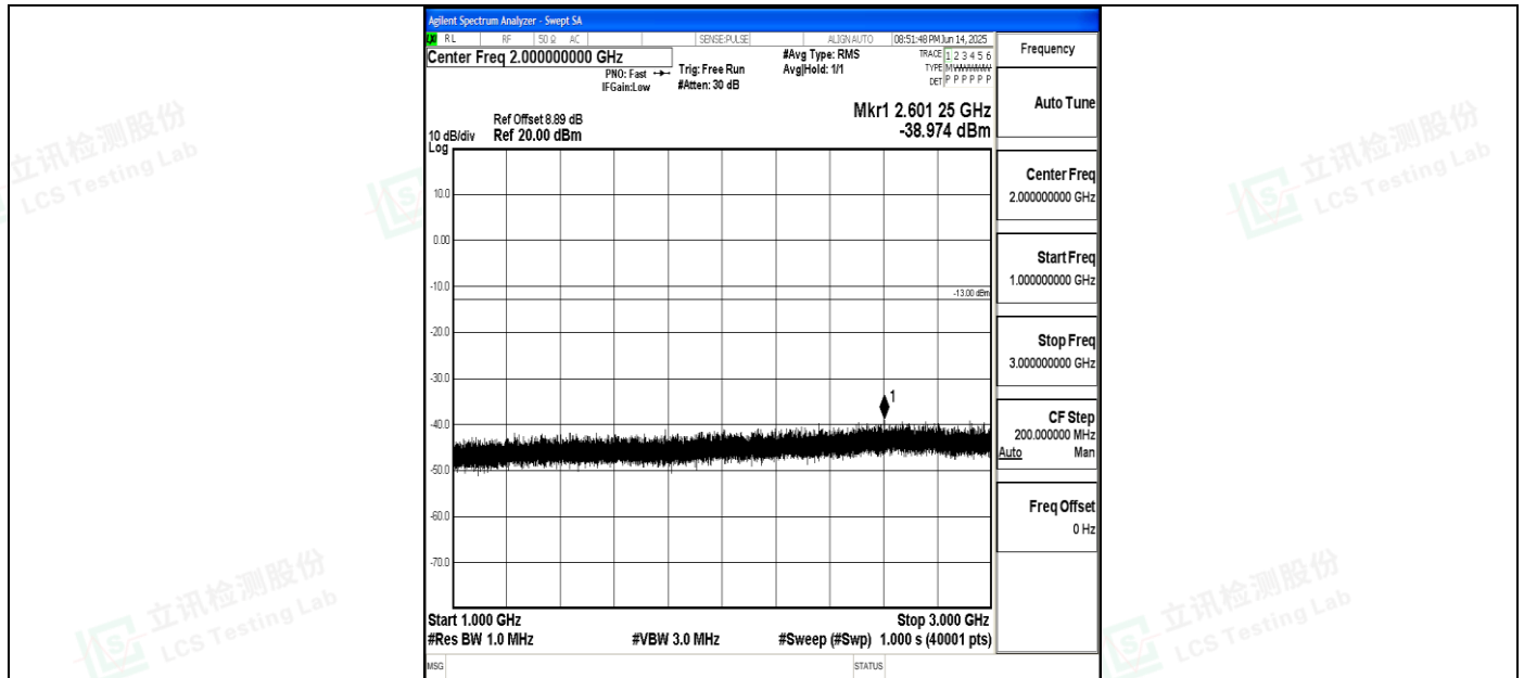
Band5_1.4MHz_16QAM_20407_1RB#0_1000~3000_1000~3000
