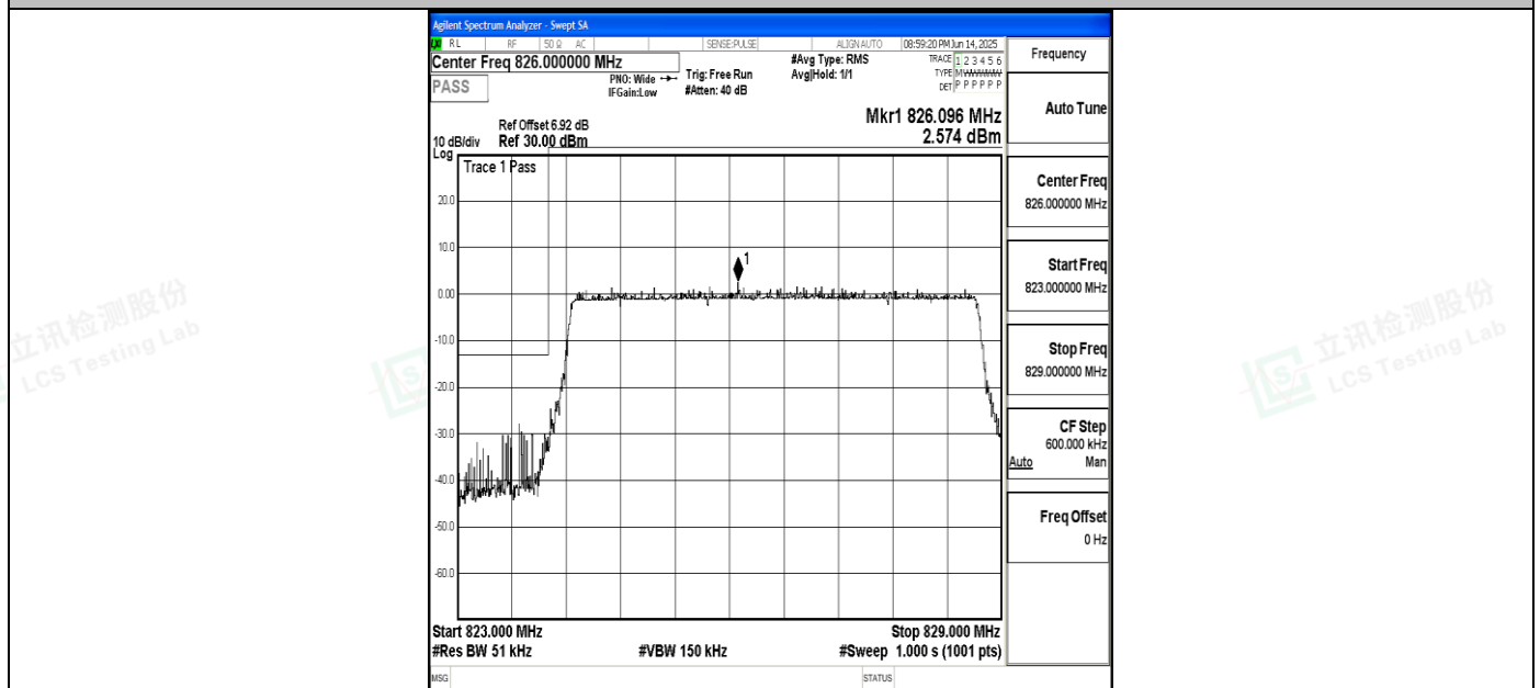
Band5_5MHz_16QAM_20425_25RB#0
