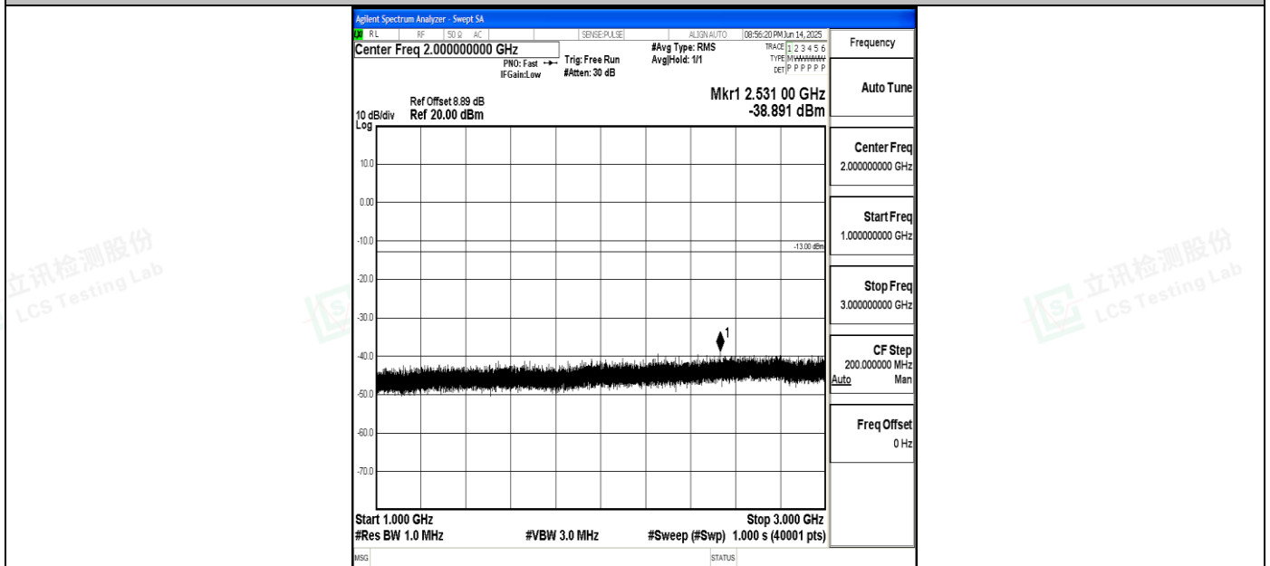
Band5_3MHz_16QAM_20415_1RB#0_1000~3000_1000~3000
