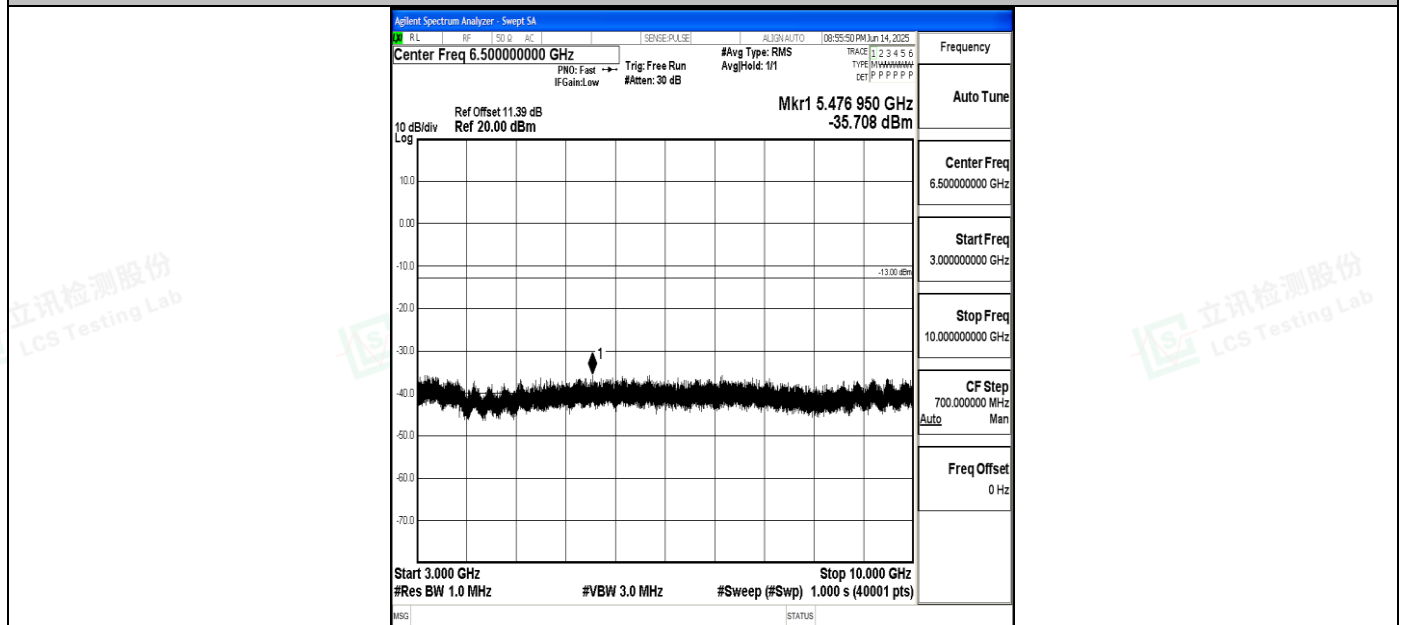
Band5_3MHz_QPSK_20415_1RB#0_3000~10000_3000~10000
