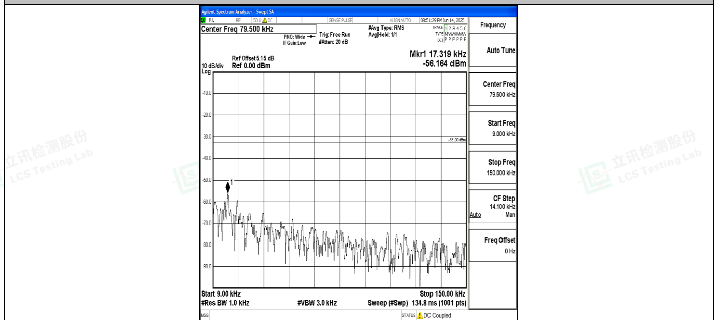
Band5_1.4MHz_16QAM_20407_1RB#0_0.009~0.15_0.009~0.15
