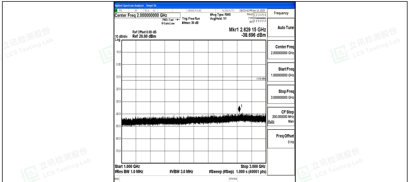
Band5_1.4MHz_QPSK_20643_1RB#0_1000~3000_1000~3000
