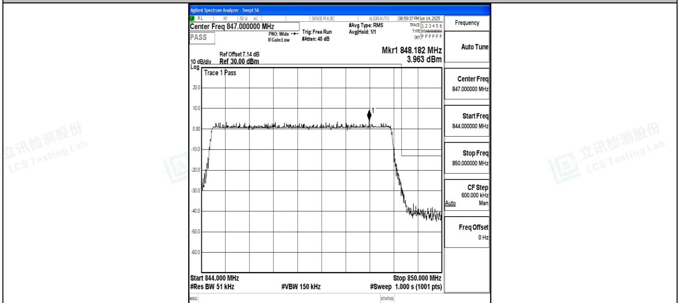
Band5_5MHz_16QAM_20625_25RB#0
