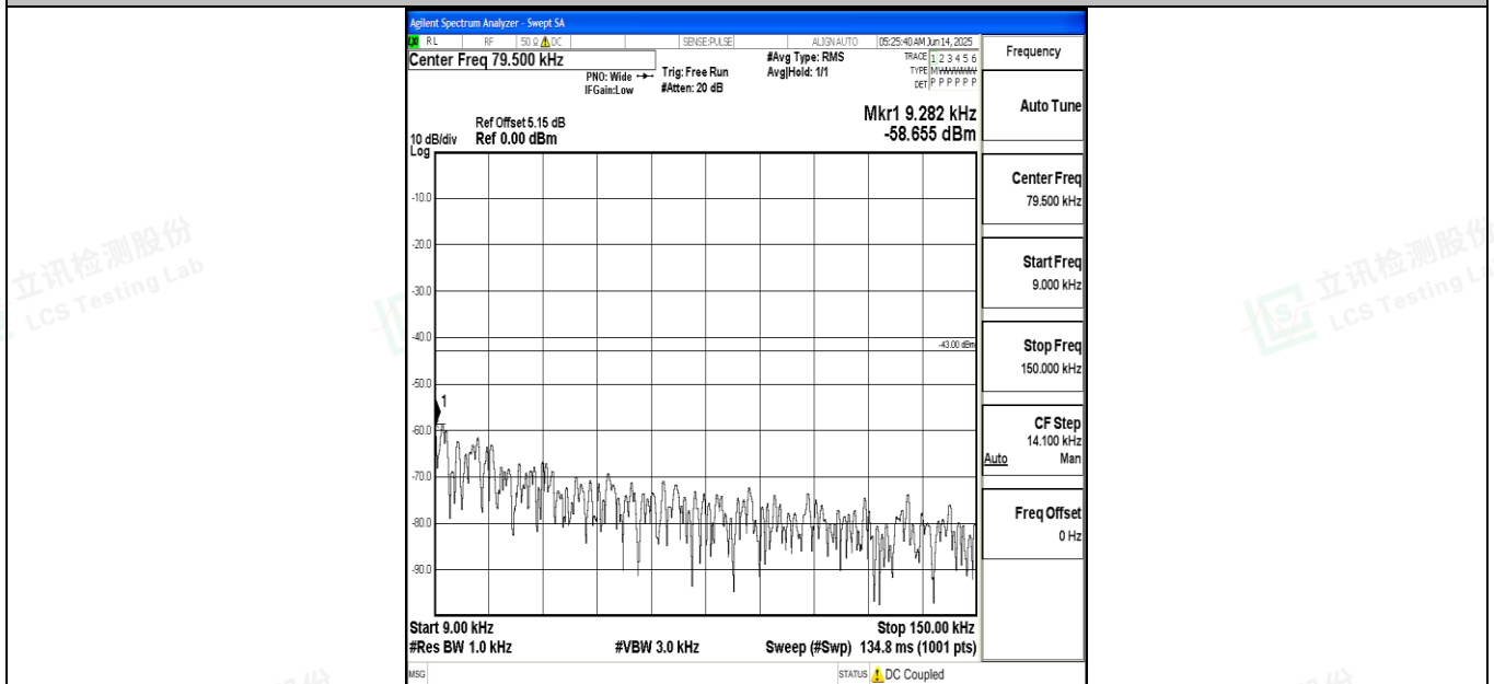
Band4_20MHz_16QAM_20300_1RB#0_0.009~0.15_0.009~0.15
