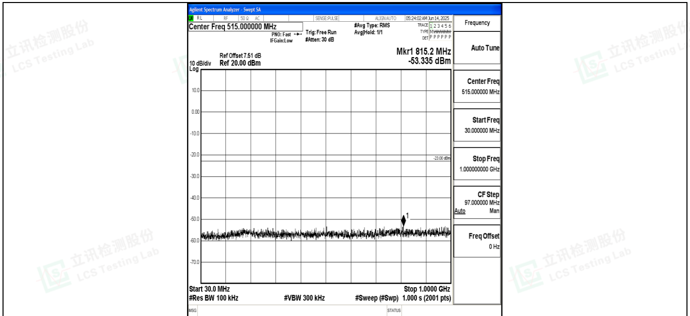
Band4_20MHz_QPSK_20175_1RB#0_30~1000_30~1000
