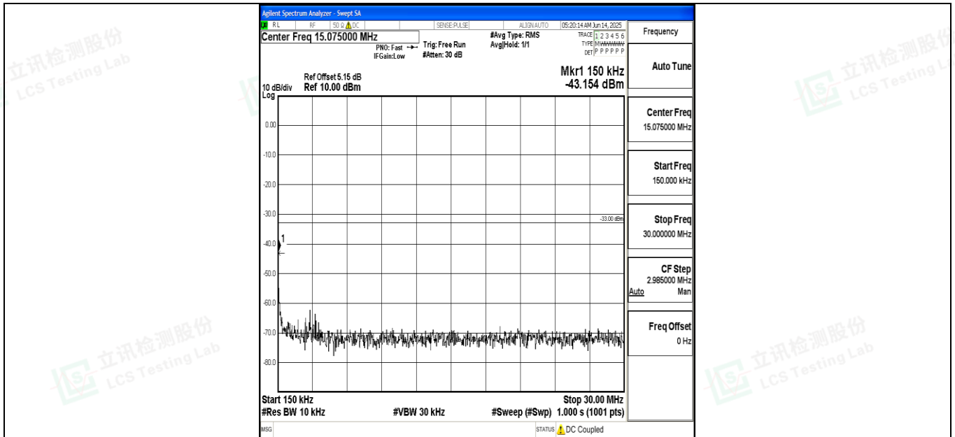
Band4_15MHz_16QAM_20175_1RB#0_0.15~30_0.15~30
