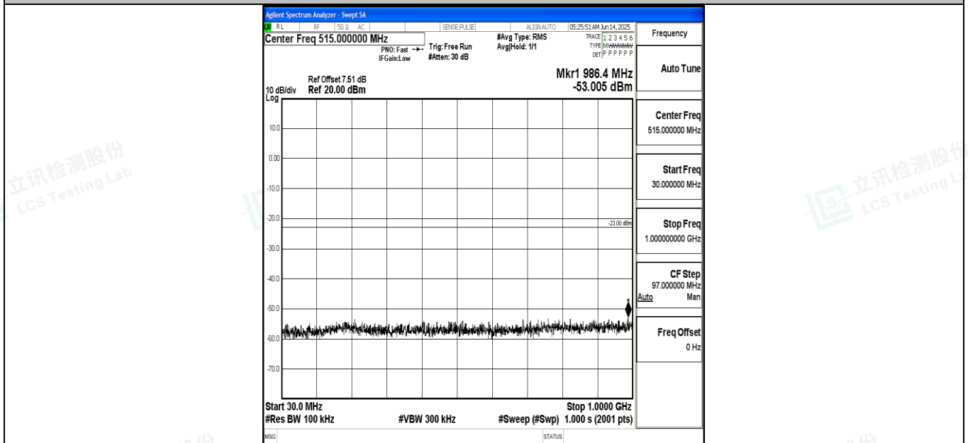
Band4_20MHz_16QAM_20300_1RB#0_30~1000_30~1000
