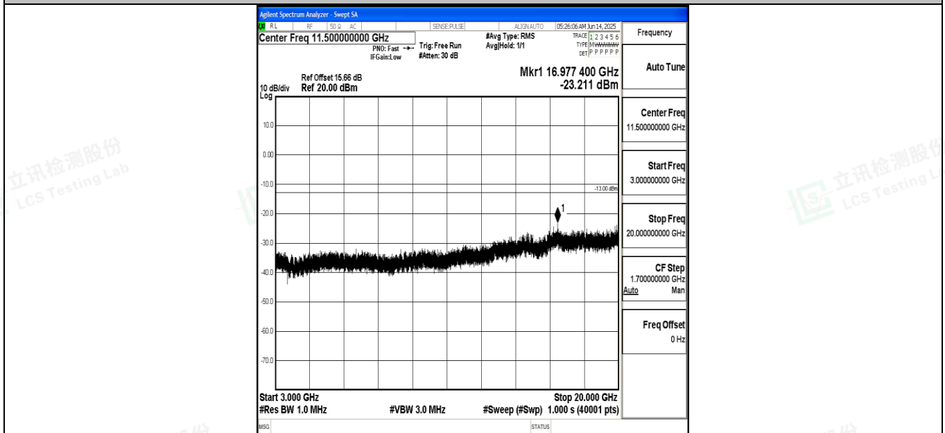
Band4_20MHz_16QAM_20300_1RB#0_3000~20000_3000~20000
