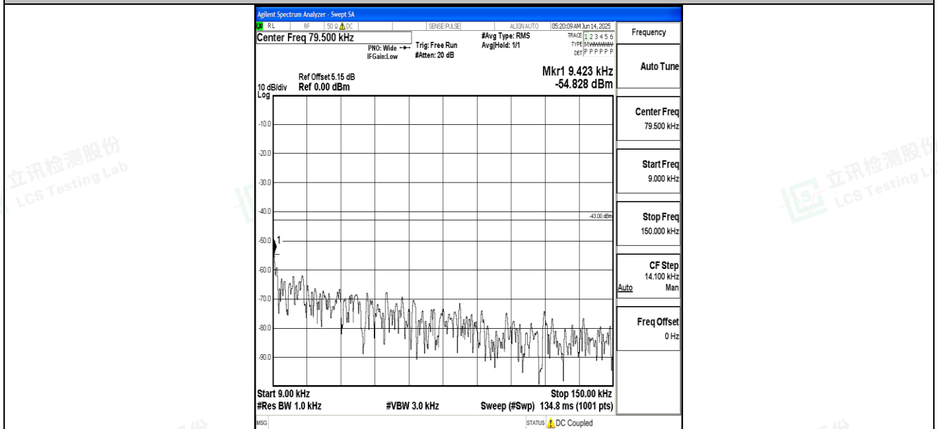
Band4_15MHz_16QAM_20175_1RB#0_0.009~0.15_0.009~0.15
