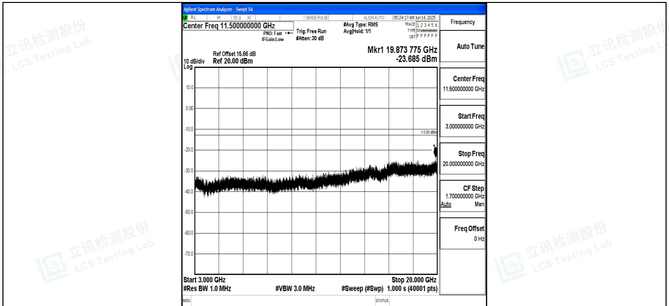
Band4_20MHz_QPSK_20175_1RB#0_3000~20000_3000~20000
