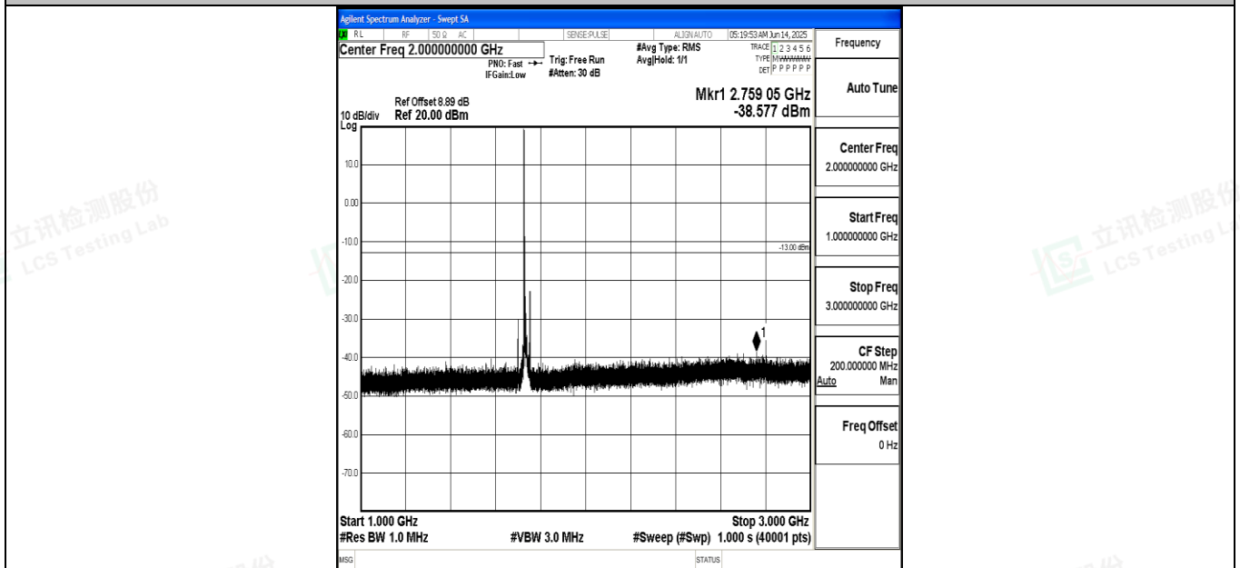
Band4_15MHz_QPSK_20175_1RB#0_1000~3000_1000~3000
