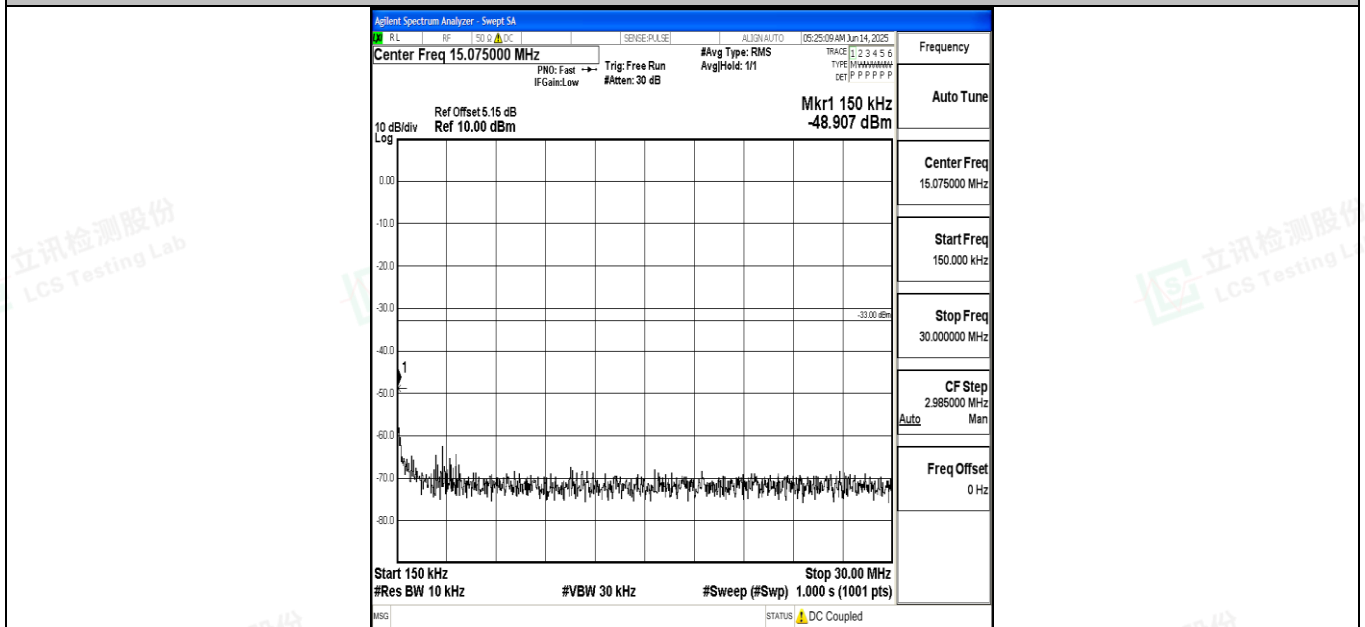
Band4_20MHz_QPSK_20300_1RB#0_0.15~30_0.15~30
