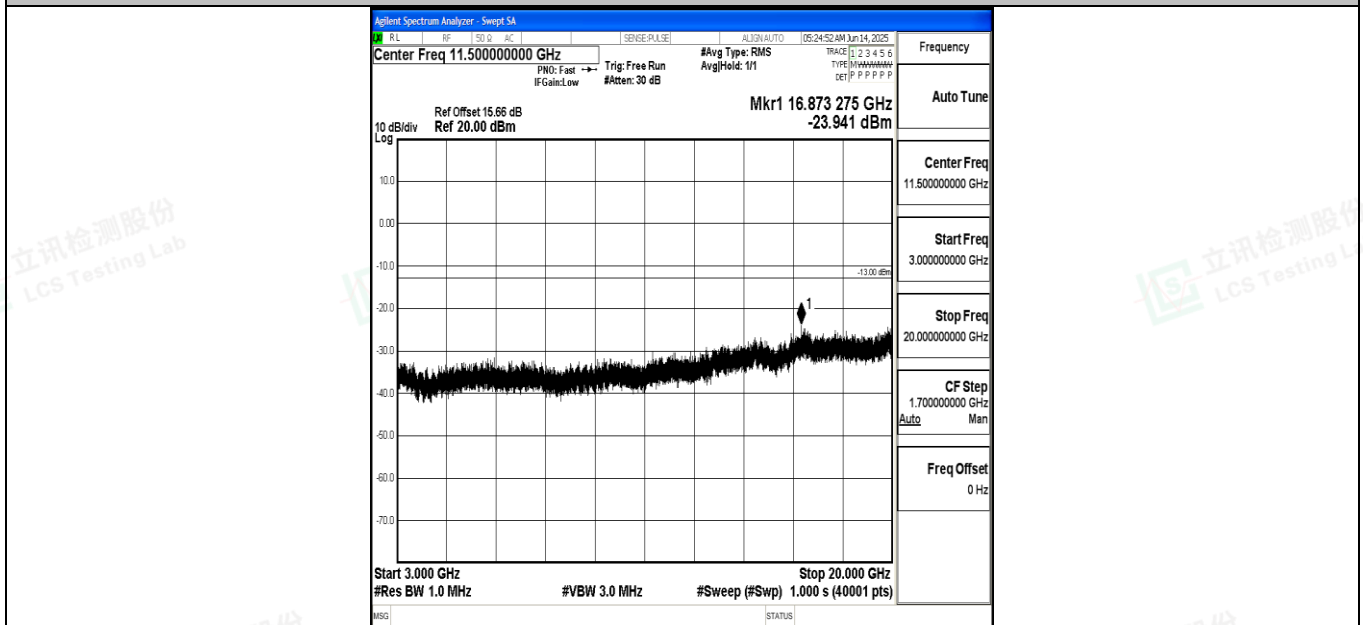
Band4_20MHz_16QAM_20175_1RB#0_3000~20000_3000~20000
