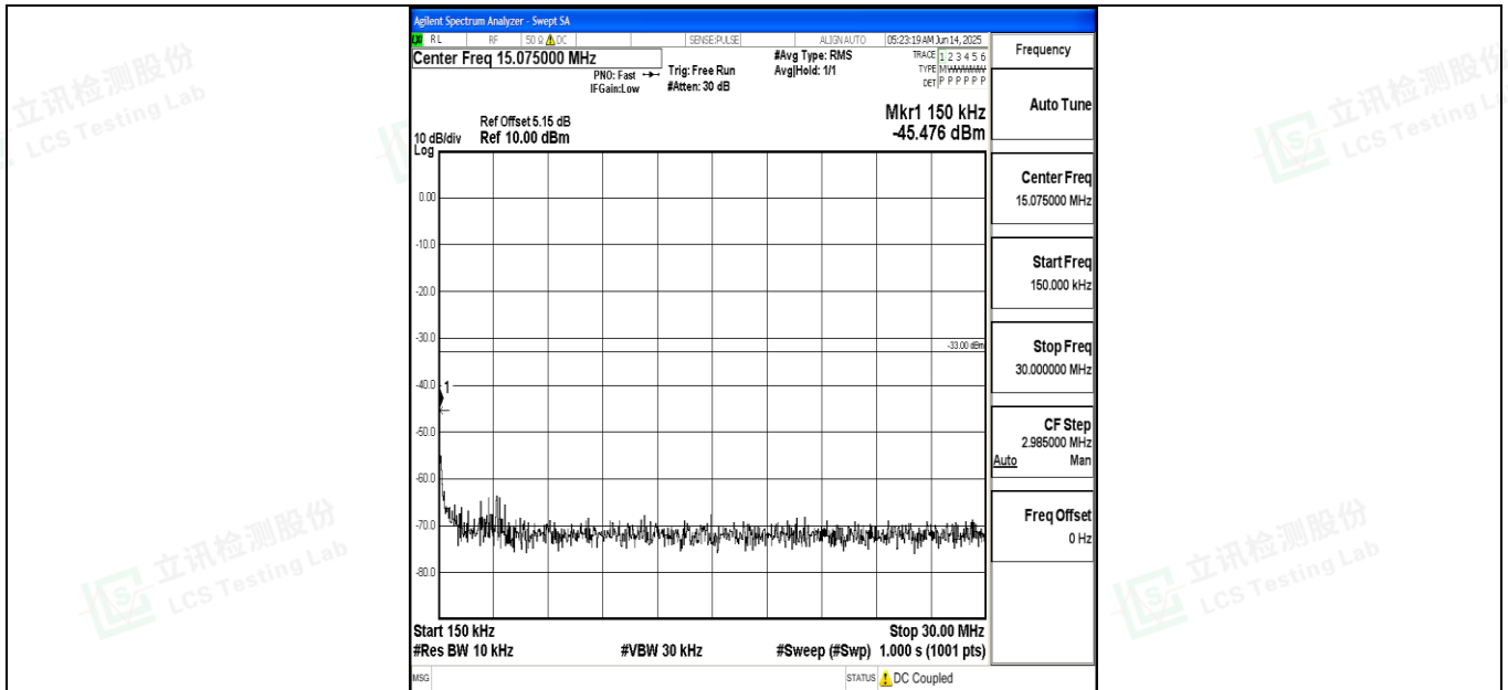
Band4_20MHz_16QAM_20050_1RB#0_0.15~30_0.15~30
