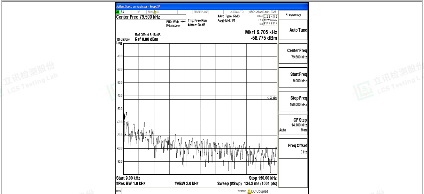
Band4_20MHz_16QAM_20175_1RB#0_0.009~0.15_0.009~0.15
