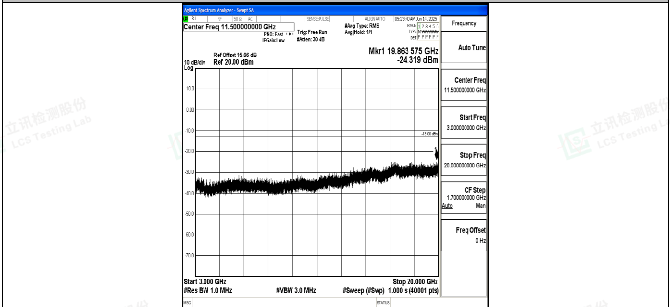
Band4_20MHz_16QAM_20050_1RB#0_3000~20000_3000~20000
