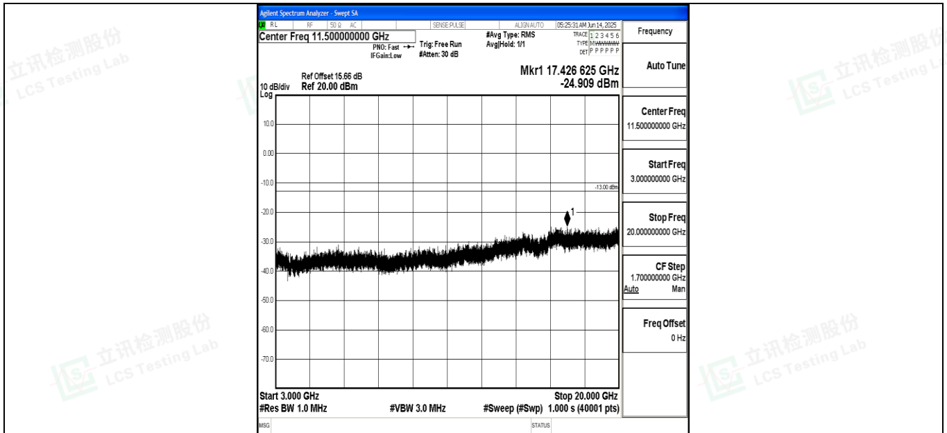
Band4_20MHz_QPSK_20300_1RB#0_3000~20000_3000~20000
