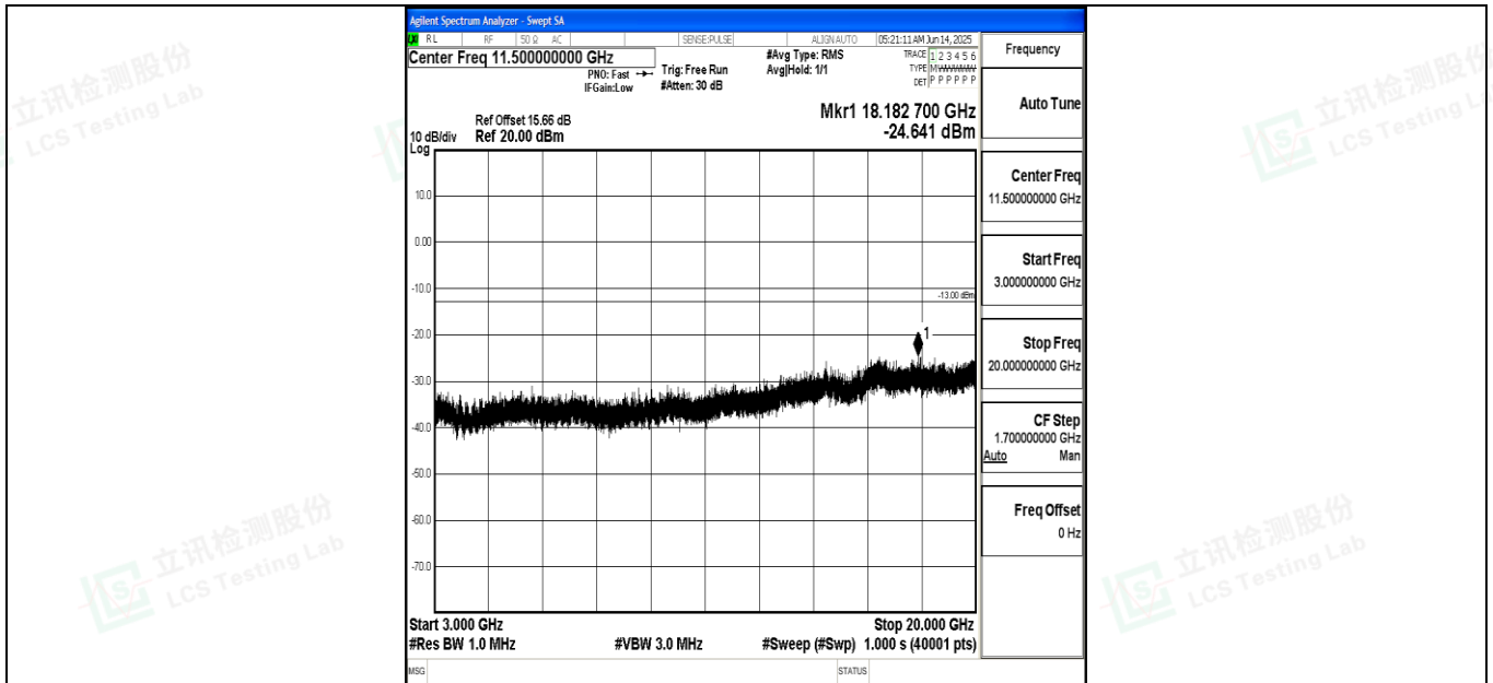
Band4_15MHz_QPSK_20325_1RB#0_3000~20000_3000~20000
