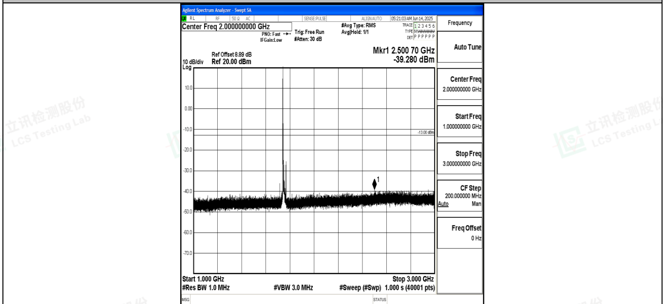
Band4_15MHz_QPSK_20325_1RB#0_1000~3000_1000~3000
