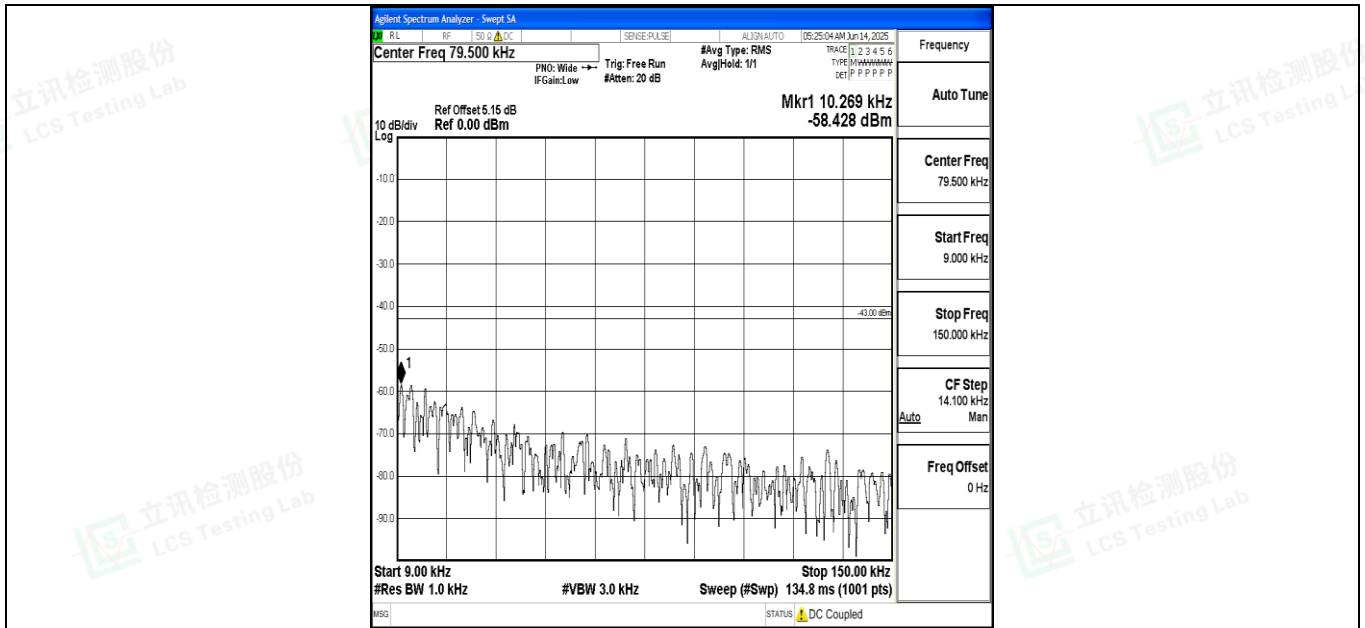
Band4_20MHz_QPSK_20300_1RB#0_0.009~0.15_0.009~0.15
