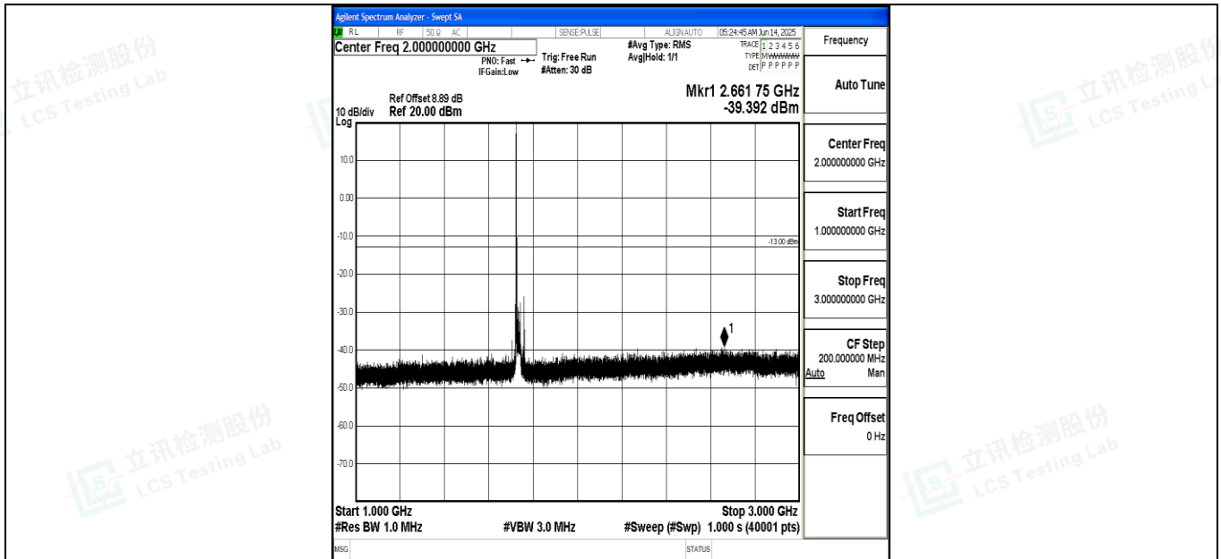
Band4_20MHz_16QAM_20175_1RB#0_1000~3000_1000~3000
