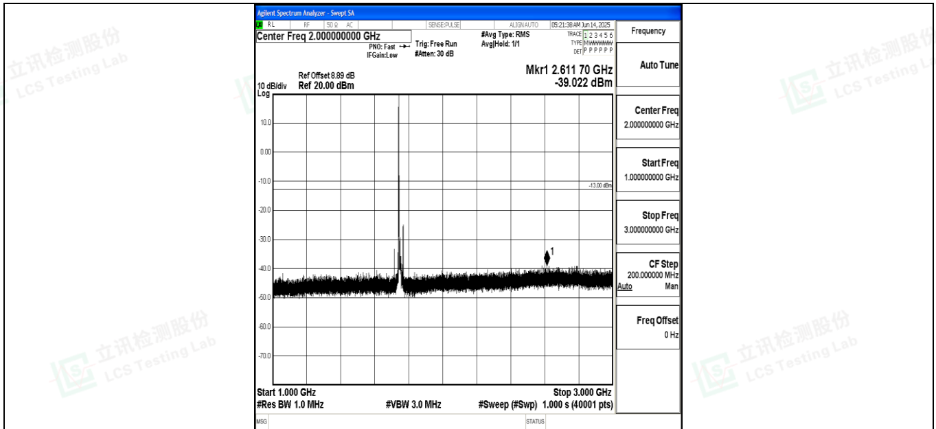
Band4_15MHz_16QAM_20325_1RB#0_1000~3000_1000~3000
