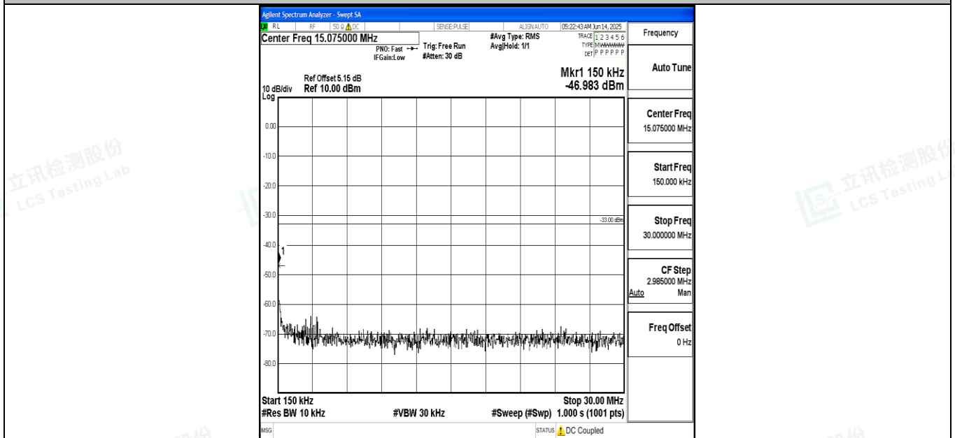
Band4_20MHz_QPSK_20050_1RB#0_0.15~30_0.15~30
