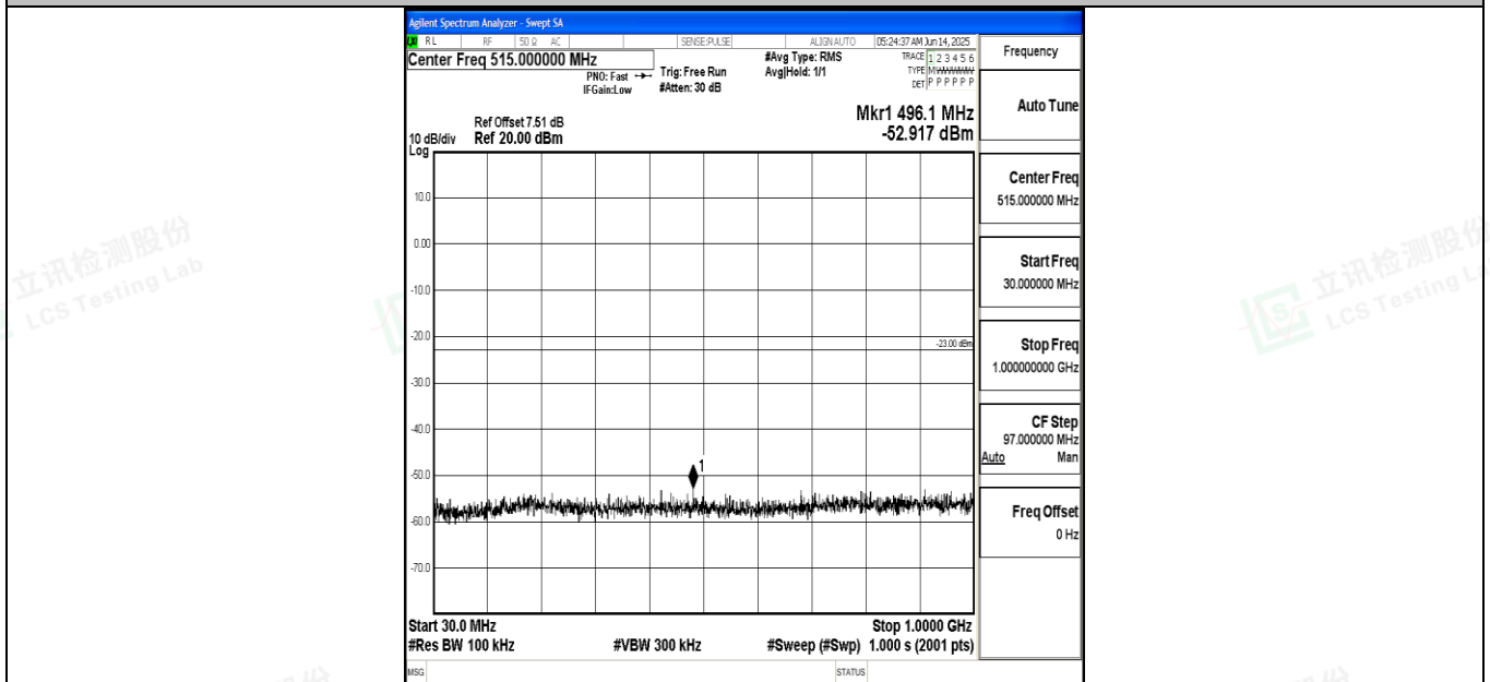
Band4_20MHz_16QAM_20175_1RB#0_30~1000_30~1000
