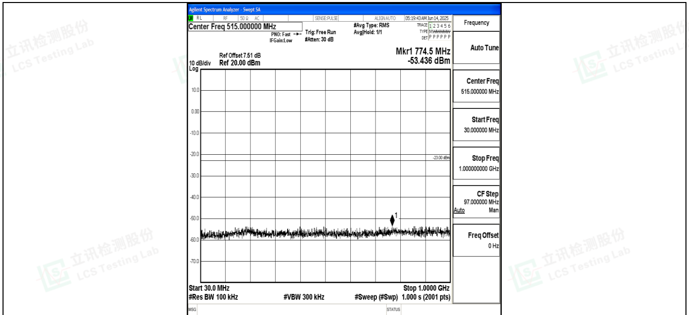
Band4_15MHz_QPSK_20175_1RB#0_30~1000_30~1000
