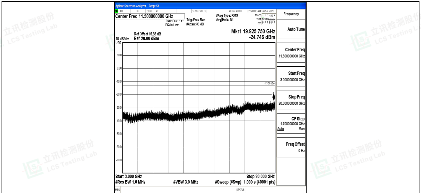
Band4_15MHz_QPSK_20175_1RB#0_3000~20000_3000~20000
