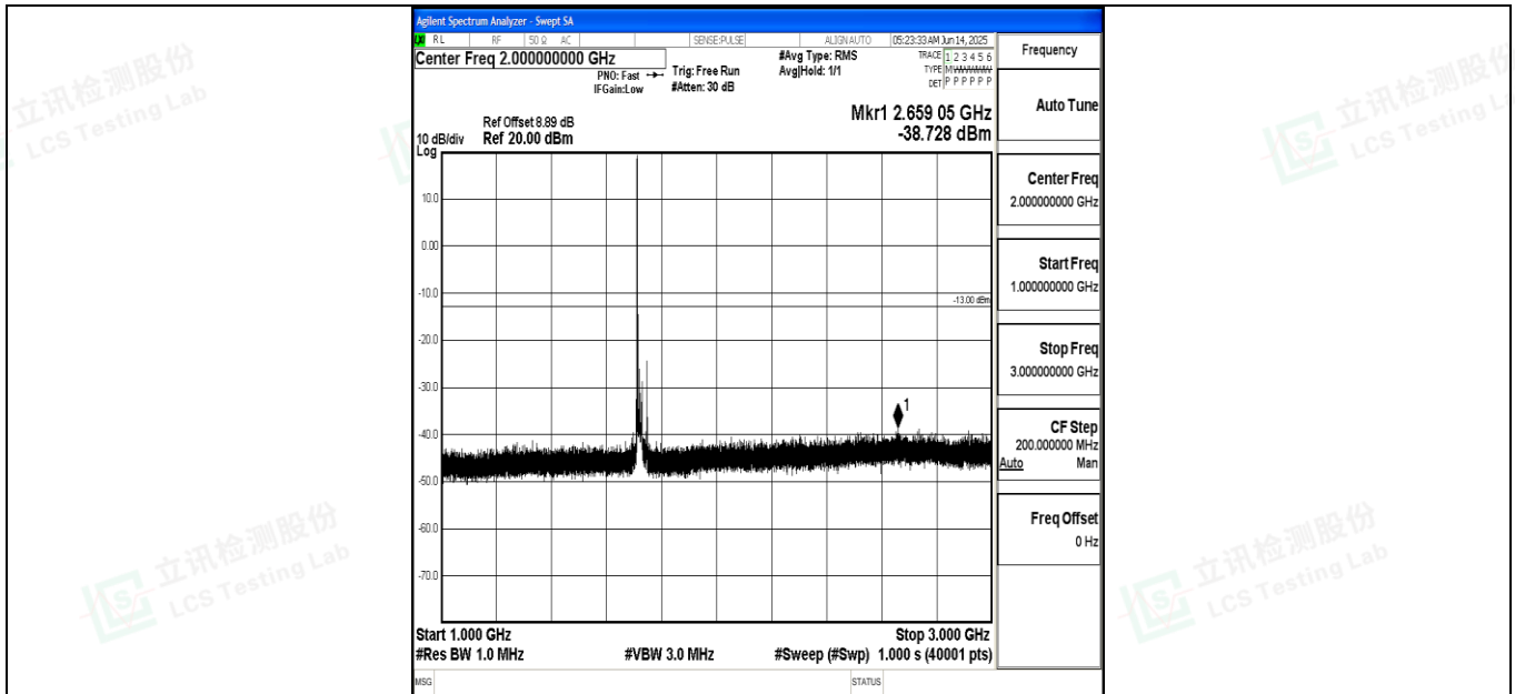
Band4_20MHz_16QAM_20050_1RB#0_1000~3000_1000~3000
