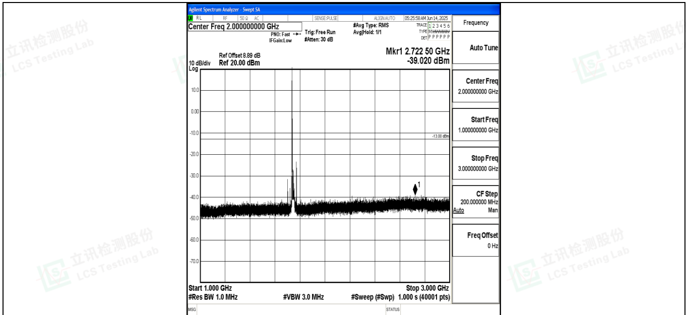
Band4_20MHz_16QAM_20300_1RB#0_1000~3000_1000~3000
