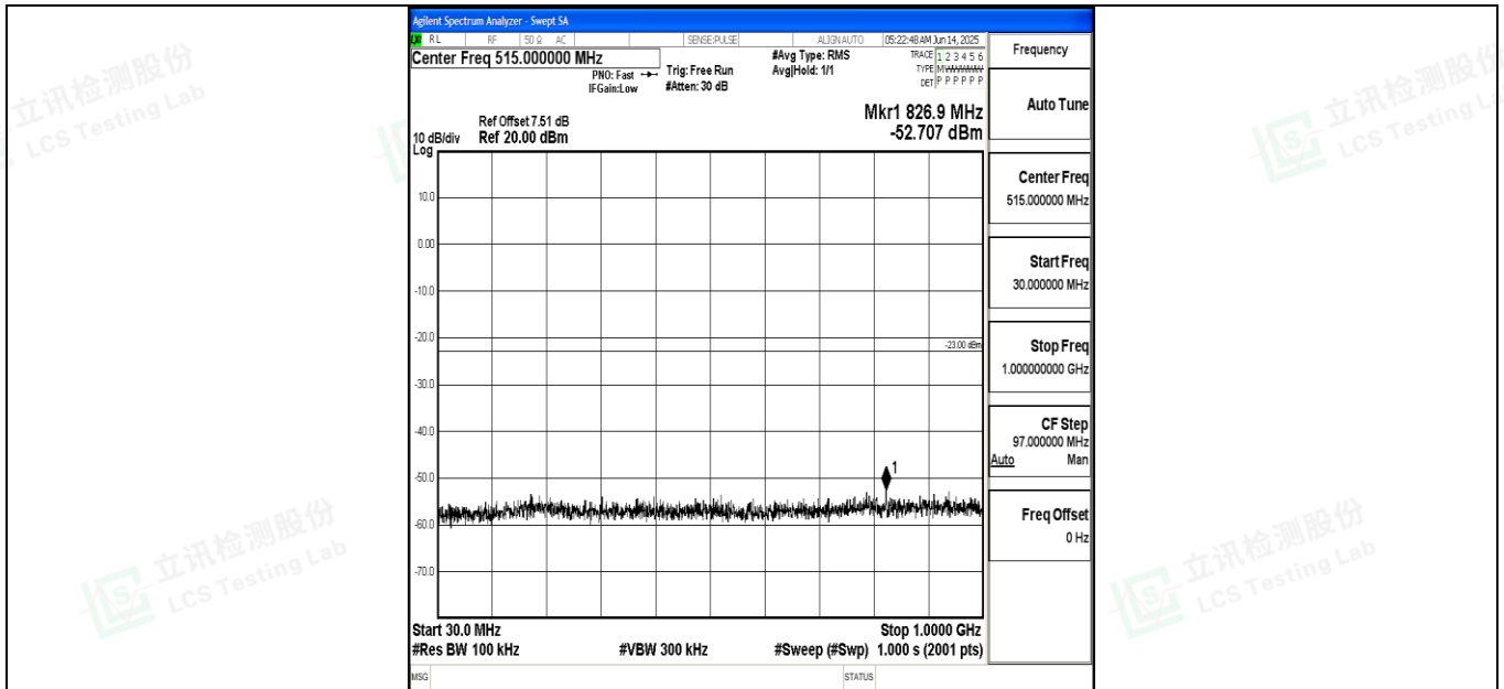
Band4_20MHz_QPSK_20050_1RB#0_30~1000_30~1000
