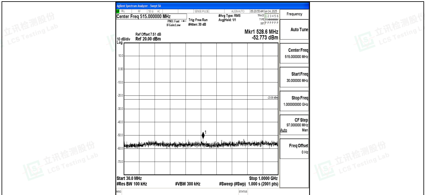
Band4_15MHz_QPSK_20325_1RB#0_30~1000_30~1000
