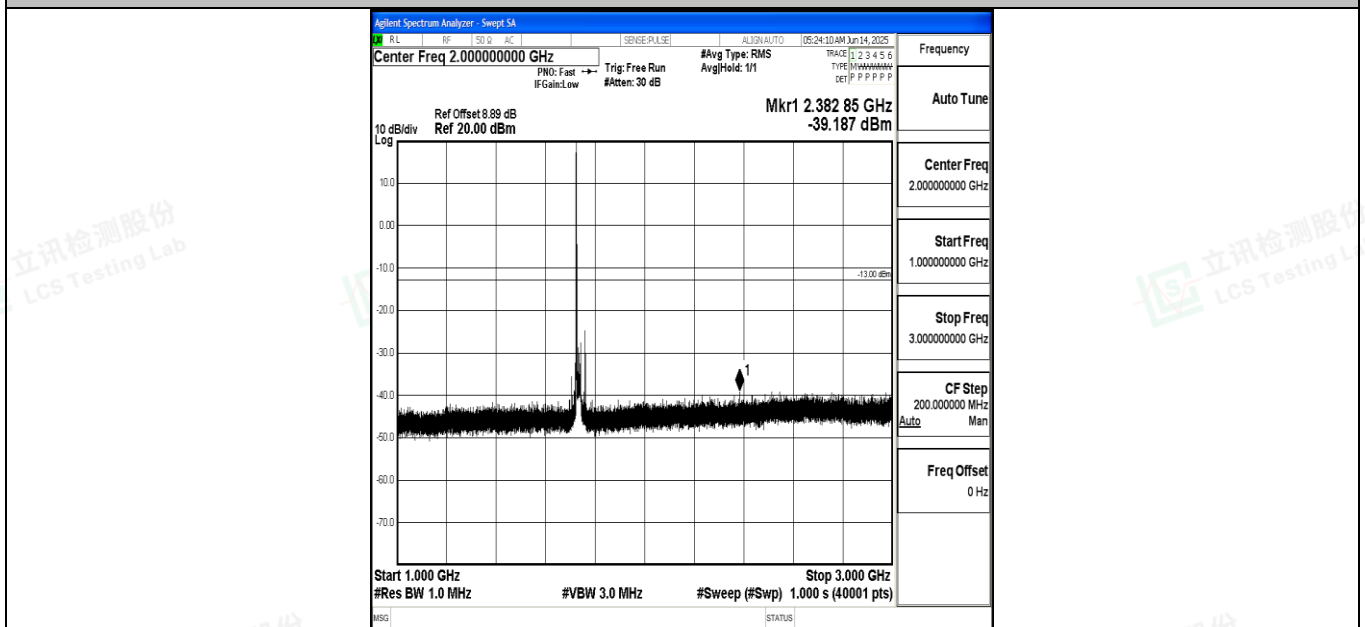
Band4_20MHz_QPSK_20175_1RB#0_1000~3000_1000~3000
