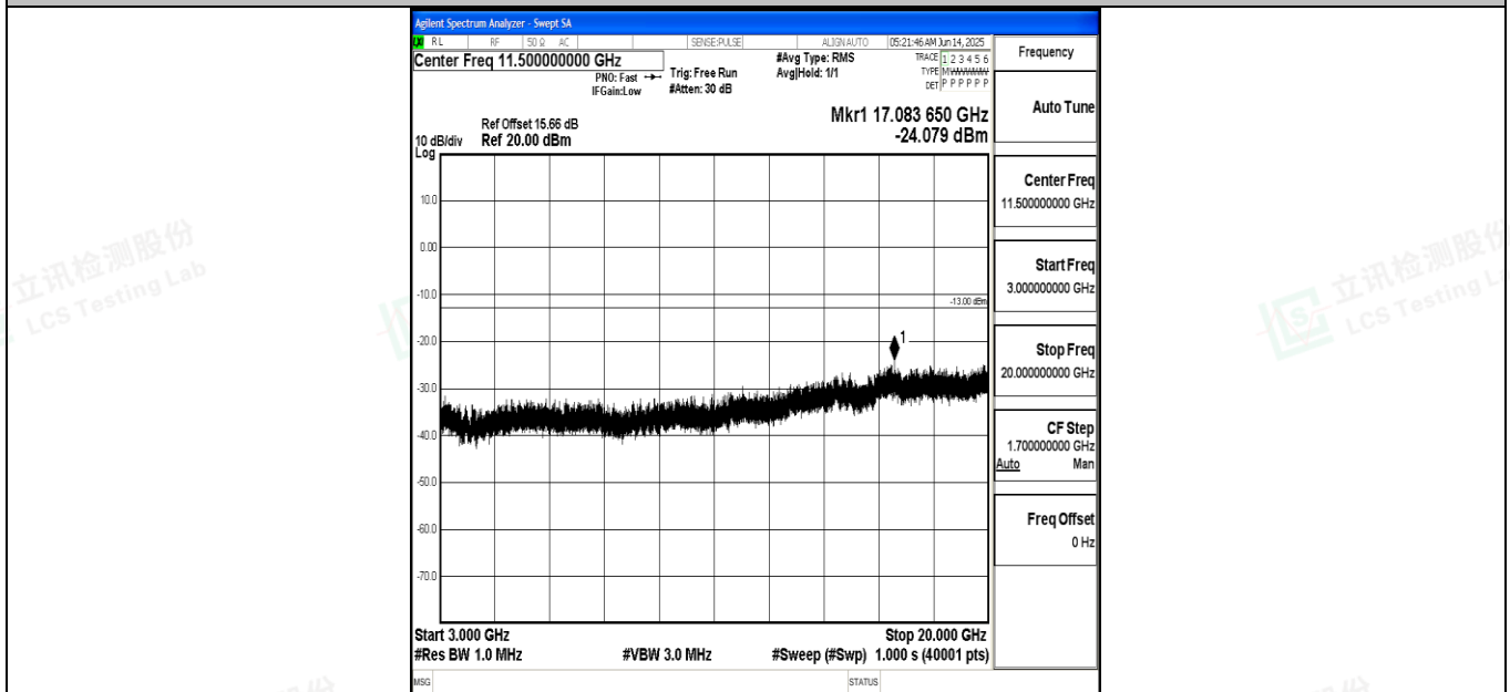
Band4_15MHz_16QAM_20325_1RB#0_3000~20000_3000~20000
