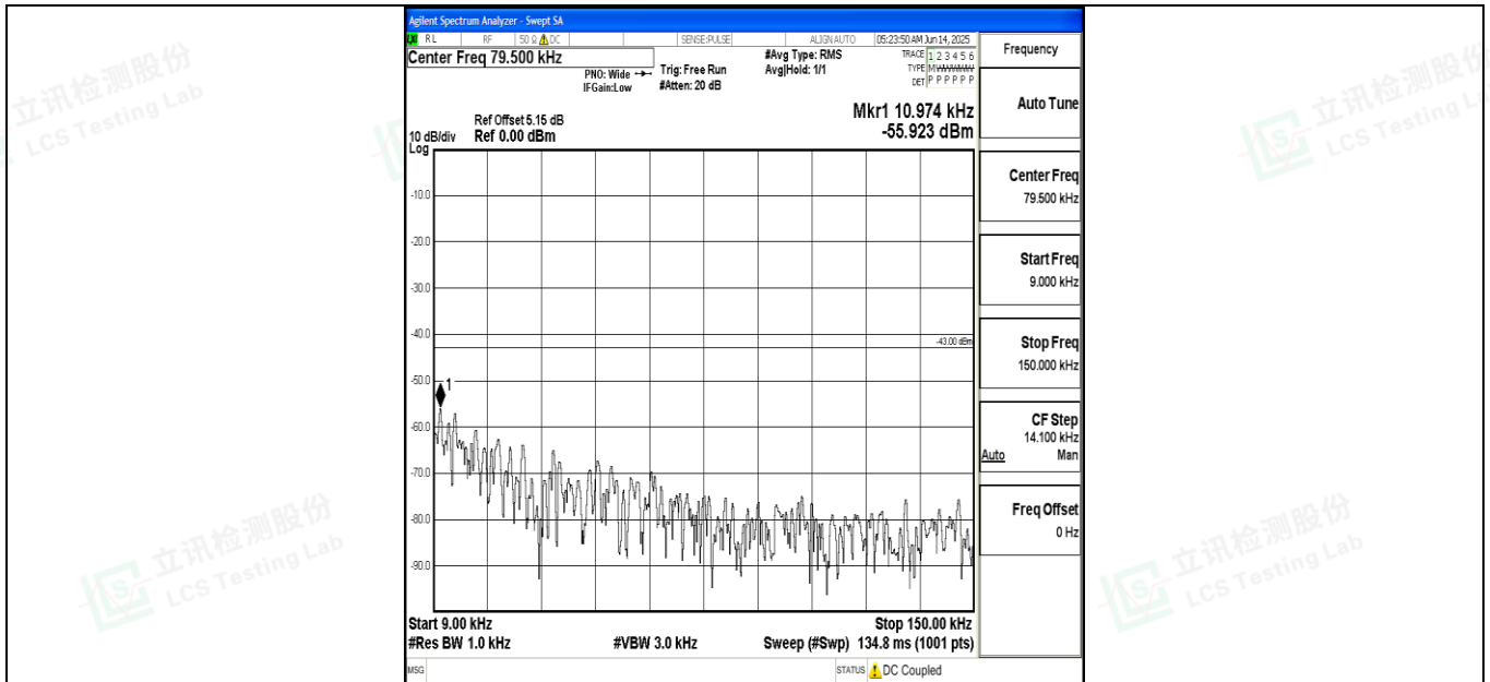
Band4_20MHz_QPSK_20175_1RB#0_0.009~0.15_0.009~0.15
