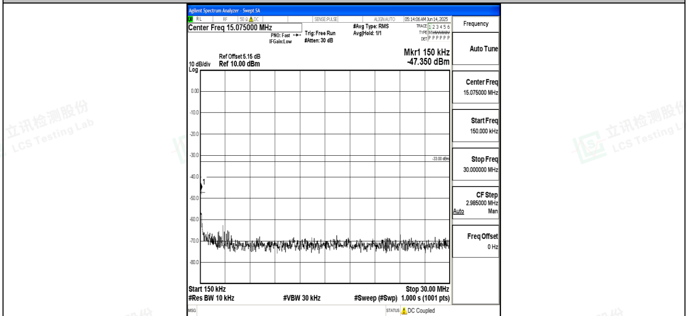
Band4_10MHz_QPSK_20000_1RB#0_0.15~30_0.15~30
