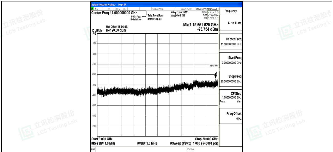
Band4_3MHz_QPSK_20385_1RB#0_3000~20000_3000~20000
