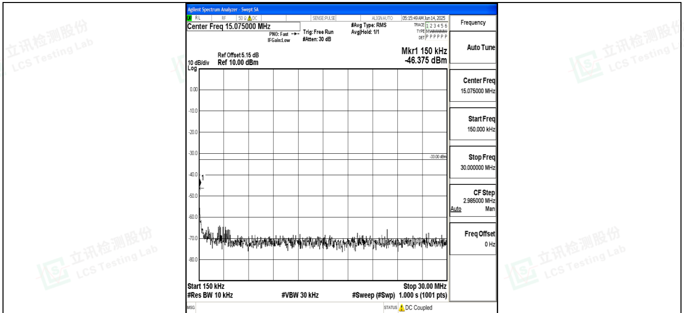
Band4_10MHz_16QAM_20175_1RB#0_0.15~30_0.15~30
