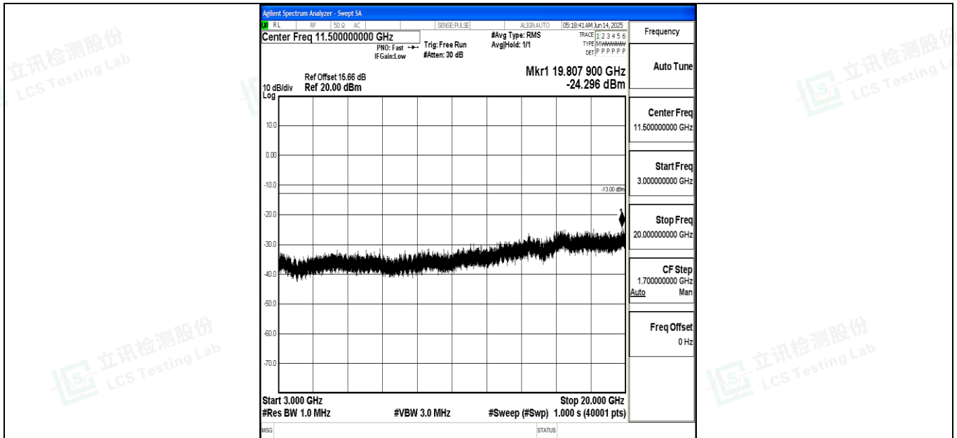
Band4_15MHz_QPSK_20025_1RB#0_3000~20000_3000~20000
