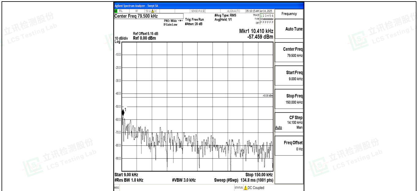
Band4_15MHz_QPSK_2025_1RB#0_0.009~0.15_0.009~0.15
