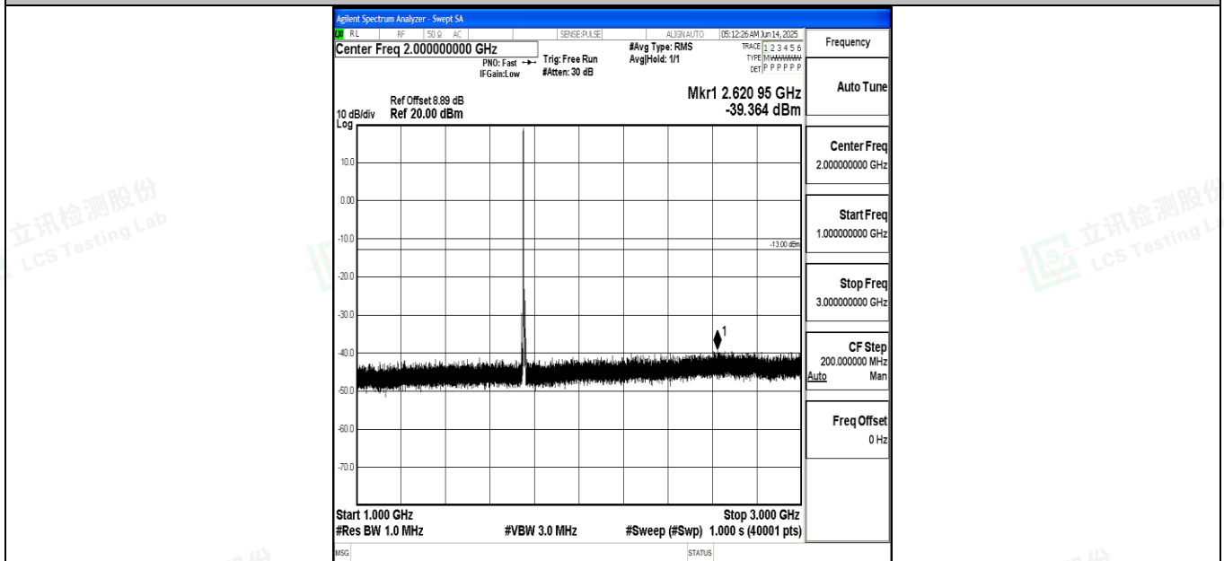
Band4_5MHz_QPSK_20375_1RB#0_1000~3000_1000~3000
