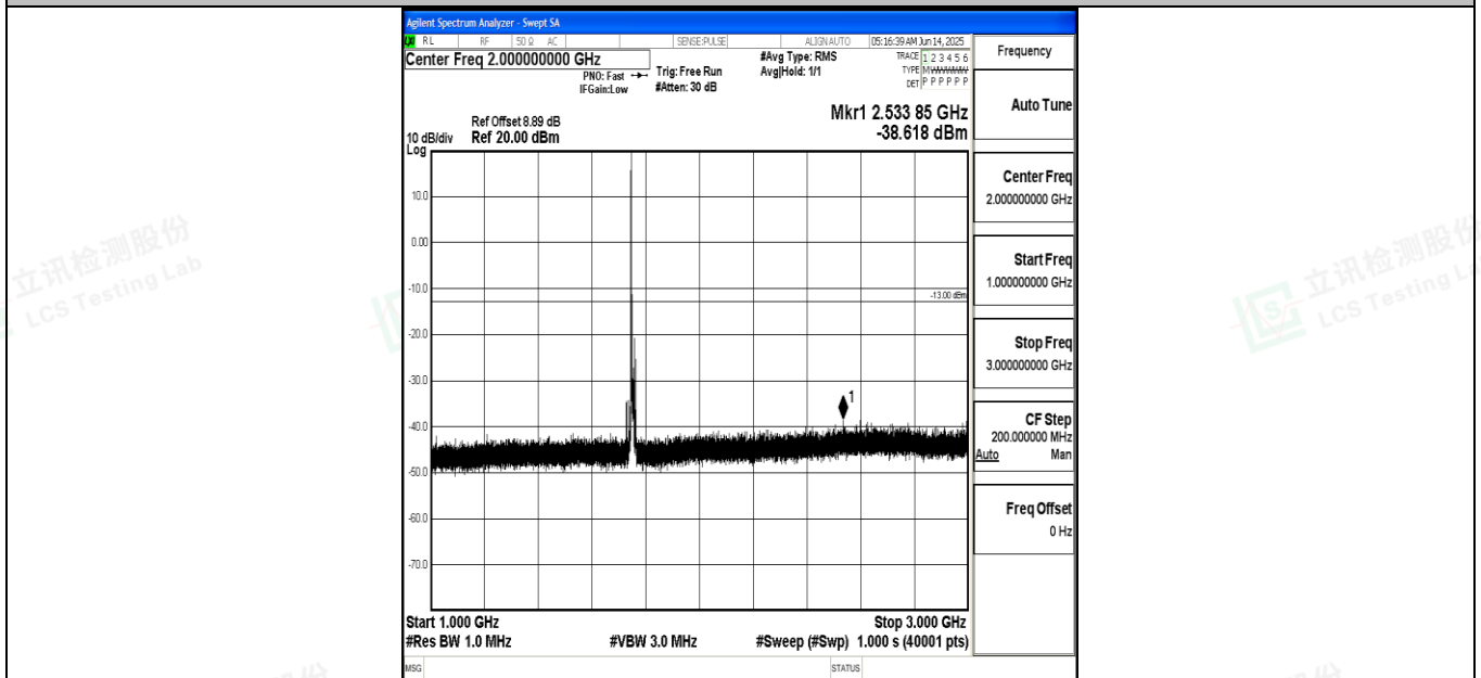
Band4_10MHz_QPSK_20350_1RB#0_1000~3000_1000~3000
