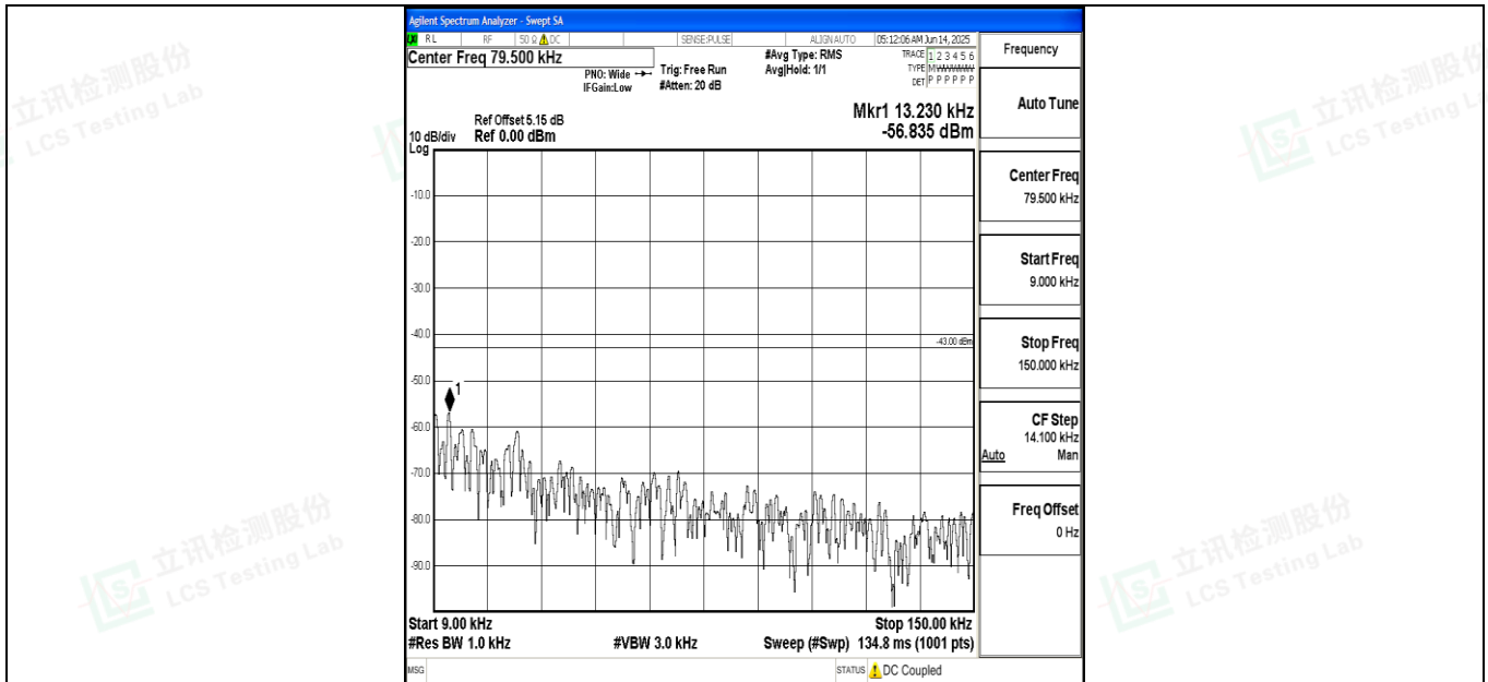
Band4_5MHz_QPSK_20375_1RB#0_0.009~0.15_0.009~0.15
