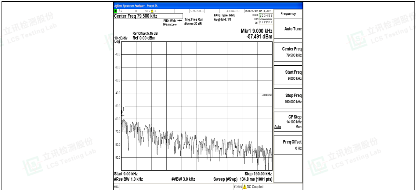
Band4_5MHz_QPSK_19975_1RB#0_0.009~0.15_0.009~0.15
