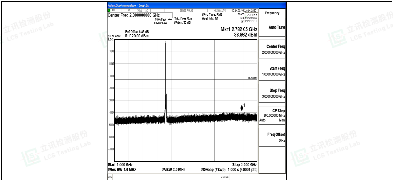
Band4_10MHz_16QAM_20000_1RB#0_1000~3000_1000~3000
