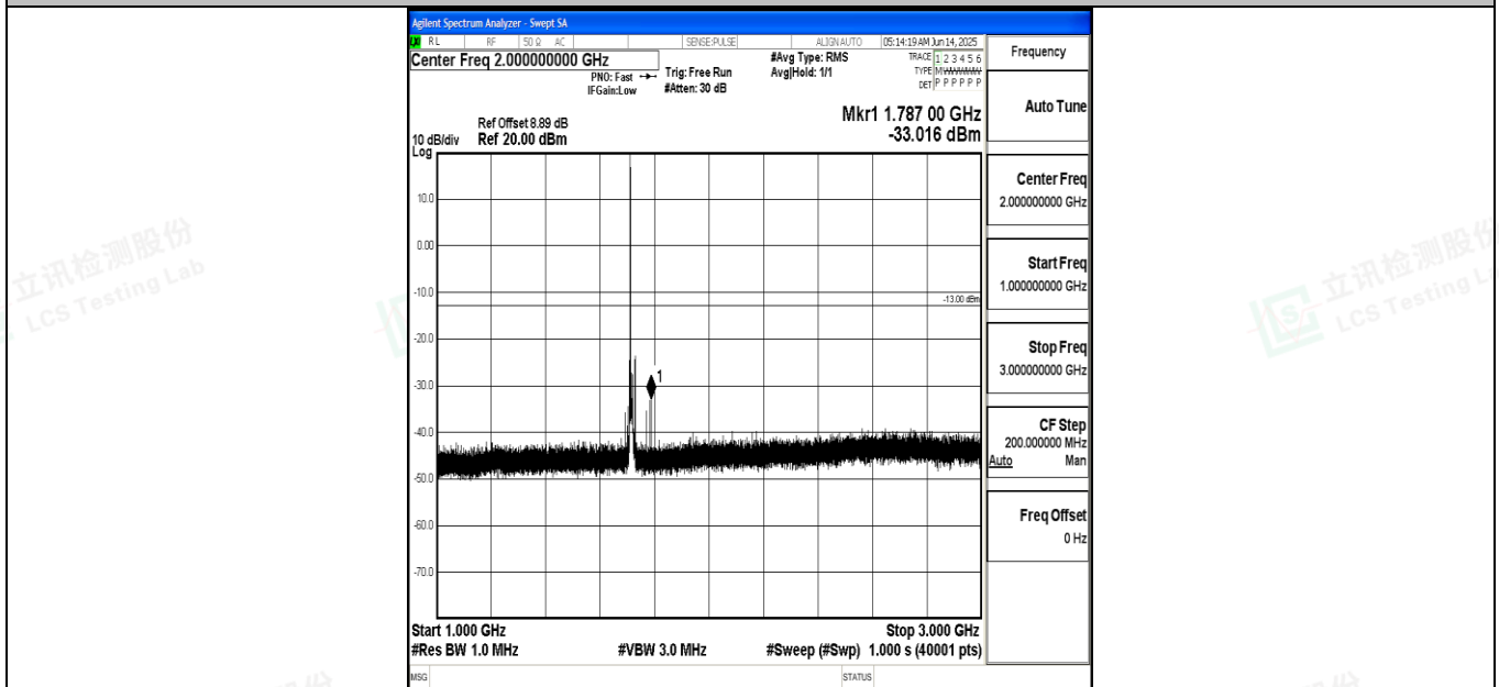
Band4_10MHz_QPSK_20000_1RB#0_1000~3000_1000~3000
