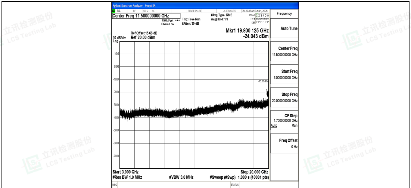
Band4_10MHz_QPSK_20175_1RB#0_3000~20000_3000~20000
