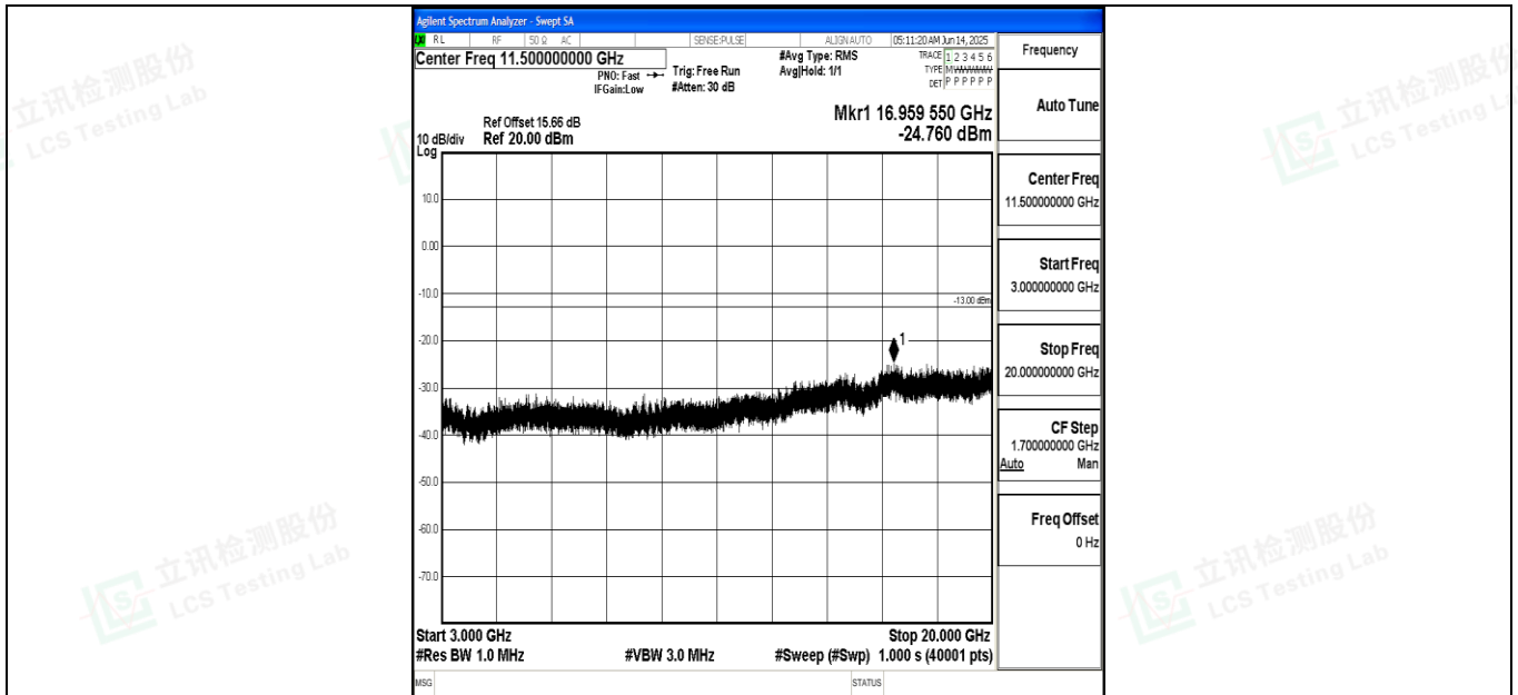
Band4_5MHz_QPSK_20175_1RB#0_3000~20000_3000~20000
