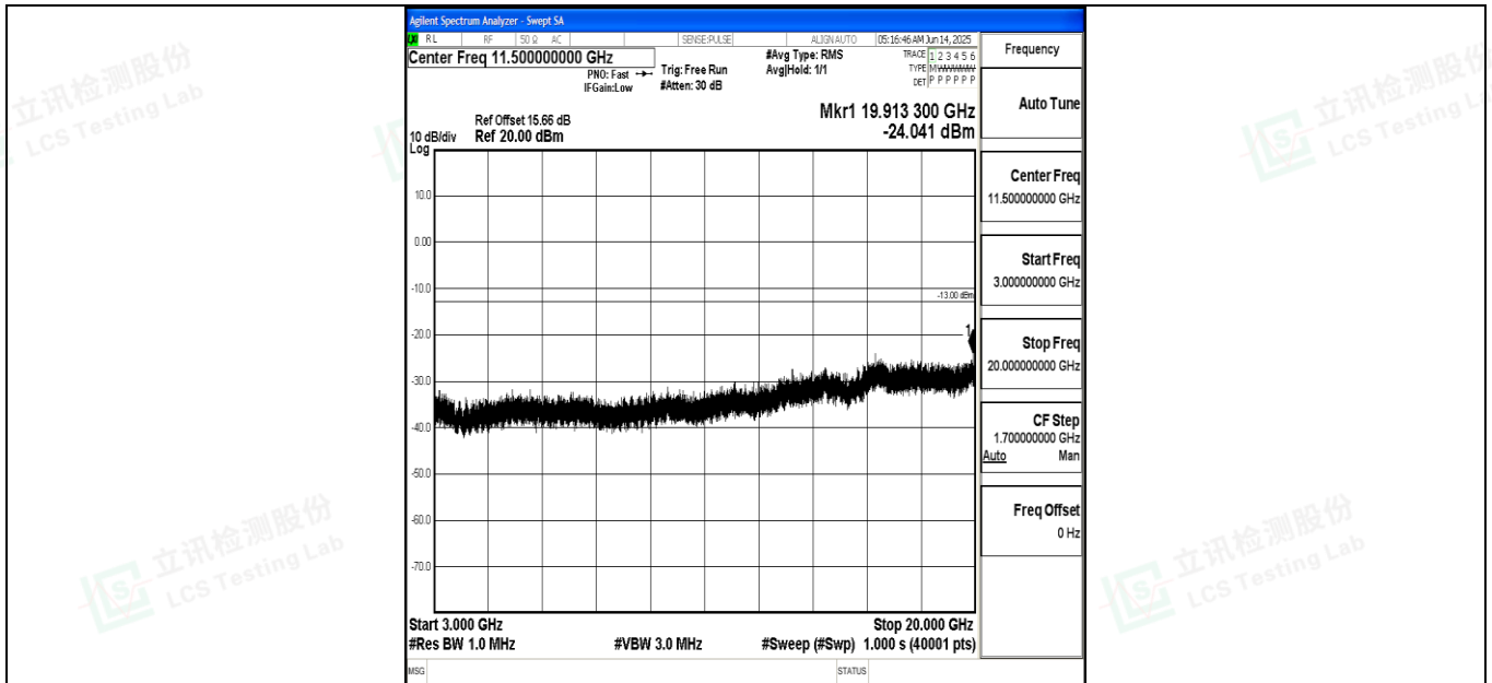
Band4_10MHz_QPSK_20350_1RB#0_3000~20000_3000~20000
