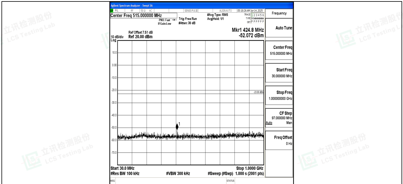
Band4_15MHz_QPSK_20025_1RB#0_30~1000_30~1000
