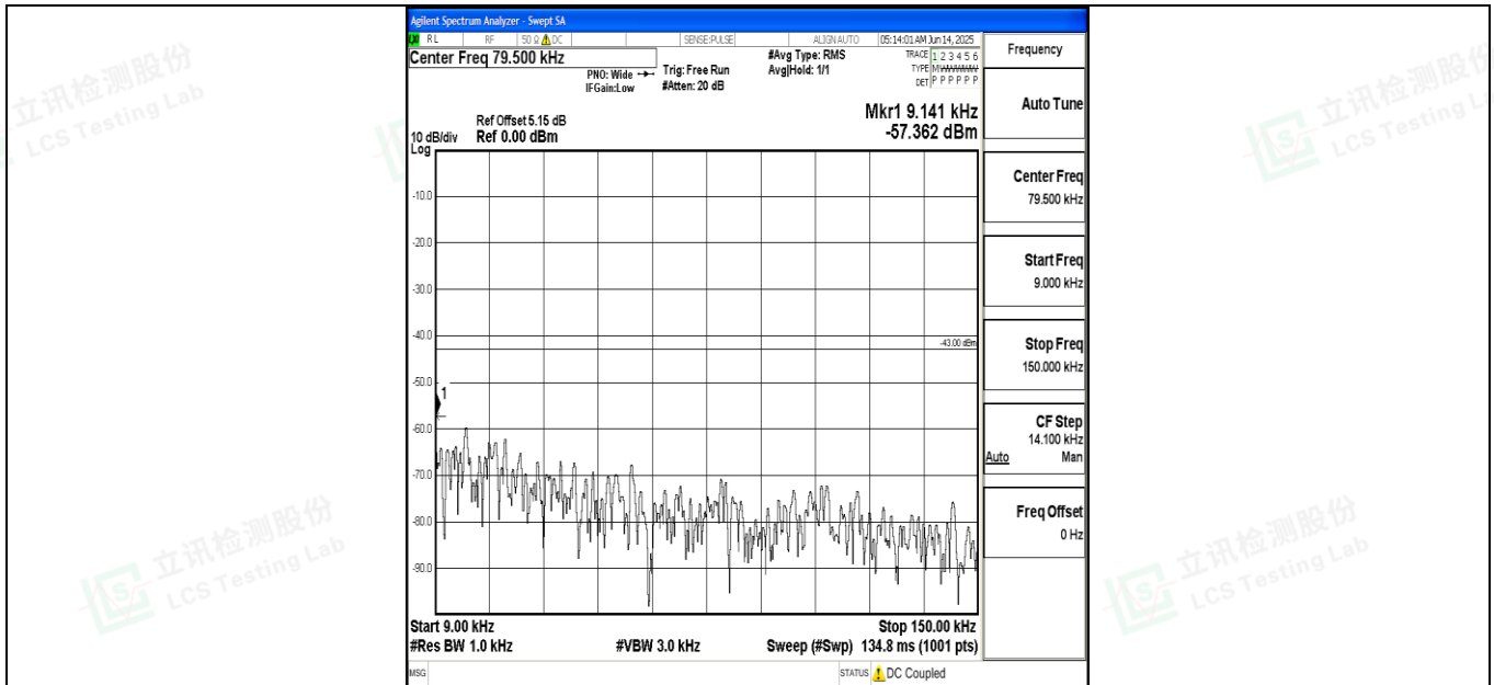
Band4_10MHz_QPSK_20000_1RB#0_0.009~0.15_0.009~0.15
