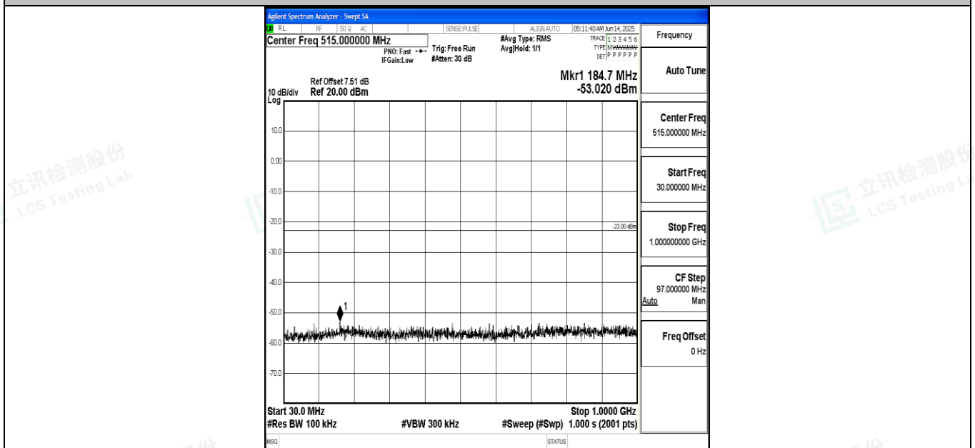
Band4_5MHz_16QAM_20175_1RB#0_30~1000_30~1000
