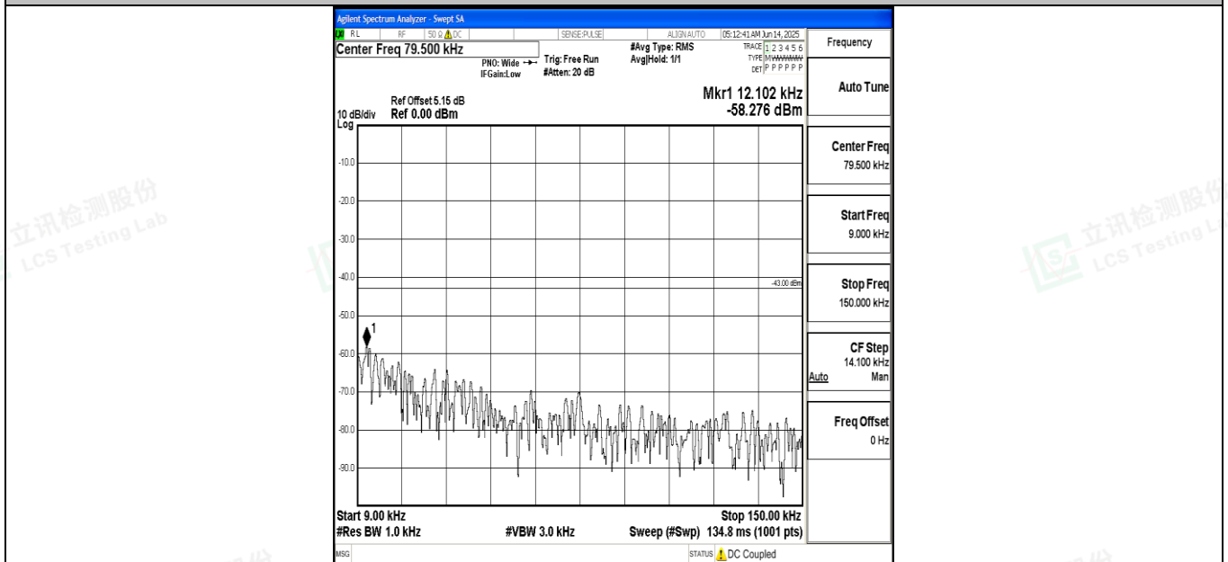
Band4_5MHz_16QAM_20375_1RB#0_0.009~0.15_0.009~0.15
