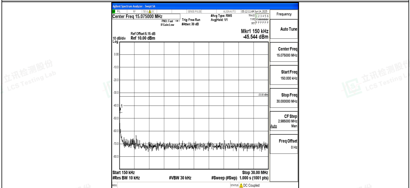
Band4_5MHz_QPSK_20375_1RB#0_0.15~30_0.15~30
