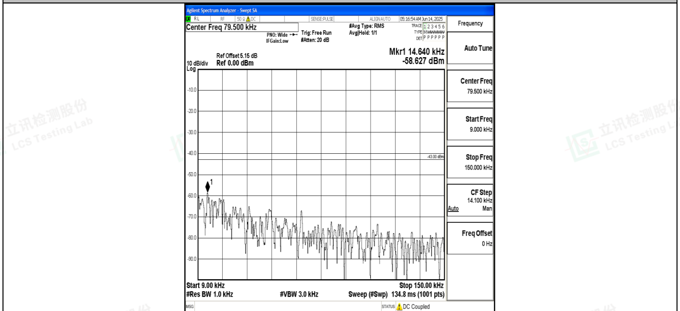
Band4_10MHz_16QAM_20350_1RB#0_0.009~0.15_0.009~0.15
