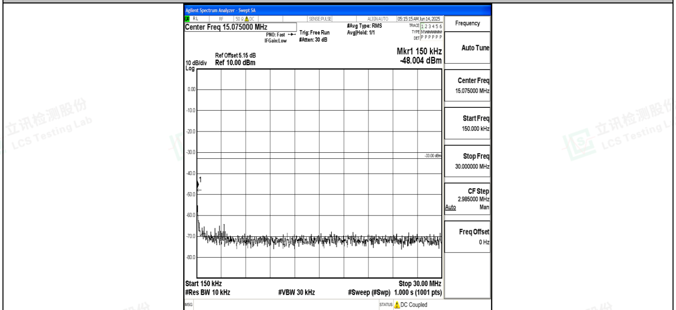
Band4_10MHz_QPSK_20175_1RB#0_0.15~30_0.15~30
