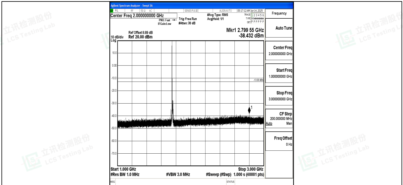
Band4_10MHz_16QAM_20350_1RB#0_1000~3000_1000~3000
