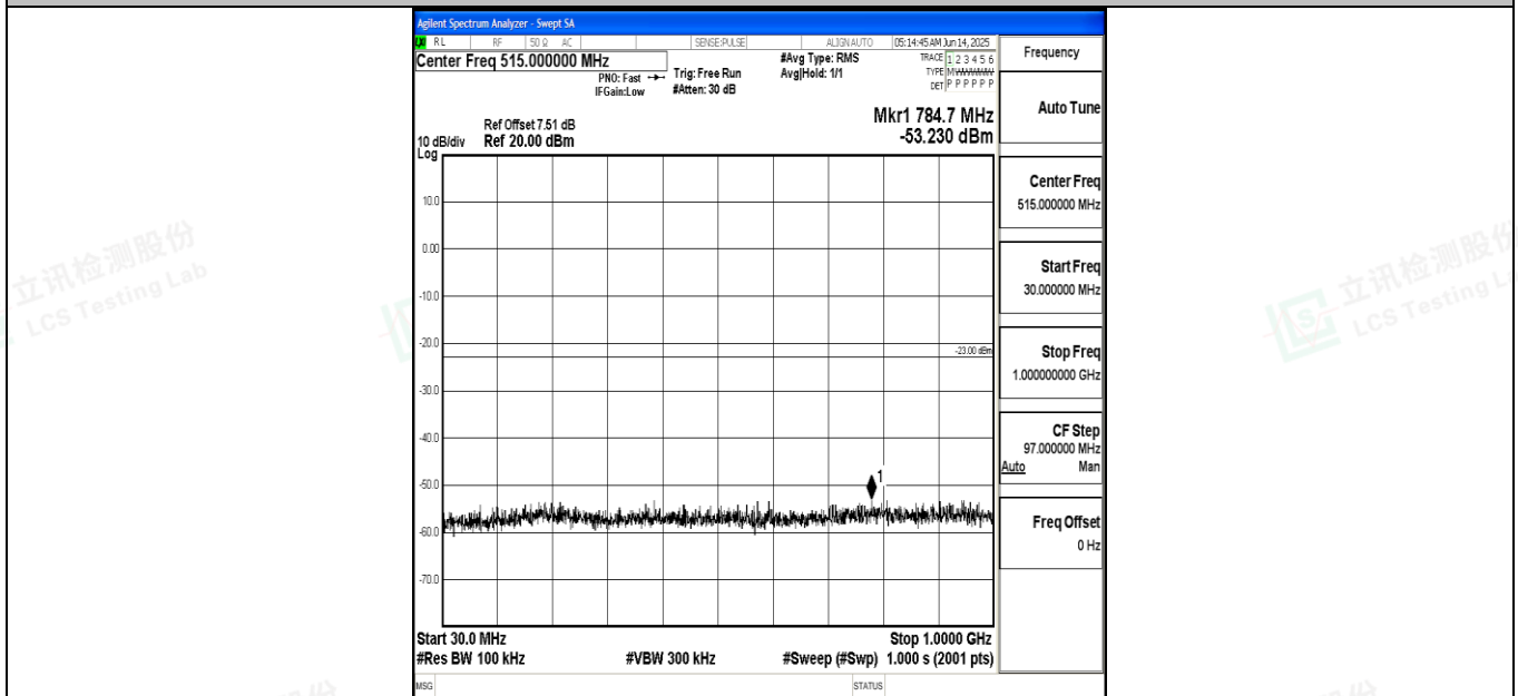
Band4_10MHz_16QAM_20000_1RB#0_30~1000_30~1000
