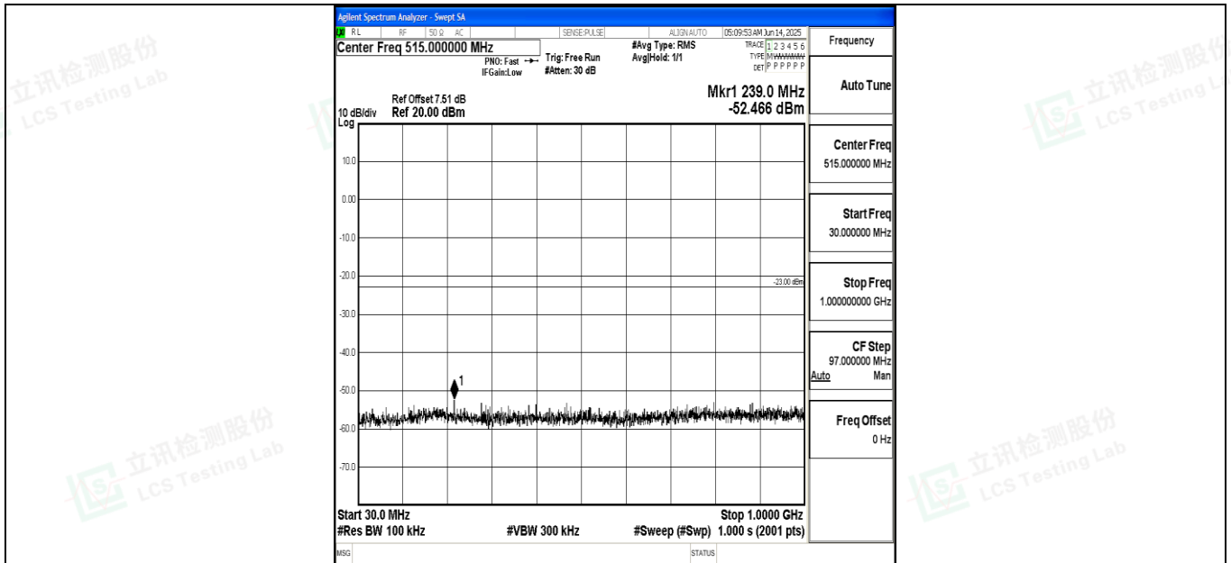
Band4_5MHz_QPSK_19975_1RB#0_30~1000_30~1000
