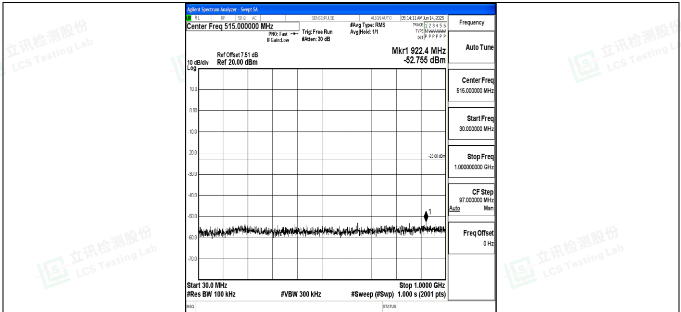
Band4_10MHz_QPSK_20000_1RB#0_30~1000_30~1000
