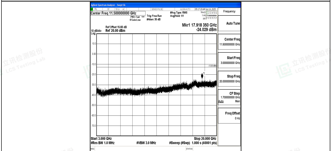
Band4_10MHz_16QAM_20350_1RB#0_3000~20000_3000~20000
