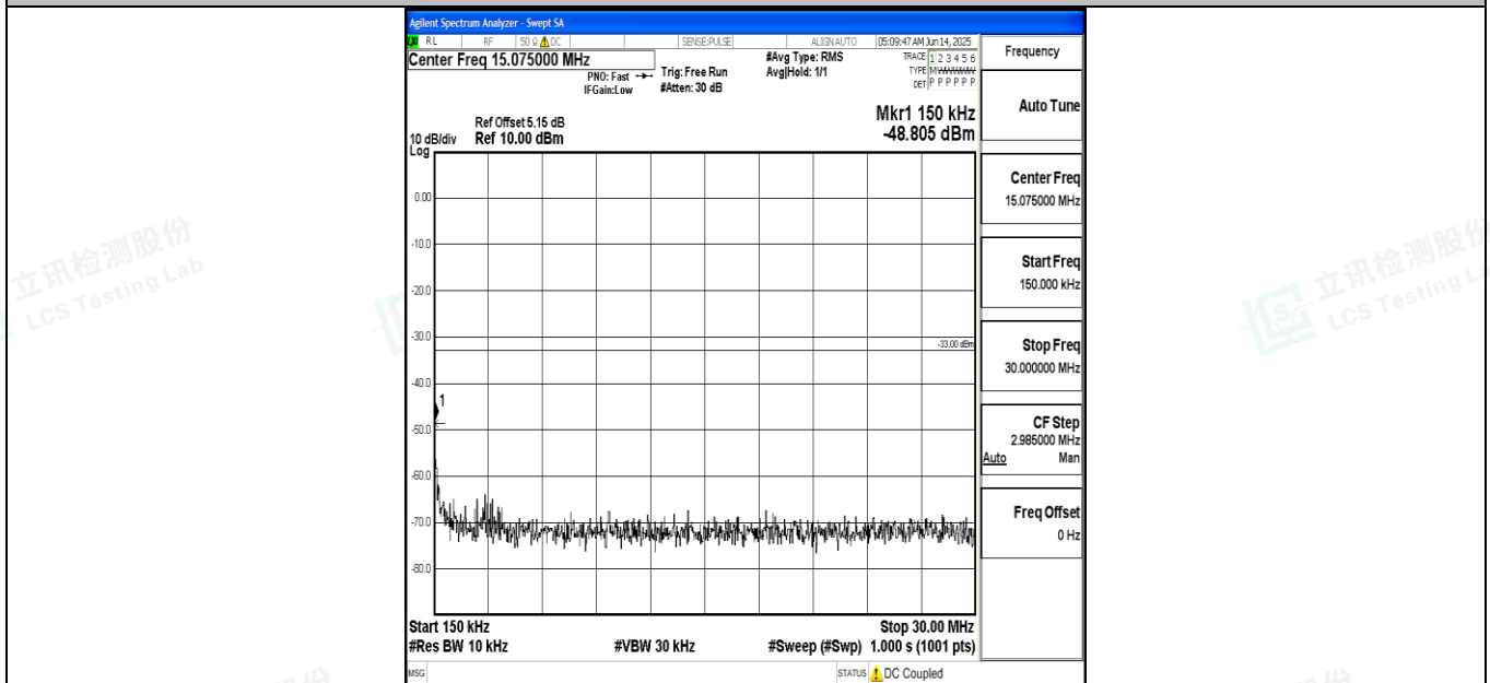
Band4_5MHz_QPSK_19975_1RB#0_0.15~30_0.15~30
