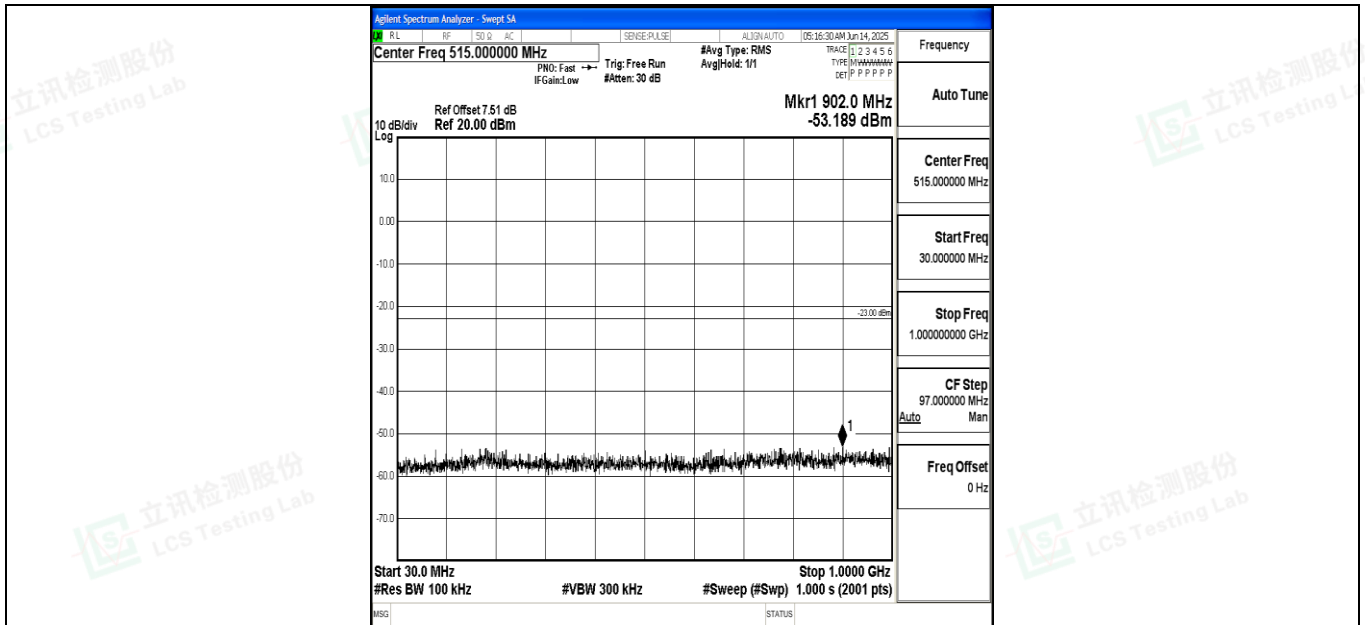
Band4_10MHz_QPSK_20350_1RB#0_30~1000_30~1000
