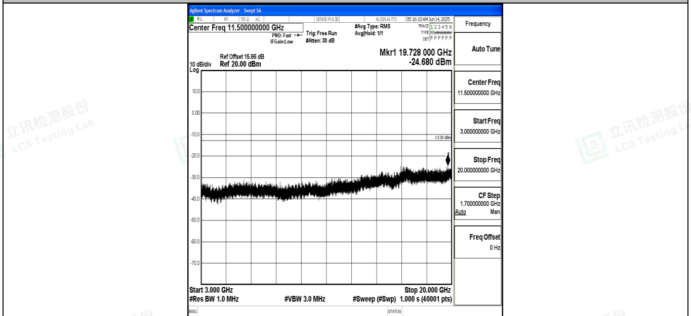
Band4_10MHz_16QAM_20175_1RB#0_3000~20000_3000~20000
