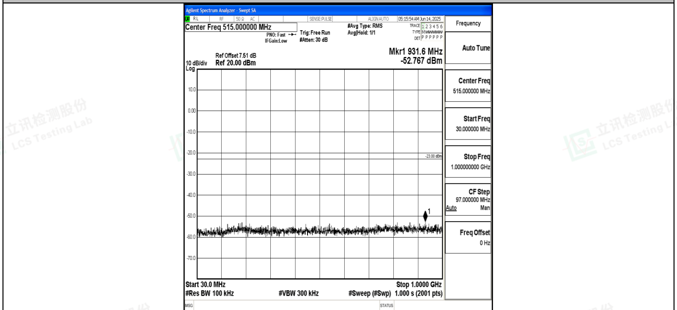
Band4_10MHz_16QAM_20175_1RB#0_30~1000_30~1000
