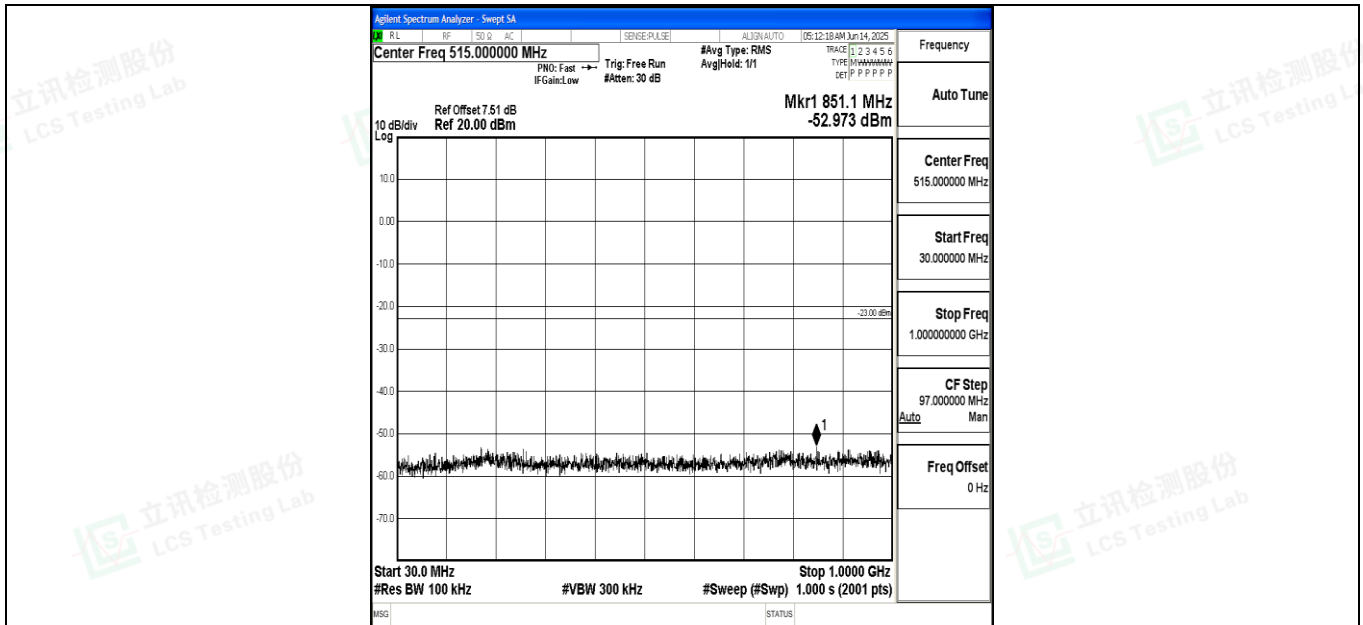
Band4_5MHz_QPSK_20375_1RB#0_30~1000_30~1000
