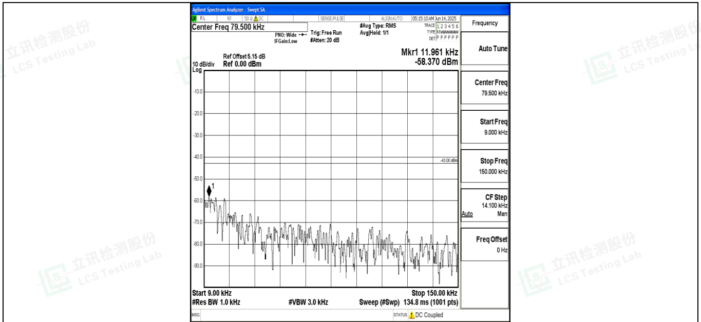
Band4_10MHz_QPSK_20175_1RB#0_0.009~0.15_0.009~0.15
