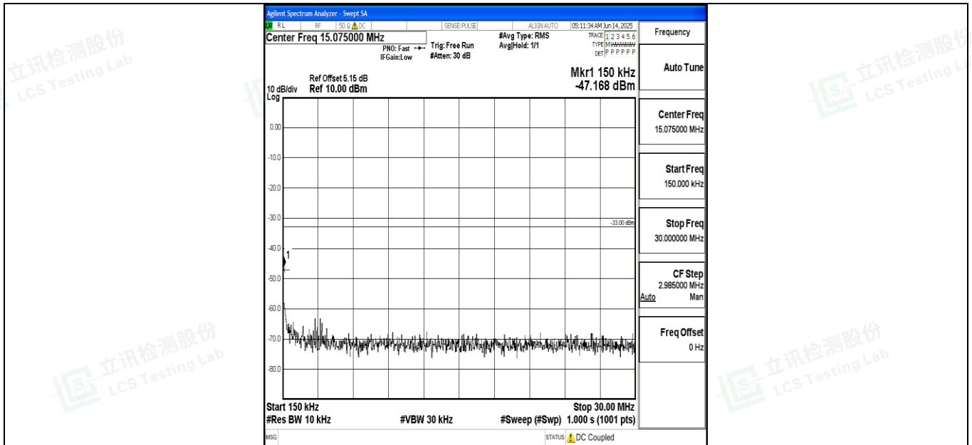
Band4_5MHz_16QAM_20175_1RB#0_0.15~30_0.15~30
