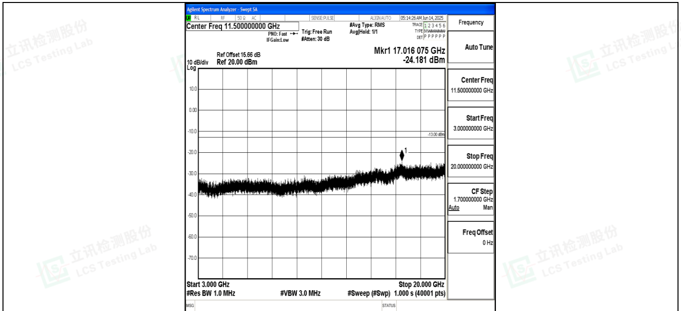
Band4_10MHz_QPSK_20000_1RB#0_3000~20000_3000~20000
