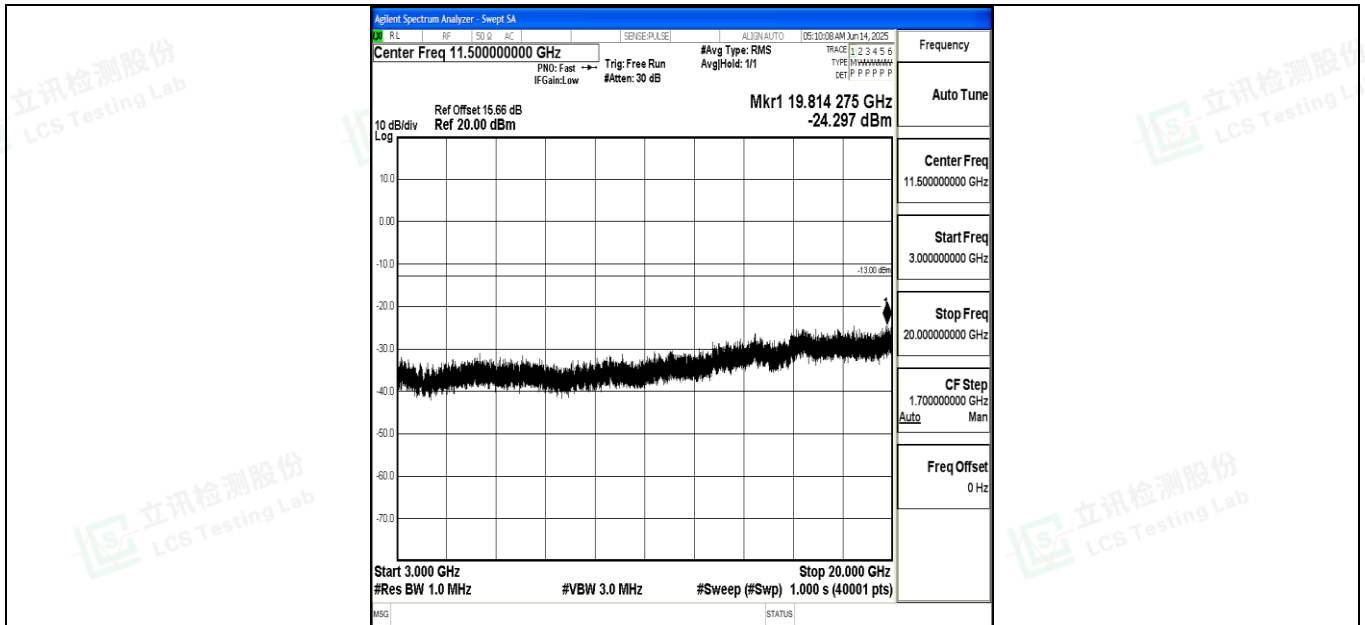
Band4_5MHz_QPSK_19975_1RB#0_3000~20000_3000~20000
