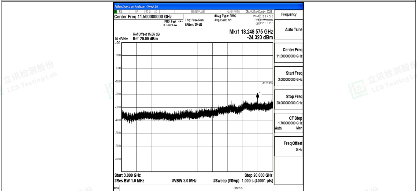
Band4_15MHz_16QAM_20025_1RB#0_3000~20000_3000~20000
