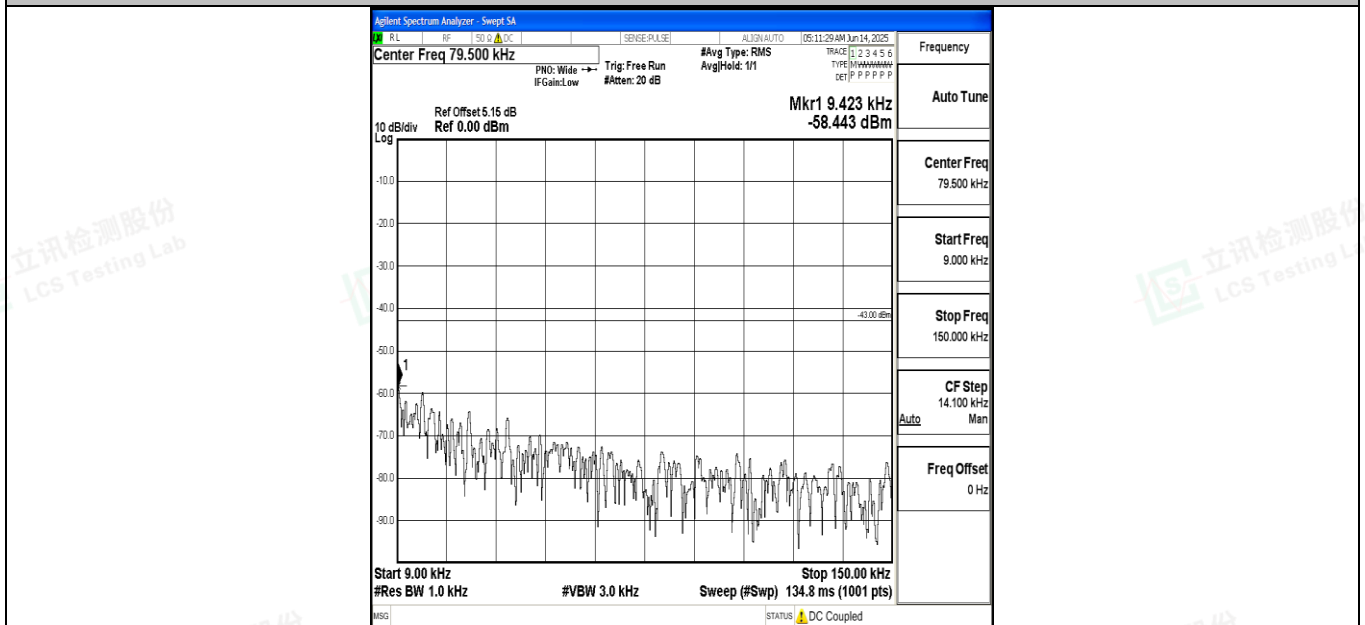
Band4_5MHz_16QAM_20175_1RB#0_0.009~0.15_0.009~0.15
