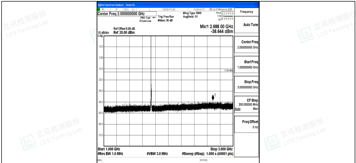
Band4_5MHz_16QAM_20175_1RB#0_1000~3000_1000~3000
