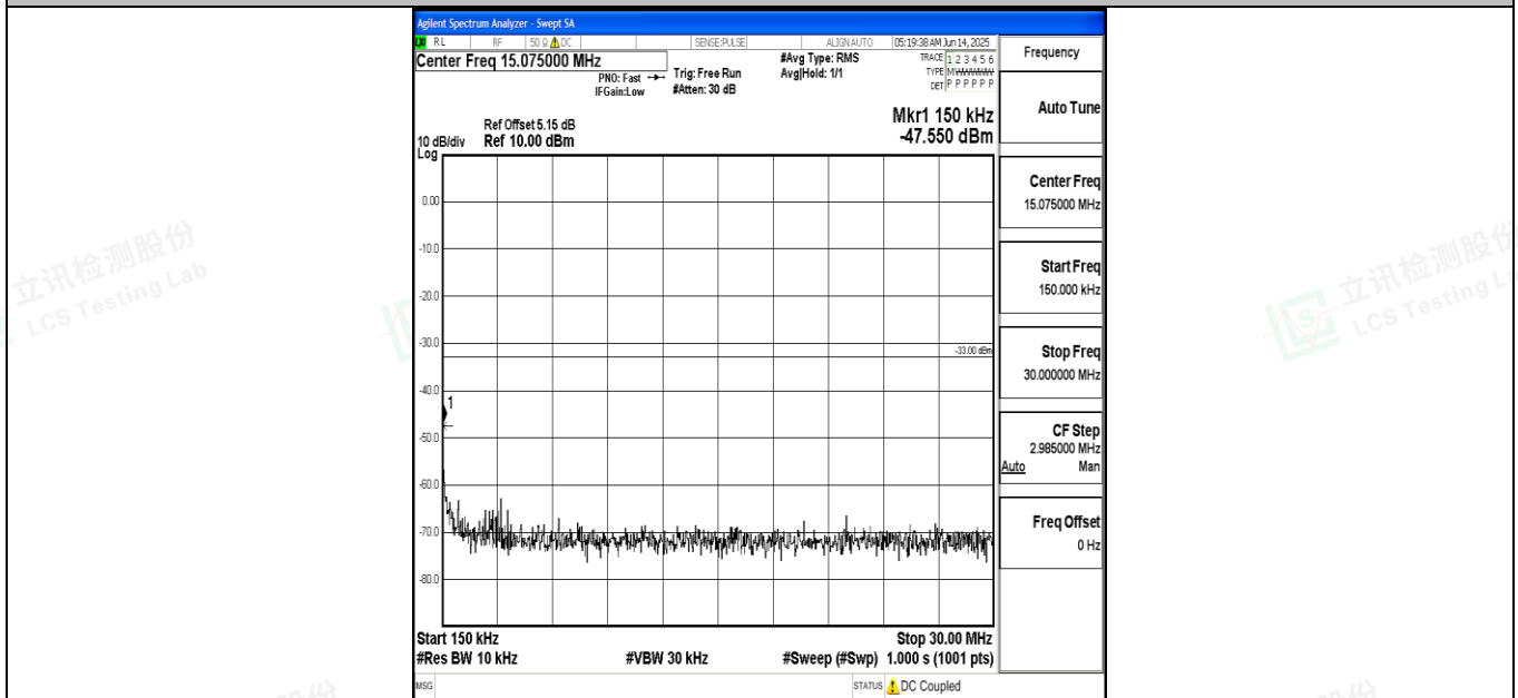
Band4_15MHz_QPSK_20175_1RB#0_0.15~30_0.15~30
