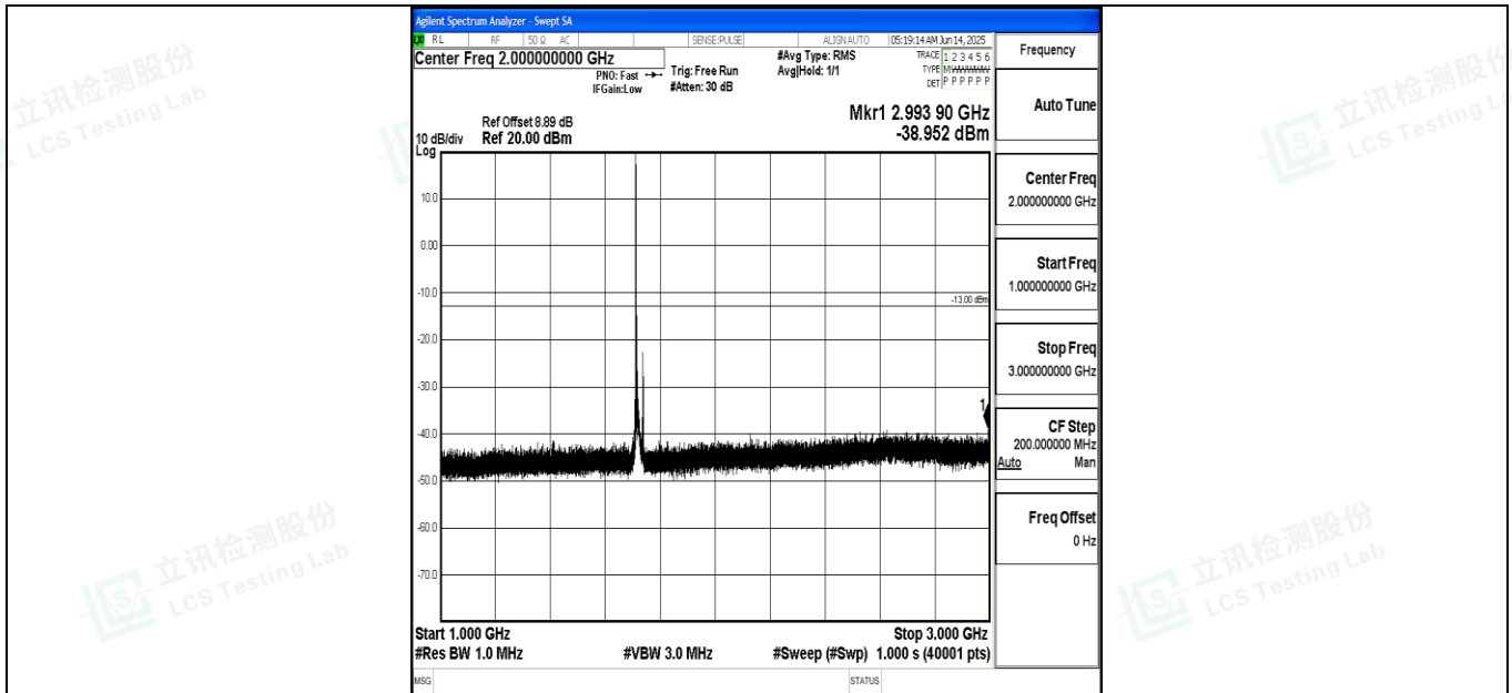
Band4_15MHz_16QAM_20025_1RB#0_1000~3000_1000~3000
