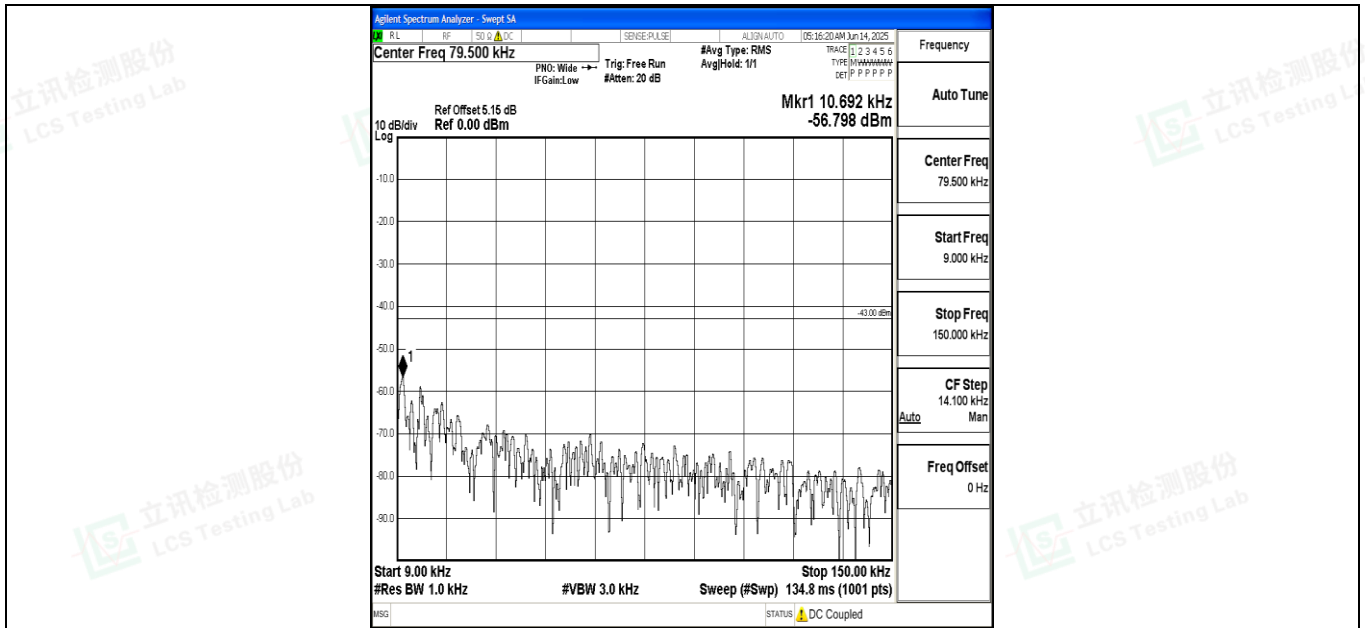
Band4_10MHz_QPSK_20350_1RB#0_0.009~0.15_0.009~0.15
