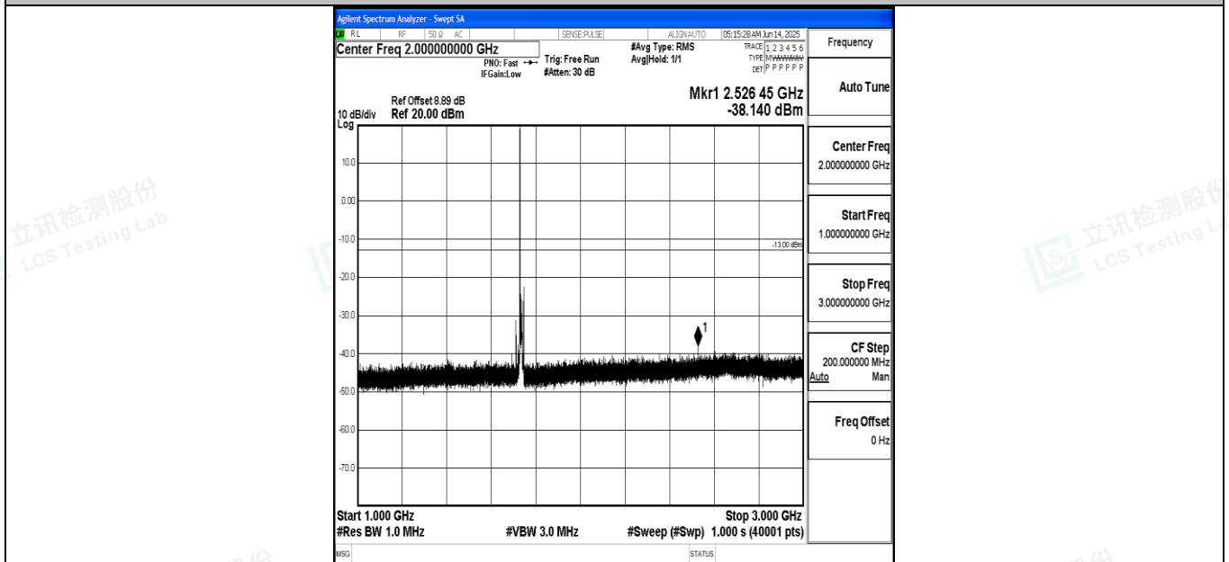
Band4_10MHz_QPSK_20175_1RB#0_1000~3000_1000~3000
