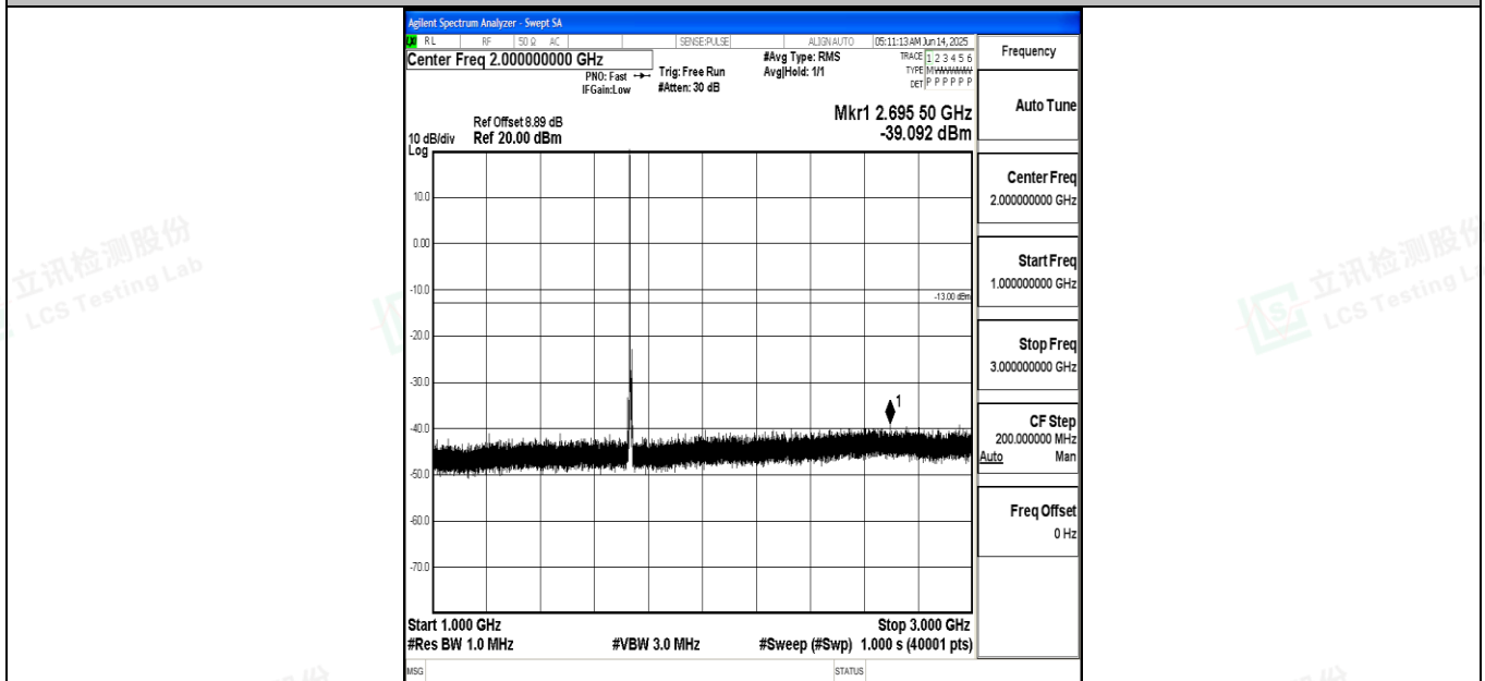
Band4_5MHz_QPSK_20175_1RB#0_1000~3000_1000~3000
