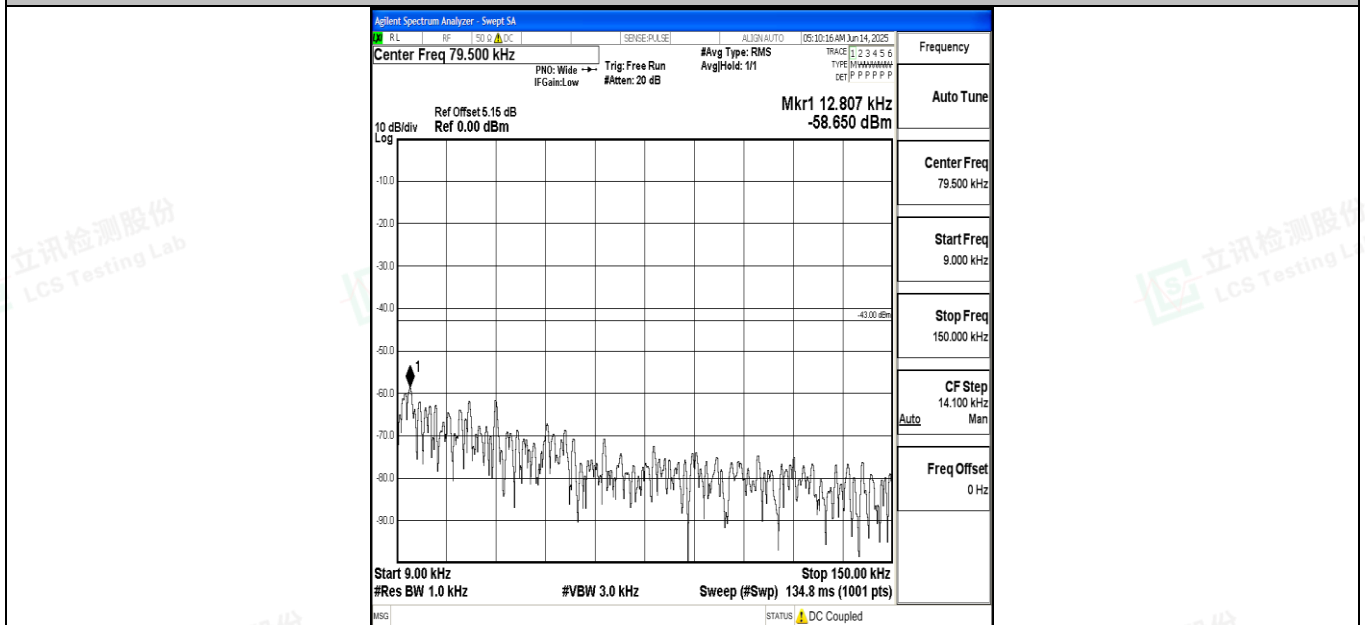
Band4_5MHz_16QAM_19975_1RB#0_0.009~0.15_0.009~0.15
