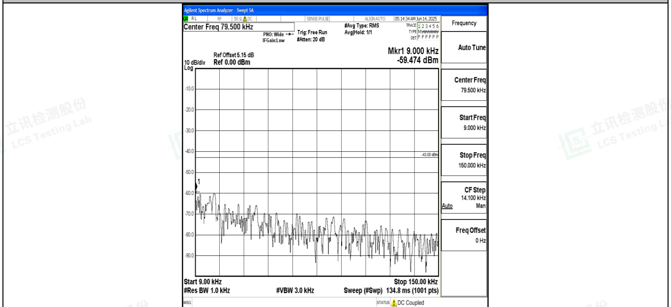
Band4_10MHz_16QAM_20000_1RB#0_0.009~0.15_0.009~0.15
