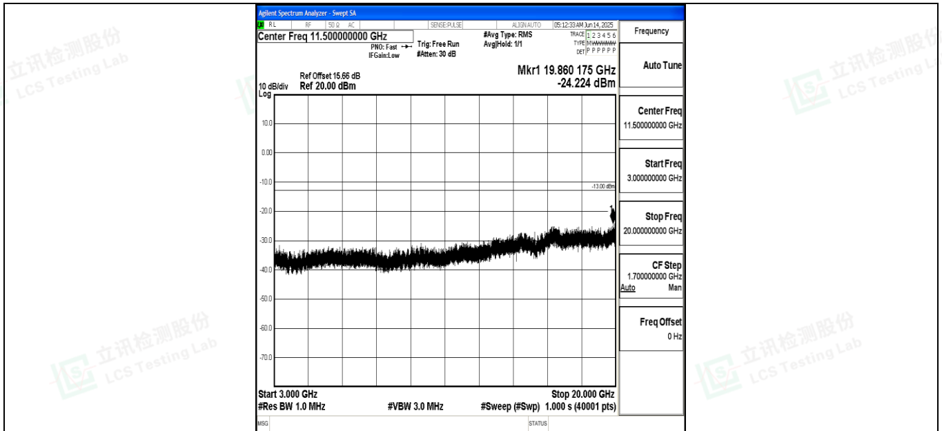
Band4_5MHz_QPSK_20375_1RB#0_3000~20000_3000~20000
