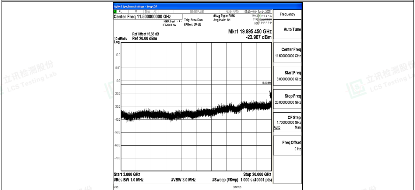
Band4_5MHz_16QAM_19975_1RB#0_3000~20000_3000~20000
