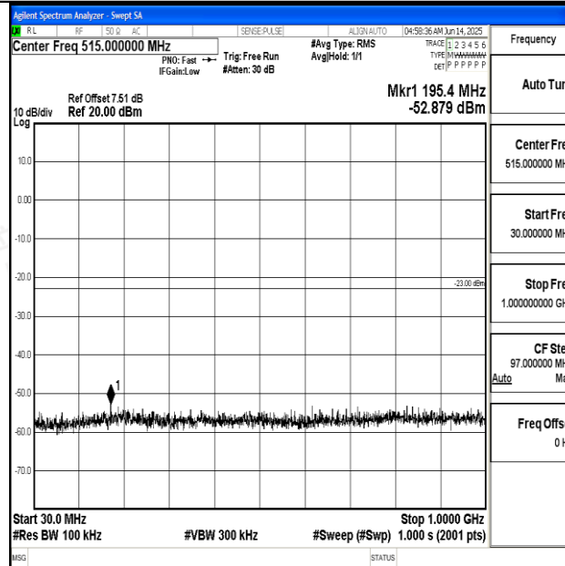
Band2_20MHz_16QAM_18900_1RB#0_30~1000_30~1000
