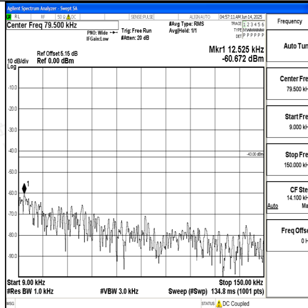
Band2_20MHz_16QAM_18700_1RB#0_0.009~0.15_0.009~0.15
