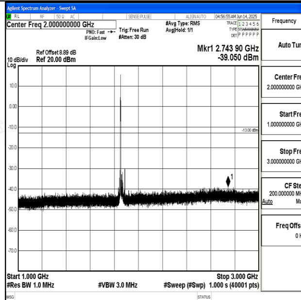
Band2_20MHz_QPSK_18700_1RB#0_1000~3000_1000~3000
