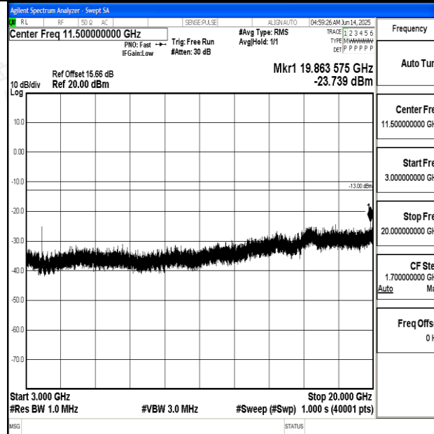
Band2_20MHz_QPSK_19100_1RB#0_3000~20000_3000~20000
