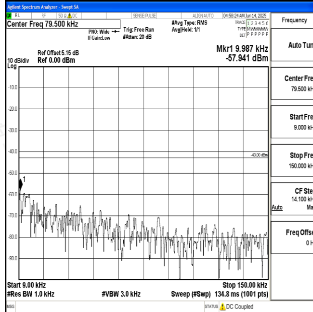
Band2_20MHz_16QAM_18900_1RB#0_0.009~0.15_0.009~0.15
