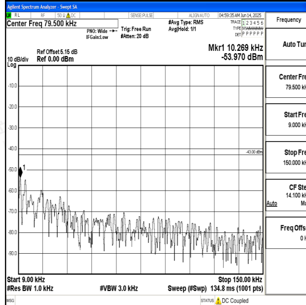
Band2_20MHz_16QAM_19100_1RB#0_0.009~0.15_0.009~0.15
