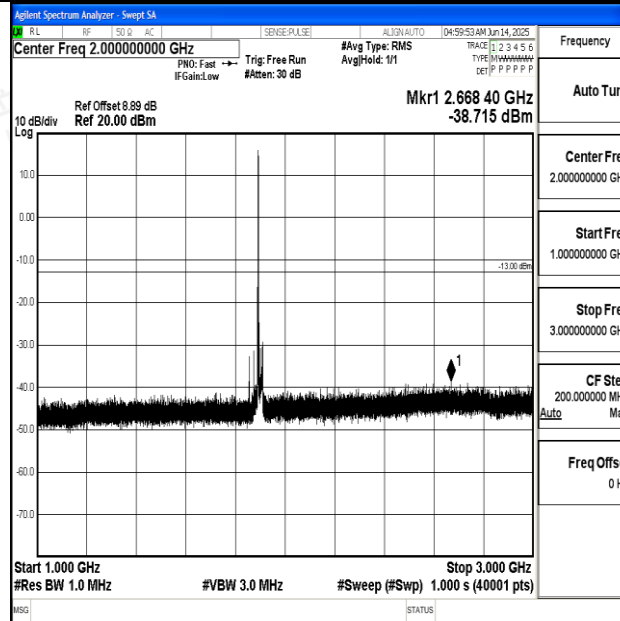
Band2_20MHz_16QAM_19100_1RB#0_1000~3000_1000~3000
