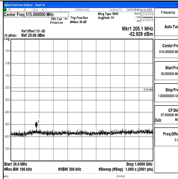
Band2_20MHz_QPSK_18900_1RB#0_30~1000_30~1000
