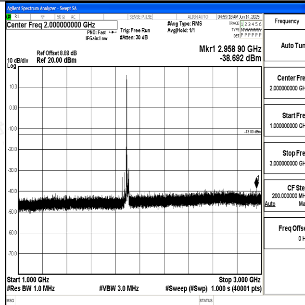
Band2_20MHz_QPSK_19100_1RB#0_1000~3000_1000~3000
