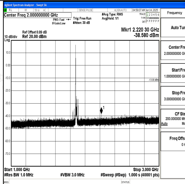
Band2_20MHz_QPSK_18900_1RB#0_1000~3000_1000~3000
