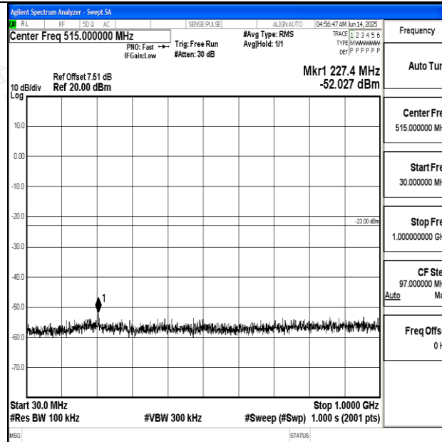
Band2_20MHz_QPSK_18700_1RB#0_30~1000_30~1000
