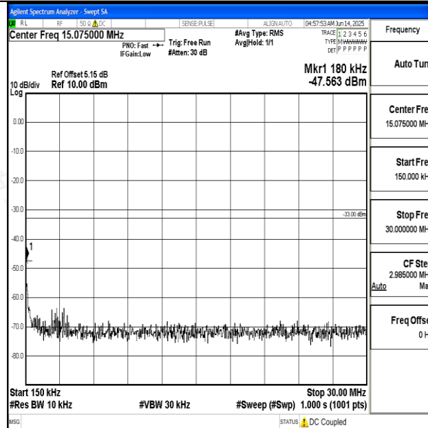
Band2_20MHz_QPSK_18900_1RB#0_0.15~30_0.15~30
