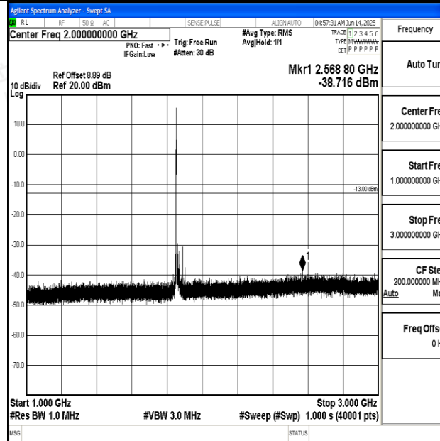
Band2_20MHz_16QAM_18700_1RB#0_1000~3000_1000~3000
