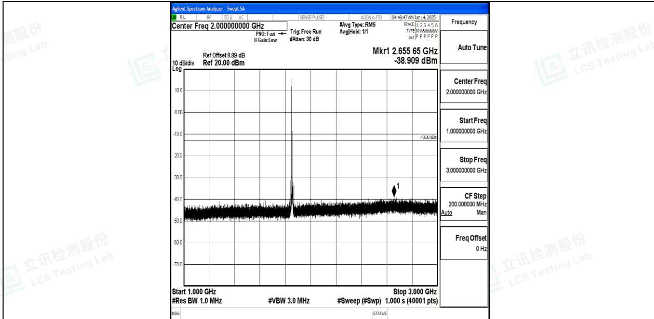
Band2_10MHz_16QAM_18650_1RB#0_1000~3000_1000~3000
