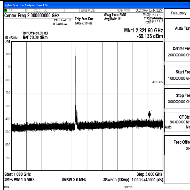
Band2_15MHz_QPSK_18675_1RB#0_1000~3000_1000~3000
