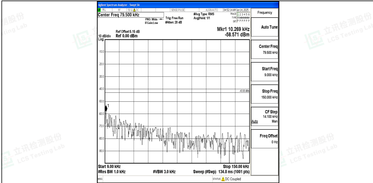
Band2_15MHz_QPSK_18675_1RB#0_0.009~0.15_0.009~0.15
