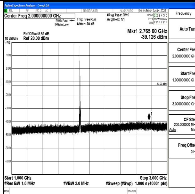
Band2_5MHz_QPSK_18900_1RB#0_1000~3000_1000~3000
