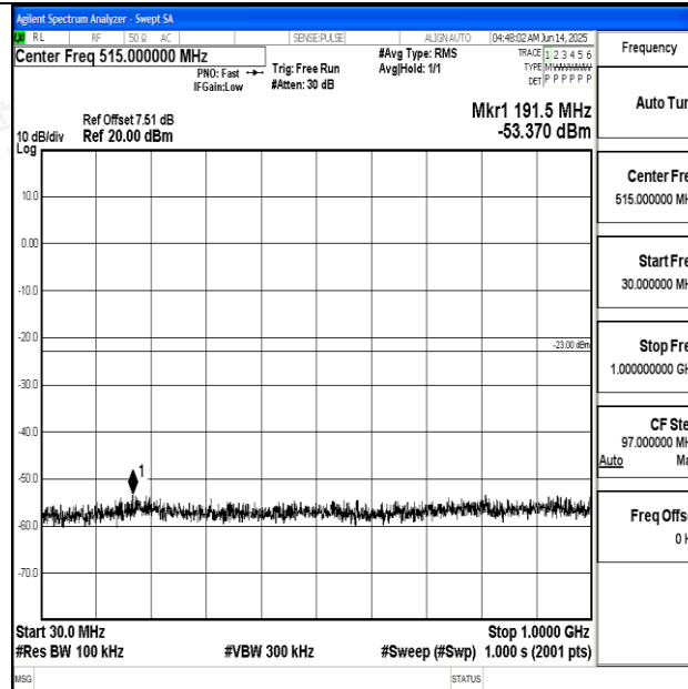
Band2_10MHz_QPSK_18650_1RB#0_30~1000_30~1000
