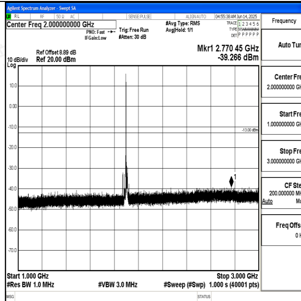
Band2_15MHz_16QAM_19125_1RB#0_1000~3000_1000~3000
