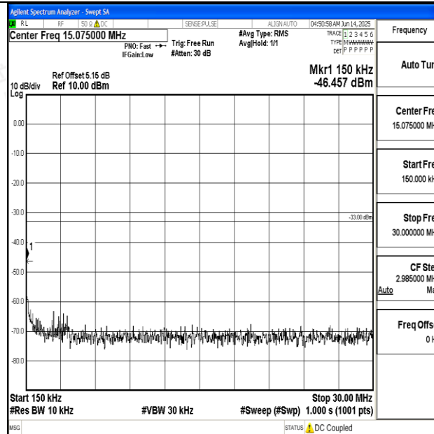
Band2_10MHz_16QAM_19150_1RB#0_0.15~30_0.15~30
