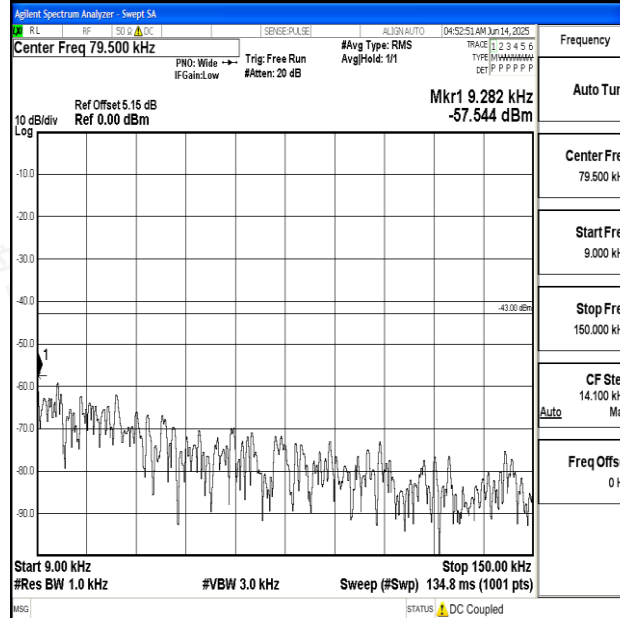
Band2_15MHz_16QAM_18675_1RB#0_0.009~0.15_0.009~0.15
