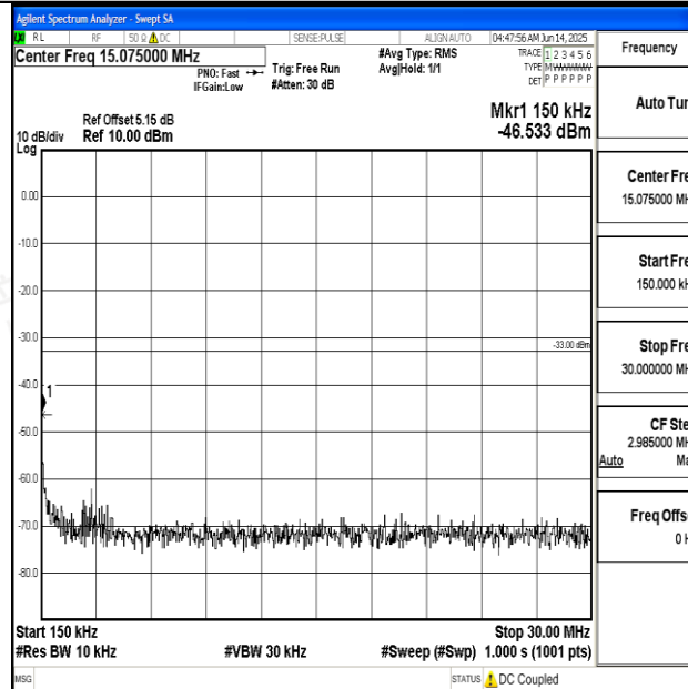
Band2_10MHz_QPSK_18650_1RB#0_0.15~30_0.15~30
