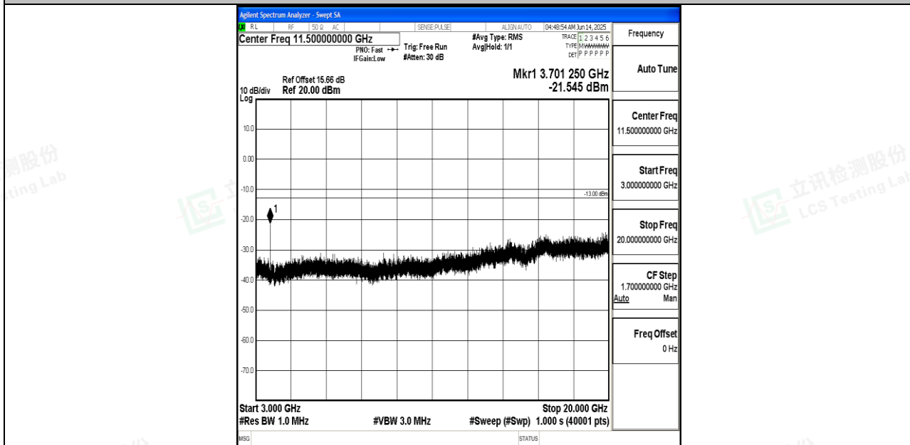
Band2_10MHz_16QAM_18650_1RB#0_3000~20000_3000~20000
