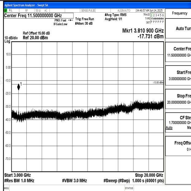
Band2_5MHz_16QAM_19175_1RB#0_3000~20000_3000~20000
