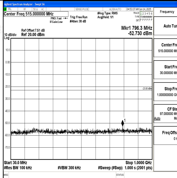
Band2_15MHz_QPSK_18900_1RB#0_30~1000_30~1000
