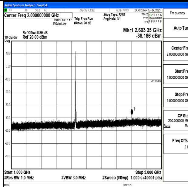
Band2_10MHz_QPSK_18650_1RB#0_1000~3000_1000~3000
