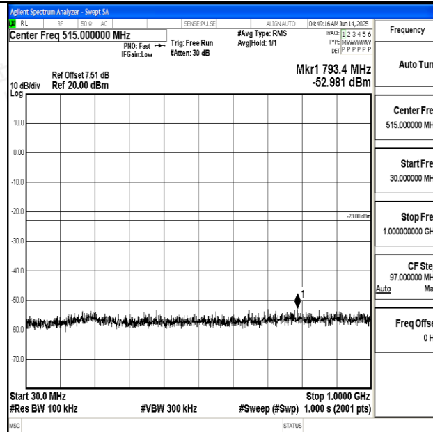
Band2_10MHz_QPSK_18900_1RB#0_30~1000_30~1000
