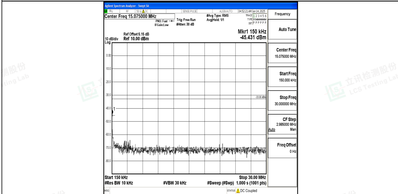
Band2_15MHz_QPSK_18675_1RB#0_0.15~30_0.15~30
