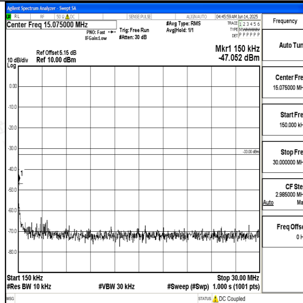
Band2_5MHz_QPSK_19175_1RB#0_0.15~30_0.15~30
