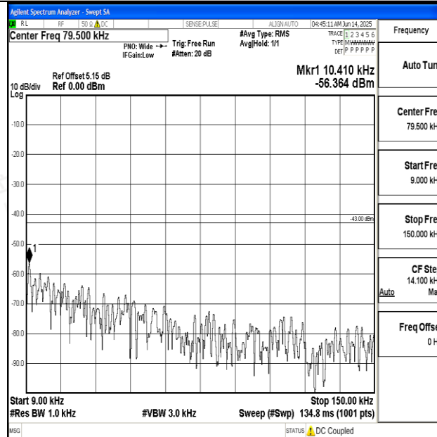
Band2_5MHz_16QAM_18900_1RB#0_0.009~0.15_0.009~0.15
