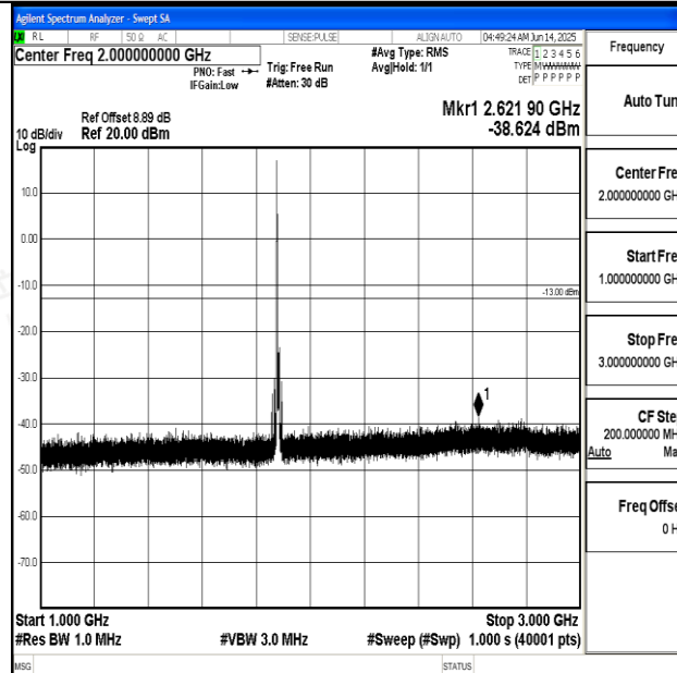
Band2_10MHz_QPSK_18900_1RB#0_1000~3000_1000~3000
