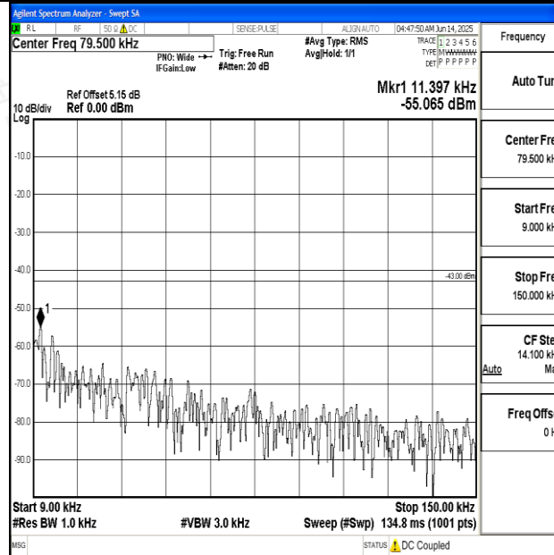
Band2_10MHz_QPSK_18650_1RB#0_0.009~0.15_0.009~0.15
