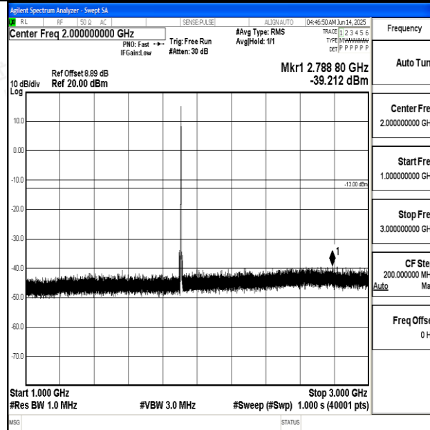
Band2_5MHz_16QAM_19175_1RB#0_1000~3000_1000~3000
