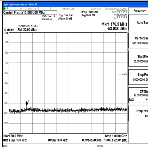
Band2 10MHz 16QAM 19150 1RB#0 30~1000 30~1000
