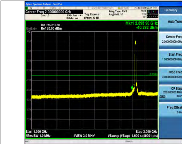
Band41_20MHz_QPSK_41140_100RB#0_18000~27000_18000~27000
