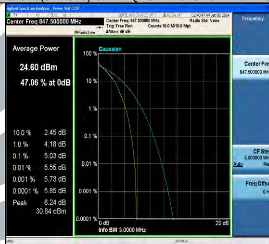
Band26(824-849)-3MHz-64QAM-26805-15RB#0-PASS
