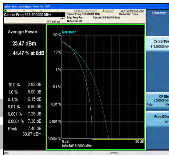
Band26(814-824)-5MHz-64QAM-26740-25RB#0-PASS
