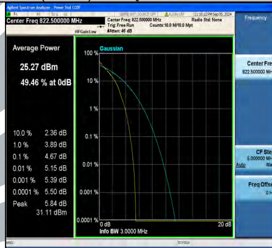
Band26(814-824)-3MHz-64QAM-26705-15RB#0-PASS
