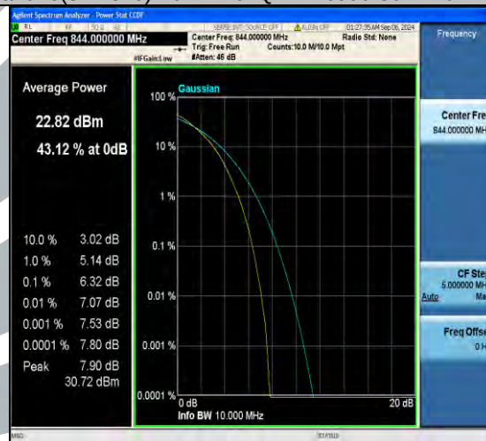
Band26(824-849)-10MHz-16QAM-26840-50RB#0-PASS
