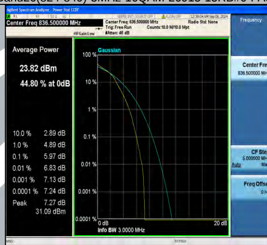
Band26(824-849)-3MHz-16QAM-27025-15RB#0-PASS
