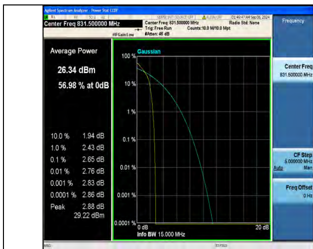
Band26(824-849)-15MHz-QPSK-26915-1RB#0-PASS
