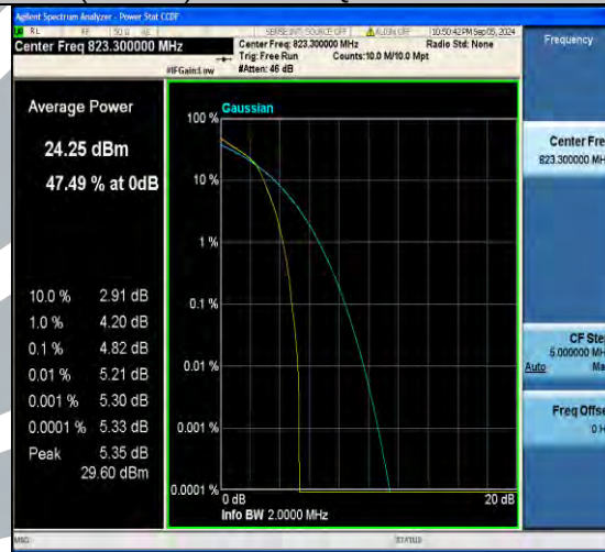
Band26(814-824)-3MHz-QPSK-26705-15RB#0-PASS
