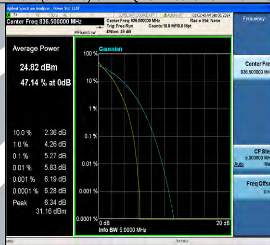
Band26(824-849)-5MHz-QPSK-27015-25RB#0-PASS
