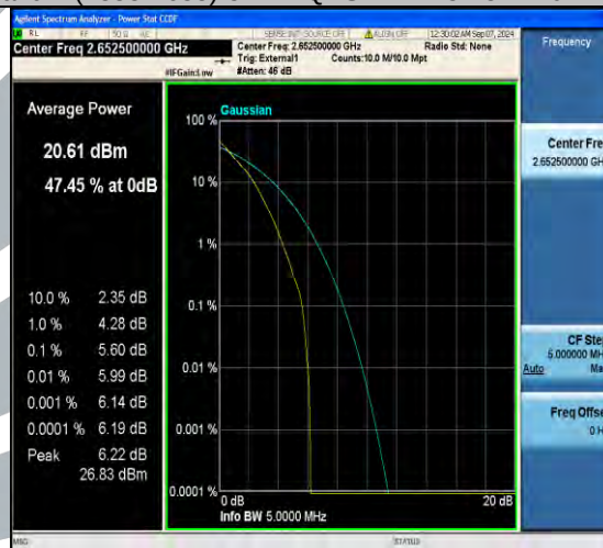
Band41(2555-2655)-5MHz-64QAM-40265-25RB#0-PASS
