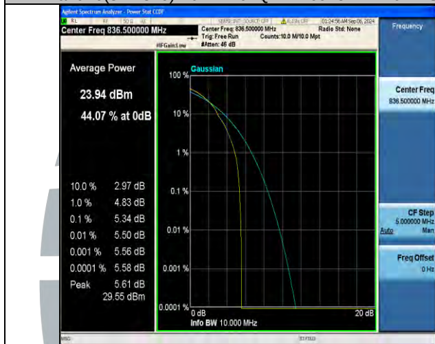
Band26(824-849)-10MHz-64QAM-26990-1RB#0-PASS
