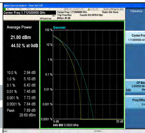
Band4-5MHz-64QAM-20175-25RB#0-PASS
