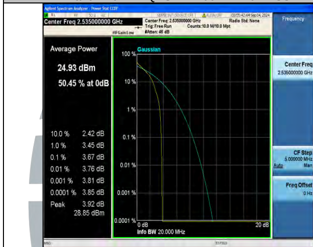
Band7-20MHz-QPSK-21350-1RB#0-PASS
