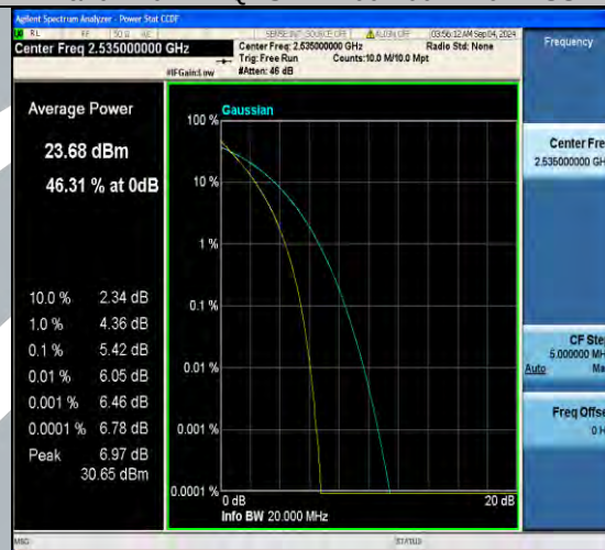
Band7-20MHz-QPSK-21350-100RB#0-PASS
