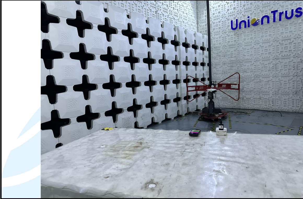
Radiated emission Test Setup (30 MHz~1 GHz) _Test Mode 1
