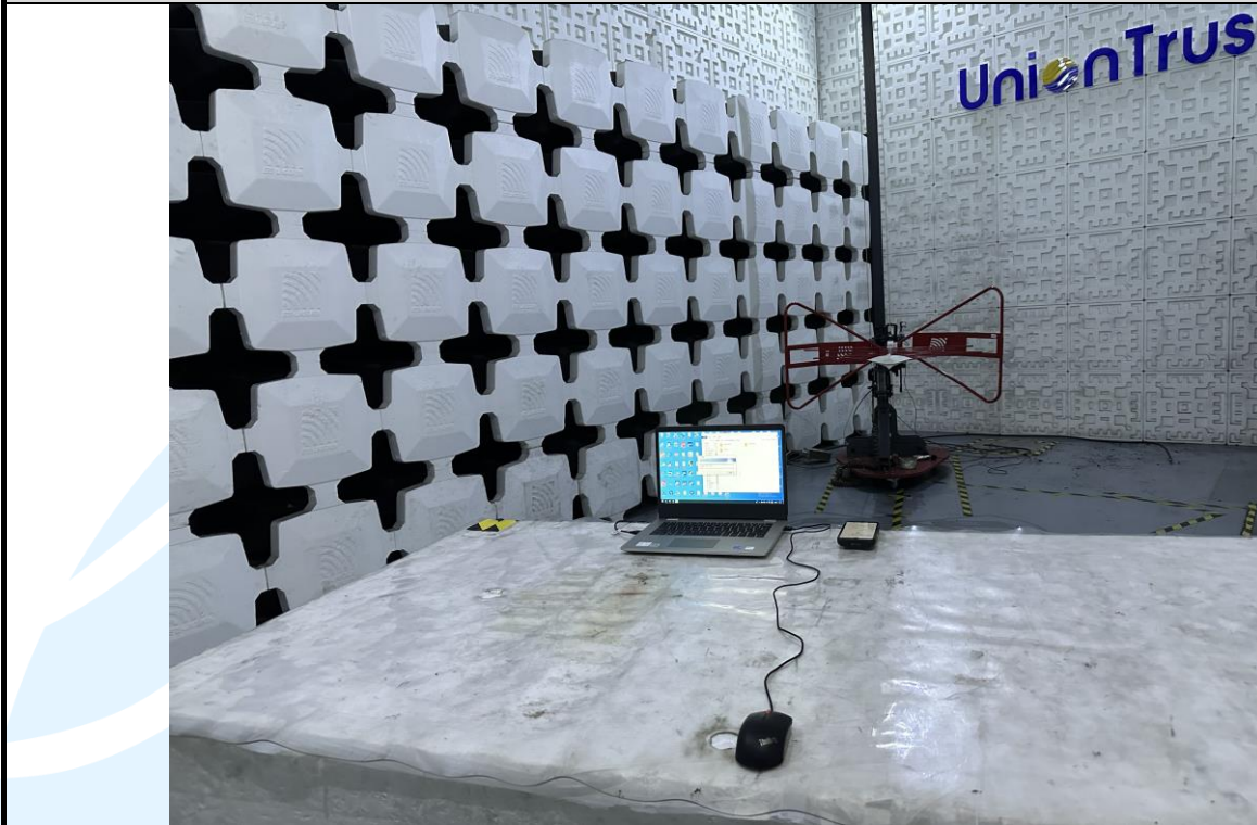
Radiated emission Test Setup (30 MHz~1 GHz) _Test Mode 8
