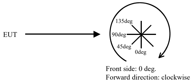
Figure 2: Antenna angle
