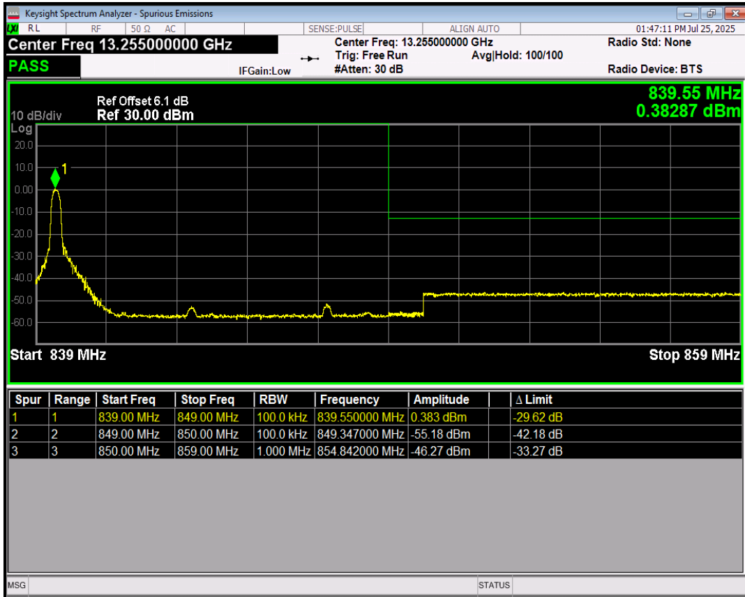
Band5 64QAM BW=10MHz Channel=20600 RB Size=1 Position=#Max
