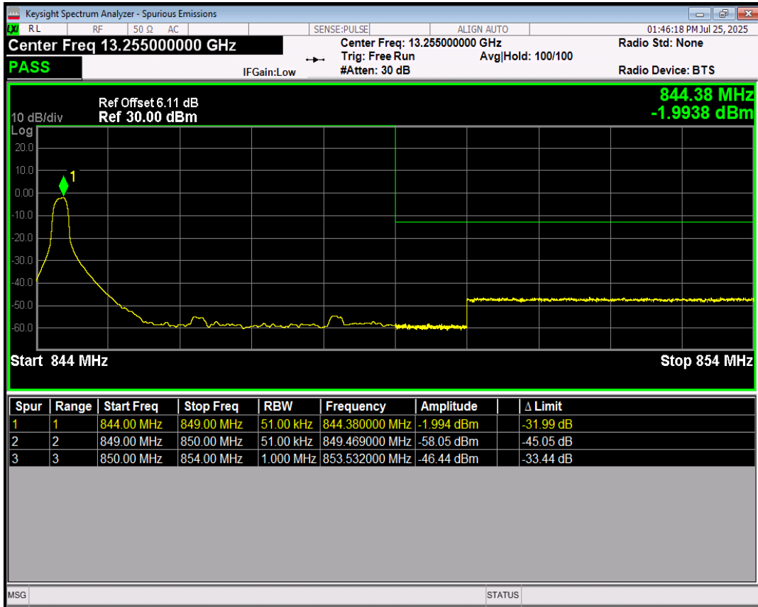
Band5 64QAM BW=5MHz Channel=20625 RB Size=1 Position=#Max
