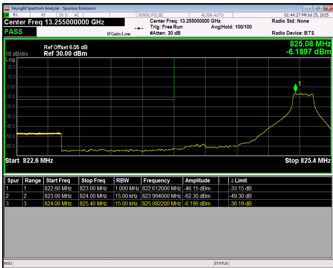
Band5 64QAM BW=1.4MHz Channel=20407 RB Size=6 Position=#0
